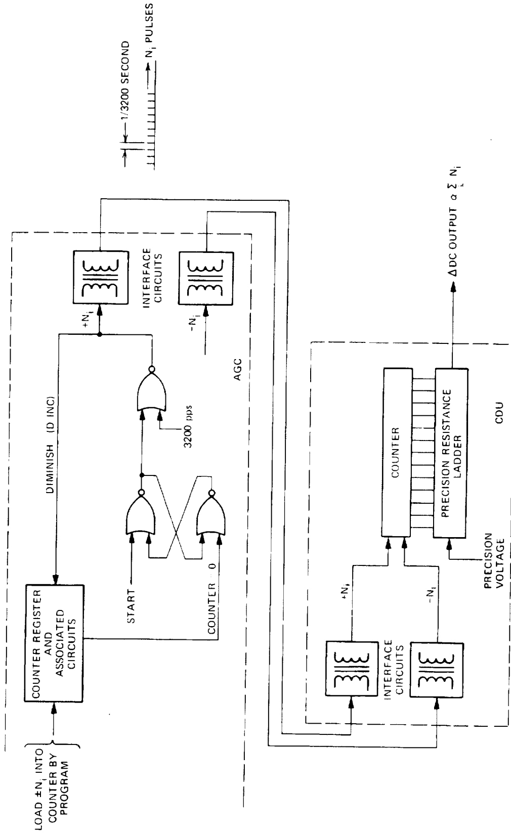
Fig. 3-20 Digital to Analog Conversion by Resistance Ladder
