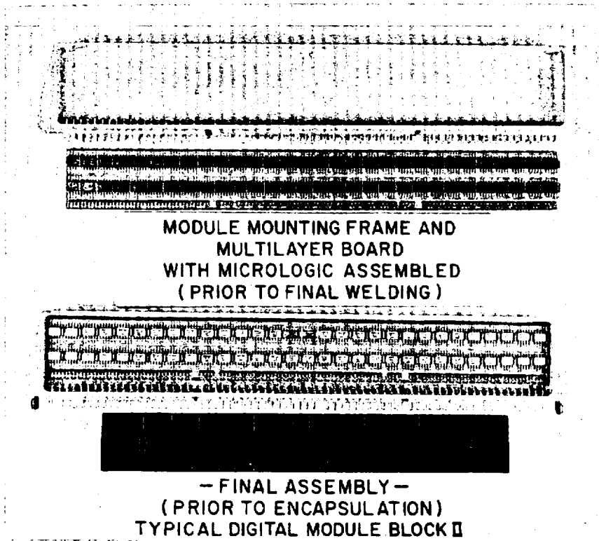
Fig. 2-9 Logic Module Containing 120 Microcircuit Units
