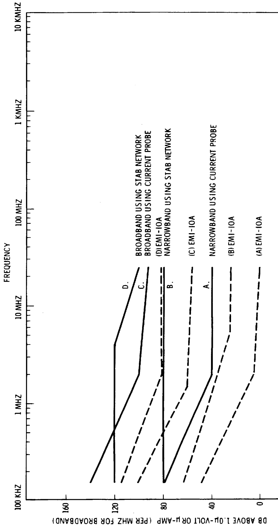
Fig. 6-9 Conducted Interference Test Limits
