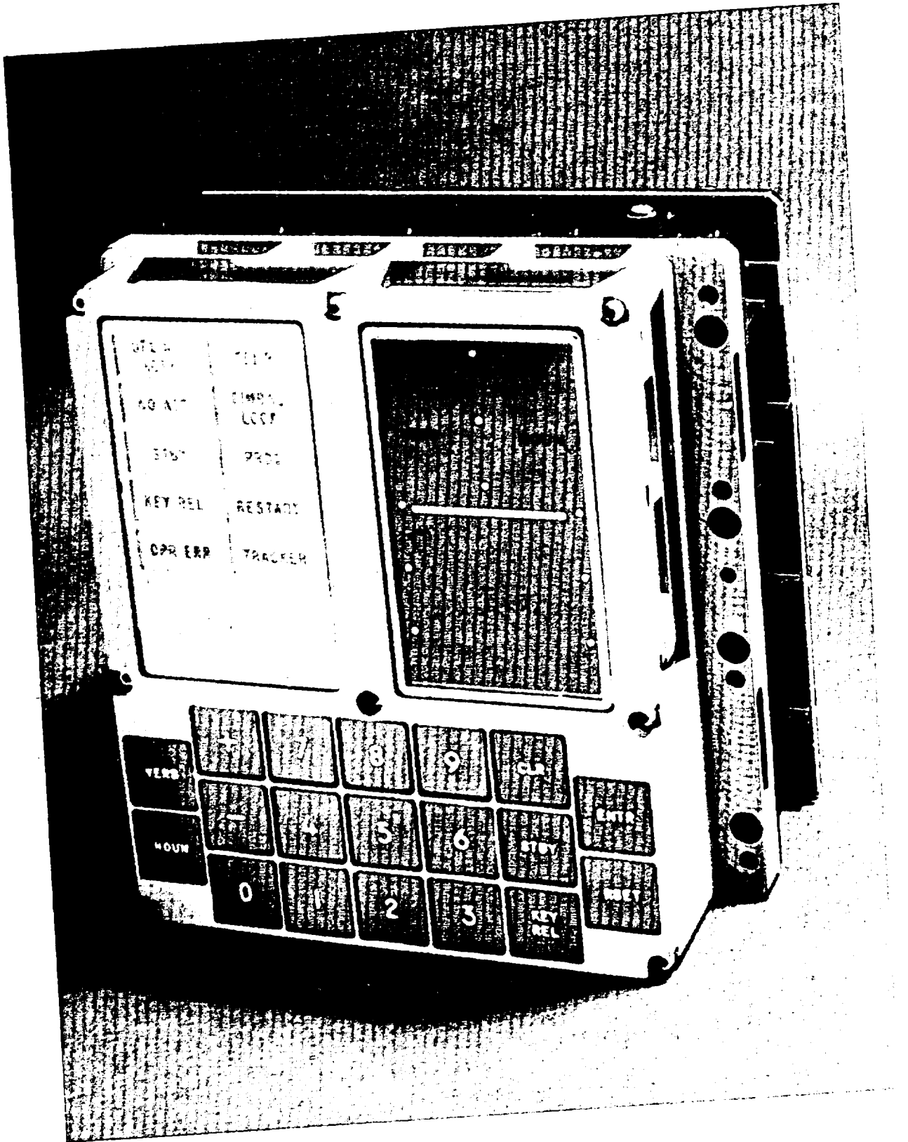
Fig. 2-5 DSKY Front Panel
