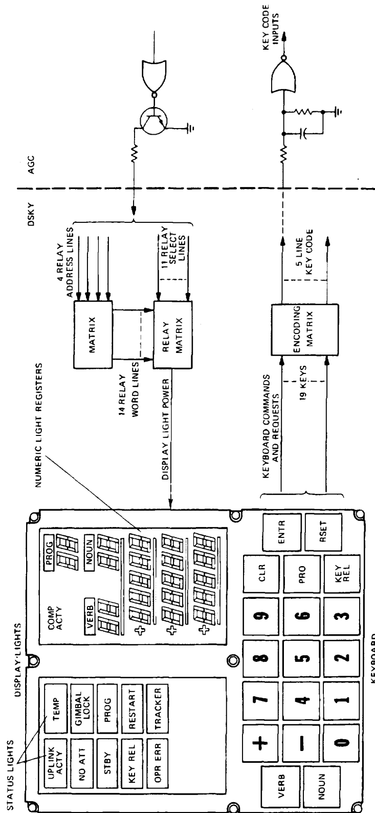
Fig. 3-25 DSKY Block Diagram
