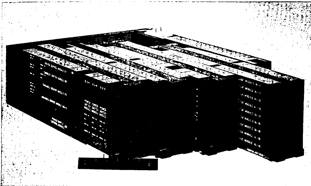
Fig. 1-7 Dual Computer Model
