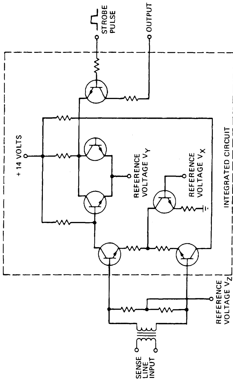
Fig. 3-11 Sense Amplifier Circuit
