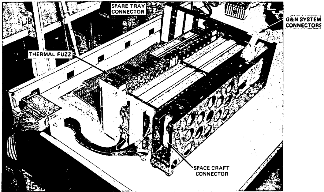
Fig. 1-6 Block 0 Computer
