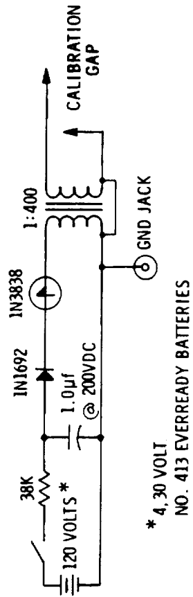
Fig. 6-13 Spark Generator for Radiated Transient Test
