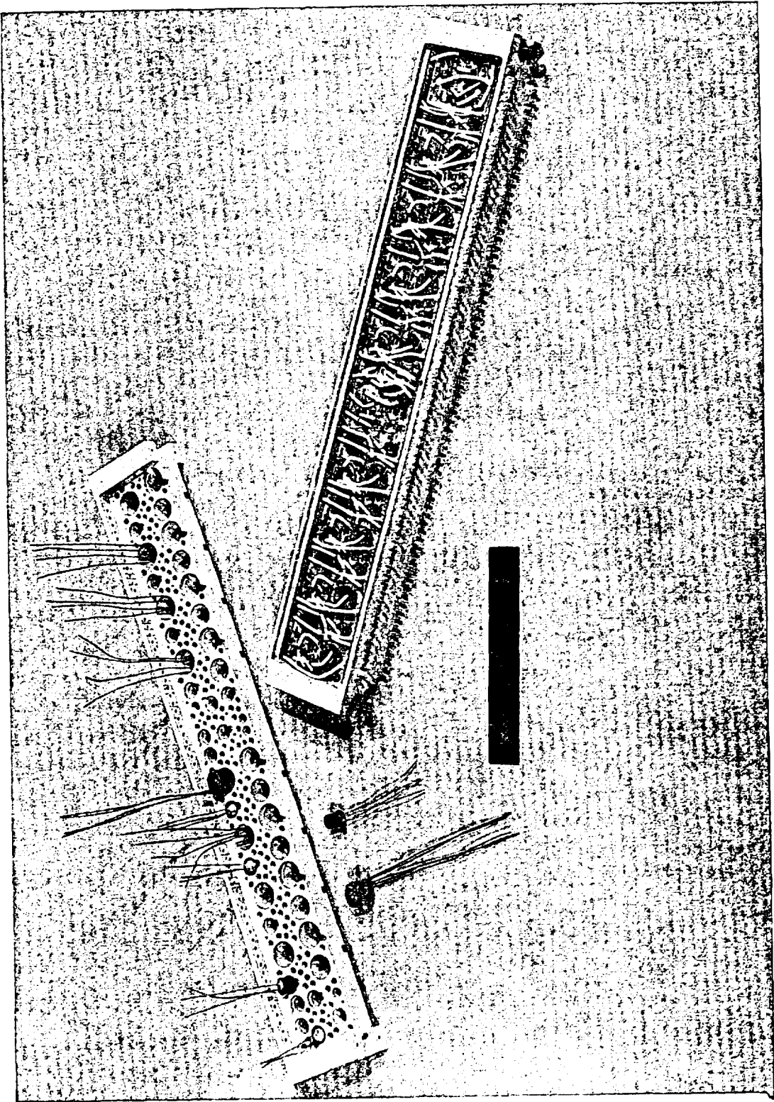
Fig. 3-32 Typical Welded Cordwood Construction
