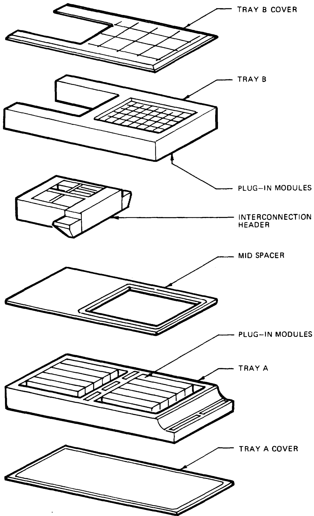
Fig. 3-27 Exploded View of Computer
