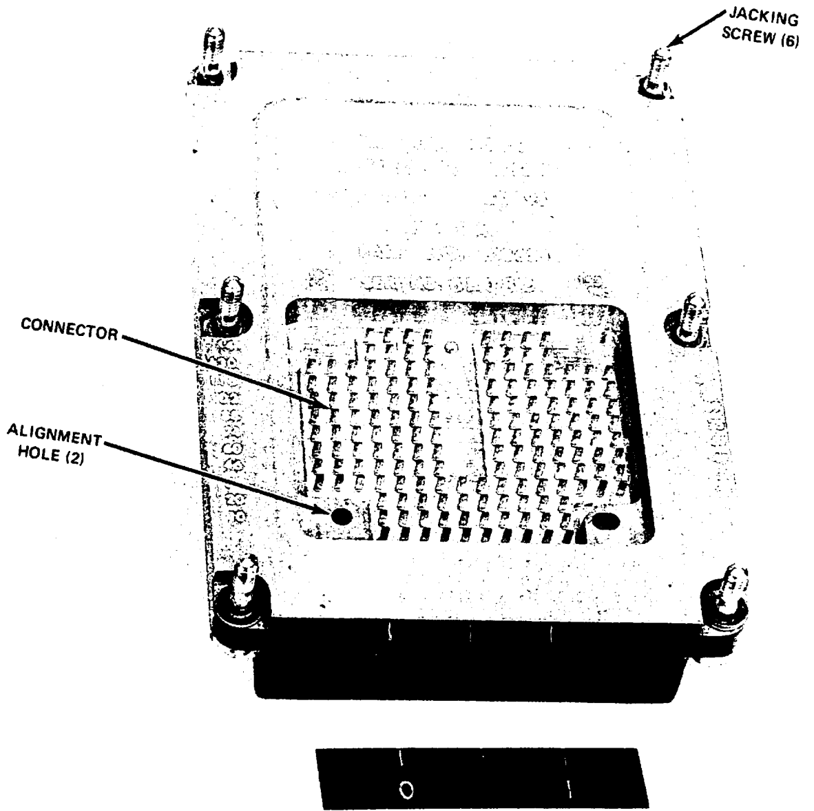
Fig. 3-45 Rear Side of Digital Indicator
