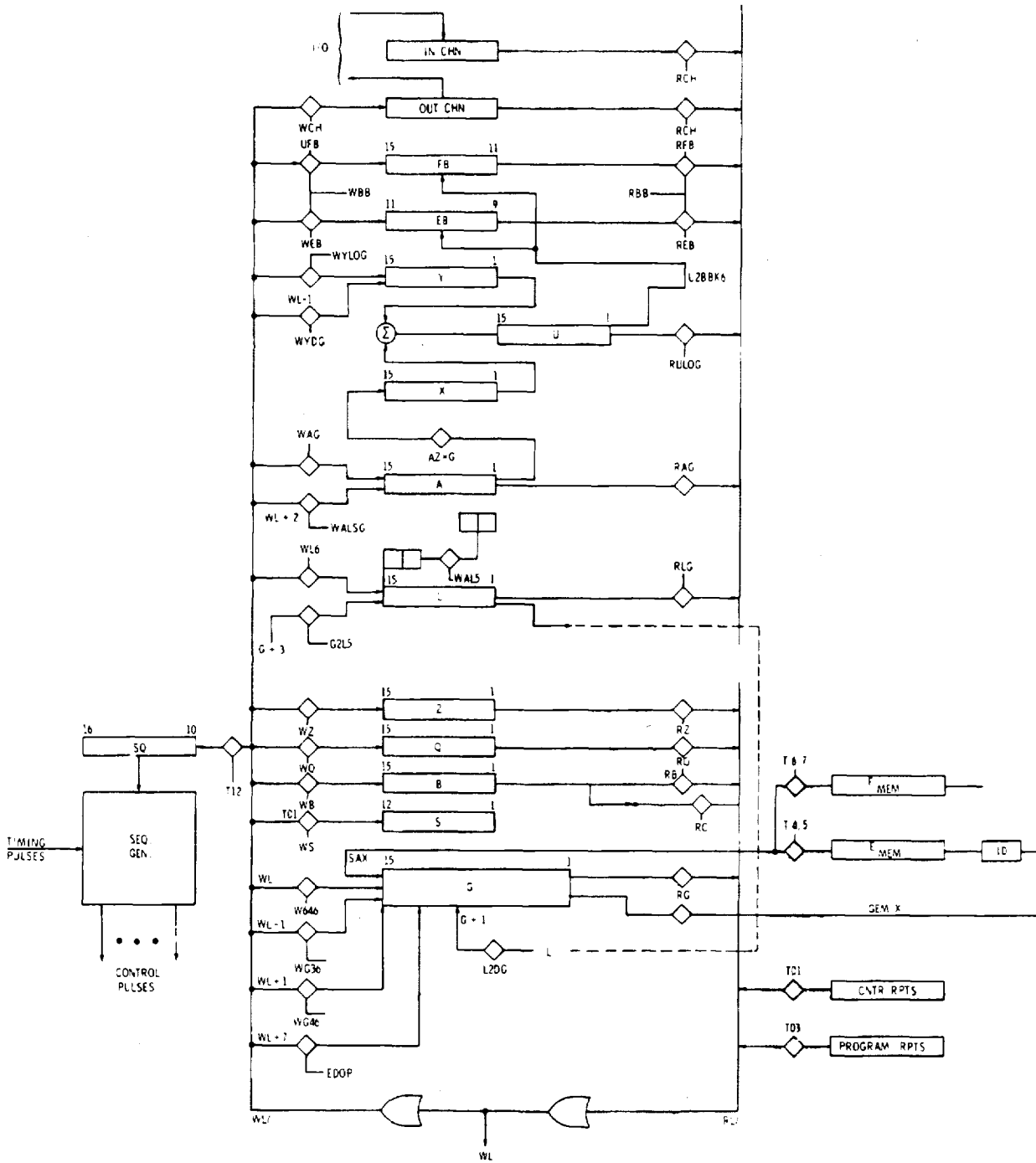
Fig. 3-5 Central Processor
