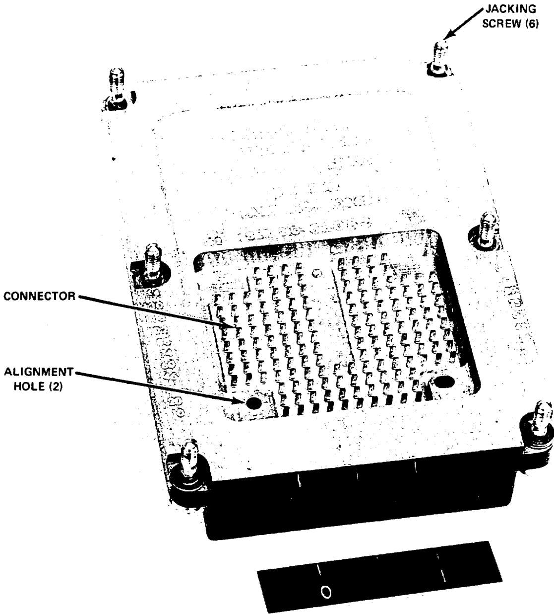
Fig. 3-45 Rear Side of Digital Indicator
