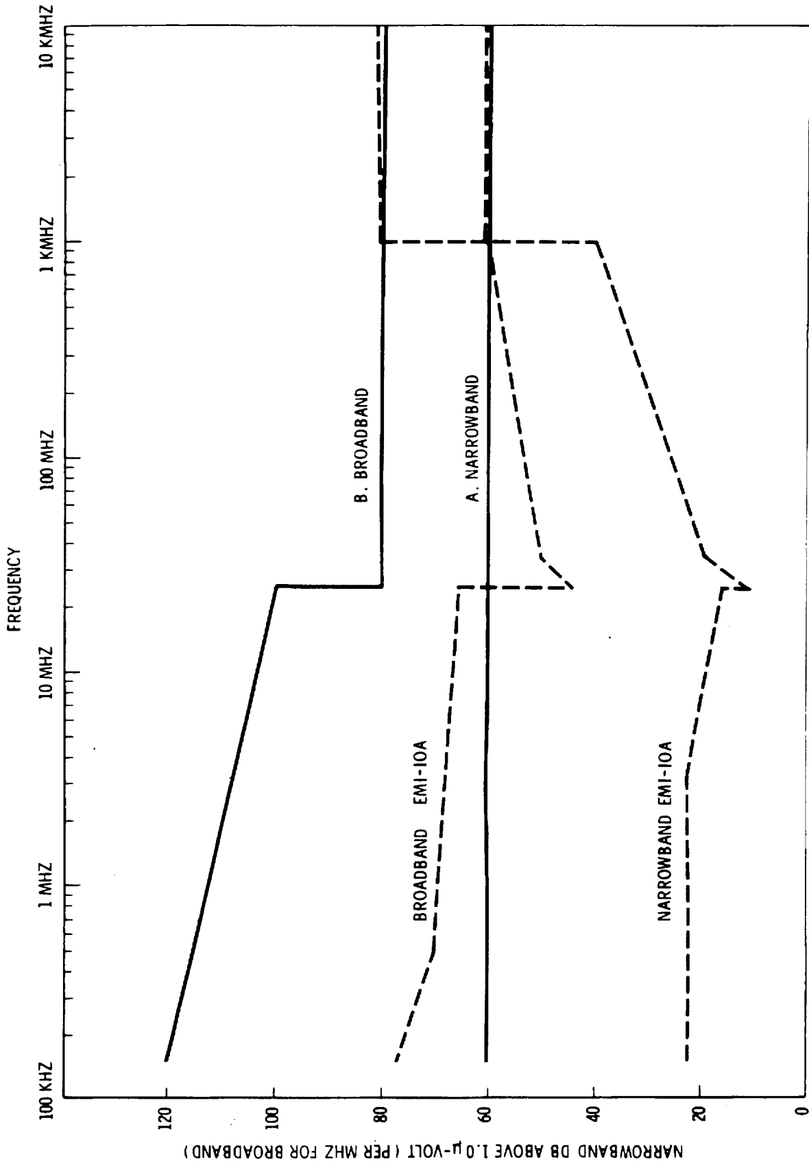
Fig. 6-11 Radiated Interference Test Limits - 150 KHz to 10 KMHz
