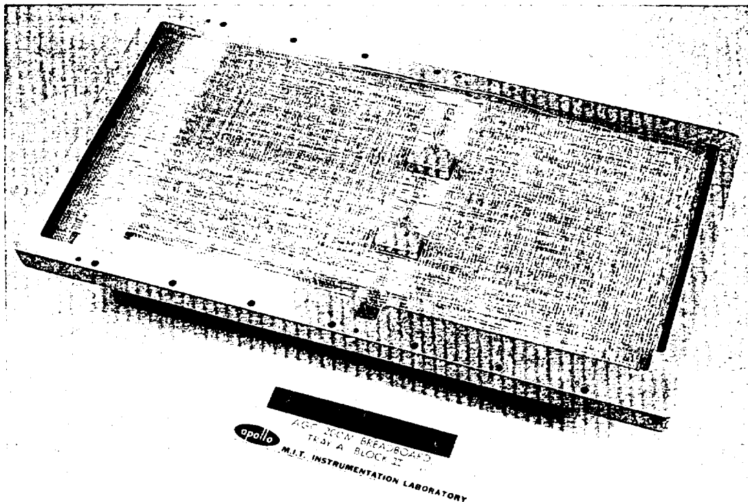
Fig. 2-10 Photograph of Wire-Wrapped Tray Connections
