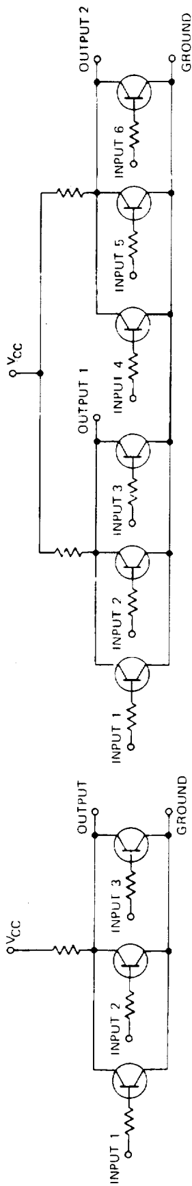
BLOCK I EQUIVALENT CIRCUIT
