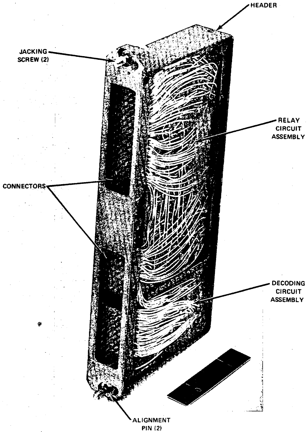
Fig. 3-41 Typical Indicator Driver Module
