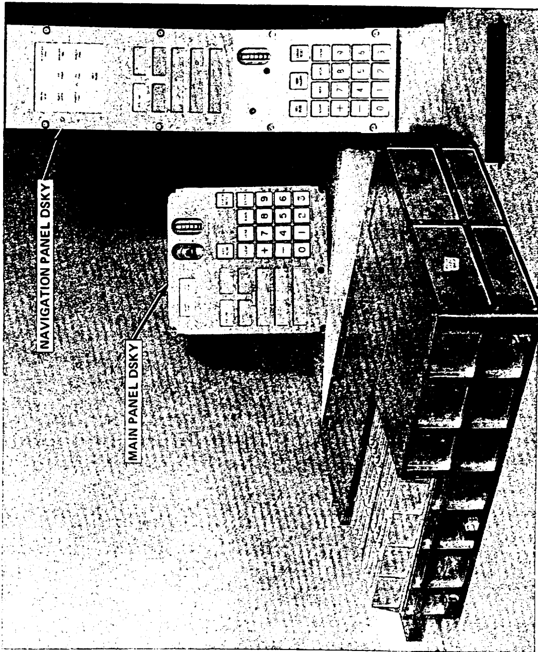
Fig. 1-8 Block I Computer and DSKYs
