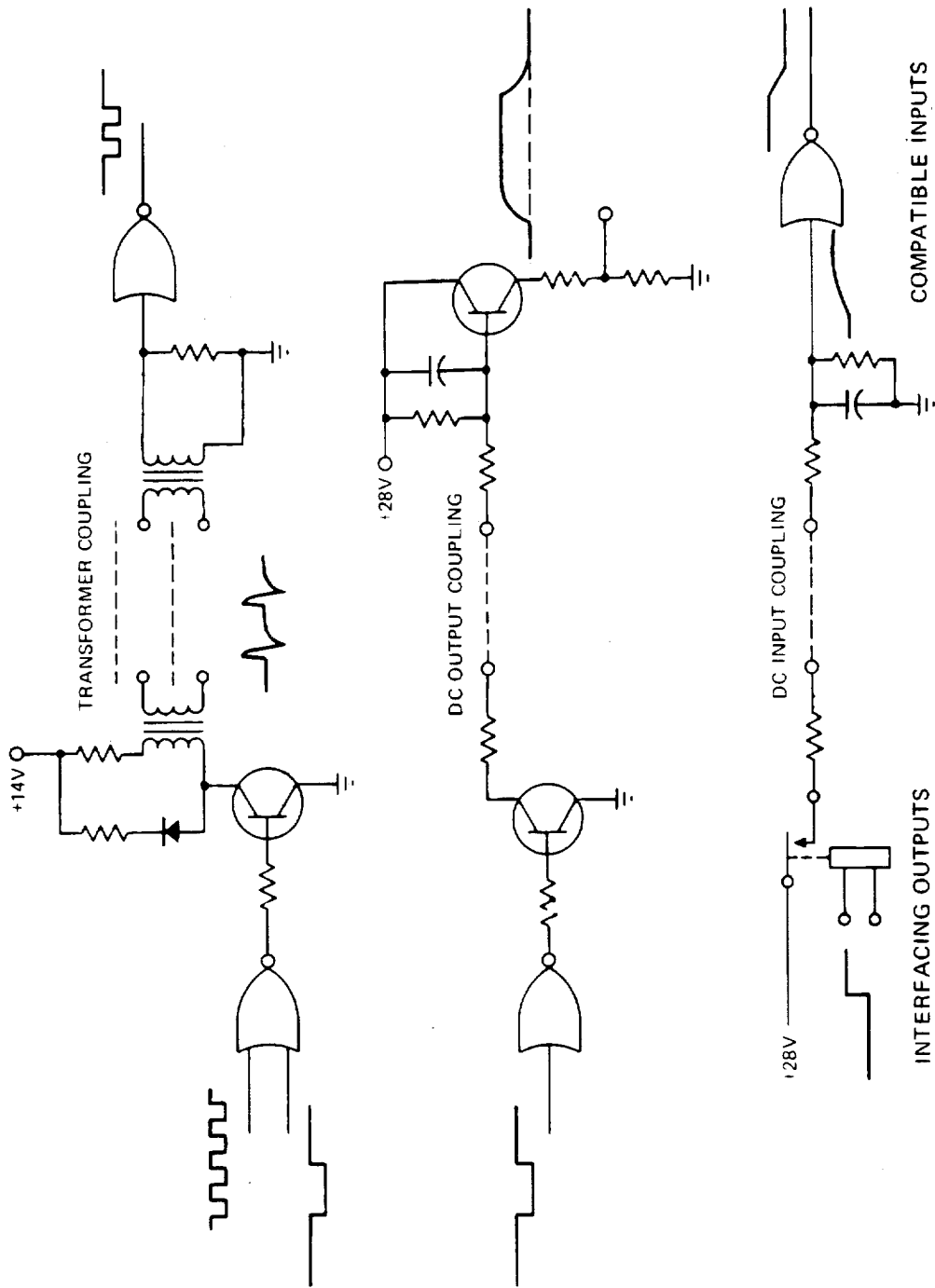
Fig. 3-17 Examples of Interface Circuits
