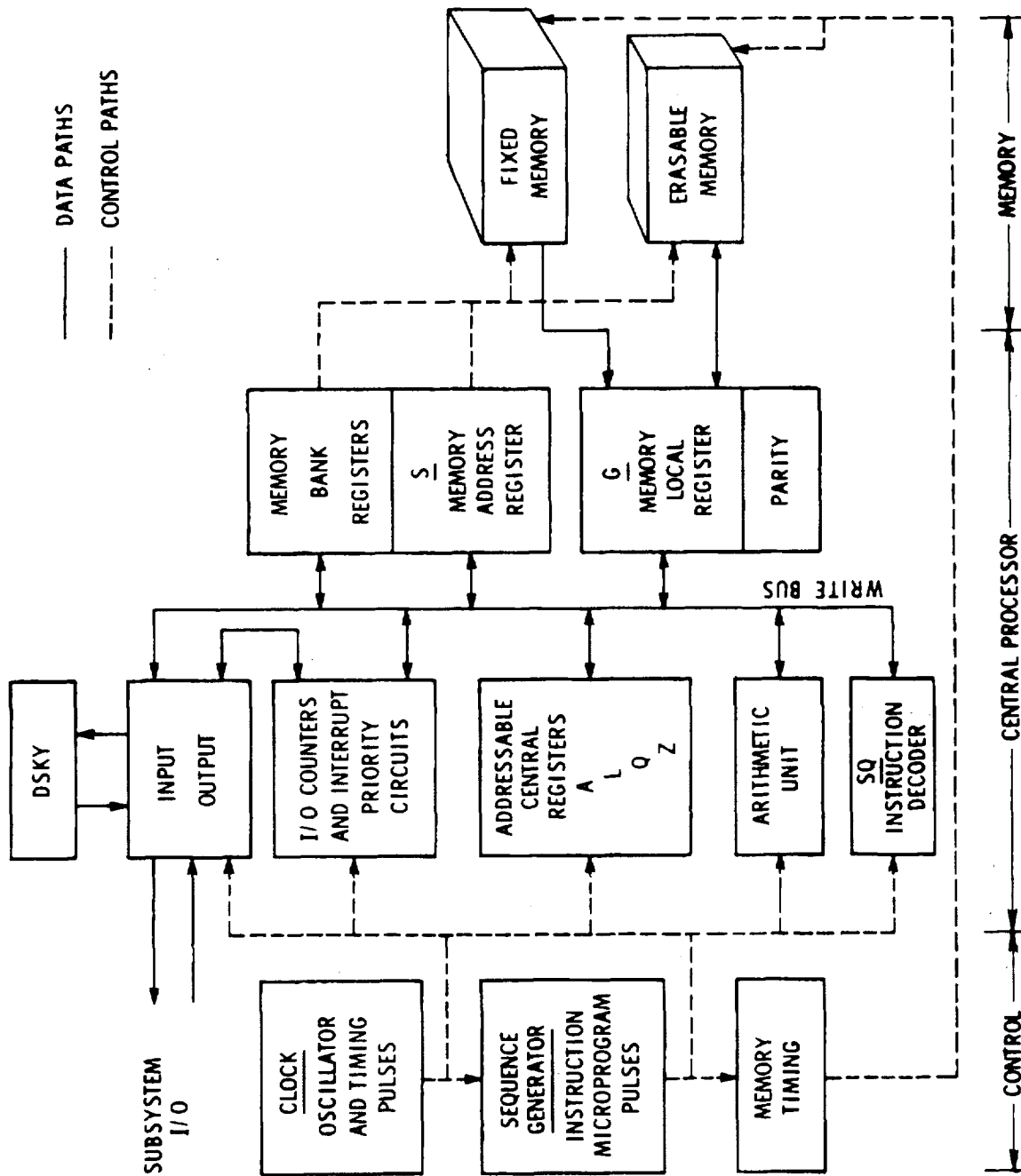
Fig. 2-4 Computer Simplified Block Diagram
