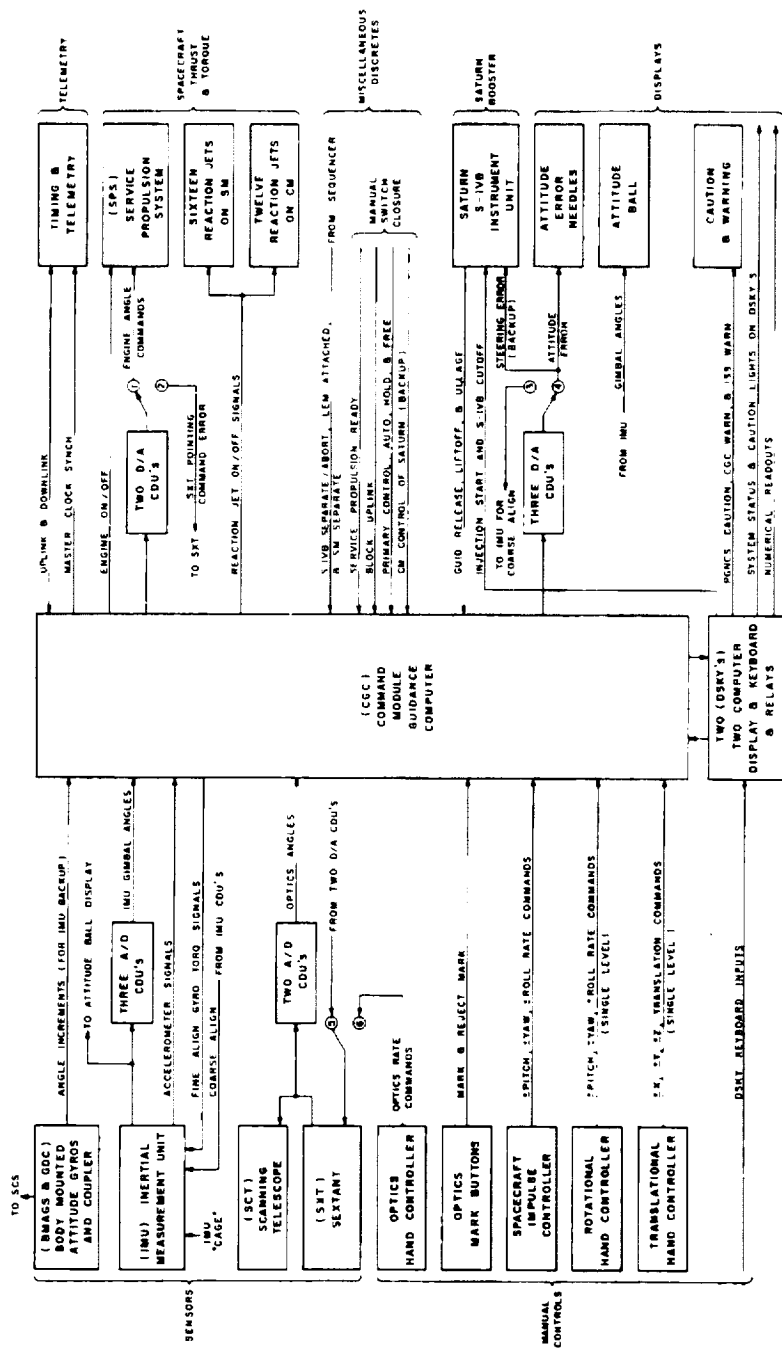
Fig. 3-15 GN&C Interconnections in Command Module
