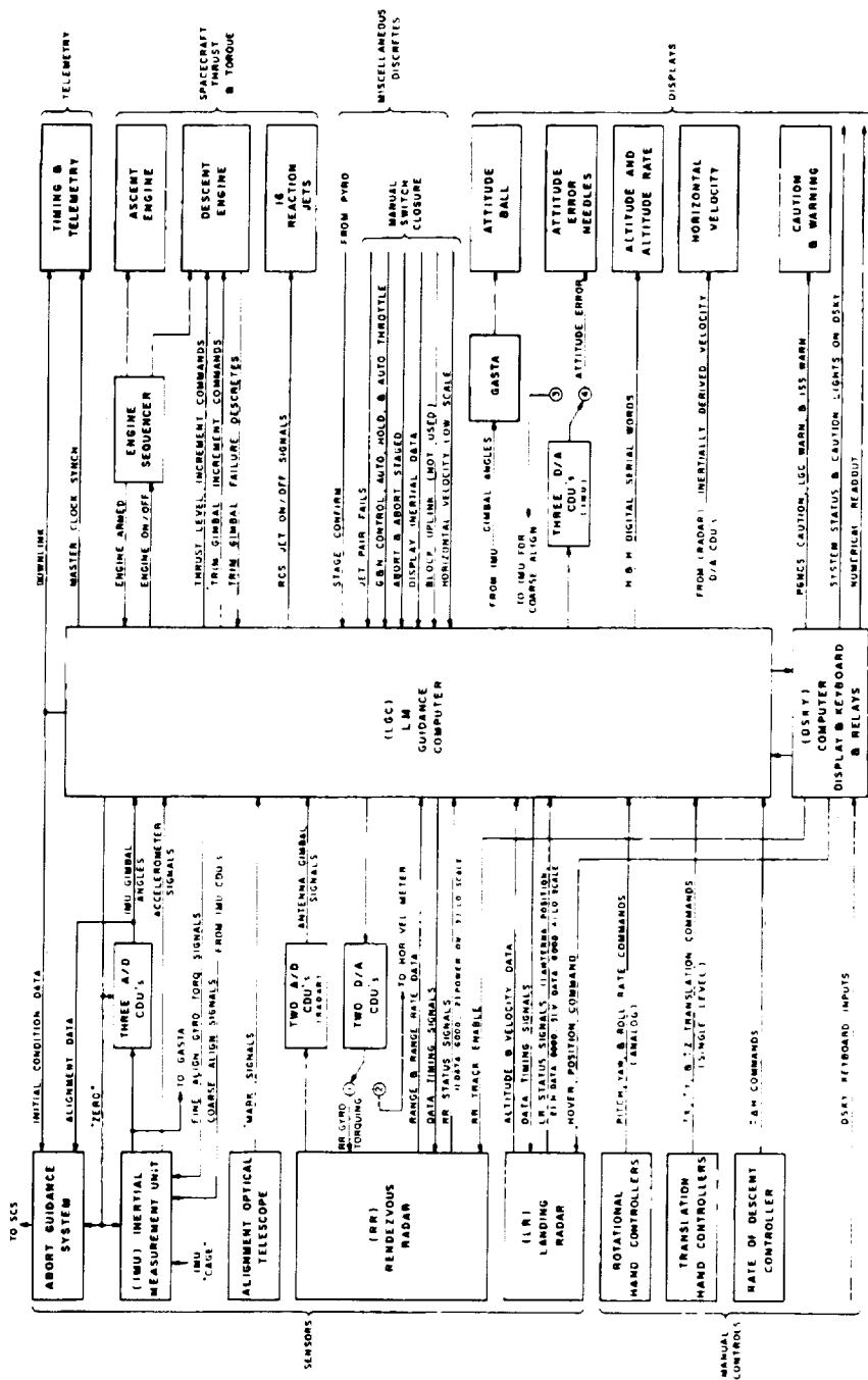
Fig. 3-16 GN&C Interconnections in Lunar Module
