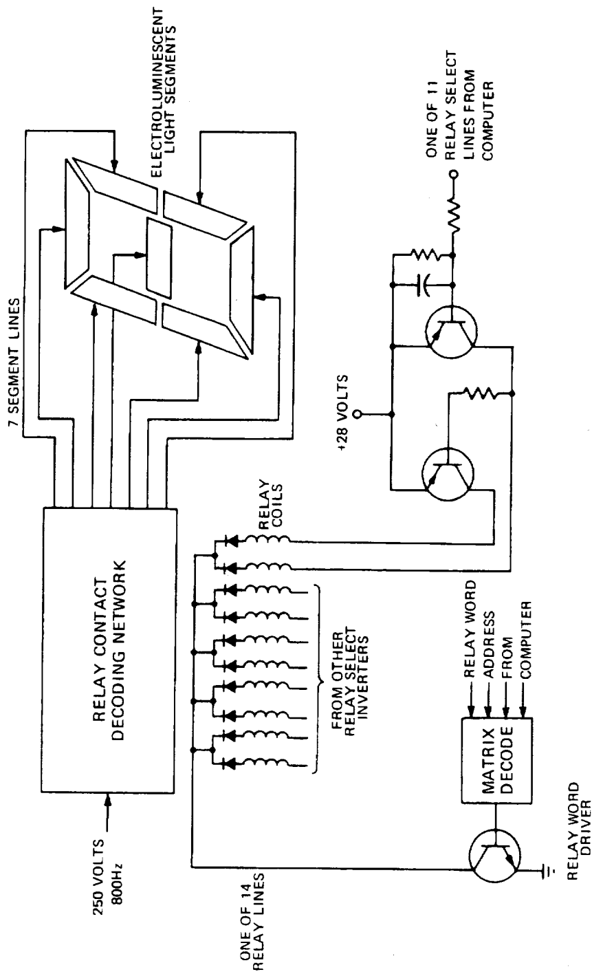
Fig. 3-24 DSKY Display Circuits - Simplified Diagram
