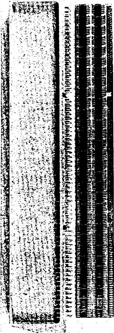
MODULE MOUNTING FRAME AND MULTILAYER BOARD WITH MICROLOGIC ASSEMBLED ( PRIOR TO FINAL WELDING )
