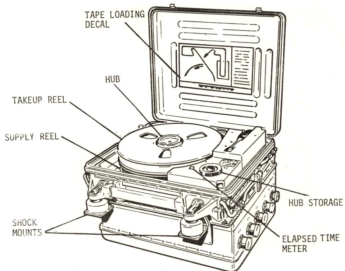
EREP Tape Recorder
