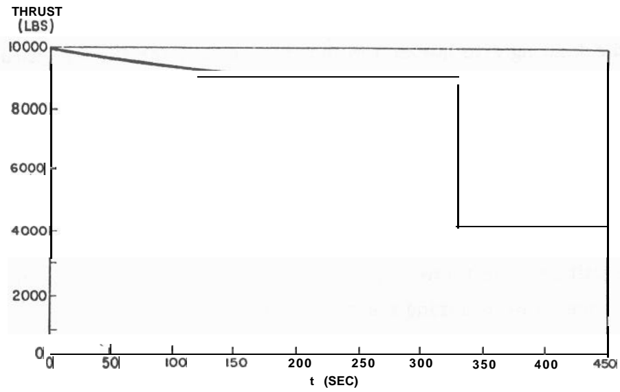
30498 Fig. 21 Thrust vs Time for Landing Trajectory
