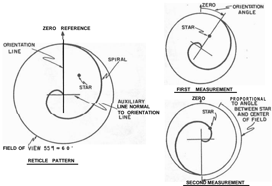
Fig. 8 AOT Reticle Pattern Lunar Surface IMU Alignment
