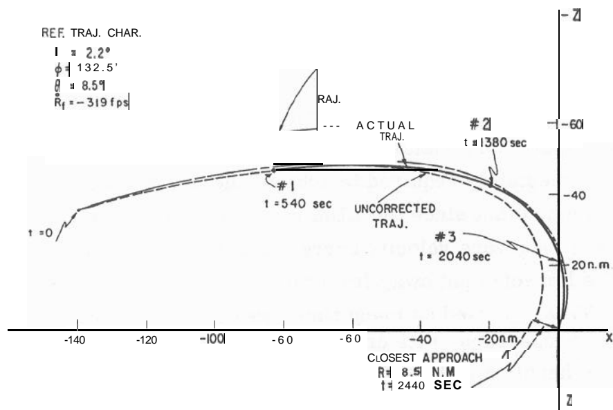
30471 Fig. 34 Rendezvous from Ascent - XZ Plane Trajectory Projection
