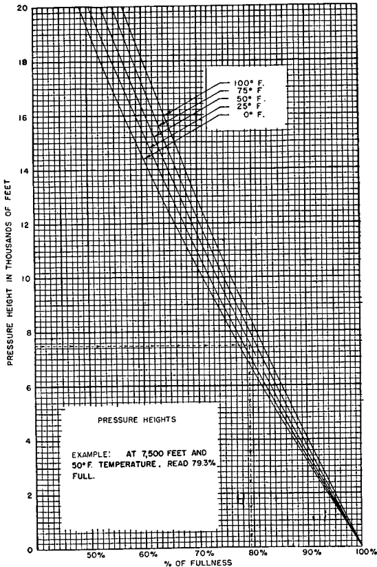
FIGURE 3.—Pressure height.
