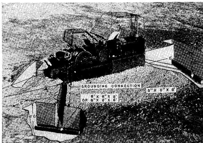
FIGURE 8.—Winch anchorages.
