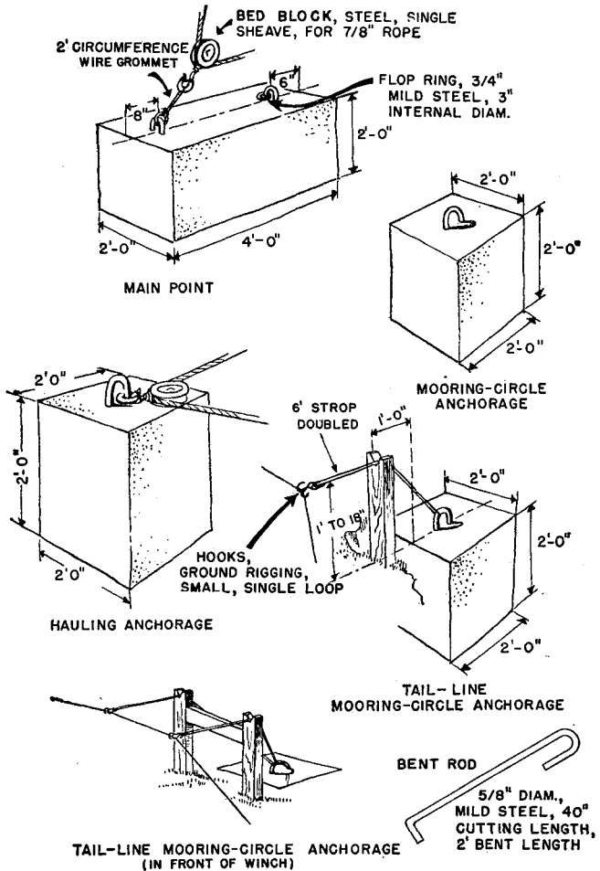
FIGURE 6.—Anchorage.
