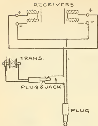
Type CP telephone.
