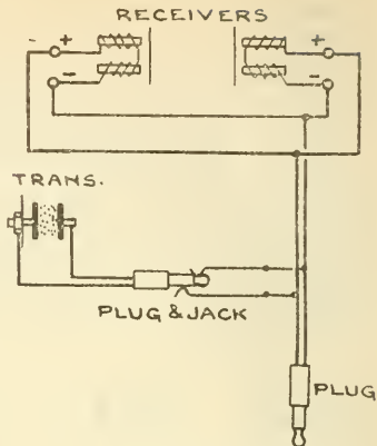
Type CS telephone.
