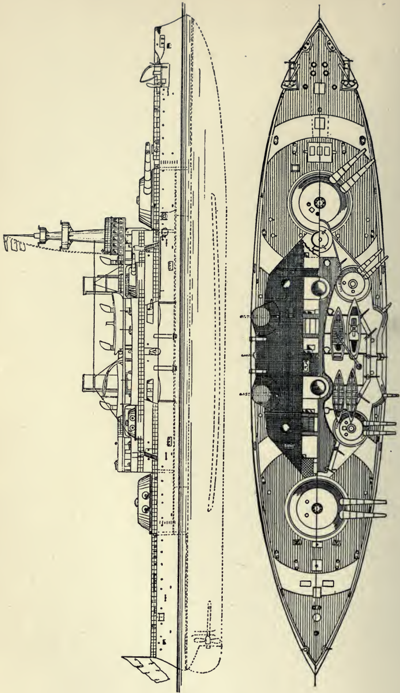
Main deck, superstructure, bridges and stowage of boats.
