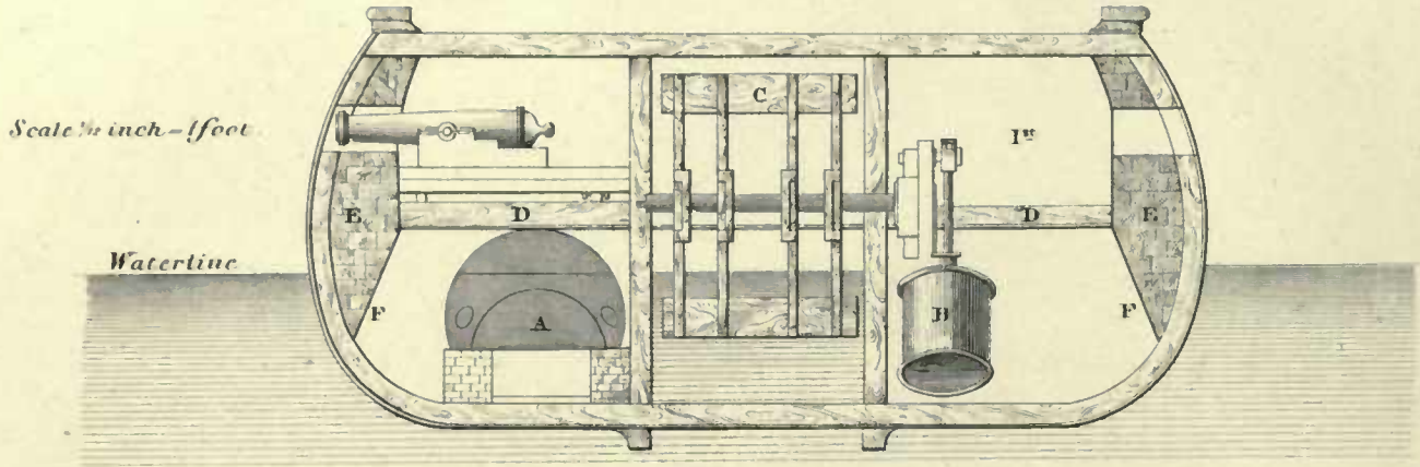
Figure I d Transverse section A her Boiler B the steam Engine C the water wheel . E E her wooden walls 5 feet thick, diminishing to below the waterline as at F F draught of water 9 feet D D her gun deck
