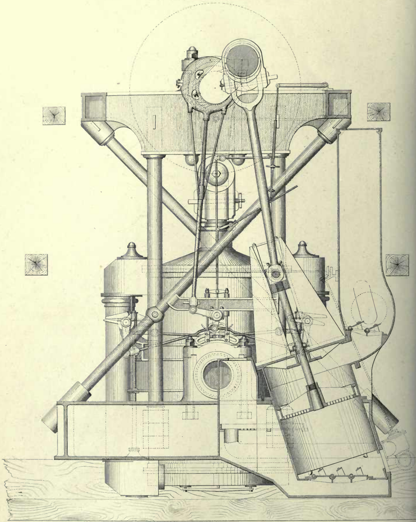
SIDE ELEVATION & SECTION thro' air pump.
