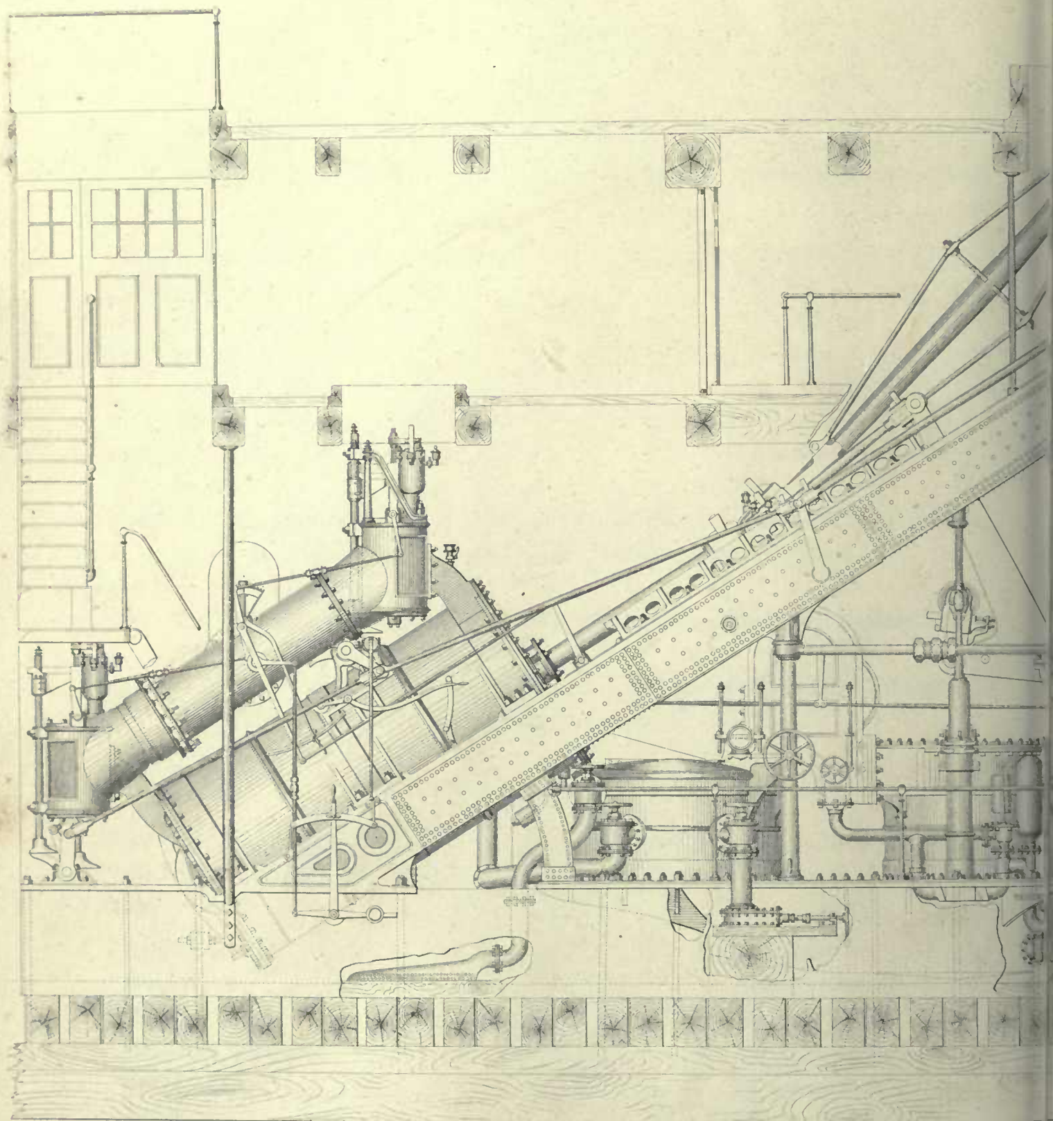
SIDE ELEVATION
