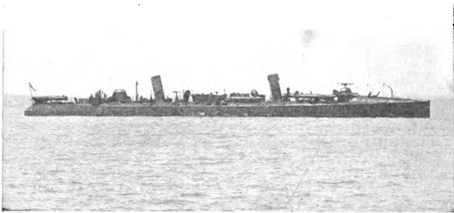
Foote , Torpedo-boat. 160 x 16; draft, 5; displacement, 142. Speed, 24.5 knots. Battery, three eighteen-inch torpedo tubes, three one-pounder guns.
