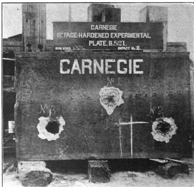
Kruppized Armor-plate Showing Effect of a 5.6-inch Projectile, Weighing 100 Pounds.
