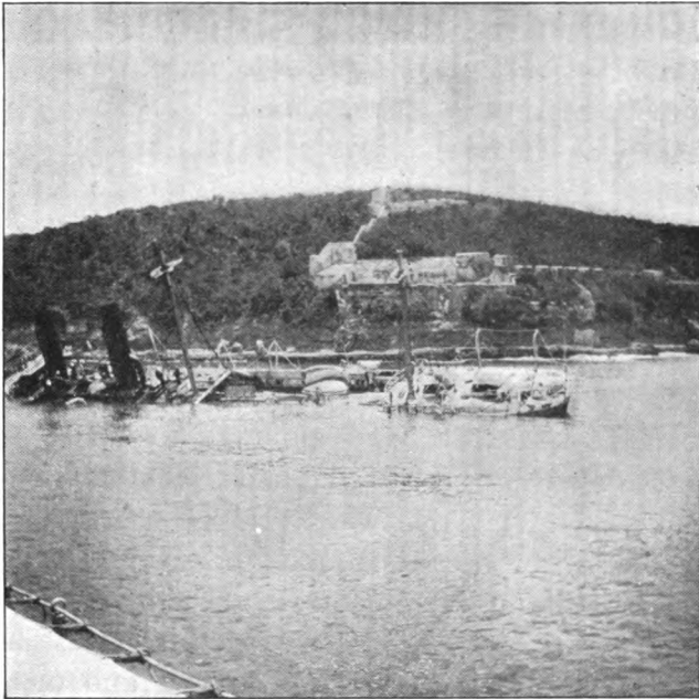
The Reina Mercedes as She Lies at the Entrance to Santiago Harbor. Reina Mercedes , Cruiser. Dimensions, 279 x 43; draft, 16.5; displacement, 3,090. Speed, 17.5 knots. Main Battery, six 6.2-inch guns.
