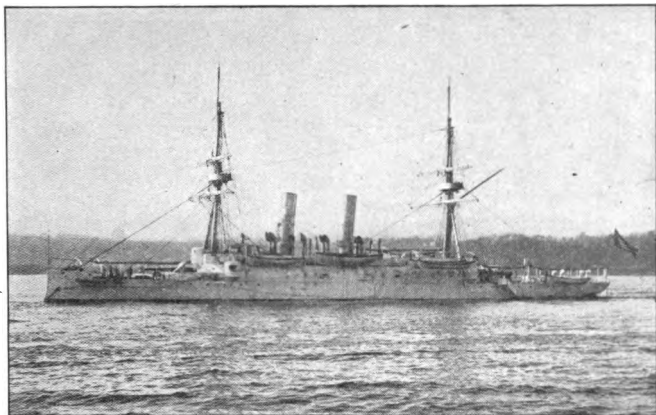
Atlanta , Protected Cruiser. Dimensions, 271 x 42; draft, 21; displacement, 3,000. Speed, 15.6 knots. Main Battery, two eight-inch, six six-inch guns.
