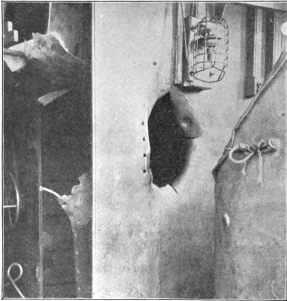
Shot-hole Starboard Hammock Berthing, Midships in the Texas .
