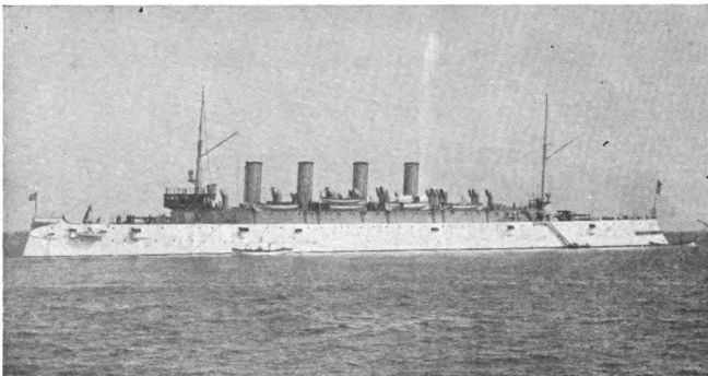
Columbia , Protected Commerce-Destroyer. Dimensions, 412 x 58; draft, 25; displacement, 7,375. Speed, 22.8 knots. Main Battery, one eight-inch, two six-inch slow-fire, eight rapid-fire four-inch guns.
