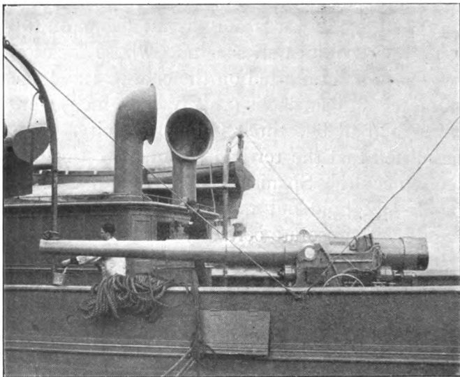
A six-inch Gun on the Aft-deck of the Auxiliary Hyst .
