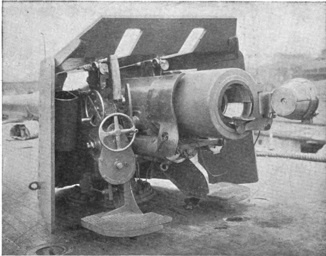
A Six-Inch Gun on the New Orleans .
