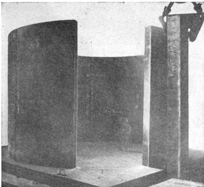
A Barbette before it is installed.
