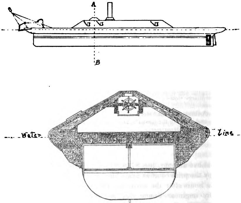
CONFEDERATE IRON-CLAD Atlanta , CAPTURED BY THE Weehawken . Enlarged section on A-B showing framing, wooden armor, etc.
