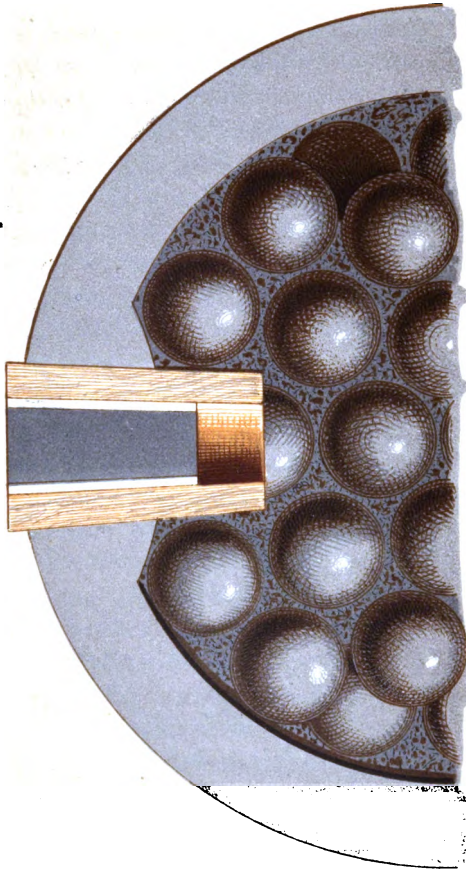
Section of 12 pdr. Shrapnel For Boat Howitzers U.S. Fuze. — Full size.
