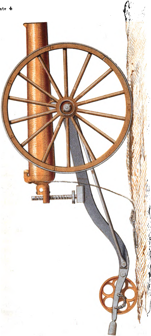
Naval Field Carriage (12 pdr. of 750)
