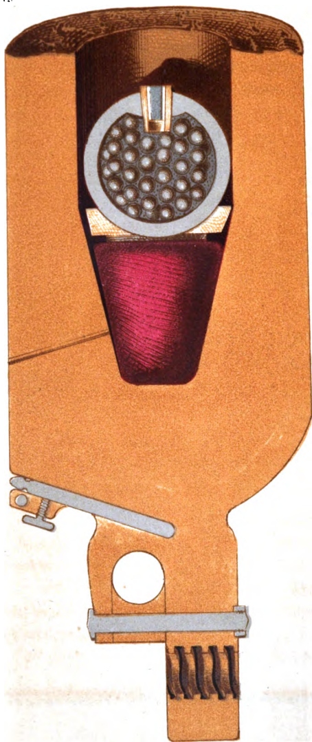
Section of Boat Howitzers.
