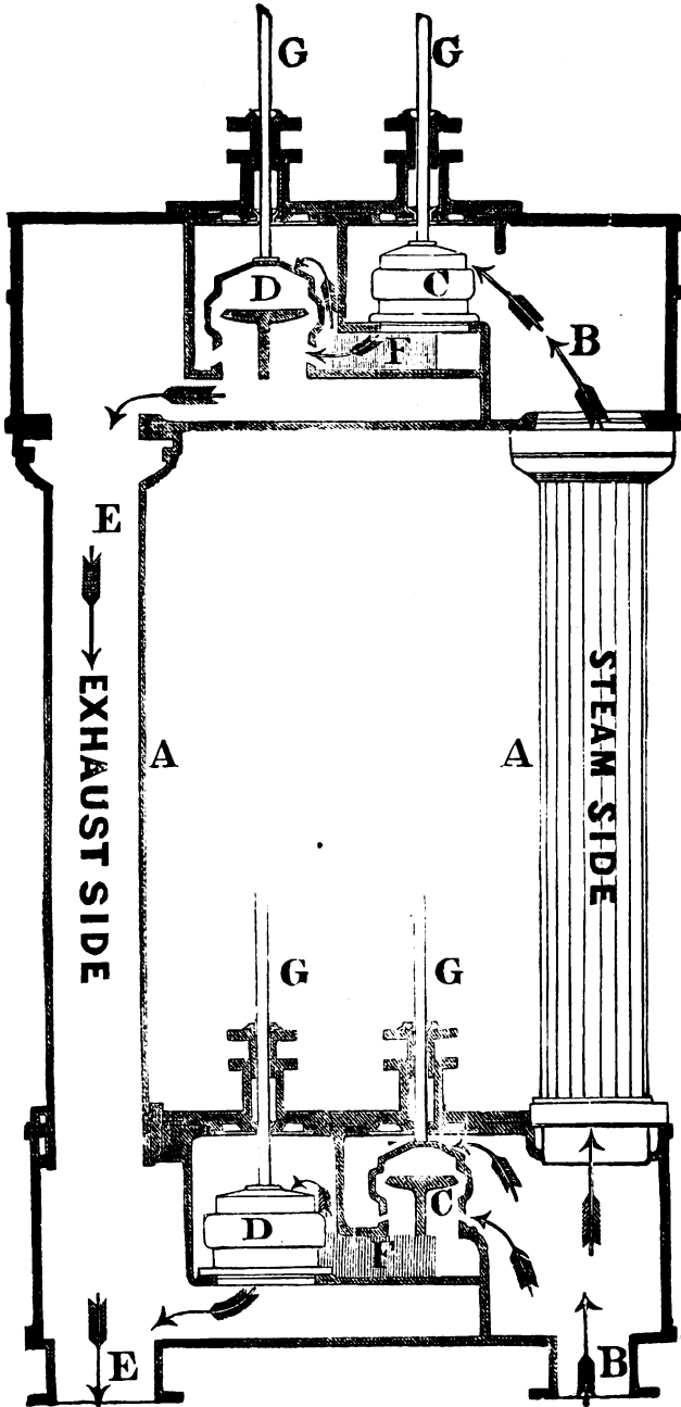
SECTION OF A STEAM ENGINE CYLINDER SIDE PIPES, WITH CORNISH DROP VALVES.
