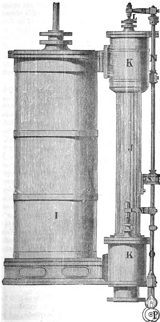
SIDE VIEW OF CYLINDER AND SIDE PIPES, WITH CORNISH VALVES AND REVOLVING TAPSETS.
