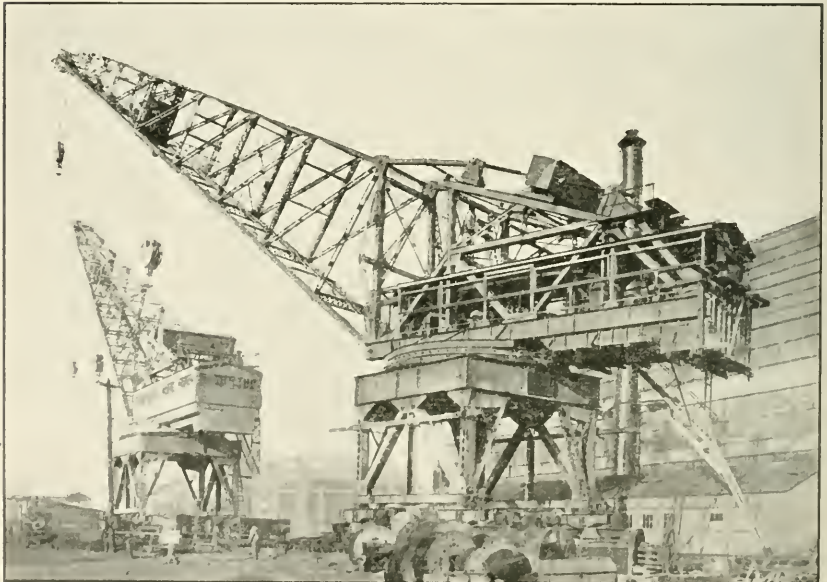
Locomotive cranes (50-ton) for Dry Dock No. 3, Navy Yard, Philadelphia, Pa.
