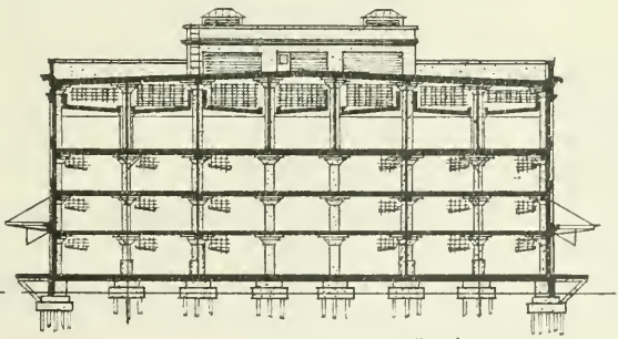
Cross Section on Line "B-B" 1 INCH = 20 FEET
