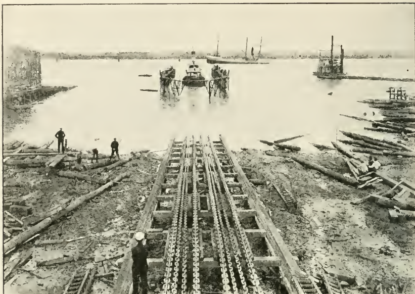
Marine railway, Navy Yard, Charleston, S. C. Cradle submerged.
