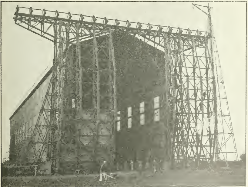
Frame dirigible hangar, United States Naval Air Station, Paimboeuf, France; late construction view.
