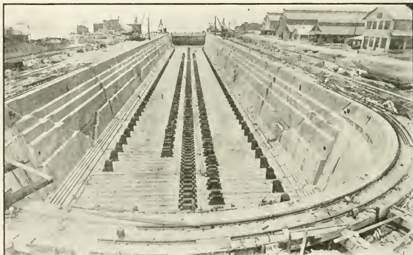
Dry Dock No. 1, Naval Station, Pearl Harbor, Hawaii. General view of interior from head end.
