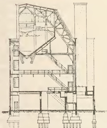
BOILER ROOM ch = 20 feet.
