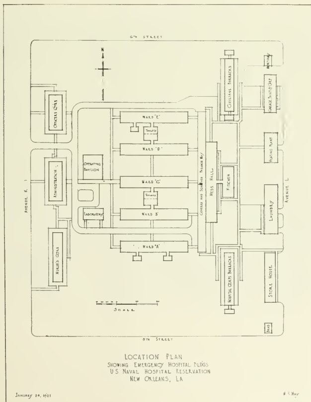
Plot plan, Naval Hospital, New Orleans, La.
