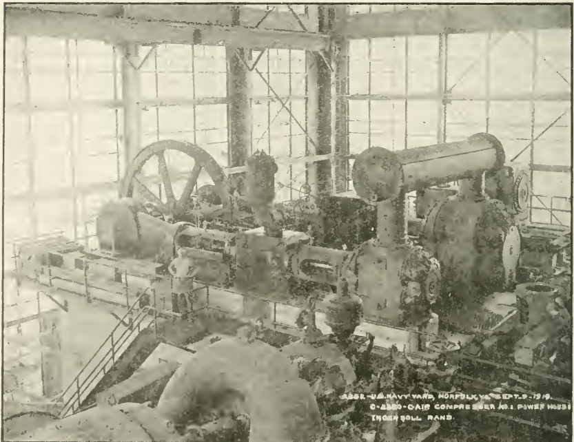
Reciprocating air compressor (6,500 cubic feet per minute) in power plant, Navy Yard, Norfolk, Va.
