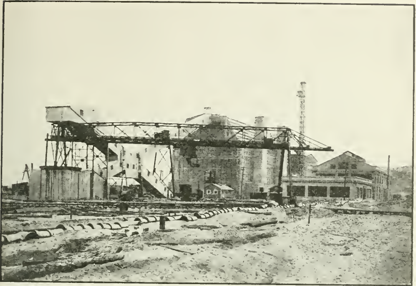
General view of power plant at Philadelphia Navy Yard, showing coal and ash handling plant.
