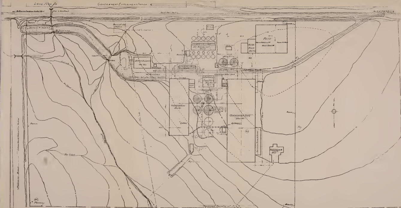
Plot plan of United States Helium Production Plant, Fort Worth, Tex.
