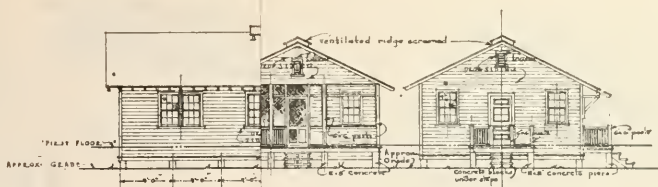
ELEVATION SOUTH ELEVATION OFFICERS' QUARTERS SCALE 1/8" = 1'-0"
