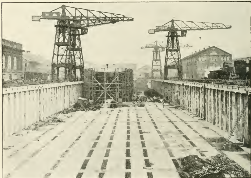
Shipbuilding dock, Navy Yard, Puget Sound, Wash. General view showing U. S. S. Pyro under construction.
