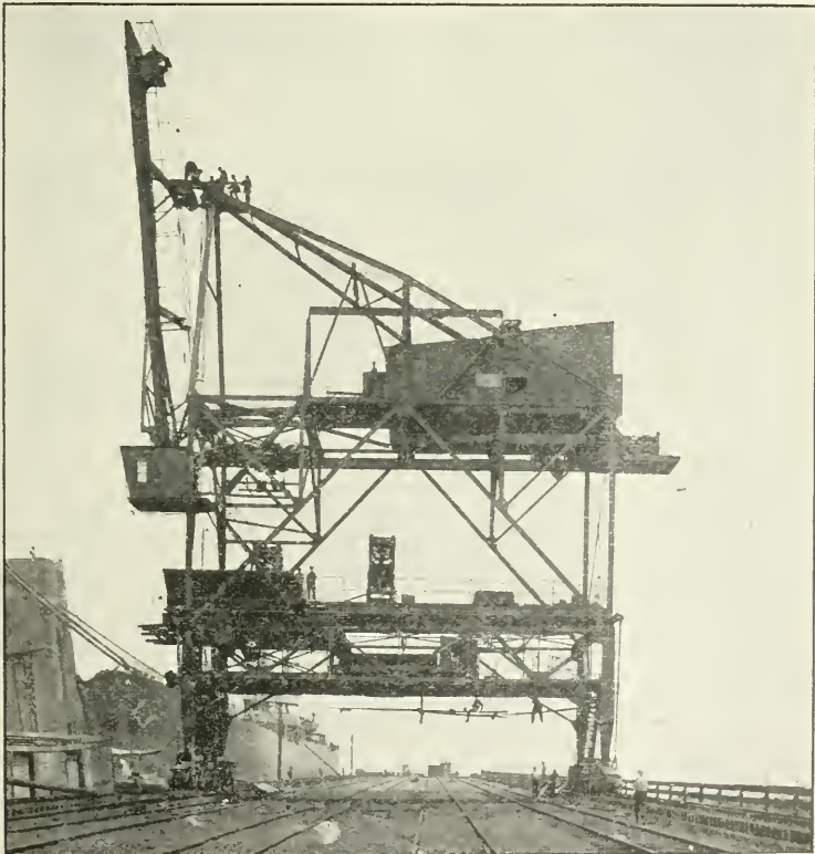
Mead-Morrison coal unloader, Emergency Fuel Depot, Constable Hook, N. J.
