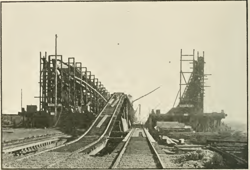
Double slip for destroyer construction, Navy Yard, Mare Island, Calif.
