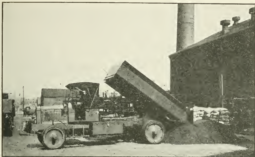
Typical yard 7-ton back-dumping truck.
