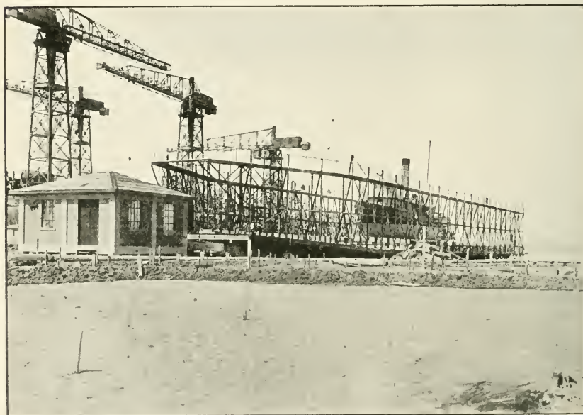
Marine railway, Navy Yard, Charleston, S. C. Cradle ashore.
