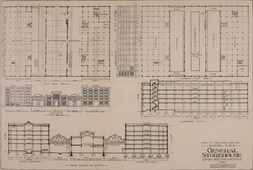
Design of general storehouse, Navy Yard, Washington, D. C., showing special bays for crane service.
