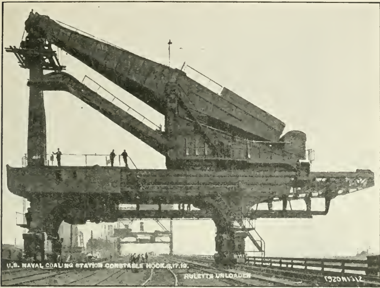
Hulette unloader, Emergency Fuel Depot, Constable Hook, N. J.
