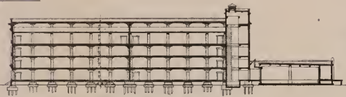
Longitudinal Section on Line "O-O"
