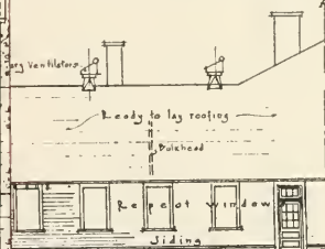
ELEVATION Scale 1/4" = 1'-0"
