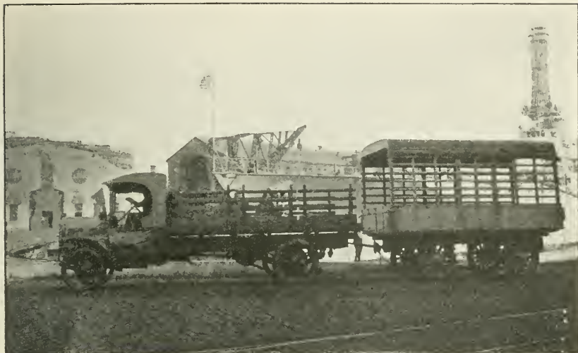
Typical yard 5-ton truck and trailer.
