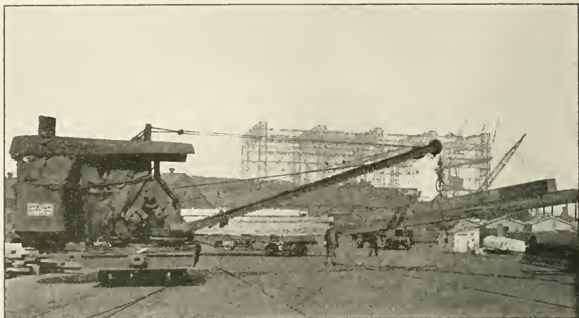
Typical yard 5-ton locomotive crane.
