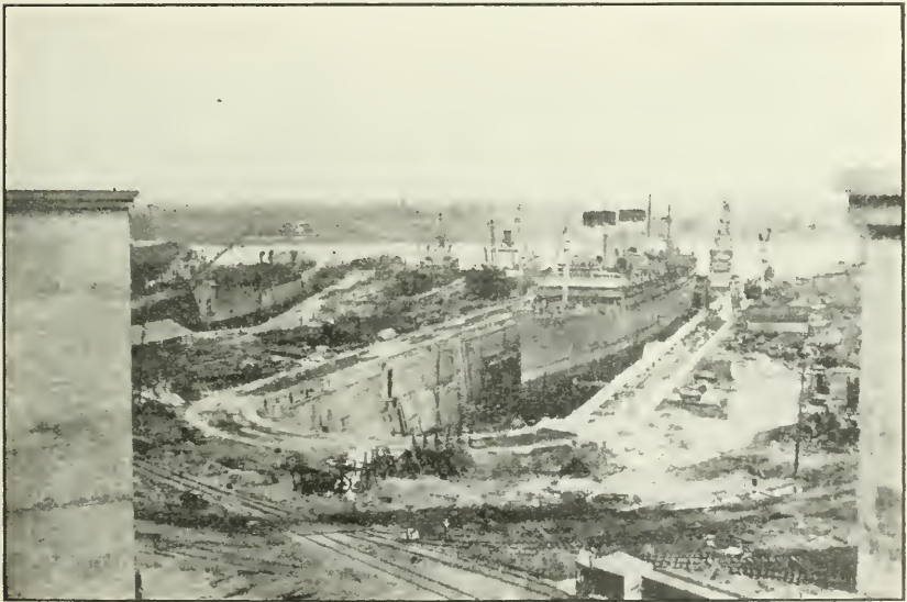
Dry docks at Navy Yard, Norfolk, Va., with vessels docked. Left to right: No. 3, U. S. S. Jupiter ; No. 6, S. S. Dio ; No. 7, S. S. Eastern Victor ; No. 4, U. S. S. Mount Vernon .
