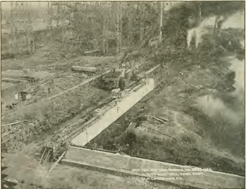
Construction of concrete retaining wall, Navy Yard, Norfolk, Va.
