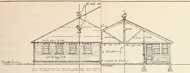
SECTION B-B Scale 1/4" = 1'-0"
