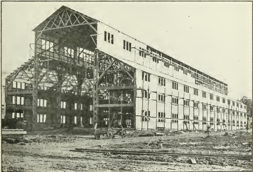
Boat-storage building (timber), Navy Yard, Mare Island, Calif.
