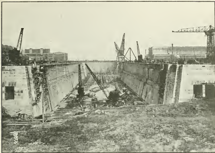
Dry Dock No. 3, Navy Yard, Philadelphia, Pa., under construction. View taken from cofferdam at entrance.
