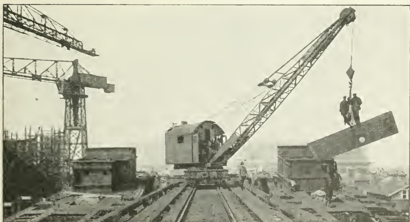
Twenty-five-ton locomotive crane on elevated trestle for twin minesweeper construction, Navy Yard, Philadelphia, Pa.
