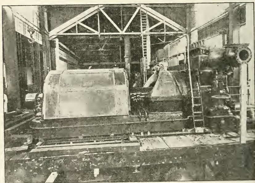
7,500-kilovolt-ampere turbo-generator in power plant at Naval Proving Ground and Smokeless-Powder Factory, Indianhead, Md.
