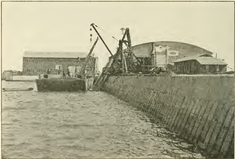
Concrete sheet-pile protection of existing bulkhead walls of lagoon, Naval Operating Base, Hampton Roads, Va.
