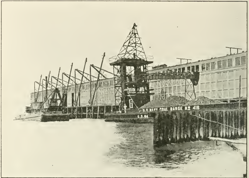
Derricks for supporting De Mayo elevators. Bunkering Depot, Newport News, Va.
