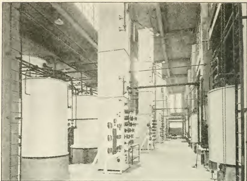
Interior view, separation building, United States Helium-Production Plant, Fort Worth, Texas.
