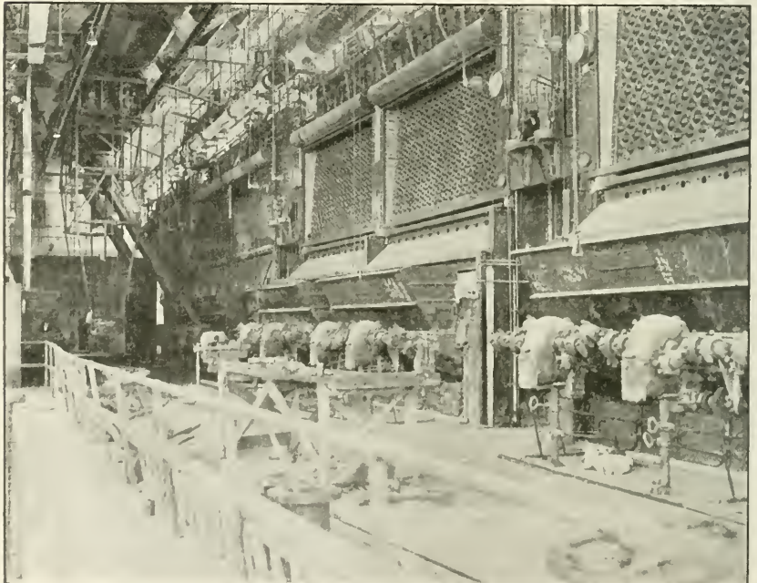
Battery of boilers in power plant at Navy Yard, Norfolk, Va.
