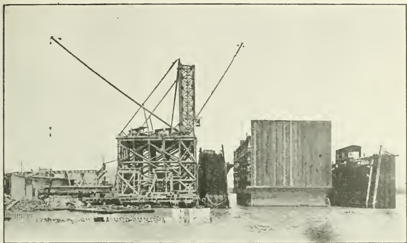
Dry Dock No. 1, Naval Station, Pearl Harbor, Hawaii. Pump well before launching from floating dock.
