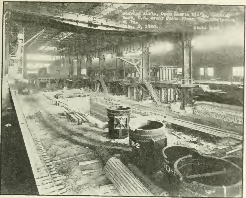
Pouring aisle in open-hearth building, Armor Plant, Charleston, W. Va.
