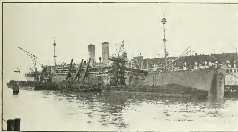
Mitchner elevators, steam fueling barge, and escalade in operation at Bunkering Depot, Pier 4, Lamberts Point, Va.
