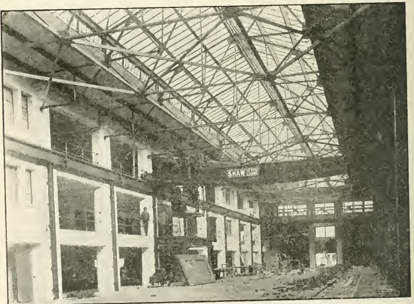
Interior of general storehouse, Navy Yard, Washington, D. C., showing crane service.
