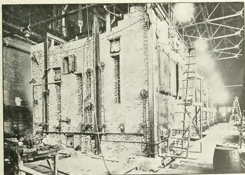
Boiler installation at power plant, Navy Yard, Puget Sound, Wash.
