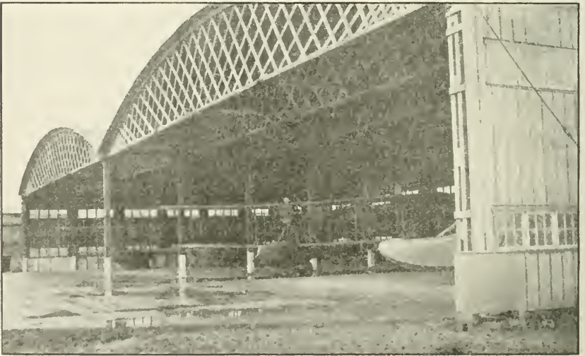
Seaplane hangars, United States Naval Air Station, Pauillac, France.
