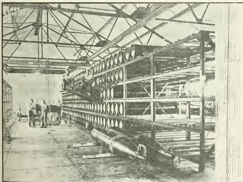
Typical torpedo racks and crane as designed by the Bureau.
