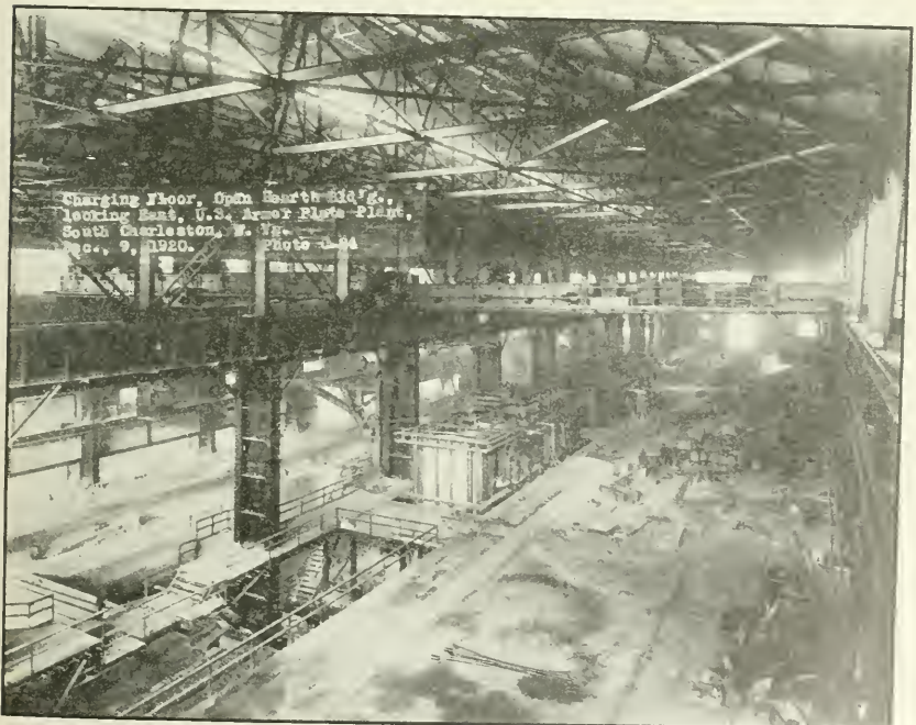
Charging floor of open-hearth building, Armor Plant, Charleston, W. Va.
