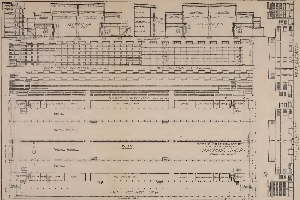
Bureau layout for industrial yard machine shop.
