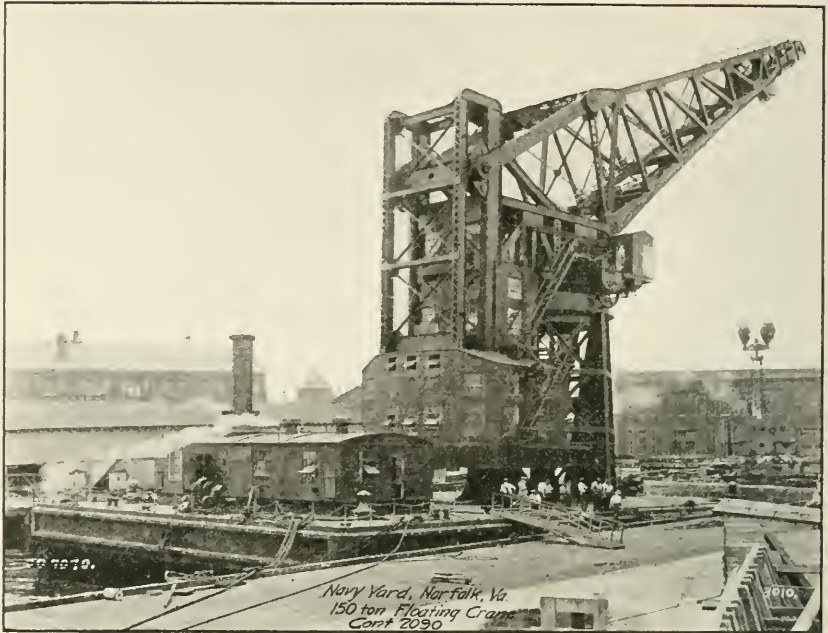
Floating crane (150-ton), Navy Yard, Norfolk, Va.
