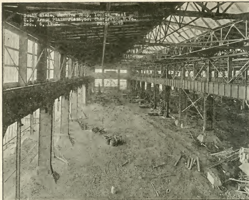
South aisle of machine shop, Armor Plant, Charleston, W. Va.
