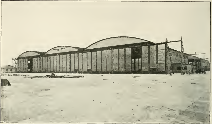
Seaplane hangars, Hampton Roads, Va.; curve-truss, sliding-door type.
