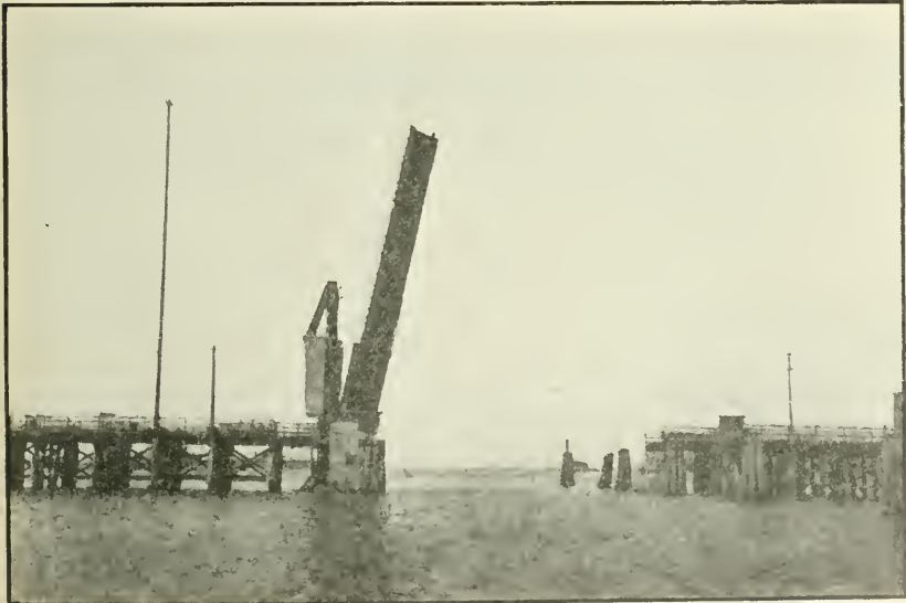
Causeway connecting Mare Island Navy Yard with mainland; bascule bridge raised.
