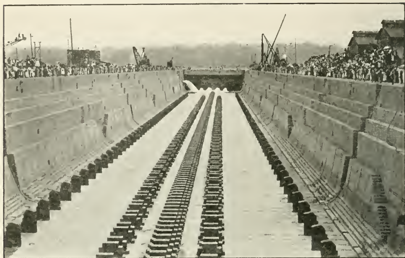
Dry Dock No. 1, Naval Station, Pearl Harbor, Hawaii. View of completed structure at formal opening.
