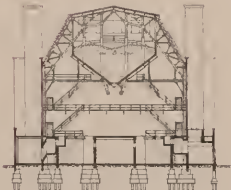
SECTION THROUGH BOILER ROOM Scale 1/8" = 1'-0"
