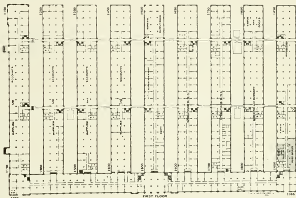
Typical floor plan of Navy unit, emergency office buildings, Potomac Park, Washington, D. C.
