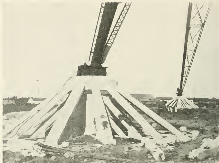
FIG. 6.—Lafayette Radio Station. Tower footings as designed by French engineers.
