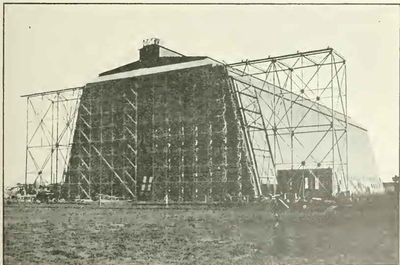
Typical dirigible hangar, San Diego, Calif.
