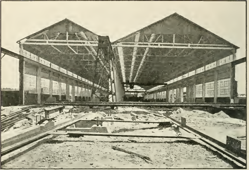
Ship fabricating shed, Navy extension to plant of Newport News Shipbuilding and Dry Dock Co., Newport News, Va.
