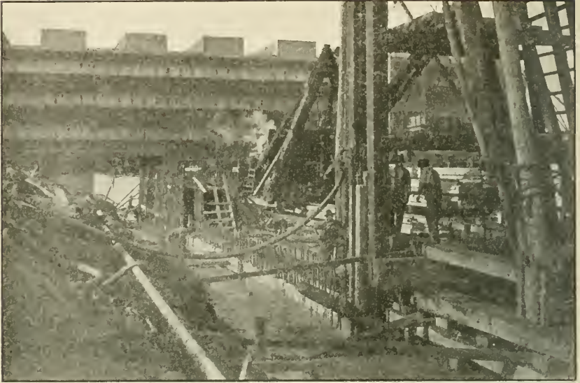
Quay wall construction, Navy Yard, Norfolk, Va. Jetting of concrete sheet piles in foreground.
