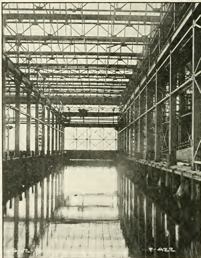
Interior view of wet slip, Squantum destroyer plant.
