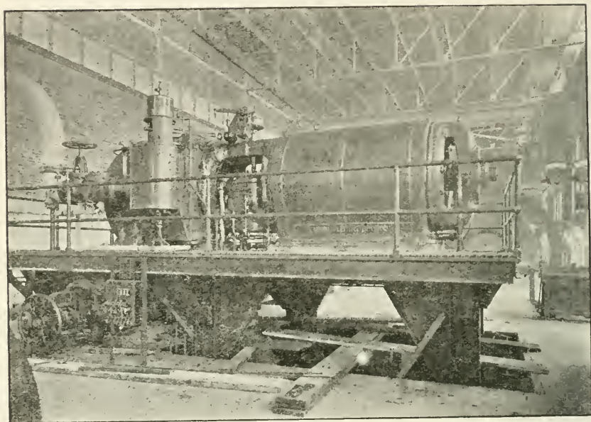
Turbo-alternator in power plant, Navy Yard, Puget Sound, Wash.
