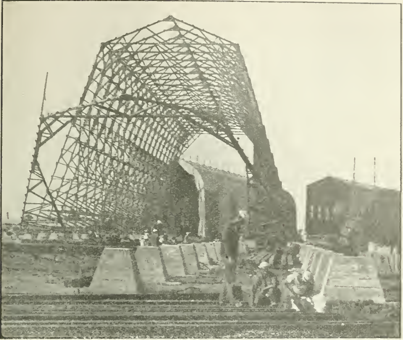
Frame dirigible hangar, United States Naval Air Station, Paimboeuf, France; early construction view.
