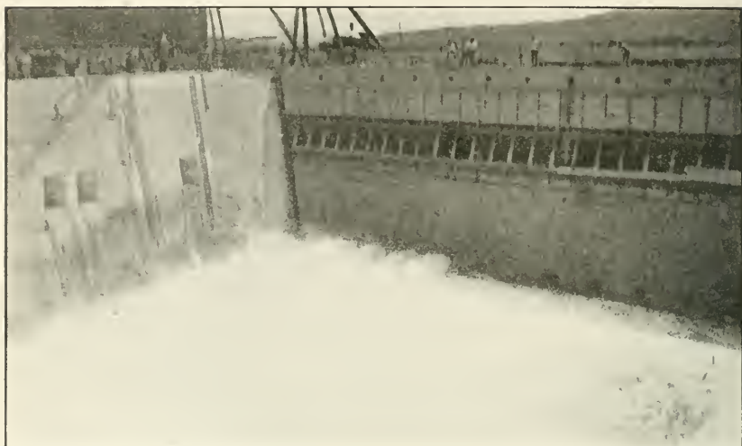
Dry Dock No. 1, Naval Station, Pearl Harbor, Hawaii. Admitting water through caisson for testing pumps.
