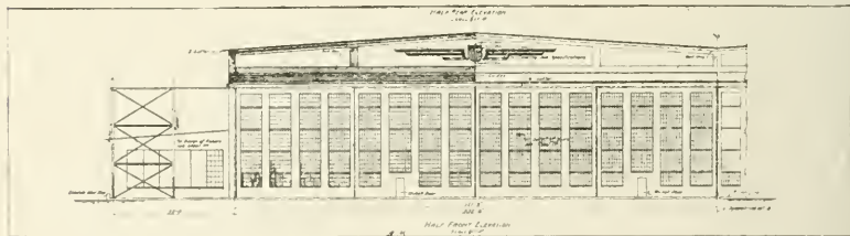
Elevation of standard 151-foot seaplane hangar.
