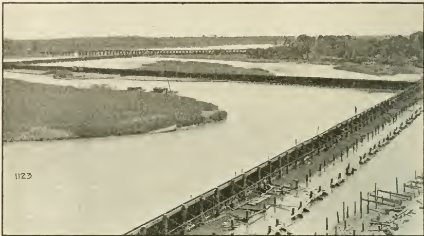
Bulkheads along Boush Creek, Naval Operating Base, Hampton Roads, Va.
