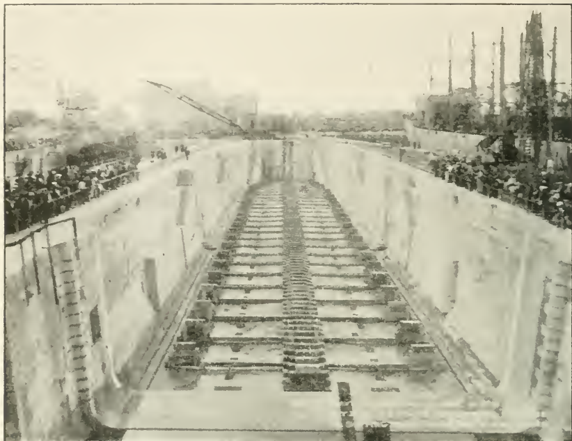
Dry Dock No. 6, Navy Yard, Norfolk, Va., before first flooding ceremonial. Looking toward head end.
