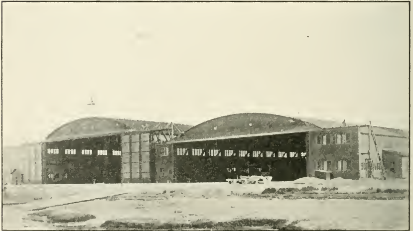
Seaplane hangars, Cape May, N. J.; curve-truss, sliding-door type.
