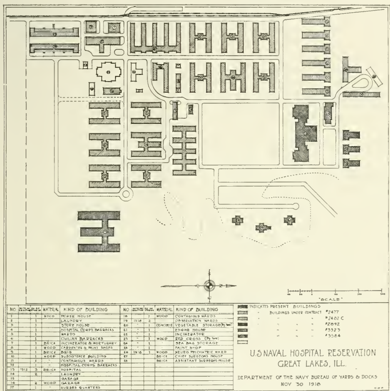
Plot plan of hospital reservation, Naval Training Station, Great Lakes, Ill.
