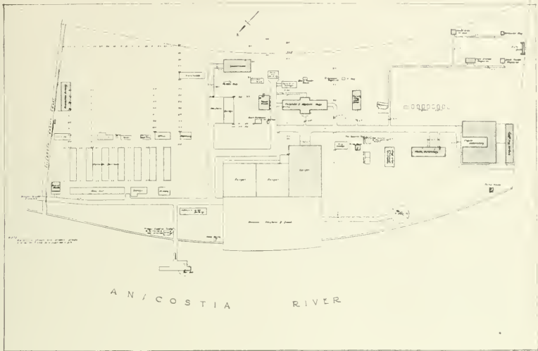
Existing plan of Naval Air Station, Anacostia, D. C., showing temporary buildings.
