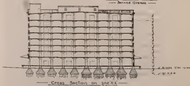
— Cross Section on line A-A —
