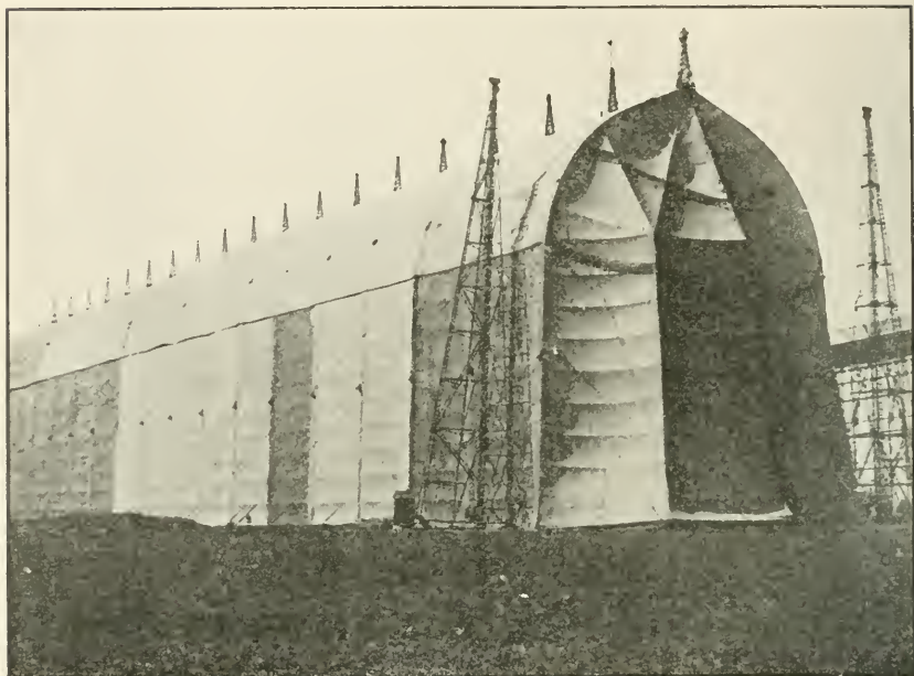
Canvas dirigible hangar, United States Naval Air Station, Paimboeuf, France.
