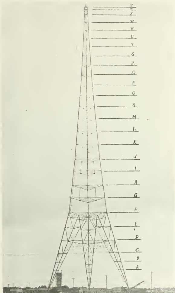
FIG. 2.—Lafayette Radio Station. Individual tower with panel points indicated.
