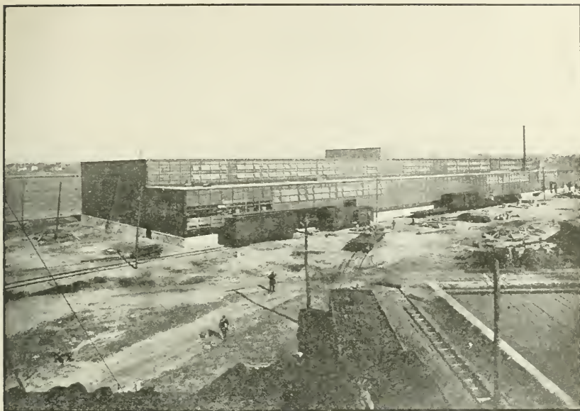
Boiler shop of Bethlehem Shipbuilding Corporation (Ltd.), at Providence, R. I.
