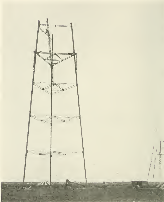
FIG. 3.—Lafayette Radio Station. Erection tower in process of construction.
