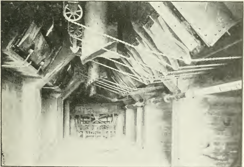
Ash-removal system at power plant, Navy Yard, Philadelphia, Pa.
