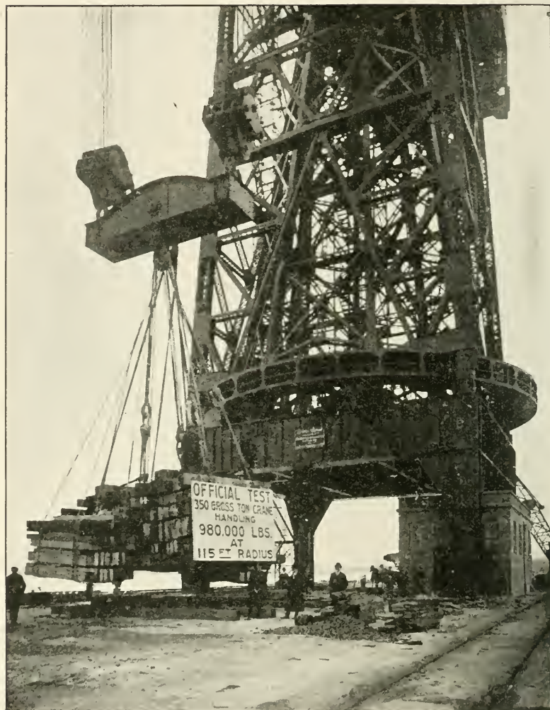
Official test of 350-ton fitting-out crane, Navy Yard, Philadelphia, Pa.
