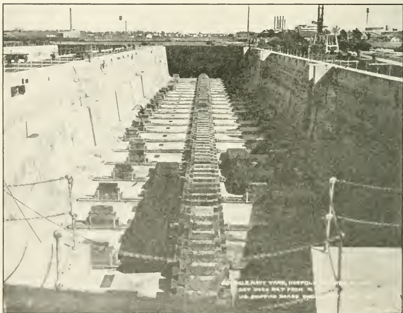
Dry Dock No. 7, Navy Yard, Norfolk, Va. Looking toward caisson.
