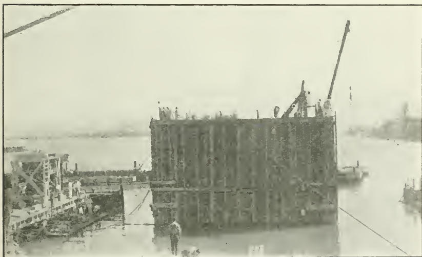
Dry Dock No. 1, Naval Station, Pearl Harbor, Hawaii. Pump well after launching from floating dock.
