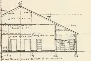
SECTION A-A Scale 1/4" = 1'-0"
