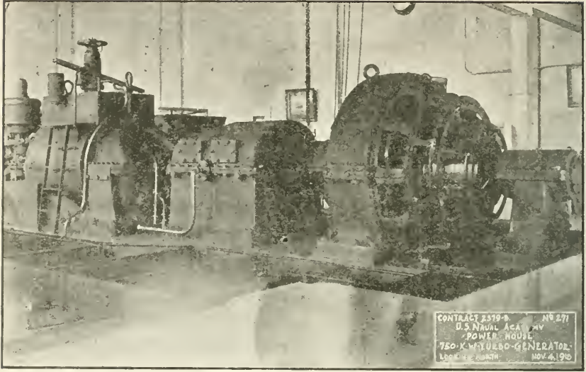
750-kilowatt turbo-generator as installed in Naval Academy power plant, Annapolis, Md.
