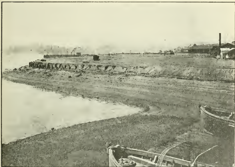
Filling operation in progress, Navy Yard, Puget Sound, Wash., showing extension of shore line.
