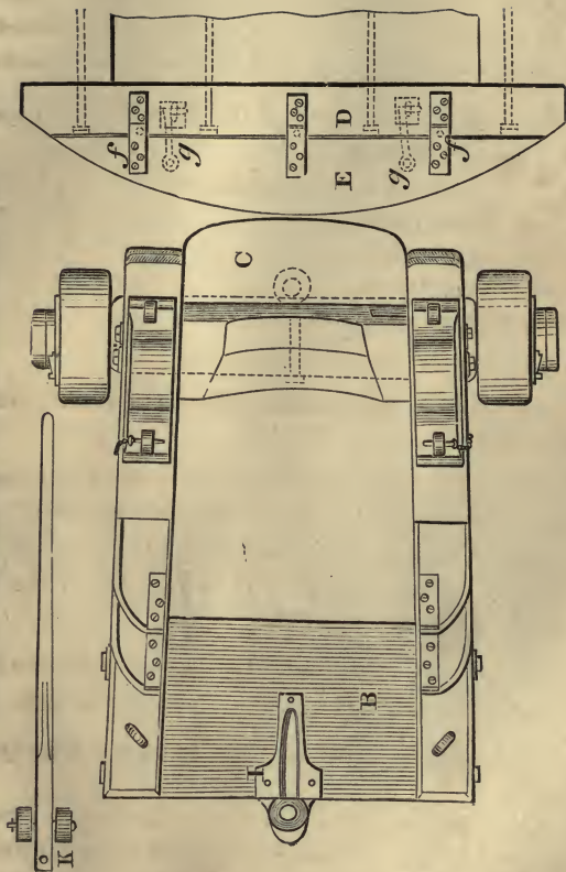
Marsilly Carriage for IX-Inch Shell Gun. Fig. 2.
