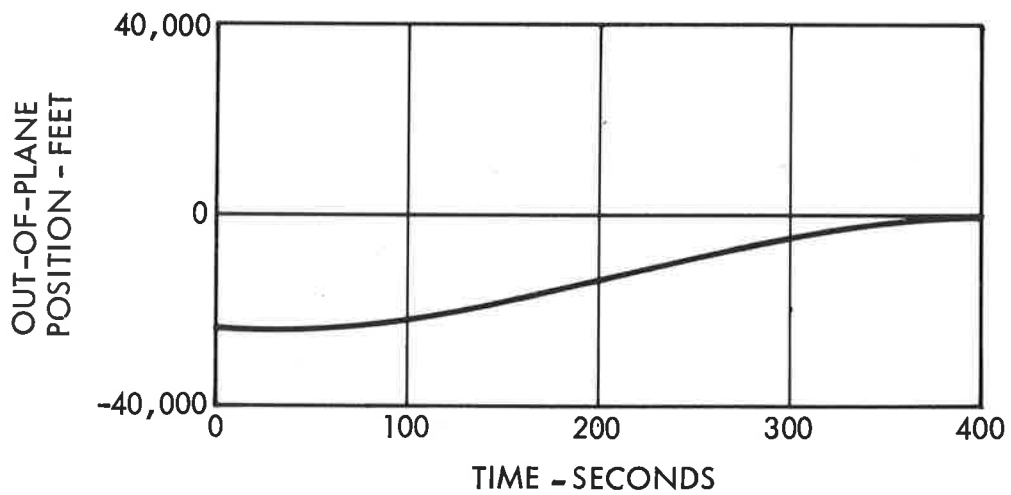
Figure 22. 4. Out-of-Plane Position versus Time for Lunar Surface Abort
