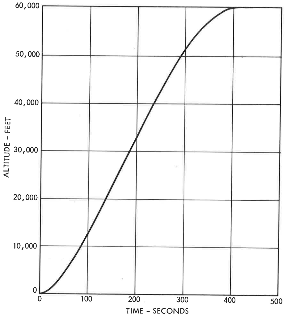
Figure 22.2. Altitude versus Time for Lunar Surface Abort
