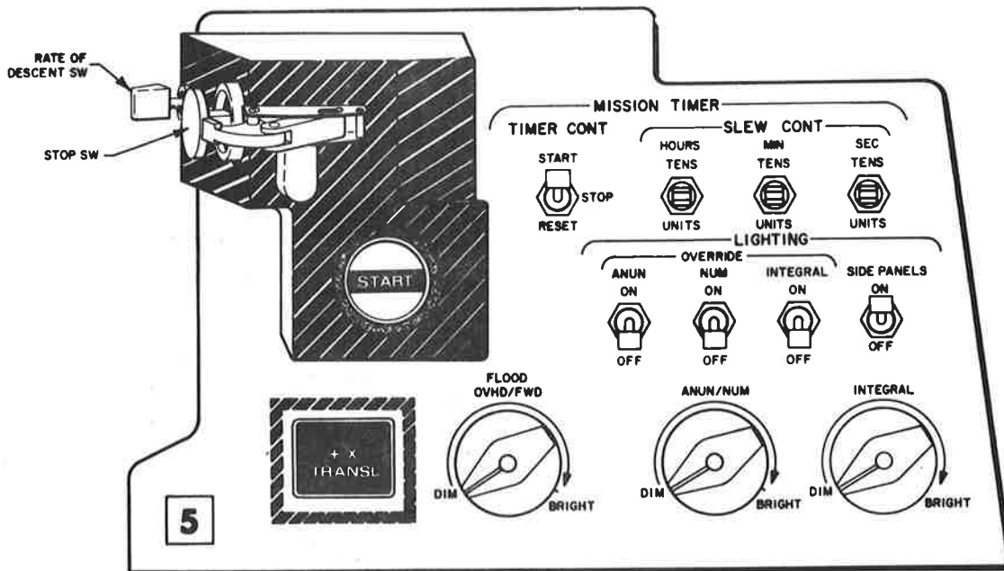
Figure 3.5 Bottom Panel (Panel 5)
