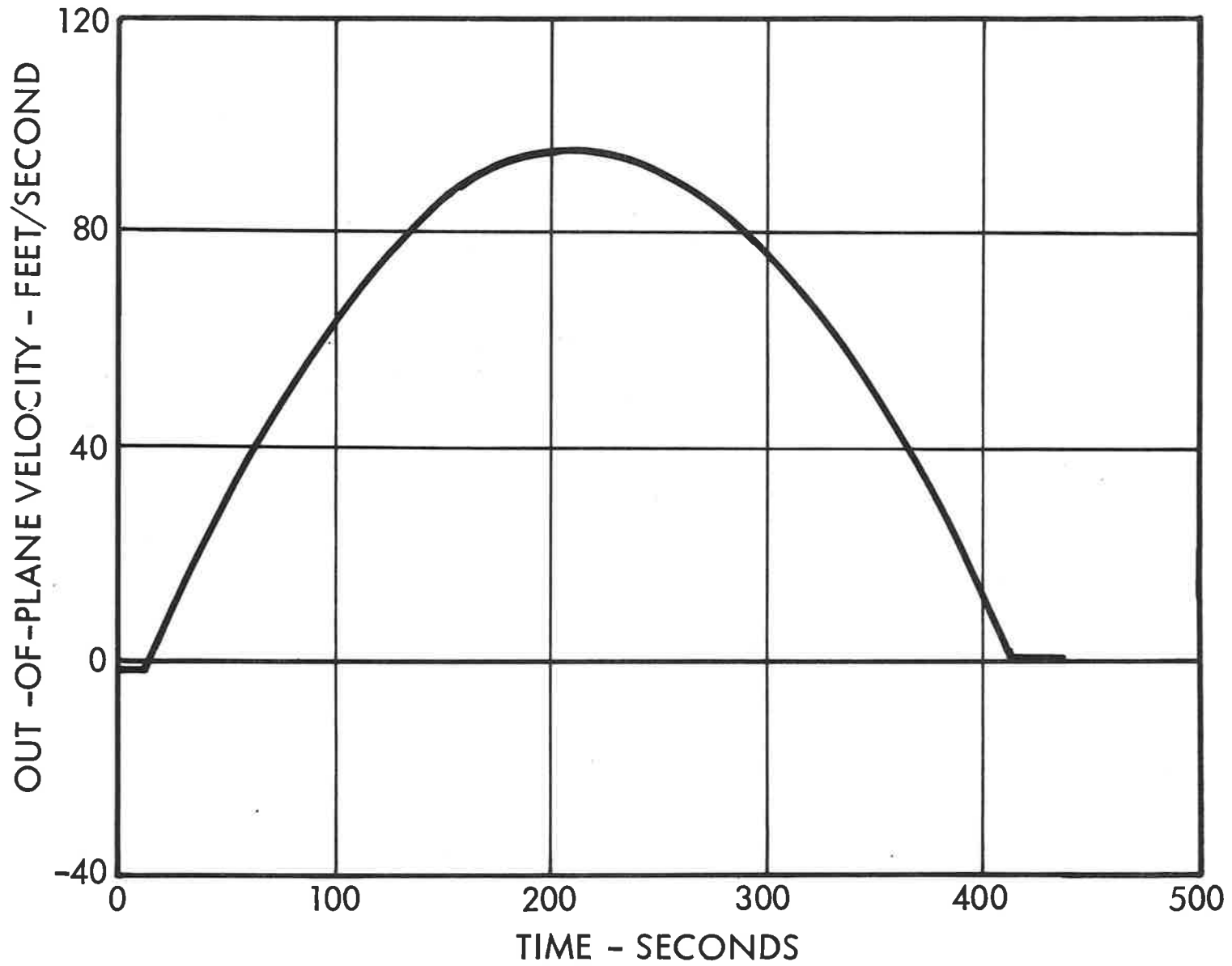
Figure 22.5 Out-of-Plane Velocity Versus Time for Lunar Surface Abort
