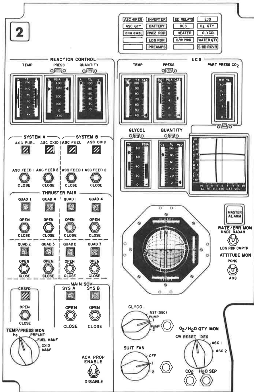
Figure 3.3. Center Console, Systems Engineer (Panel 2)
