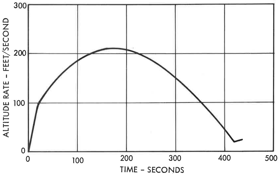
Figure 22. 3. Altitude Rate versus Time for Lunar Surface Abort
