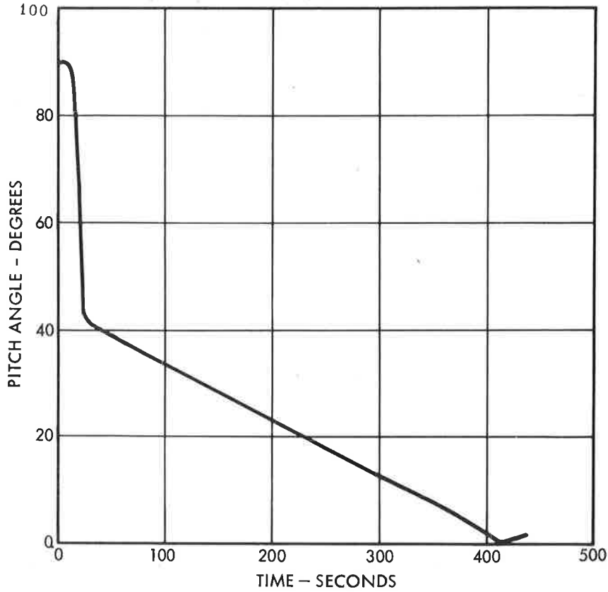
Figure 22.6. Pitch Angle versus Time for Lunar Surface Abort
