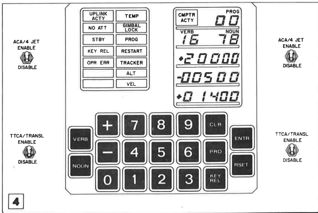
Figure 3.6 Bottom Center Panel (DSKY, Panel 4)
