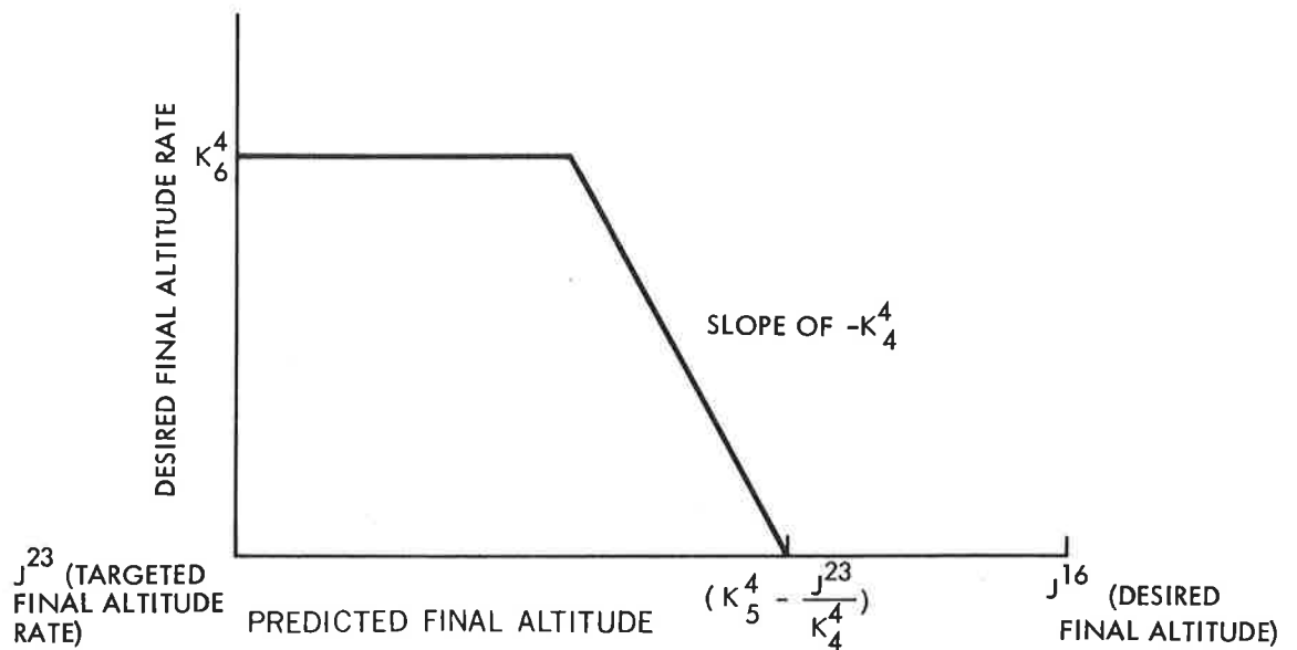
Figure 22.1. Desired Final Altitude Rate versus Final Altitude
