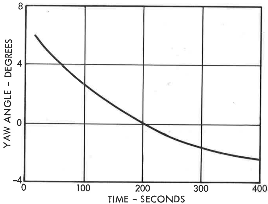
Figure 22.7. Yaw Angle versus Time for Lunar Surface Abort
