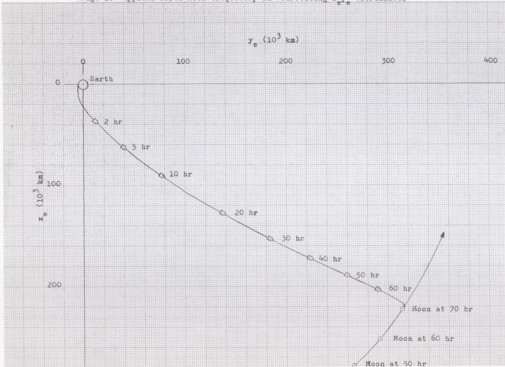
Fig. 1. Typical Earth-Moon Trajectory in Nonrotating x_e y_e Coordinates
