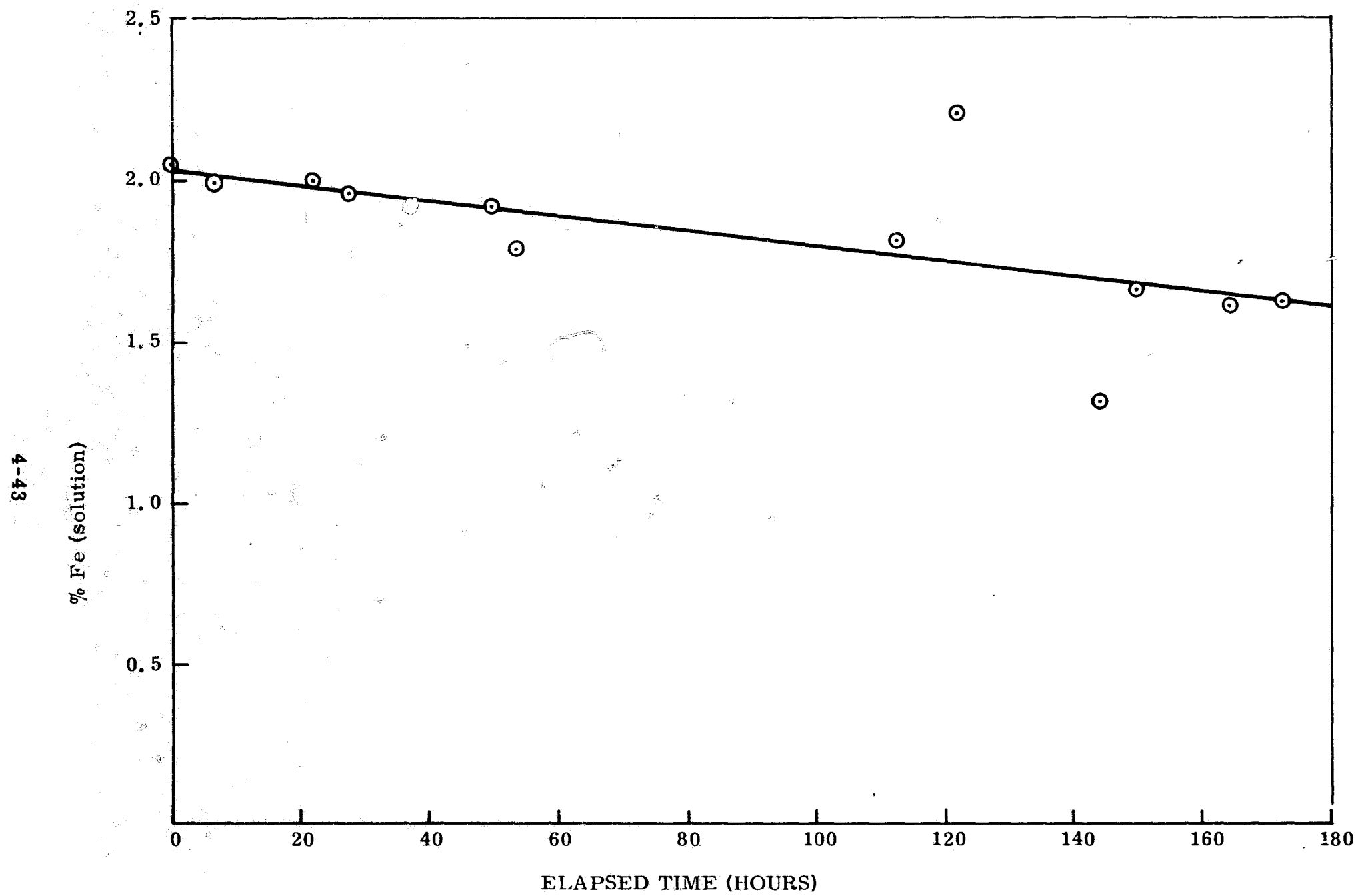
Fig. 4.26 Time variation of Fe percentage.
