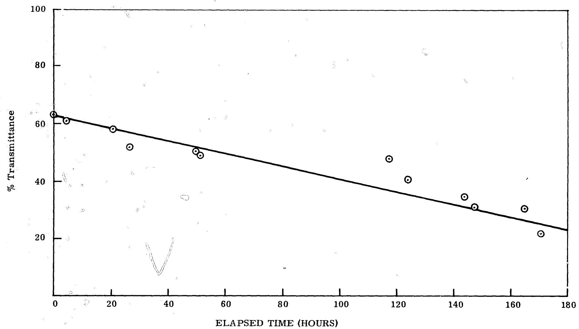
Fig. 4.27 Transmittance variation.
