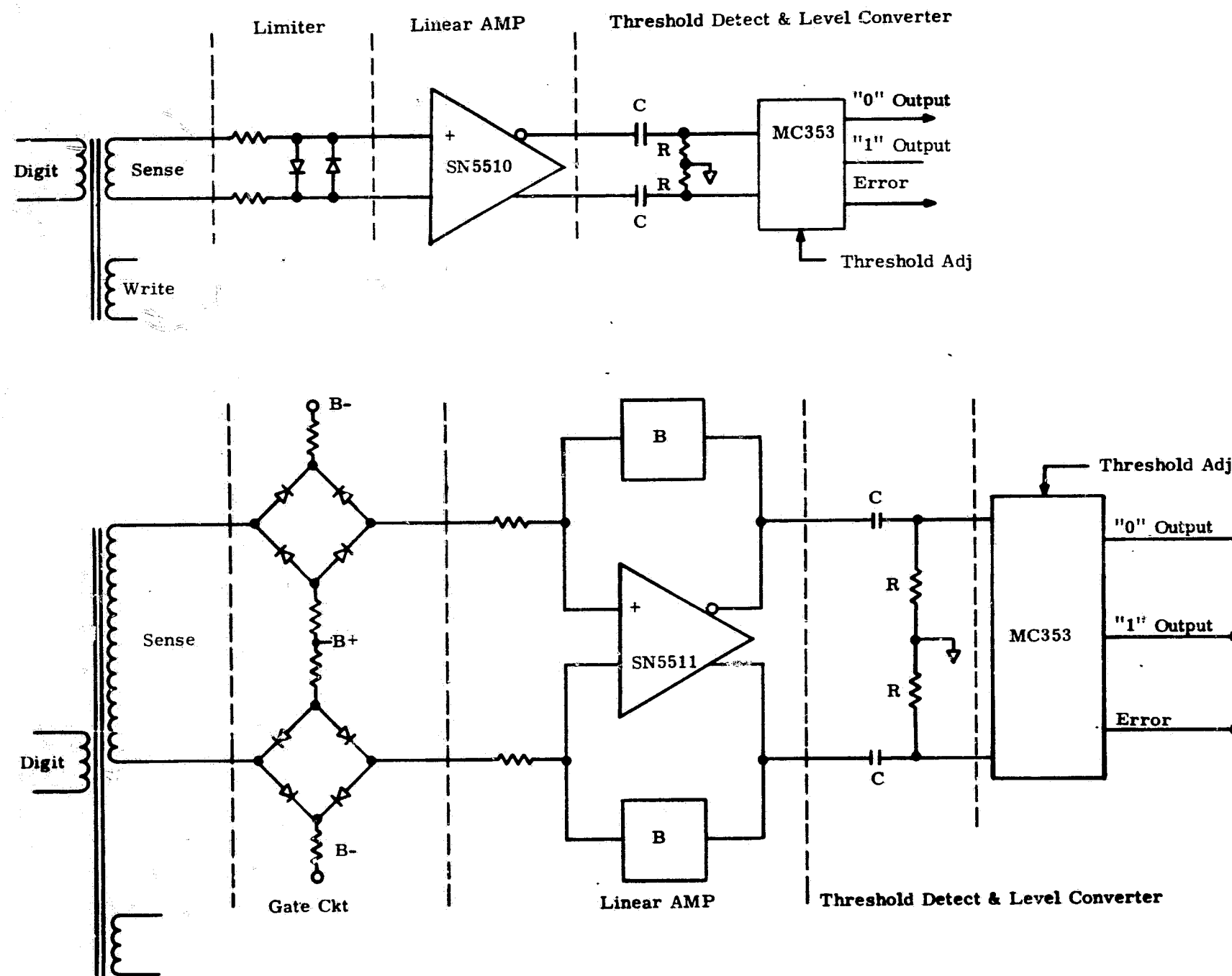
Fig. 4.48 Possible sensing configurations.
