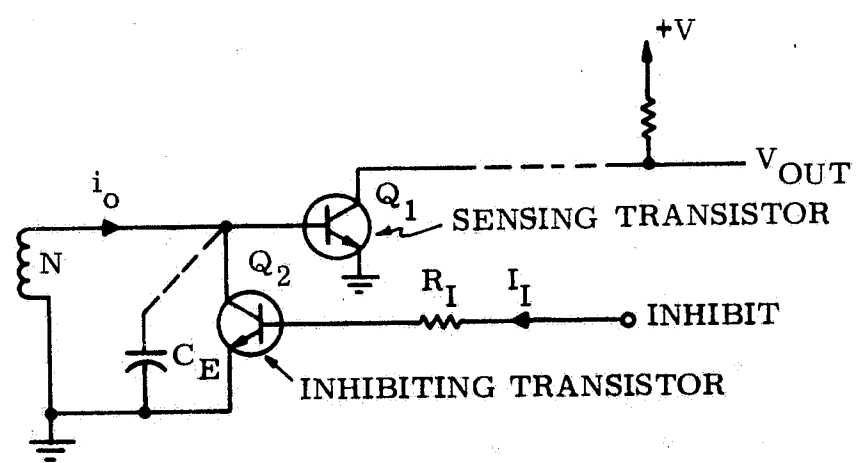
Fig. 4.7 Saturating-transistor amplifier.
