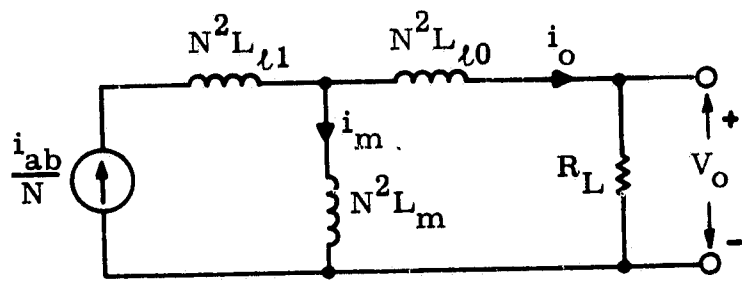
Fig. 4.3 Simplified equivalent circuit.
