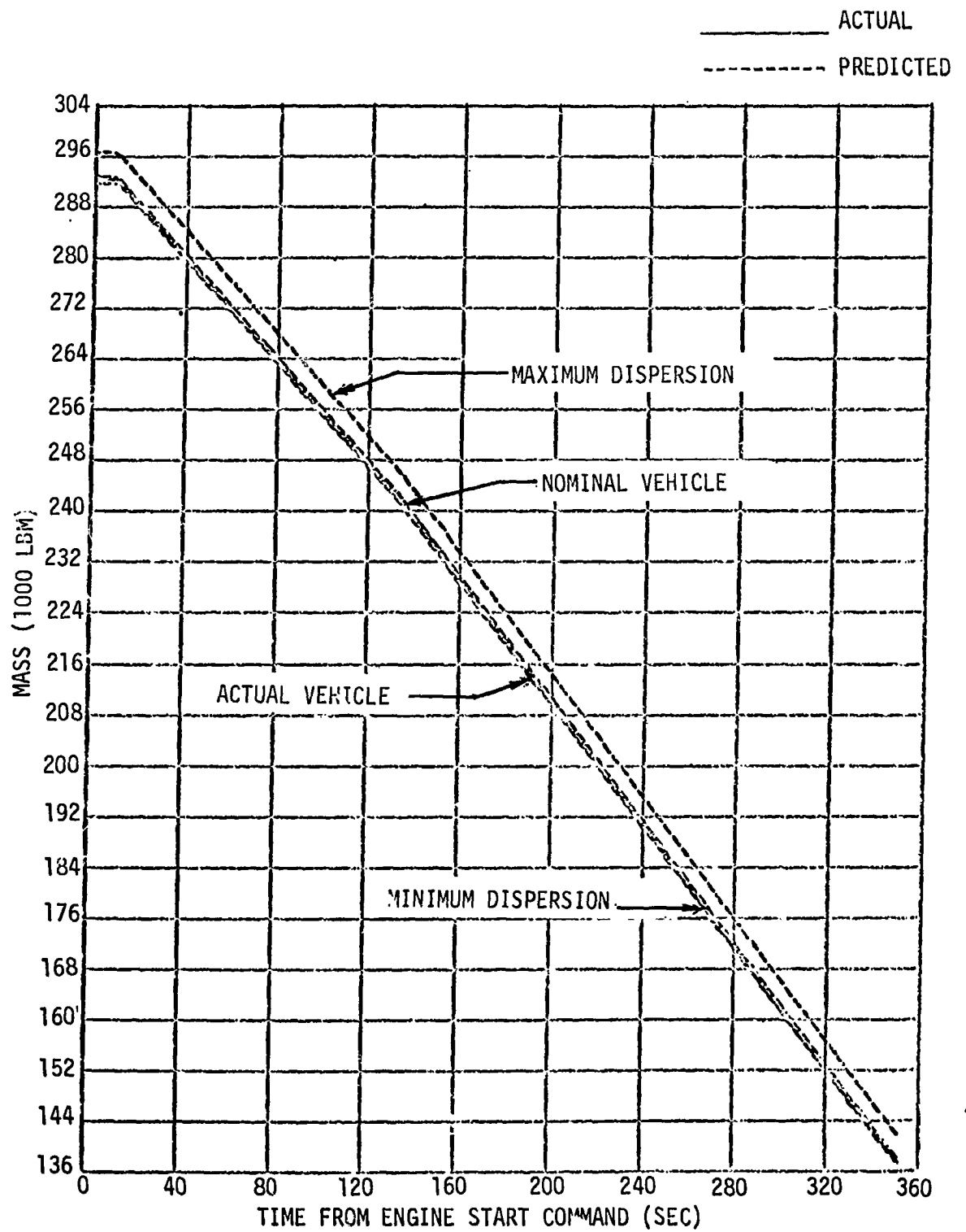
Figure 8-2. Third Flight Stage Vehicle Mass (Second Burn)
