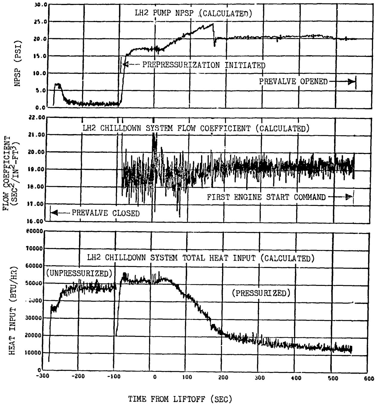
Figure 12-15. LH2 Pump Chillo-down--First Burn (Sheet 2 of 2)
