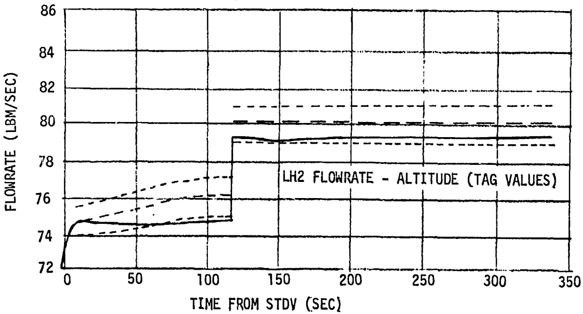
Figure 9-3. Second Burn Tag Values (Sheet 2 of 2)
