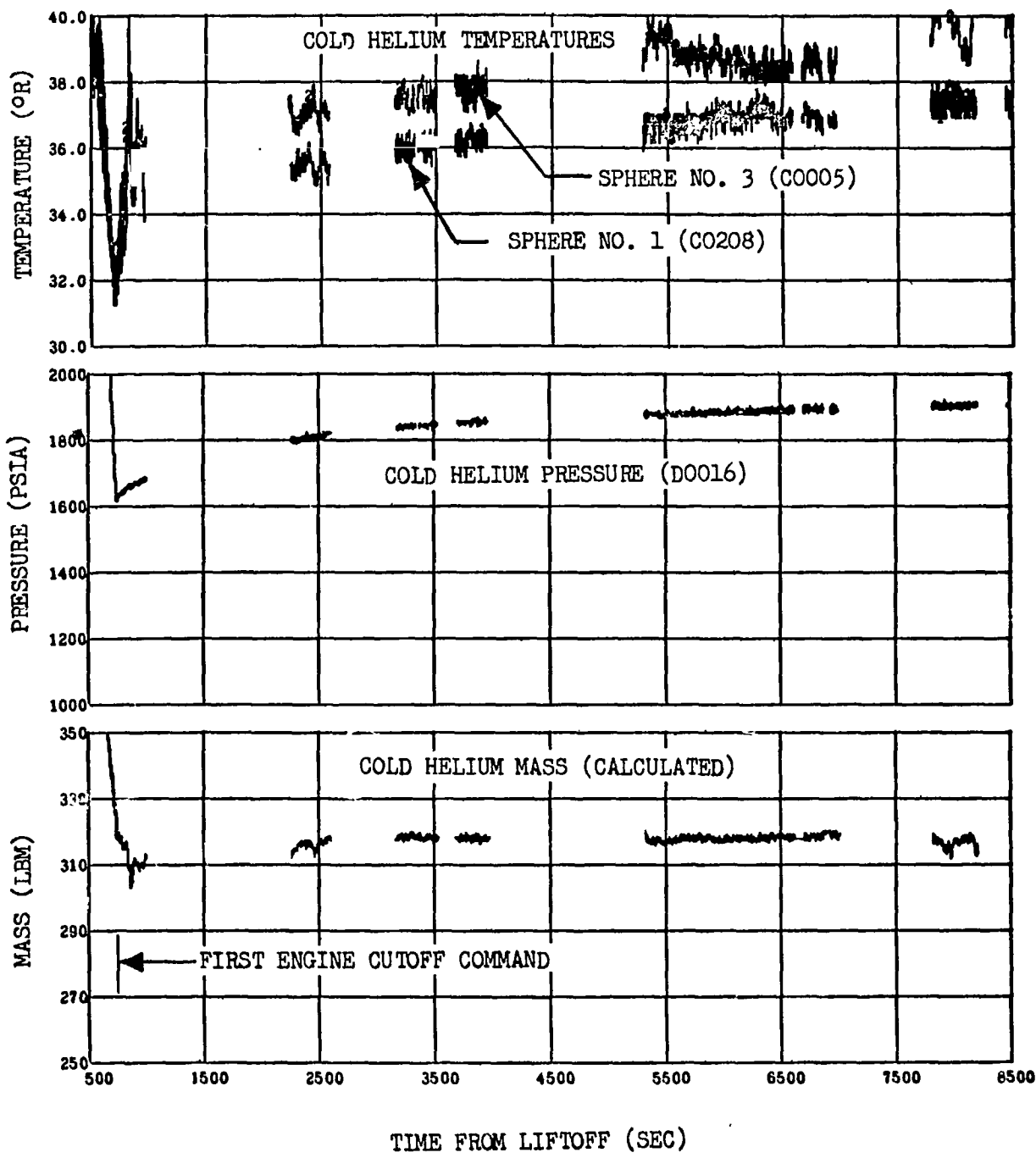
Figure 11-13. Cold Helium Sphere Conditions--Earth Orbit
