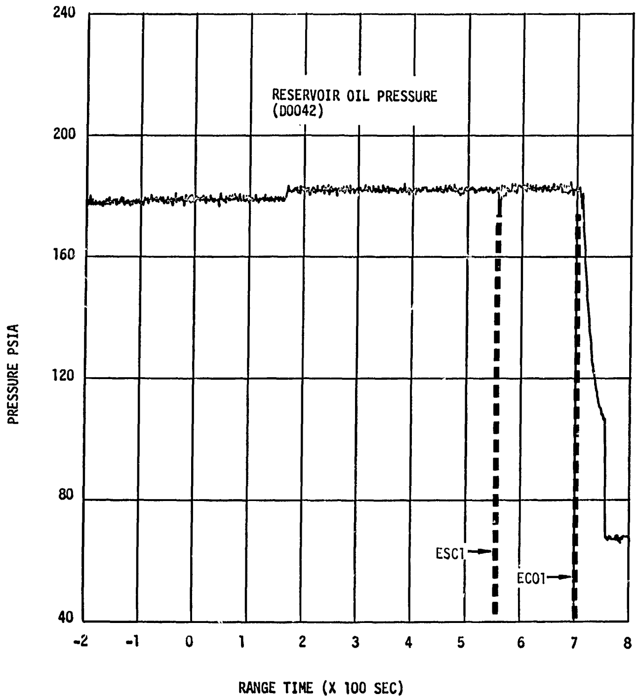
Figure 22-3. Reservoir Oil Press - Boost & 1st Burn
