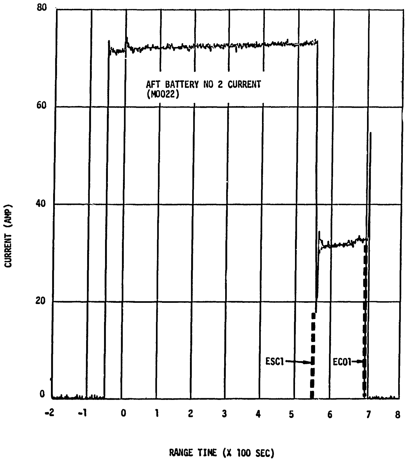
Figure 22-4. Aft Battery No. 2 Current Boost & 1st Burn
