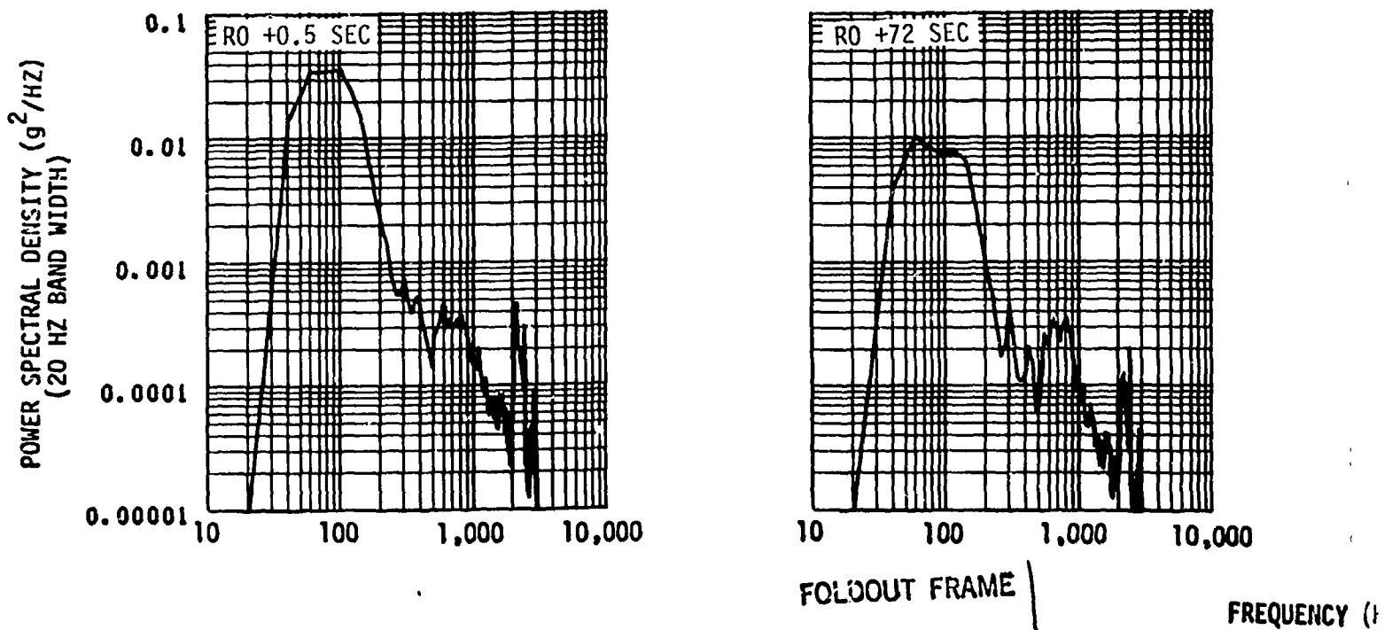
Figure 25-19. Vibration Measured at LH2 Prevalve, R
