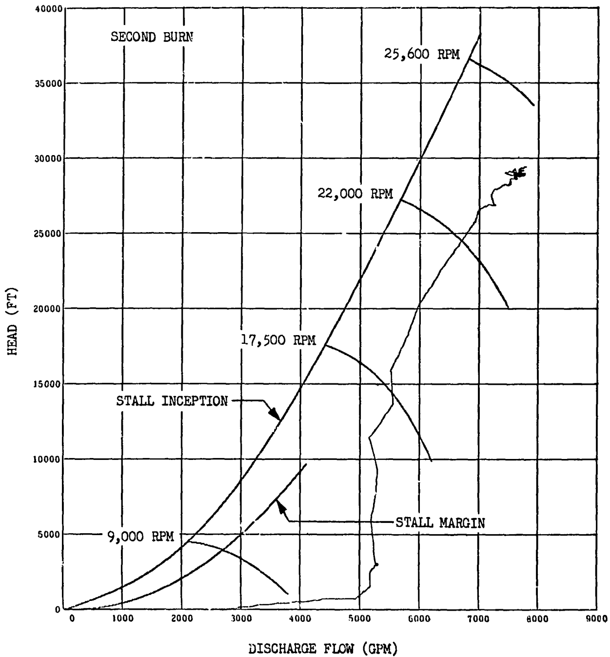
Figure 9-37. LH2 Pump Performance During Engine Start (Sheet 2 of 2)
