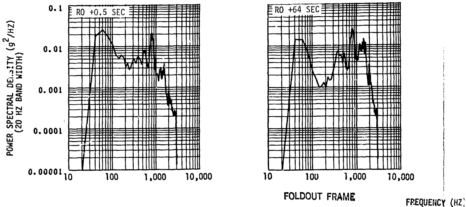
Figure 25-27. Vibration Measured at LH2 Vent Disconnect,
