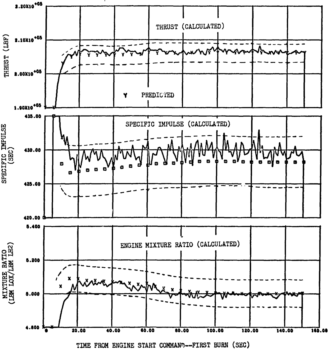
Figure 9-34. Engine Steady State Performance--First Burn (Sheet 1 of 3)
