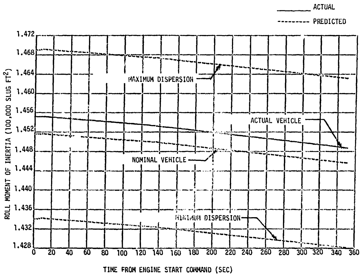
Figure 8-6. Third Flight Stage Vehicle Roll Moment of Inertia (Second Burn)
