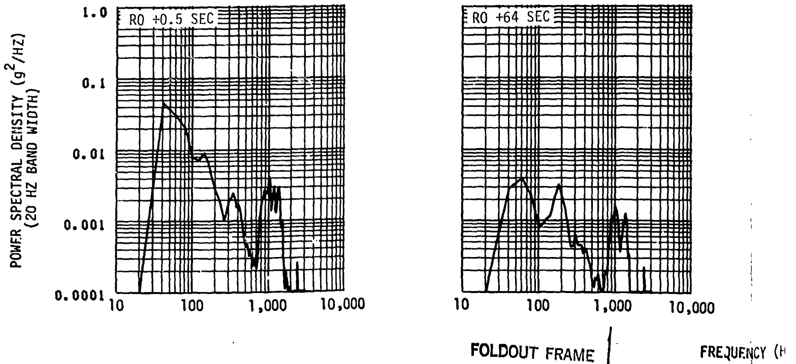
Figure 25-21. Vibration Measured on APS No. 1 Propellant Contr
