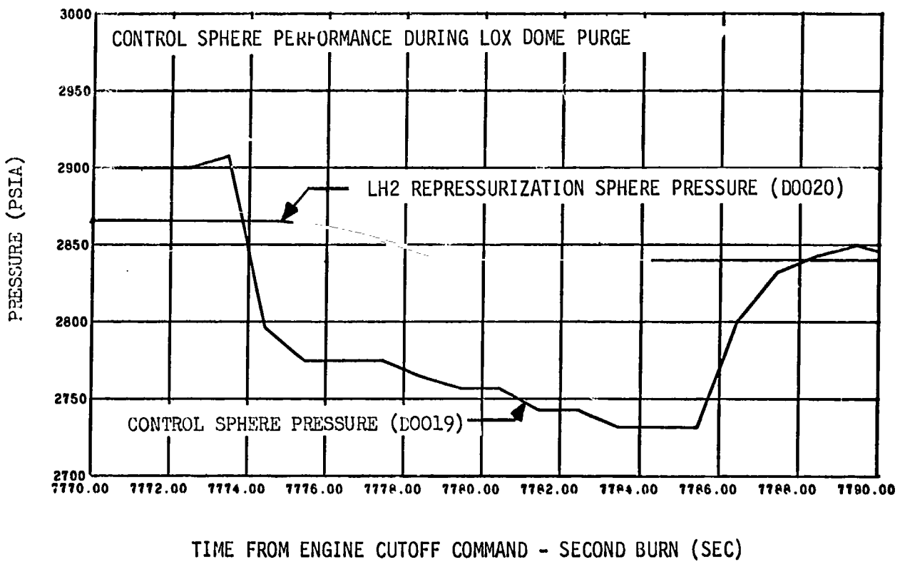
Figure 9-21. Engine Control Sphere Performance During Fuel Lead Experiment (Sheet 1 of 2)
