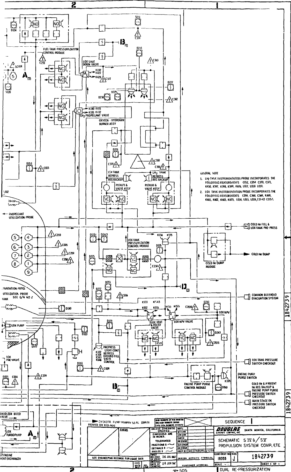
FOLDDOUT FRAME 2 Figure 3-1. Schematic, S-IVB/SV Propulsion - Complete
