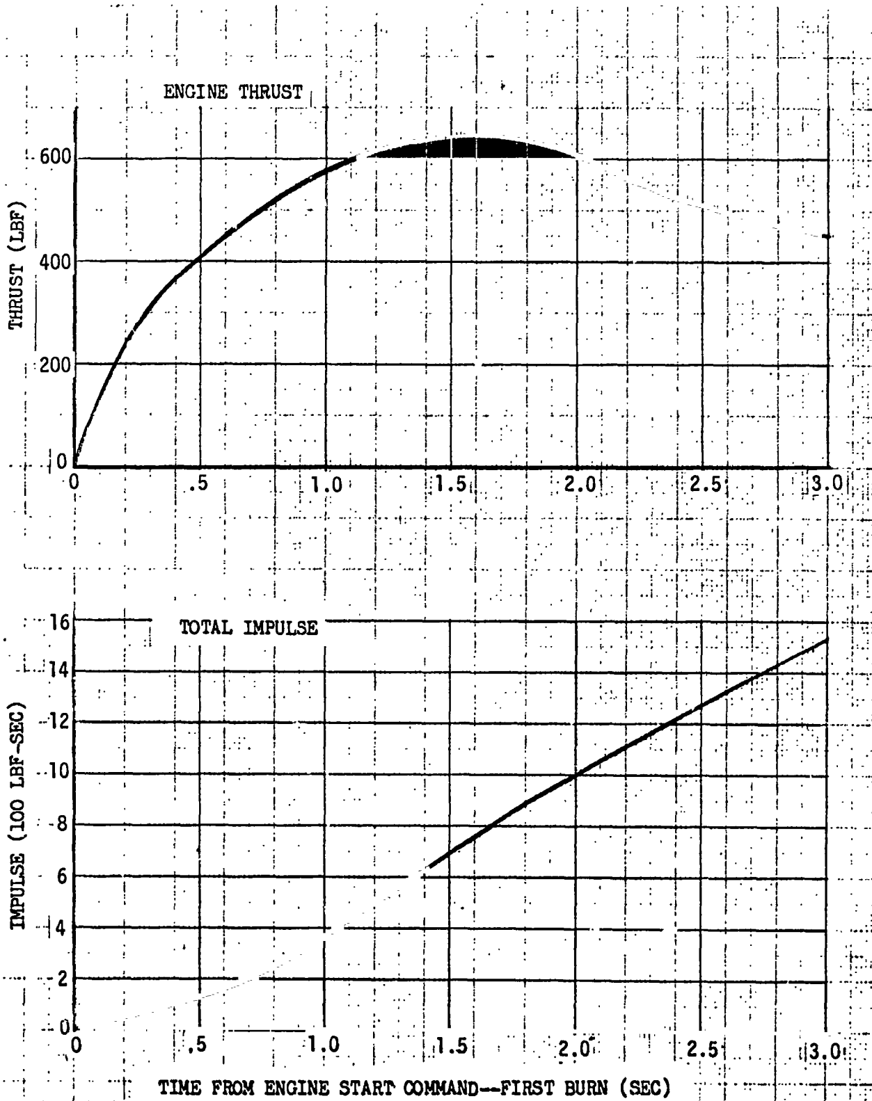
Figure 9-22. Fuel Lead Characteristics--First Burn (Sheet 2 of 2)
