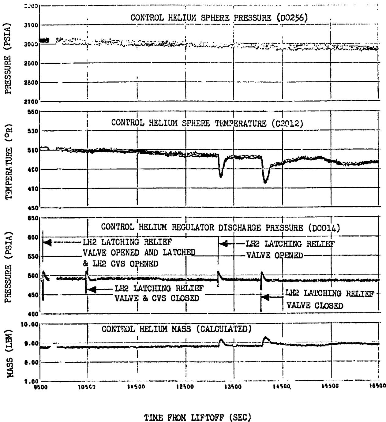
Figure 15-5. Pneumatic Control and Purge System Performance-- Translunar Coast
