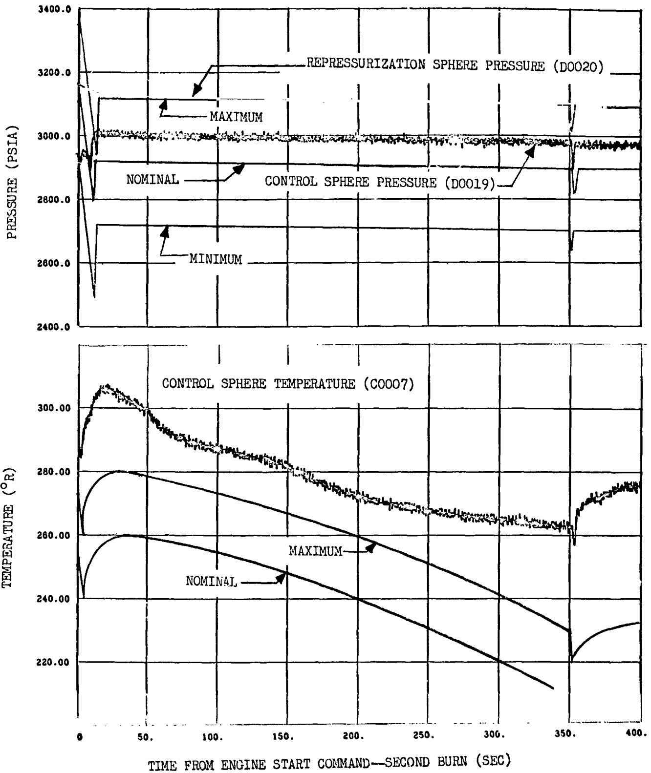
Figure 9-18. Control Sphere Conditions (Sheet 2 of 2)
