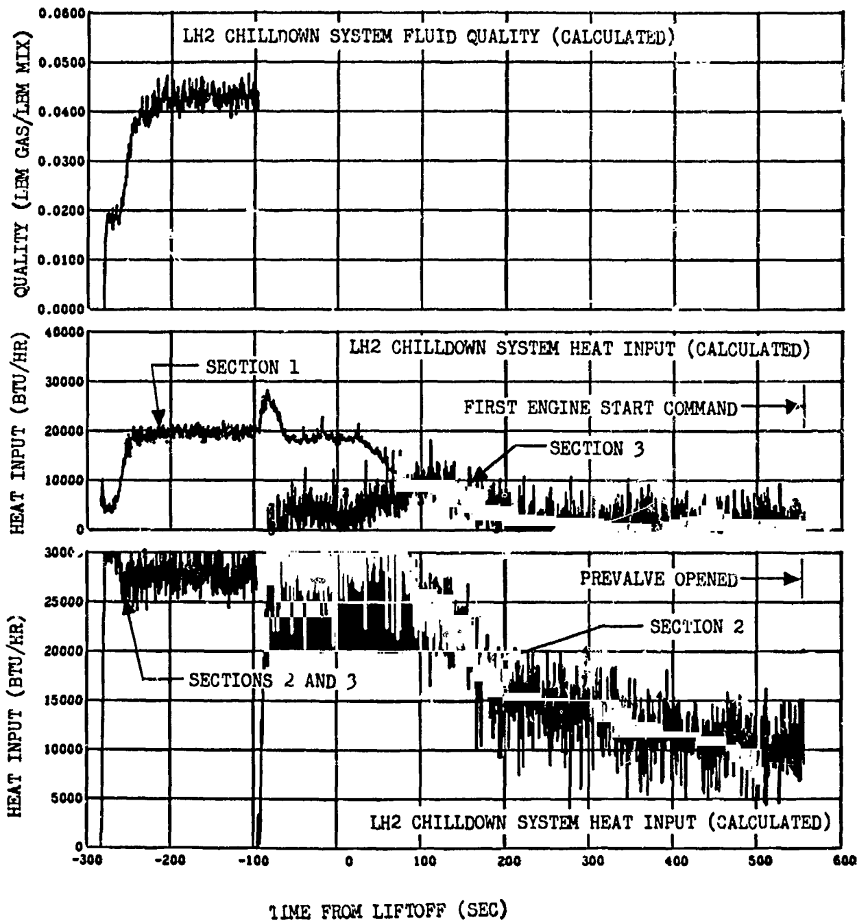
Figure 12-15. LH2 Pump Chilldown--First Burn (Sheet 1 of 2)
