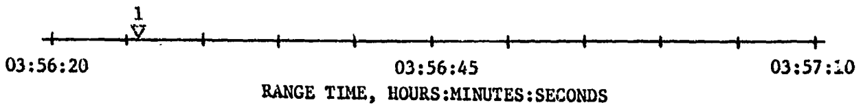
Figure 21-24. Roll Attitude Control During LM Extraction
