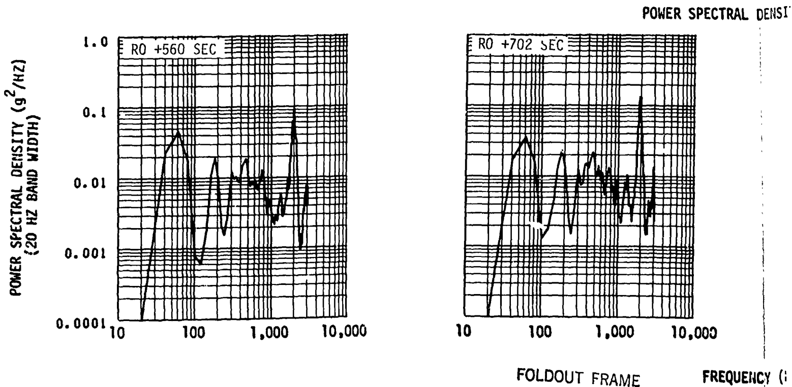
Figure 25-5. Vibration Measured on Main Fuel Valve, Tangent
