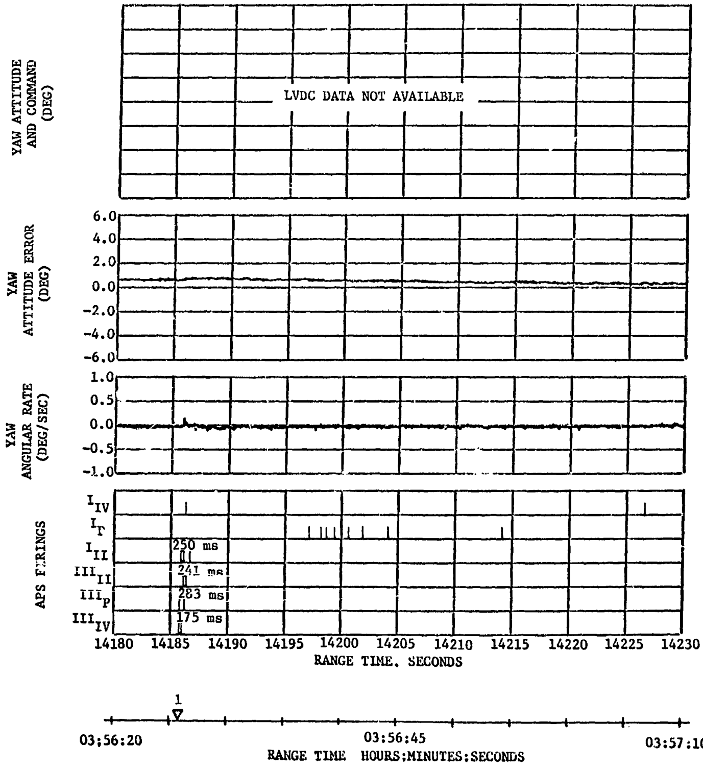
Figure 21-23. Yaw Attitude Control During LM Extraction
