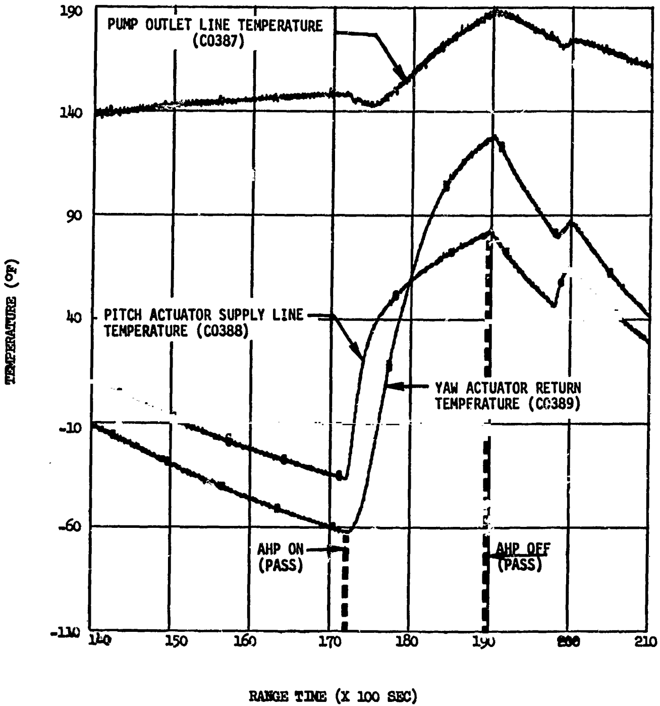
Figure 22-18. Hydraulic System Line Temp - Propellant Dump
