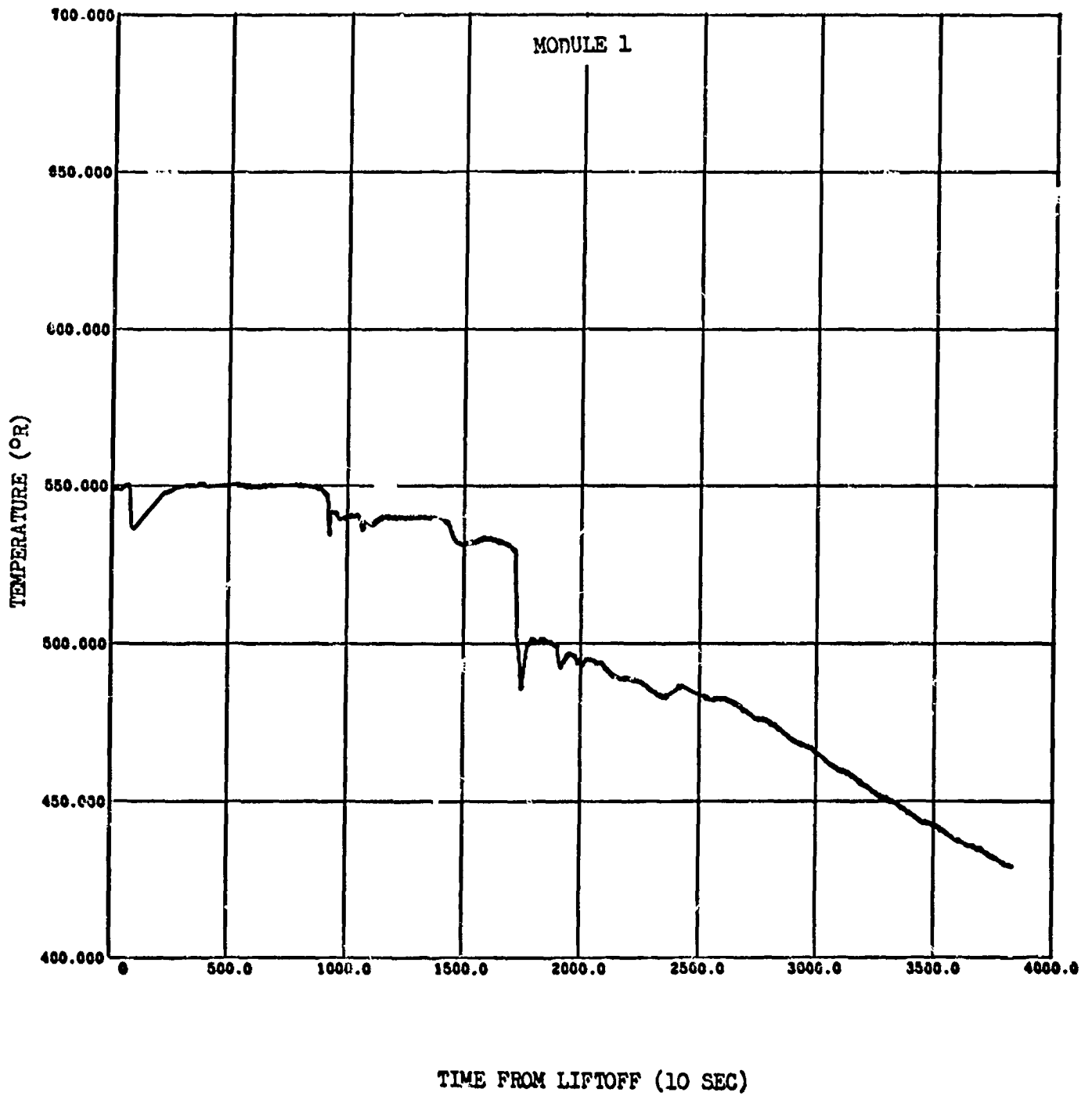
Figure 14-3. APS Module 1 Helium Bottle Temperatures
