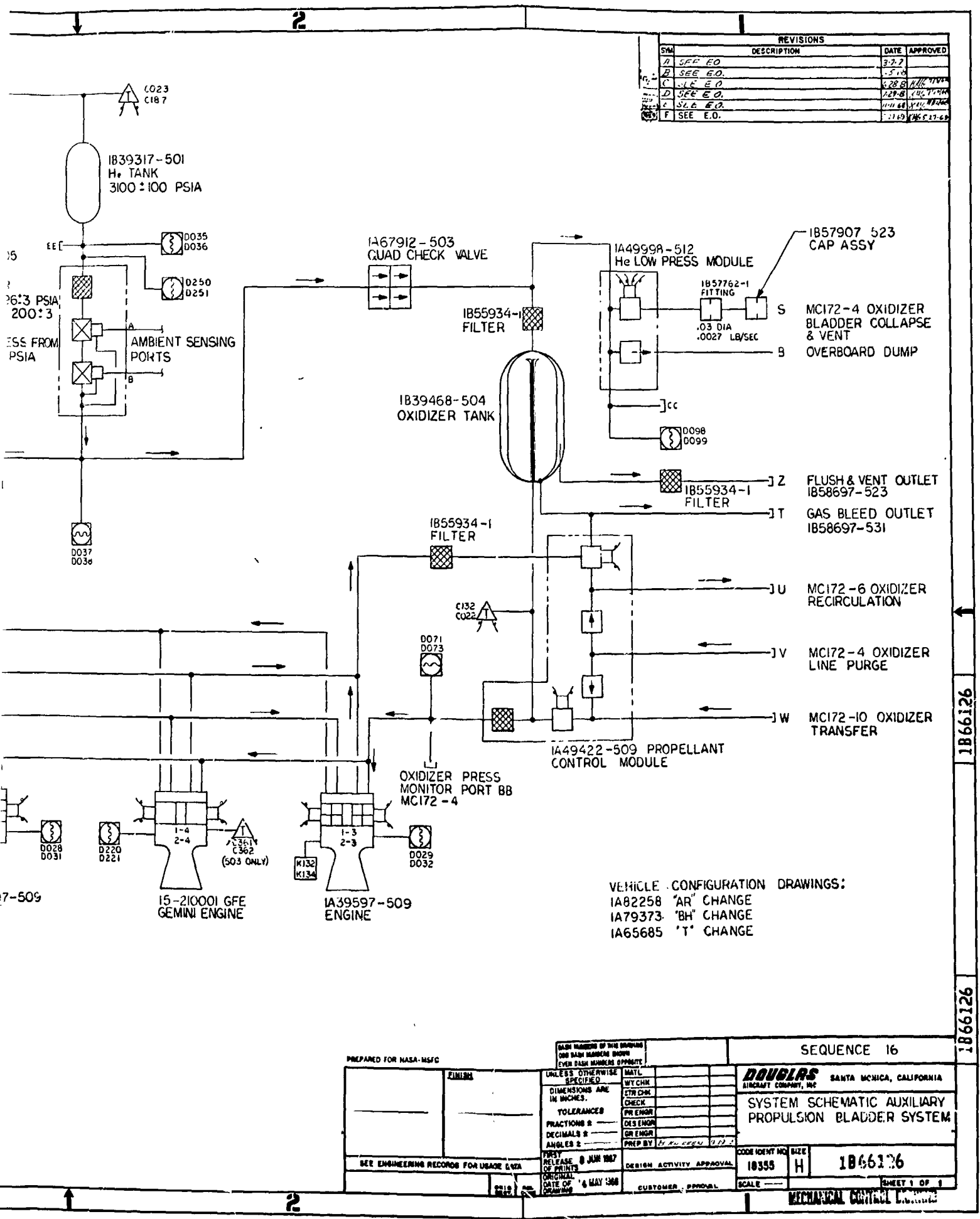
Figure 14-1. Schematic, Auxiliary Propulsion Bladder System FOLDOUT FRAME 14-11
