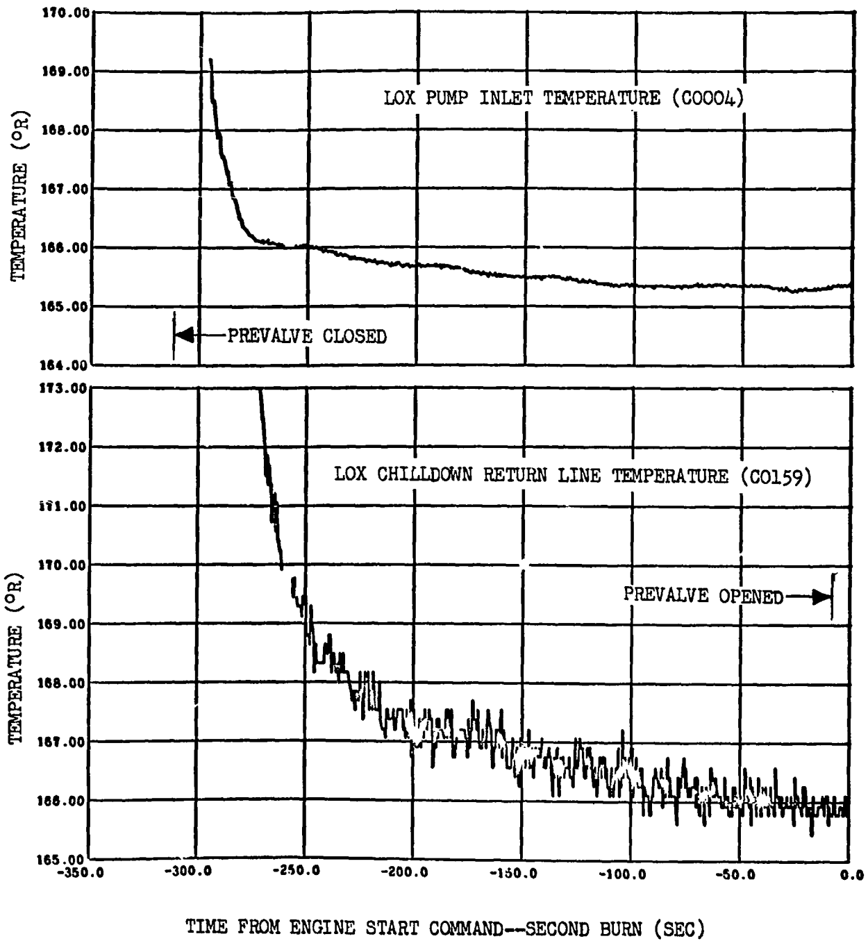
Figure 11-17. LOX Pump Chilldown System Operation--Second Burn (Sheet 2 of 2)
