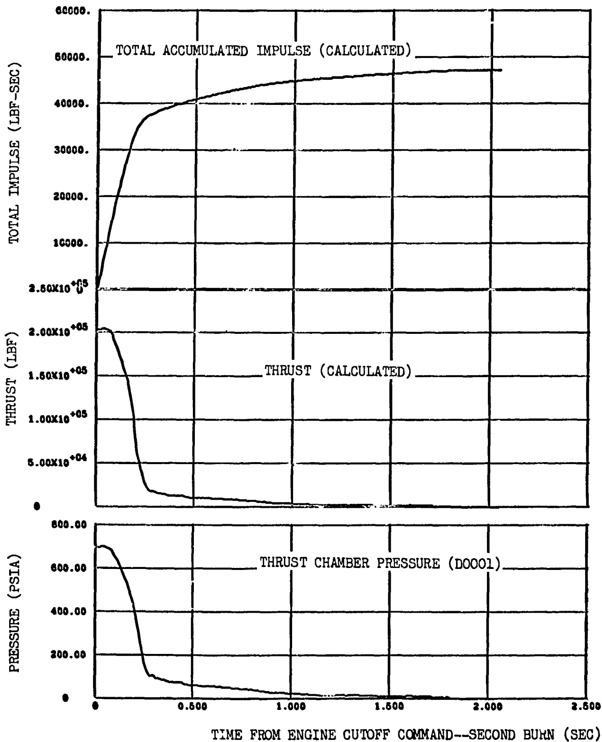
Figure 9-36. Engine Cutoff Transient Characteristics (Sheet 2 of 2)
