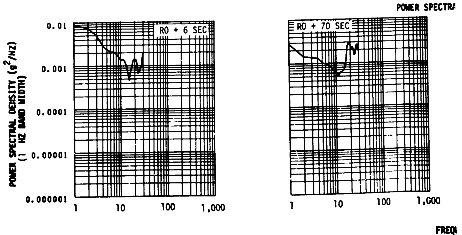
Figure 25-36. Forward Skirt Body Bending,
