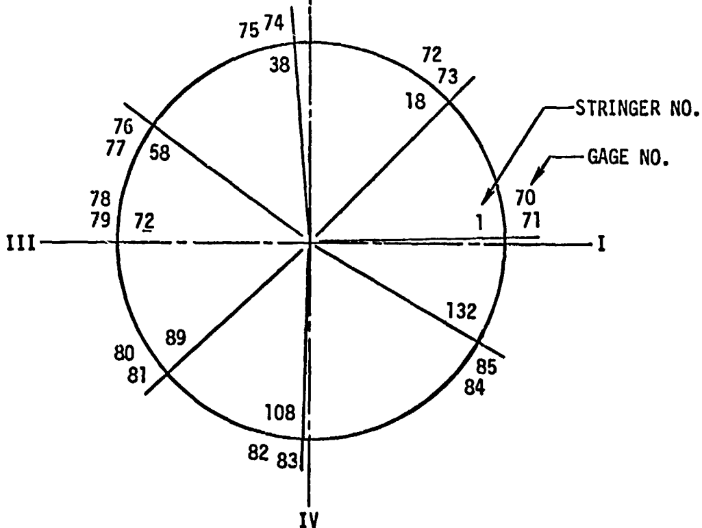
Figure 23-1. Stringer Strain Gage Locations
