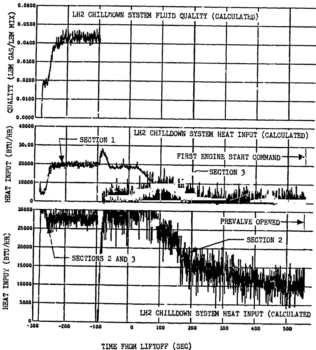
Figure 12-15. LH2 Pump Chilldown--First Burn (Sheet 1 of 2)
