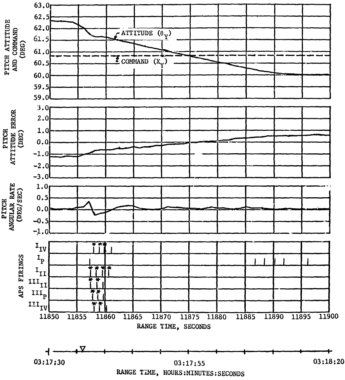
Figure 21-19. Pitch Attitude Control During Hard Docking
