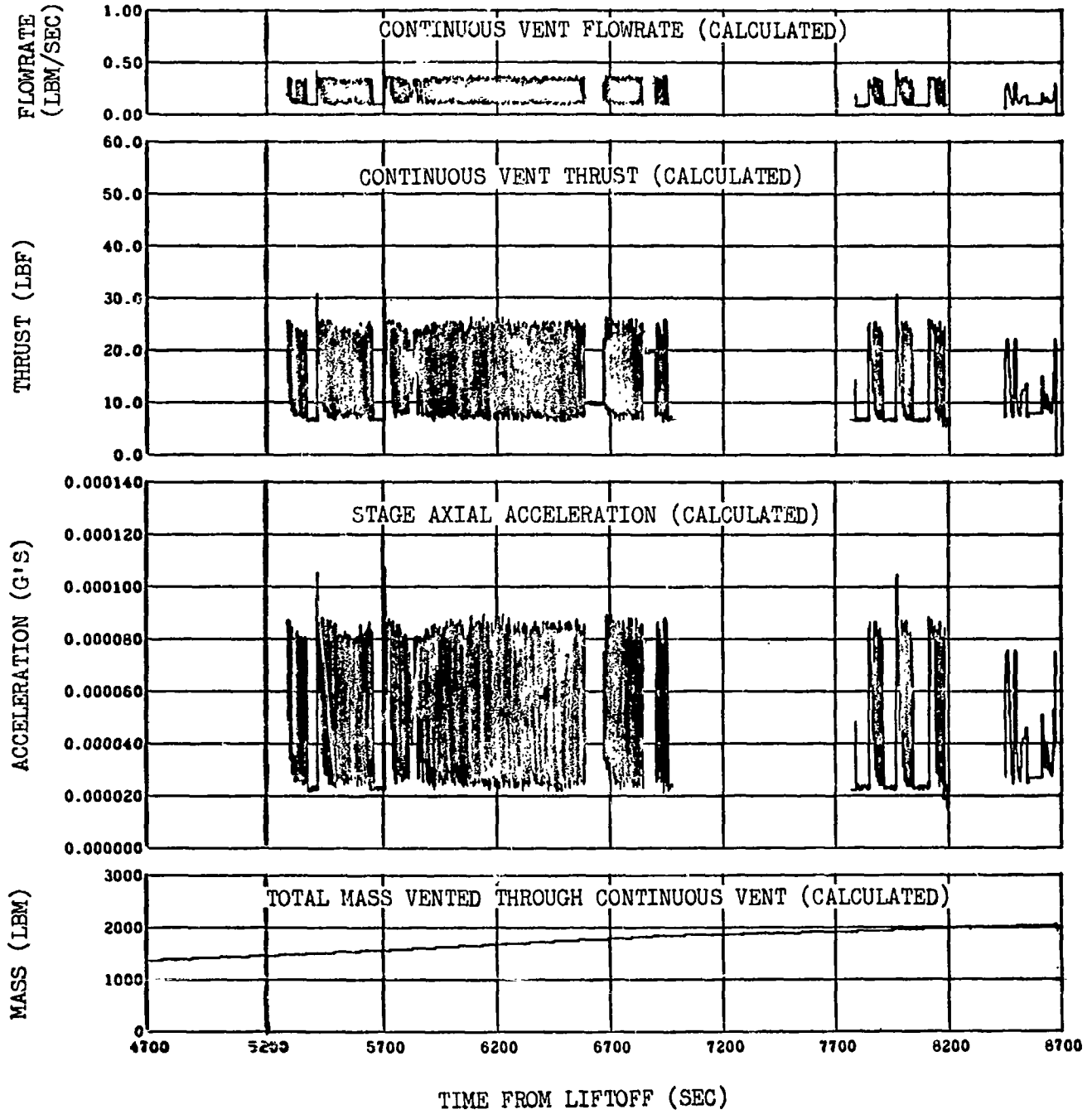
Figure 12-8. LH2 Tank Continuous Vent System Performance-- Earth Orbit (Sheet 2 of 2)
