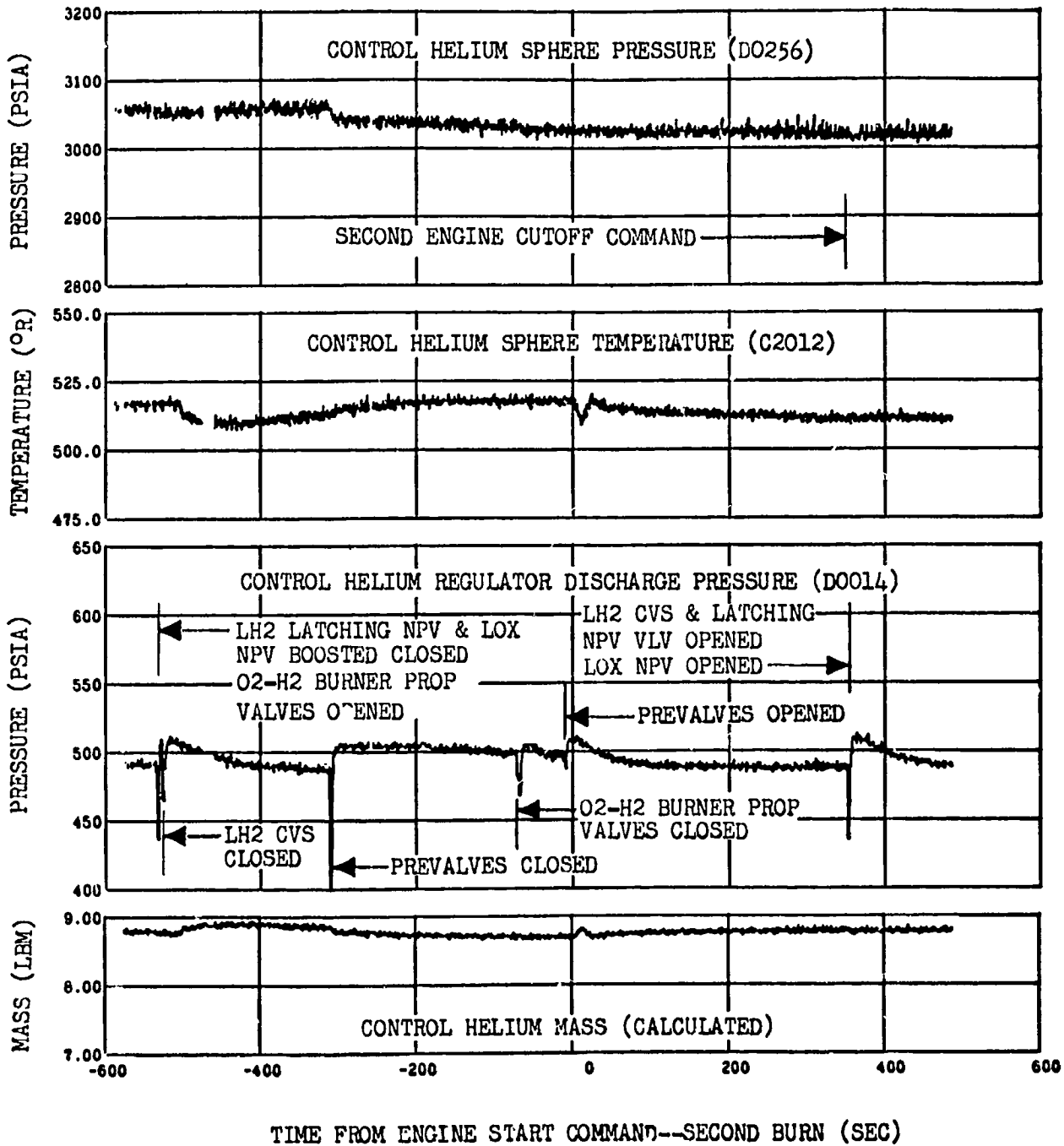
Figure 15-4. Pneumatic Control and Purge System Performance--Second Burn
