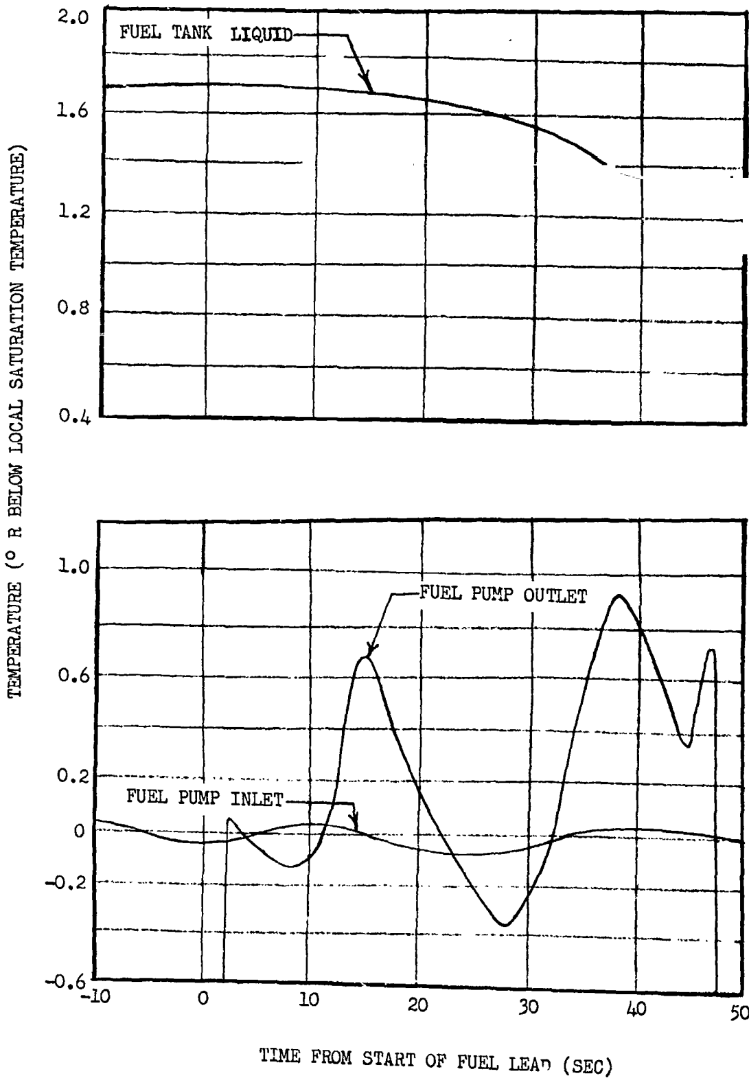
Figure 9-55. Fuel Lead Subcooling
