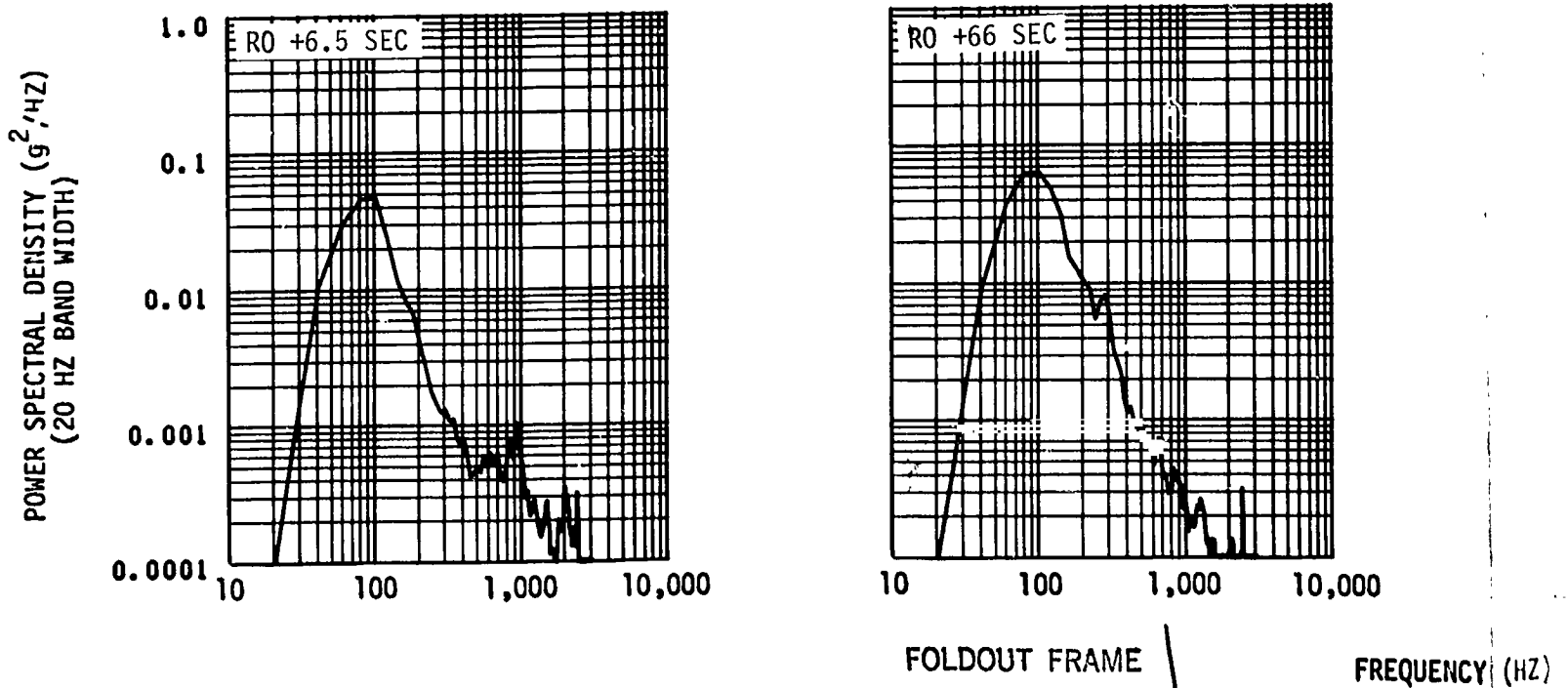
Figure 25-17. Vibration Measured on LH2 Feedline at Tan:
