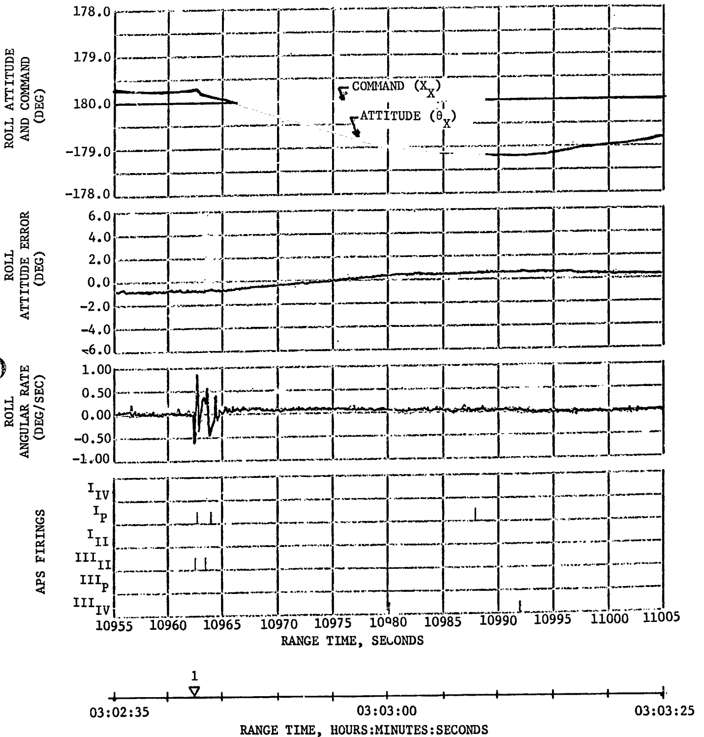
Figure 21-18. Roll Attitude Control During S-IVB/CSM Separation
