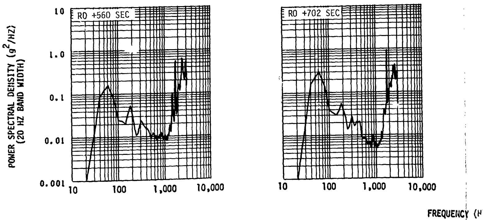
Figure 25-3. Vibration Measured at LH2 Turbopump, Radial FOLDOUT FRAME
