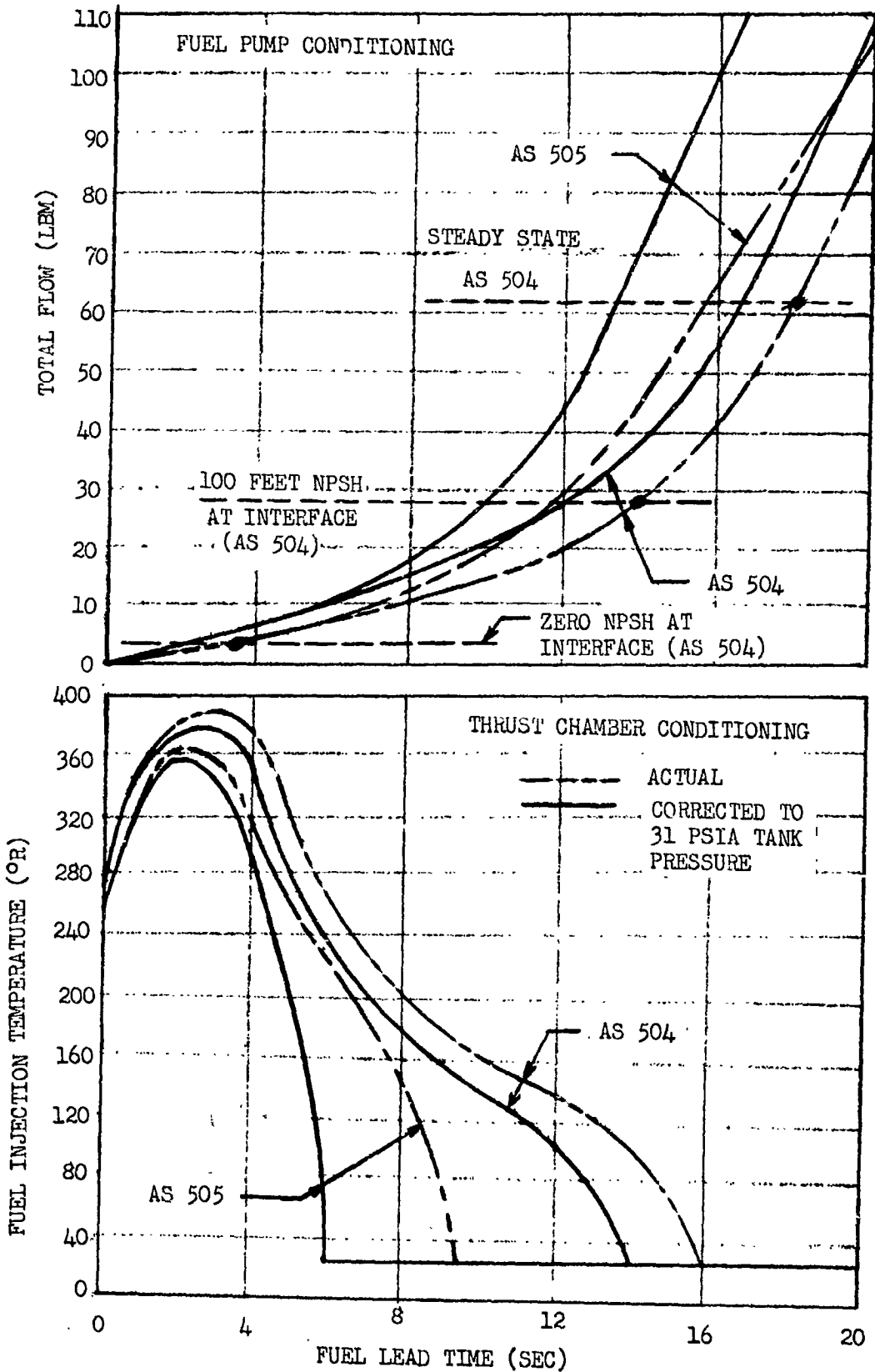
Figure 9-42. Propellant Lead Experiment Chilldown Characteristics
