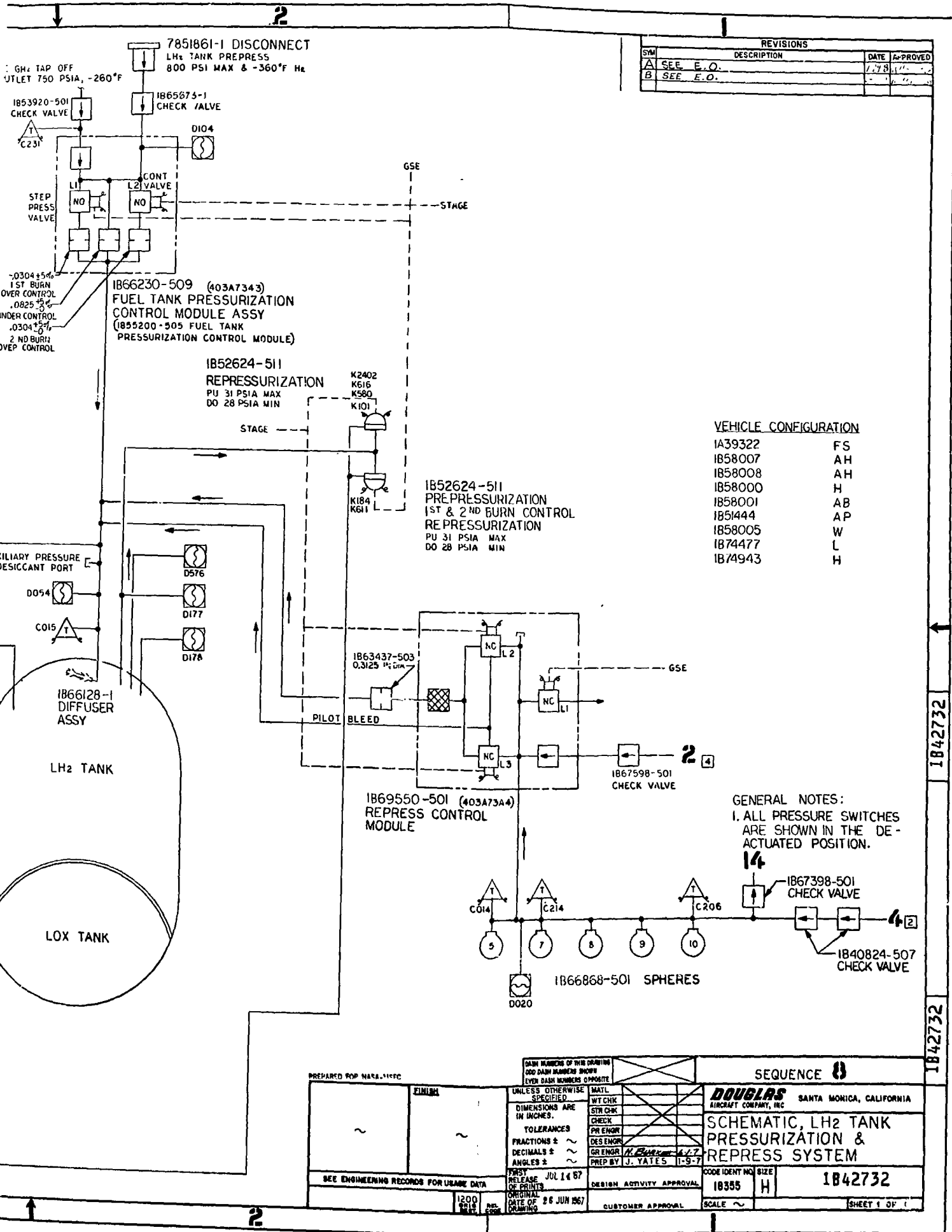
Figure 12-1. Schematic, LH2 Tank Pressurization & Repress System FOLDOUT FRAME 2 12-15
