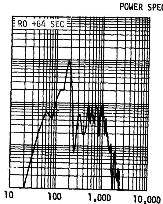
Figure 25-23. Vibration Measured at APS No. 1 Helium Regulat
