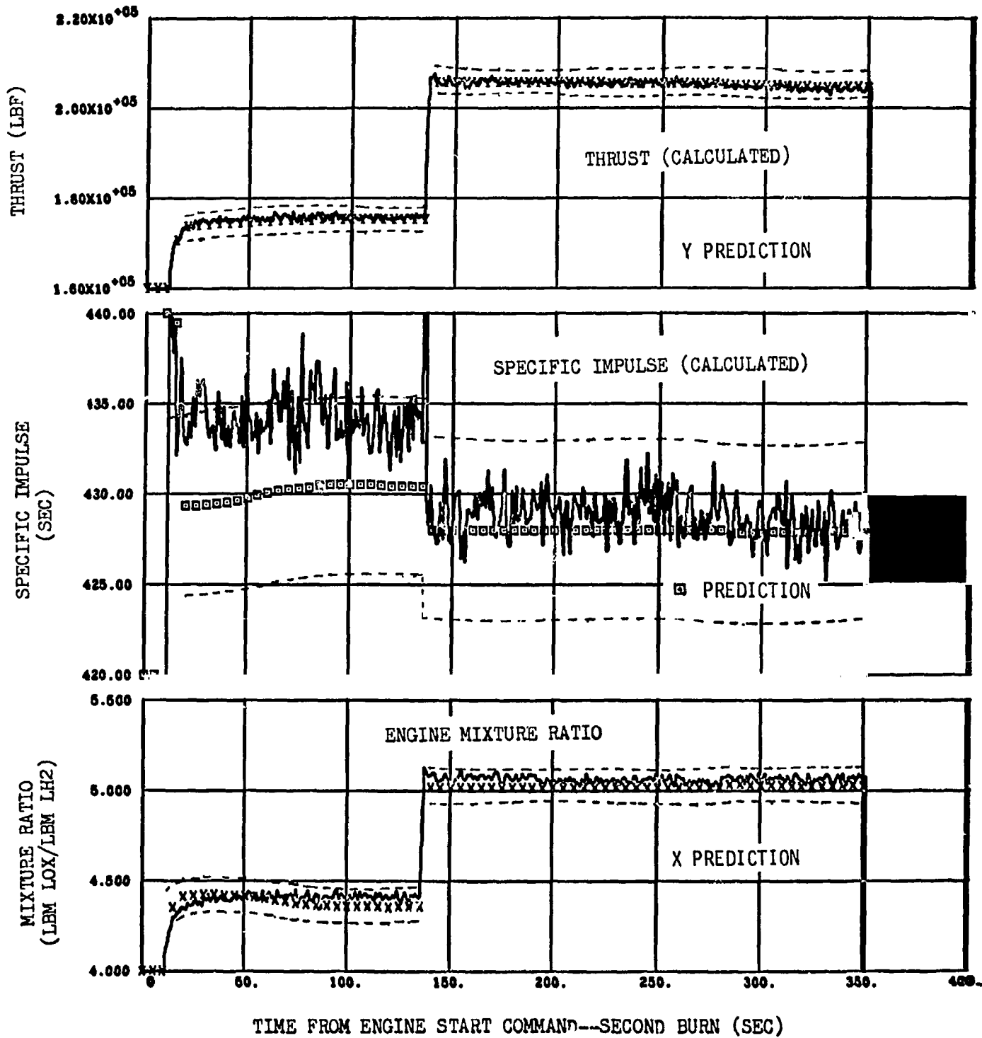
Figure 9-35. Engine Steady State Performance--Second Burn (Sheet 1 of 3)
