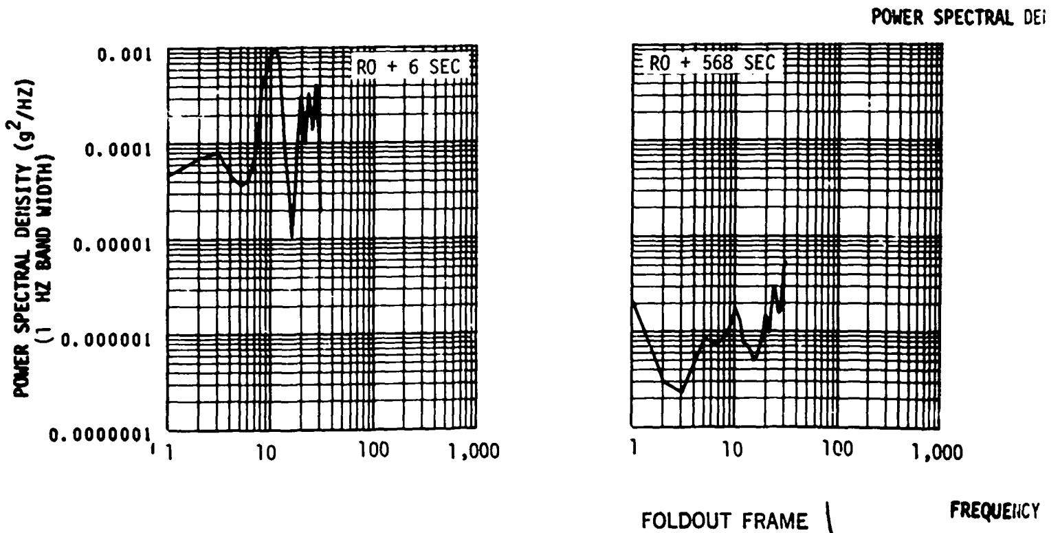
Figure 25-39. Acceleration Measured on Gimbal Block.
