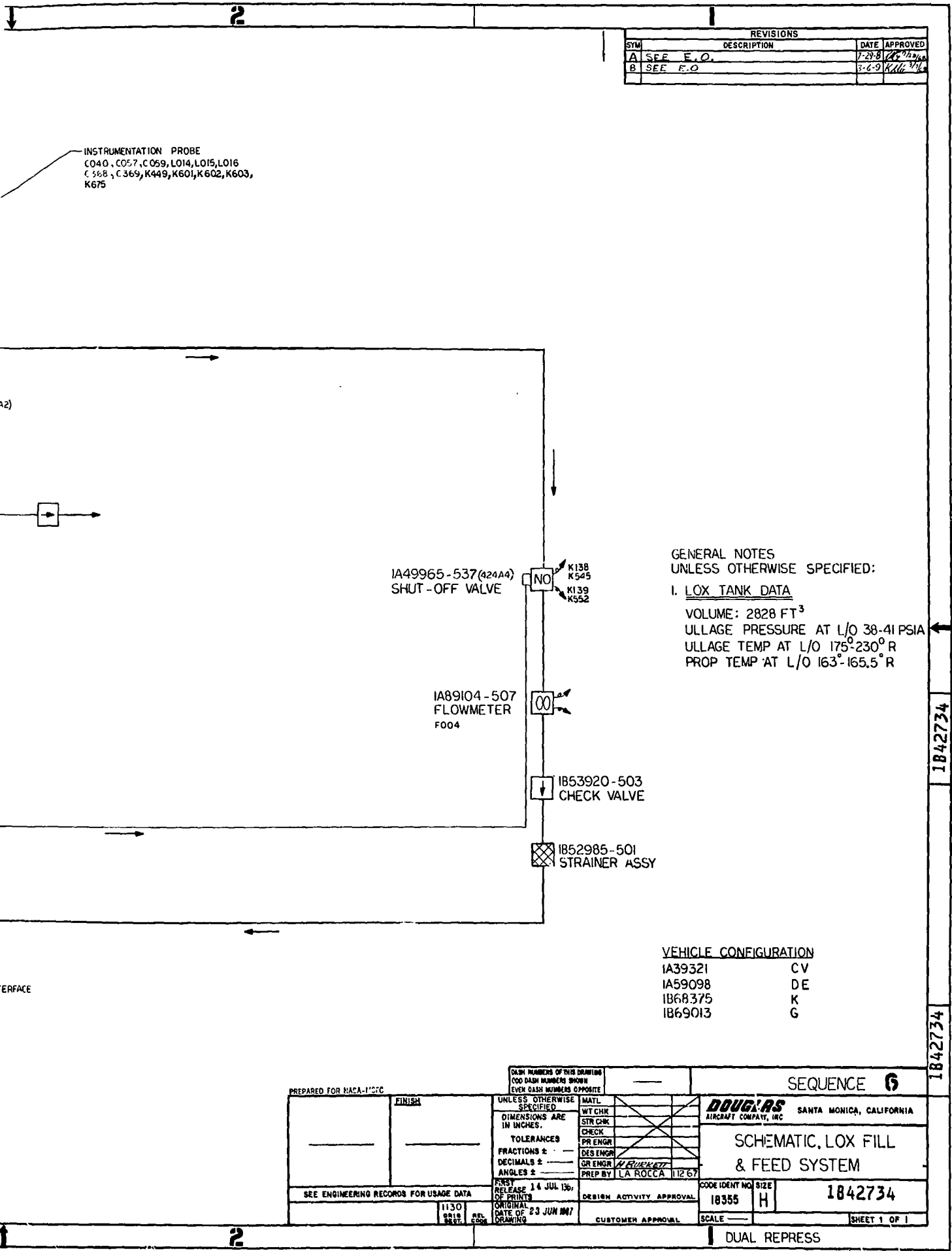
FOLDOUT FRAME 2 Figure 11-19. Schematic, LOX Fill & Feed System
