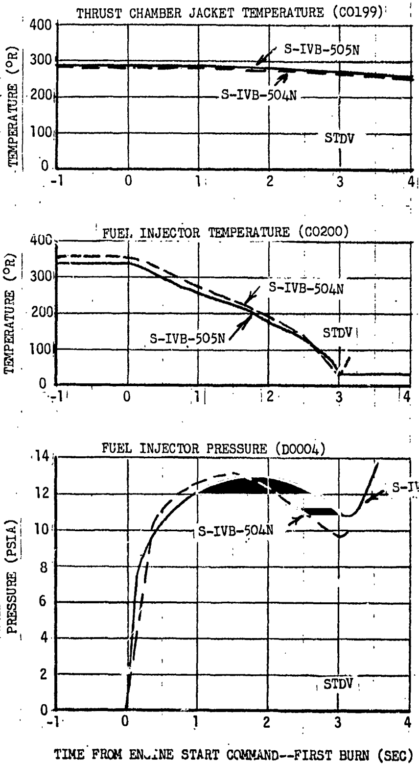
Figure 9-8. Fuel Lead--First Burn
