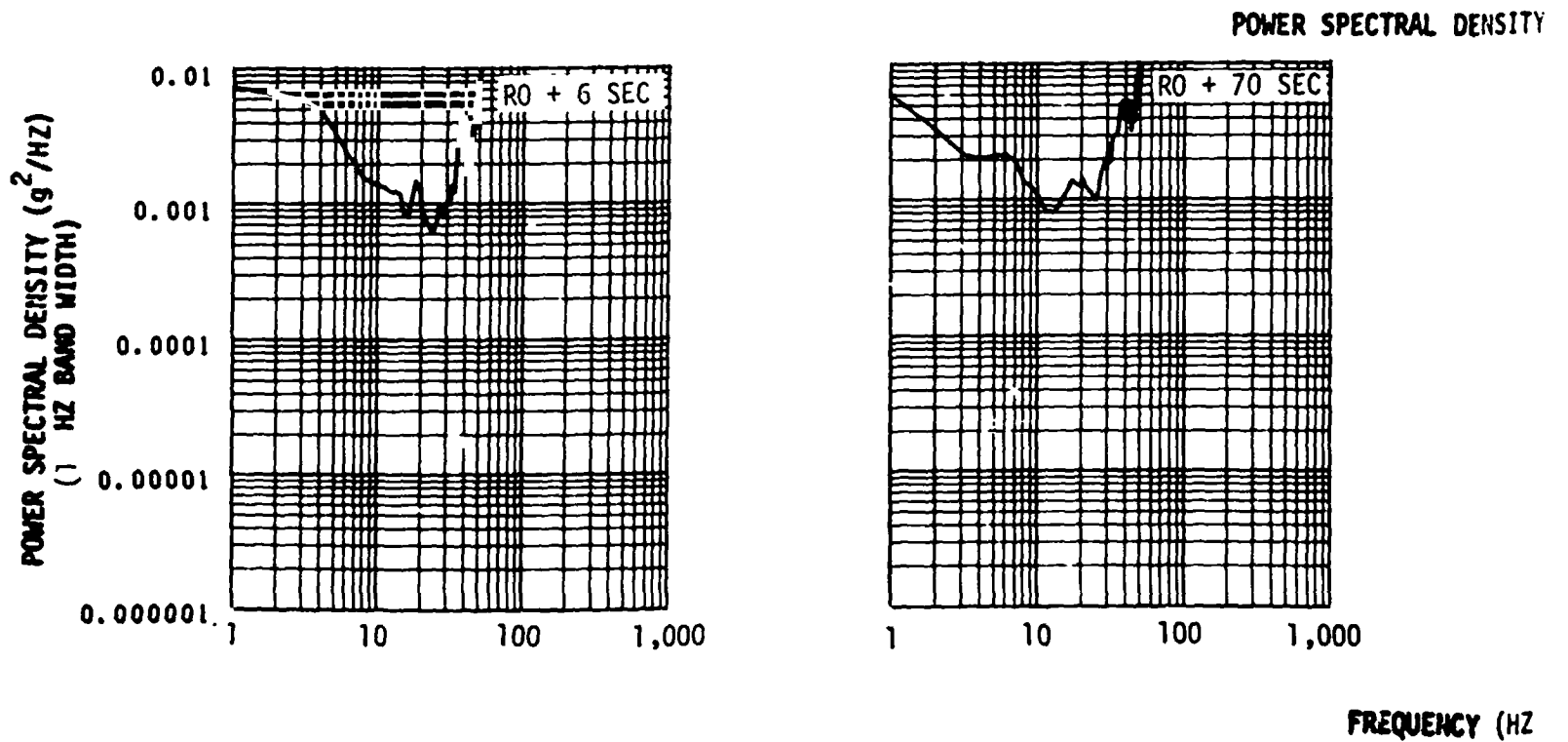
Figure 25-35. Forward Skirt Body Bending, Pitch Direct
