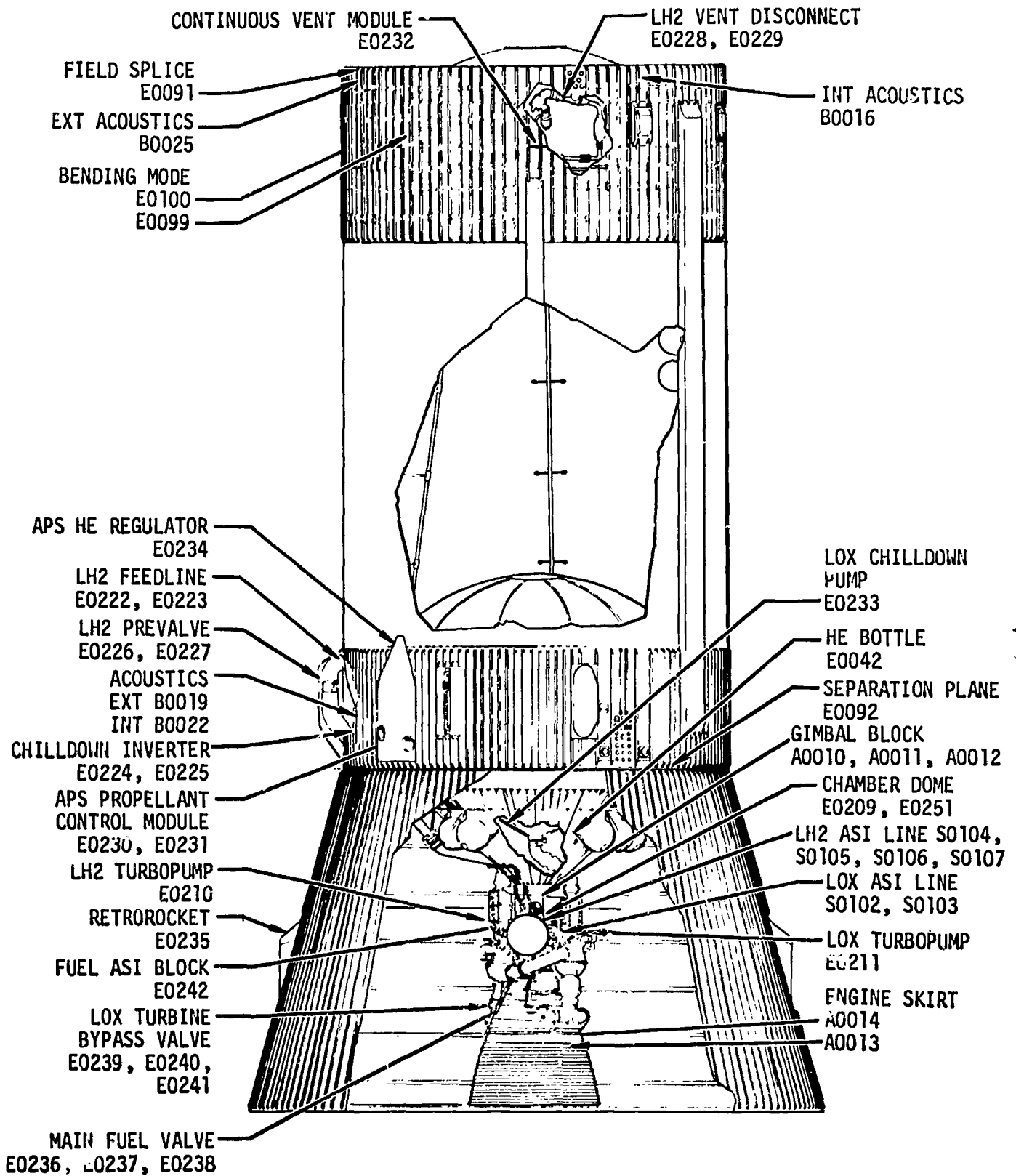
Figure 25-1. Measurement Locations
