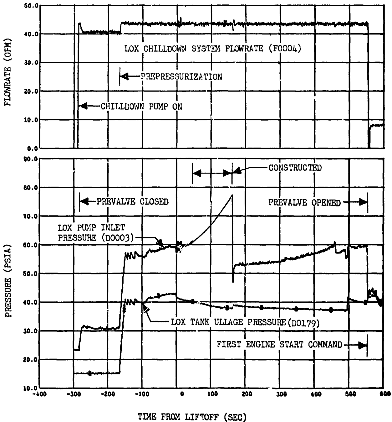
Figure 11-15. LOX Pump Chilldown System Operation-- Boost and First Burn (Sheet 1 of 2)
