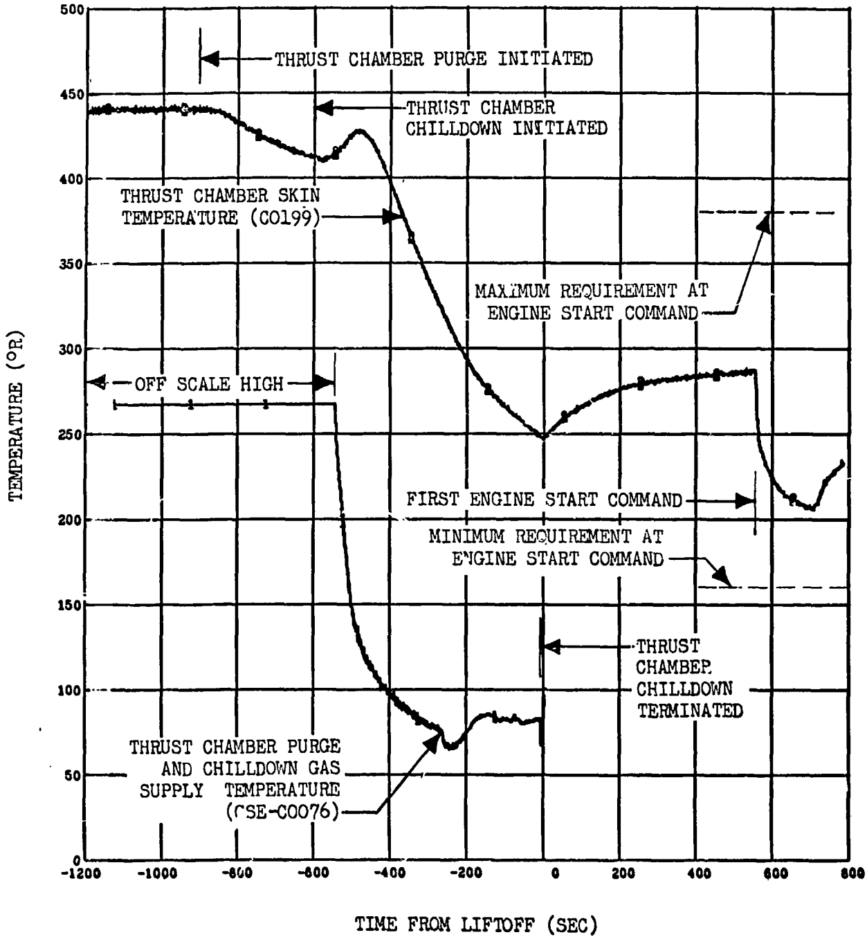
Figure 9-7. Thrust Chamber Chilledown--First Burn
