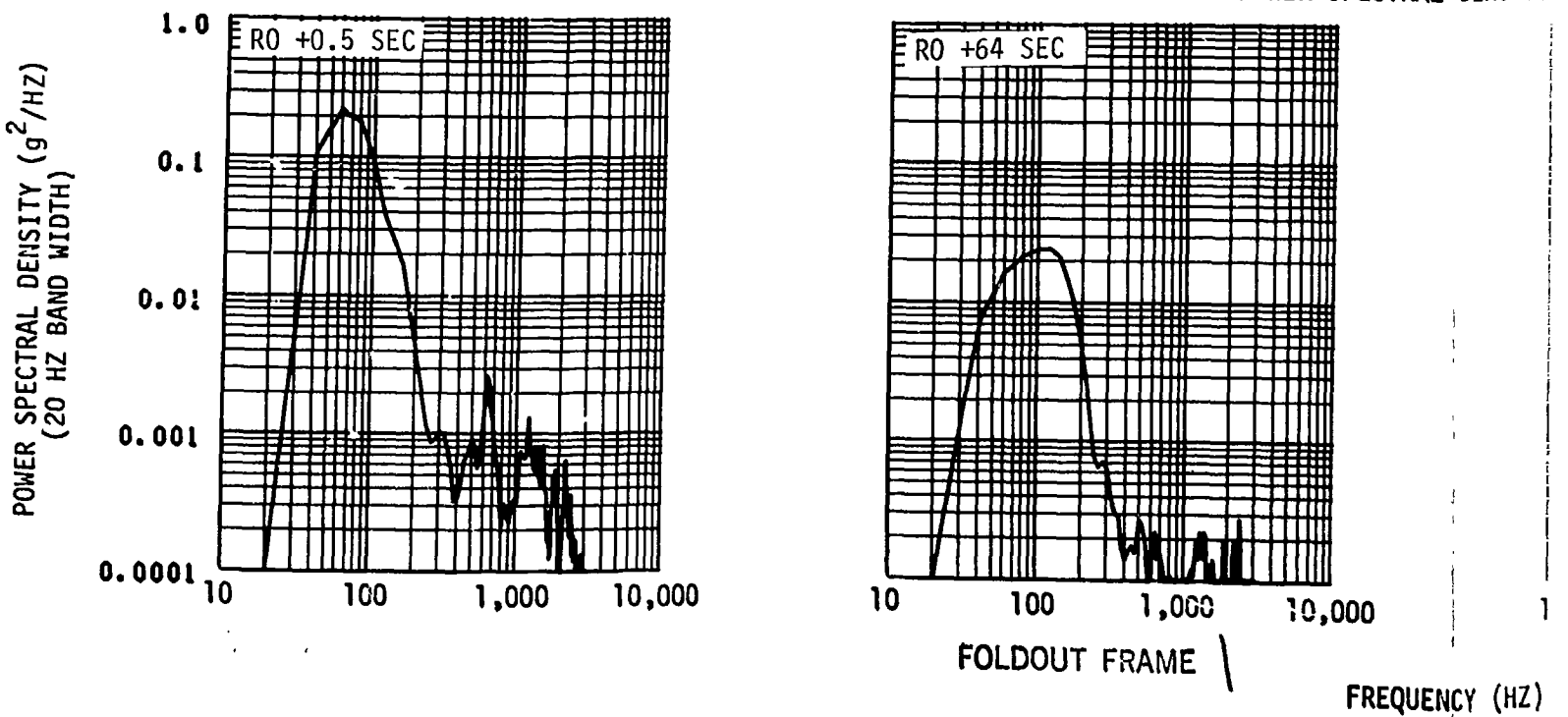
Figure 25-15. Vibration Measured at LOX Chilldown Pump,
