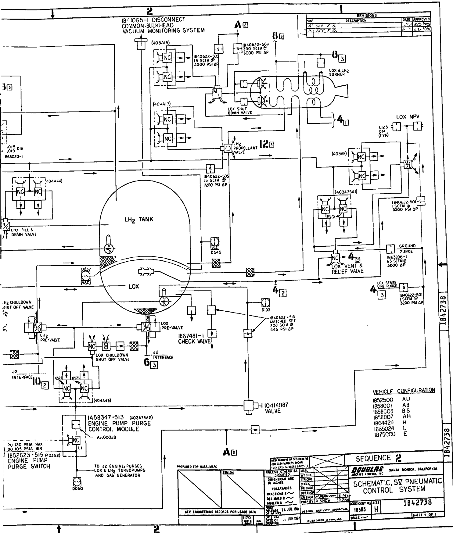
Figure 15-1. Schematic, SV Pneumatic Control System EOLDOUT FRAME 2
