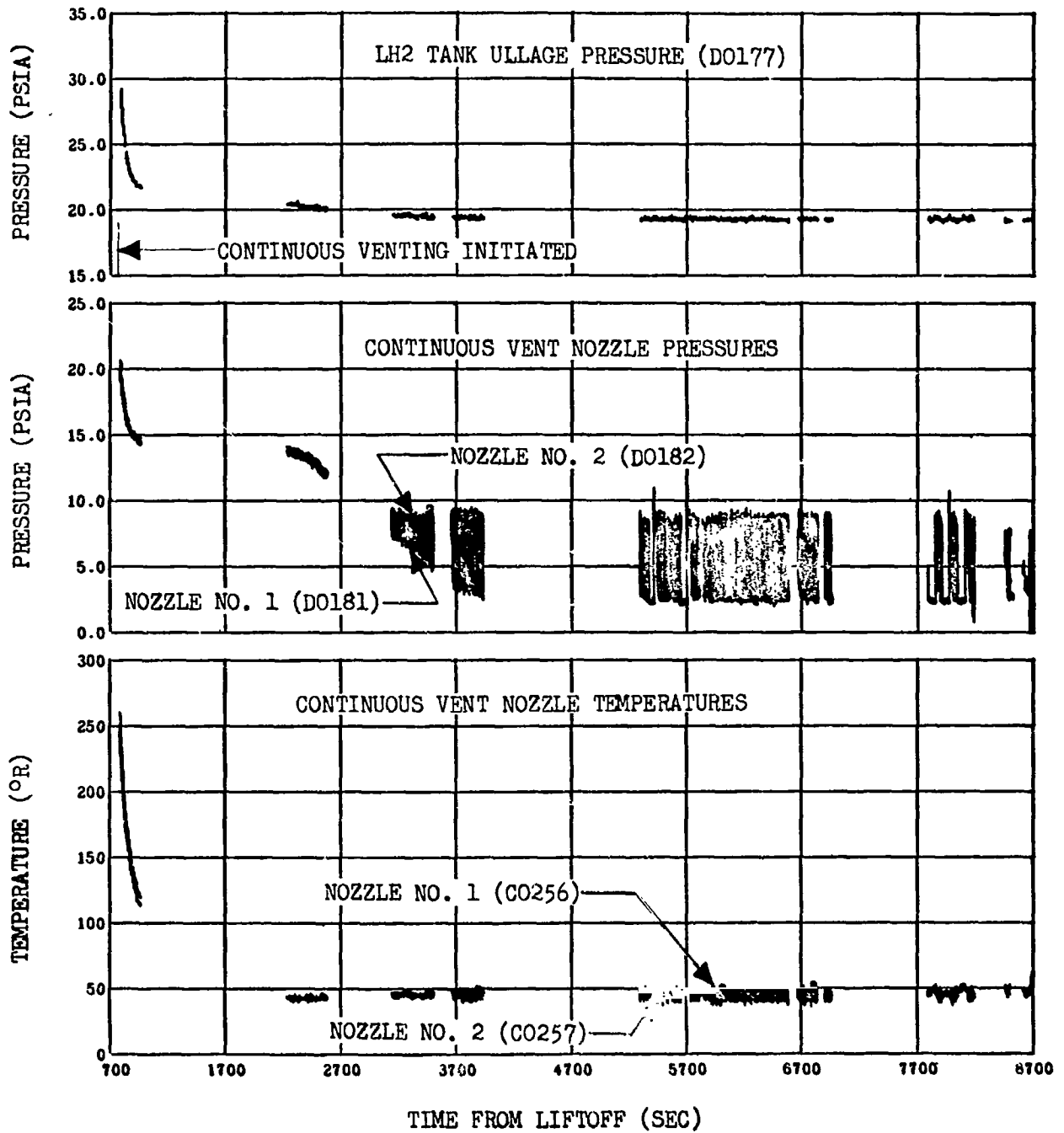
Figure 12-7. LH2 Tank Continuous Vent System Operation-- Earth Orbit
