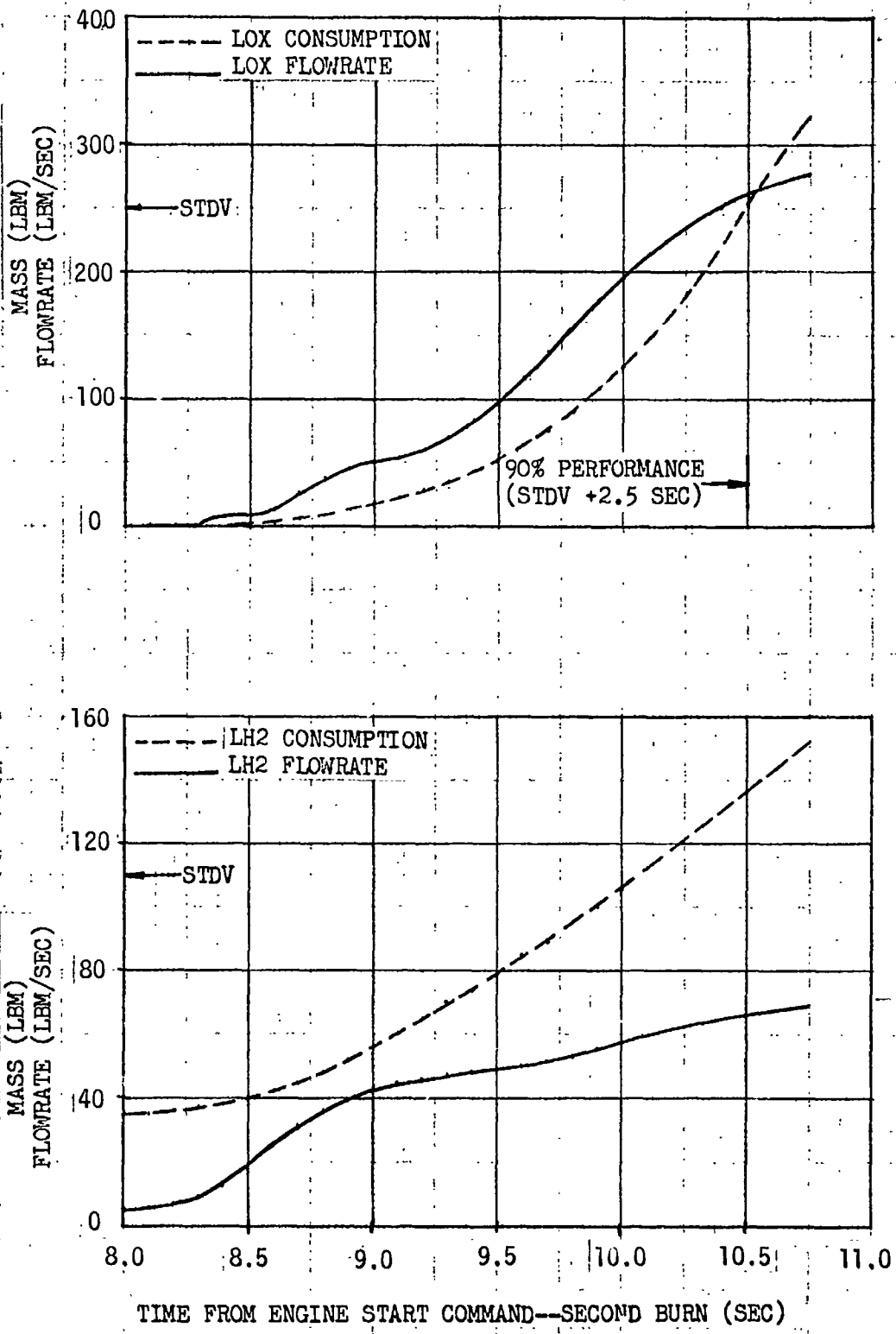
Figure 9-26. LOX and LH2 Consumption During Start Transient (Sheet 2 of 2)
