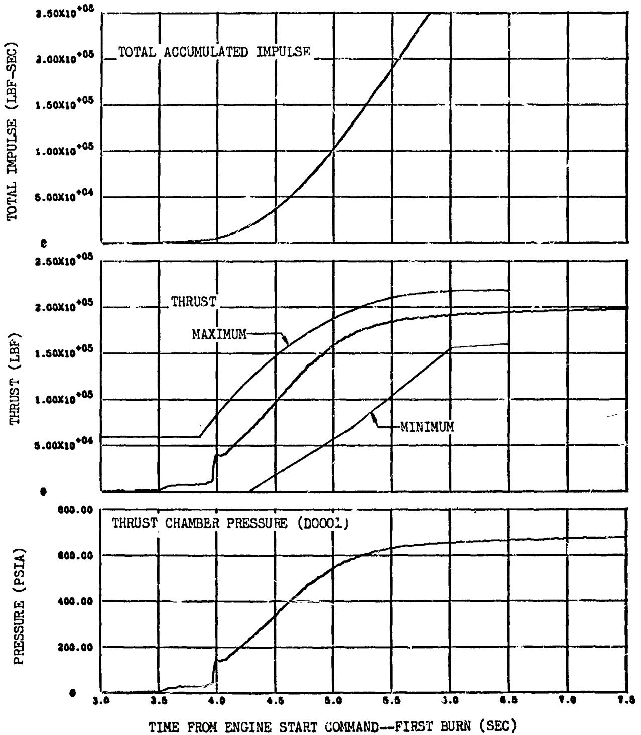
Figure 9-25. Engine Start Transient Characteristics (Sheet 1 of 2)
