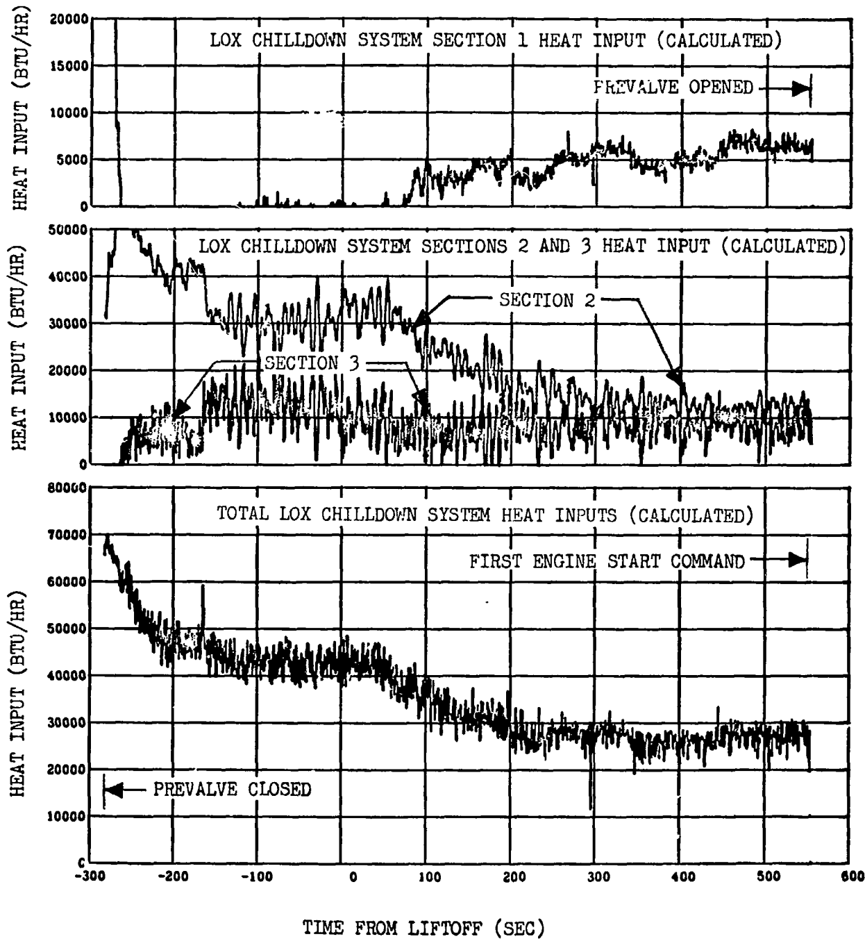
Figure 11-16. LOX Pump Chilldown System Performance-- Boost and First Burn (Sheet 2 of 2)
