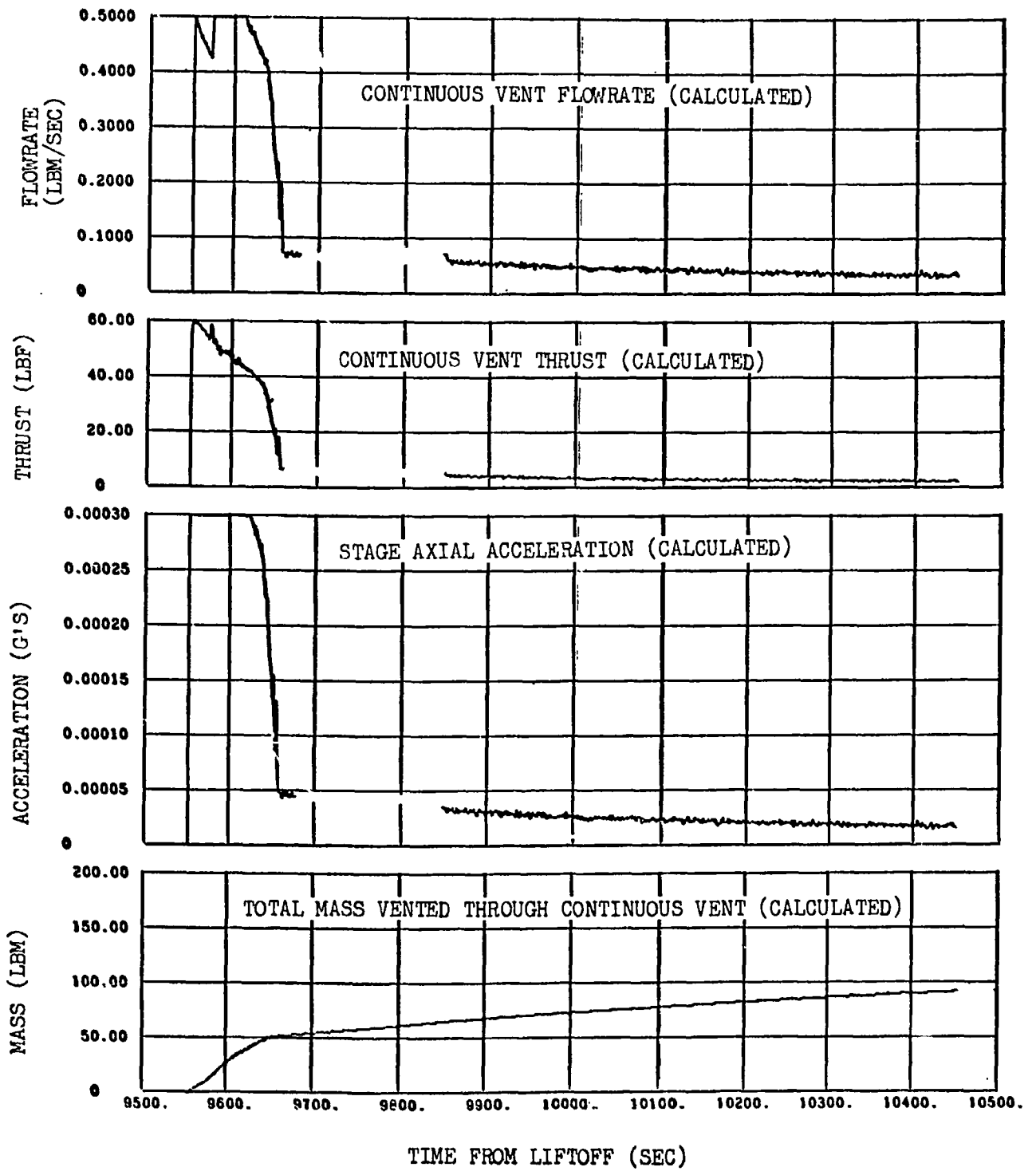
Figure 12-10. LH2 Tank Continuous Vent System Performance--- Translunar Coast
