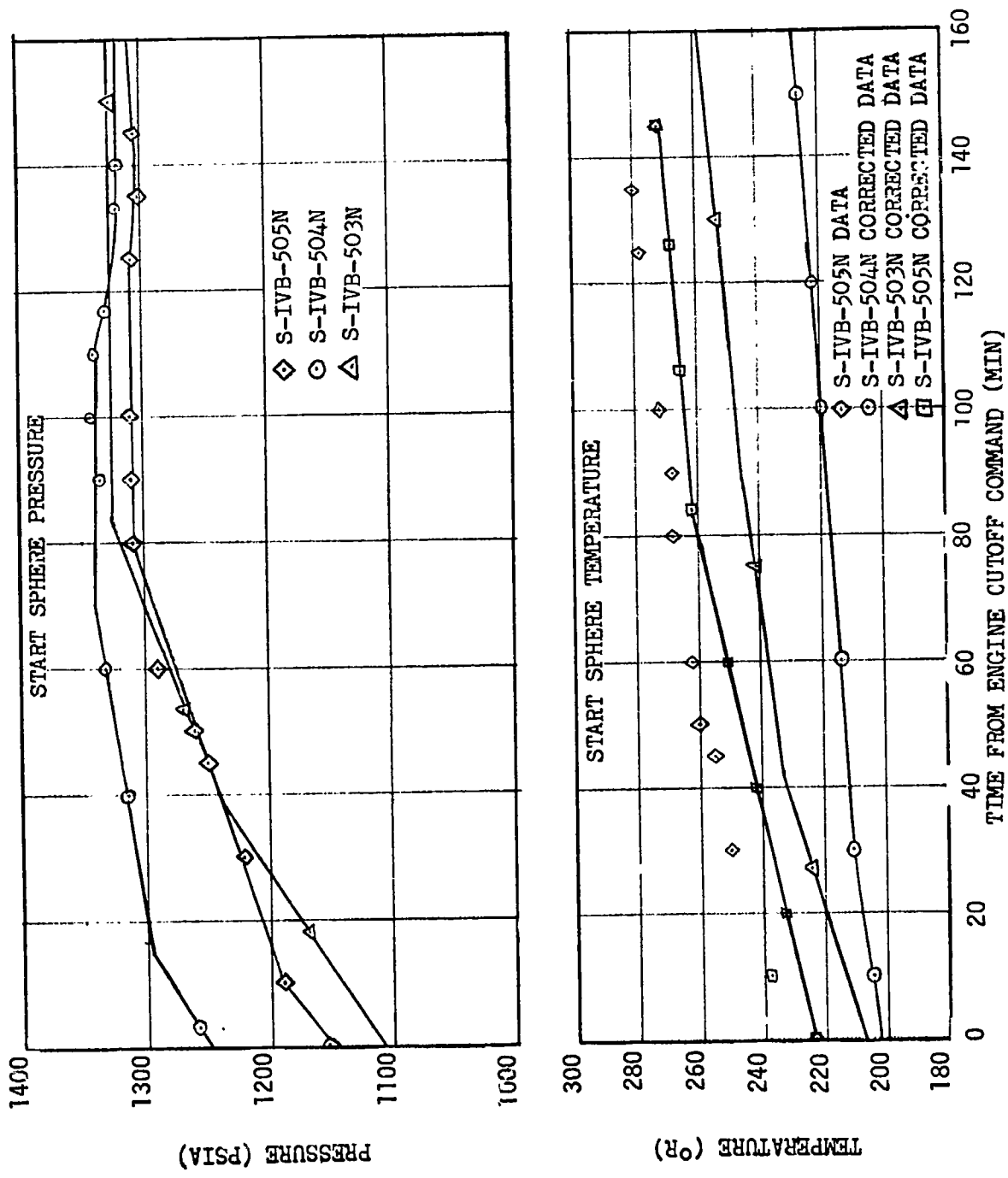
Figure 9-14. Start Sphere Conditions--Earth Orbit
