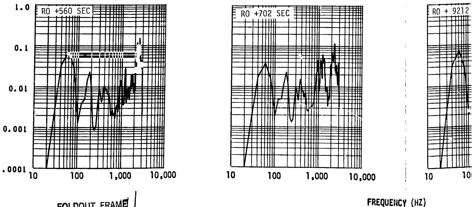
Figure 25-9. Vibration Measured on LOX Turbine Bypass Valve, Radial Directi
