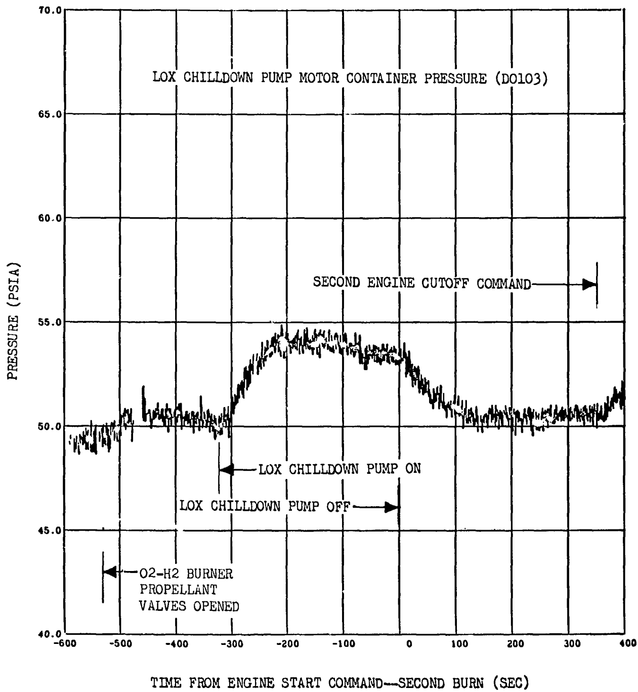
Figure 15-8. LOX Chilldown Pump Motor Container Purge Performance-- Second Burn
