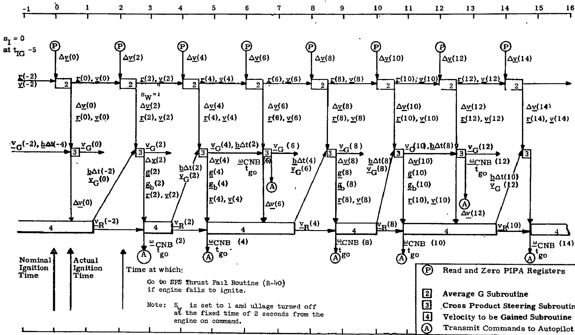
Figure 5.1-4. Normal Lambert Aim Point Subroutine Sequencing (Maneuver time greater than 6 sec) for SPS Maneuvers
