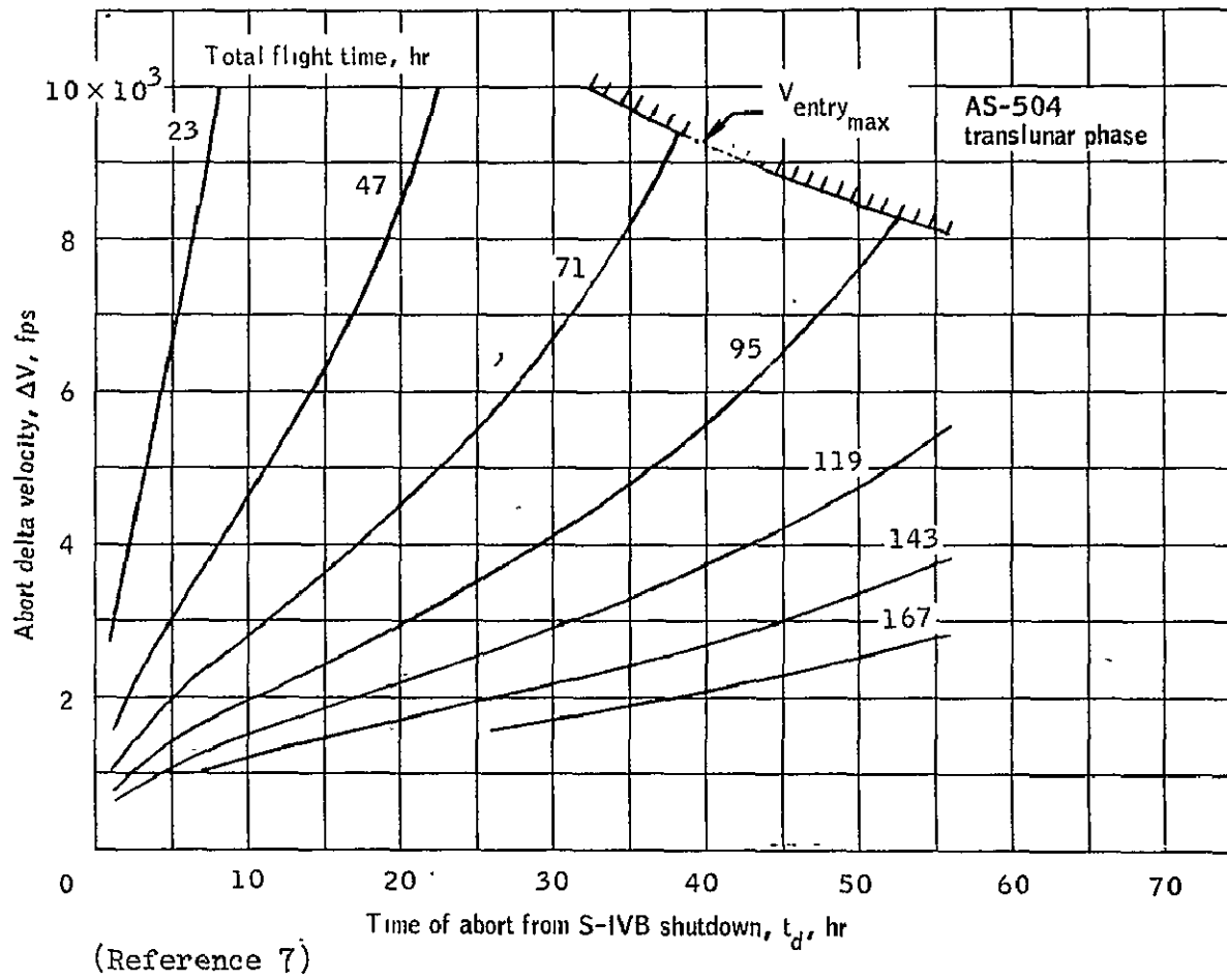
Figure 3.3-7. - Abort delta velocity and flight time required for contingency landing area C, CLA C.
