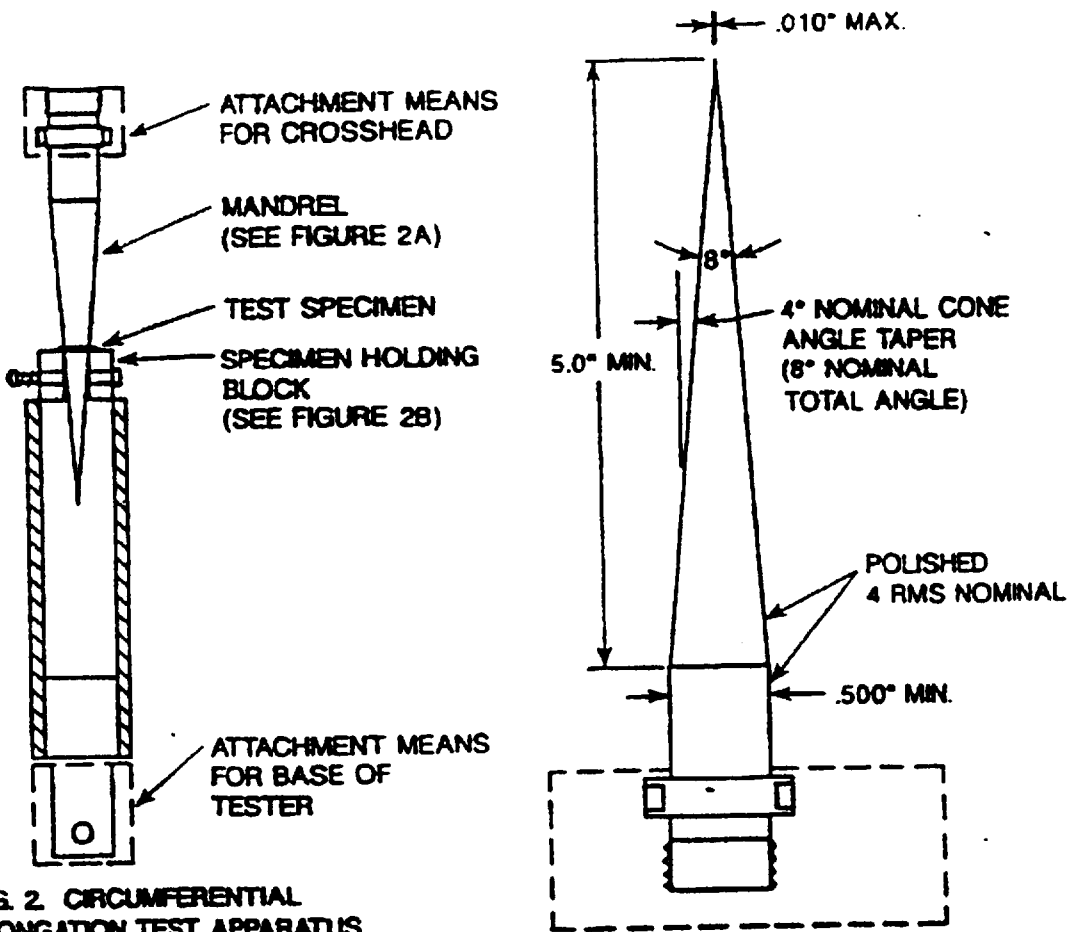
FIG. 2A. TEST MANDREL FOR CIRCUMFERENTIAL ELONGATION
