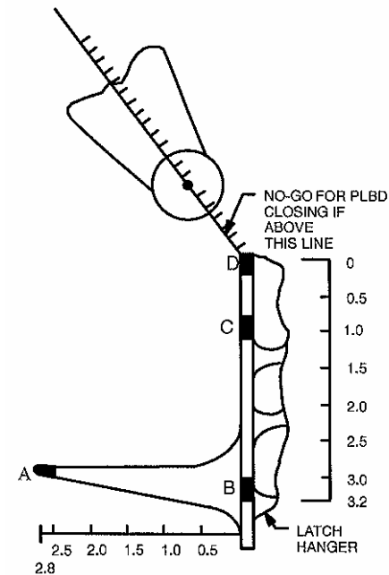
C/L LATCH EXTENDED GUIDE ROLLER TRAJECTORY NO-GO DIAGRAM
