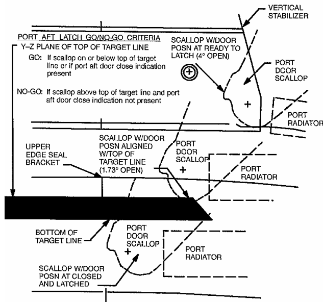
PORT AFT BULKHEAD LATCH GO/NO-GO DIAGRAM
