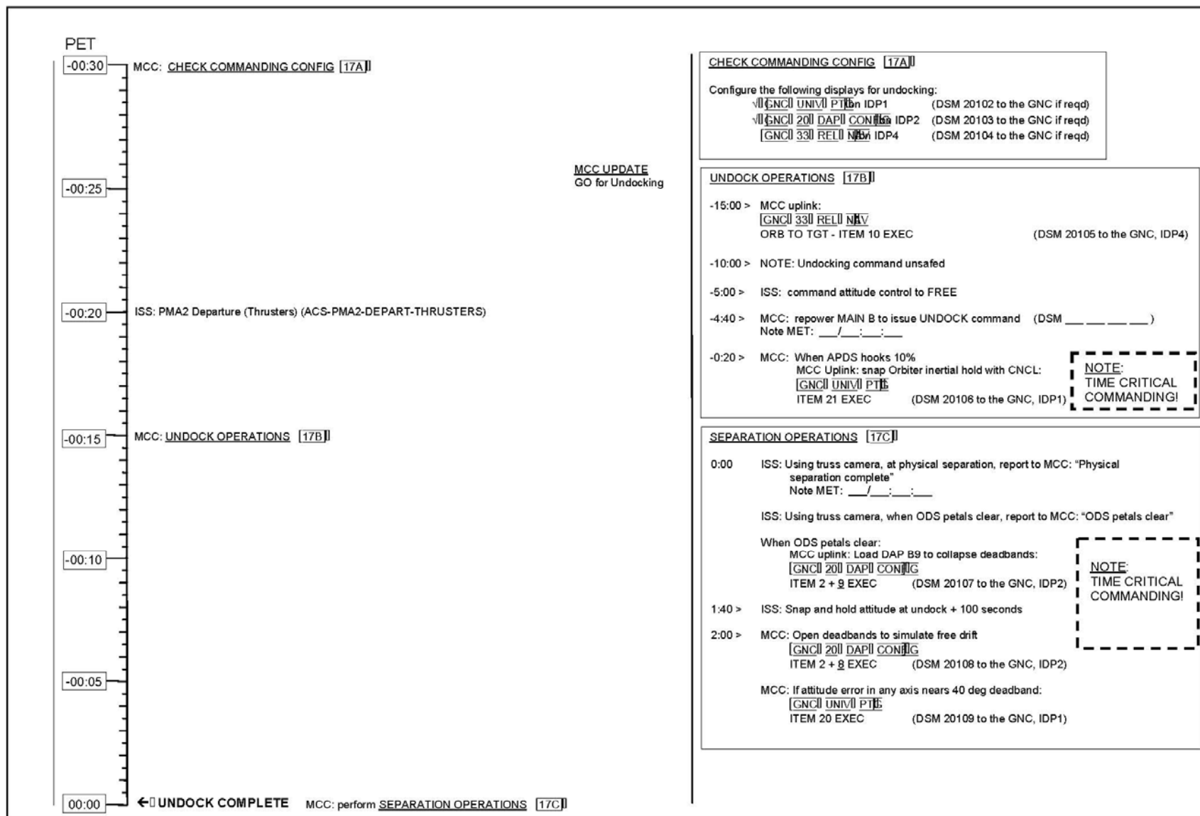
CSCS/Undock/Separation/Disposal Timeline
