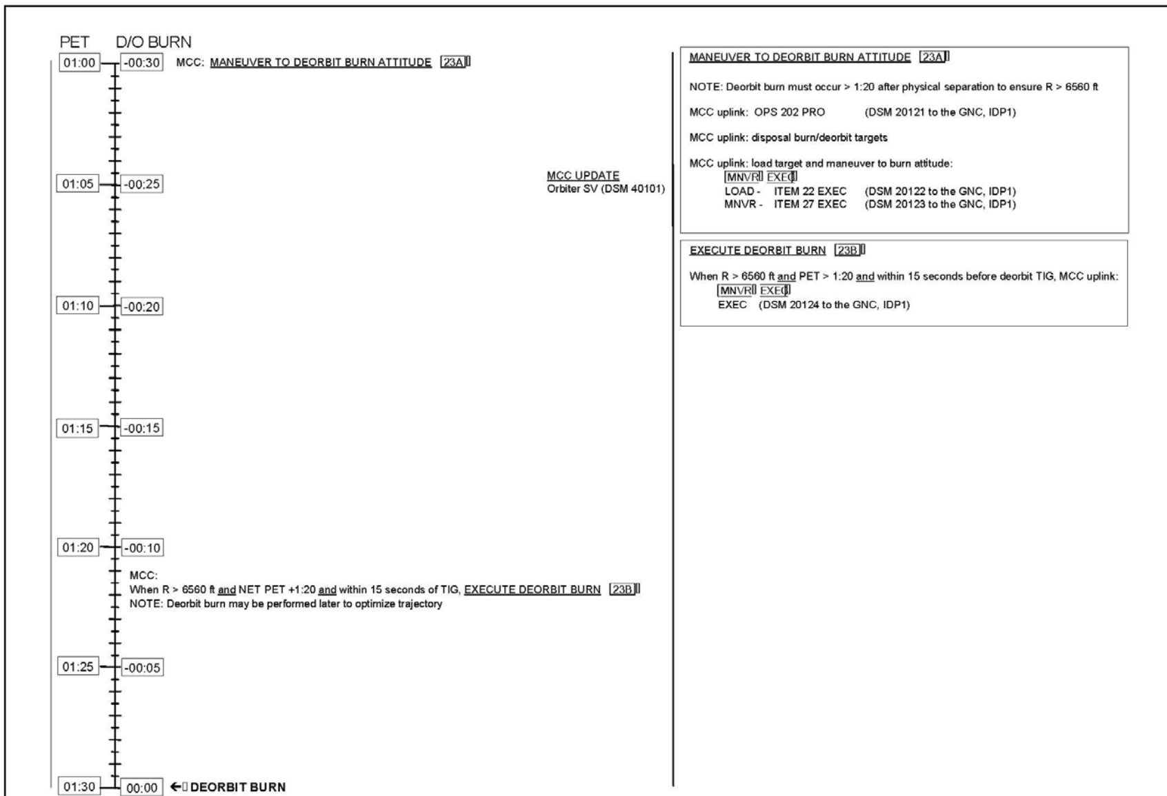
CSCS/Undock/Separation/Disposal Timeline
