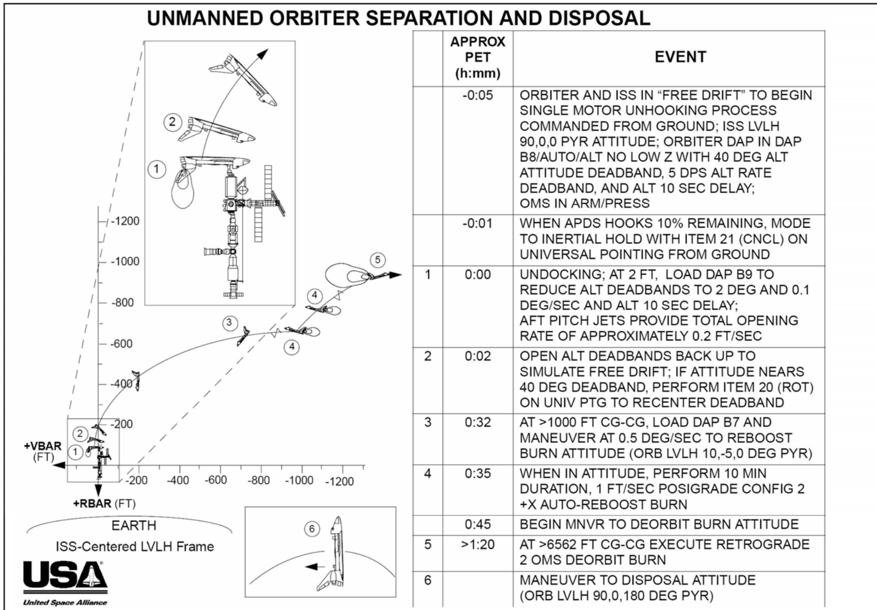
CSCS/Undock/Separation/Disposal Timeline
