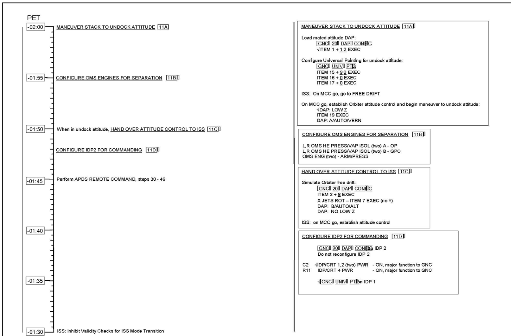
CSCS/Undock/Separation/Disposal Timeline
