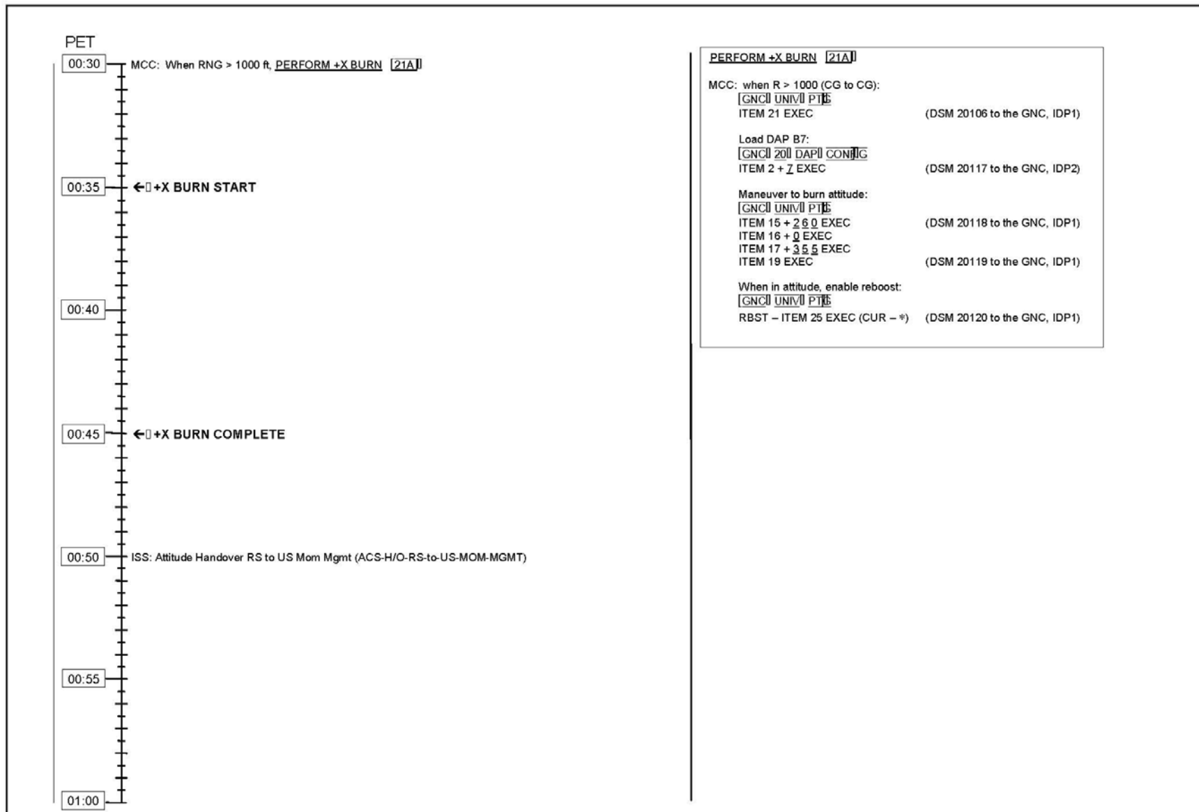
CSCS/Undock/Separation/Disposal Timeline
