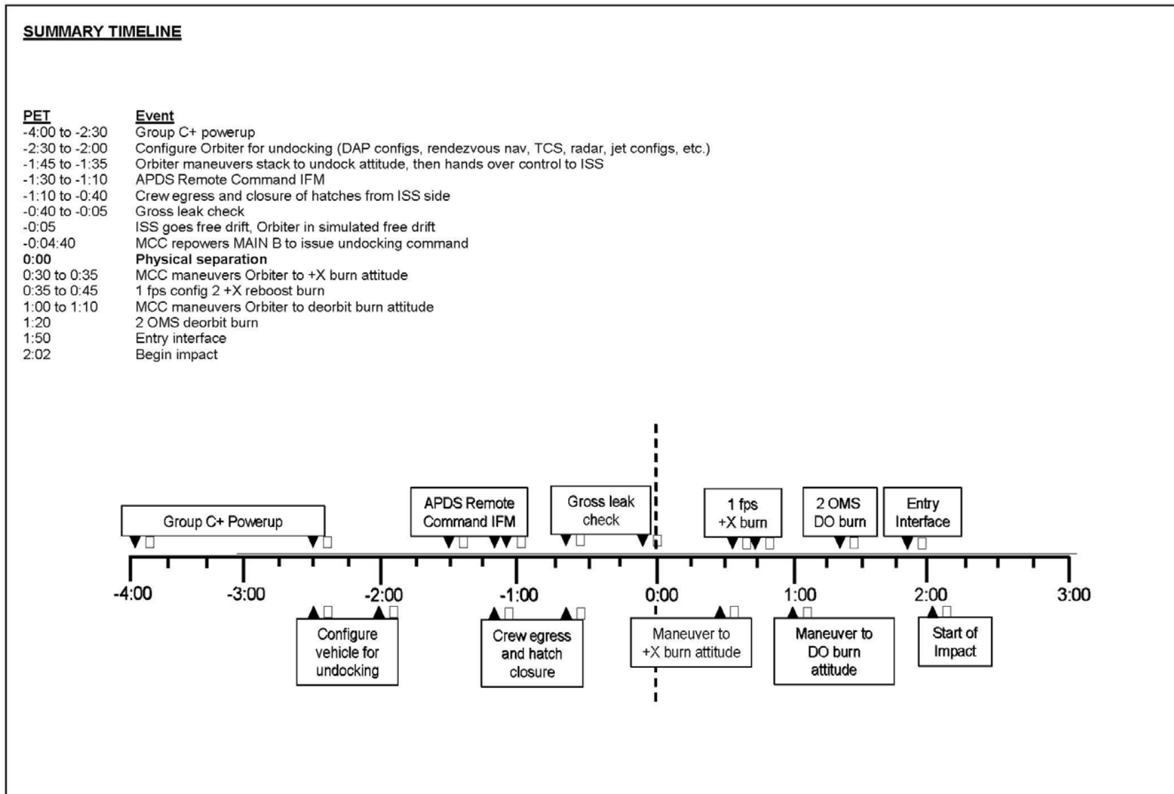
CSCS/Undock/Seperation/Disposal Timeline
