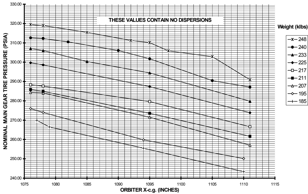
OI-26 Nominal Orbiter Main Gear Tire Pressures Contingency De-Orbit Mission Planning Assessments - Concrete Runways Contingency Abort & Emergency Landings (Nominal Vderotate @ 185 keas) Orbiter X-c.g. With Gear Deployed
