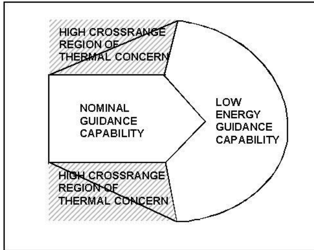
FIGURE A2-55-II - GENERIC DOWNRANGE ABORT EVALUATOR (DAE) FOOTPRINT ( 22.8 < V_I \leq 25.0 KFPS)
