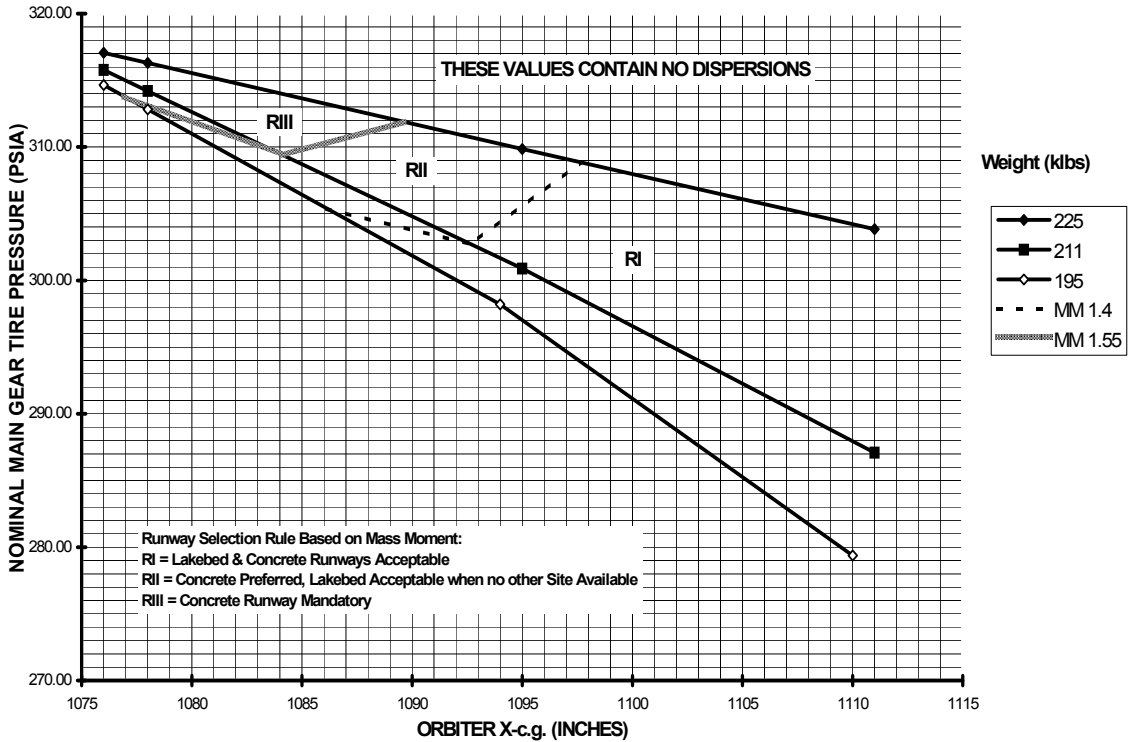
OI-26 Nominal Orbiter Main Gear Tire Pressures Contingency De-Orbit Mission Planning Assessments - Lakebed Runways Contingency Abort & Emergency Landings (Nominal Vderotate @ 185 keas) Orbiter X-cg With Gear Deployed
