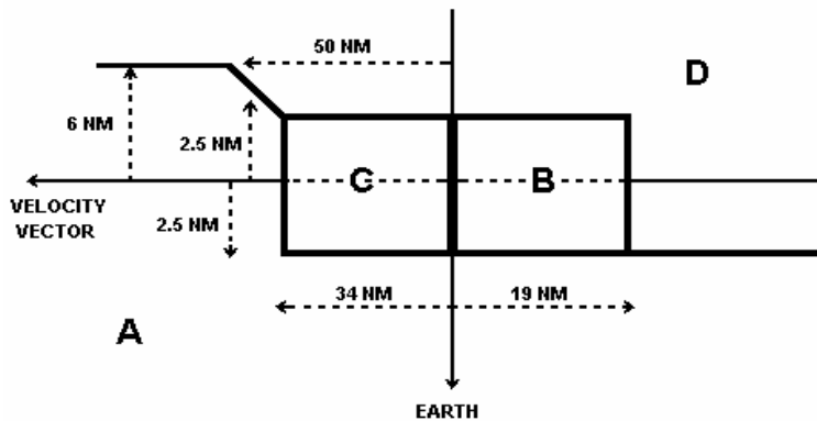
FIGURE A2-109-I - PREFERRED ATTITUDE FOR WATER DUMPS
