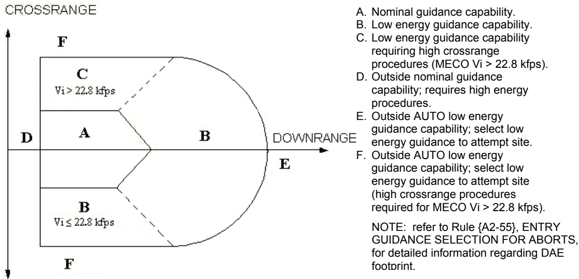
FIGURE A2-52-I - SHUTTLE LANDING FOOTPRINT (FOR ILLUSTRATION ONLY)
