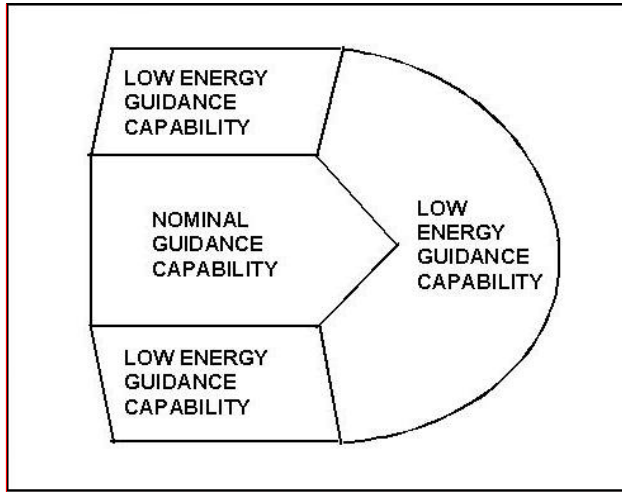
FIGURE A2-55-I - GENERIC DOWNRANGE ABORT EVALUATOR (DAE) FOOTPRINT (VI ≤ 22.8 KFPS)
