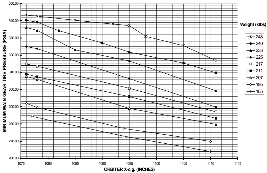
OI-26 Minimum Orbiter Main Gear Tire Pressure Mission Planning Assessments - Concrete Runways All Normal & Intact Abort Landings (Nominal Vderotate @ 185 keas) Orbiter X-c.g. With Gear Deployed
