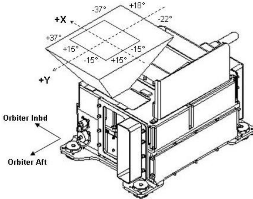
FIGURE A15-28-I - LCS NOMINAL AND MAX FOV ILLUSTRATION ©[042507-8047]
