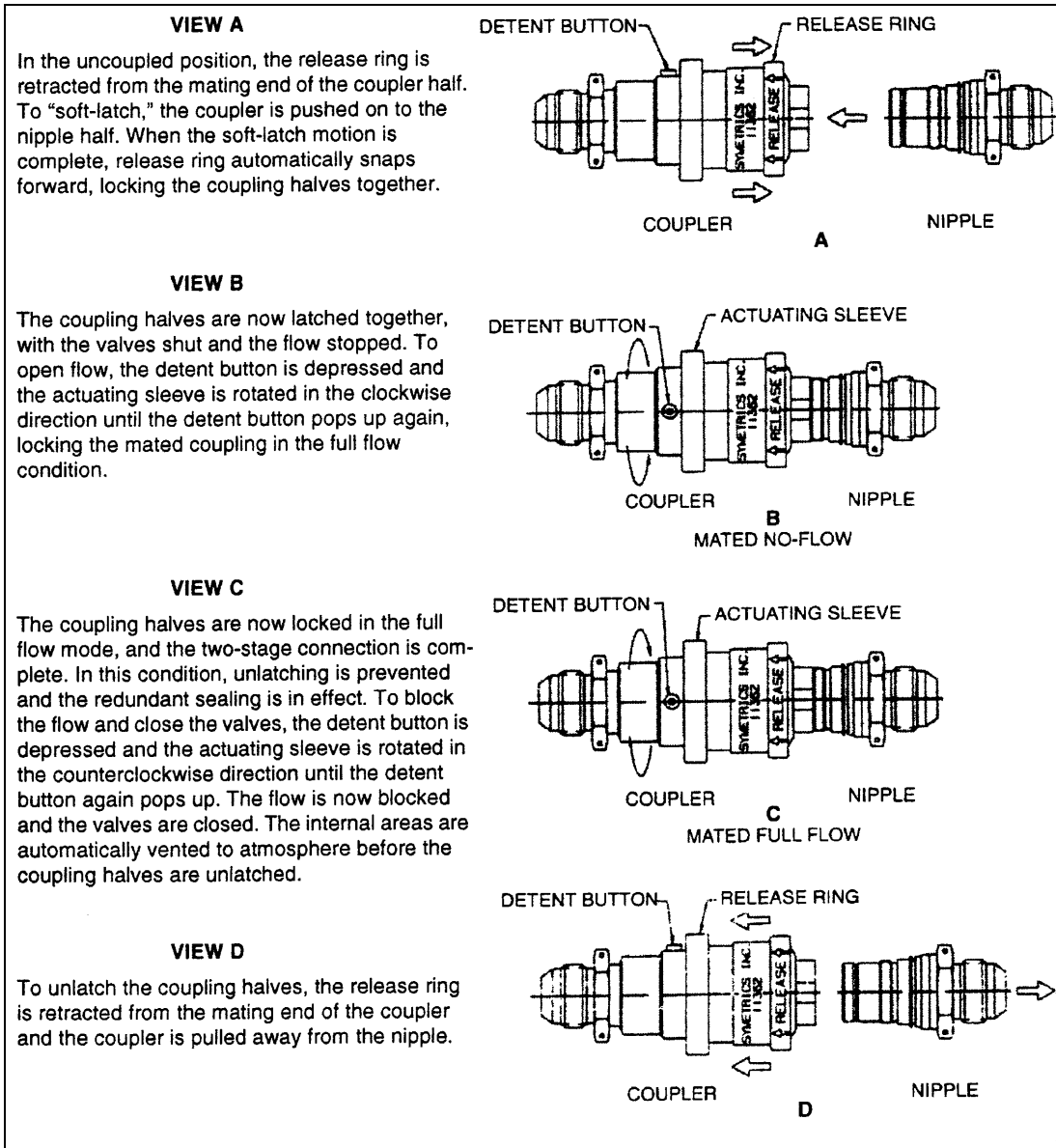
Figure 2.- Two-Stage High-Pressure QDs.
