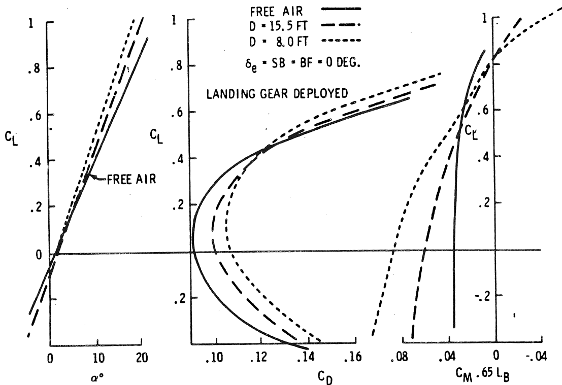
Figure 5-40.- Orbiter ground effects.
