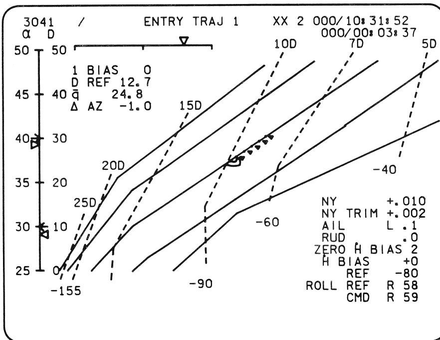
Figure 5-7.- Entry trajectory 1 (typical initial display).
