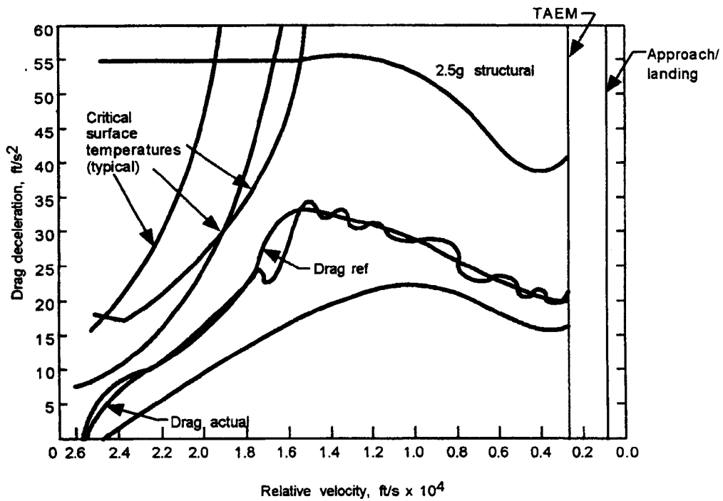
Figure 2-1. Simplified entry guidance
