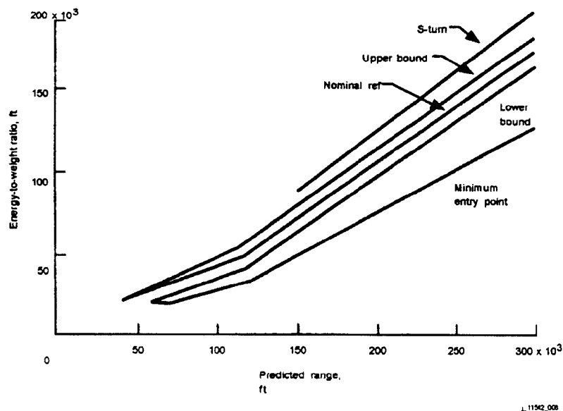
Figure 2-4. Typical TAEM energy-to-weight ratio
