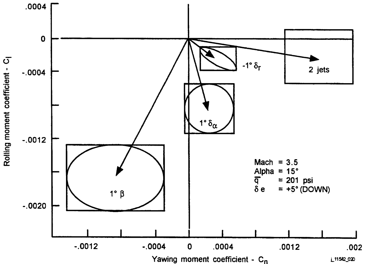
Figure A-1. Vector diagram of aerodynamic coefficients showing uncertainties
