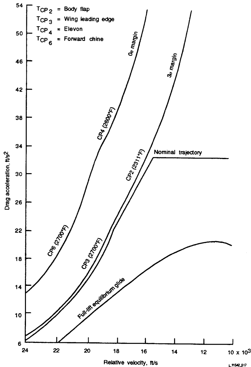
Figure 5-20. Temperature margin boundaries
