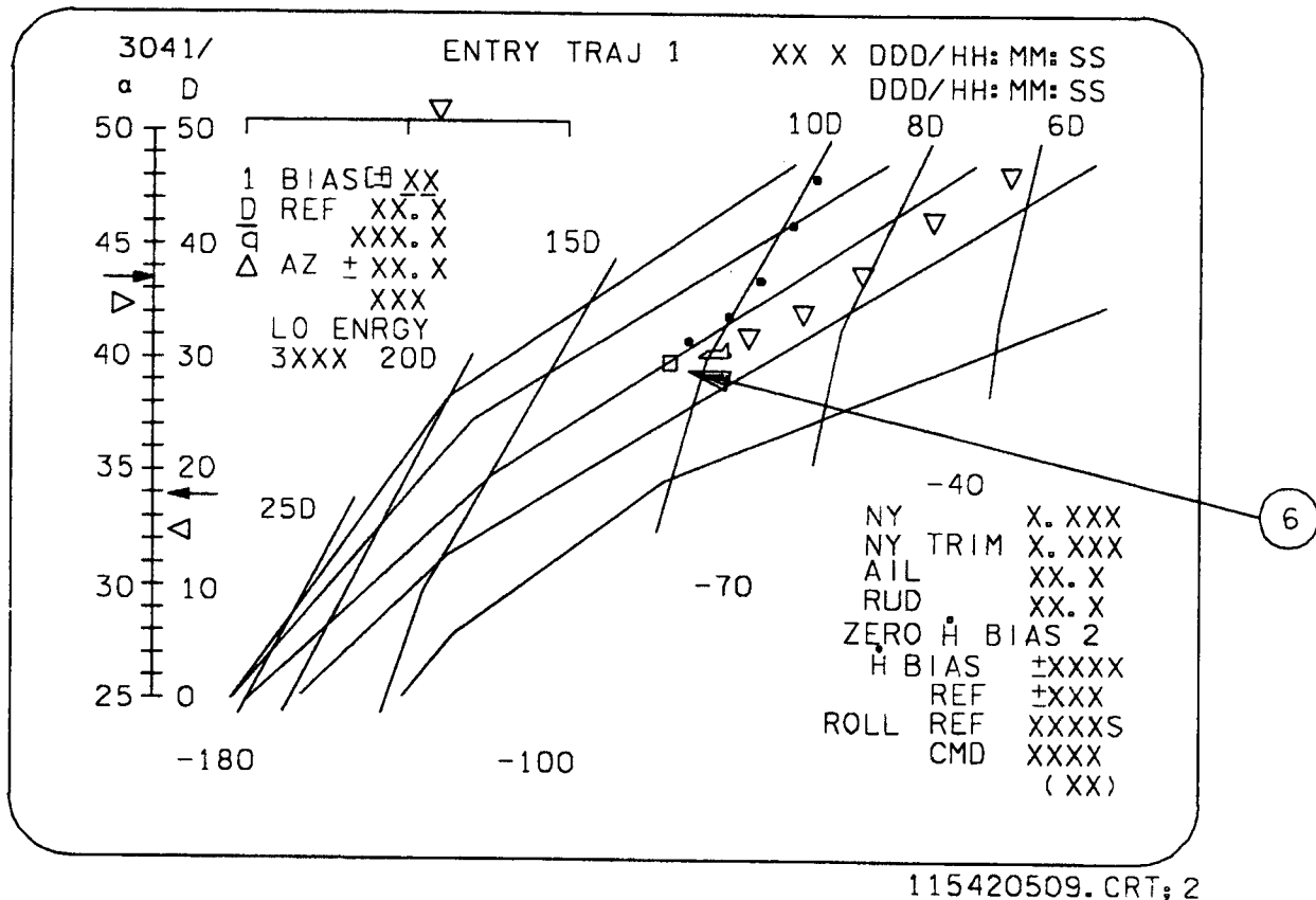
Figure 5-9. Entry TRAJ 1 (drag decreased relative to drag reference)
