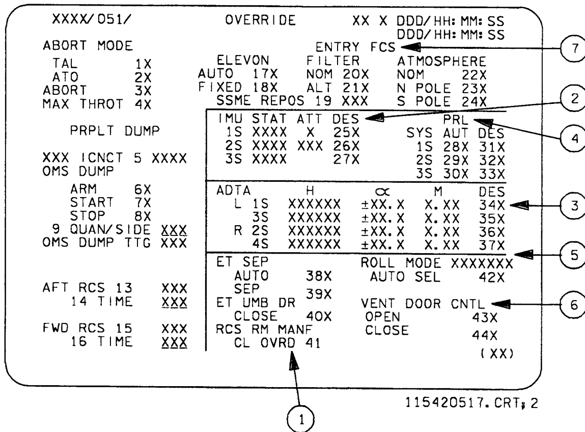
Figure 5-17. OVERRIDE display (PFS)
