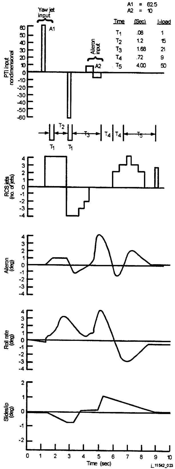
Figure A-4. Automatic PTI (Mach 5.8)
