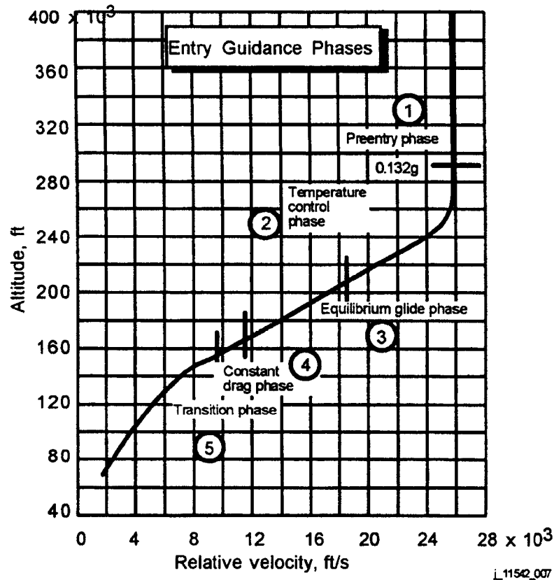
Figure 2-3. Guidance for nominal entry
