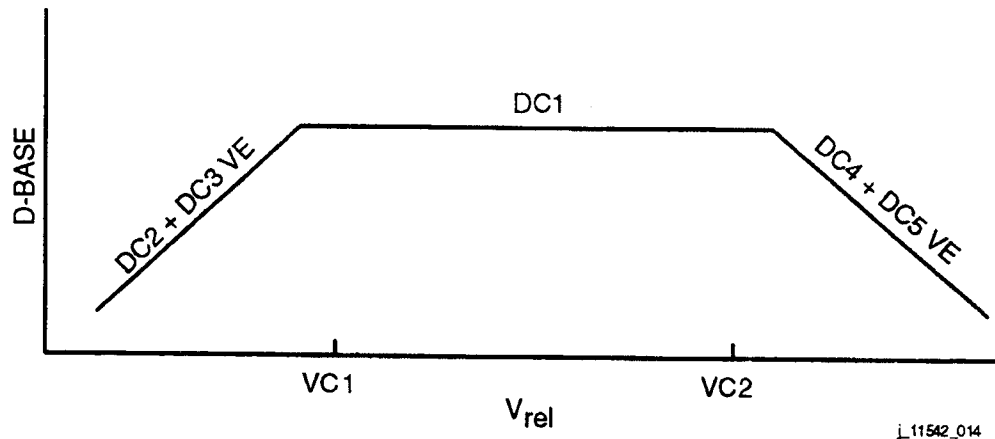
Figure 5-10. Phugoid damper plot
