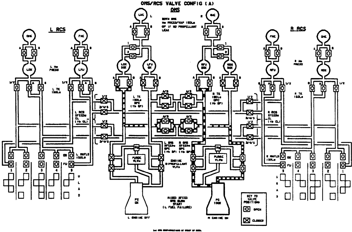
Figure 4-12. OMS/RCS valve configuration (A)
