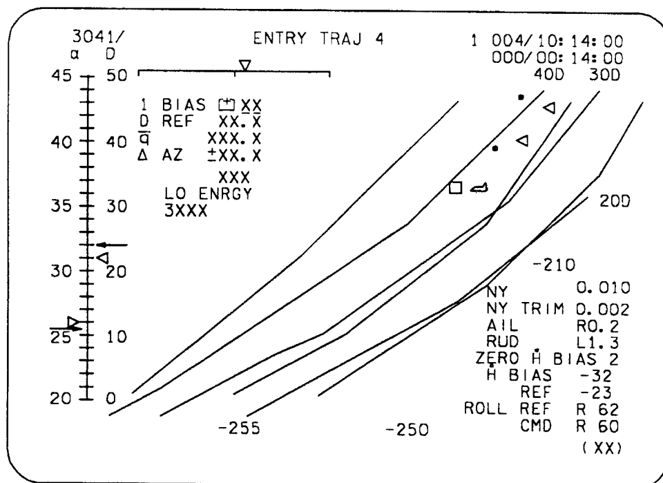
Figure 5-5. ENTRY TRAJ 4 display (PFS)
