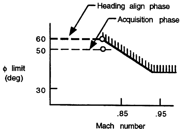
Figure 5-30. Transonic limit
