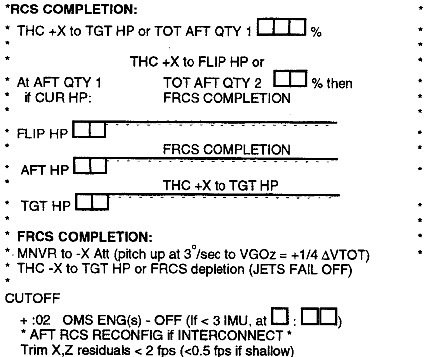
Figure 4-7. DEORBIT BURN (2 ENG) cue card
