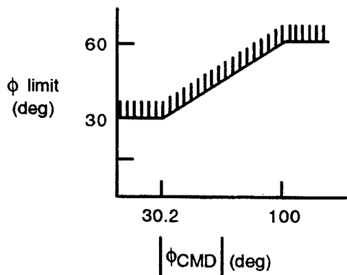
Figure 5-29. Prefinal \phi limit versus \phi CMD
