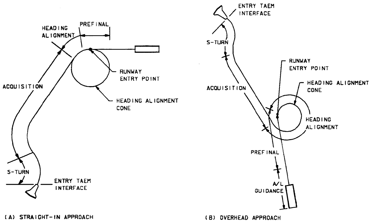
Figure 2-6. TAEM guidance phase and groundtrack geometry
