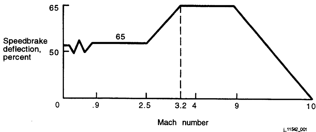
Figure 5-23. Speedbrake schedule
