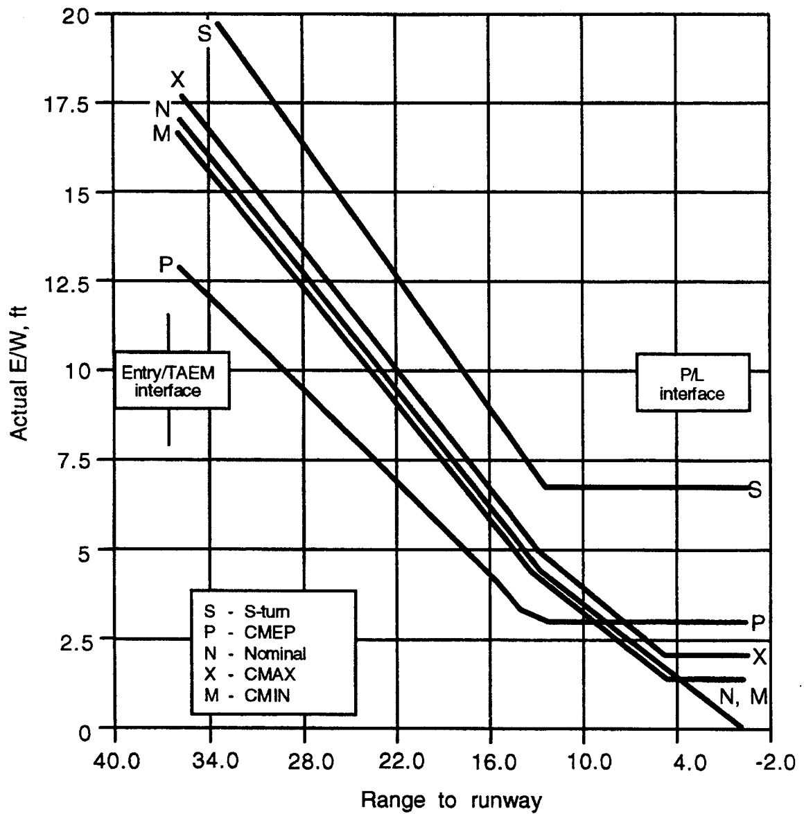
Figure 5-12. Actual energy over weight during TAEM
