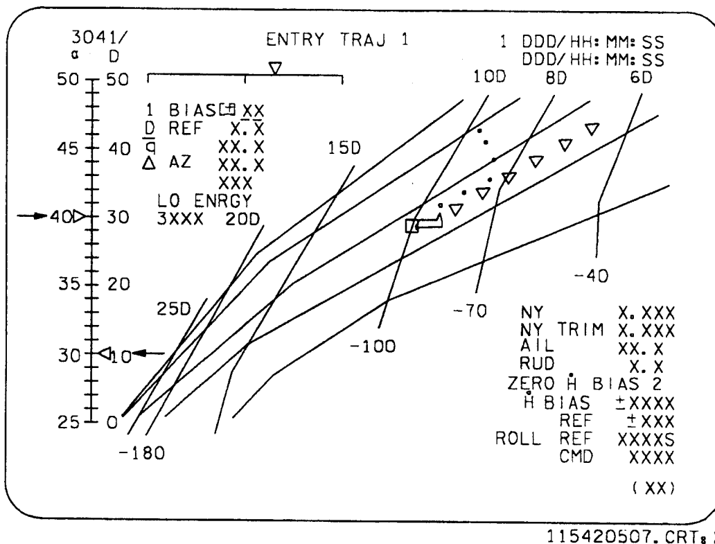
Figure 5-7. ENTRY TRAJ 1 (typical initial display)
