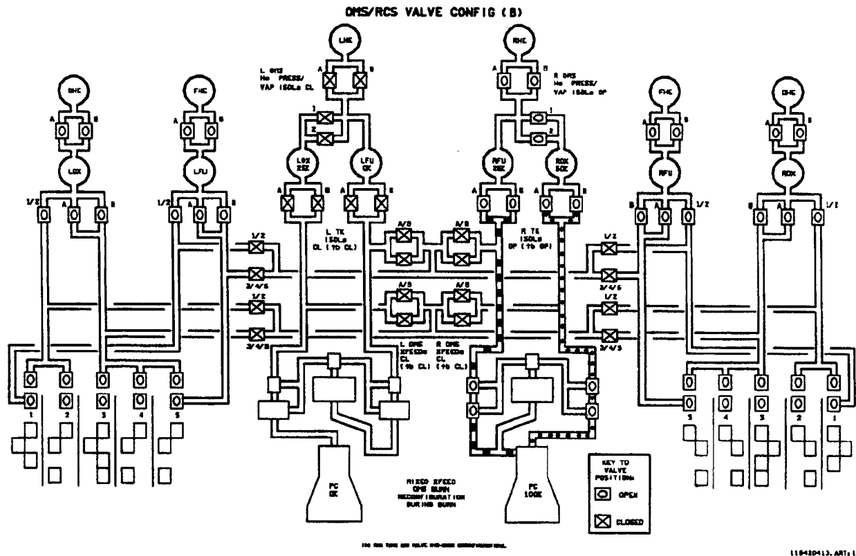
Figure 4-13. OMS/RCS valve configuration (B)
