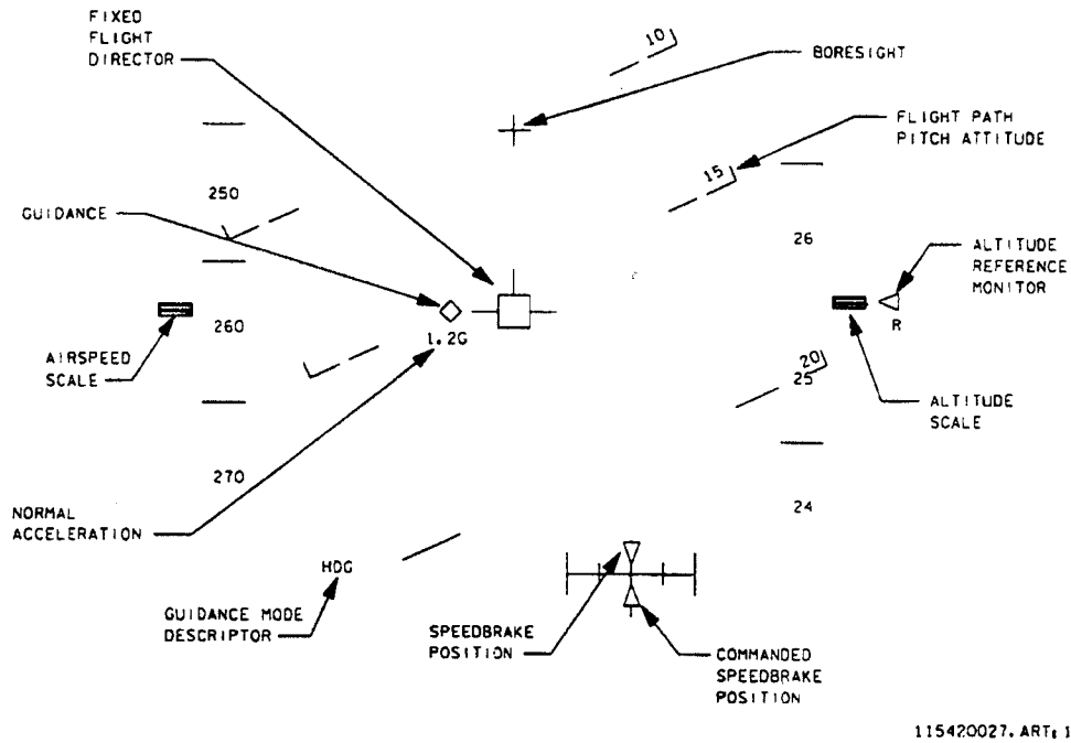
Figure 5-26. Approach and land display (TAEM heading phase)
