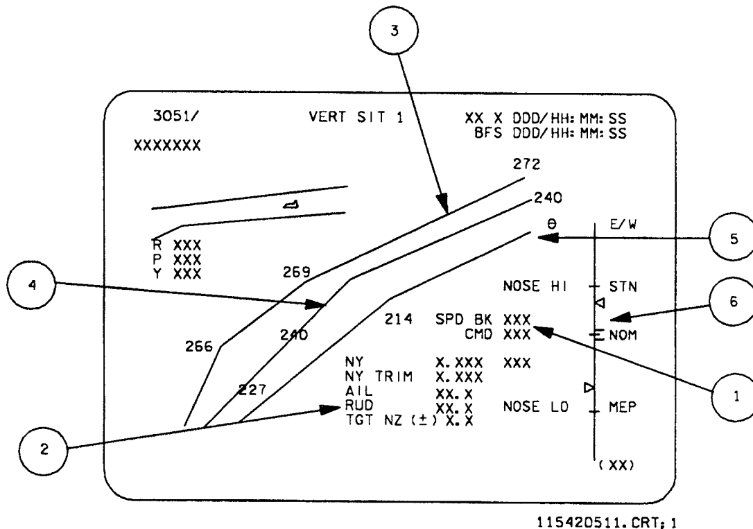
Figure 5-11. VERT SIT 1 display (PFS/BFS)
