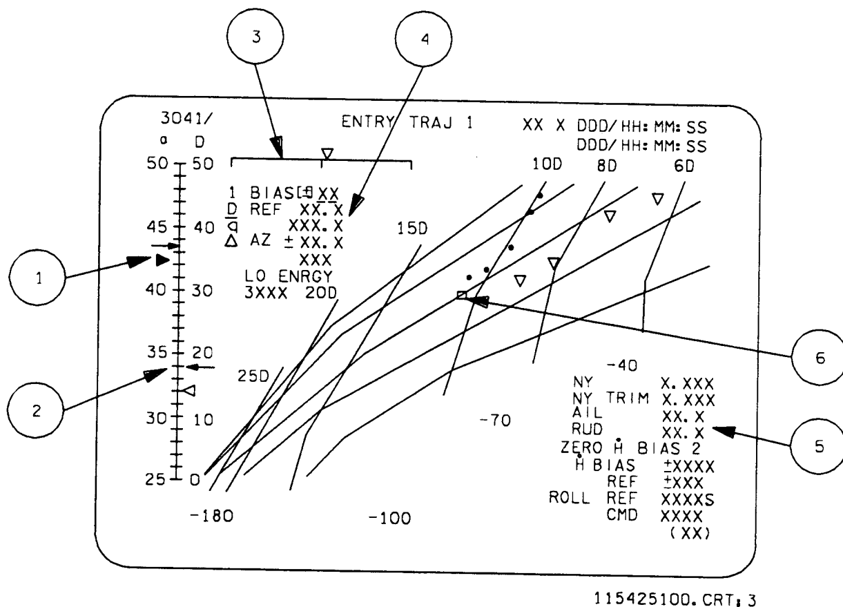
Figure 5-1. ENTRY TRAJ 1 (representative) display
