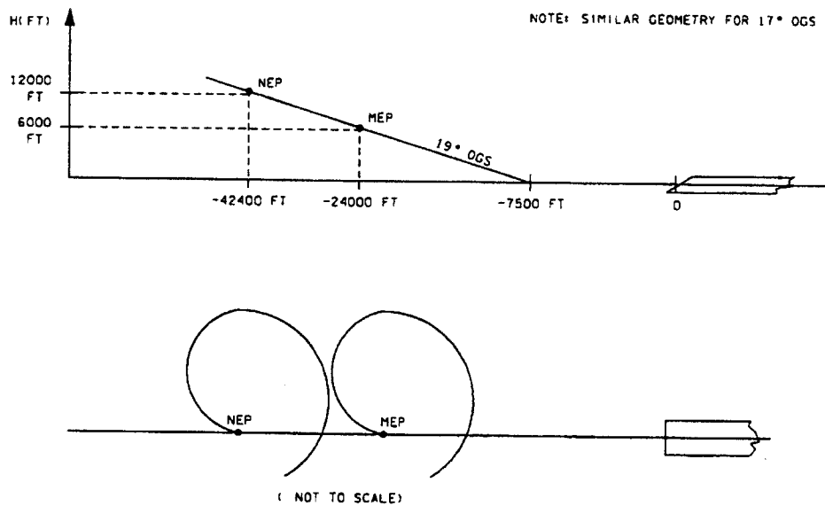
Figure 5-33. NEP/MEP geometry
