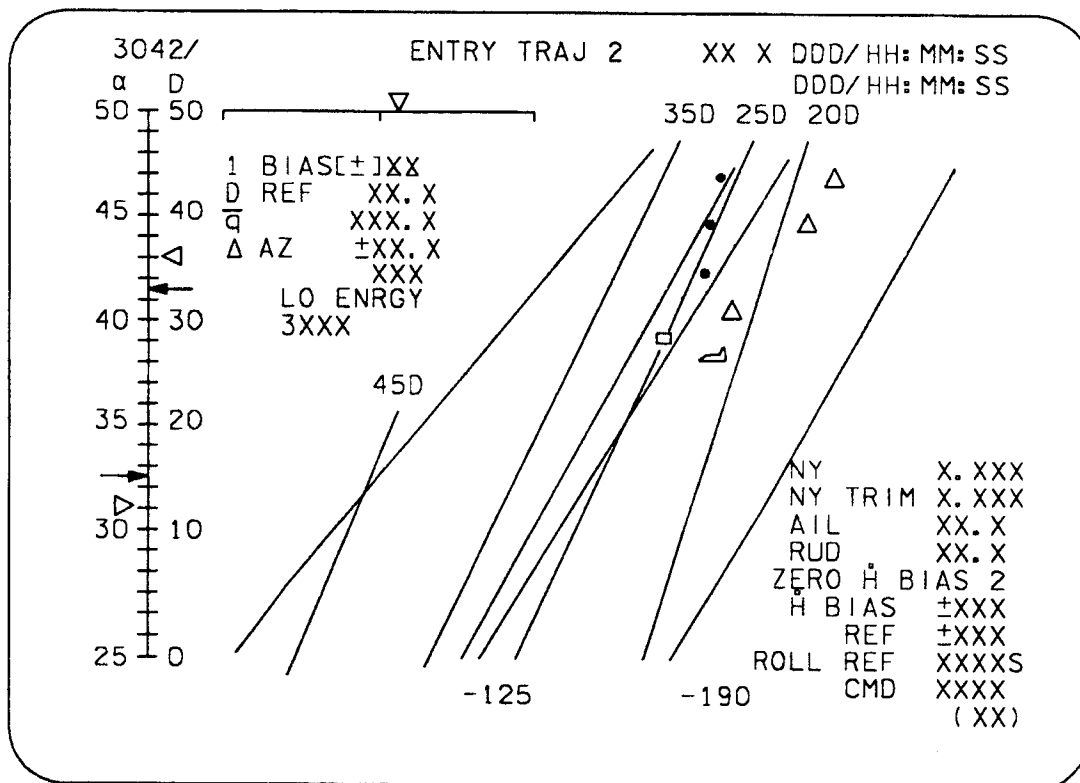
Figure 5-3. ENTRY TRAJ 2 display
