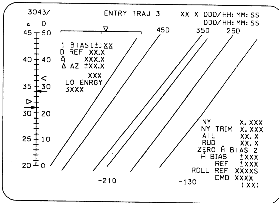
Figure 5-4. ENTRY TRAJ 3 display (PFS)
