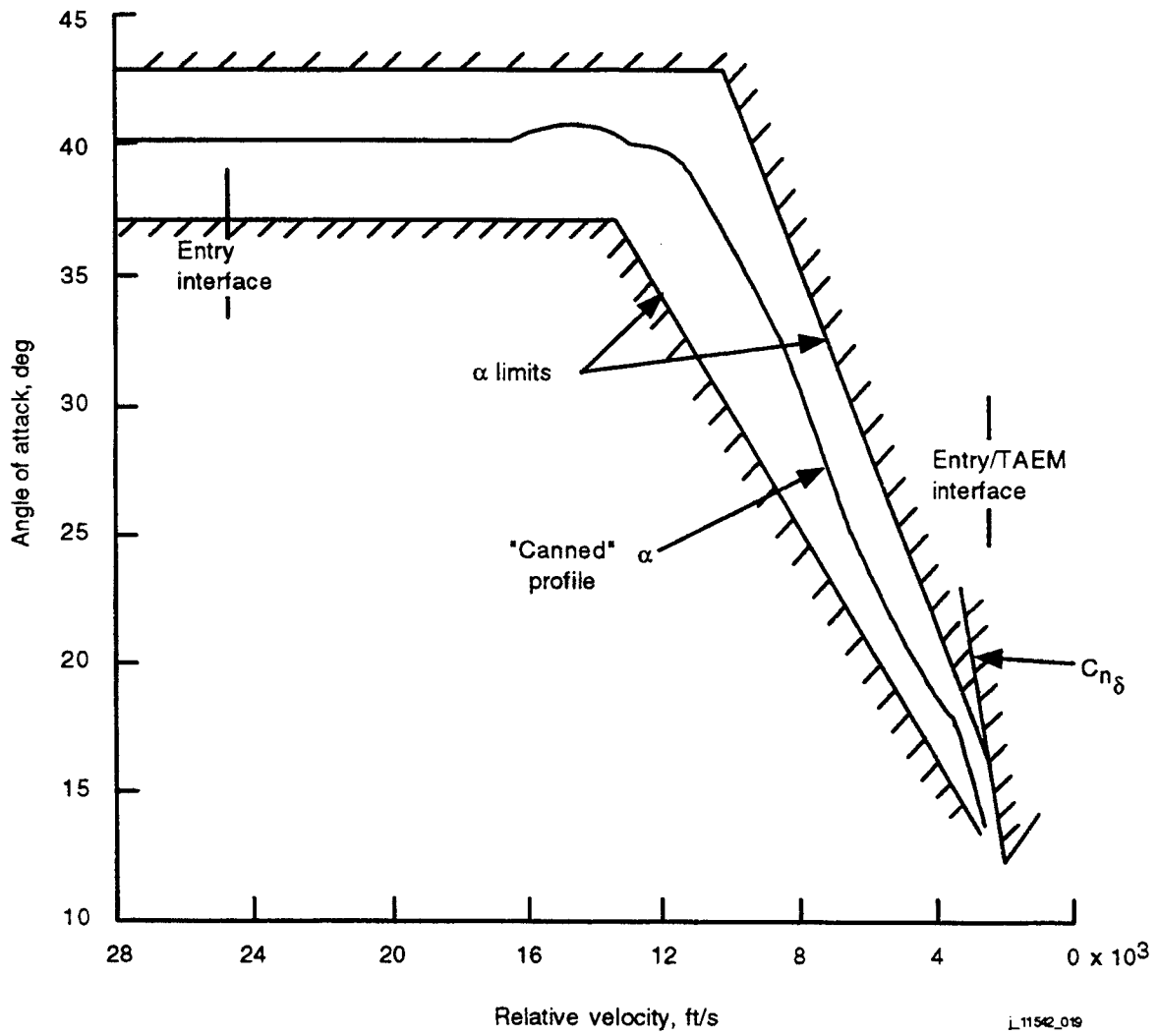
Figure 5-22. Entry angle-of-attack profile
