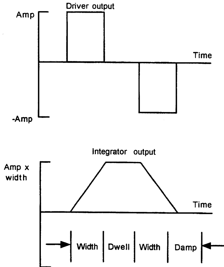
Figure A-3. Typical auto PTI output
