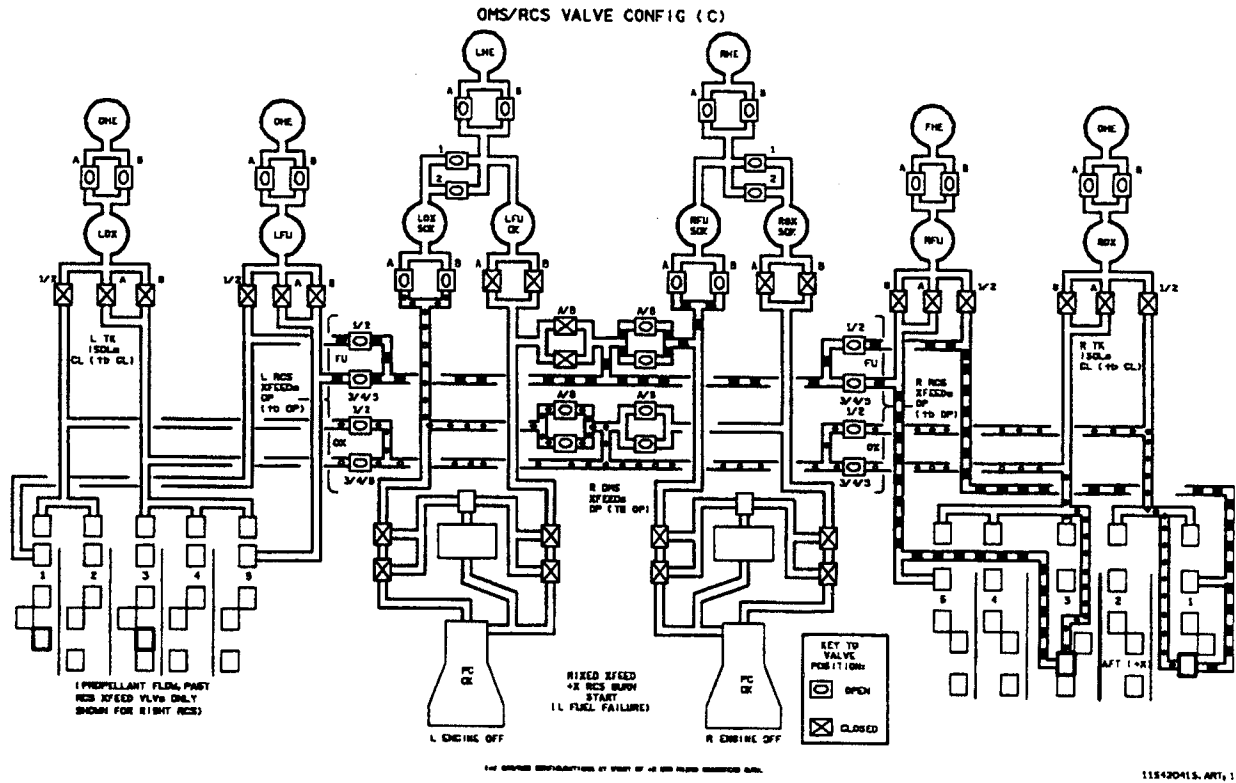
Figure 4-15. OMS/RCS valve configuration (C)
