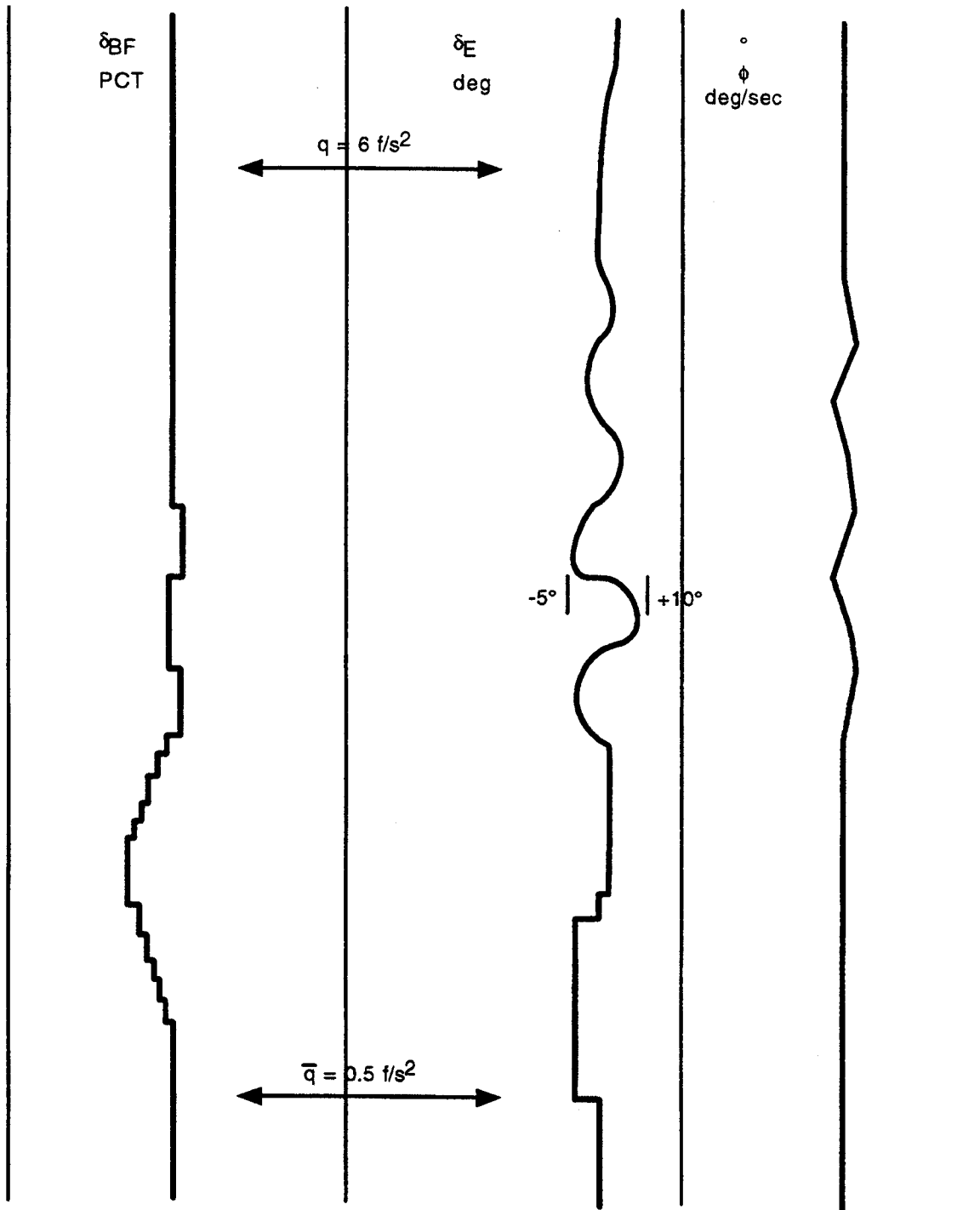
Figure 5-19. Aerosurface trim activation at low qbar
