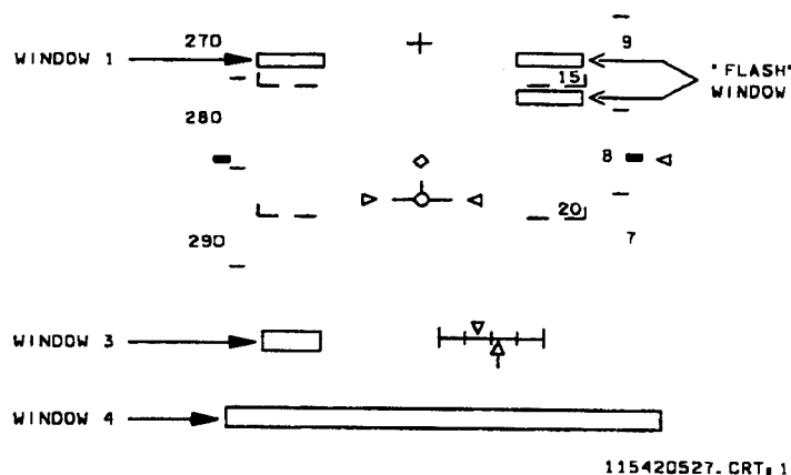
Figure 5-27. Cue/alert windows
