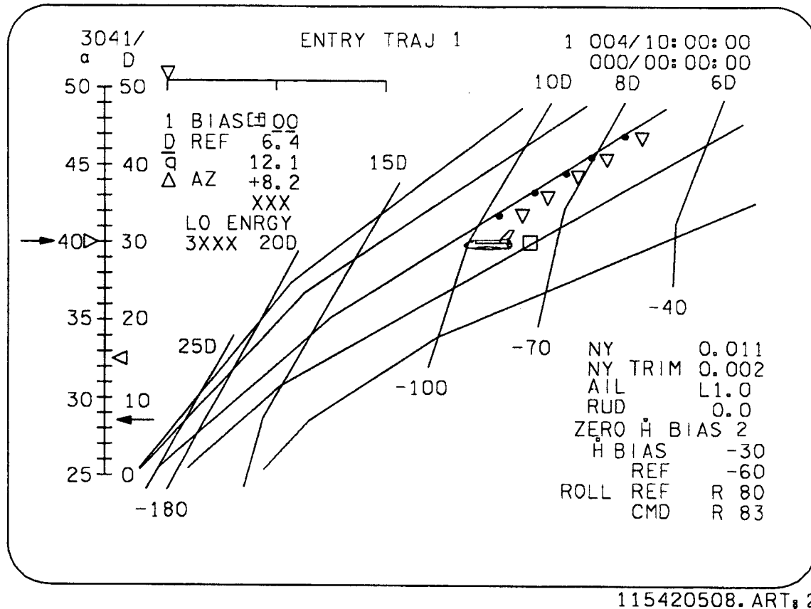
Figure 5-8. ENTRY TRAJ 1 (drag greater than drag reference)
