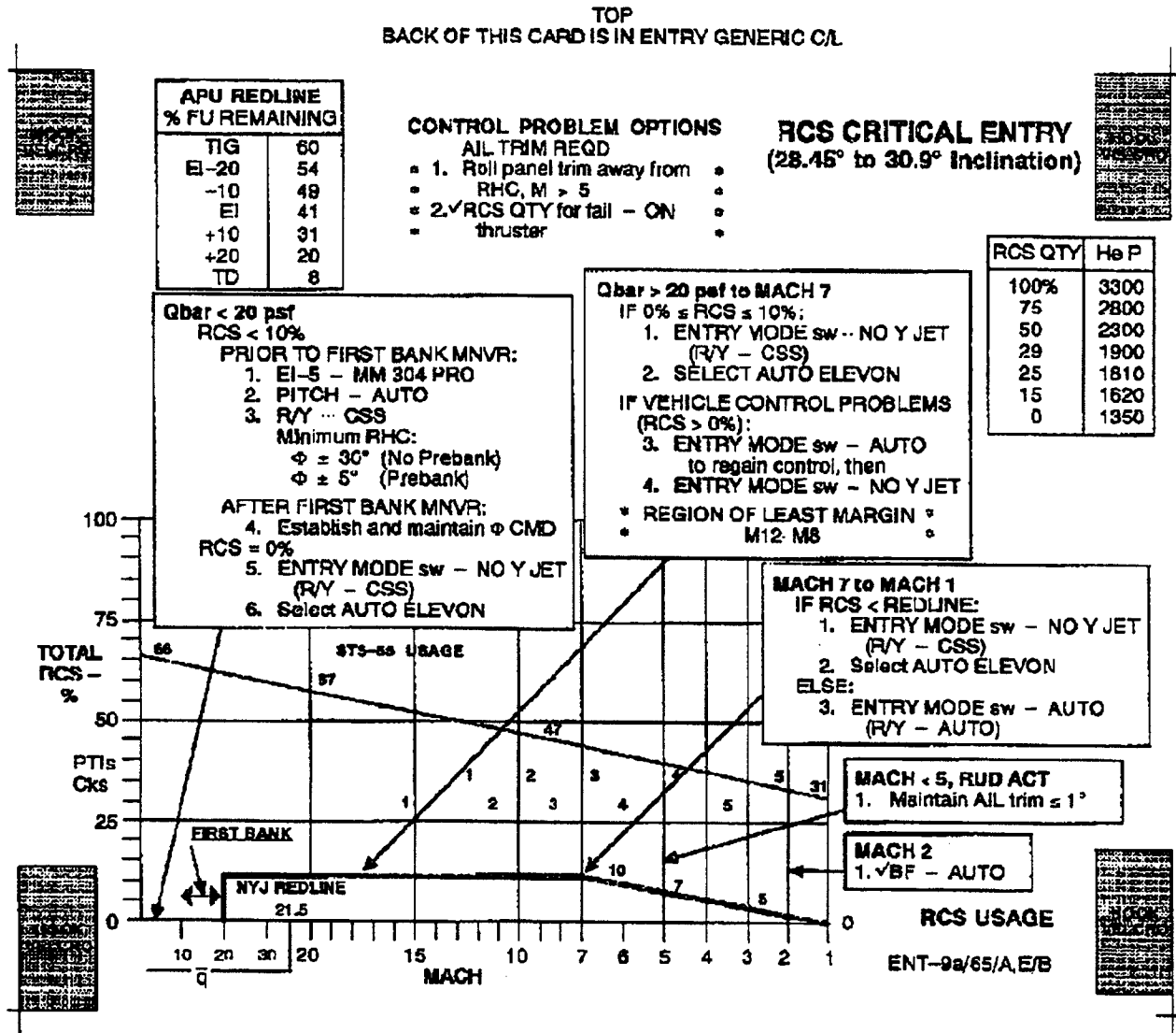
Figure 5-35. RCS CRITICAL ENTRY cue card
