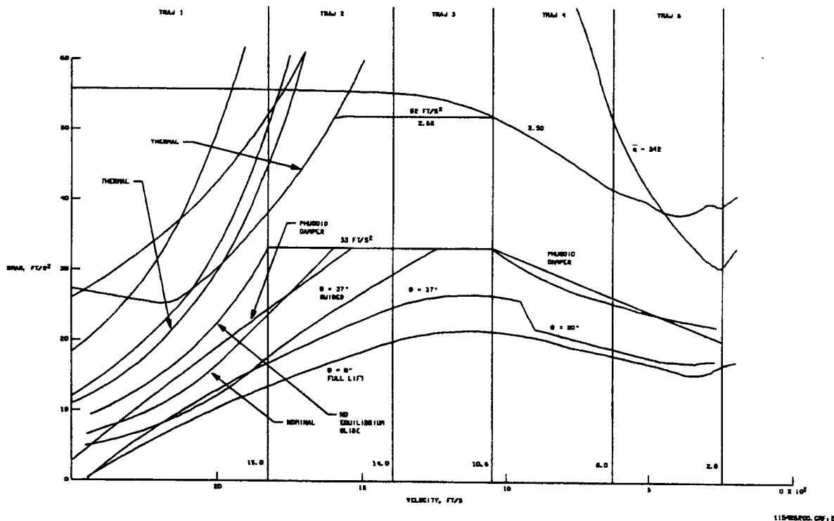
Figure 5-2. Typical drag versus velocity plot (cycle 2)
