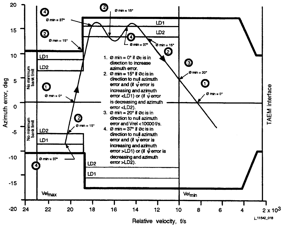
Figure 5-21. Azimuth error versus relative velocity plot
