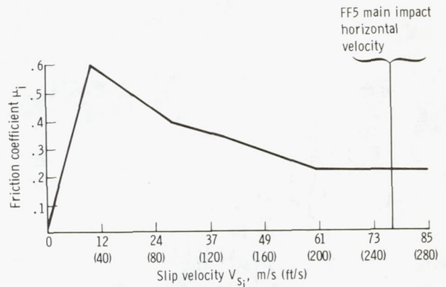
FIGURE 12.—Main gear tire/ground friction properties during spin-up.
