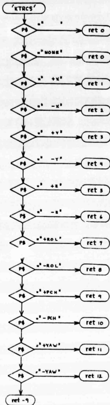
Figure 33. 'KTRCS' Function Subprogram Logic Flow
