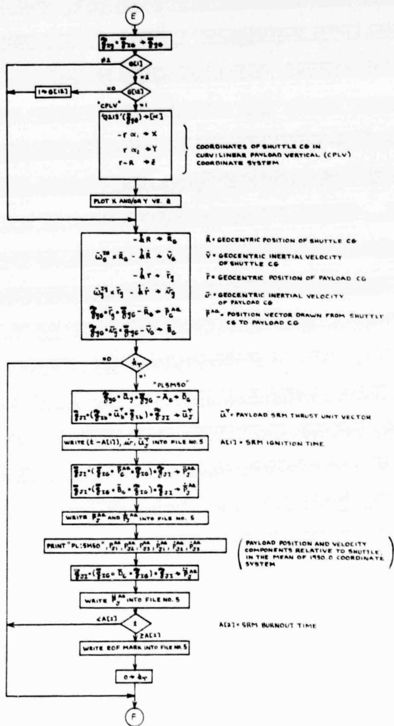
Figure 38e. %PROP Logic Flow (cont.)
