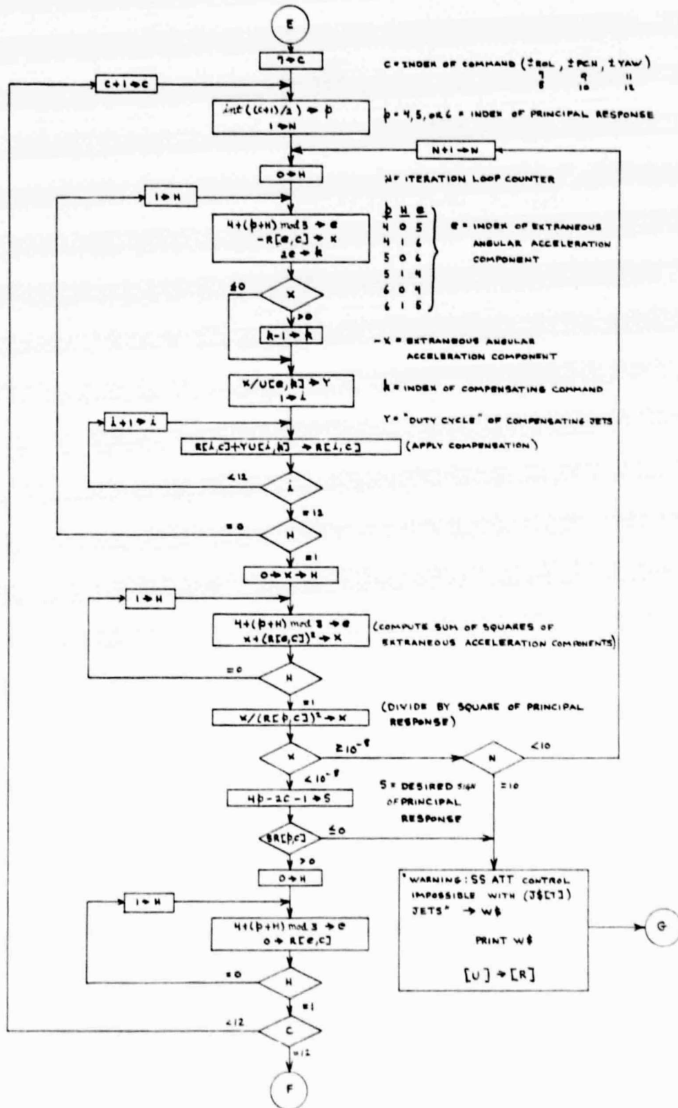
Figure 20d. %RMAT Logic Flow (cont.)
