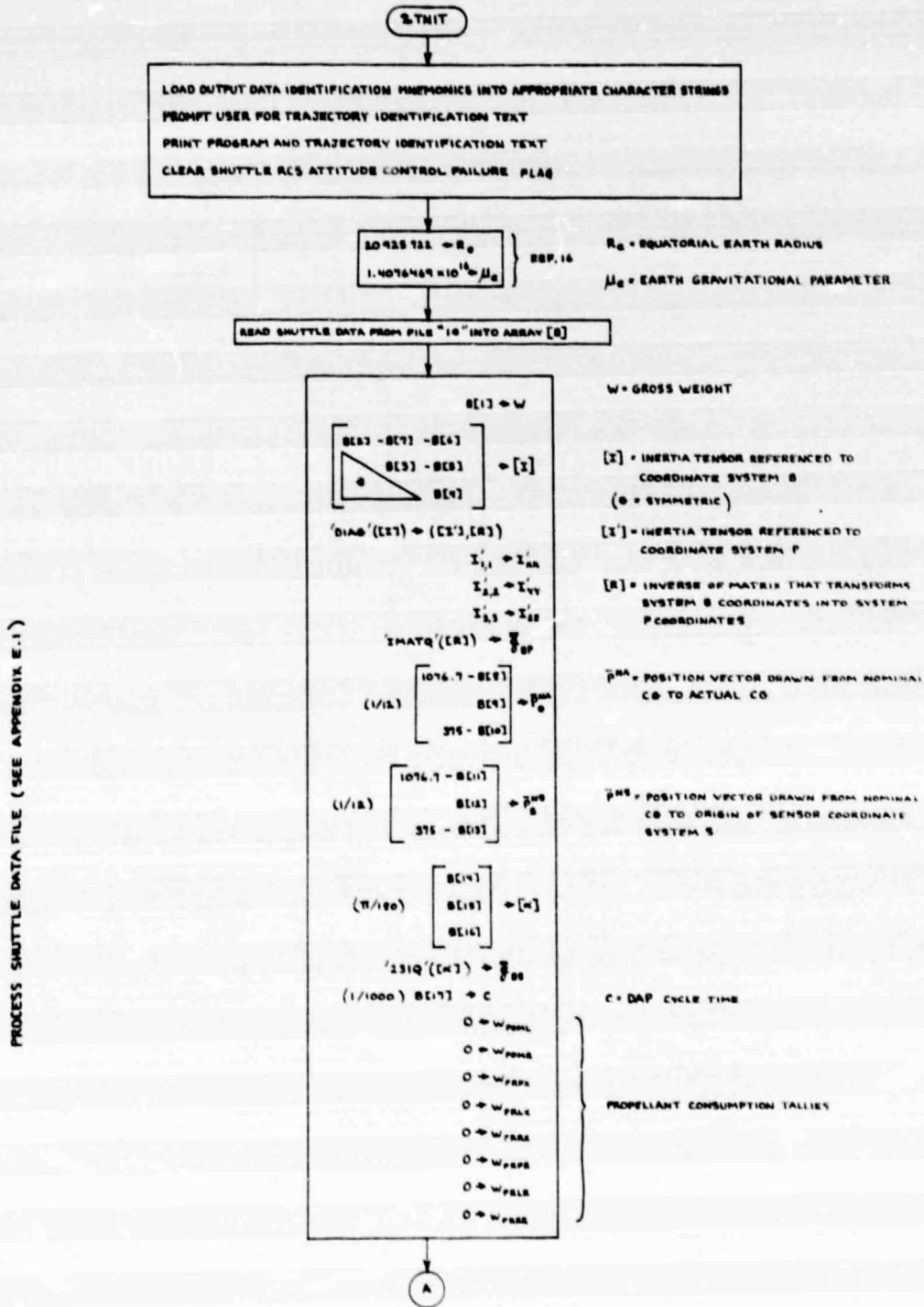
Figure 28a. %TNIT Logic Flow
