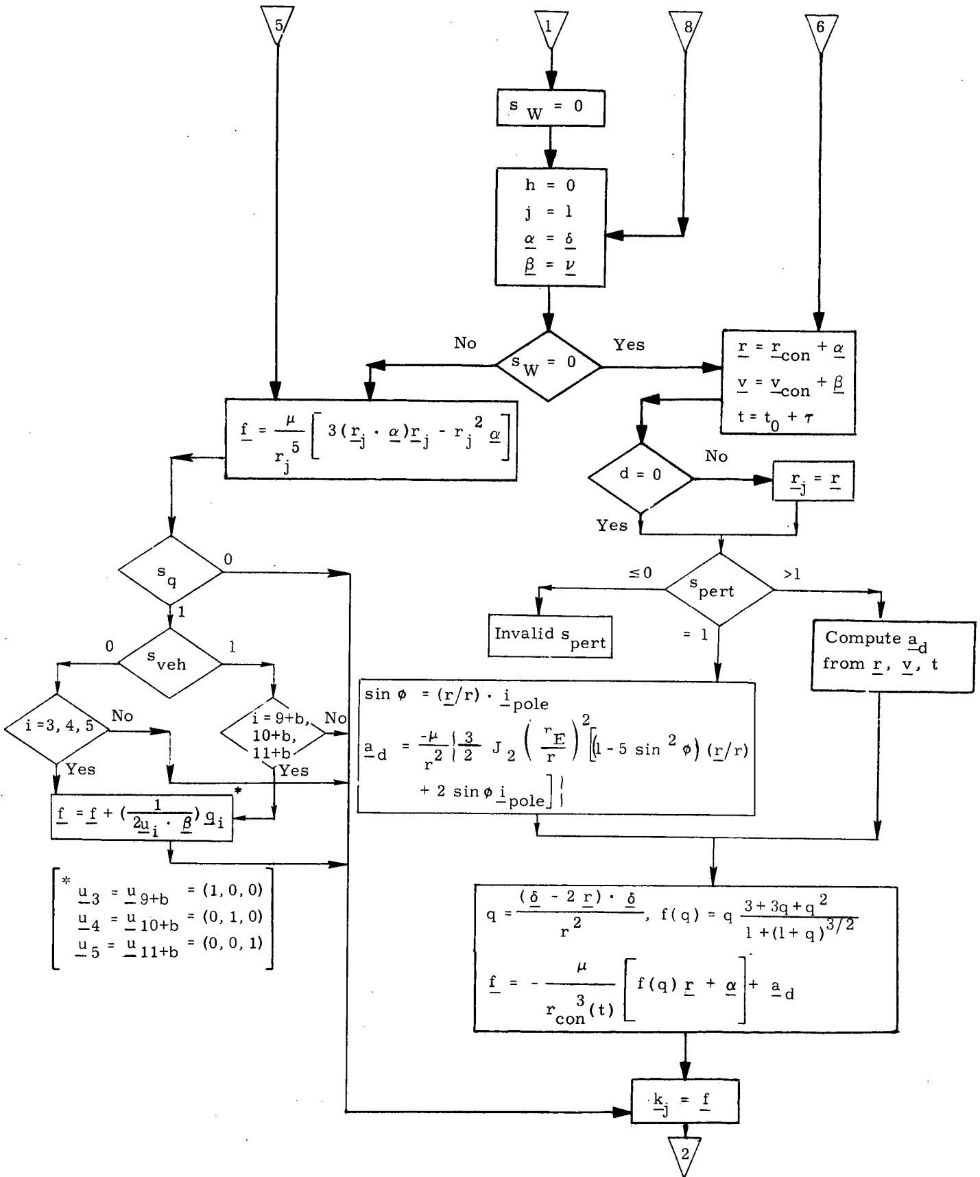
Figure 2b. Detailed Flow Diagram
