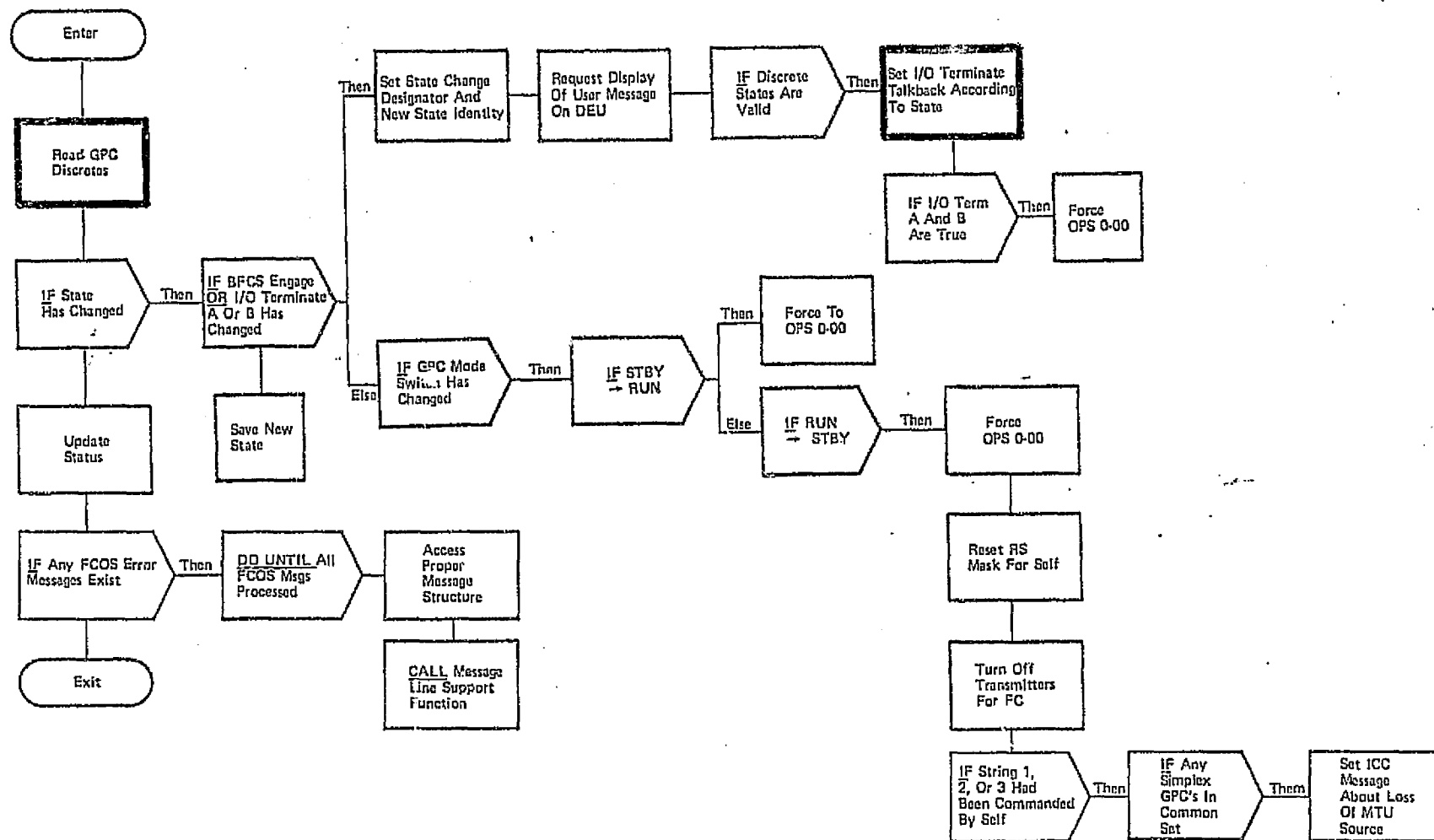
Figure 3-22. GPC Switch Monitor (ARA_GPC_SWITCH)
