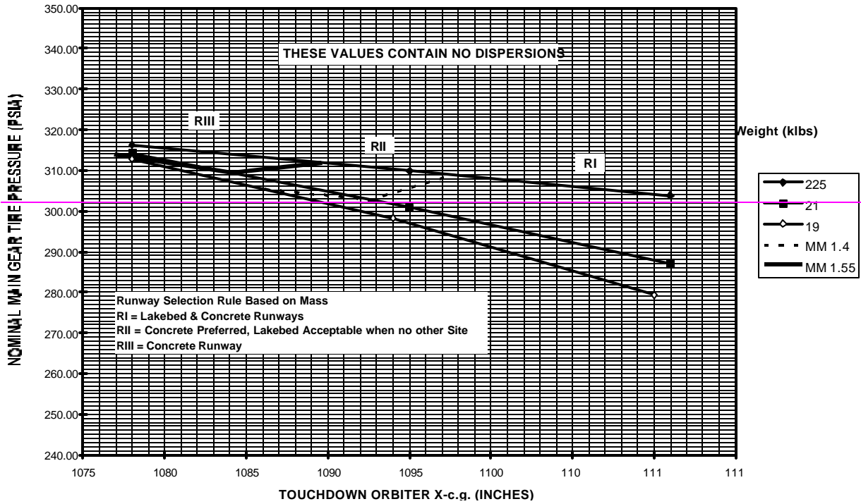
OI-23 Nominal Orbiter Main Gear Tire Pressures Contingency De-Orbit Mission Planning Assessments - Lakebed Runways Contingency Abort & Emergency Landings (Nominal Vderotate @ 185 keas)
