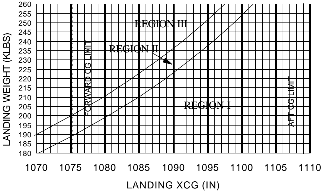
Landing Regions Chart for Hard Lakebed Hardness
