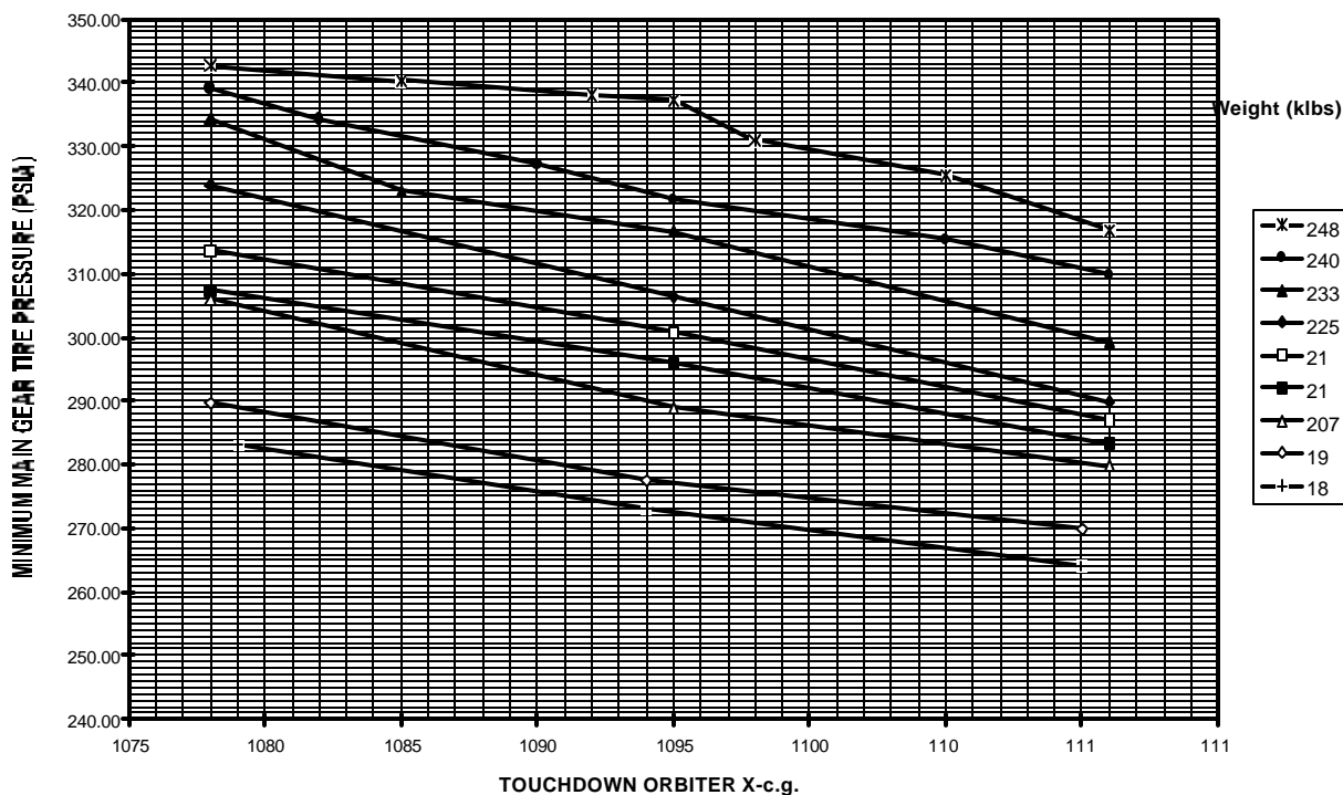
Minimum Orbiter Main Gear Tire Pressure - Concrete - Derotation Initiation at 185 KEAS
