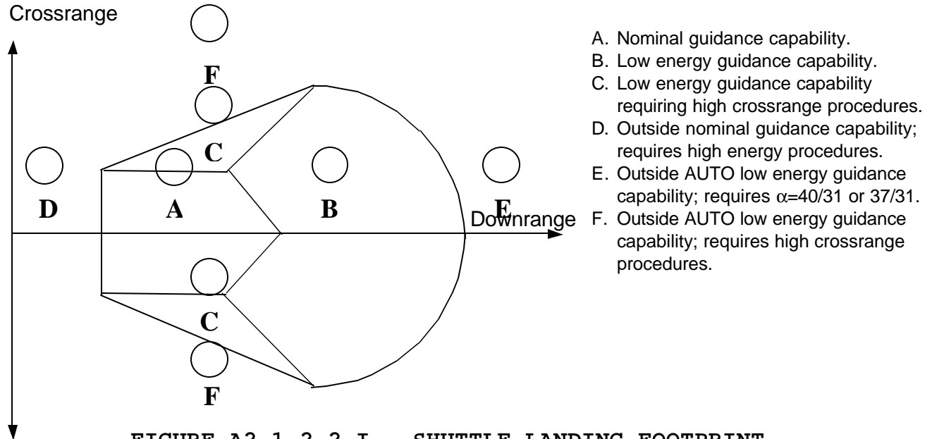
FIGURE A2.1.2-2-I - SHUTTLE LANDING FOOTPRINT
