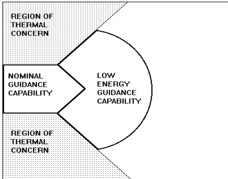
FIGURE 2-14-I - GENERIC DOWNRANGE ABORT EVALUATOR (DAE) DEPICTION
