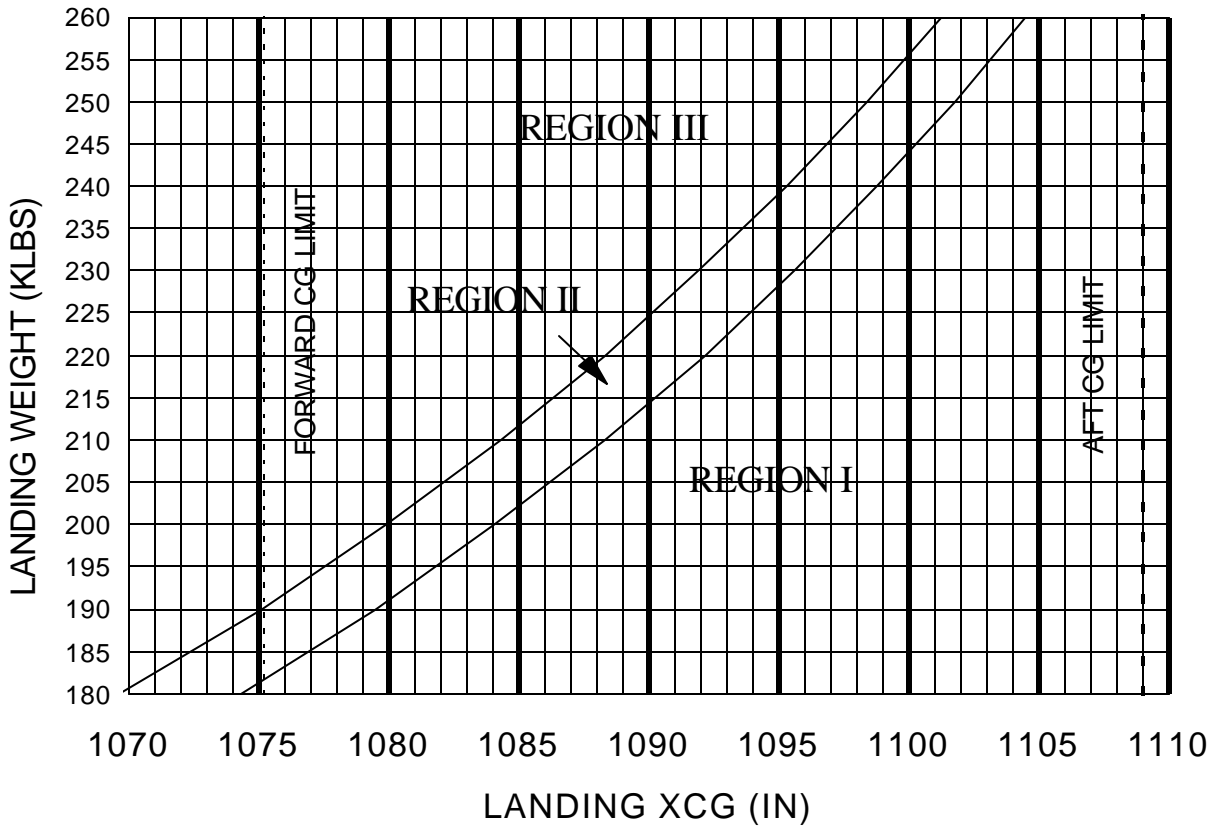
Landing Regions Chart for Medium Lakebed Hardness
