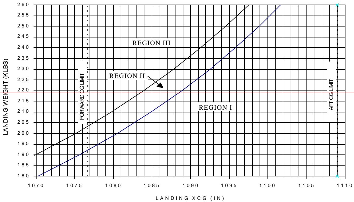
Landing Regions Chart for Hard Lakebed Hardness
