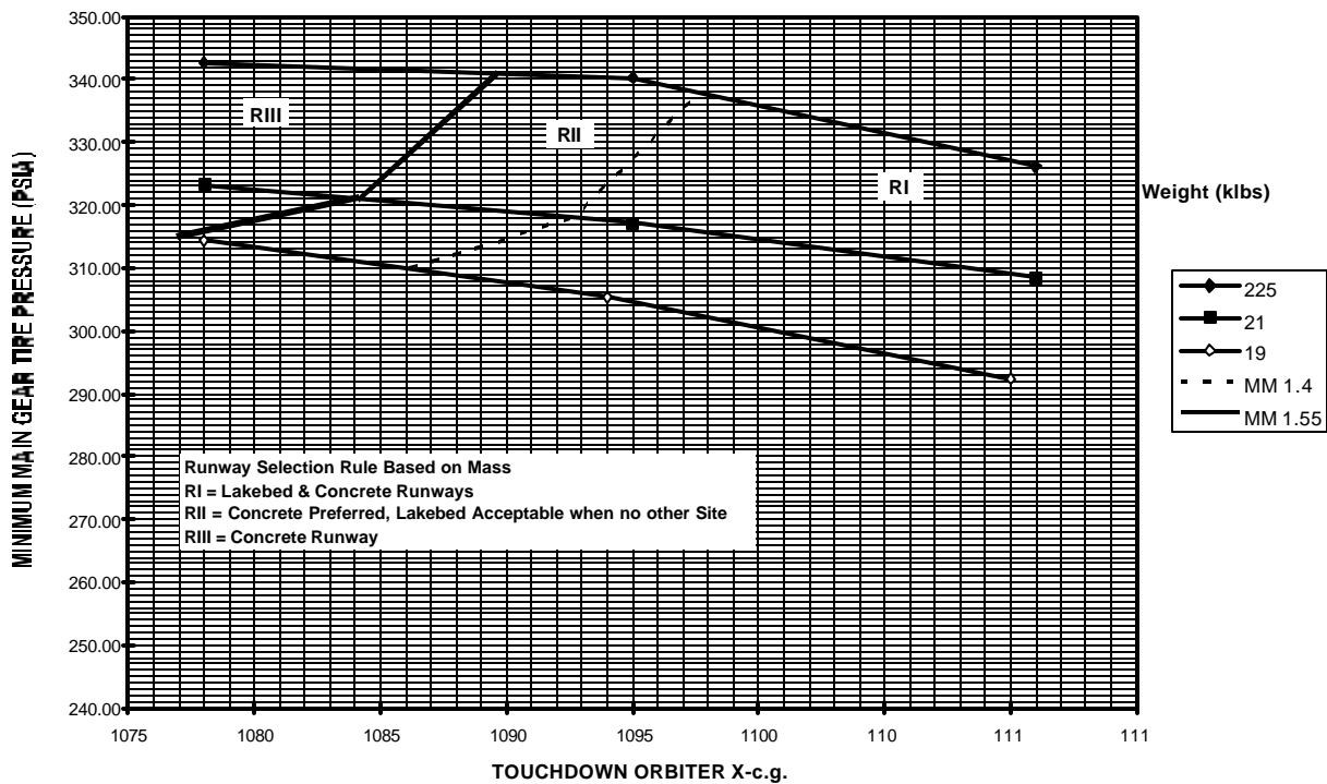
OI-23 Minimum Orbiter Main Gear Tire Pressure Mission Planning Assessments - Lakebed Runways All Normal & Intact Abort Landings (Nominal Vderotate @ 185 keas)
