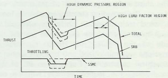
Thrust Profiles
