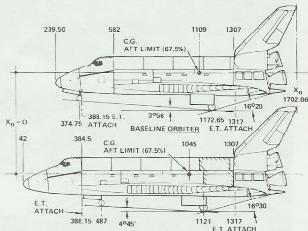
Comparison With Baseline Orbiter
