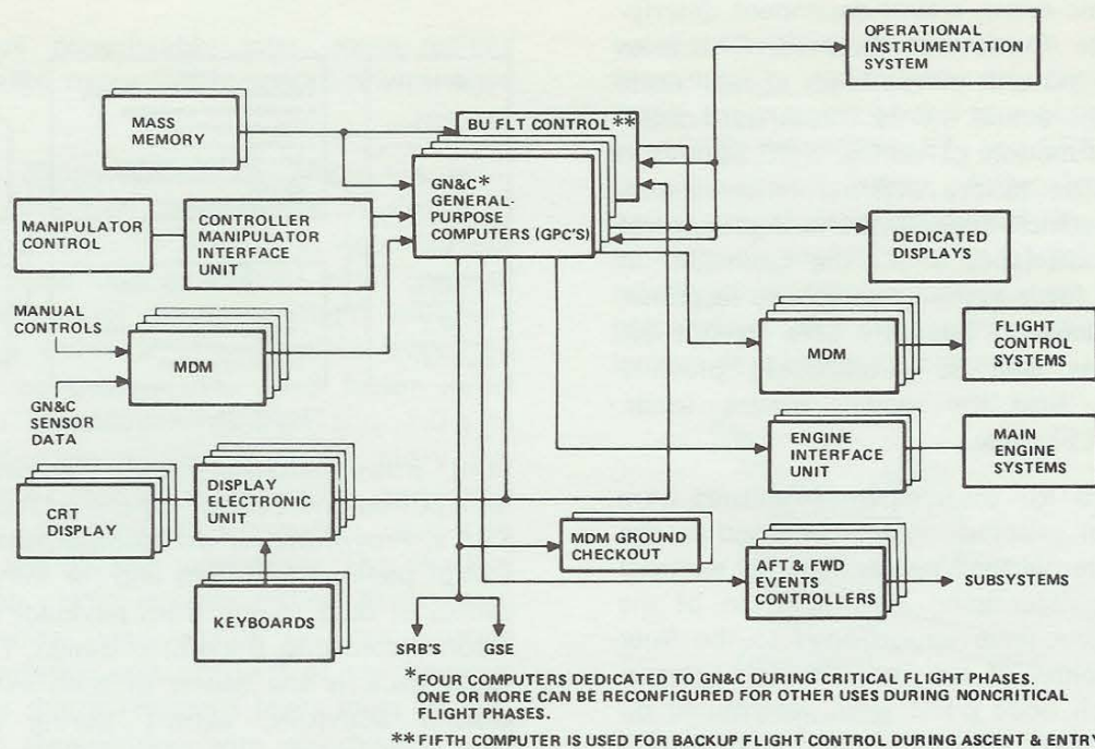
Data Processing and Software Subsystem
