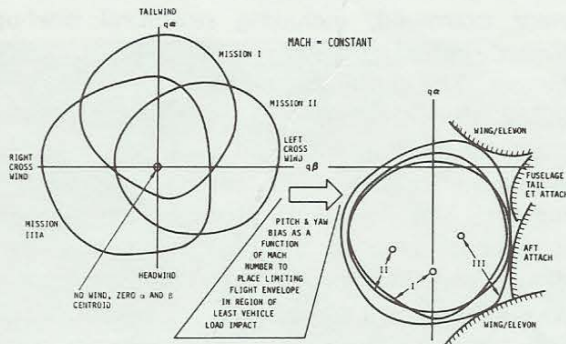
Trajectory Biasing
