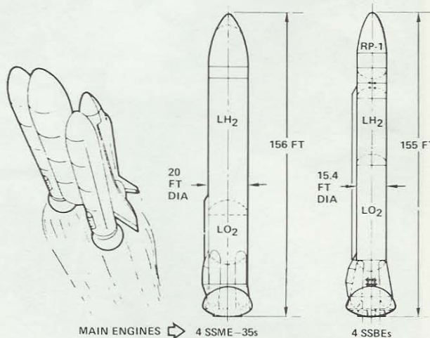
Liquid Propellant Booster Options
