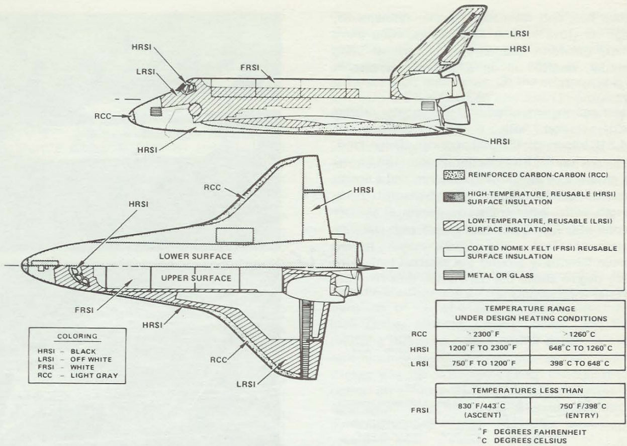
Thermal Protection System
