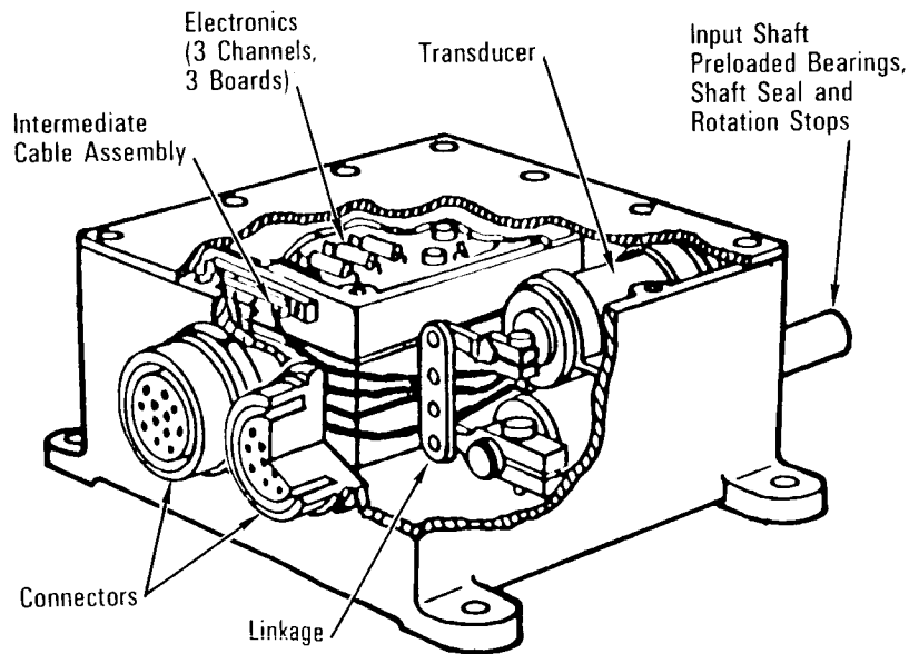
Rudder Pedal Transducer Assembly
