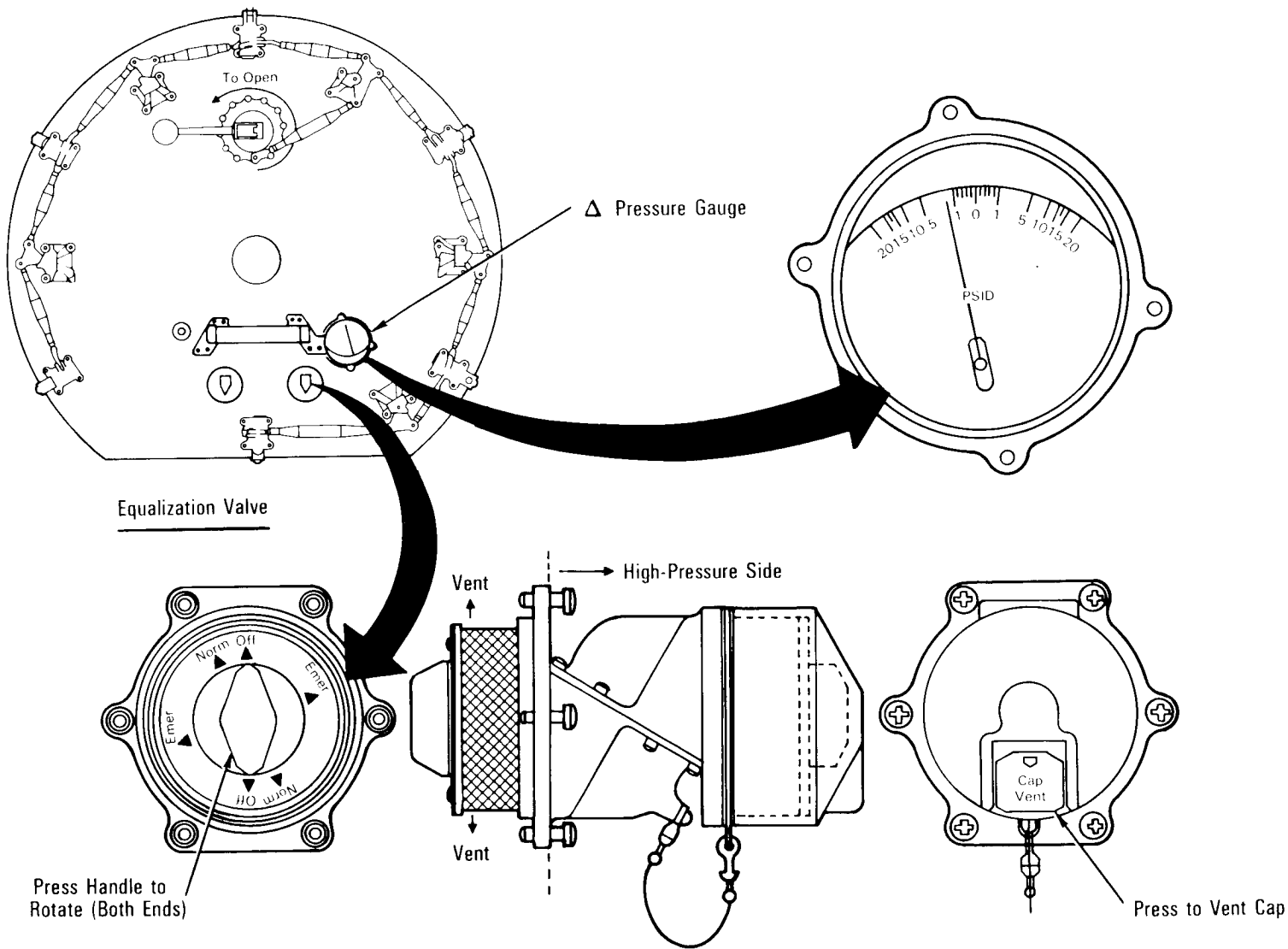
Airlock Repressurization
