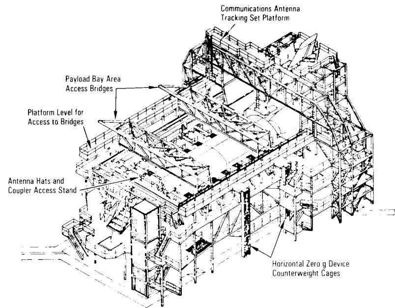
Orbiter Processing Facility Access Platforms, Front View
