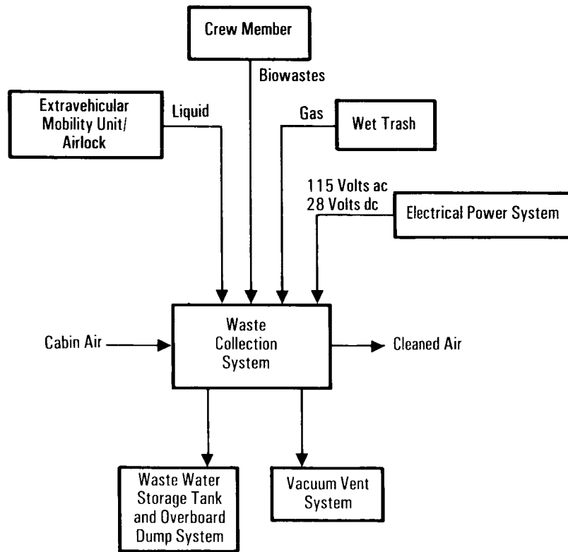
Waste Collection System
