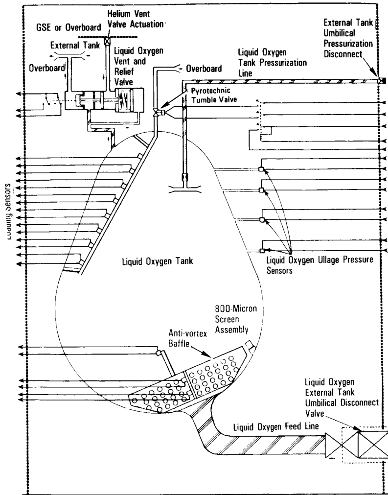
External Tank Schematic, Liquid Oxygen Tank Detail
