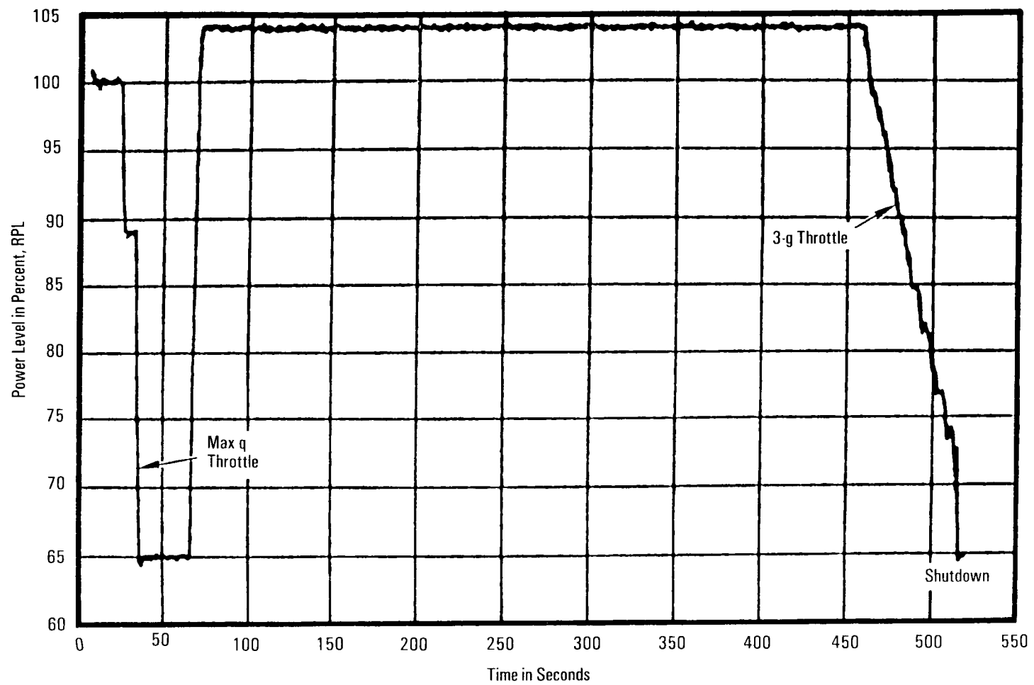
Typical 104-Percent SSME Mission—With Three Engines
