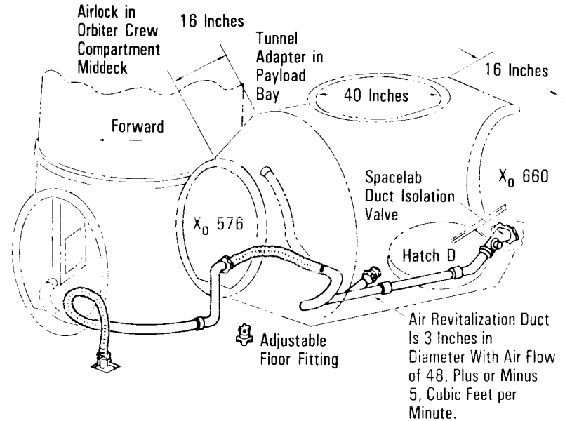
Air Circulation Duct Routing
