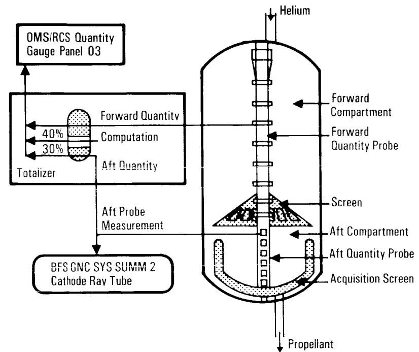
Orbital Maneuvering System Quantity Gauging
