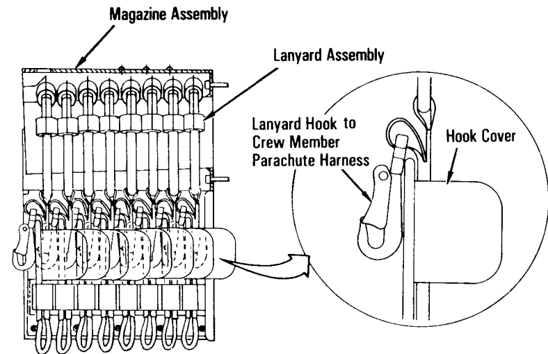
Escape Pole Magazine Assembly With Lanyards
