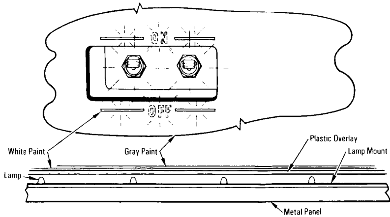
Panel Lighting Configuration
