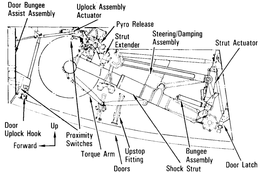
Nose Landing Gear Stowed
