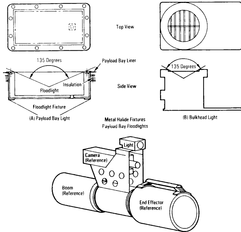
Remote Manipulator System Incandescent Light Fixture
