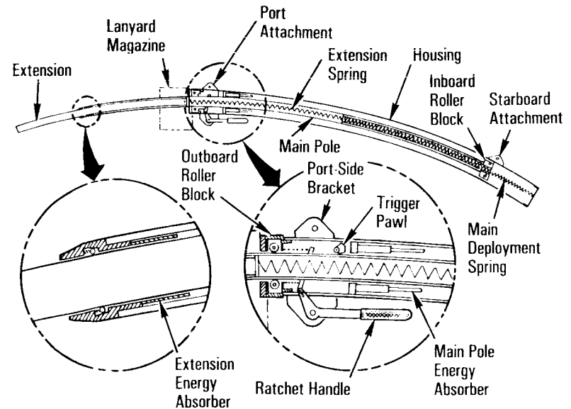
Escape Pole Deployment
