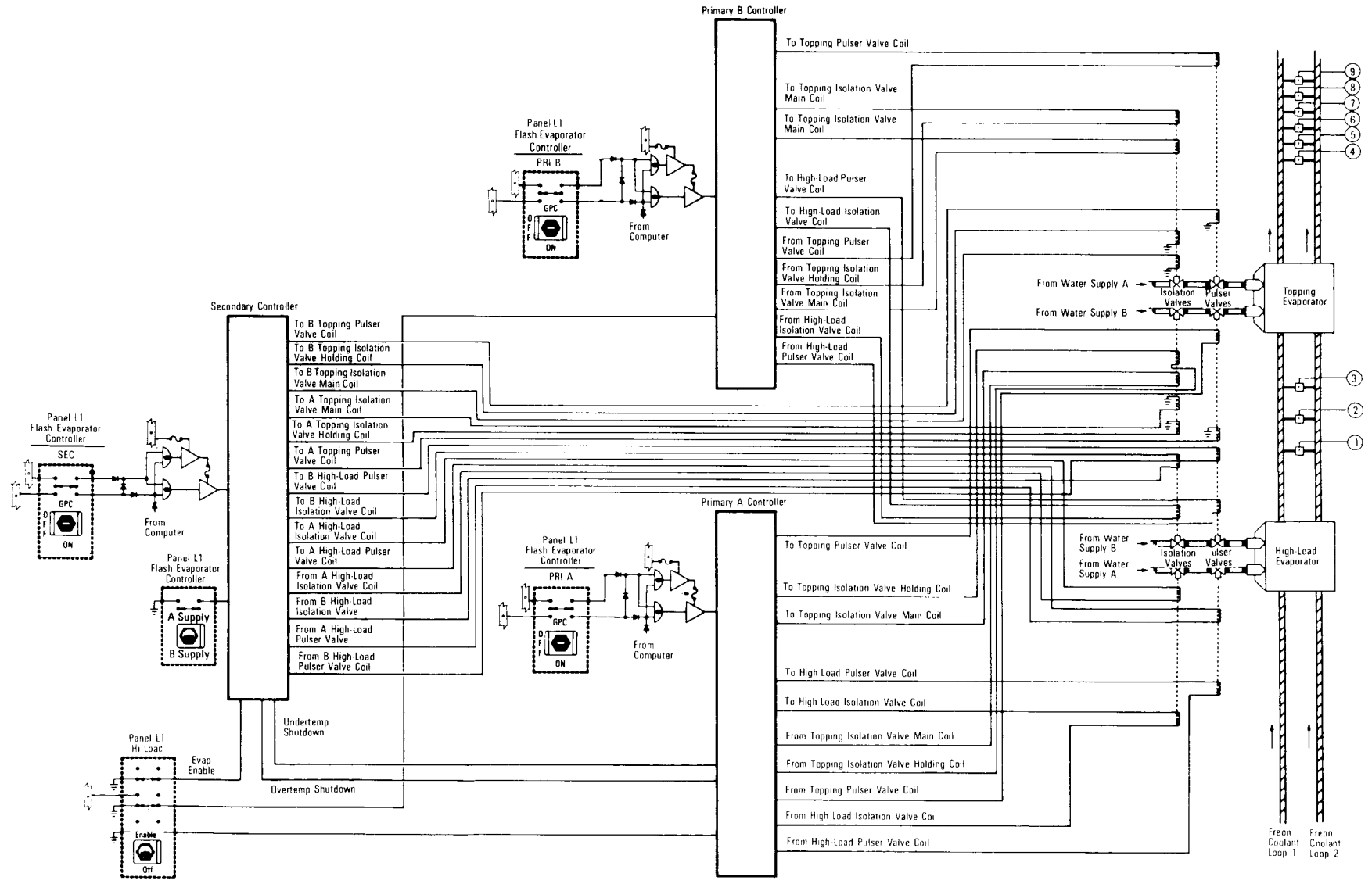
Flash Evaporator
