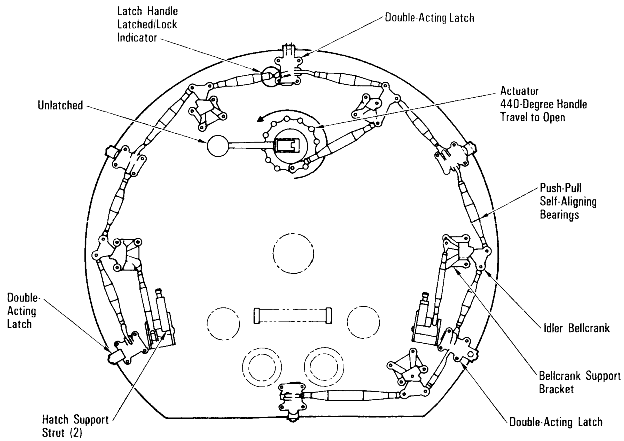
Airlock Hatch Latches
