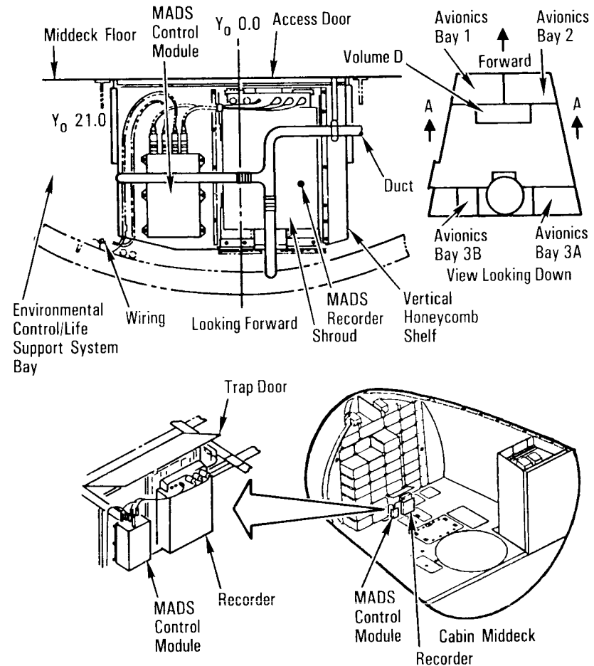
Modular Auxiliary Data System Equipment Location in Crew Compartment—Middeck of OV-103 (Discovery) and OV-104 (Atlantis)
