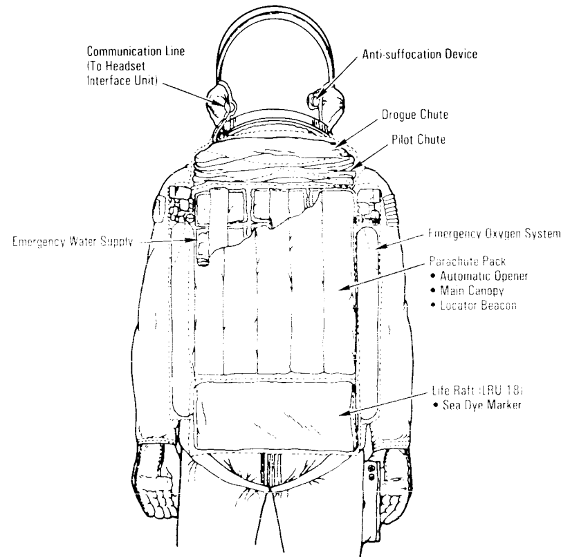
Crew Altitude Protection System
