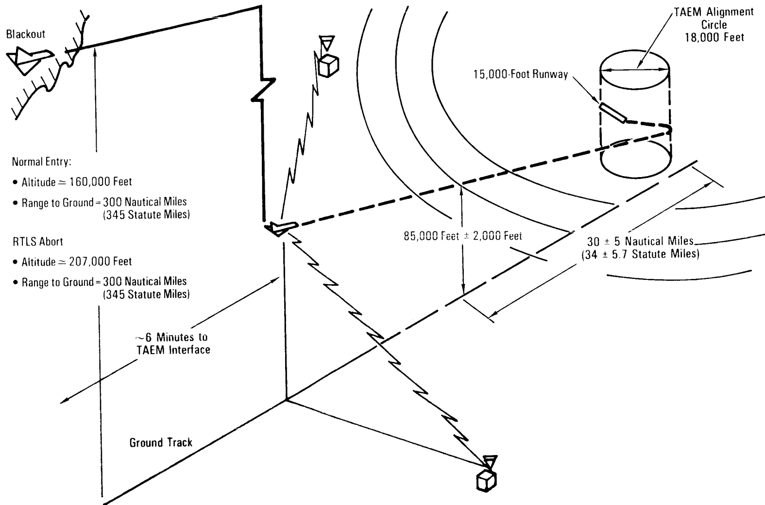
TACAN Approach Geometry
