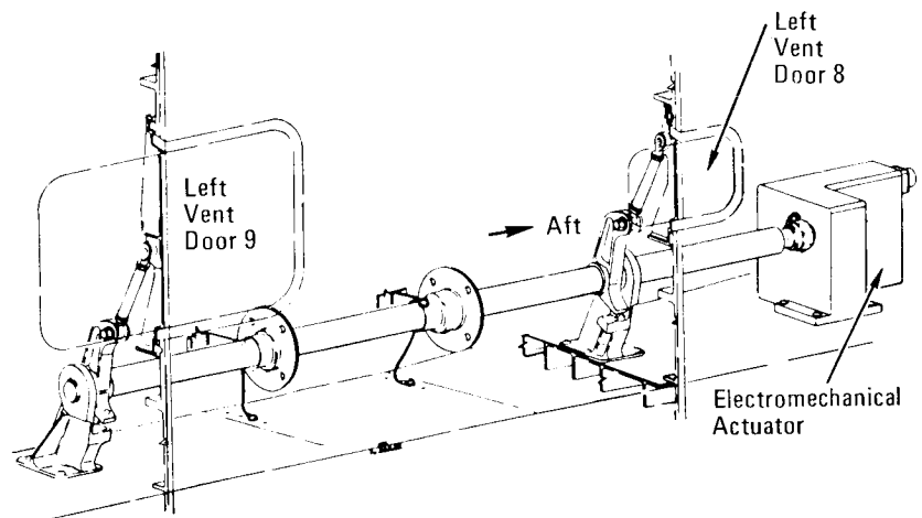
Vent Doors (8 and 9)
