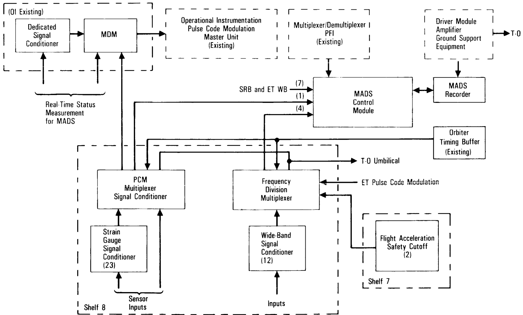
Modular Auxiliary Data System Block Diagram—OV-103 (Discovery) and OV-104 (Atlantis)
