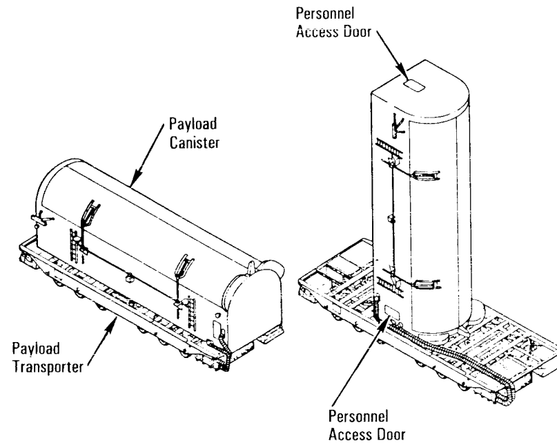
Horizontal Transportation Mode
