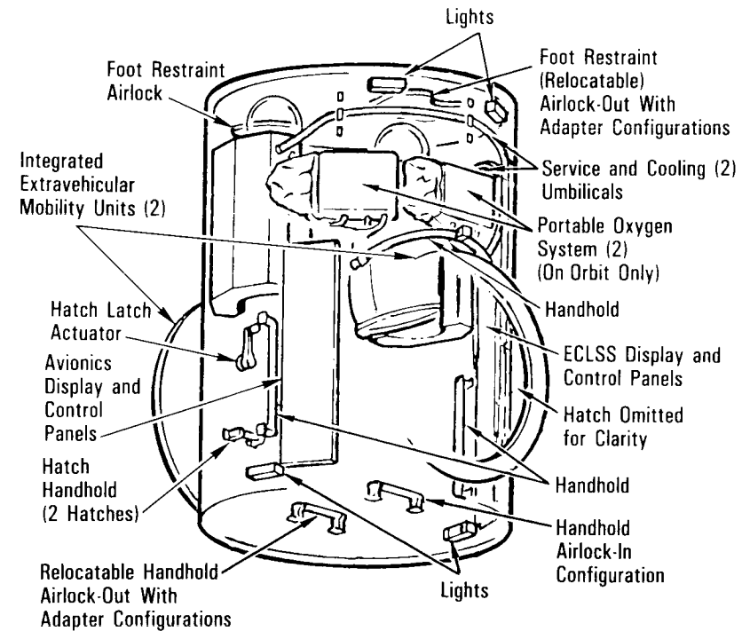
Airlock
