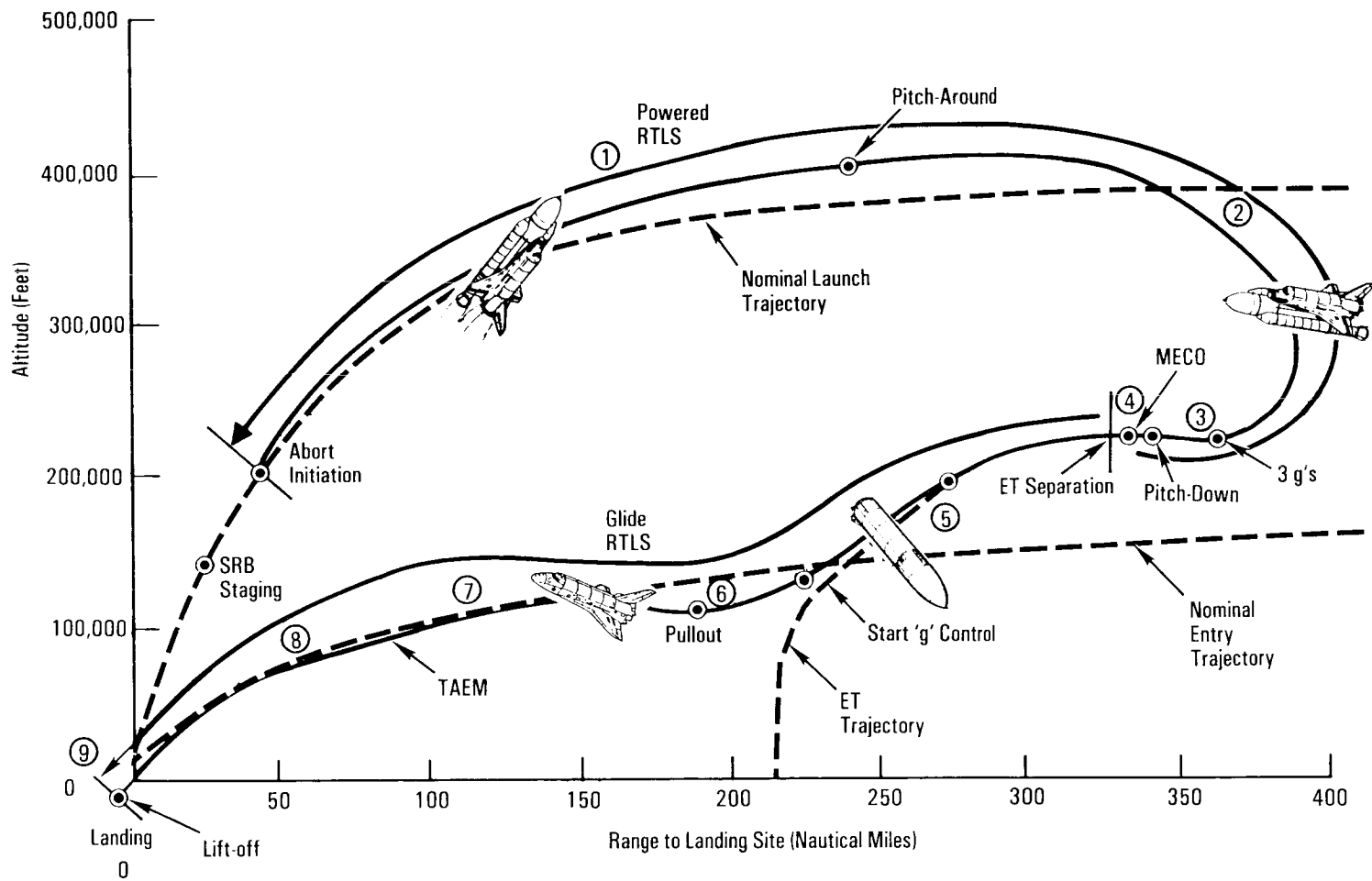
Return to Launch Site Flight Phases
