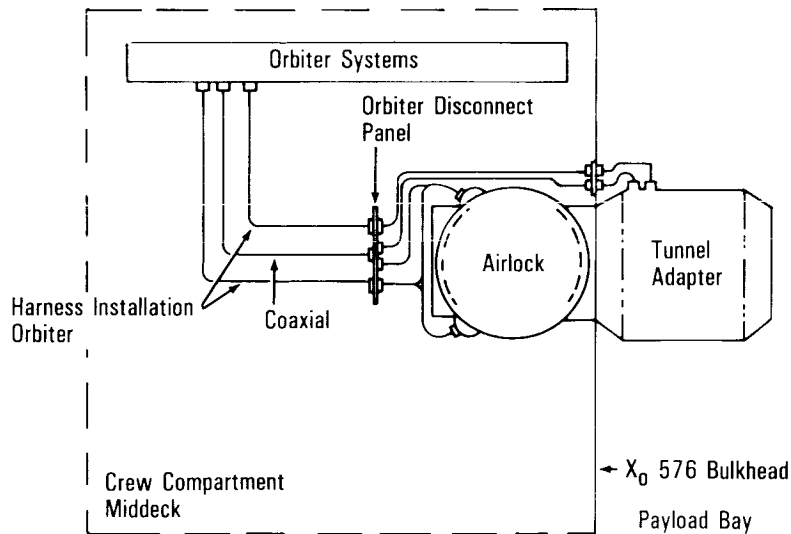
Airlock/Tunnel Adapter Harness Installation and Coaxial Antenna
