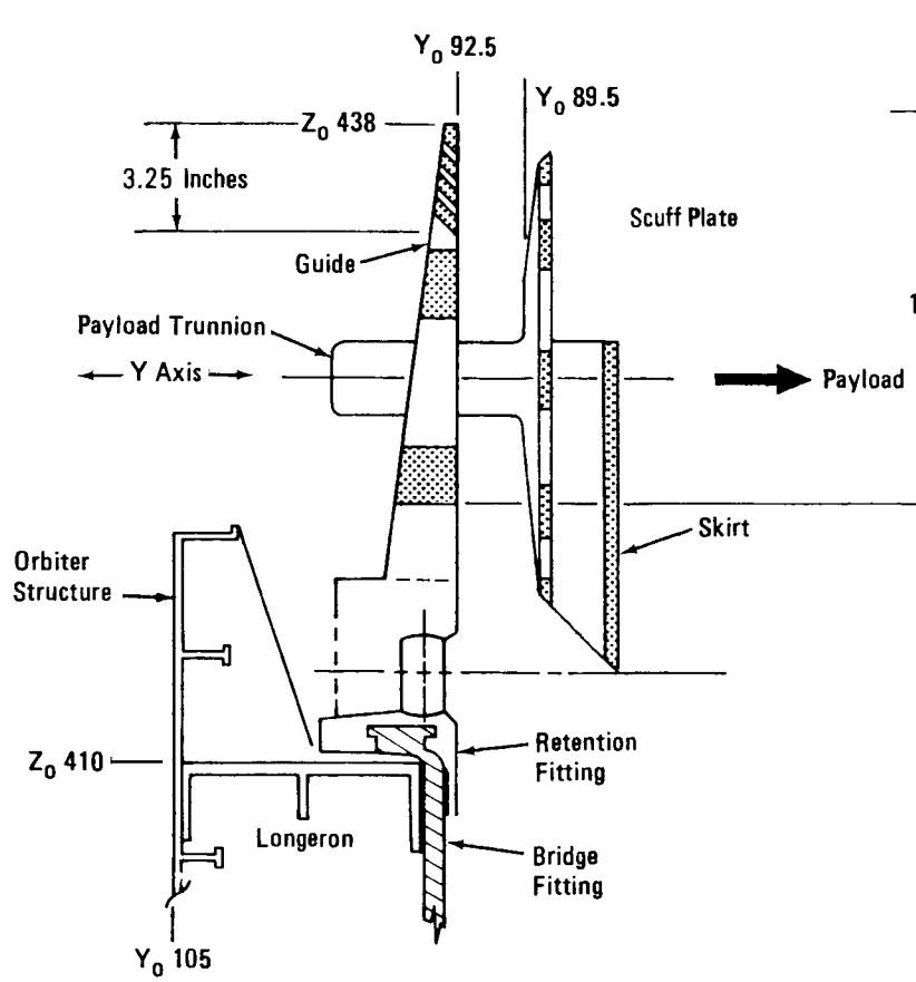
Orbiter Payload Guide and Trunnion/Scuff Plate (Nominal)
