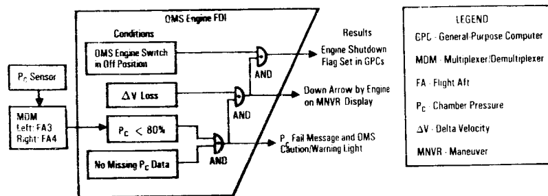
Orbital Maneuvering System Fault Detection and Identification Software
