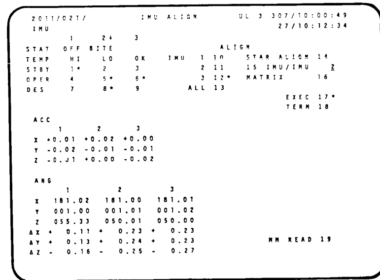
Cathode Ray Tube Display
