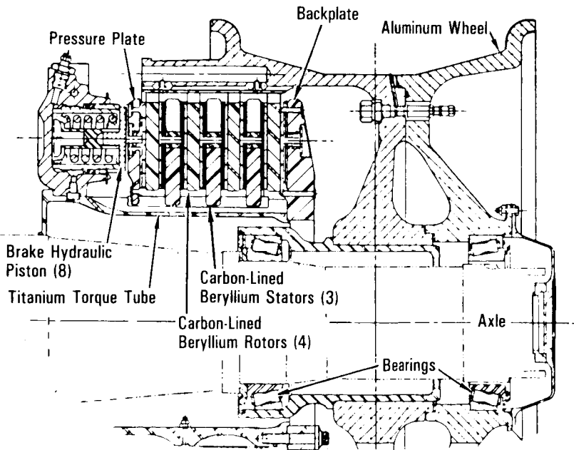
Wheel Brake Assembly
