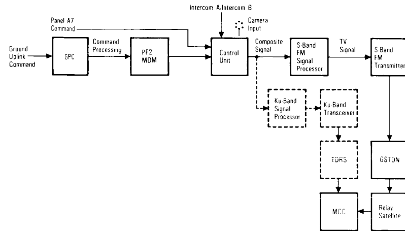
Ground Command Systems Television Data Flow
