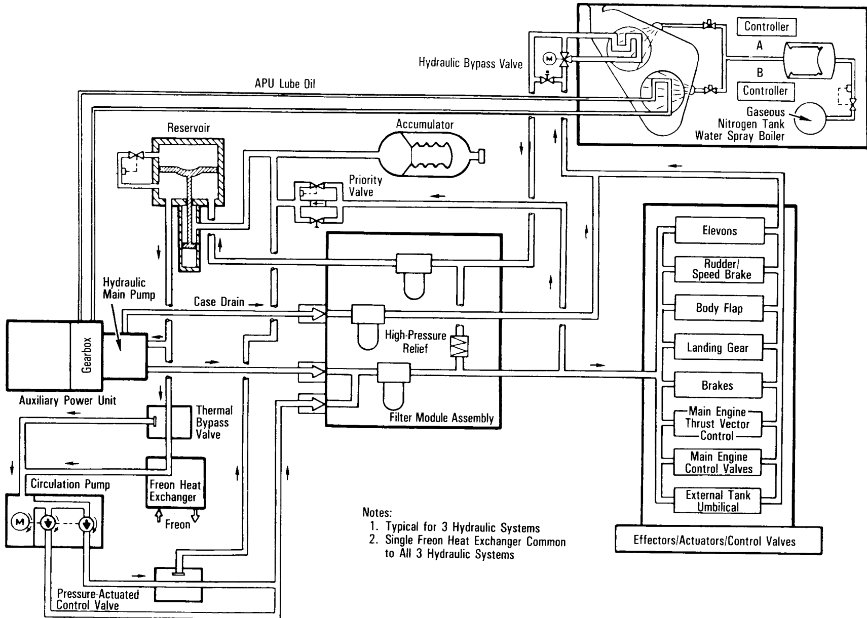
APU, Water Spray Boiler and Hydraulic System Schematic
