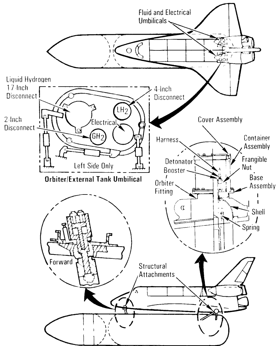
Orbiter/External Tank Separation System
