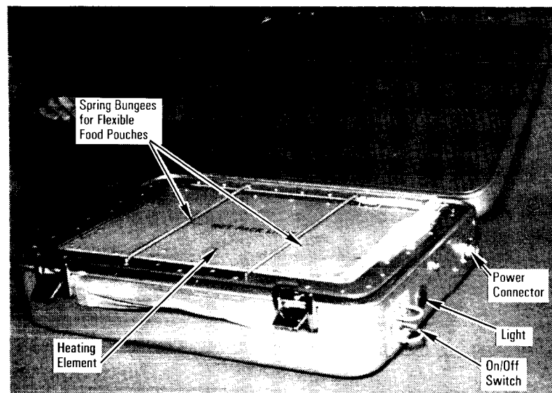
Food Warmer
