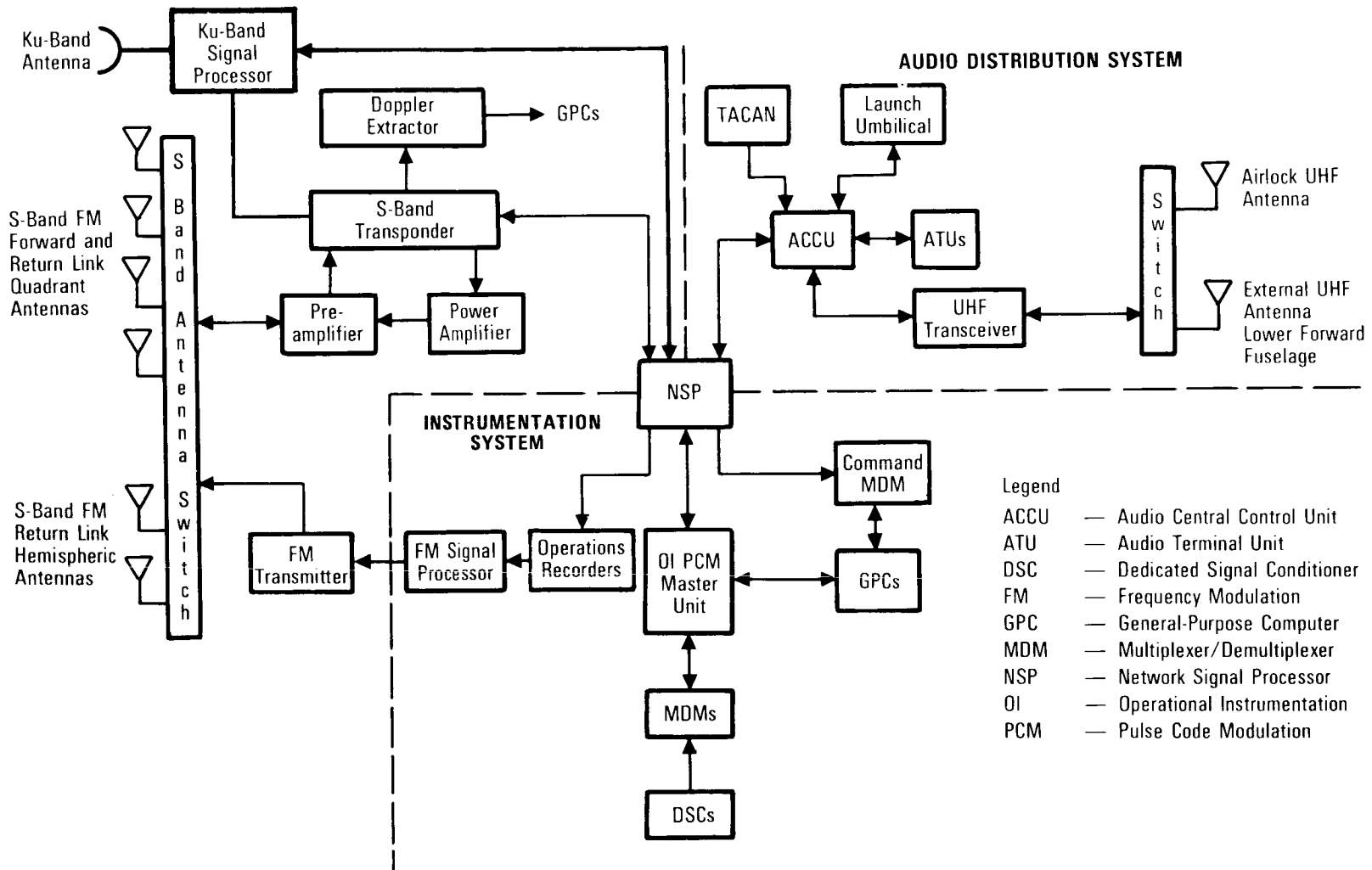
Communications System
