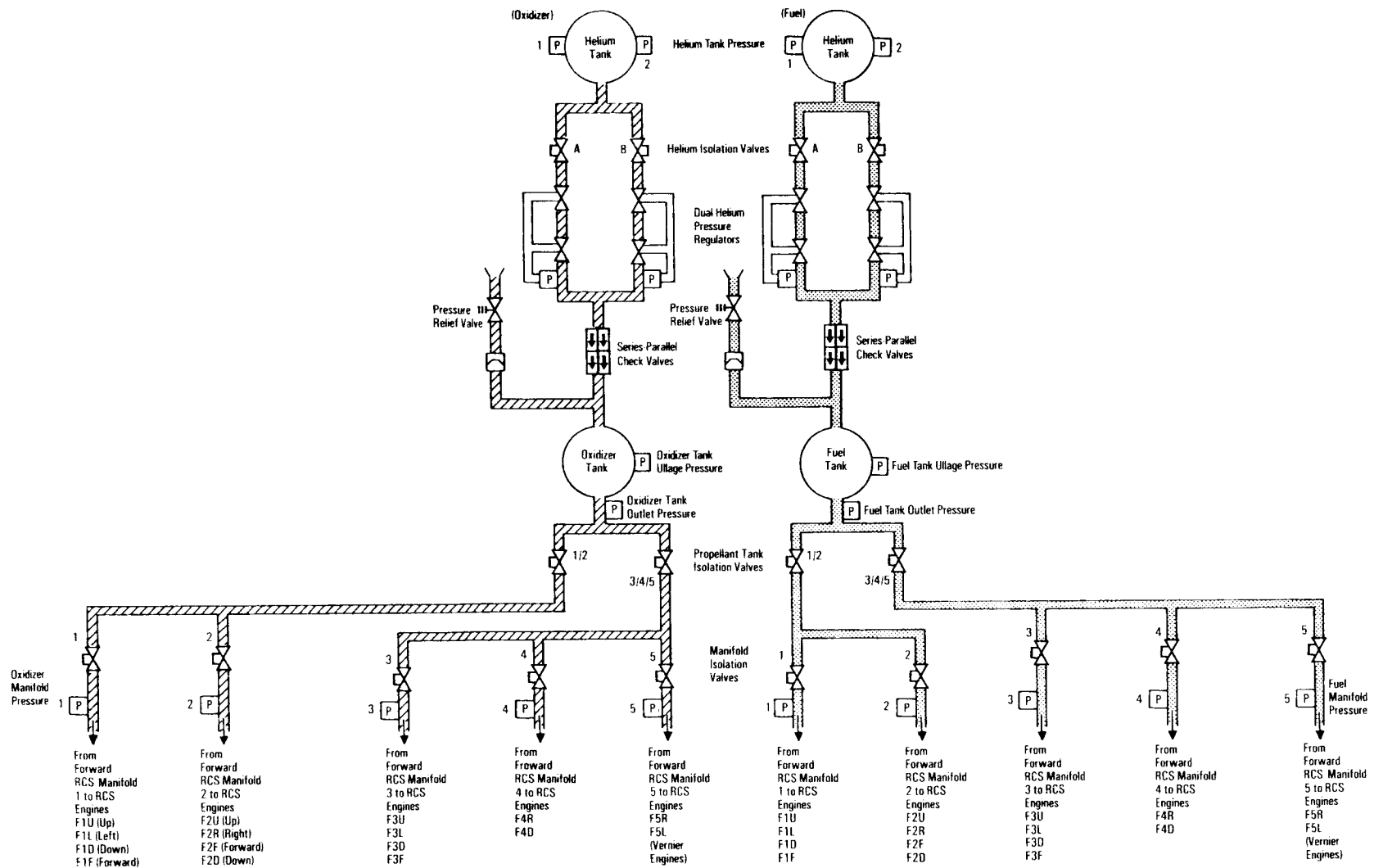
Forward Reaction Control System Pressurization and Propellant Feed System
