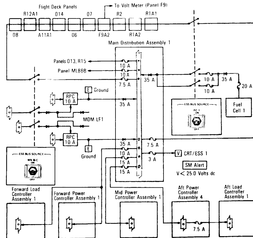
Essential Bus/BC Distribution
