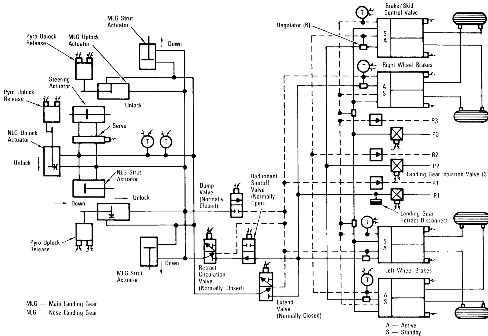
Hydraulic Actuator System—Landing Gear and Brake
