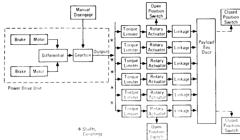
Payload Bay Door Drive System Control Mechanical Block Diagram
