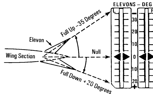
Surface Position Indicator Elevon Travel
