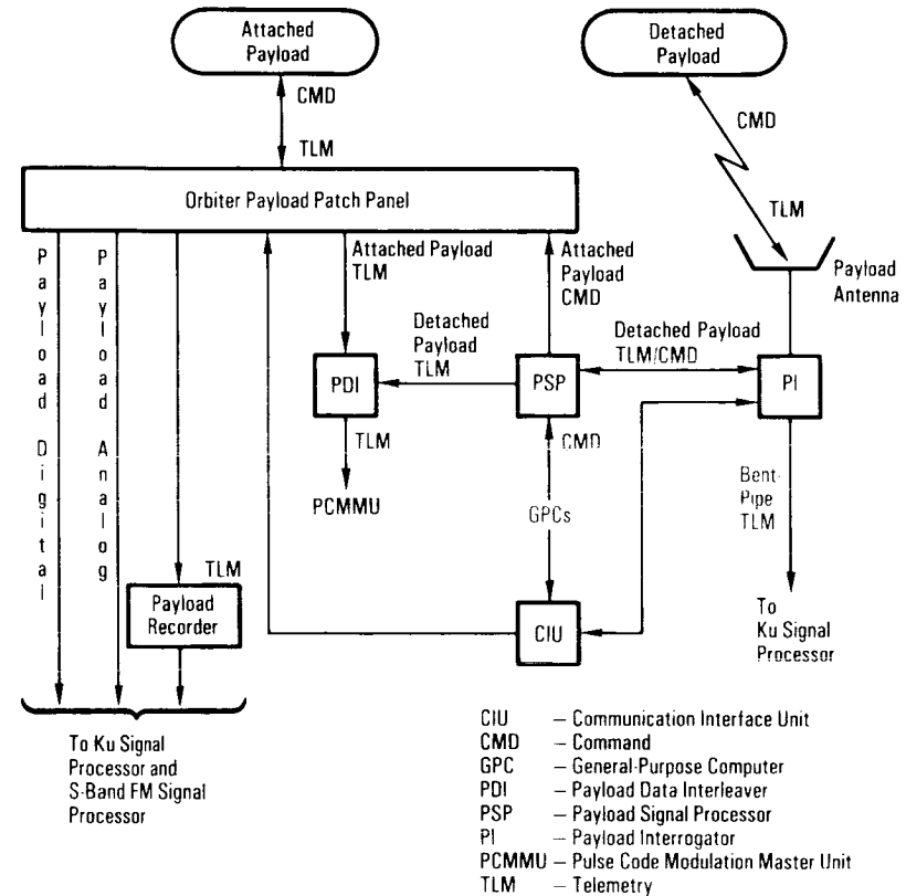
Payload Communication System
