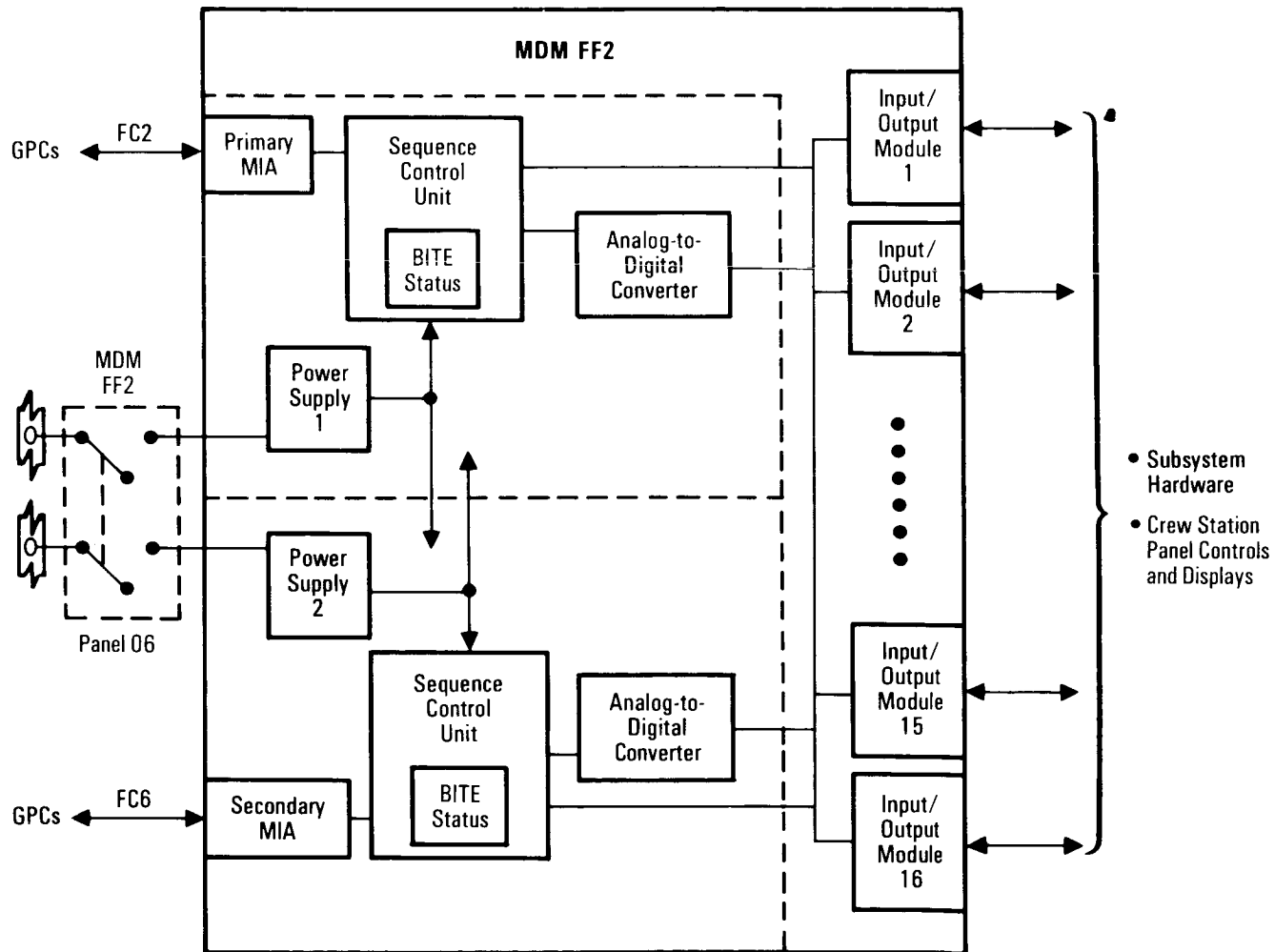
Multiplexer/Demultiplexer Functional Block Diagram
