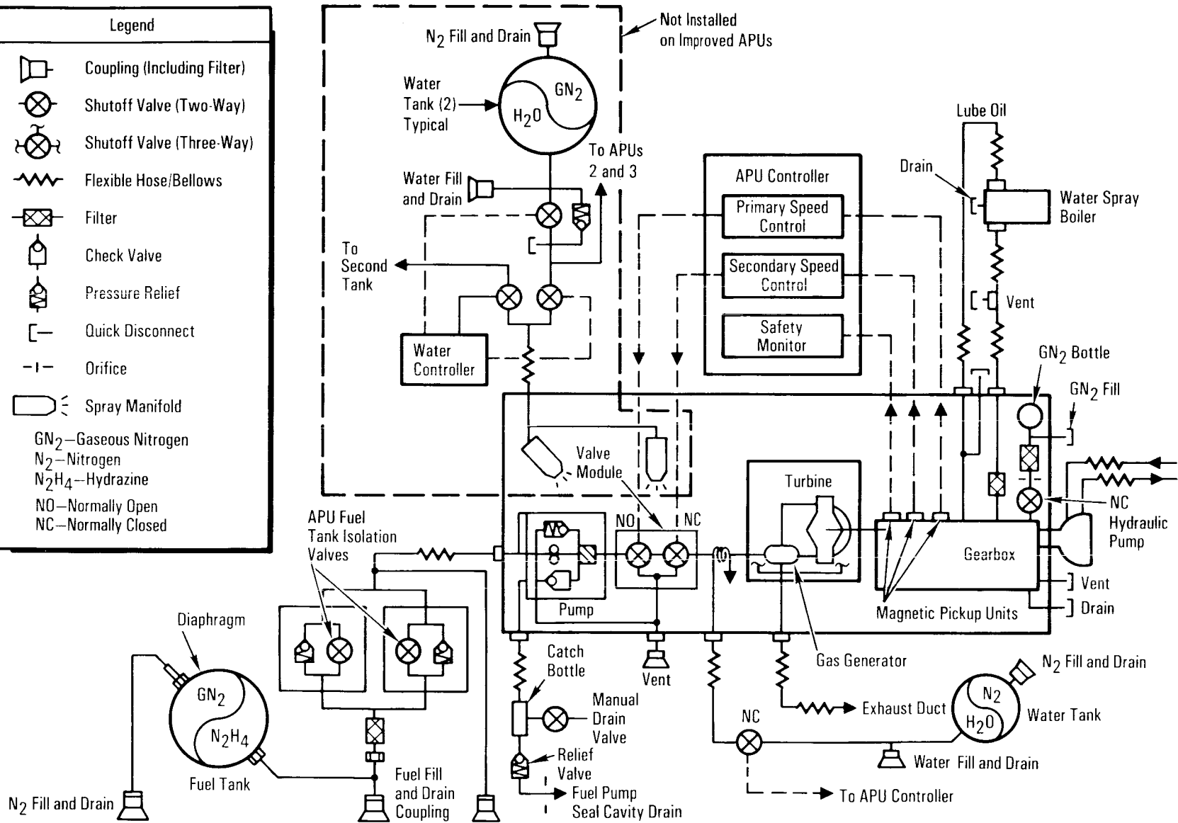
Auxiliary Power Unit
