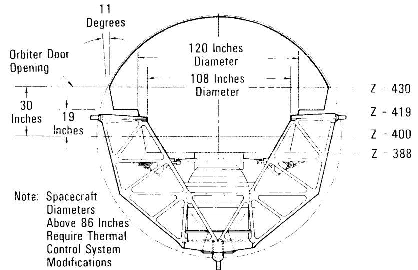
Maximum Spacecraft Envelope With PAM-D
