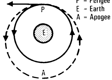
Posigrade Thrusting Maneuver
