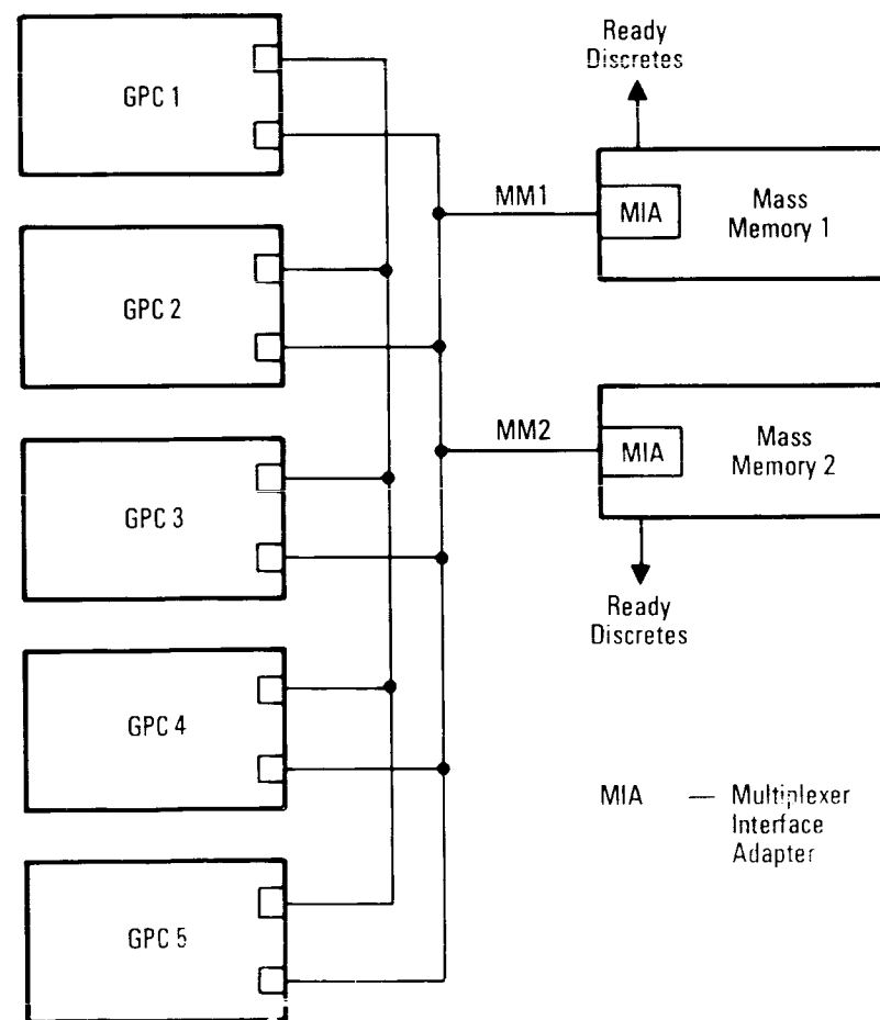
Mass Memory Data Buses
