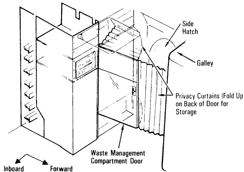
Waste Management System Privacy Curtains
