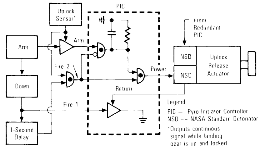
Uplock Release and Pyro Actuator Circuit (Simplified)
