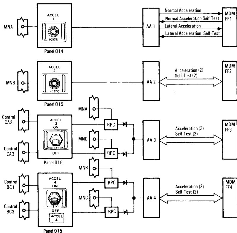
Accelerometer Assembly Power and Data Interfaces
