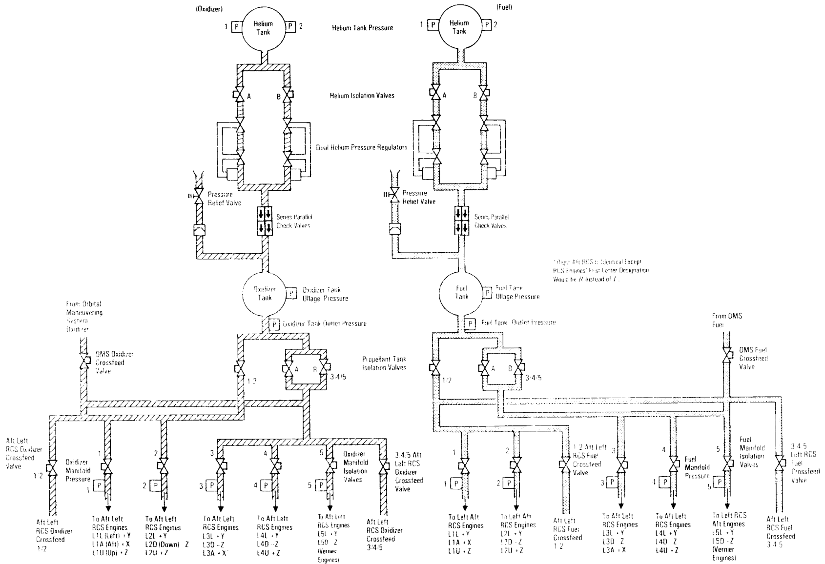
Left Aft Reaction Control System Pressurization and Propellant Feed System
