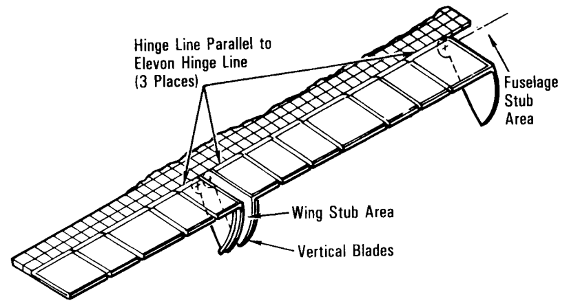
Wing Seal Panel Arrangement
