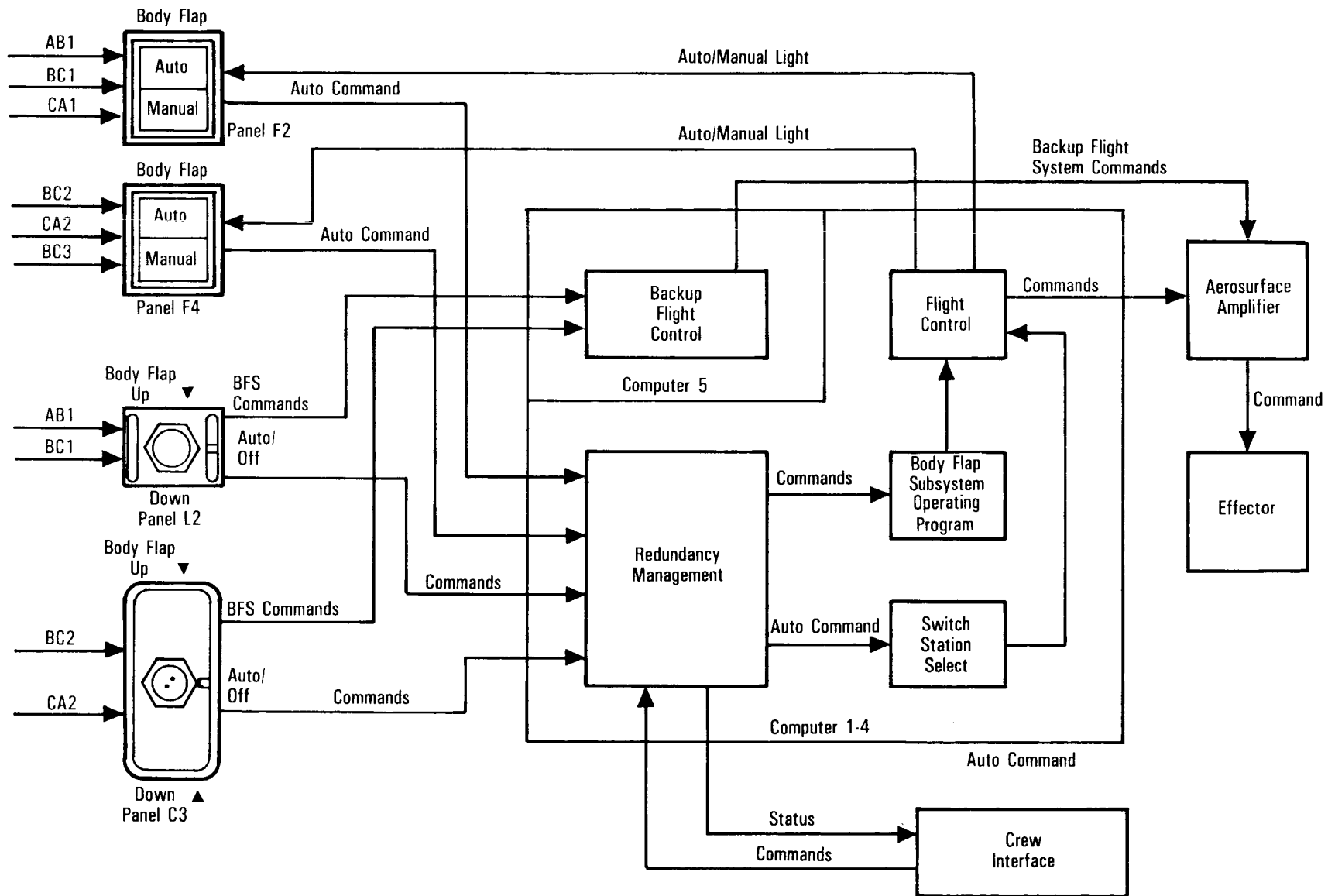
Body Flap
