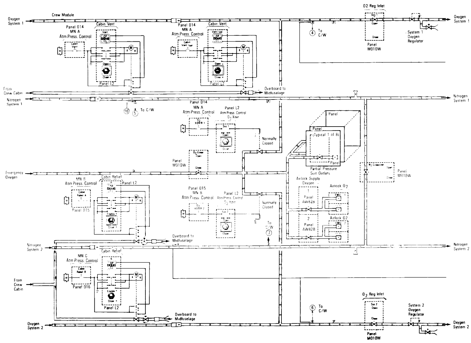
Air Revitalization System Pressurization (Sheet 2 of 3)
