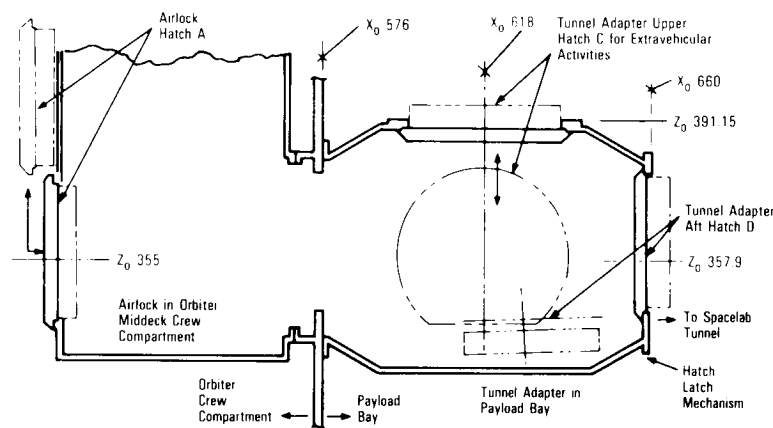
Airlock and Tunnel Adapter Hatch Mechanical Systems
