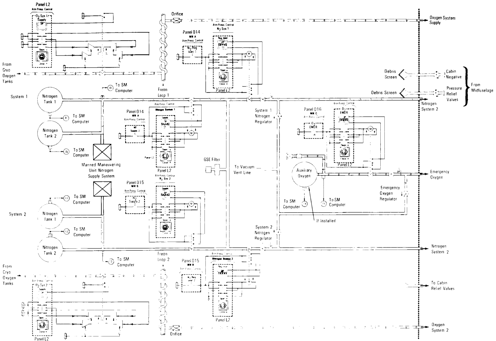
Air Revitalization System Pressurization (Sheet 1 of 3)
