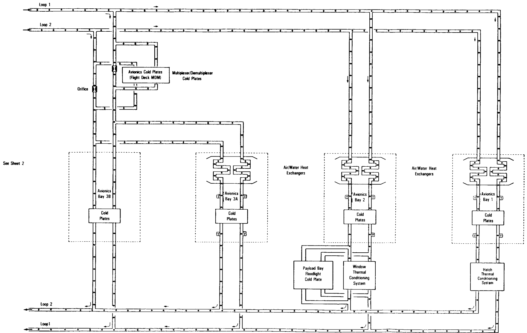
Water Coolant Loops (Sheet 3 of 3)
