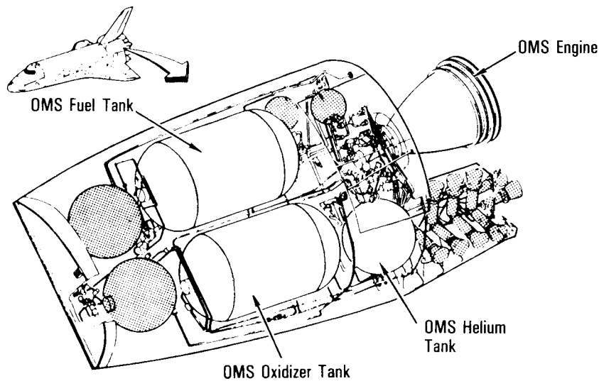
Orbital Maneuvering System
