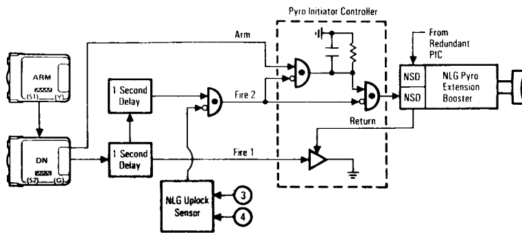
Nose Landing Gear Extension Booster Pyro Circuit
