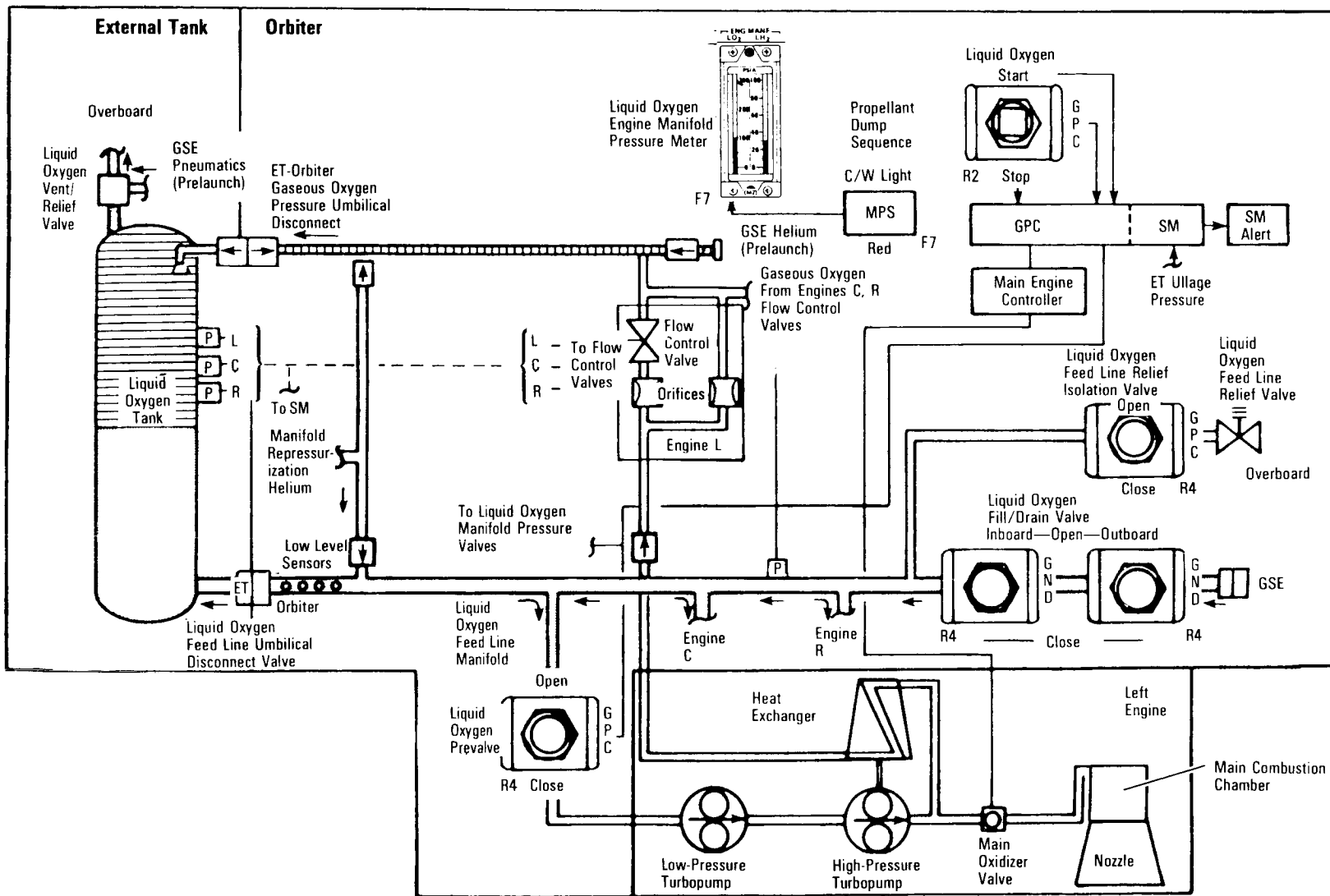
Oxidizer Flow
