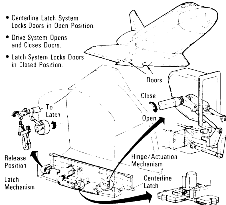
Orbiter Umbilical Doors
