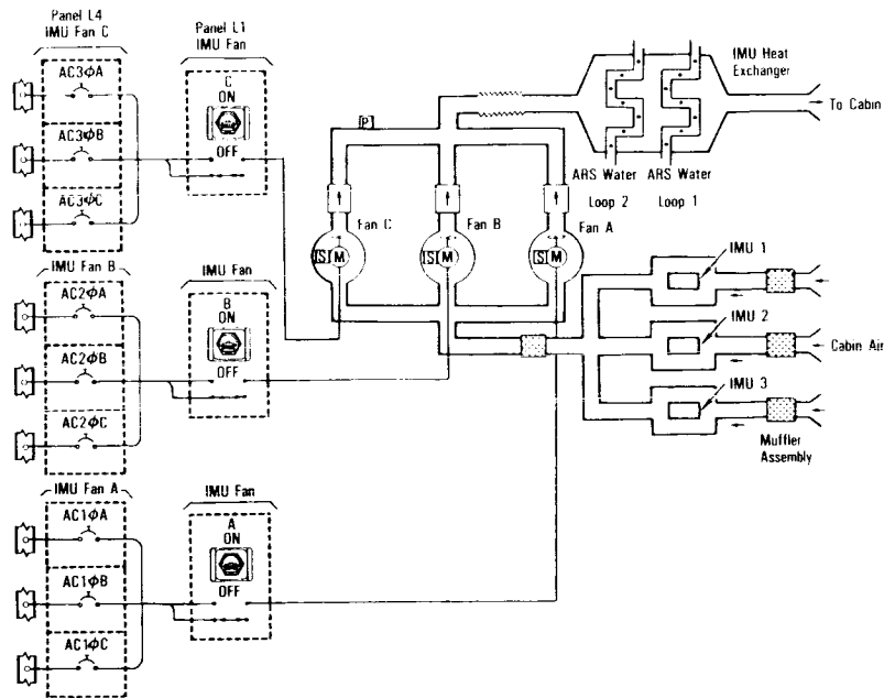
IMU Air Circulation
