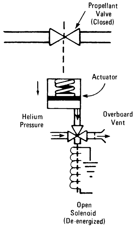
② Control Switch in Closed Position
