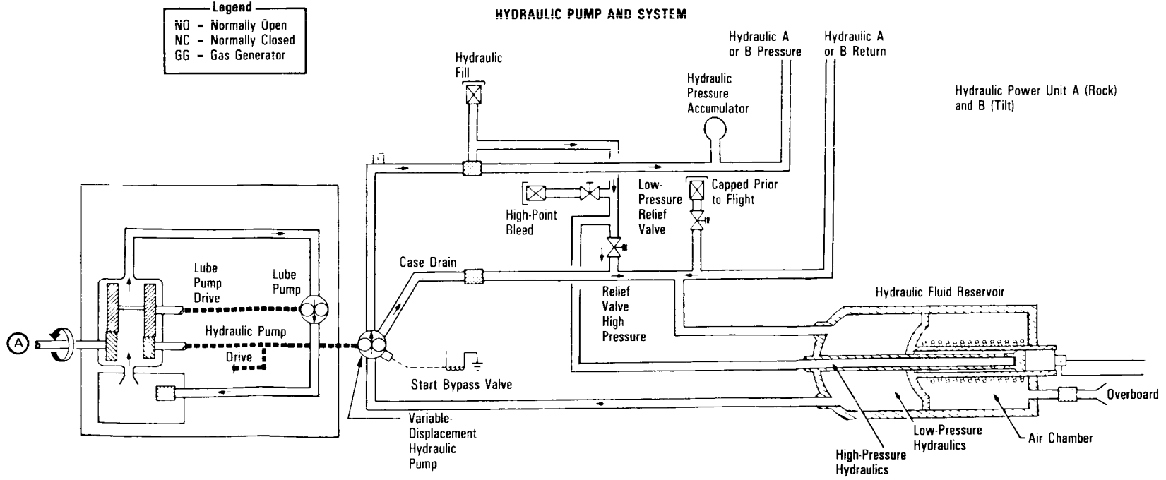
Auxiliary Power Unit and Hydraulic Pump System
