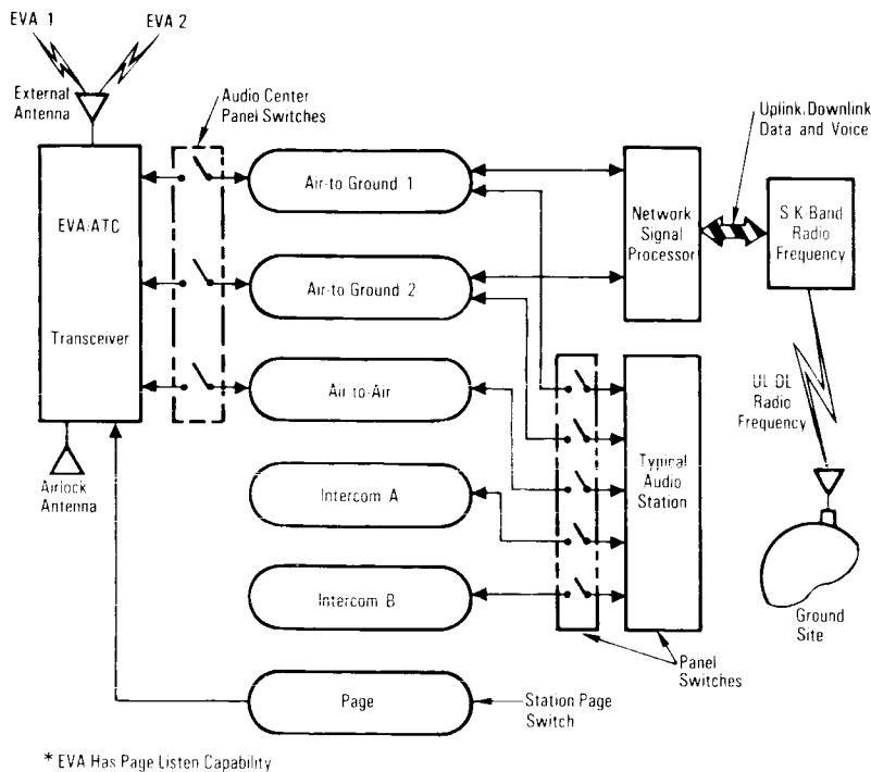
Ultrahigh Frequency/Audio Interfaces
