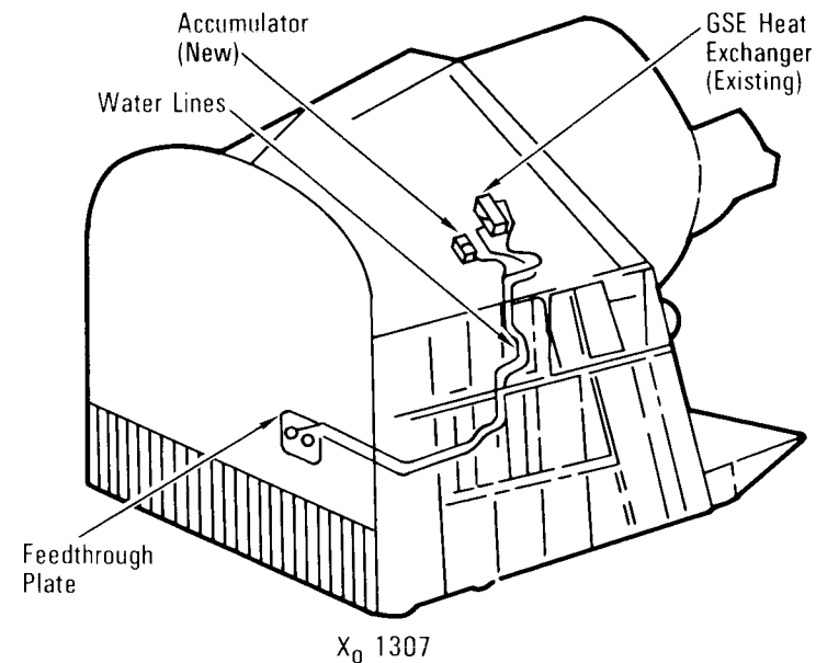
Water Coolant System and Accumulator in Aft Fuselage for RTG Cooling
