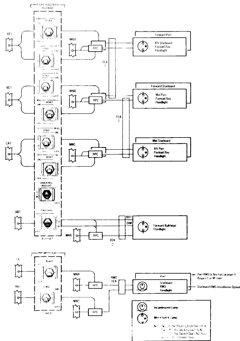
Payload Bay and Remote Manipulator System Floodlights
