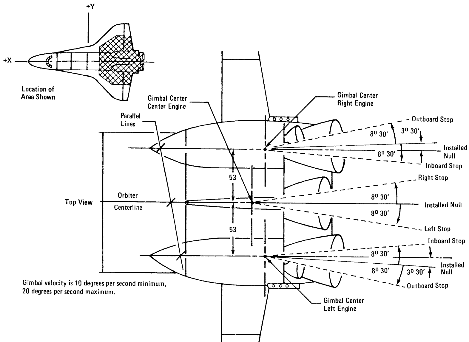
SSME Gimbal Yaw Axis
