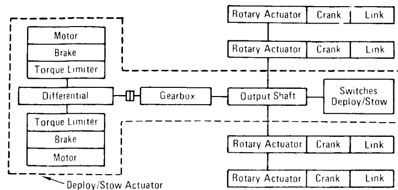
Deployable Radiator Deploy/Stow Control
