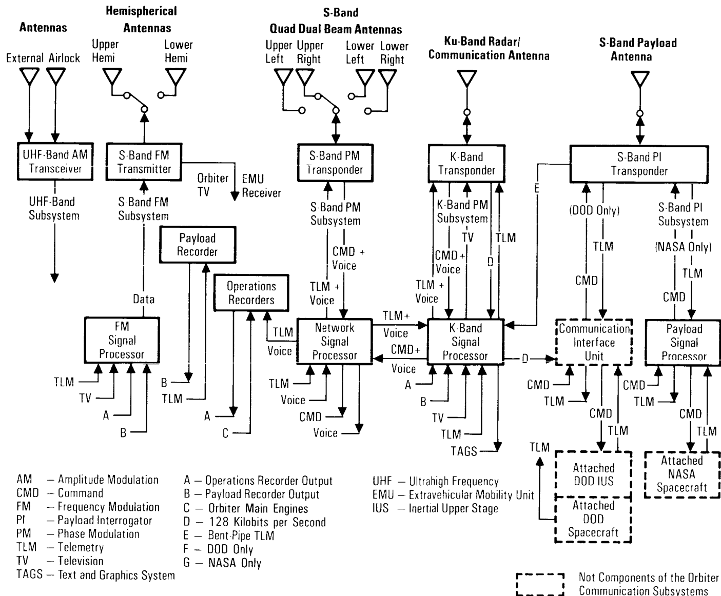
Radio Frequency and Signal Processor
