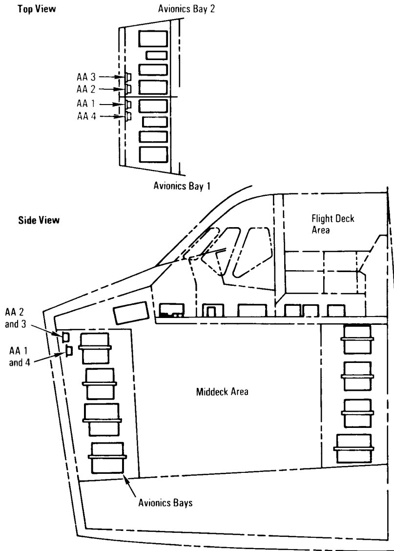
Orbiter Accelerometer Locations
