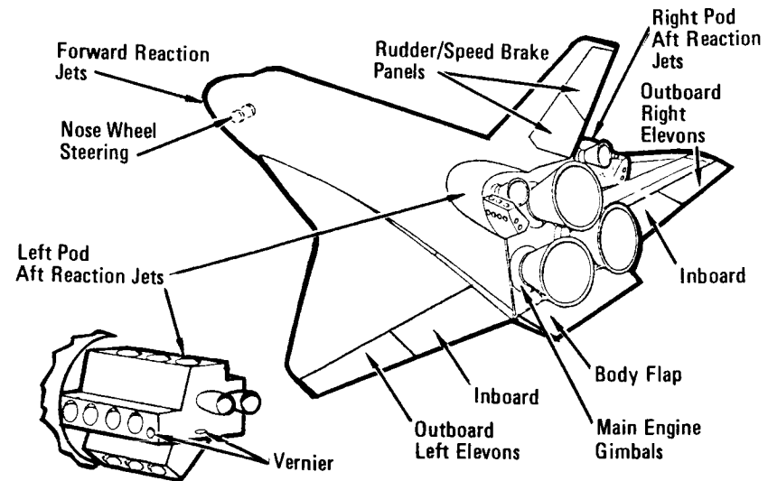
Flight Control Hardware Effector Elements
