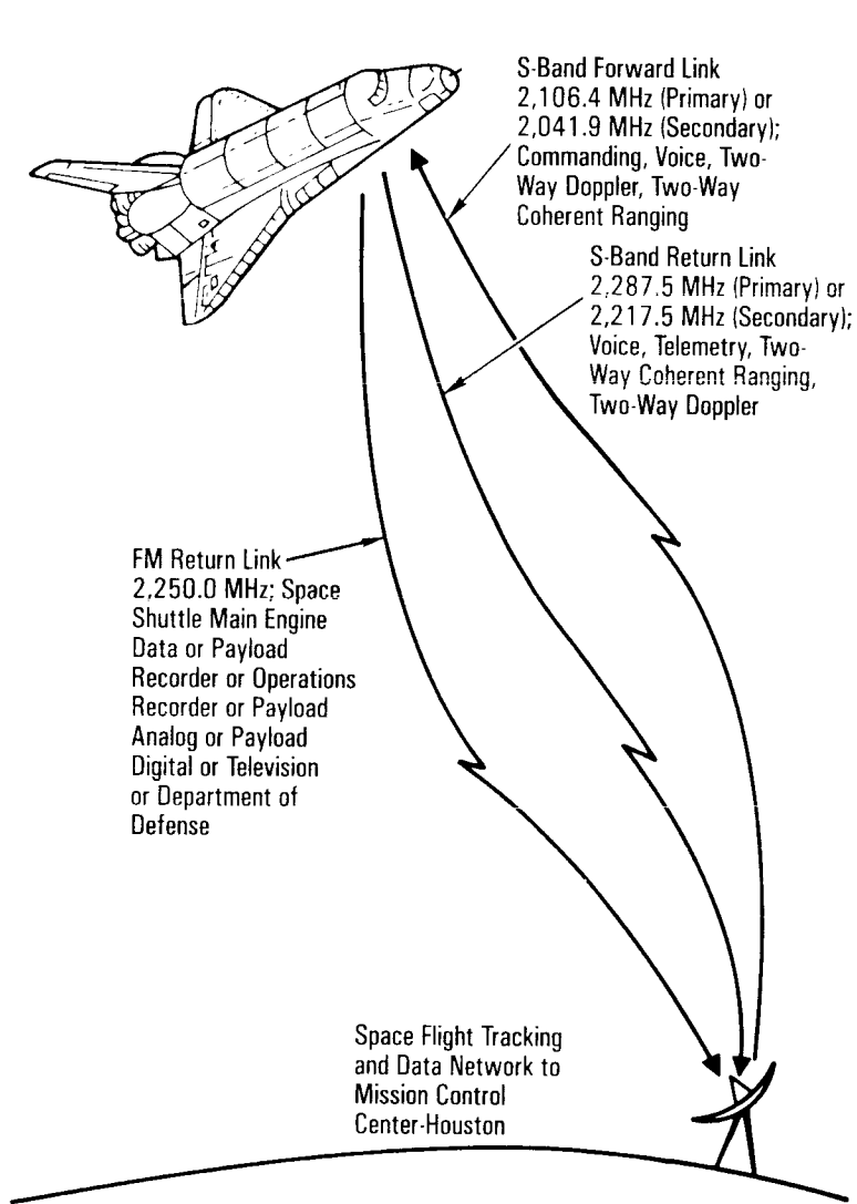
NASA S-Band Communications With Space Flight Tracking and Data Acquisition Network
