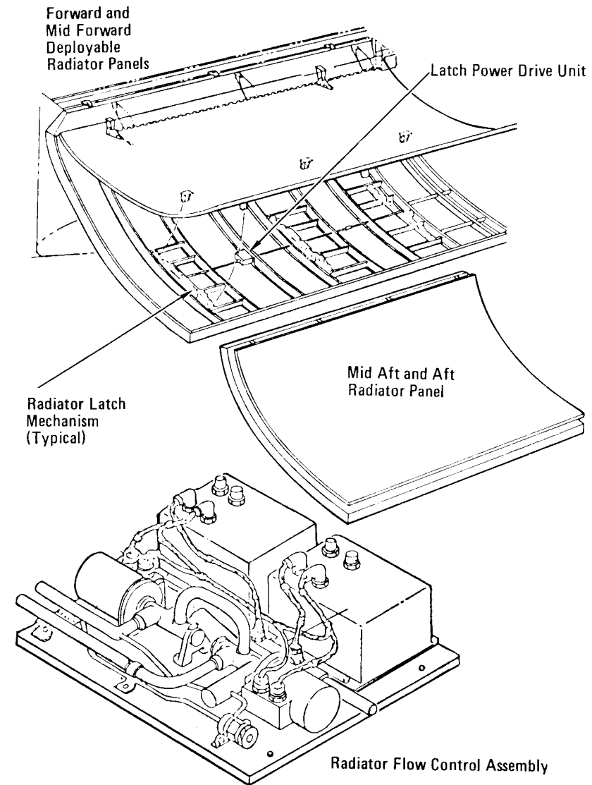
Radiators and Radiator Flow Control Assembly
