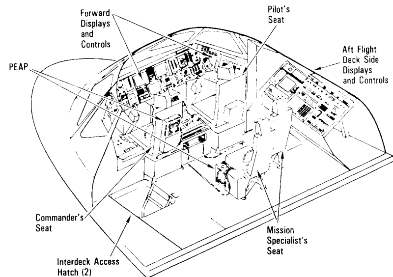
Crew Compartment Flight Deck
