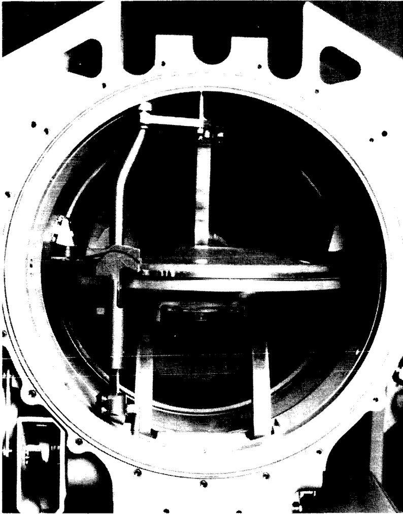
17-Inch Disconnect With Latch Feature Rotated 90 Degrees on One Flapper Valve, Disengaging Latch Permitting Flapper to Close (Other Flapper Valve Removed to Show Unlatch Feature, Disengaged)
