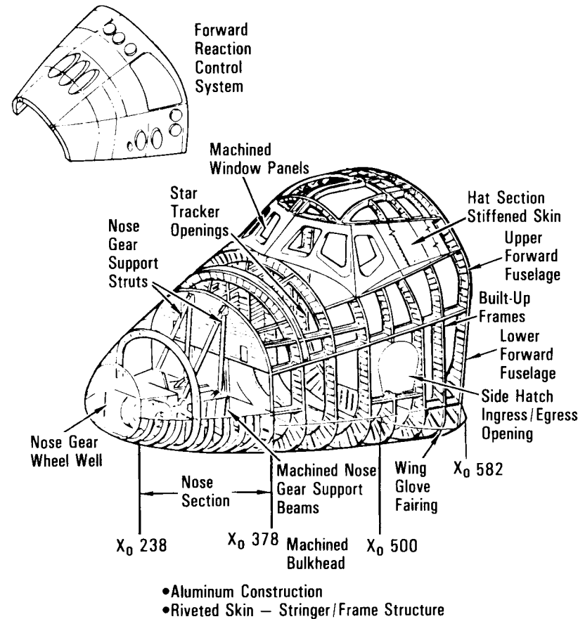
Forward Fuselage Structure
