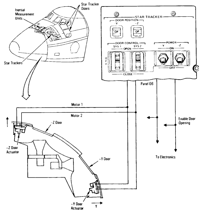
Star Tracker Doors
