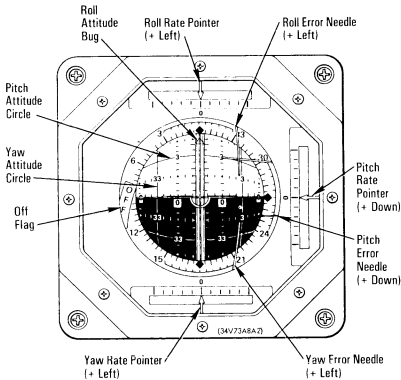
Attitude Director Indicator
