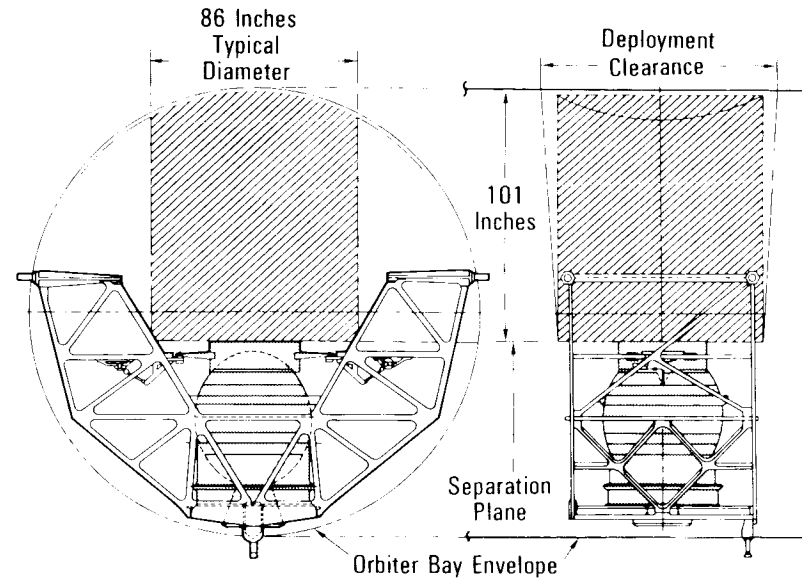
PAM-D Orbiter Vertical Installation
