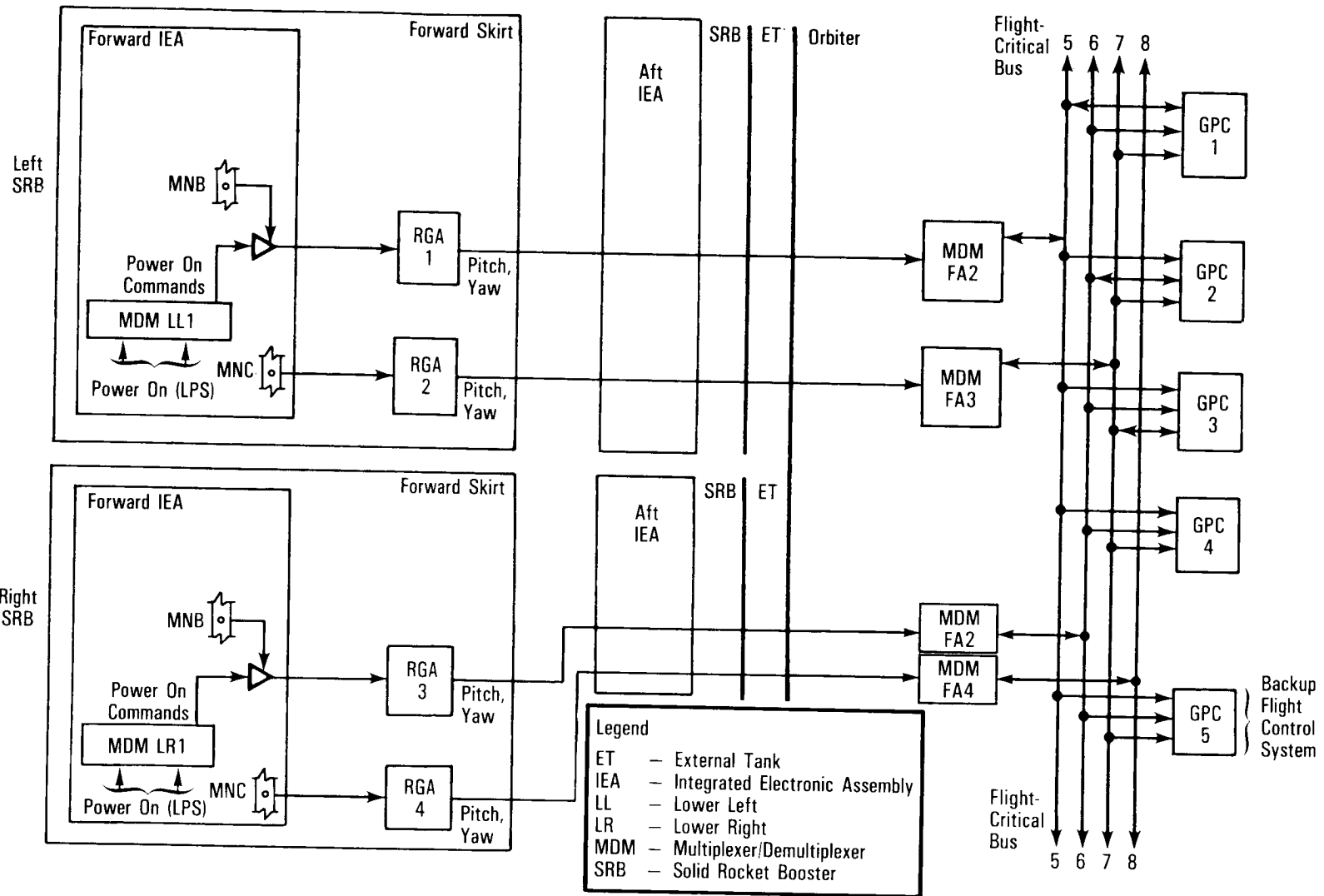
SRB Rate Gyro Assembly
