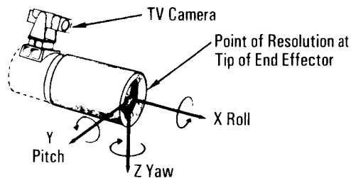
End Effector Operating System
