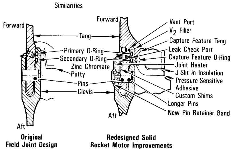
Field Joint Comparison
