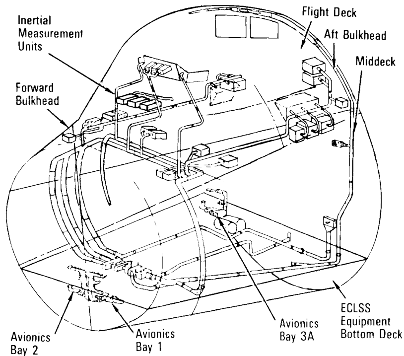
Cabin Air (IMU Loop Not Shown)
