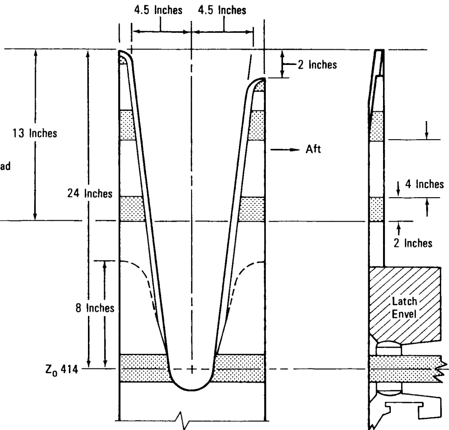
Orbiter Active Latch Guide
