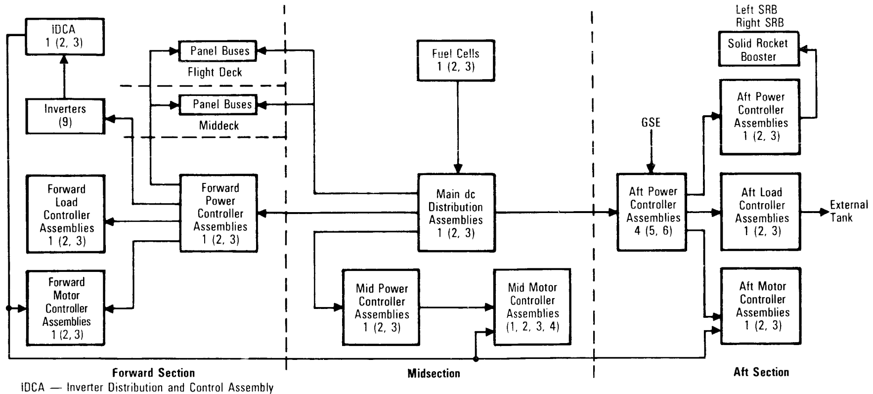
Electrical Power Distribution Block Diagram
