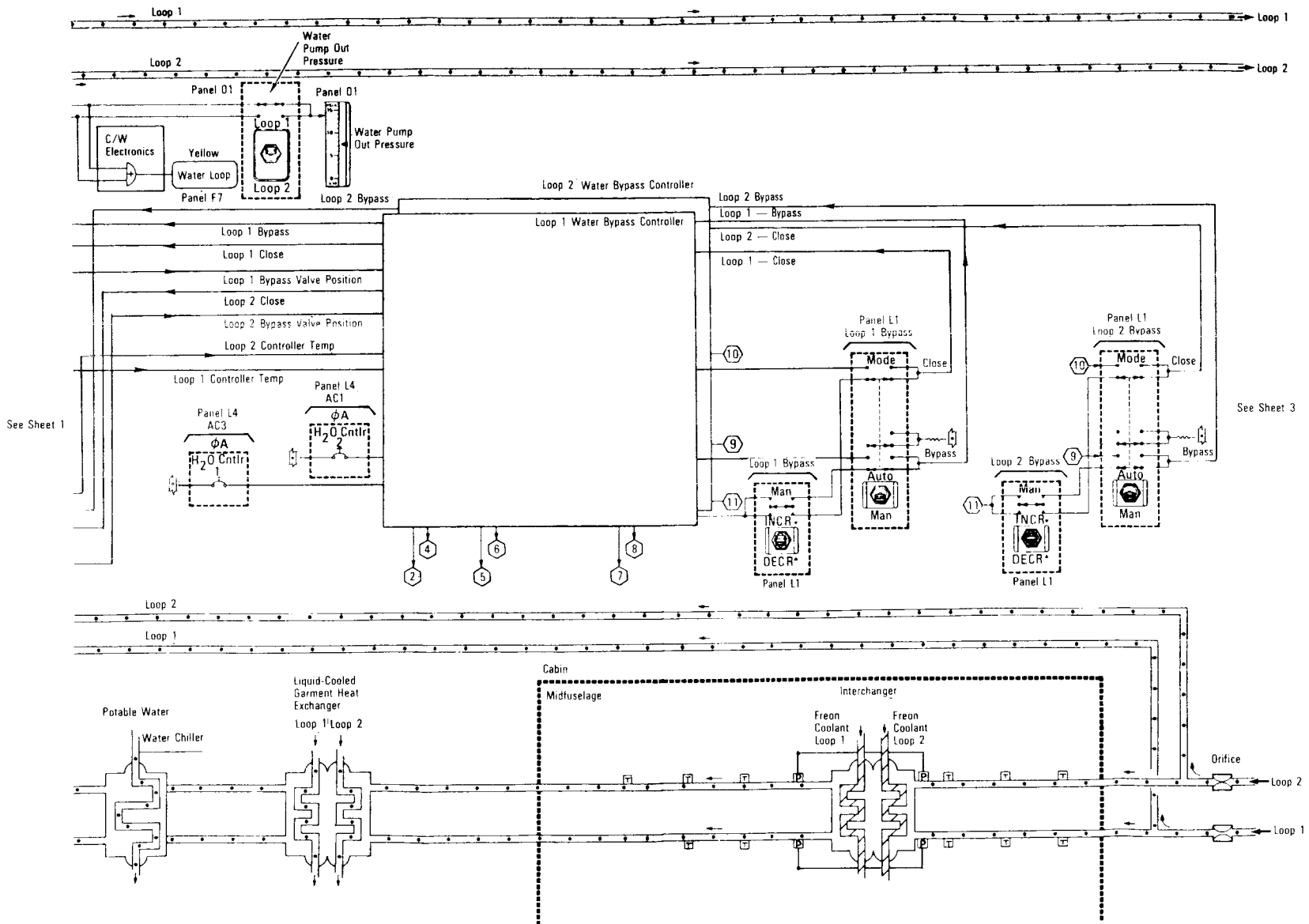
Water Coolant Loops (Sheet 2 of 3)
