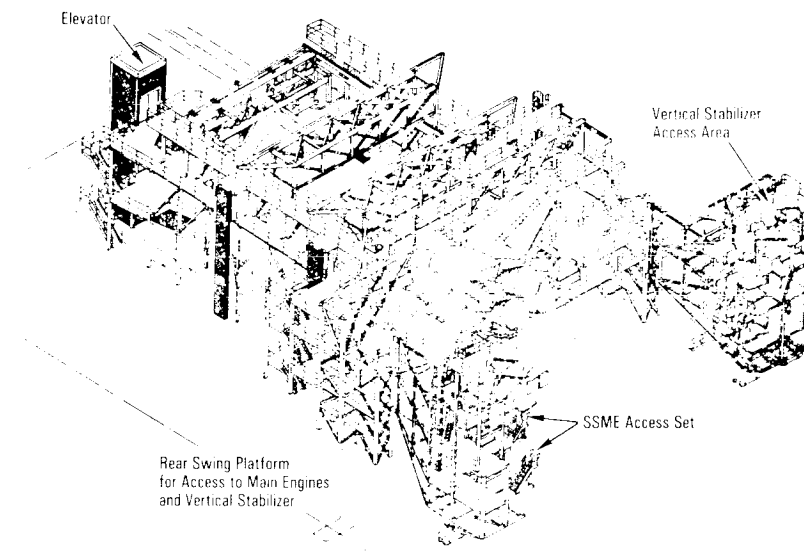
Orbiter Processing Facility Access Platforms, Facility Rear View
