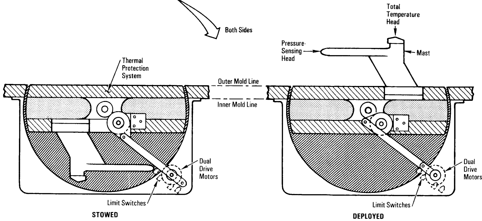
Air Data Probe Assembly
