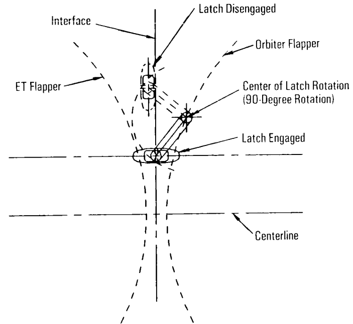
Orbiter / External Tank 17-Inch Disconnect Latch Positions, Engaged and Disengaged
