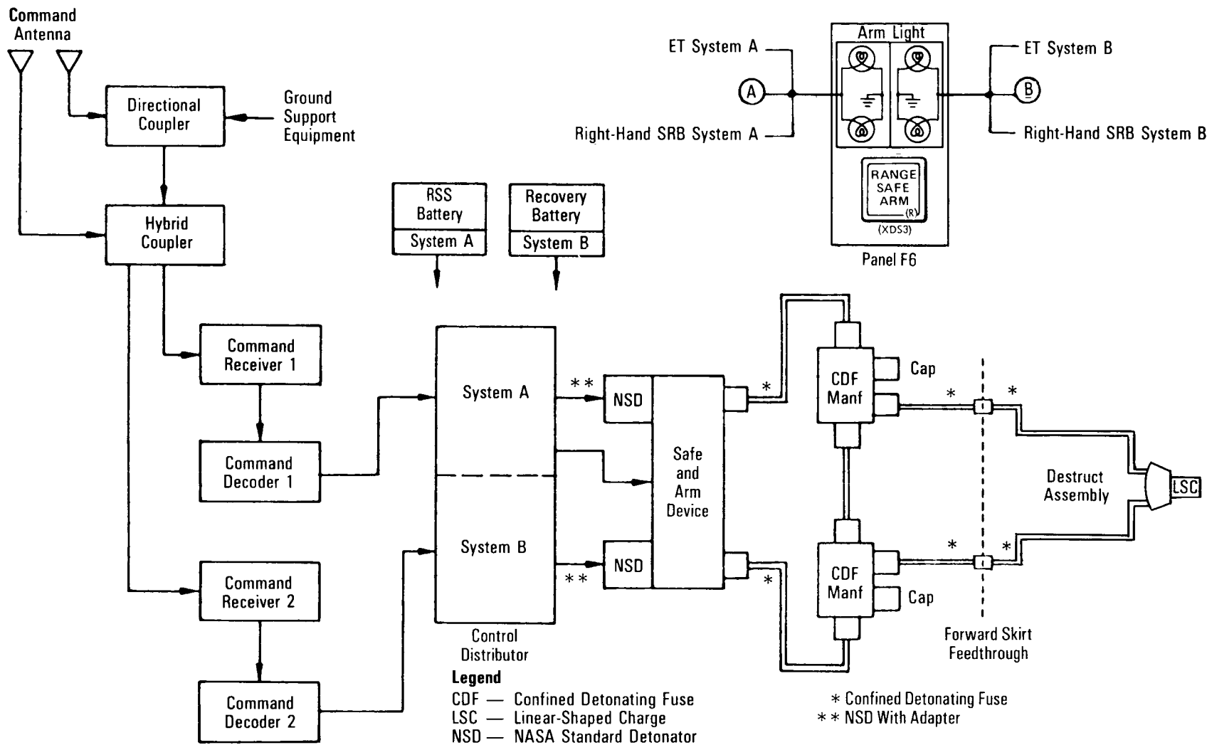
SRB Range Safety System
