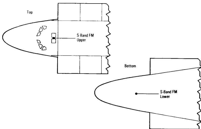
S-Band Frequency Modulation System Antenna Locations
