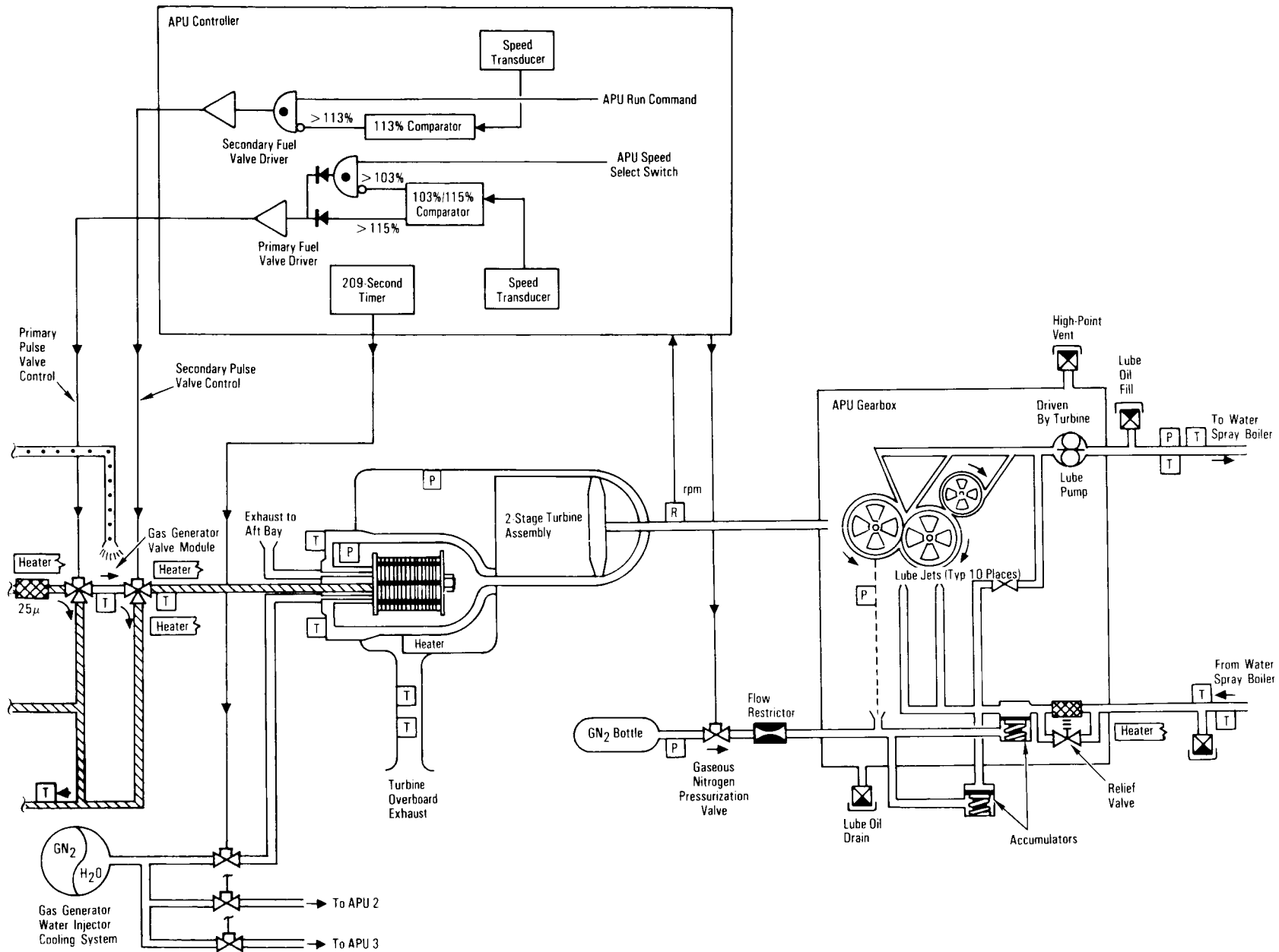
Auxiliary Power Unit System 1 and APU Fuel System Schematic
