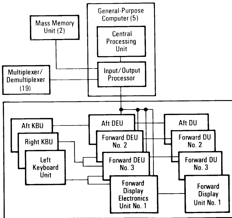
Data Processing System Hardware
