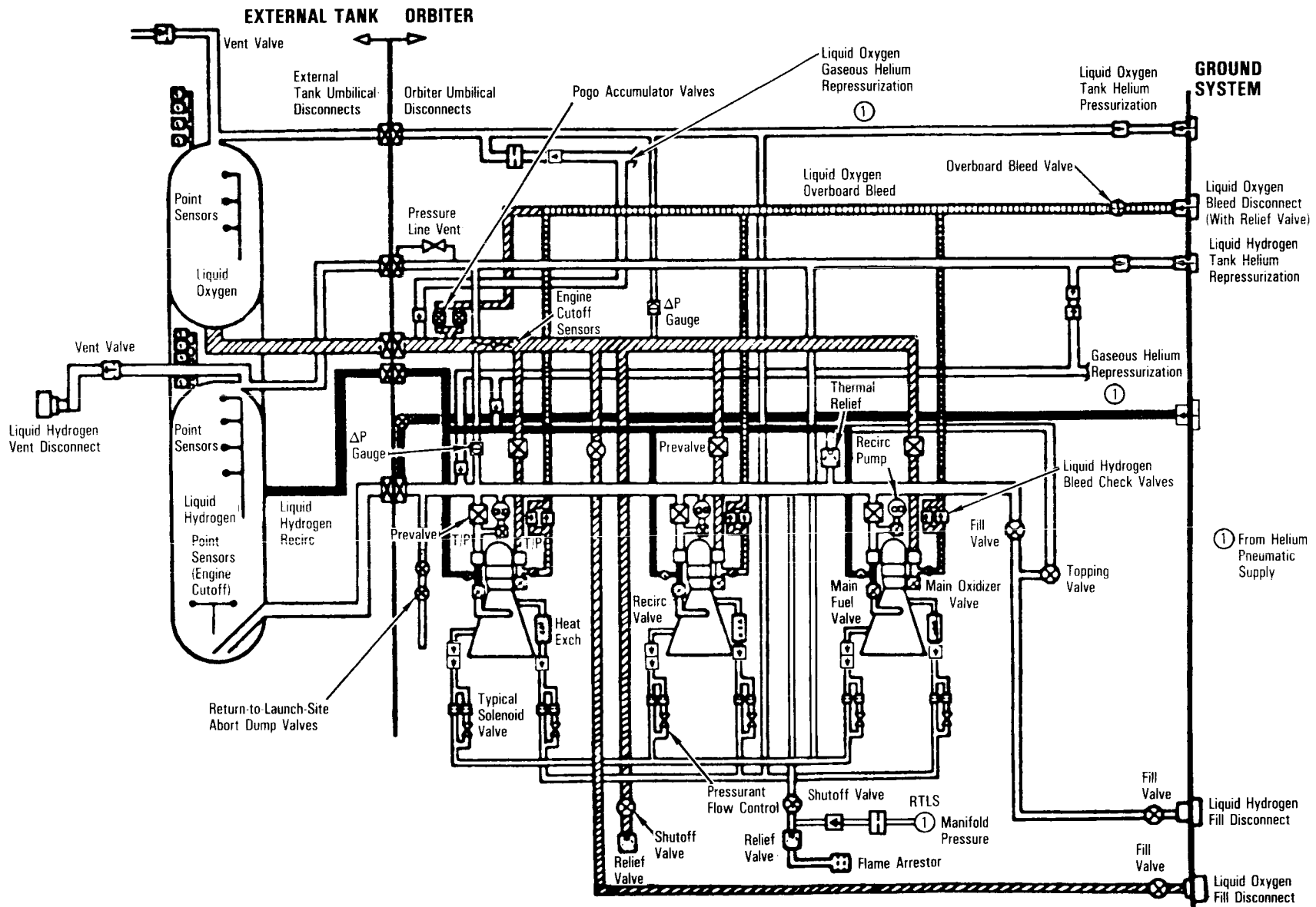
Main Propulsion System Fluid System
