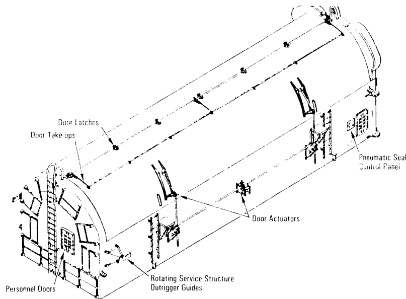
Payload Canister
