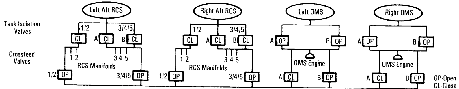
Orbital Maneuvering System Crossfeed to Aft Reaction Control System
