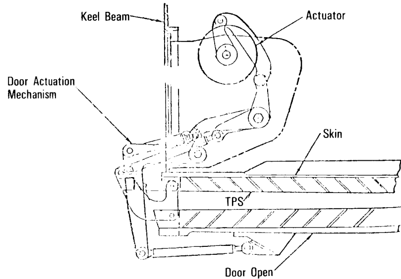
Orbiter/External Tank Umbilical Doors—Hinge/Actuation System
