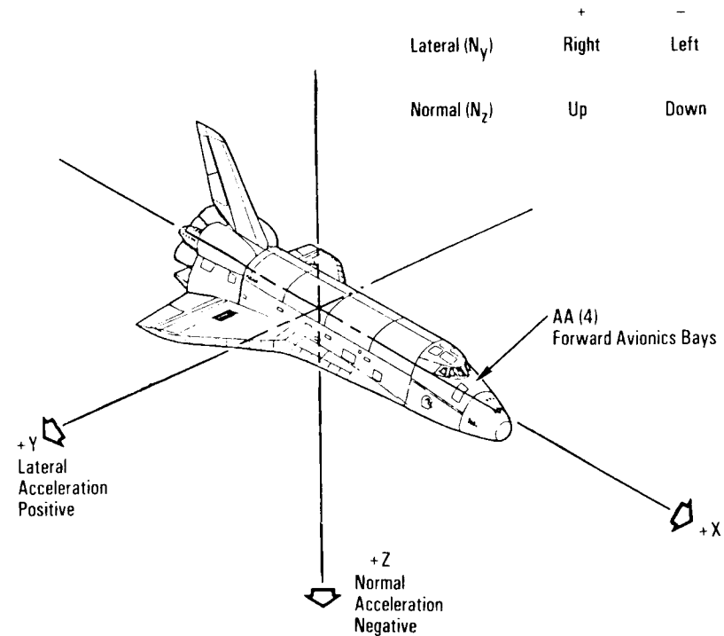
Accelerometer Assembly Location and Acceleration Axes
