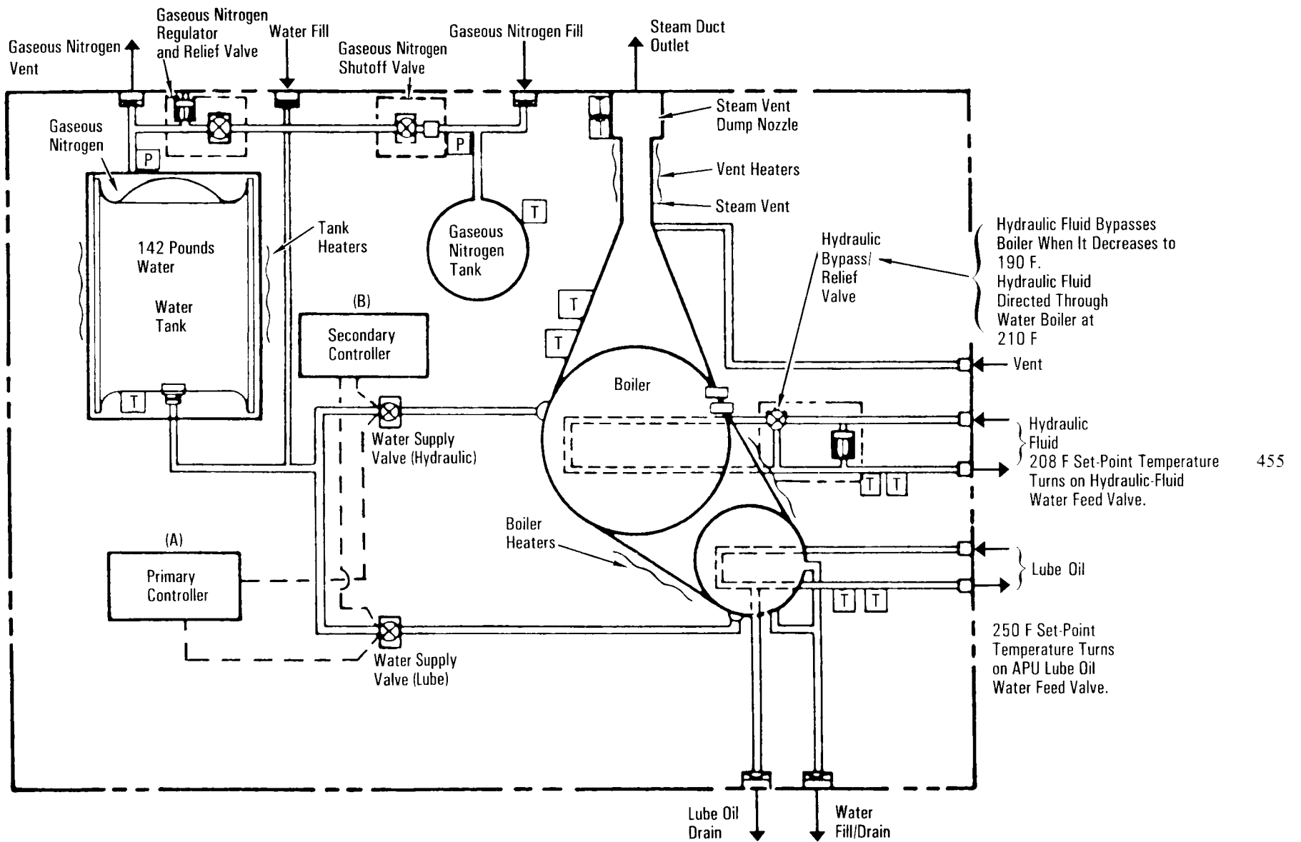
Water Spray Boiler (One of Three)
