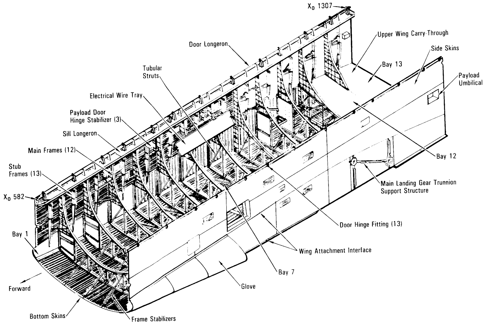
Midfuselage Structure
