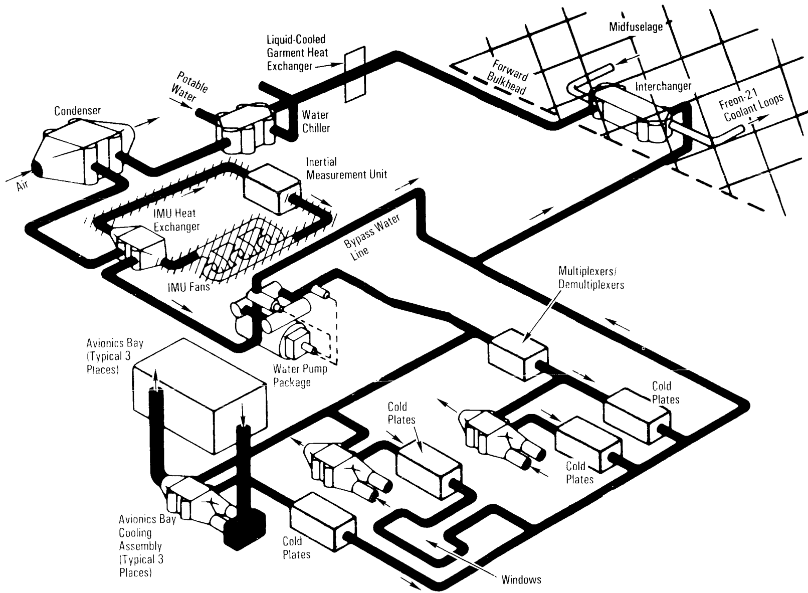
Water Coolant Loops
