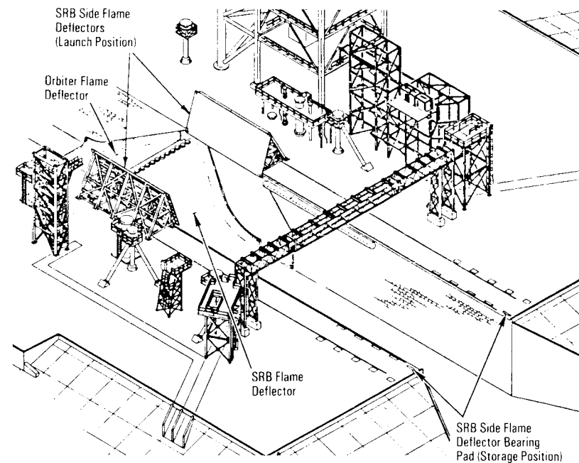
Orbiter/Solid Rocket Booster Flame Deflectors
