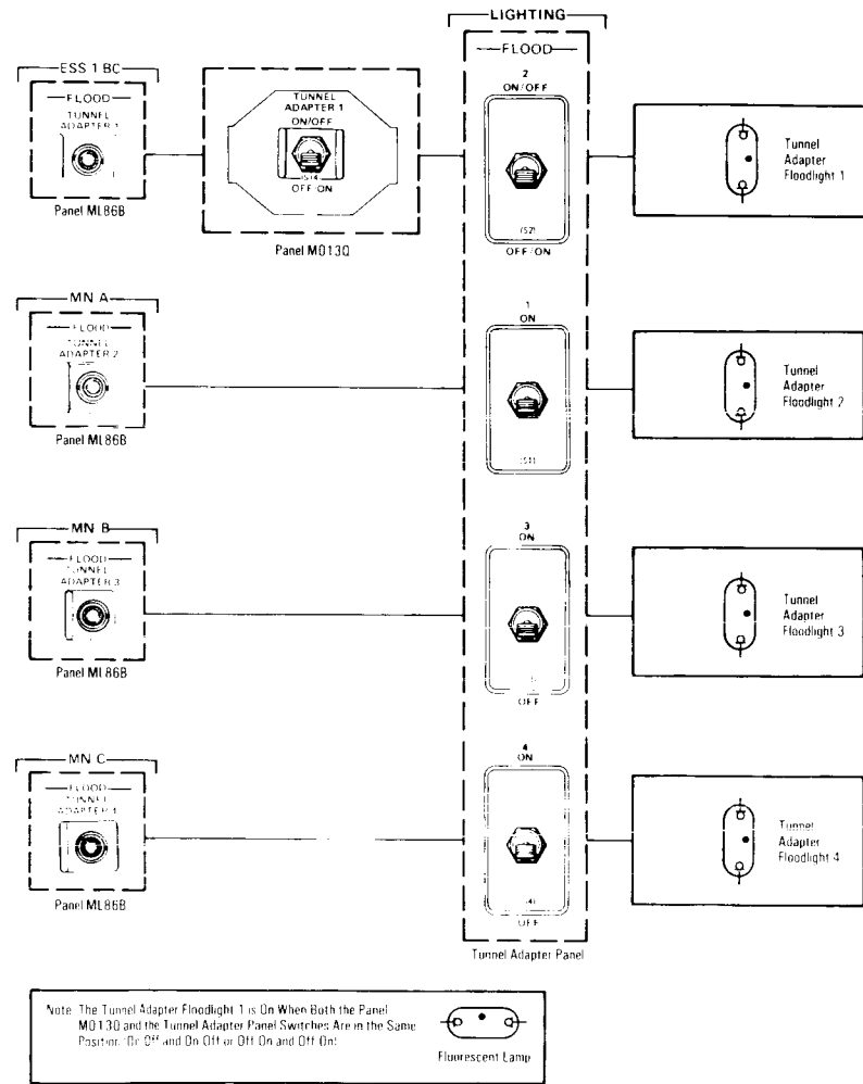
Tunnel Adapter Floodlights, If Adapter Is Installed
