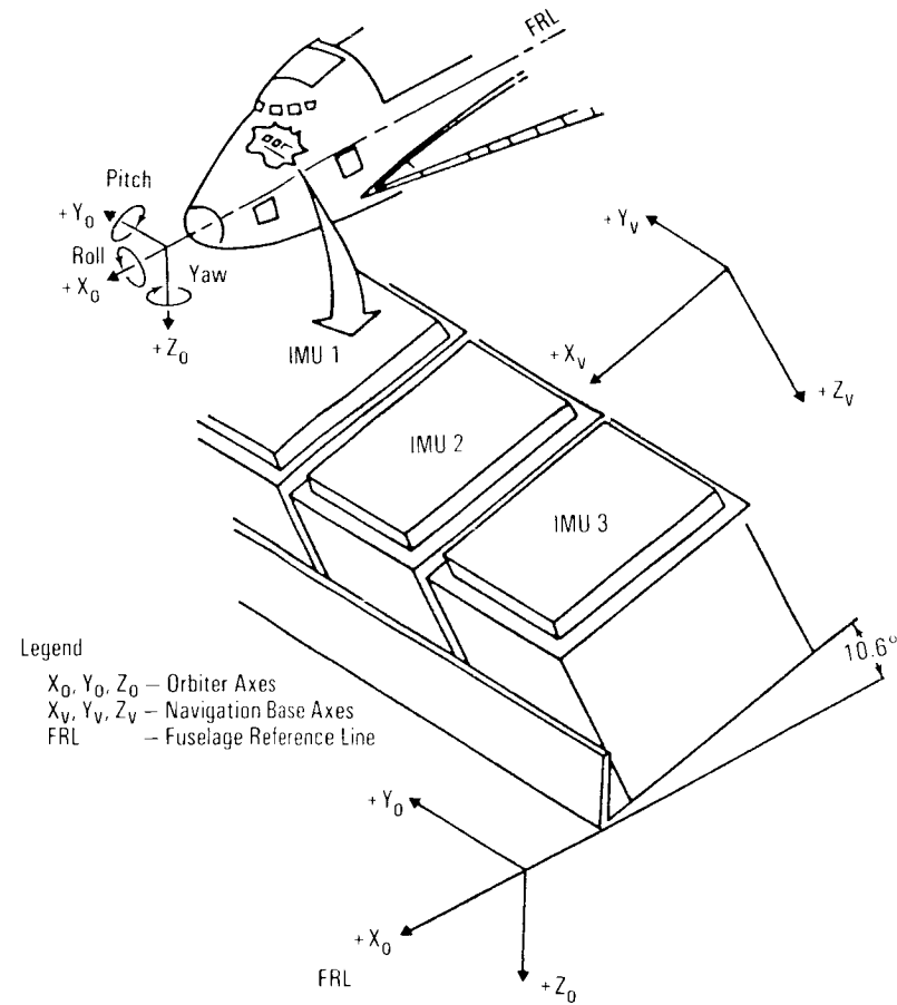
Inertial Measurement Units
