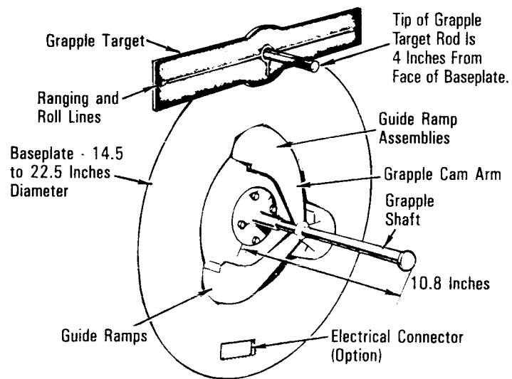
Grapple Fixture/Target Assembly
