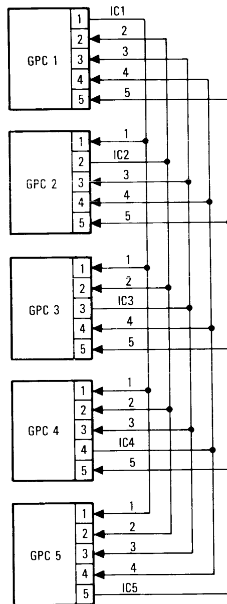
Intercomputer Communication Data Buses
