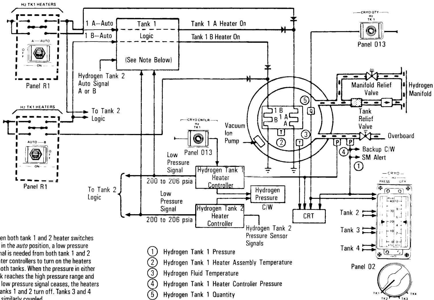
Power Reactant Storage and Distribution—Hydrogen Tank 1
