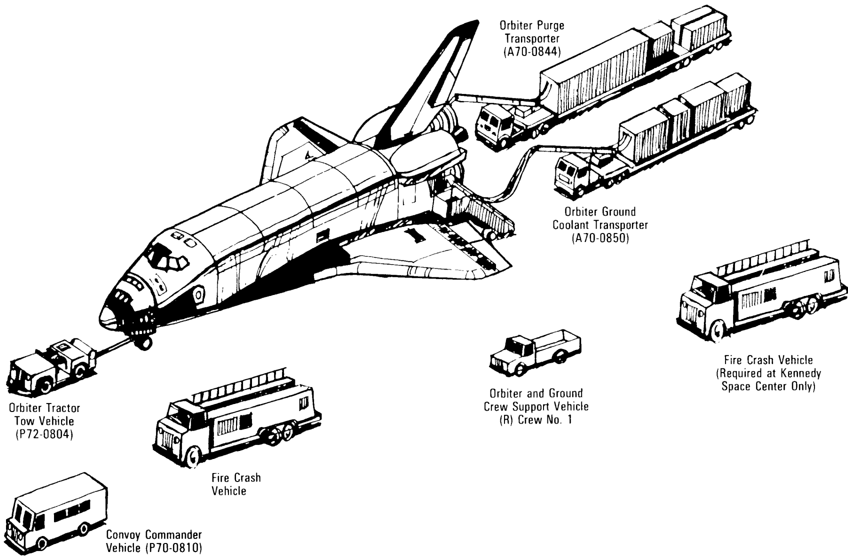
Typical Convoy Tow Configuration
