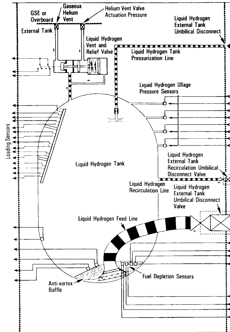
External Tank Schematic, Liquid Hydrogen Tank Detail
