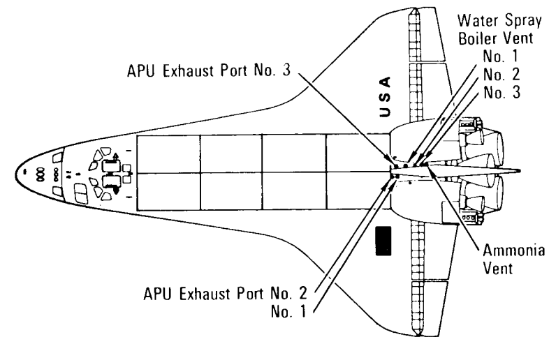
APU Exhaust and Water Spray Boiler Vent
