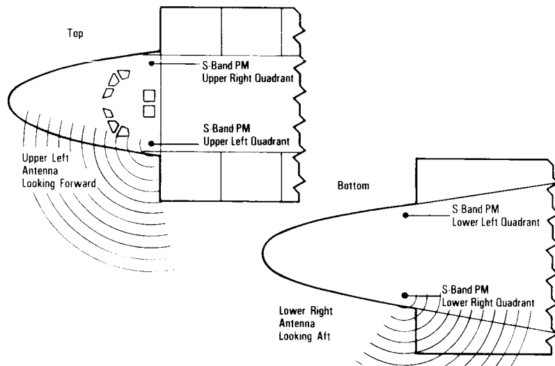
S-Band Phase Modulation System Antenna Locations
