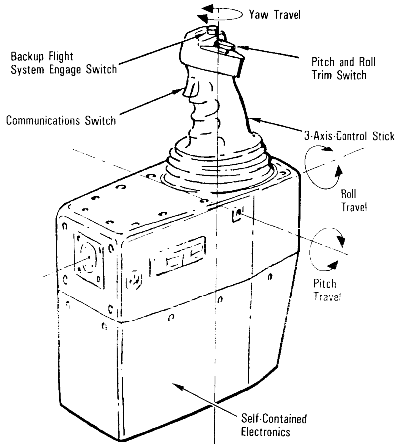
Rotational Hand Controller
