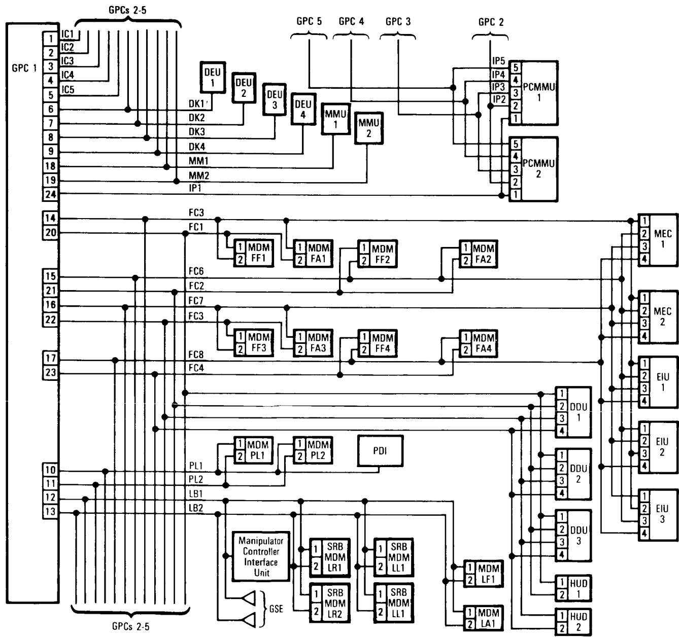
Computer Data Bus Network
