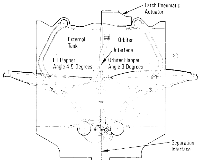
Orbiter/External Tank 17-Inch Disconnect With Latch Feature
