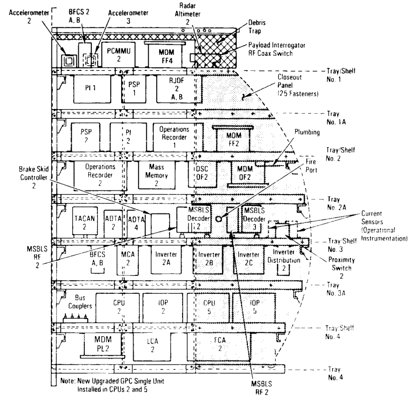
Component Locations—Bay 2
