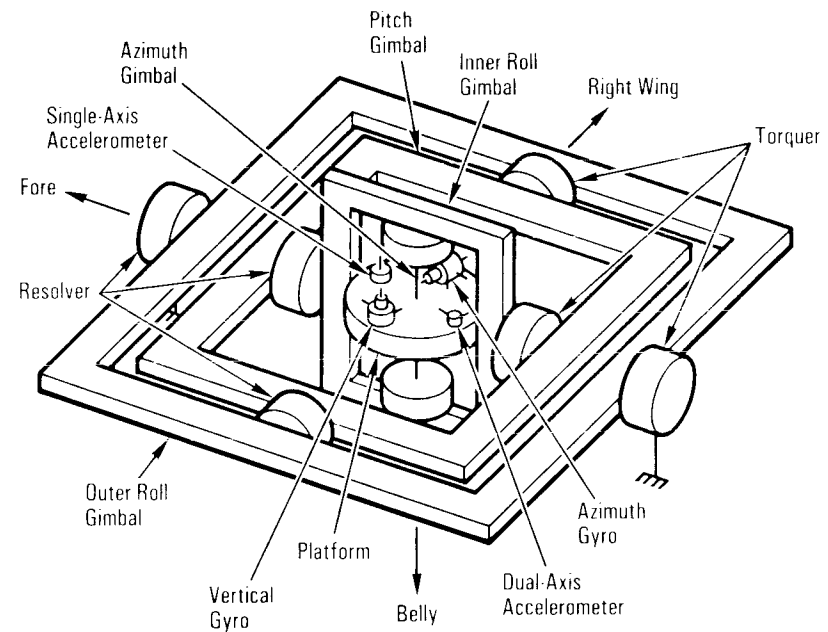
Inertial Measurement Unit Platform Assembly and Coordinate System
