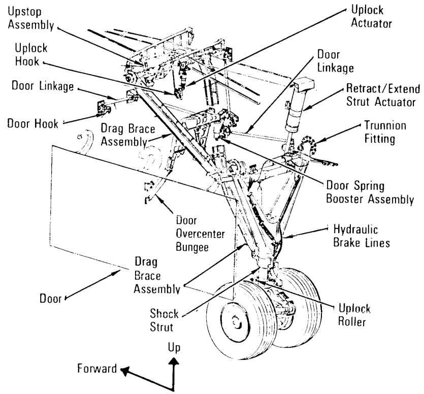
Main Landing Gear Deployed
