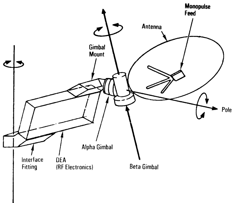
Ku-Band Deployed Assembly
