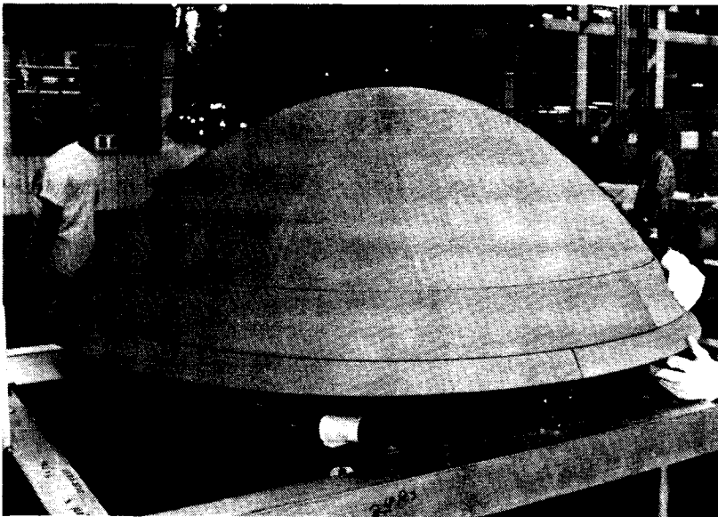
RCC Nose Cap
