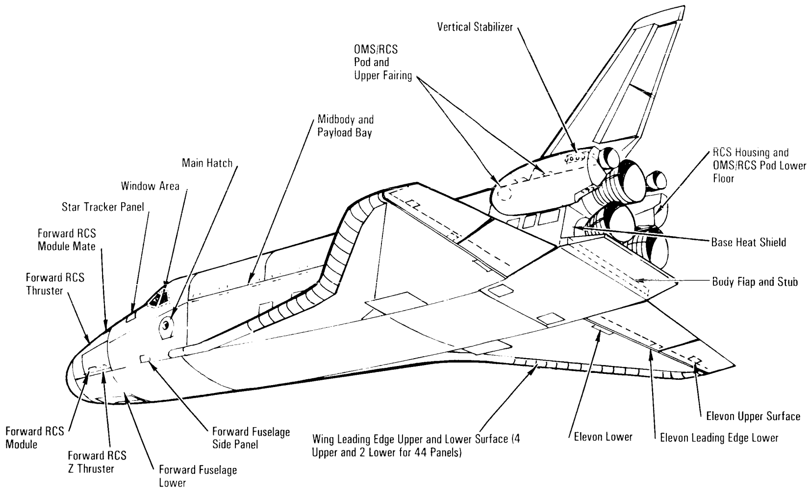
Fused Silica Insert and Plug Locations
