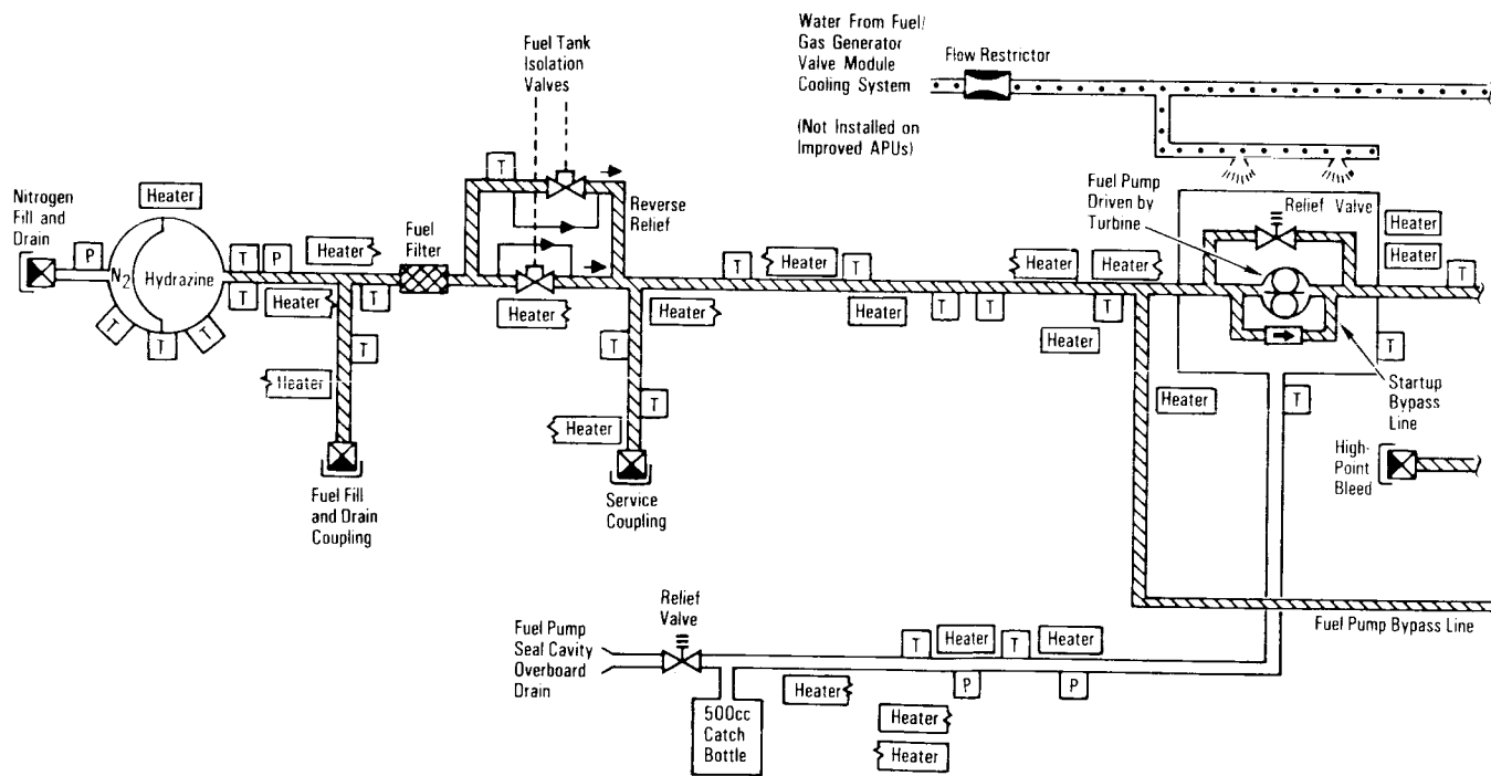
Auxiliary Power Unit System 1 and APU Fuel System Schematic
