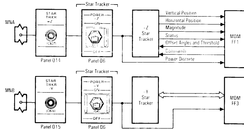
Power and Data Interfaces of the Star Trackers
