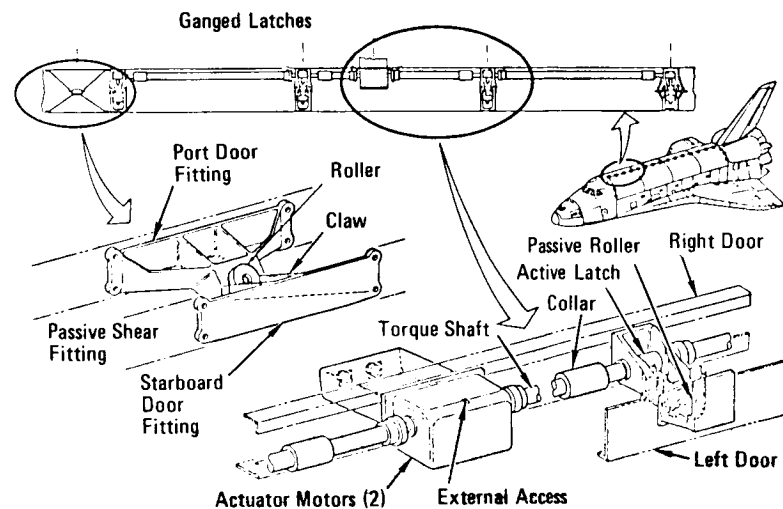
Payload Bay Door Upper Centerline Latch System
