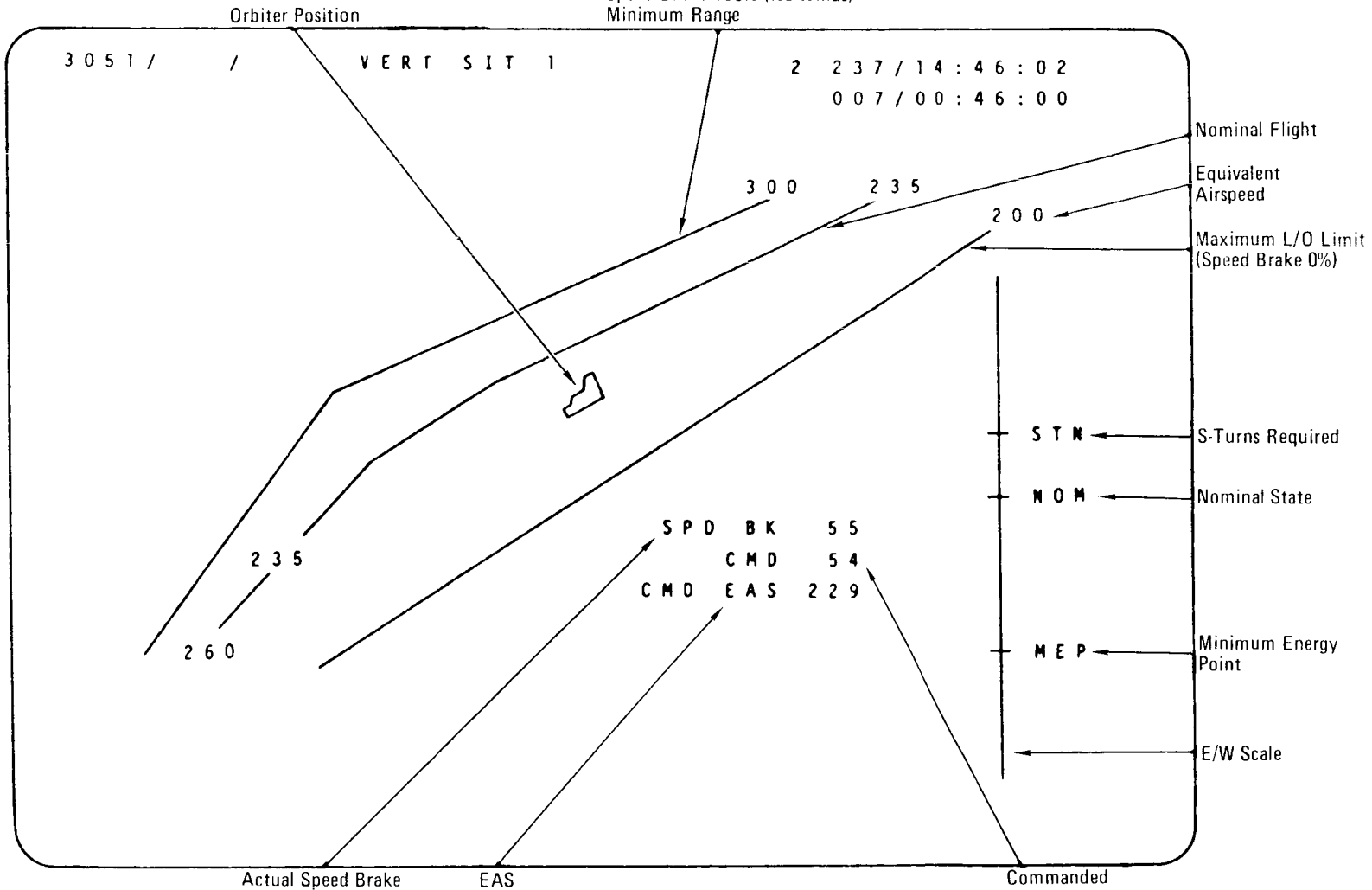
Vertical Situation Display
