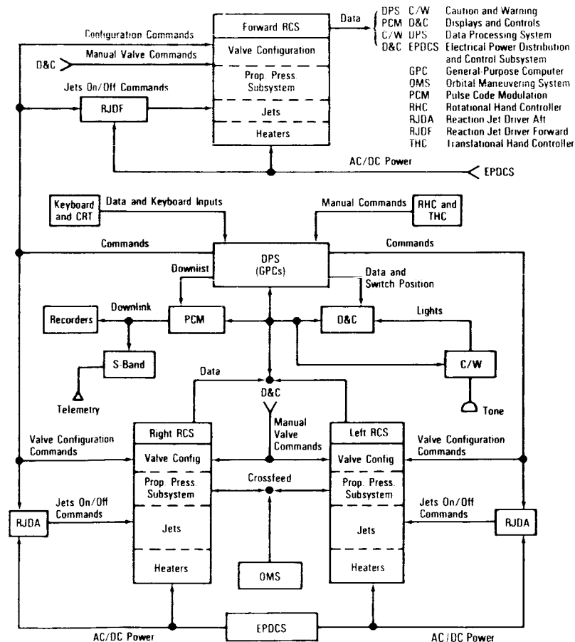
Reaction Control System Overview
