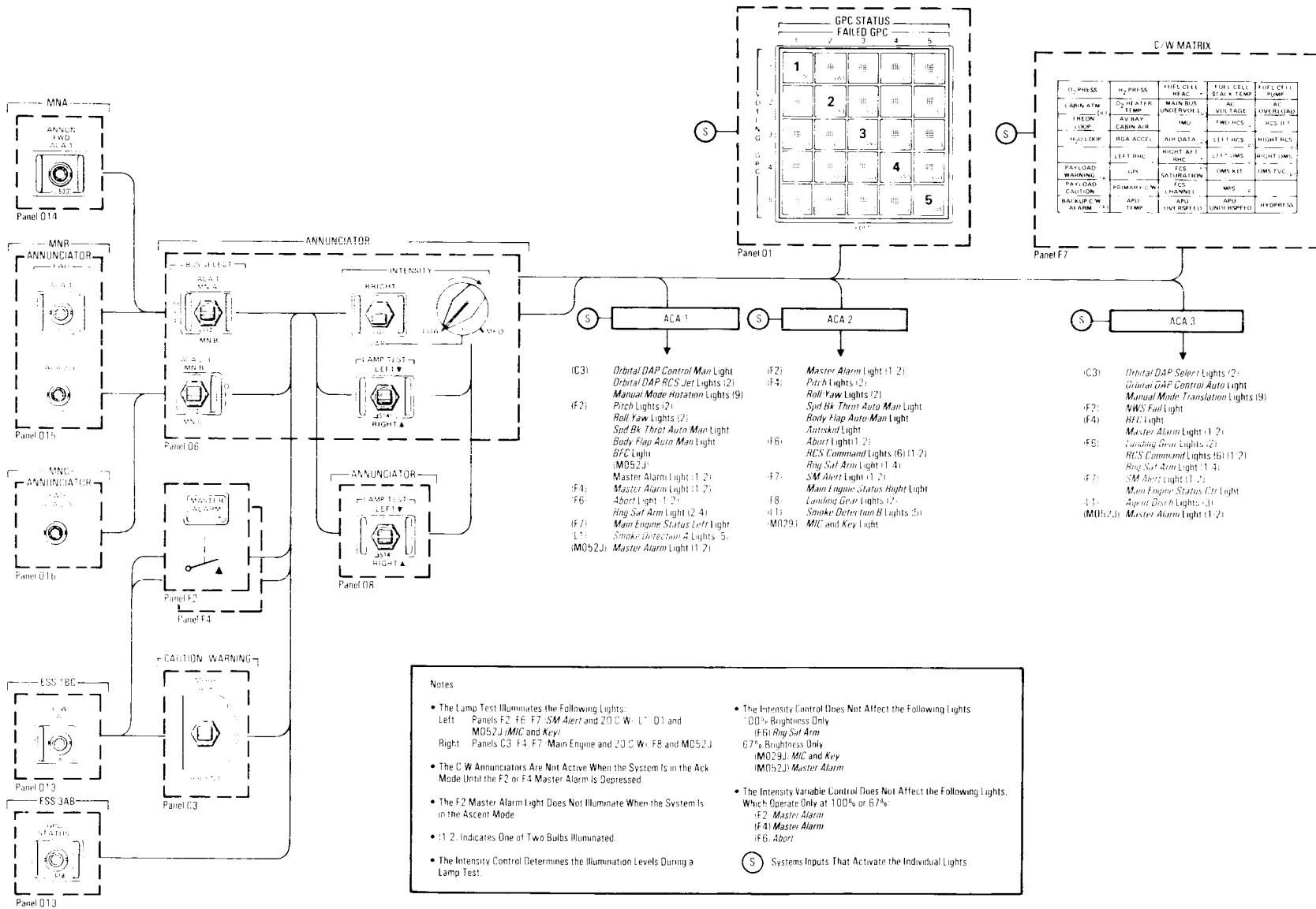
Forward Flight Deck Annunciator Light Controls
