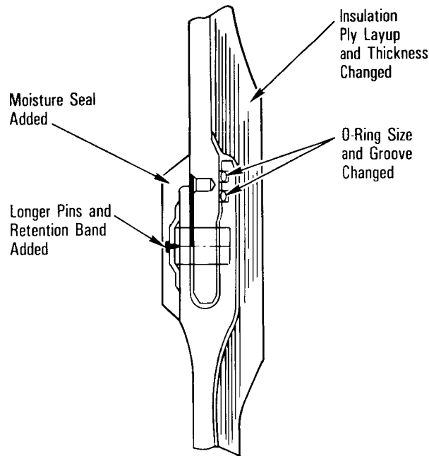
Redesigned Factory Joint
