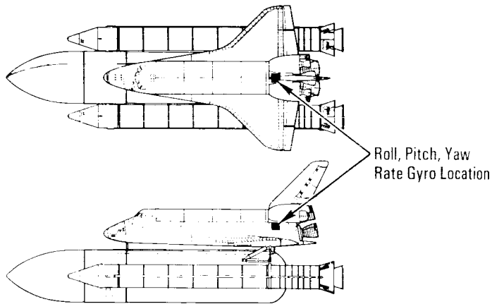
Orbiter Rate Gyro Locations
