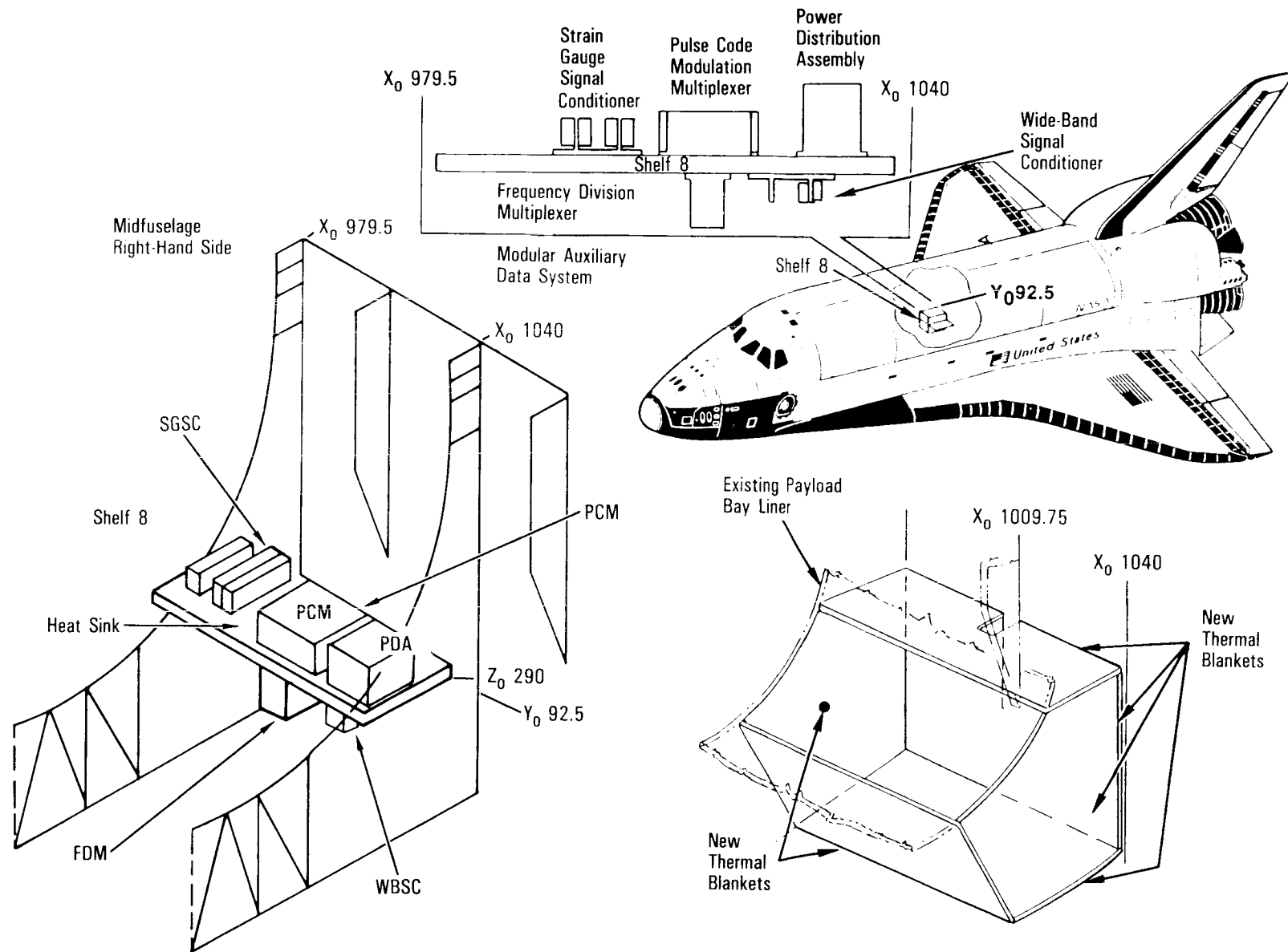
Modular Auxiliary Data System Equipment Location in Midfuselage, All Orbiters
