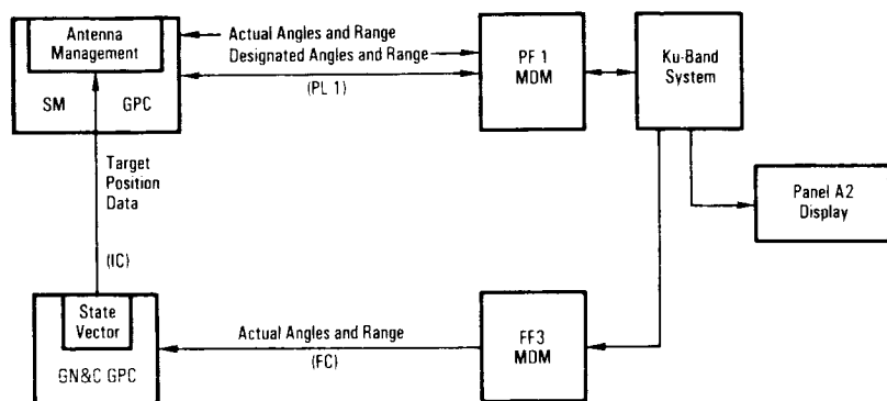
Ku-Band Designated Steering and Radar Data Interface
