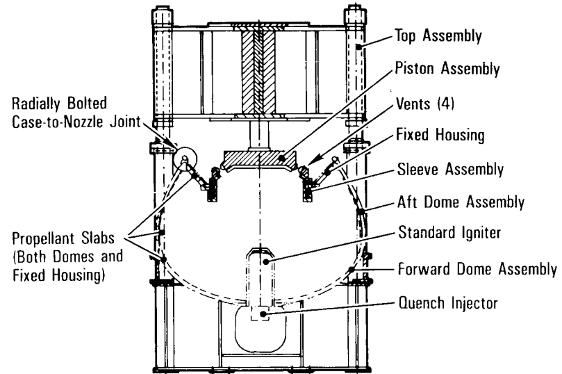
Nozzle Joint Environment Simulator Configuration
