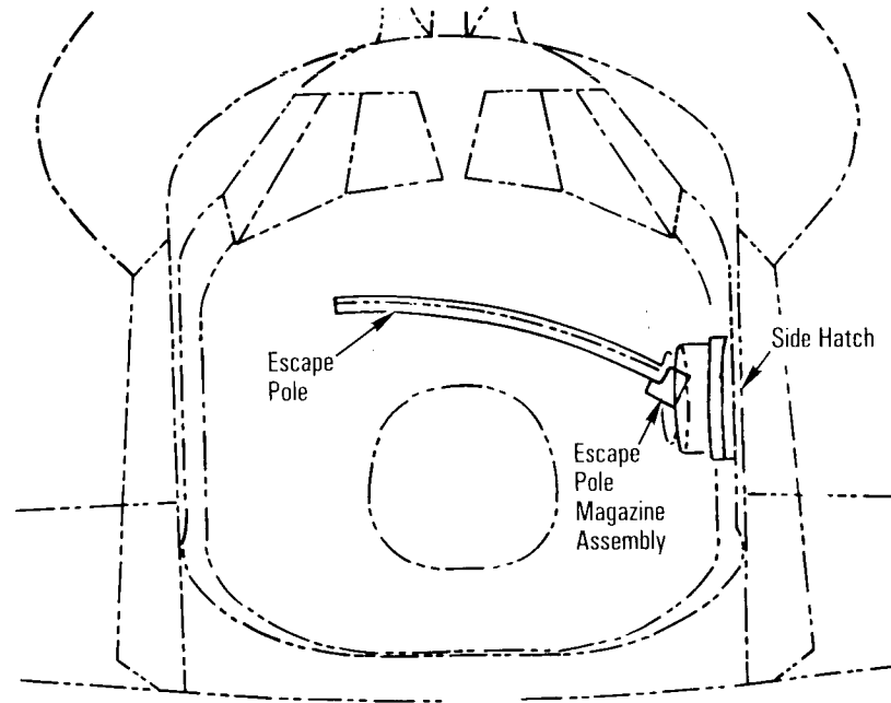
Escape Pole Ascent/Descent Position, Middeck Side View
