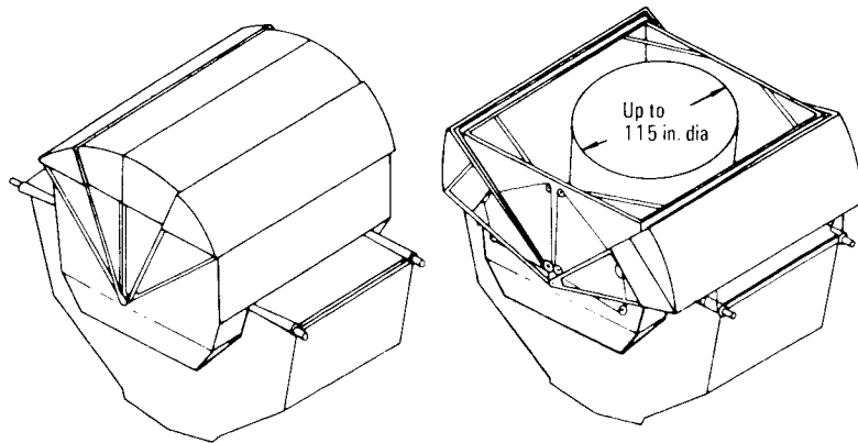
PAM-DII Sunshield
