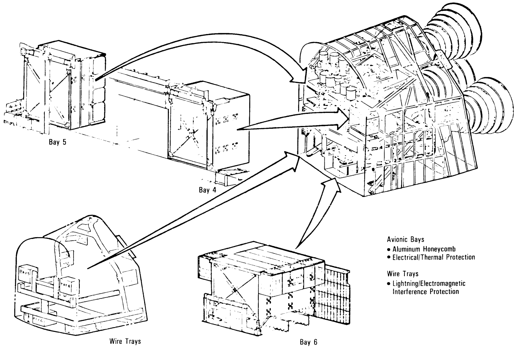
Aft Fuselage Avionics Provisions
