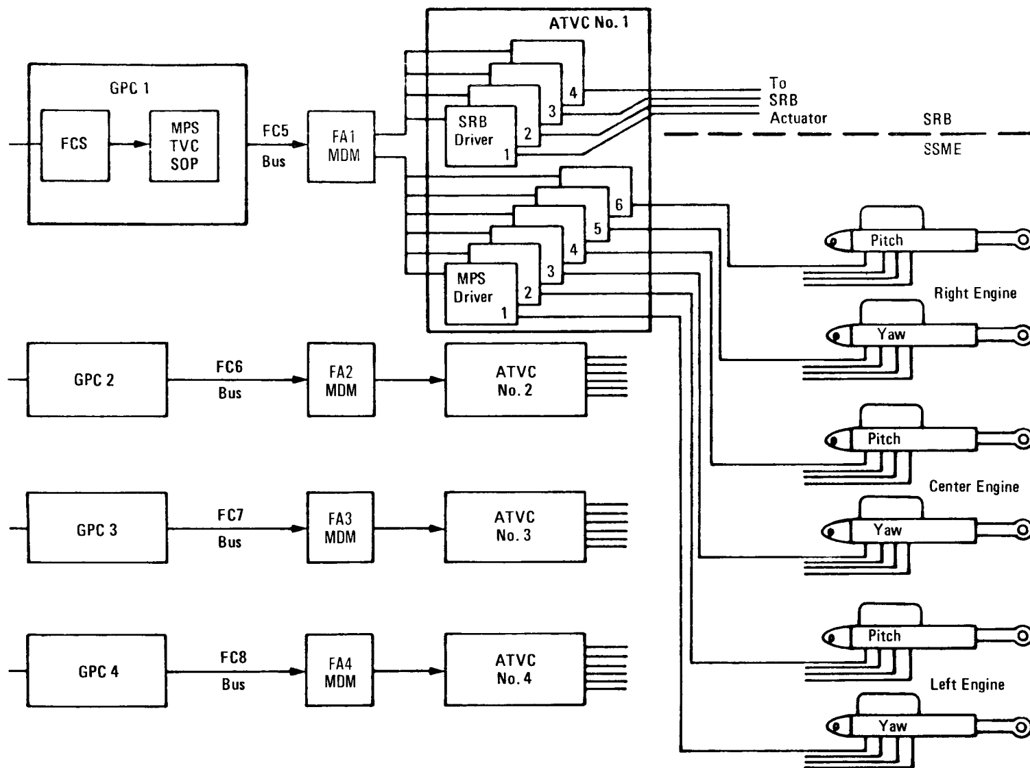
Command Flow Overview
