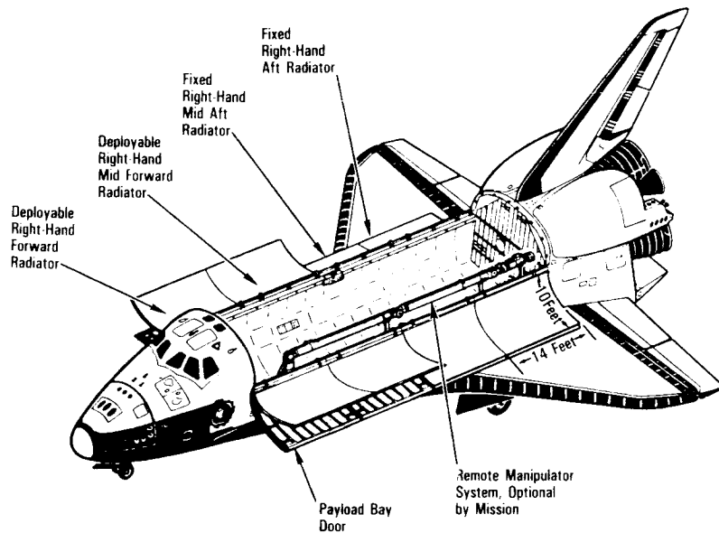
Payload Bay Radiators
