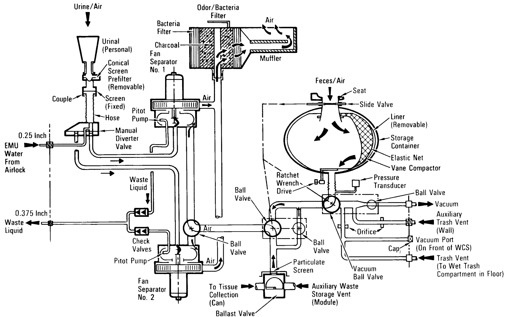
Waste Collection System Urine/Feces Collection Mode, Handle Up
