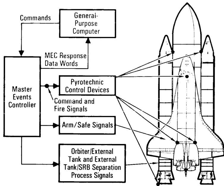
Master Events Controller
