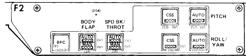
Flight Control Mode Push Button Light Indicators Panel F2 (Panel F4 Identical)
