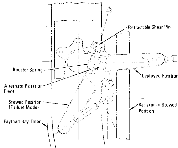
Payload Bay Door Deployable Radiator Mechanism Disconnect Features
