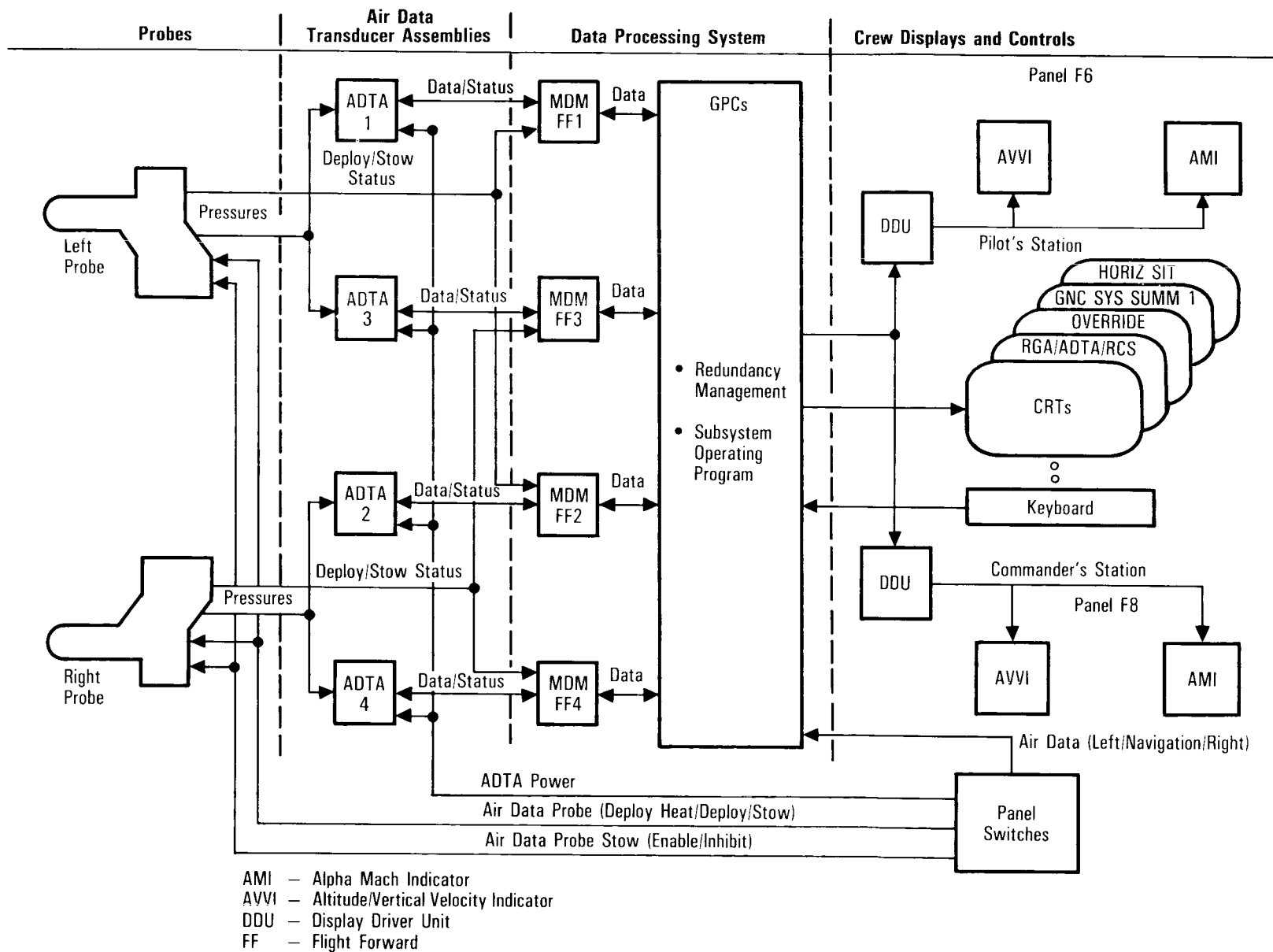
Air Data System Functional Block Diagram
