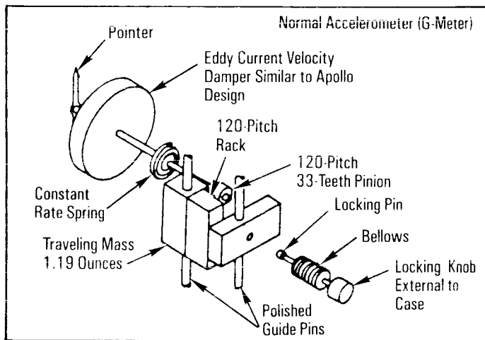
G-Meter Design
