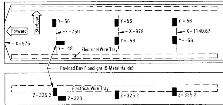
Payload Bay Forward/Mid/Aft Floodlights
