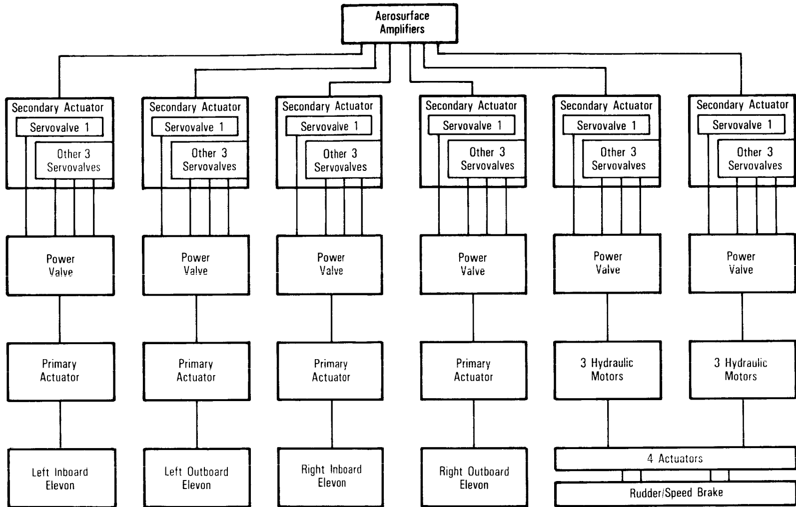
Aerosurface Amplifiers
