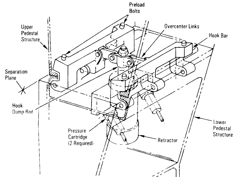
RMS Mechanical Separation System
