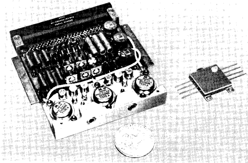
Hybrid Load Controller
