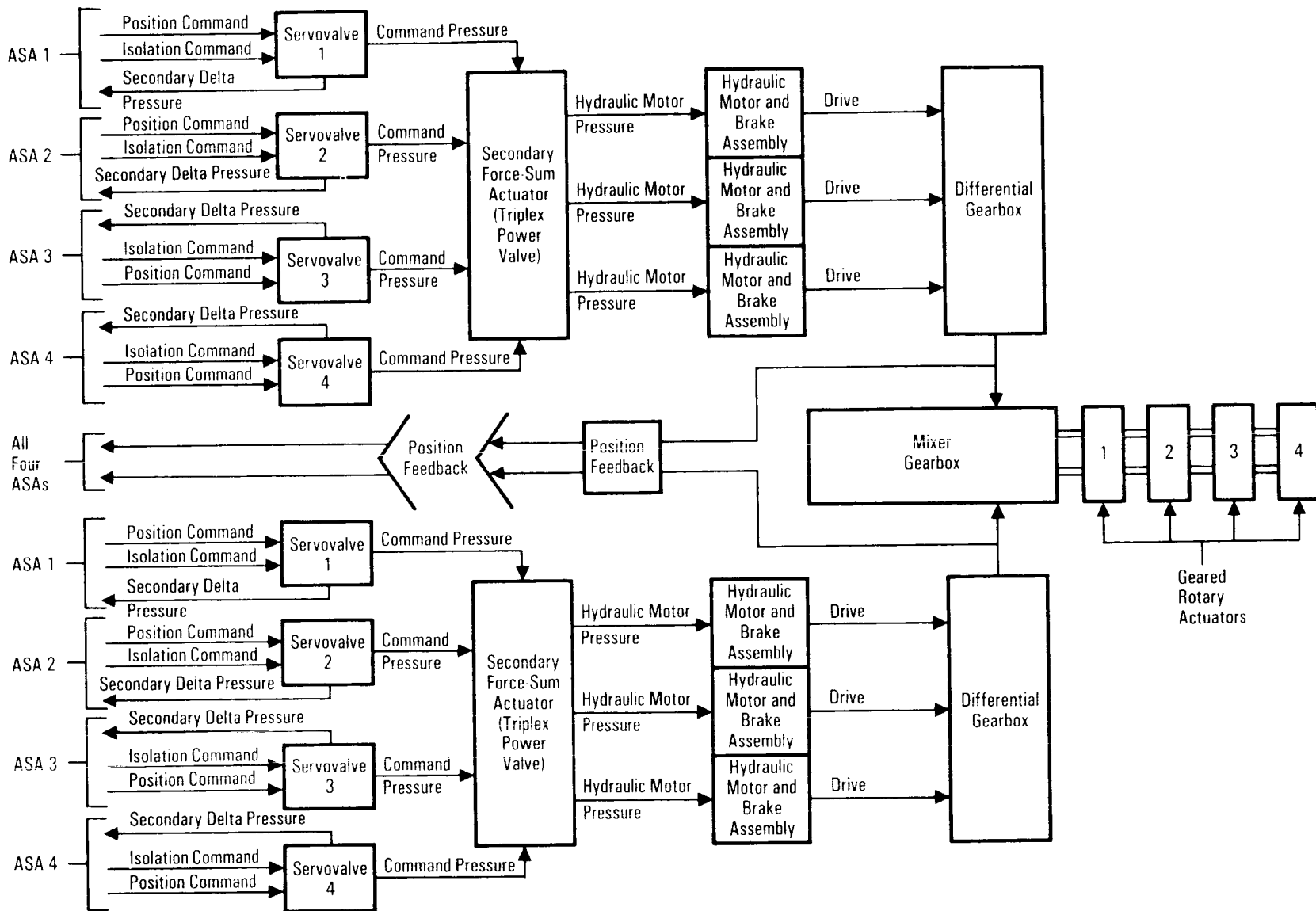
Rudder/Speed Brake Actuation Subsystem
