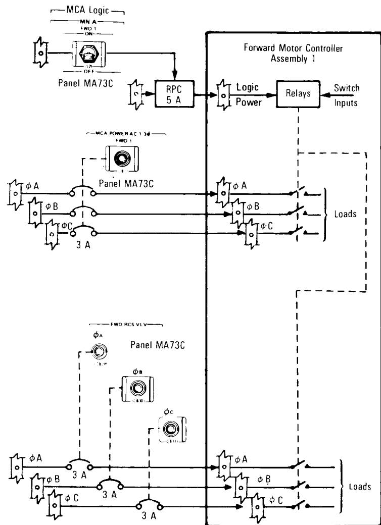
Forward Motor Controller Assembly
