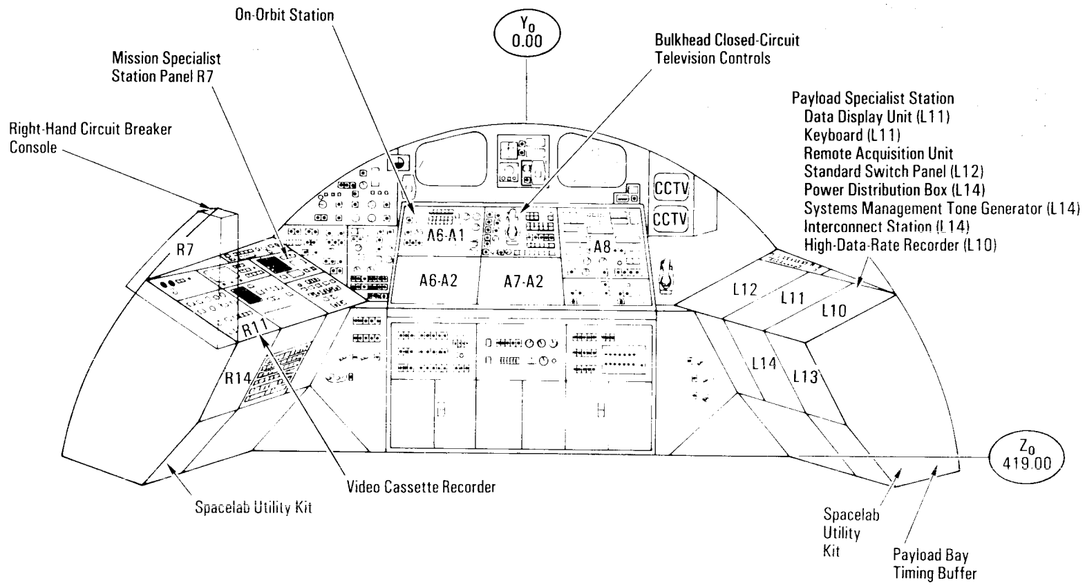
Example of a Spacelab Pressurized Module Aft Flight Deck Panel Configuration
