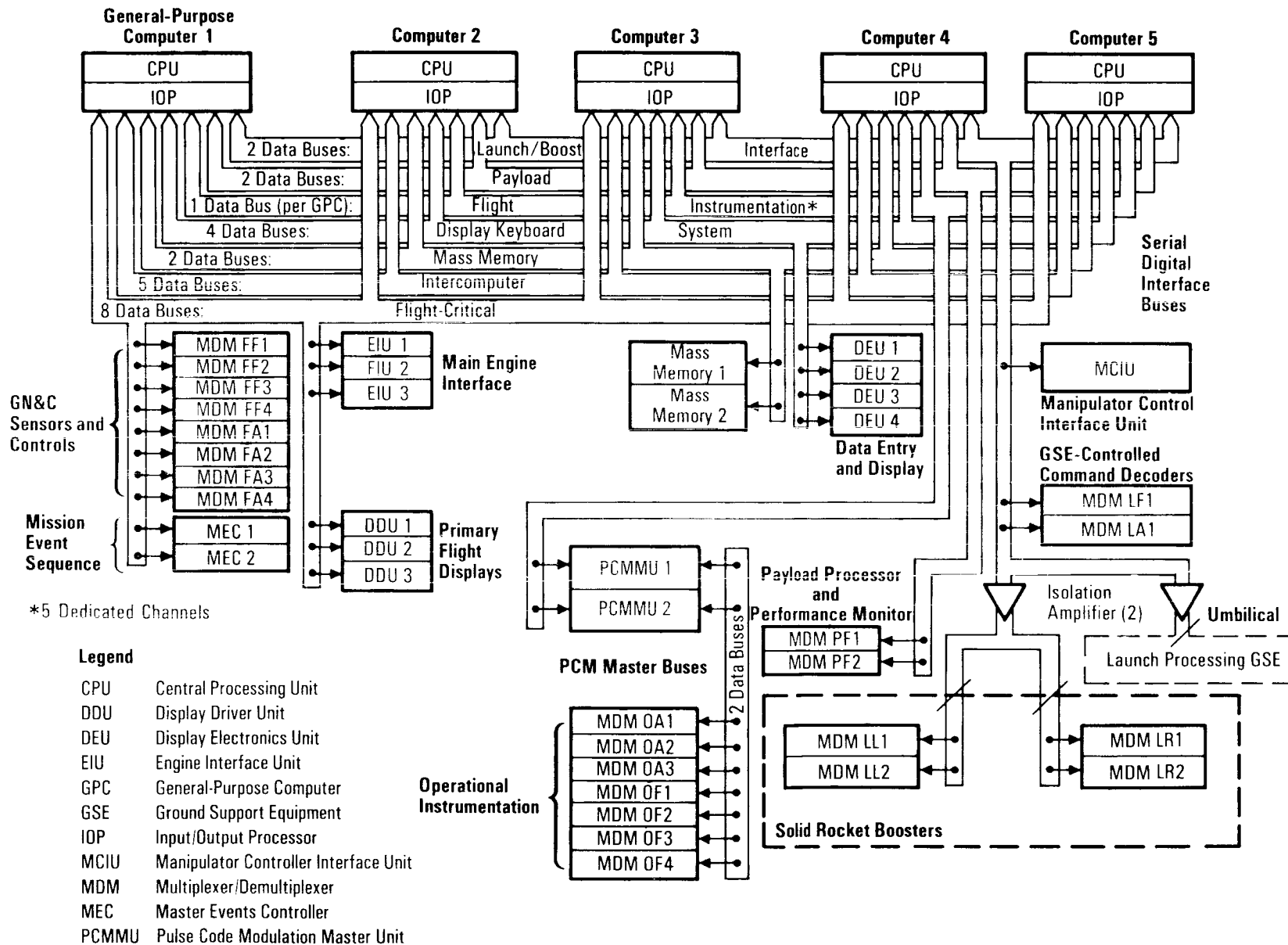
Data Processing System
