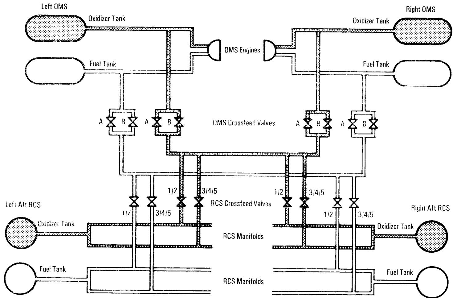
Orbital Maneuvering System Crossfeed and Crossfeed to Aft Reaction Control System
