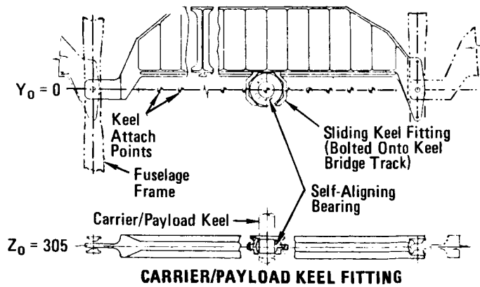
Standard Attach Fittings for Payloads
