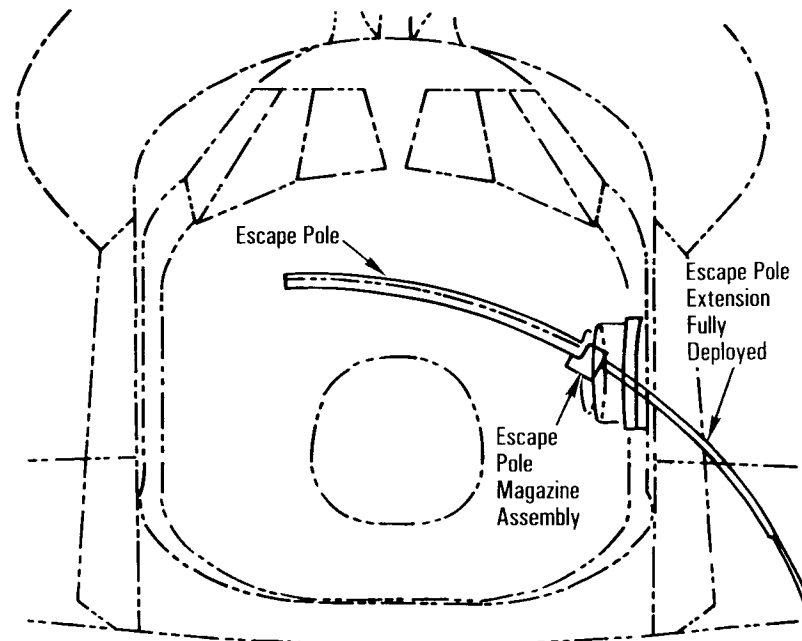
Side View of Escape Pole Fully Deployed Through Side Hatch
