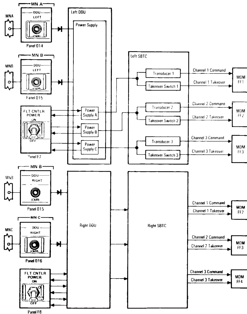
Speed Brake/Thrust Controller Power and Data Interfaces
