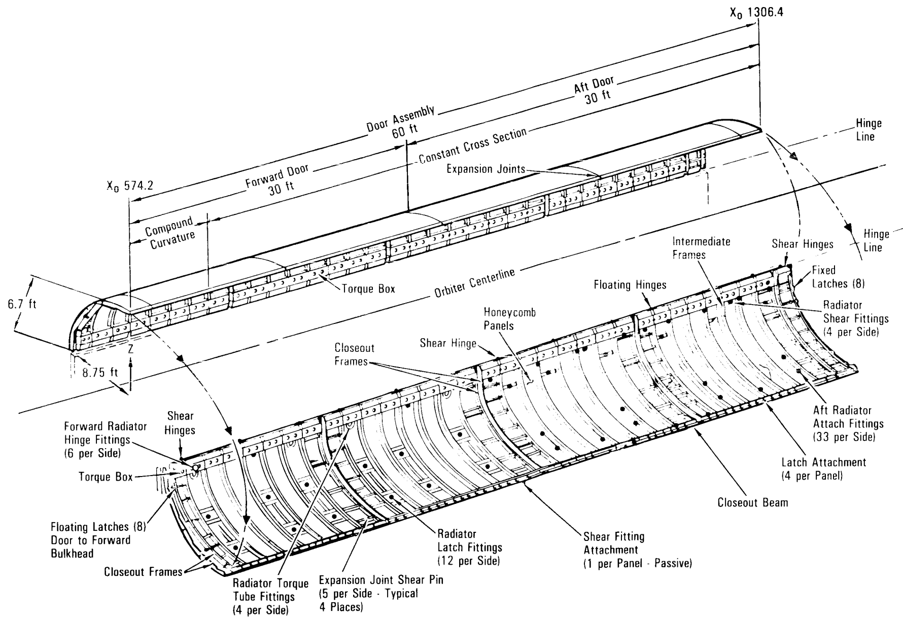
Payload Bay Doors
