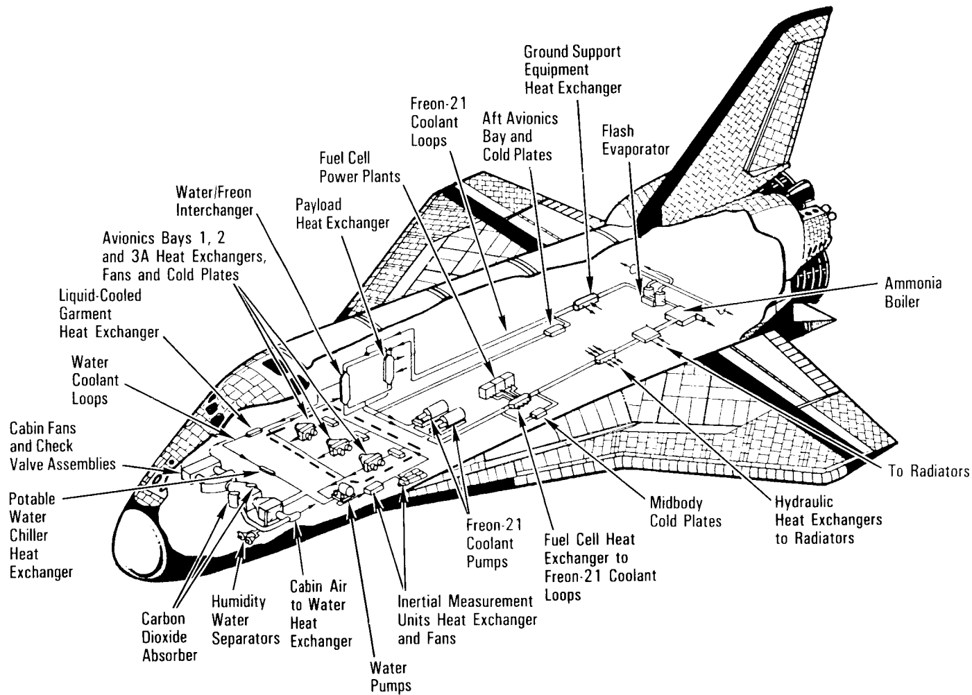
Environmental Control and Life Support System
