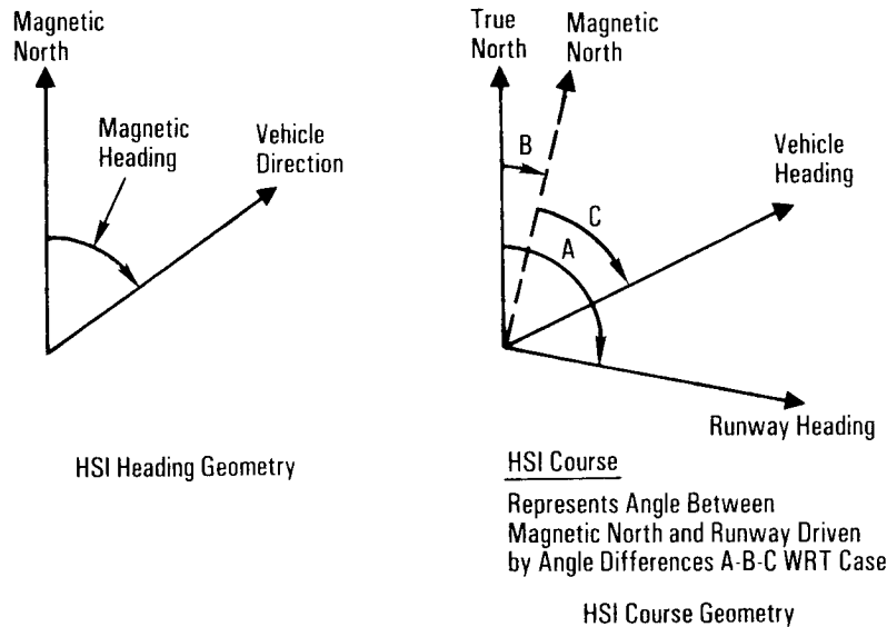
Horizontal Situation Indicator Geometries
