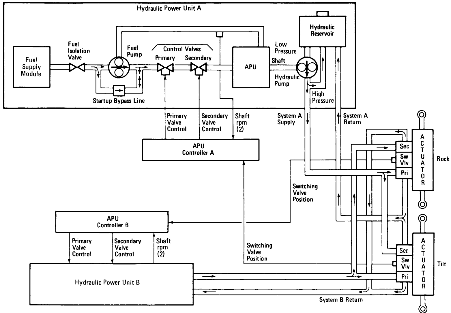
Hydraulic Power Unit System
