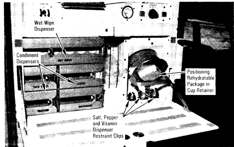
Galley Food System Accessories
