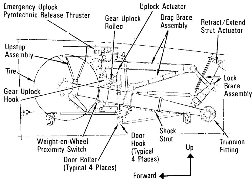
Main Landing Gear Stowed
