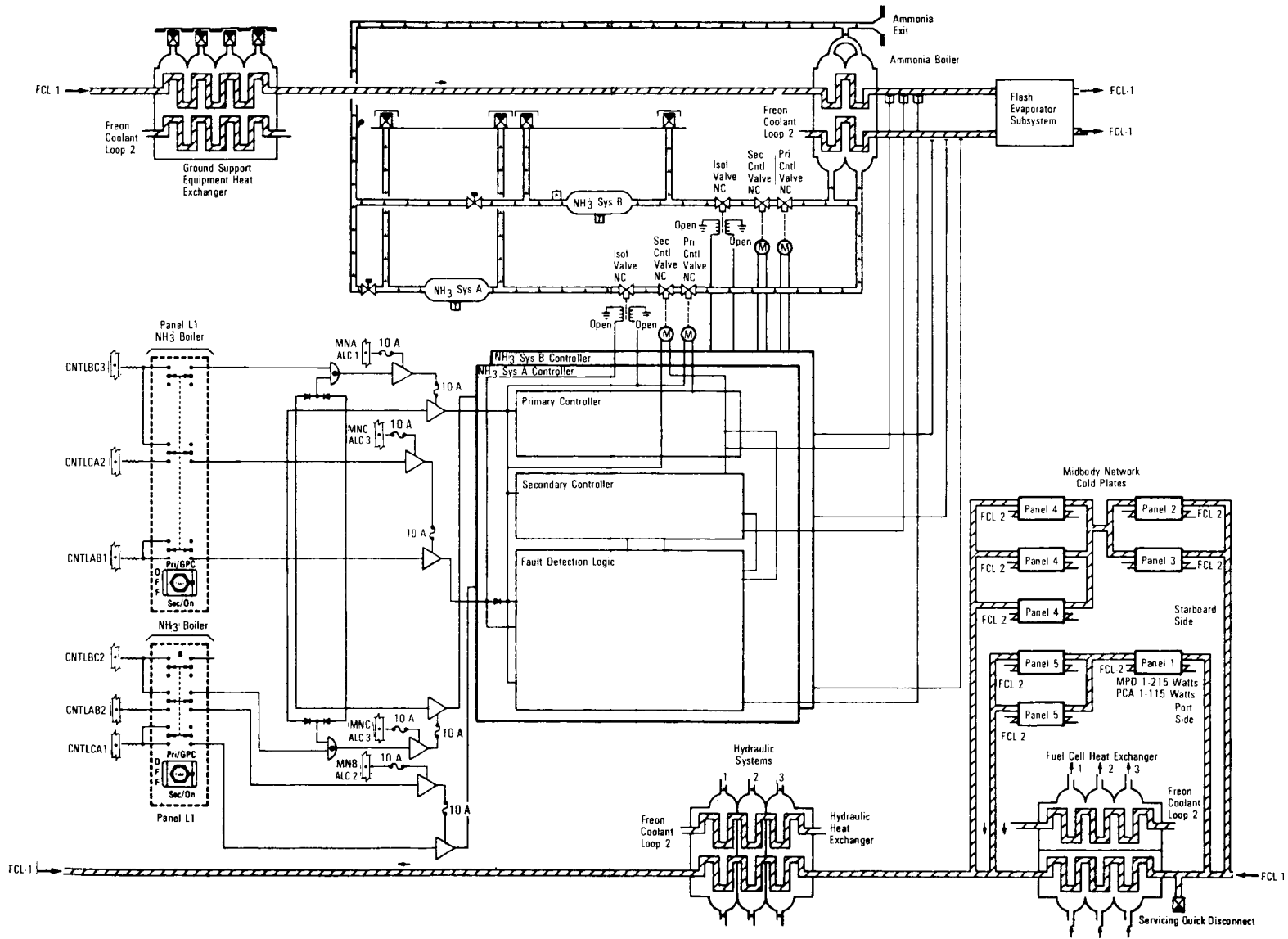
Active Thermal Control Freon-21 Coolant Loop (Sheet 2 of 3)
