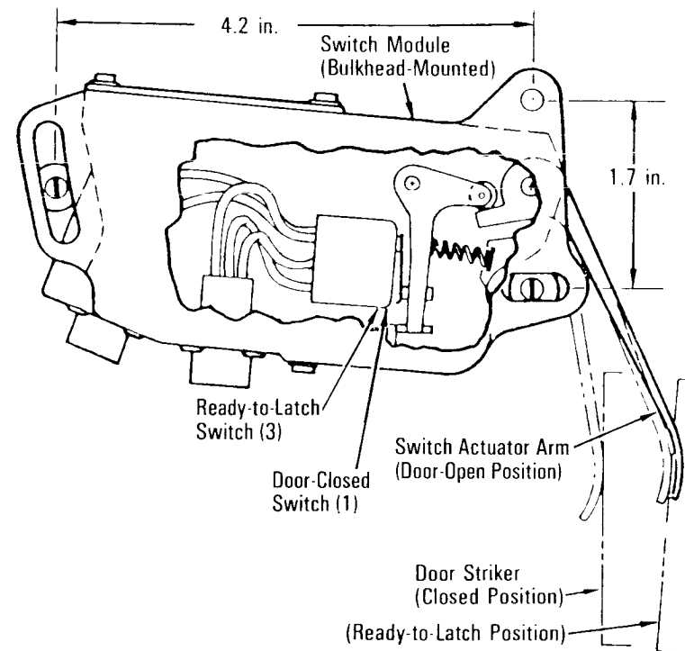
Payload Bay Door Ready-to-Latch Switch Module, Bulkhead Latches
