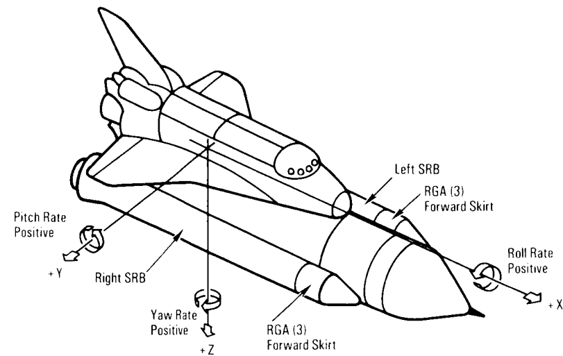
Rate Gyro Assembly Location and Rotation Axes
