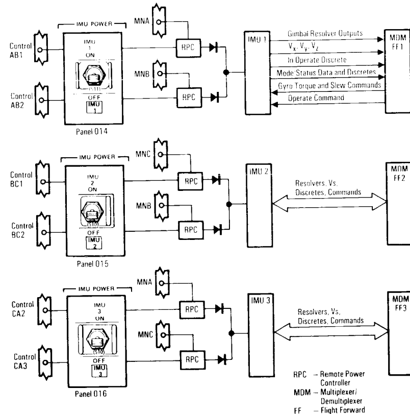
Inertial Measurement Unit Power and Data Interfaces
