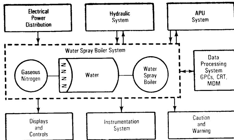
Water Spray Boiler System
