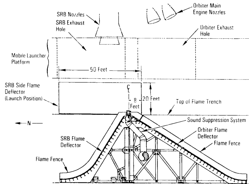
Orbiter/Solid Rocket Booster Flame Deflector
