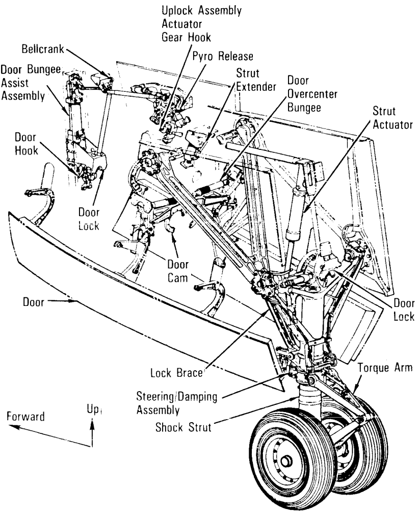
Nose Landing Gear Deployed
