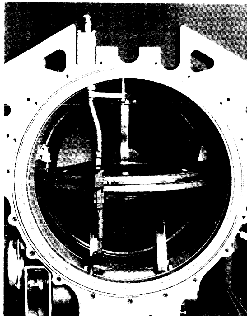
17-Inch Disconnect With Latch Feature Engaged on One Flapper Valve (Other Flapper Valve Removed to Show Latch Feature, Engagement)
