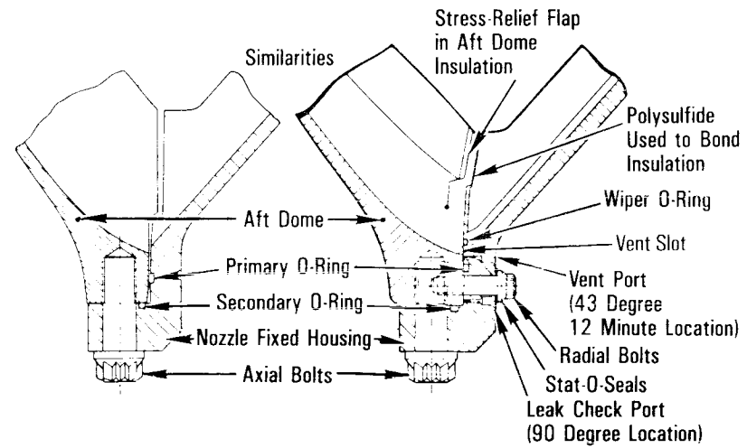
Original Case-to-Nozzle Joint Design
