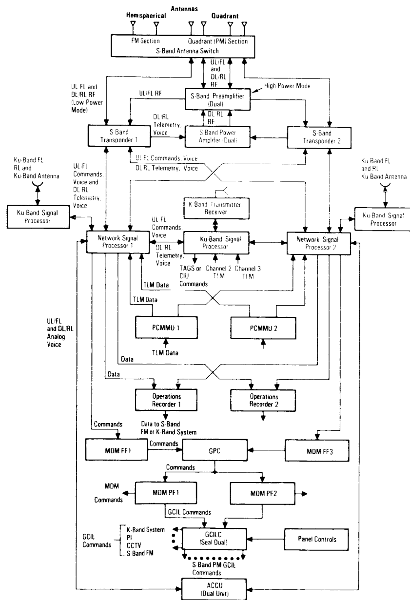
Ku-Band and S-Band System
