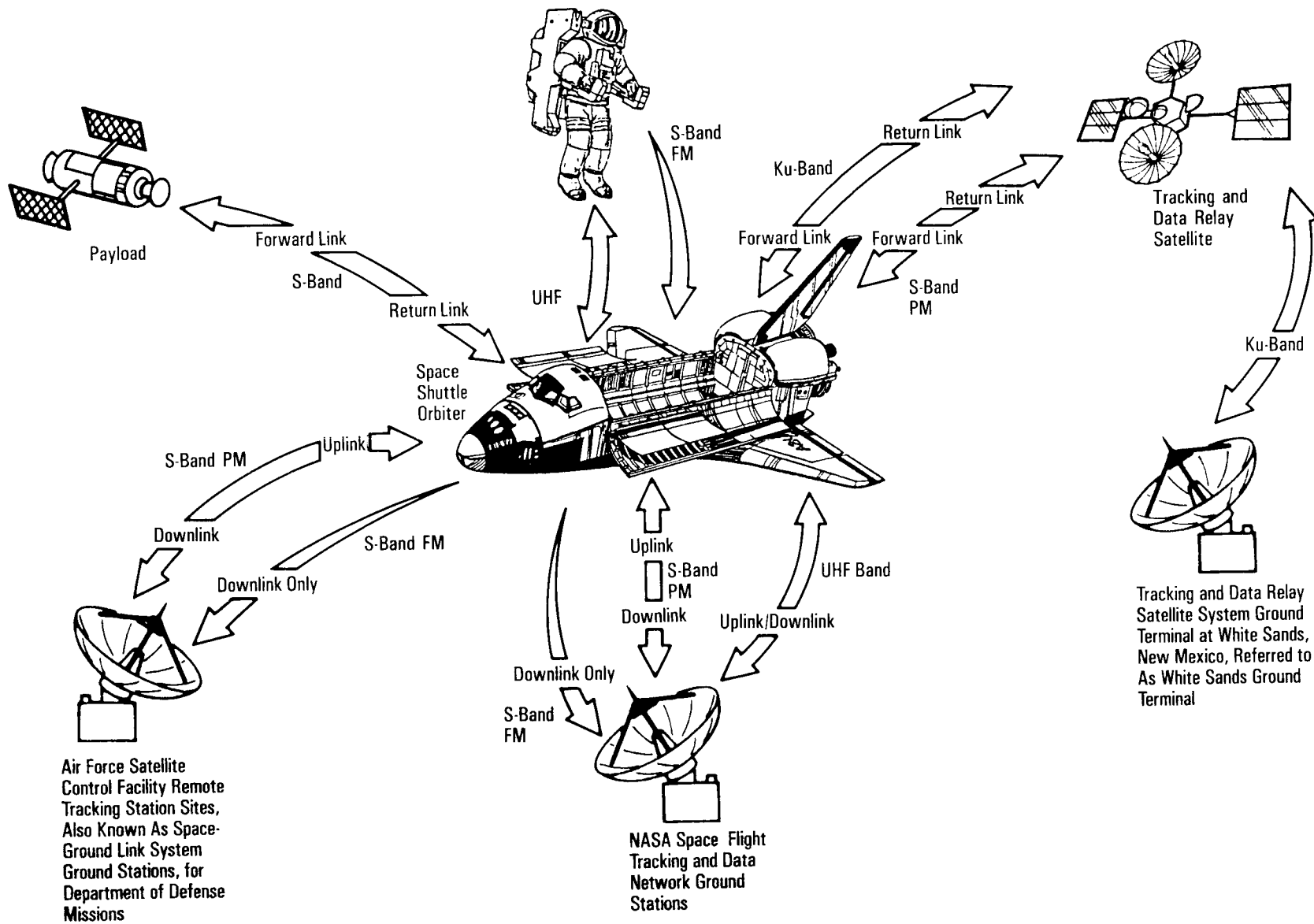
Space Shuttle Orbiter Radio Frequency Links
