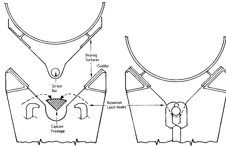
The RMS Retention Mechanism
