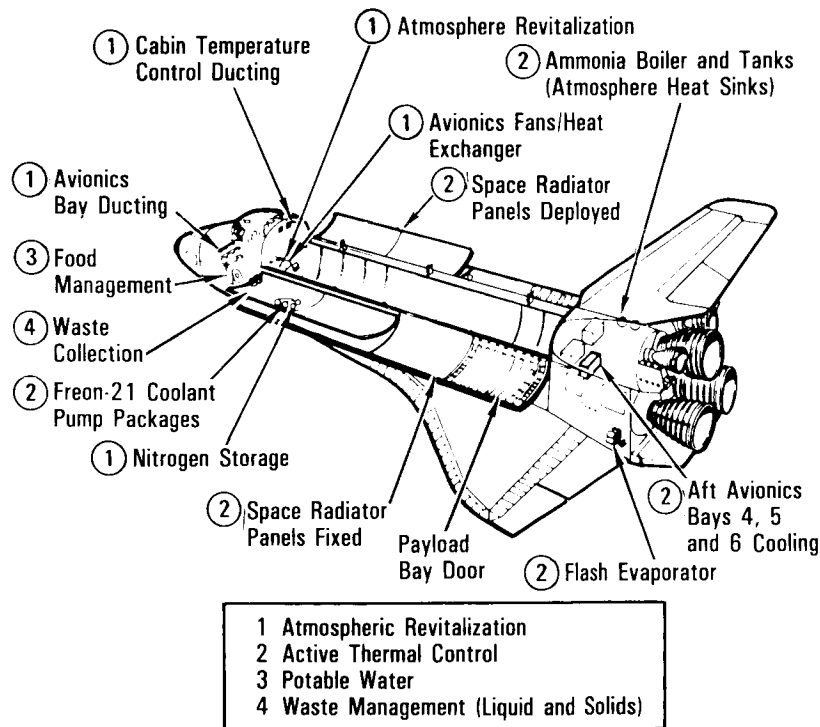
Environmental Control and Life Support System
