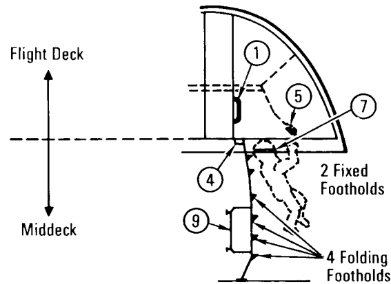
Primary Interdeck Area (Port Side Looking Aft)
