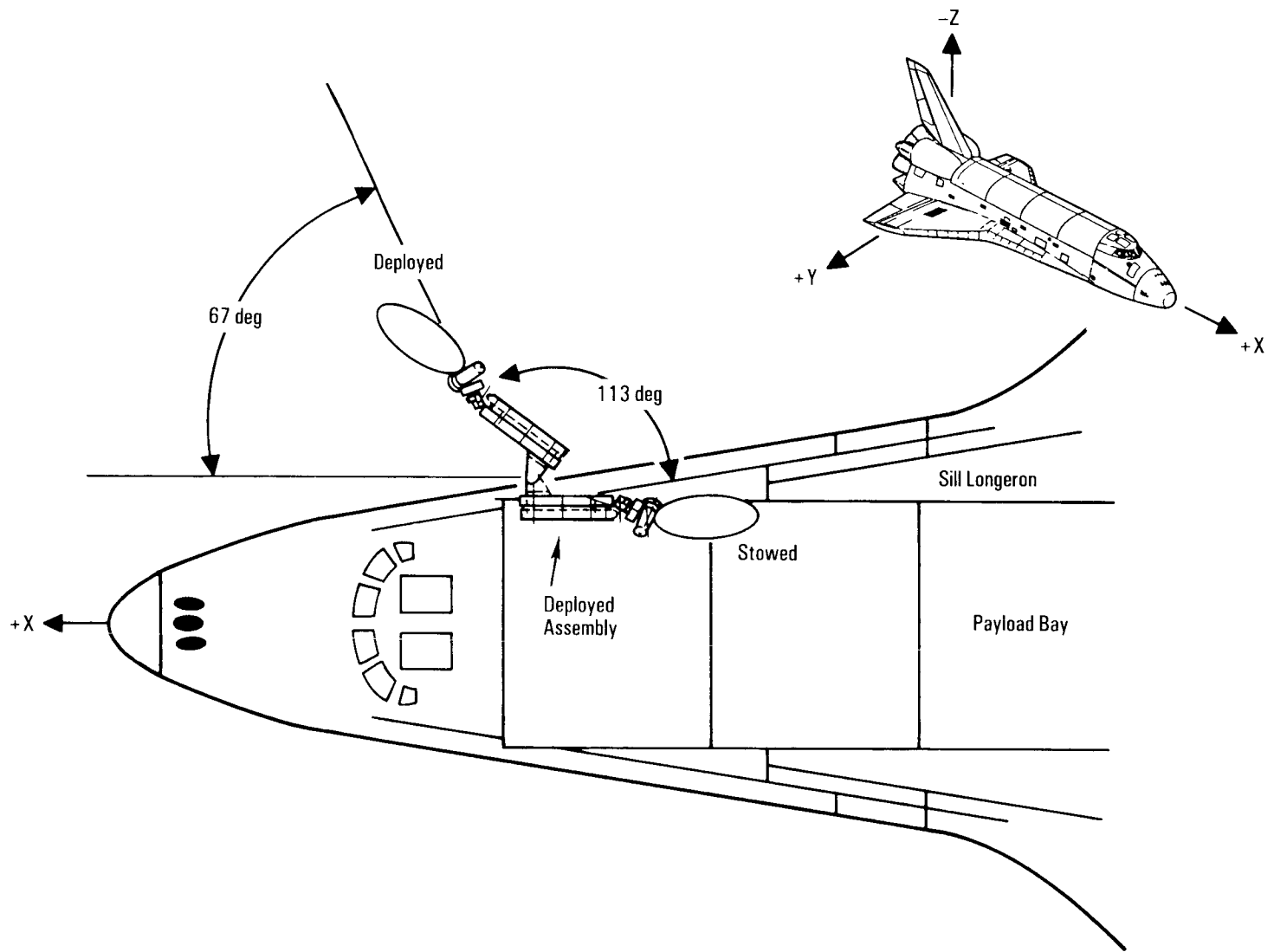
Ku-Band Deployed Assembly Location
