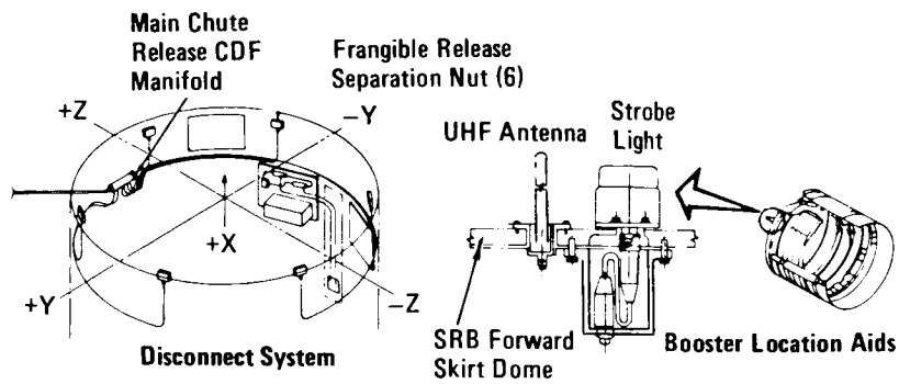
SRB Parachute Release and Retrieval Aids
