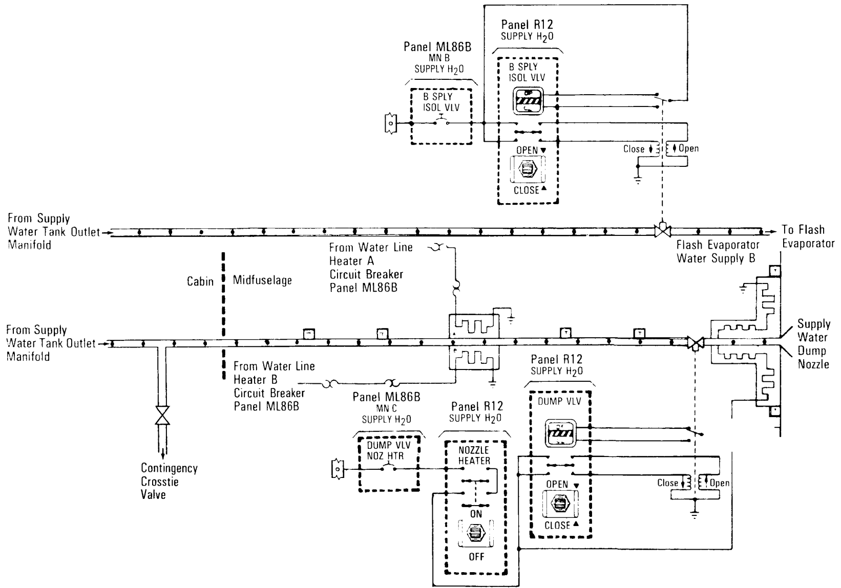
Potable Water (Sheet 3 of 3)
