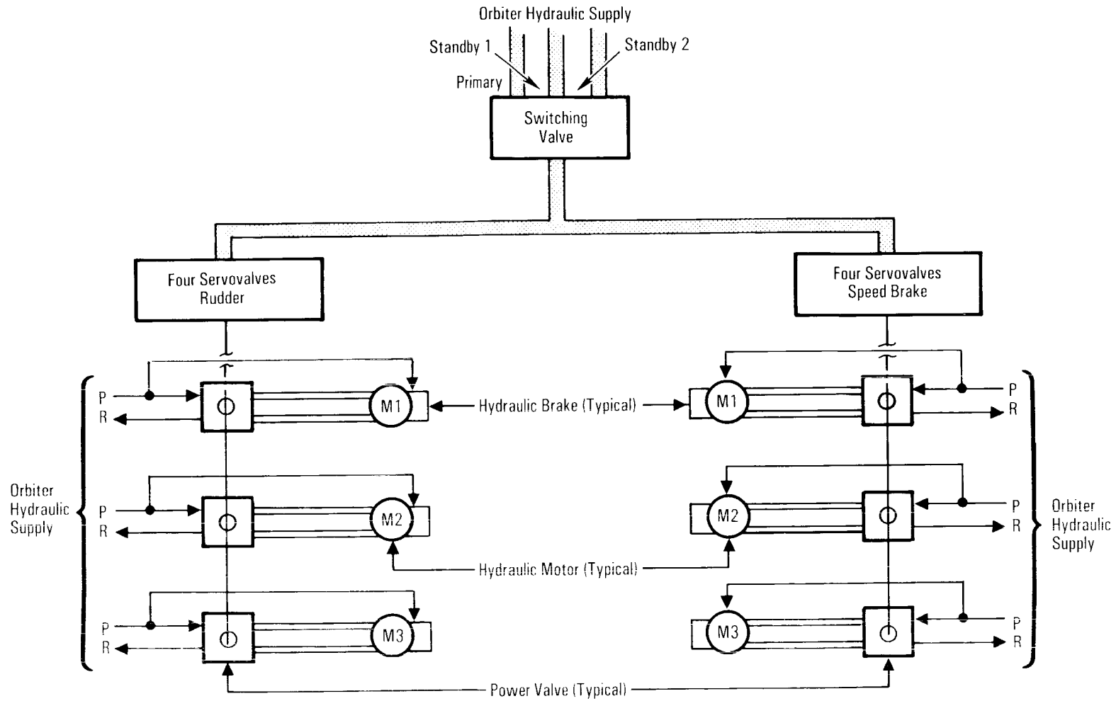
Rudder/Speed Brake Hydraulic Supply Overview
