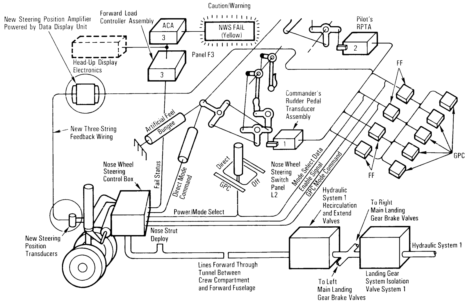
Nose Wheel Steering System Overview
