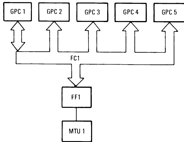
GPC Communicating Through the Forward MDM 1 With Master Timing Unit
