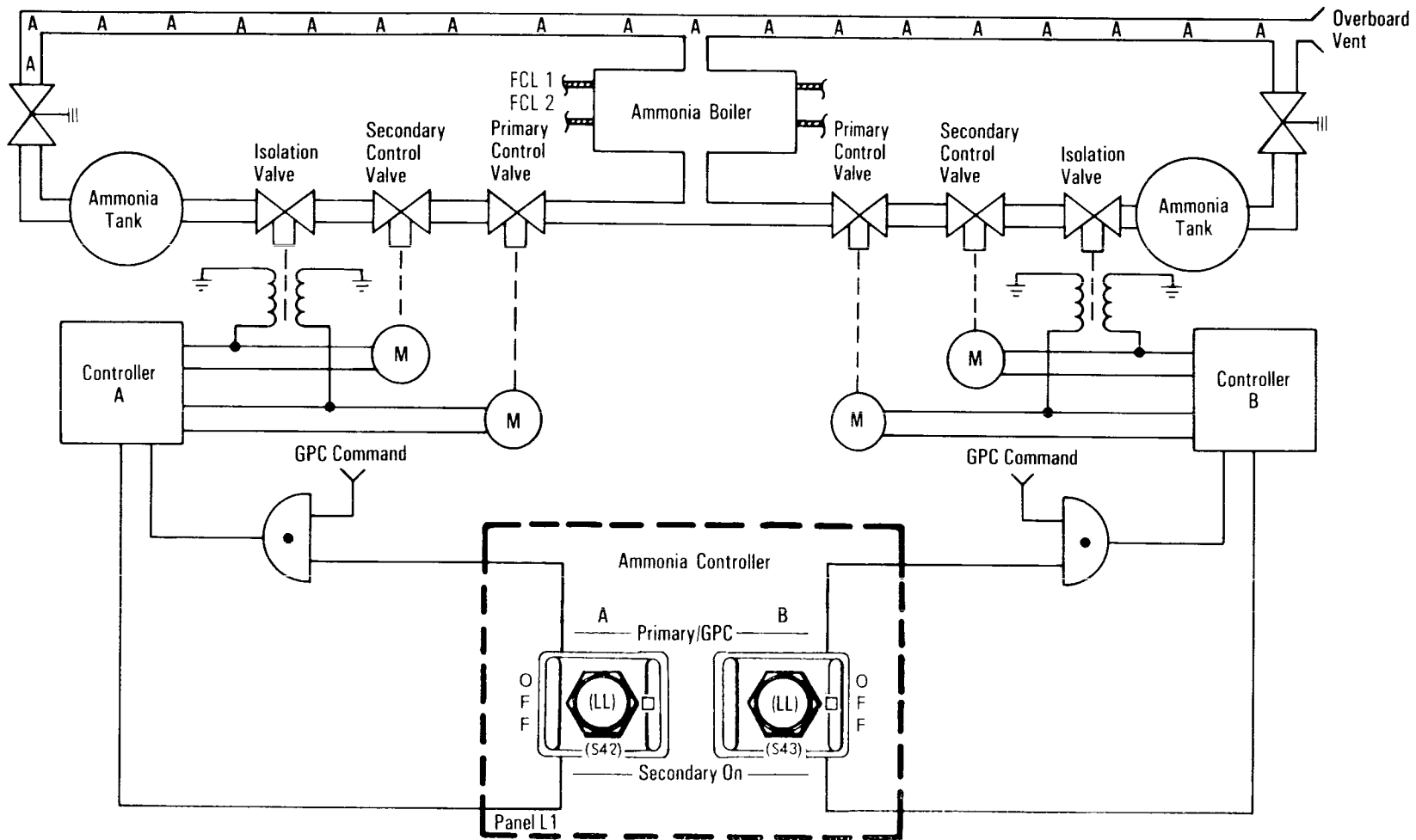
Ammonia Boiler Control
