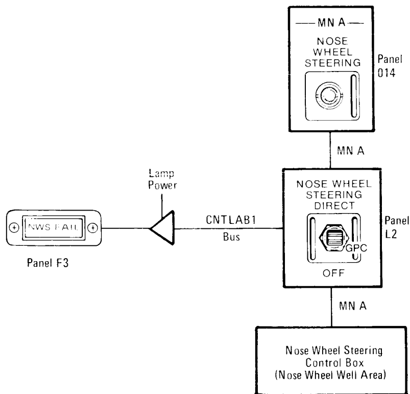
Nose Wheel Steering Power
