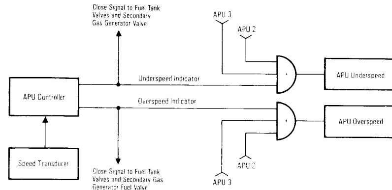
APU Overspeed/Underspeed Detection
