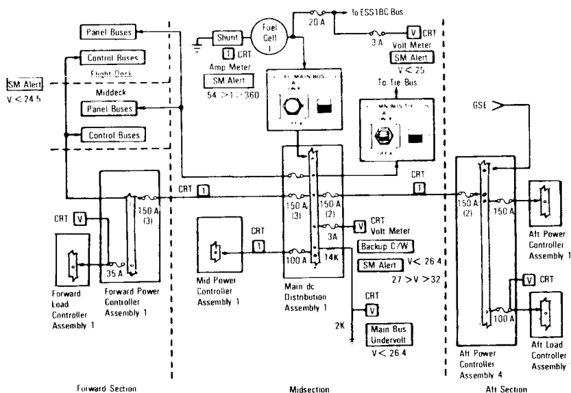
Main Bus A Distribution
