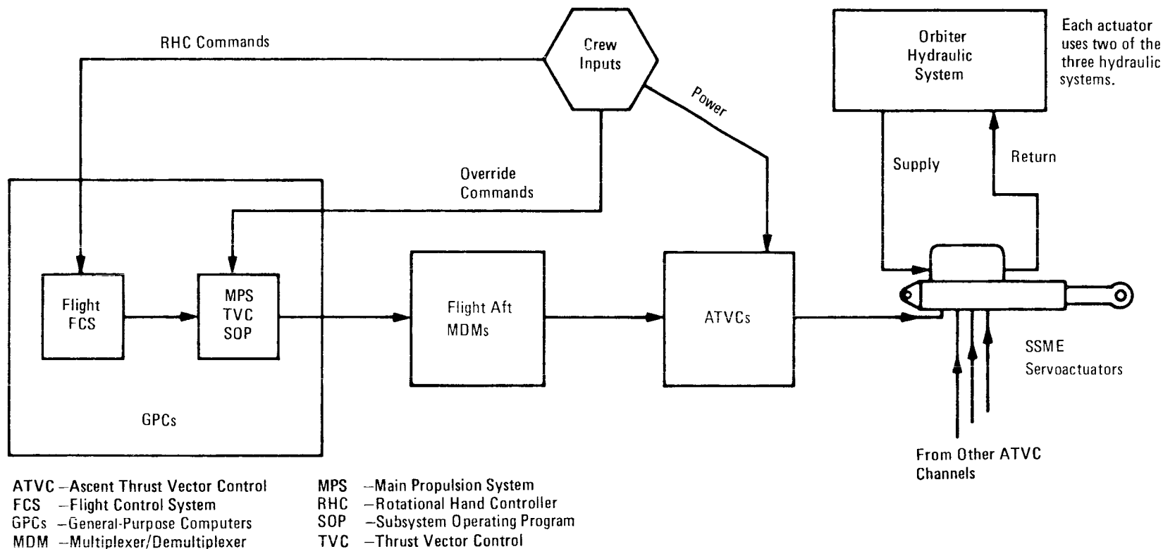
SSME Thrust Vector Control Interface Flow
