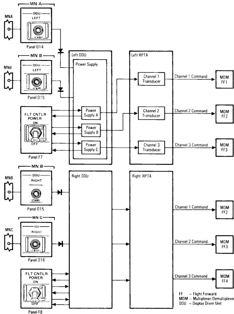
Rudder Pedal Transducer Assembly Power and Data Interfaces
