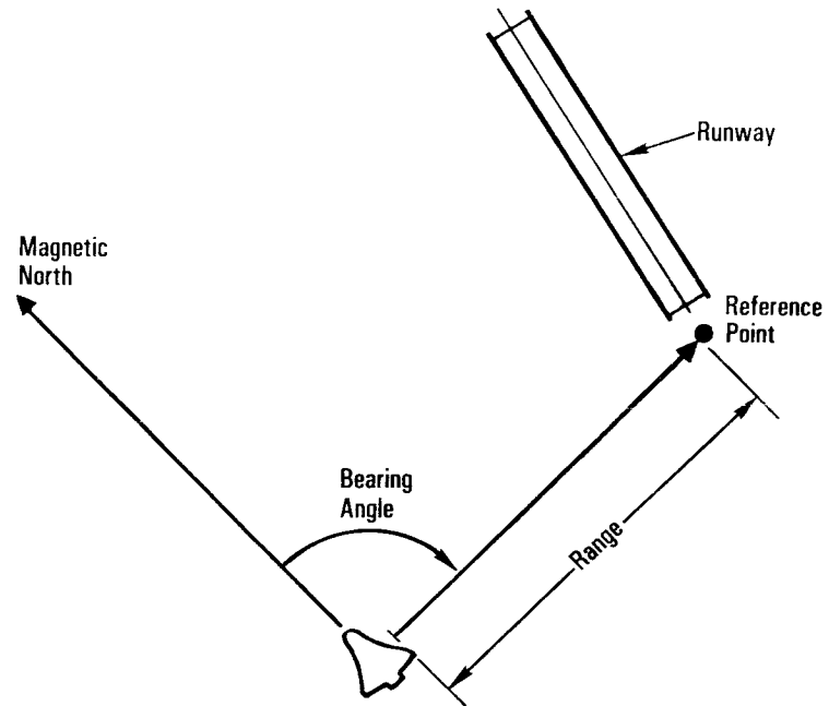
Horizontal Situation Indicator Bearing and Range Geometry
