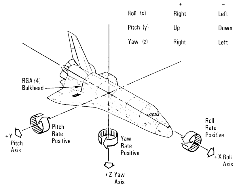
Solid Rocket Booster Rate Gyro Assembly Location and Rotation Axes
