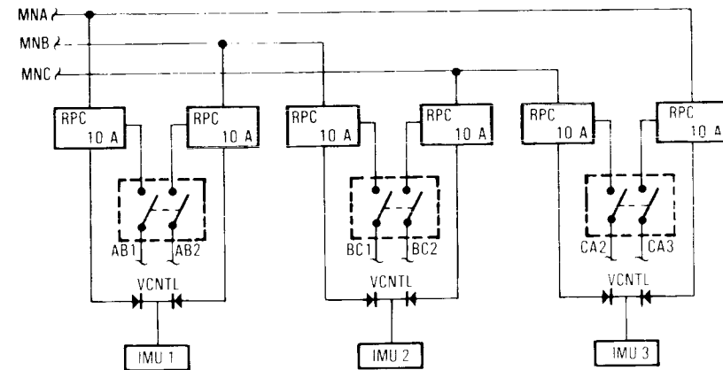
Inertial Measurement Unit Electrical Power Interface
