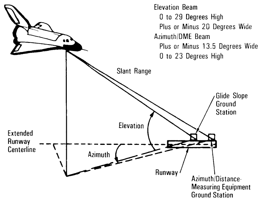
Microwave Scan Beam Landing System
