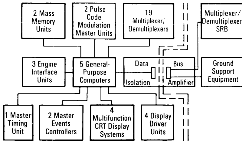
Data Processing System
