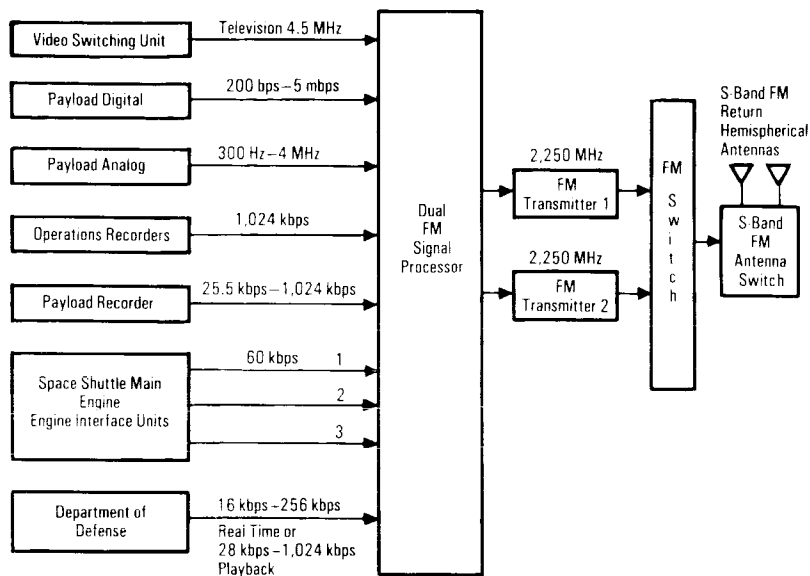
S-Band Frequency Modulation Signal Processor (Not Operative Through TDRS)
