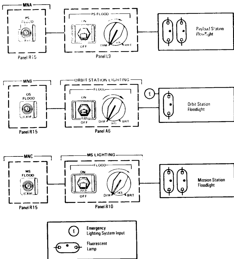
Aft Flight Deck Floodlight Control
