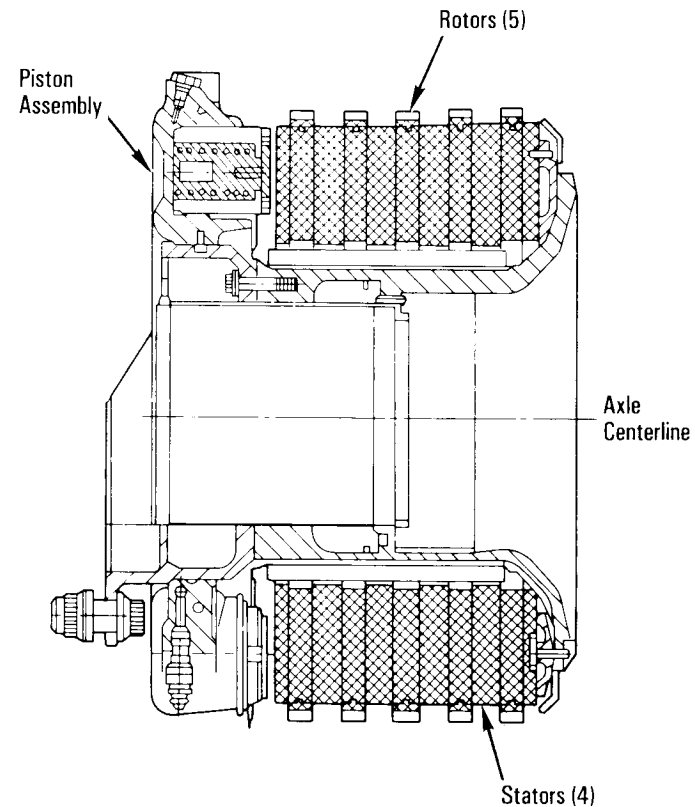
Future Main Landing Gear Carbon Brake Assembly
