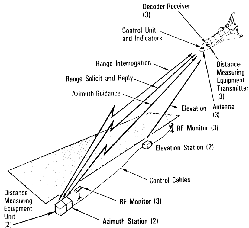
Major Microwave Scan Beam Landing System Components and Radio Frequency Links
