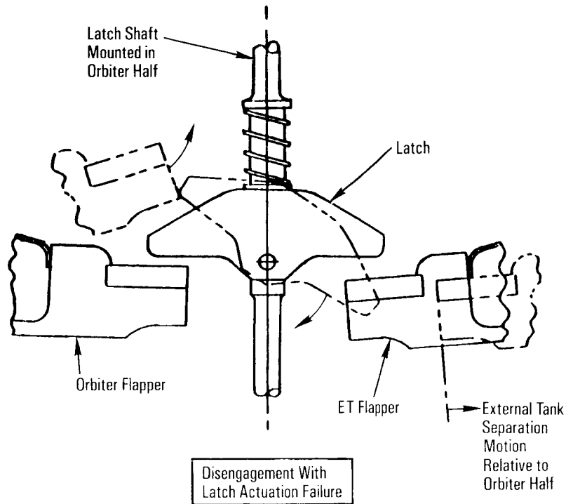
Orbiter/External Tank 17-Inch Disconnect, Backup Unlatch Feature of Flapper Valves
