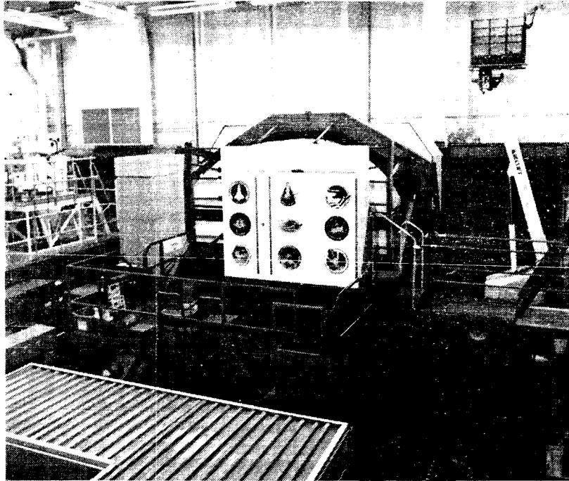
Fixed-Base Shuttle Mission Simulator
