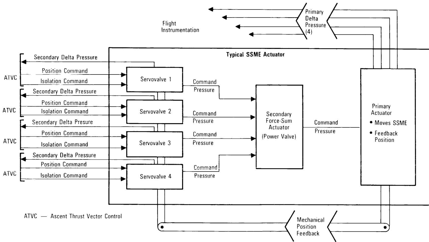
Typical SSME Actuator
