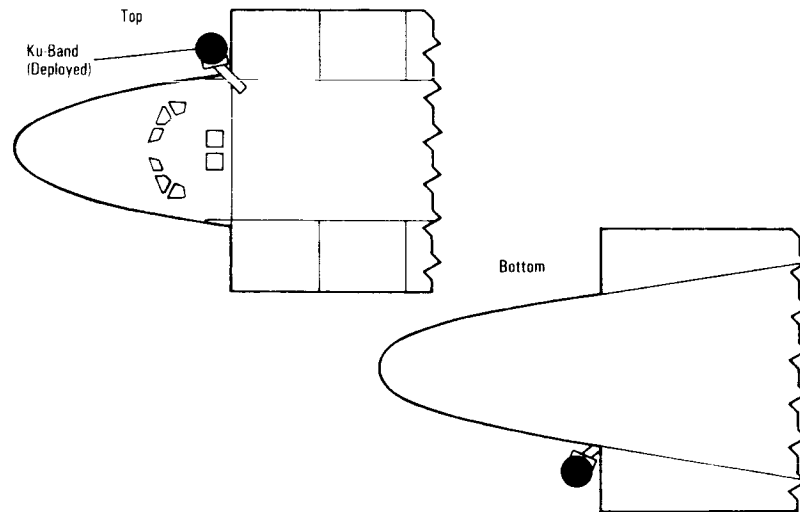
Ku-Band System Antenna Location (Deployed)
