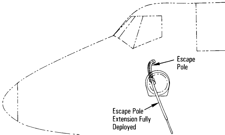
Side View of Escape Pole Deployed Through Side Hatch
