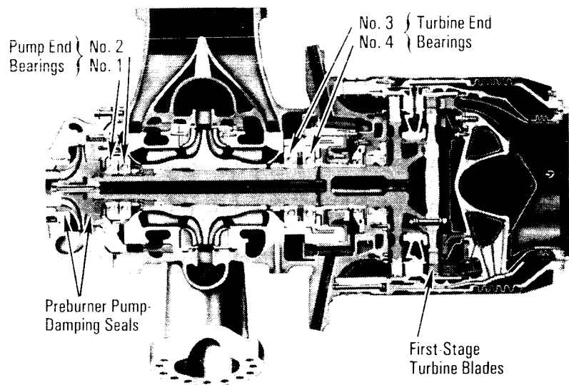
Phase II—High-Pressure Oxidizer Turbopump
