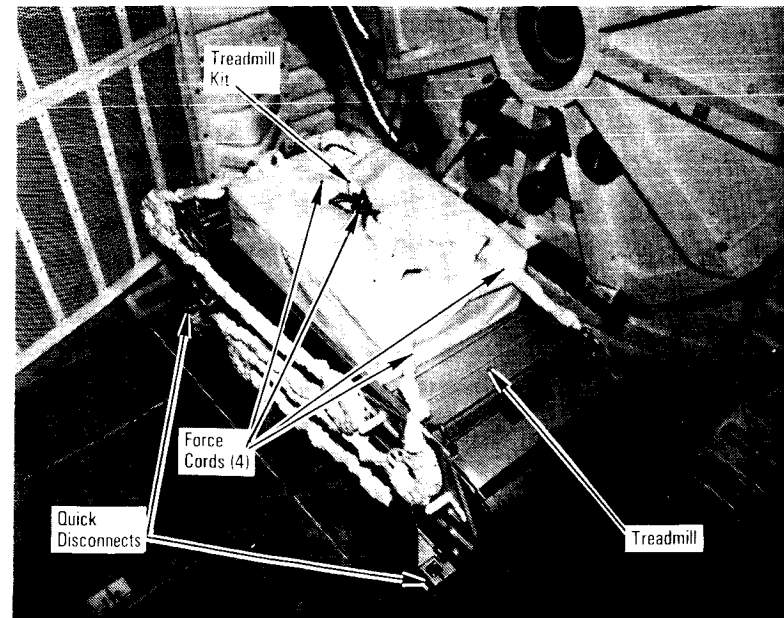
Treadmill
