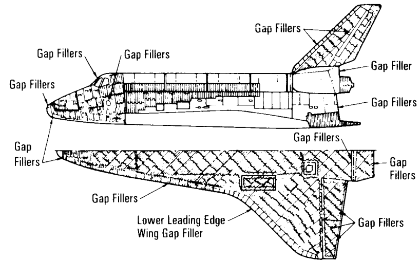
TPS Tile Gap Filler Locations
