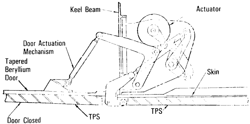
Orbiter/External Tank Umbilical Doors—Hinge/Actuation System
