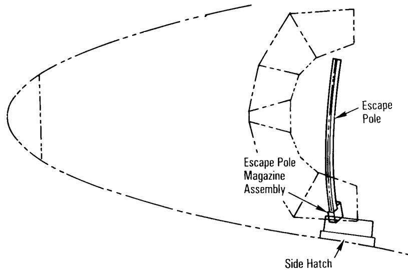
Escape Pole Ascent/Descent Position, Middeck Top View
