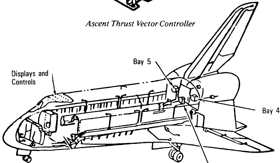
Location of Orbiter Avionics Bays
