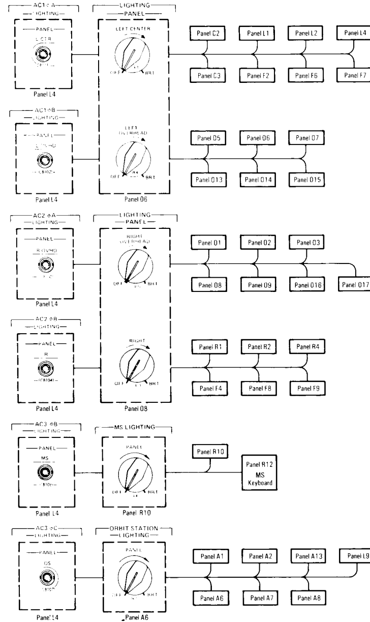
Panel Lighting Controls
