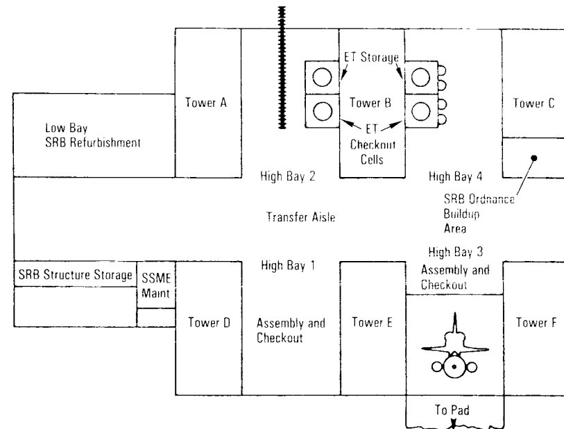
Vehicle Assembly Building Floor Plan
