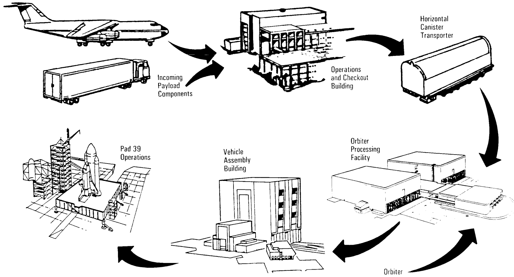
Horizontal Payload Processing Flow
