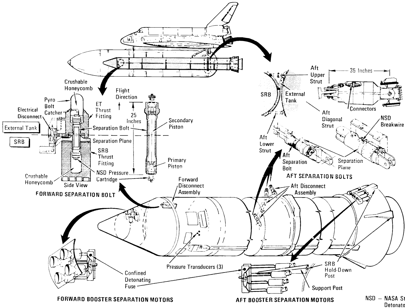
Separation System Elements
