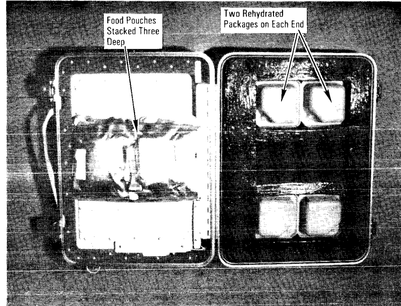
Food Warmer With Hydratable Packages in Place for Heating
