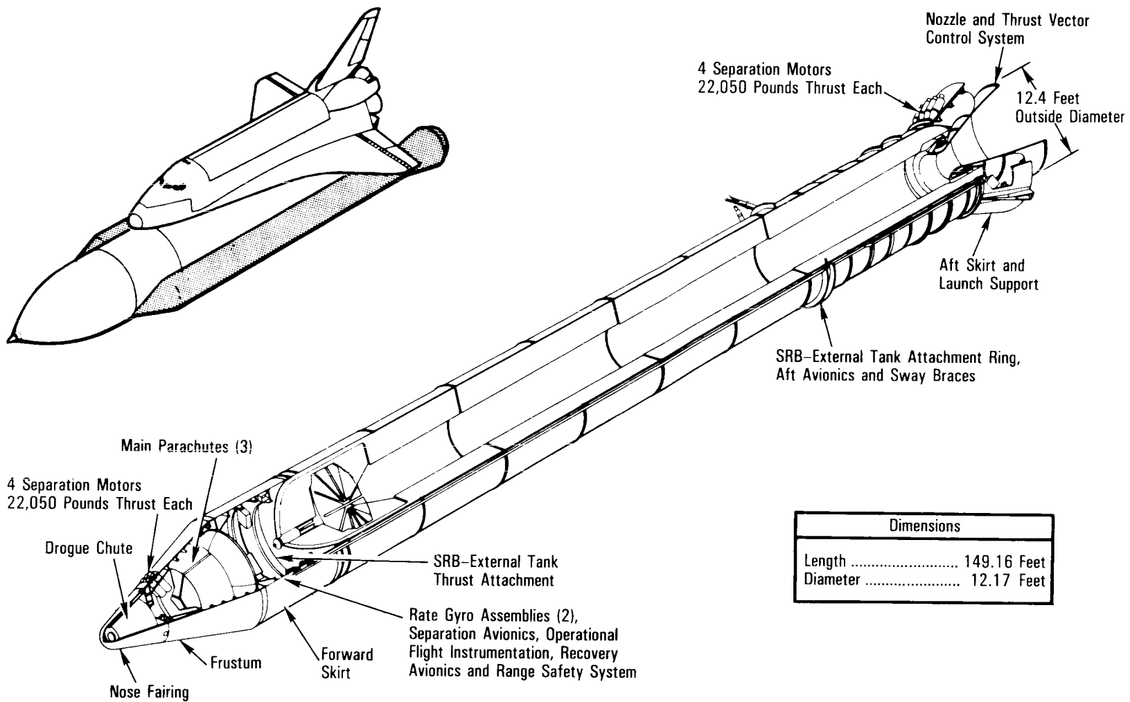
Solid Rocket Booster
