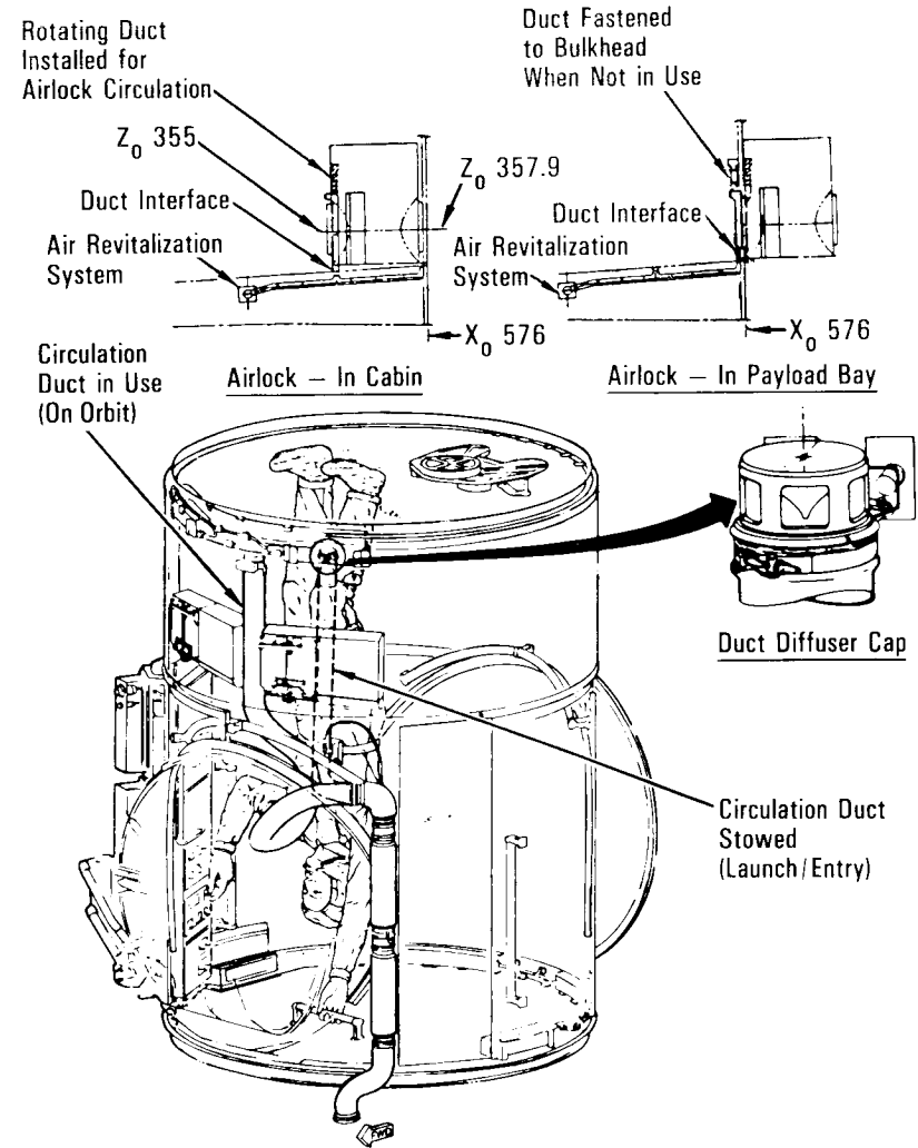
Airlock in Middeck Without Spacelab Tunnel Adapter
