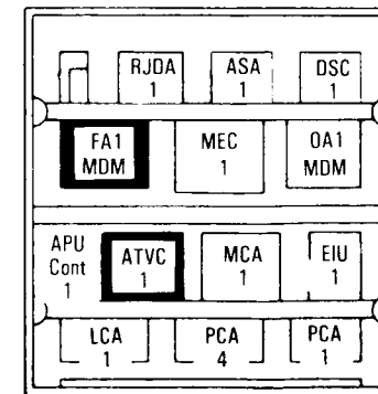
Avionics Bays 4, 5 and 6
