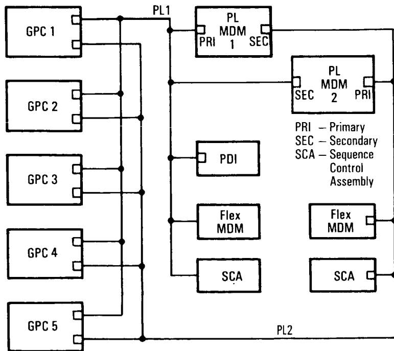
Payload Data Buses
