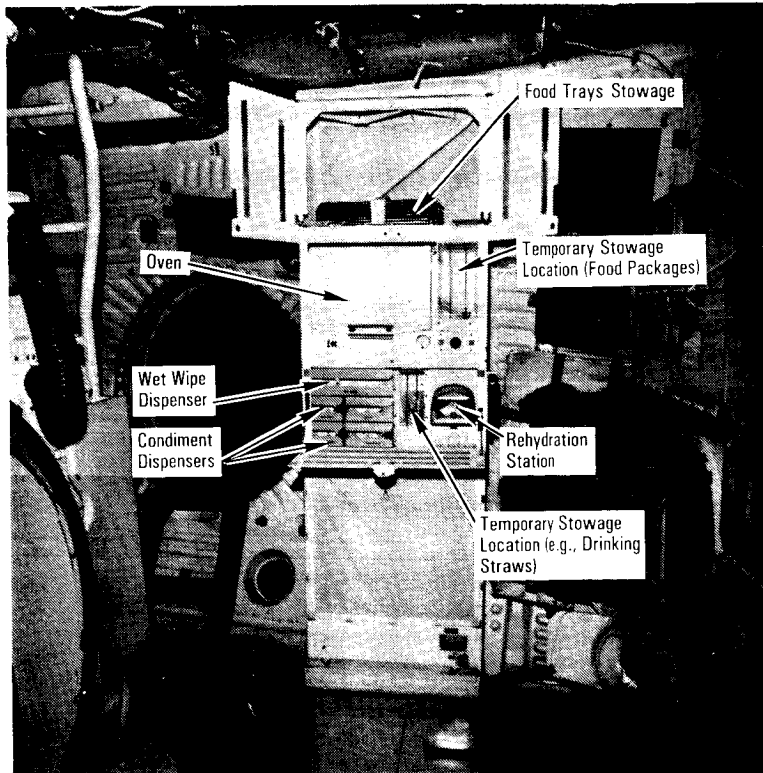
Galley System Components
