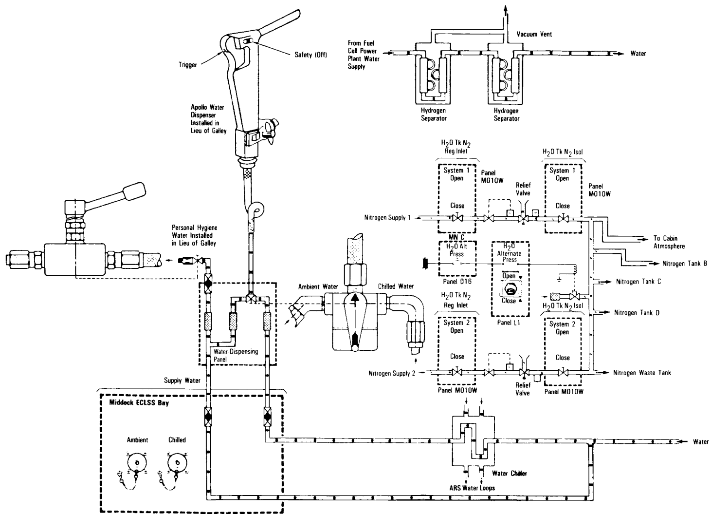
Potable Water (Sheet 1 of 3)
