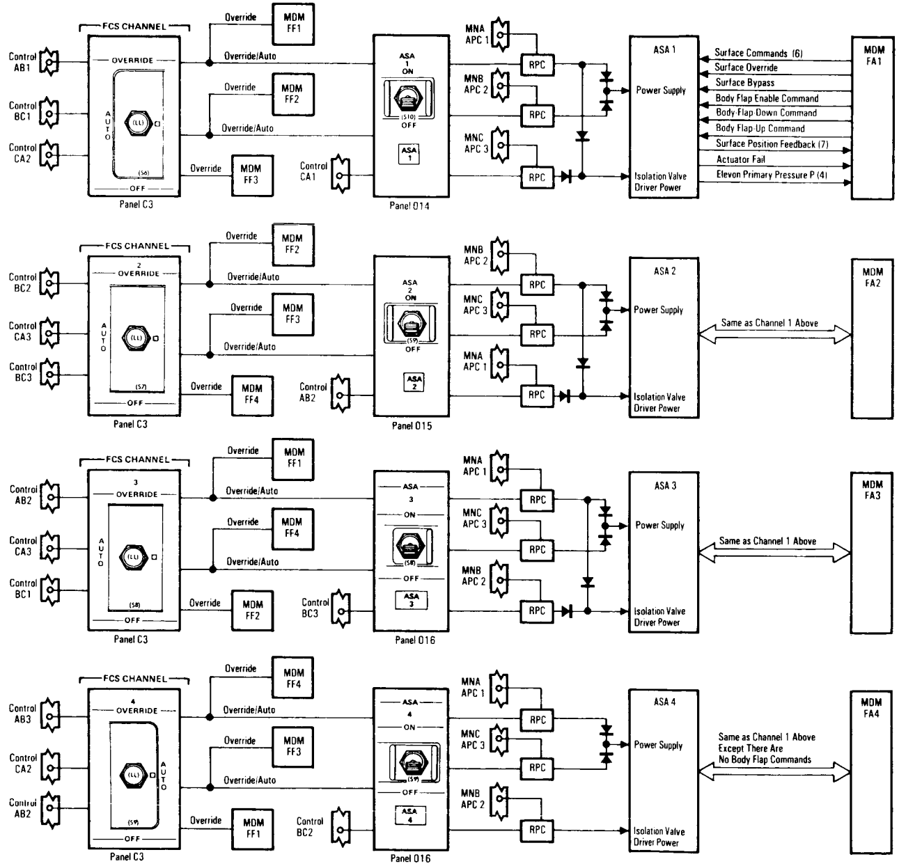
Power and Data Interfaces of Aeroface Servoamplifiers
