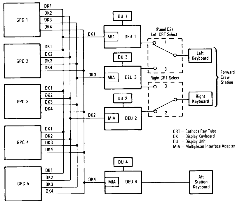
Display Electronics Unit and Keyboard Data Bus/GPC Interfaces
