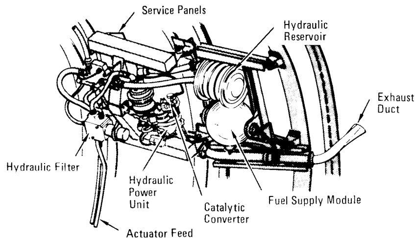
SRB Auxiliary Power Unit/Hydraulic Power Unit Location
