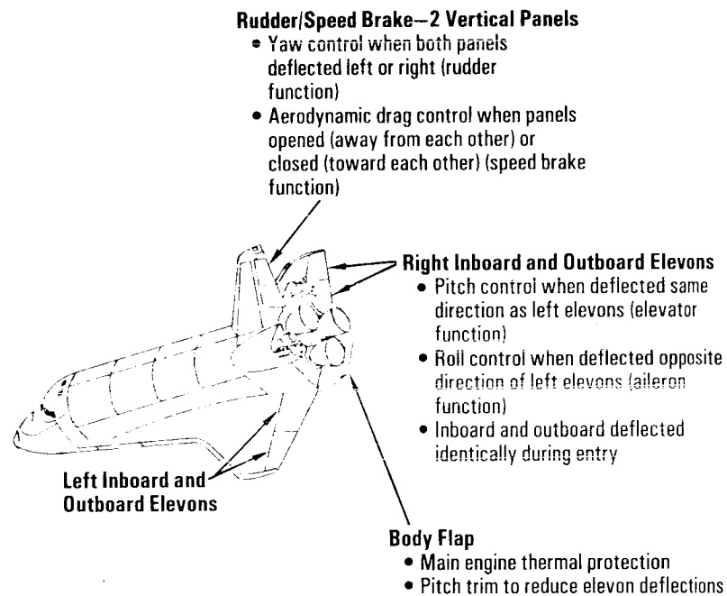
Aerodynamic Surfaces
