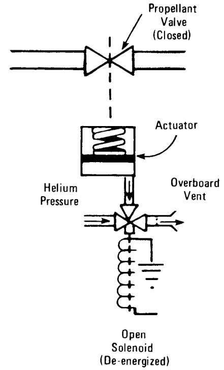
③ Control Switch in GPC Position (No GPC Command Present)
