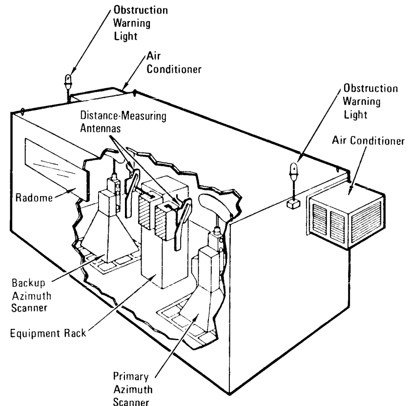
Azimuth/Distance-Measuring Equipment Shelter and Equipment
