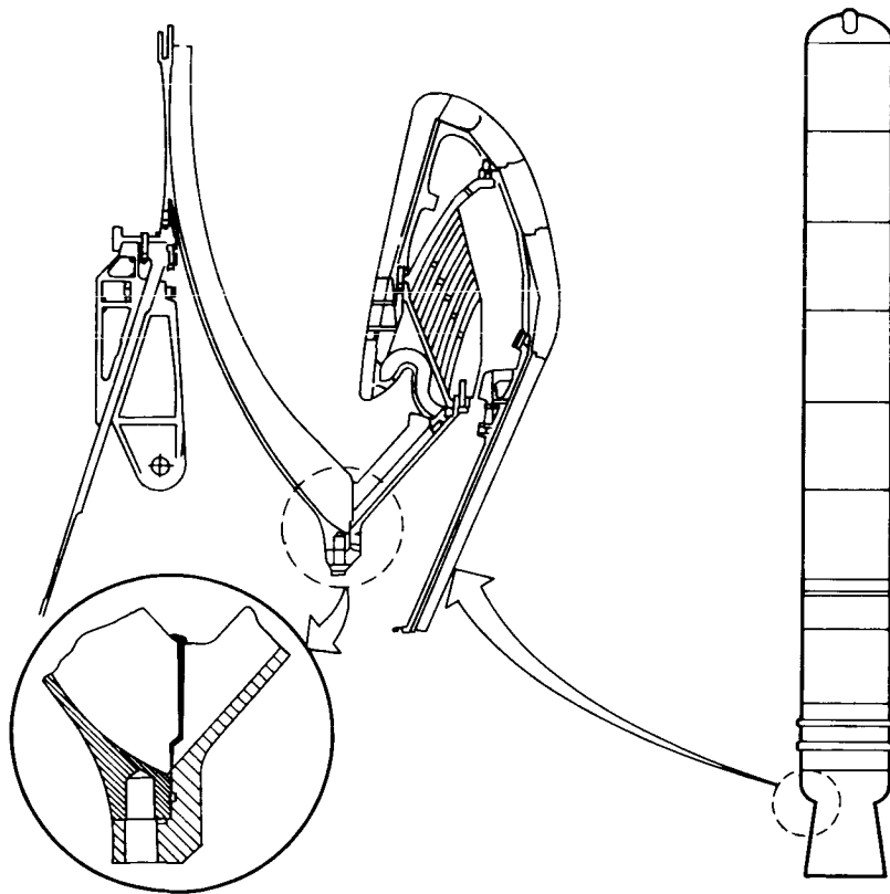
Nozzle-to-Case Joint
