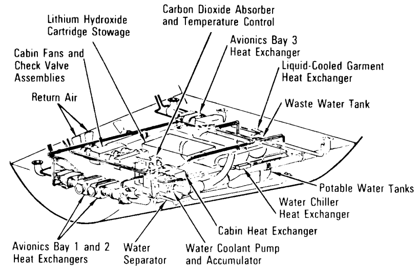
Crew Cabin Bottom Deck ECLSS (Below Middeck Floor)
