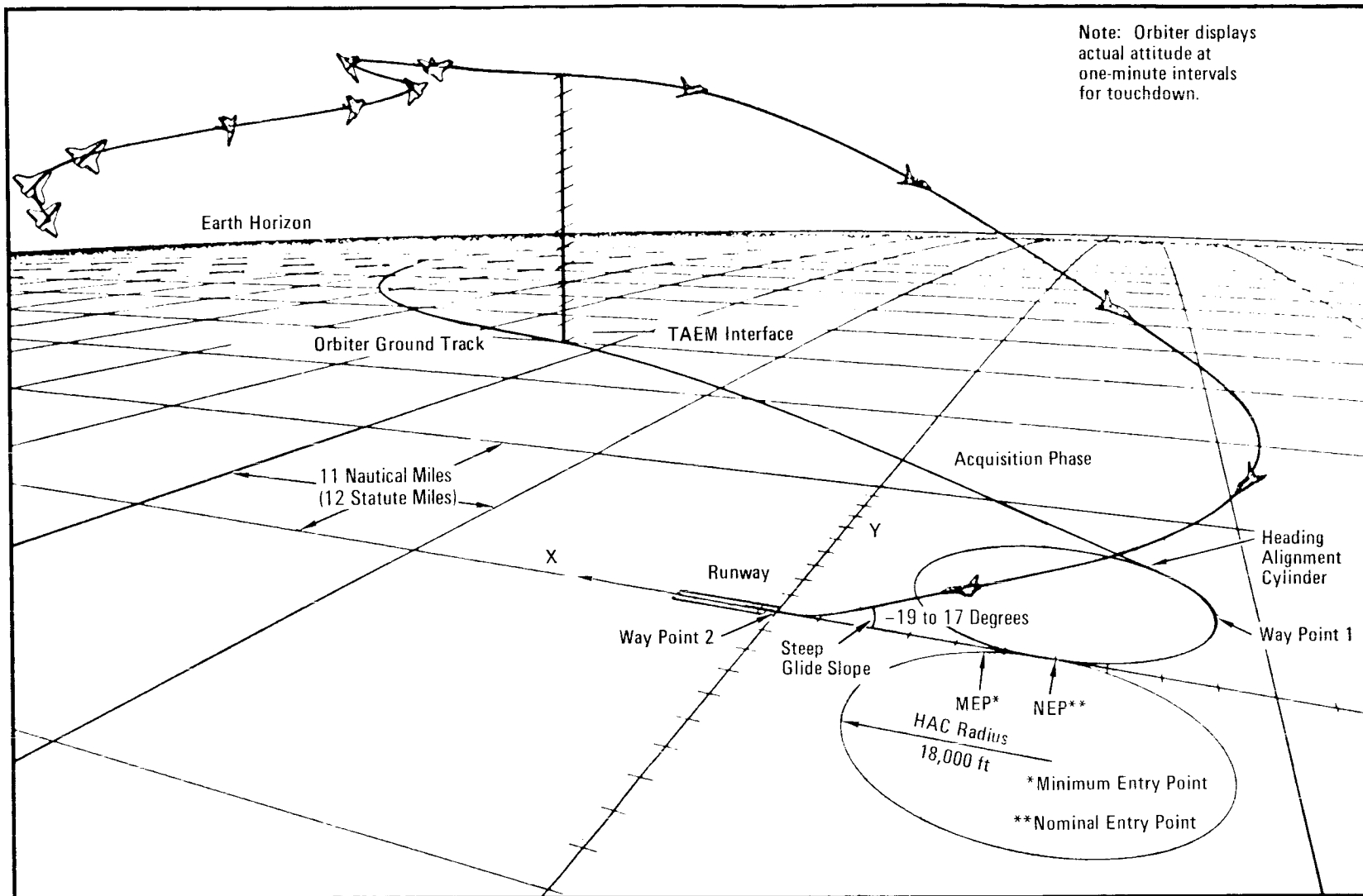
Entry Flight Profile
