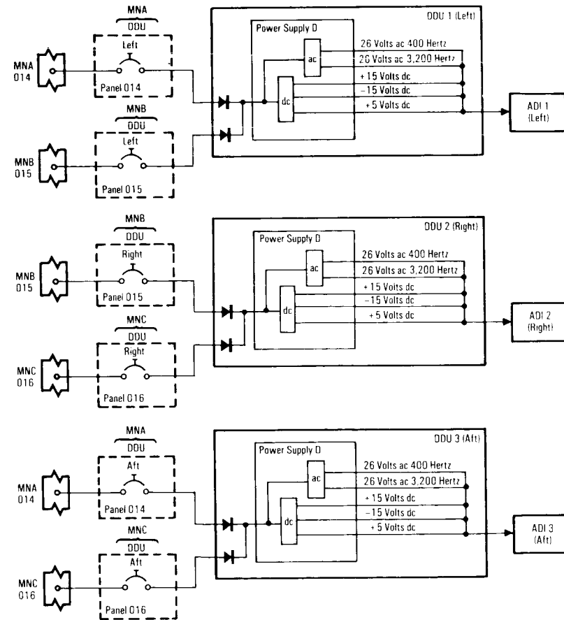
Attitude Director Indicator Power
