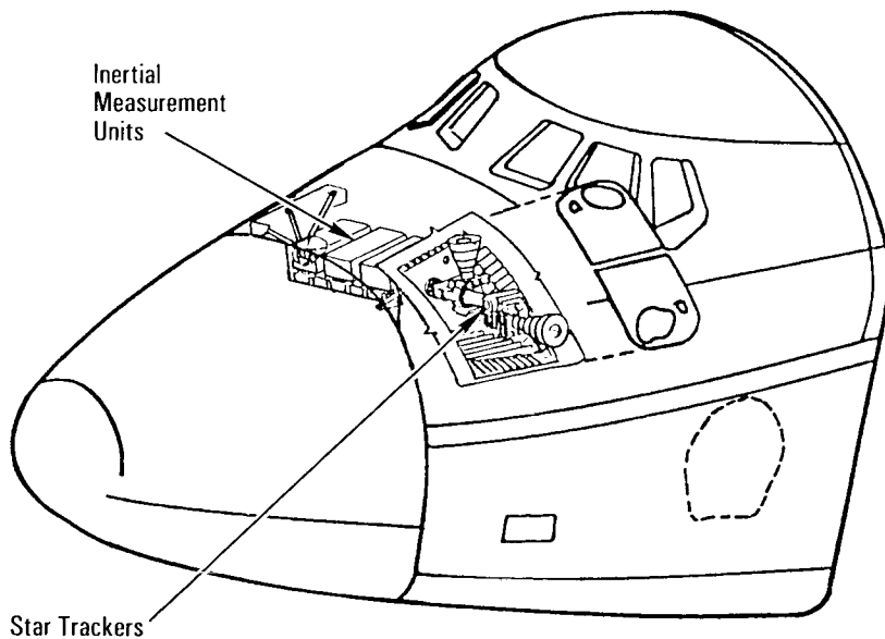
Location of Star Trackers
