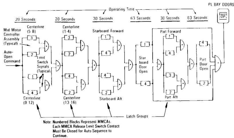
Simplified Payload Bay Door Auto-Open Signal Flow
