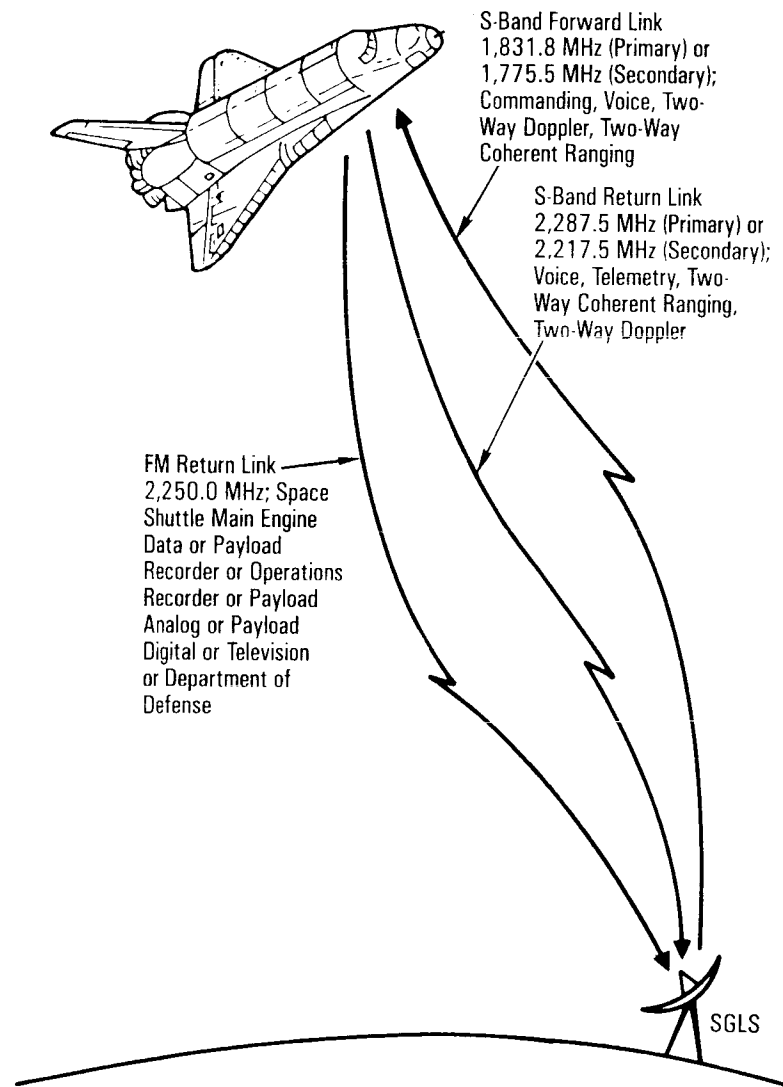
Department of Defense S-Band Communications With Air Force Satellite Control Facility Remote Tracking Station Sites, Also Known as Space-Ground Link System
