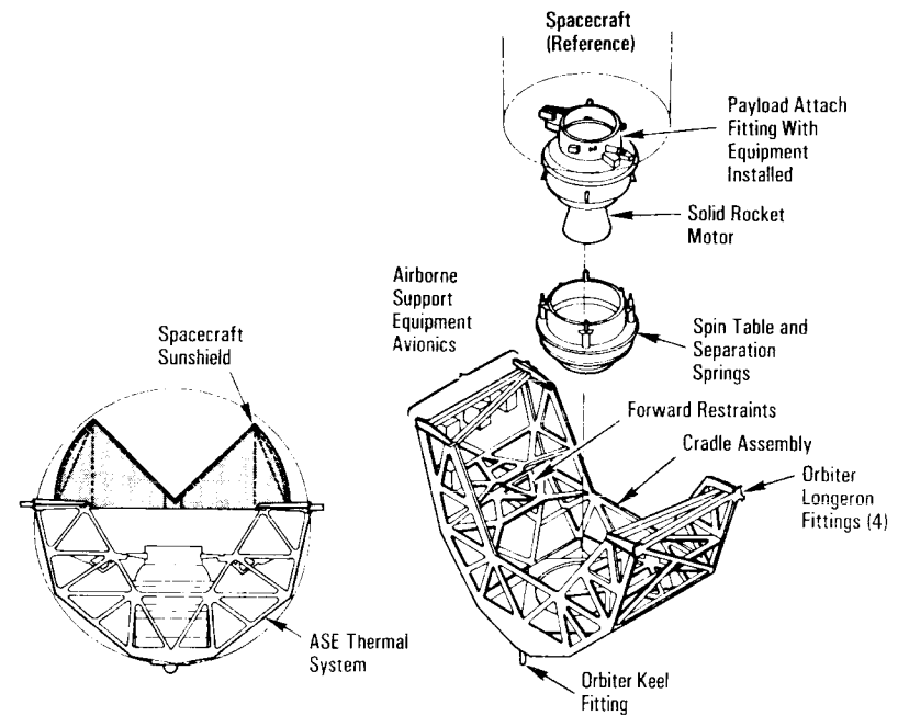
PAM System
