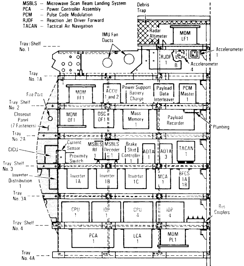
Component Locations—Bay 1
