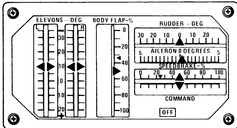
Surface Position Indicator
