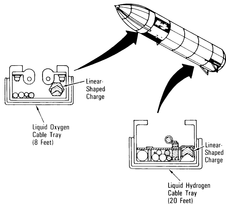
External Tank Range Safety System Linear-Shaped Charges
