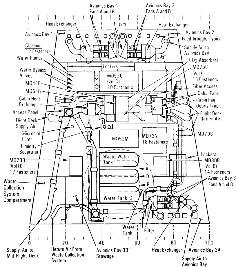
Lower Equipment Bay
