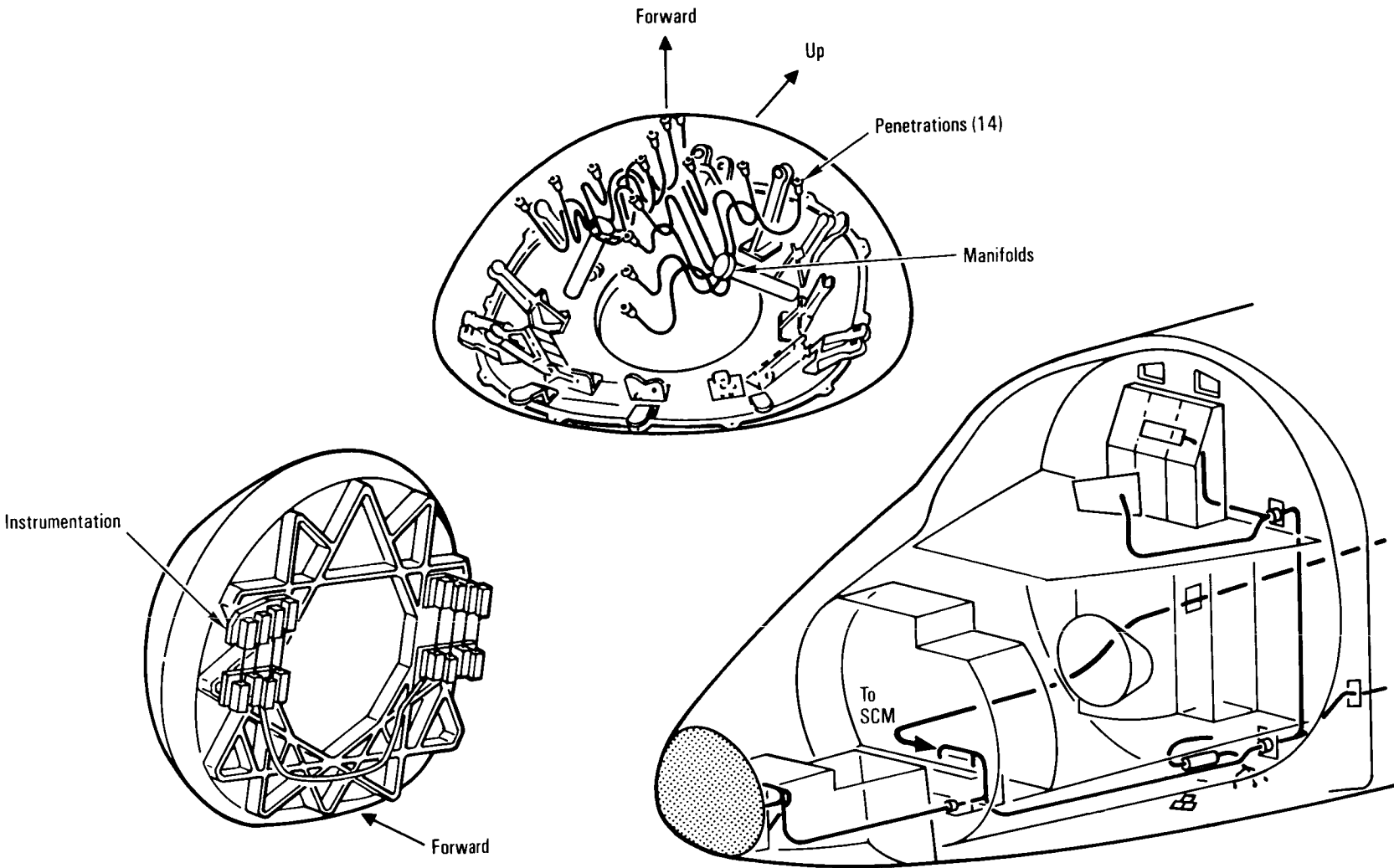
Shuttle Entry Air Data System
