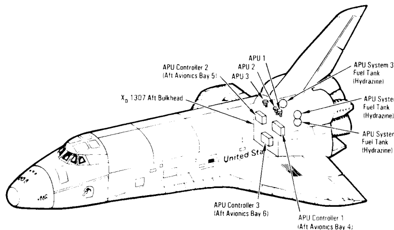
Auxiliary Power Unit, APU Controller and APU Fuel Tank Locations
