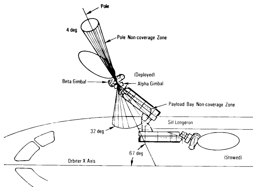
Ku-Band Antenna Non-coverage Zones
