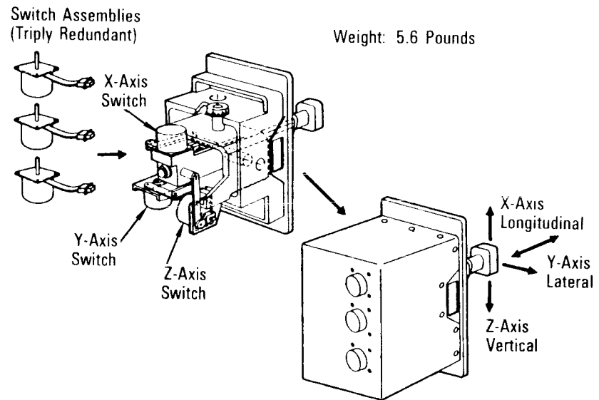
Translational Hand Controller
