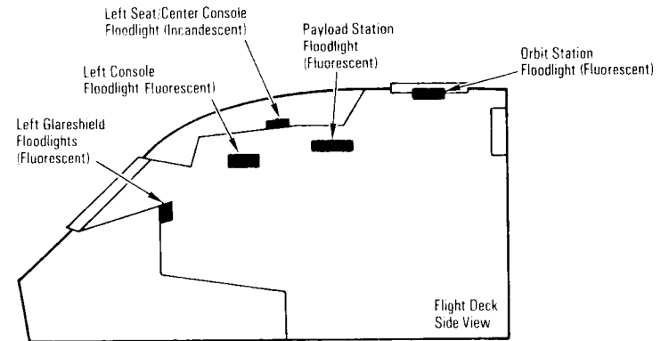
Floodlight Locations—Flight Deck Forward and Aft
