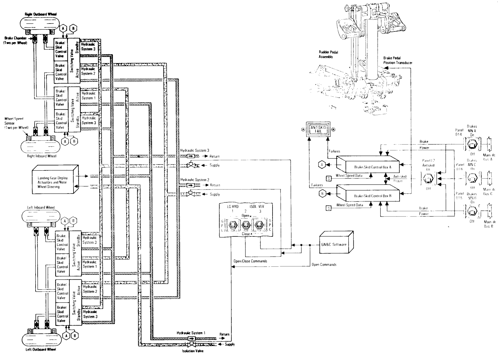
Brake/Skid Control
