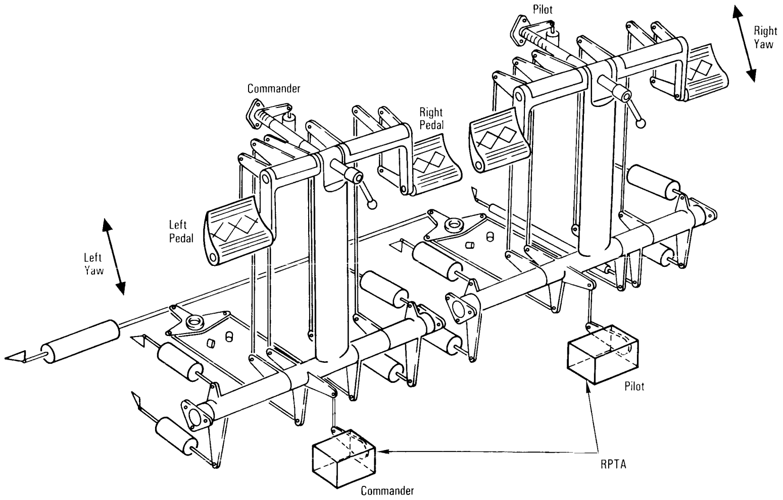
Rudder Pedal Transducer Assembly
