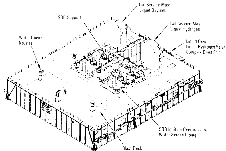
Mobile Launcher Platform, Exterior View
