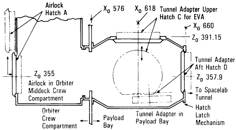
Airlock and Tunnel Adapter Hatch Mechanical Systems
