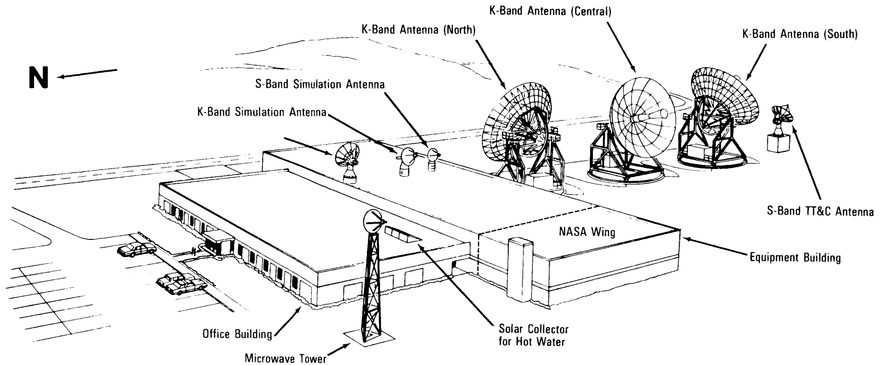
Tracking and Data Relay Satellite System Ground Station, White Sands, N.M.
