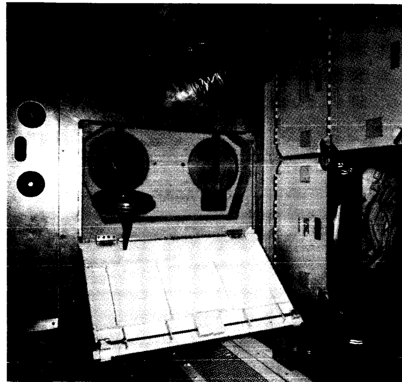
Carbon Dioxide Absorbers—Air Revitalization System
