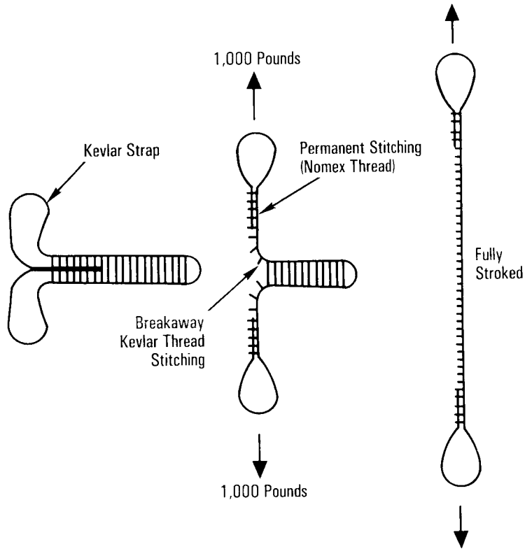
Escape Pole Magazine Assembly, Lanyard Assembly Energy Absorber
