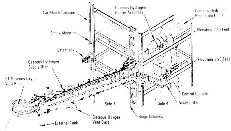
External Tank Gaseous Oxygen Vent Arm System
