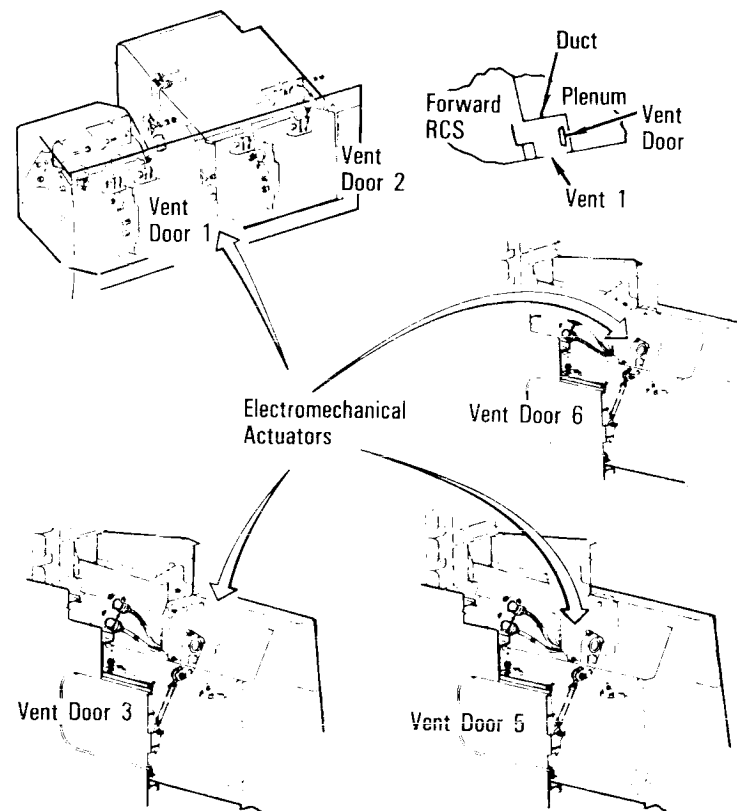
Vent Doors (1, 2, 3, 5 and 6)
