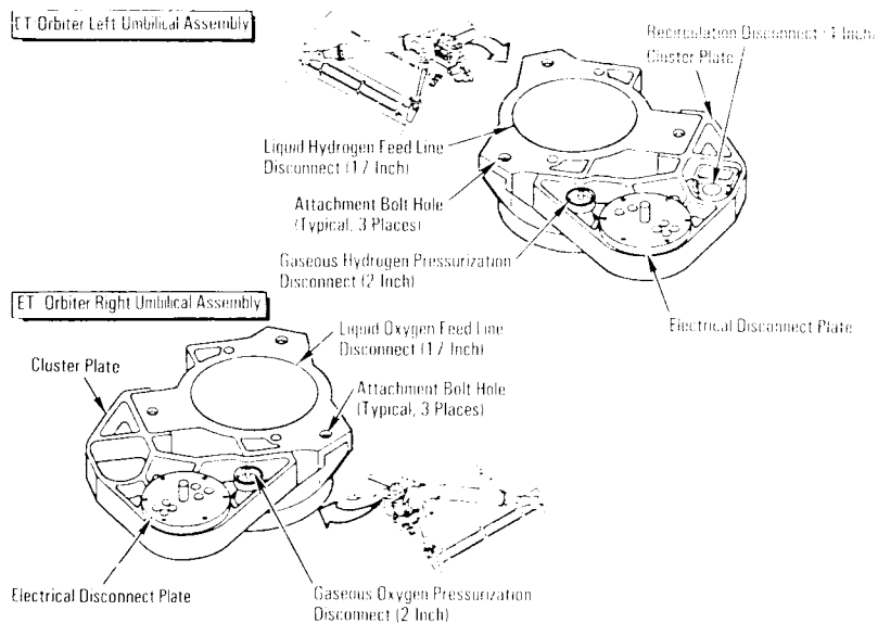
External Tank/Orbiter 17-Inch Disconnects
