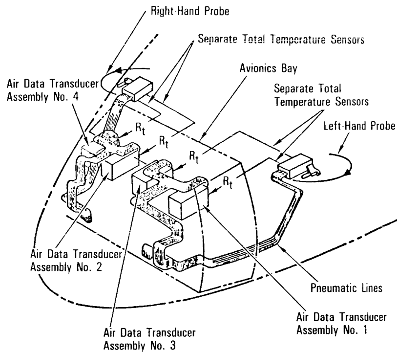
Air Data System
