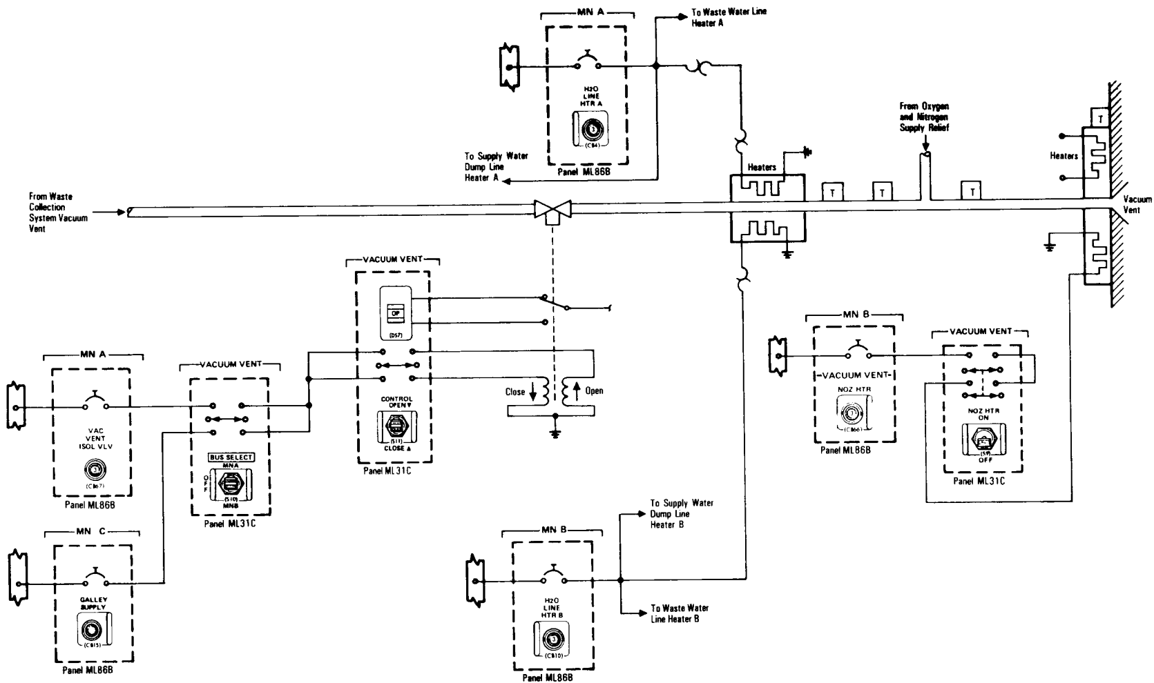
Waste Collection System Vacuum Vent Line Control Valve and Heaters
