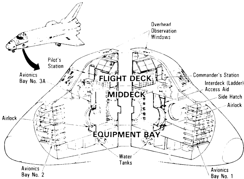
Crew Compartment and Arrangement
