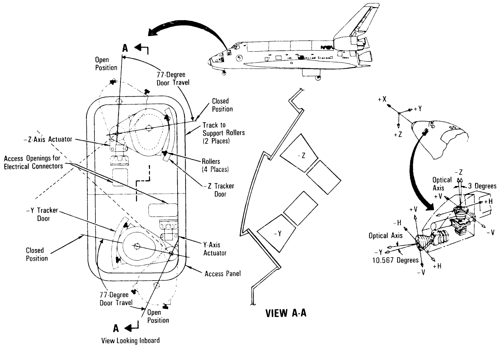
Star Trackers
