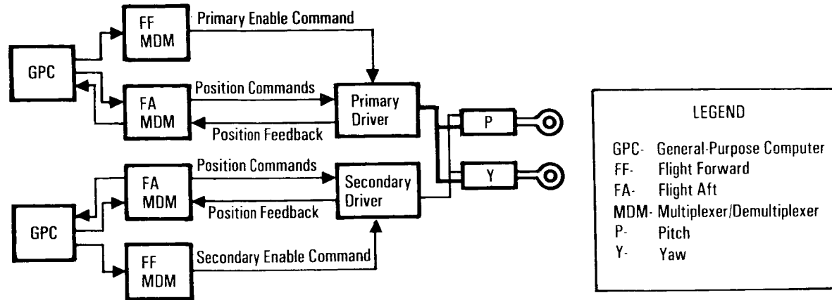
Orbital Maneuvering System Thrust Vector Control Commands and Feedback
