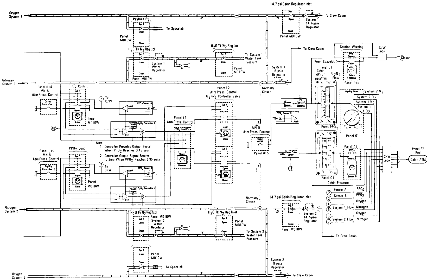
Air Revitalization System Pressurization (Sheet 3 of 3)
