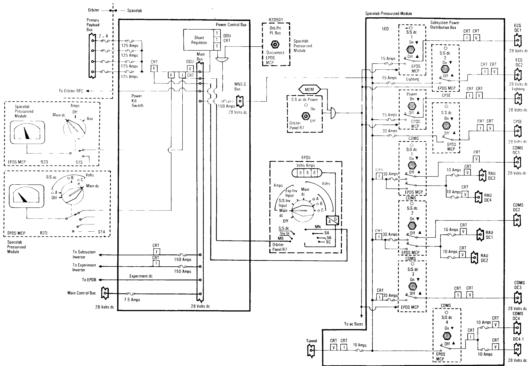
Orbiter-to-Spacelab Electrical Power Distribution—Subsystem dc Power Distribution
