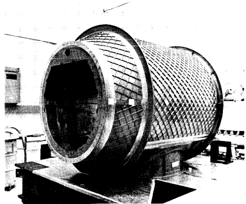
Tunnel Adapter
