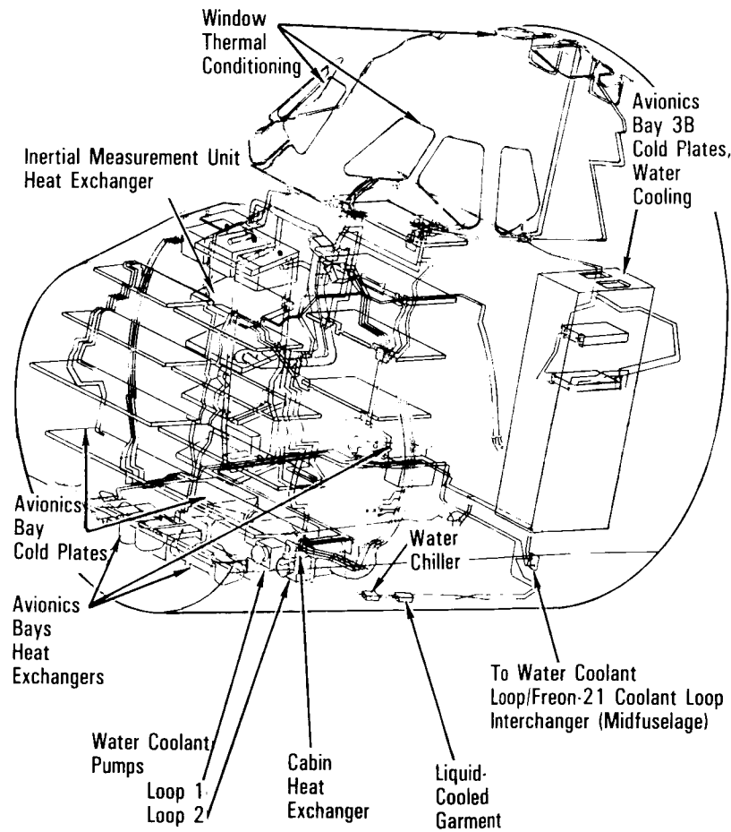
Crew Cabin Water Coolant Loops
