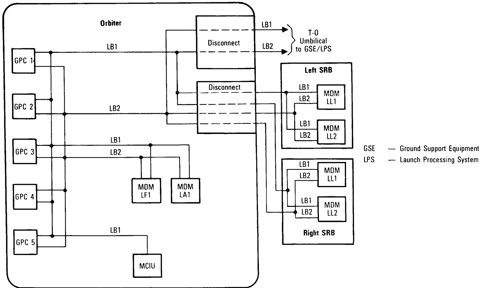
Launch/Boost Data Buses
