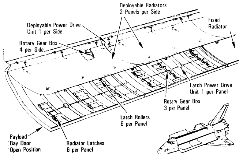
Payload Bay Door Deployable Radiator Mechanism
