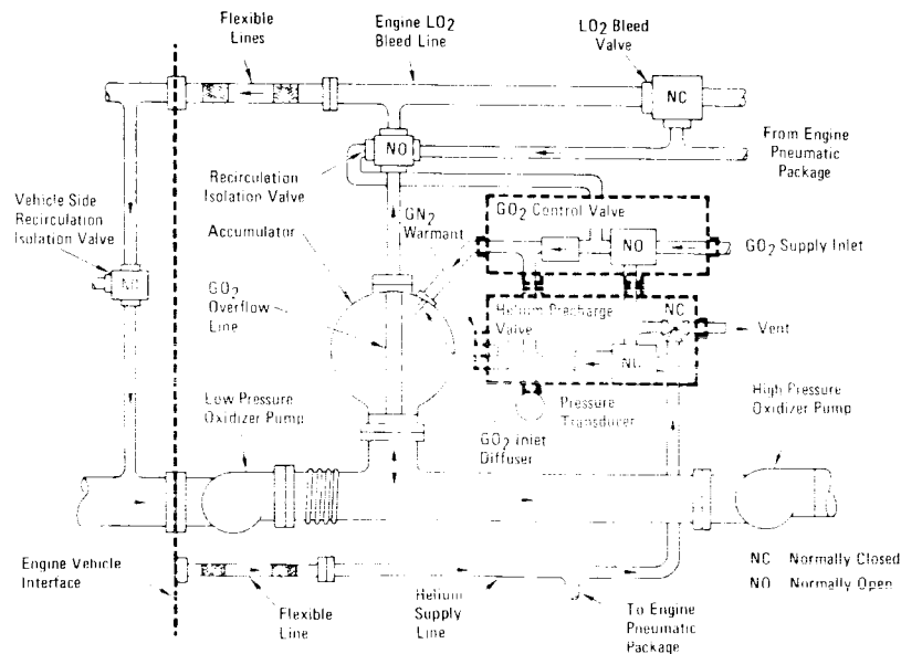
Pogo Suppression System
