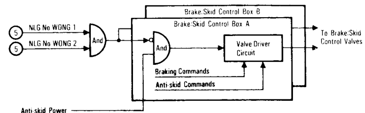
Brake/Skid Control
