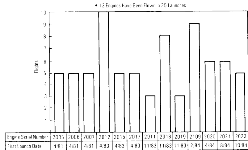
SSME Flight Experience Demonstrates Reusability (Through Feb. 1, 1986)
