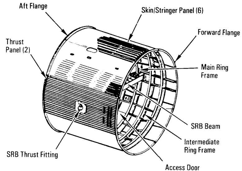
Intertank Structure
