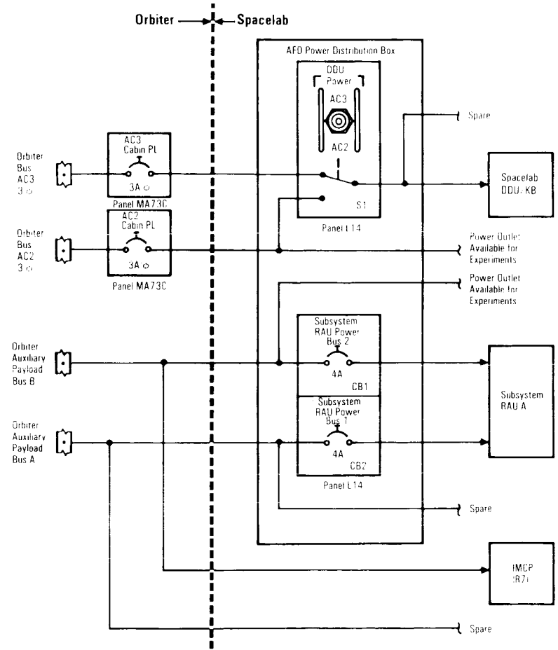
Pressurized Module Configuration—Orbiter Aft Flight Deck Power Distribution
