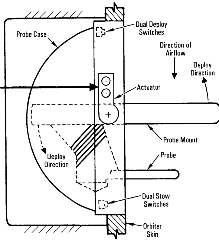
Right Air Data Probe Top View, Half Deployed
