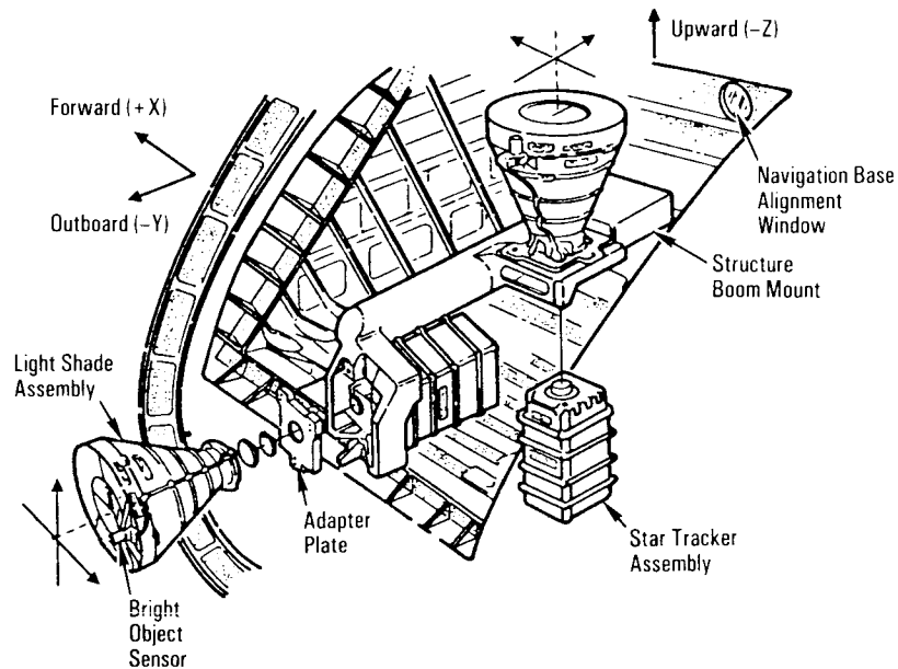
View Into Star Tracker Cavity
