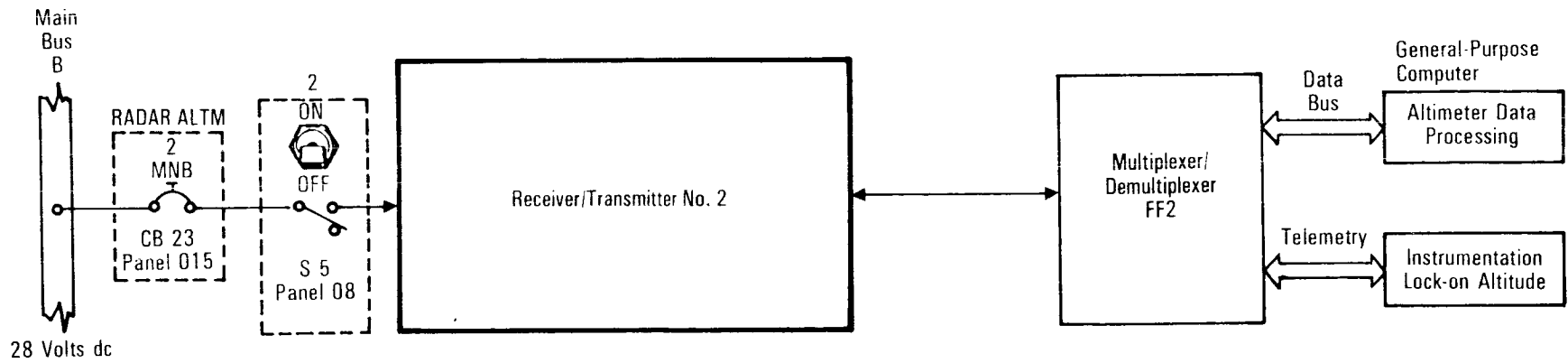
Radar Altimeter
