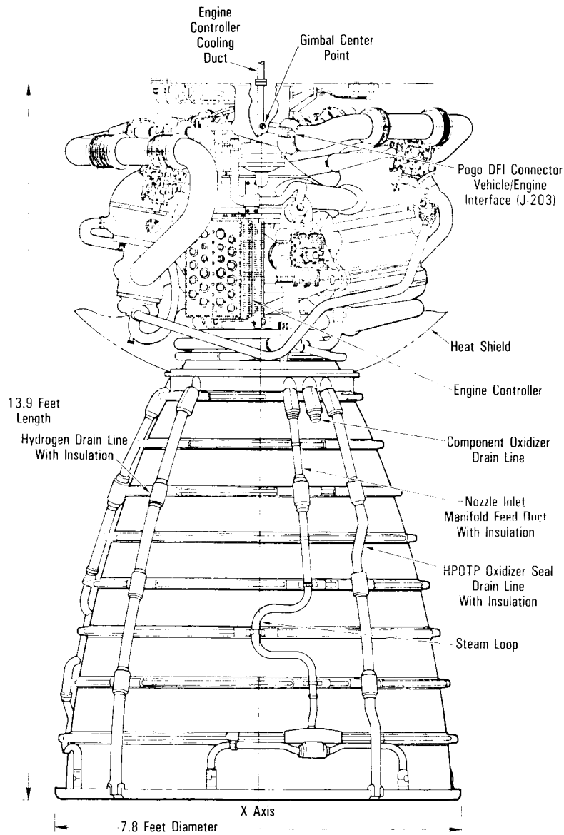
SSME Controller Side
