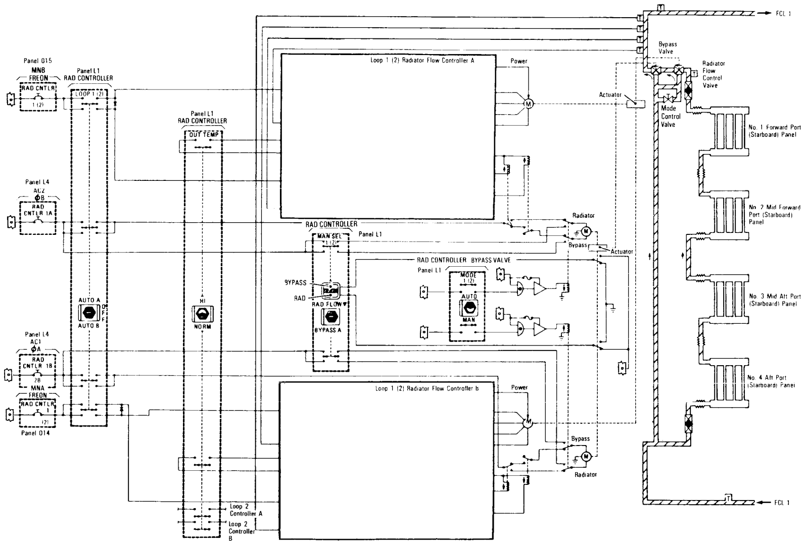
Active Thermal Control Freon-21 Coolant Loop (Sheet 1 of 3)
