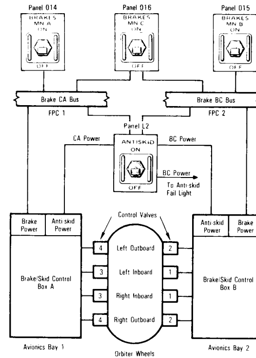
Brake/Skid Control Power
