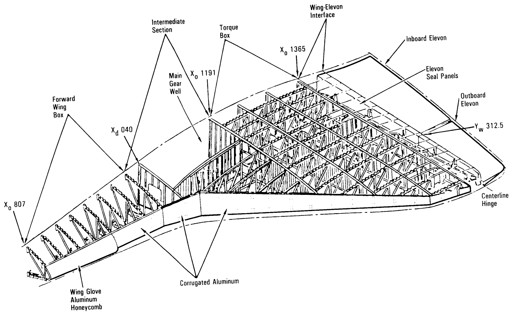
Wing Configuration
