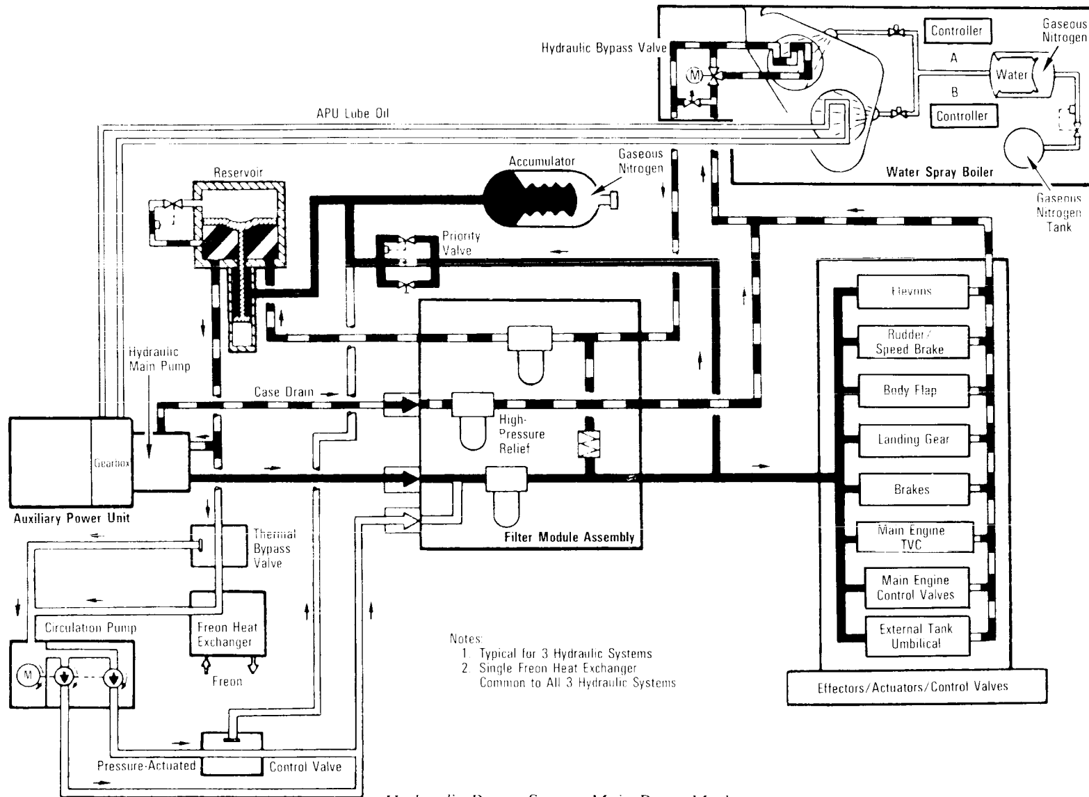
Hydraulic Power System Main Pump Mode
