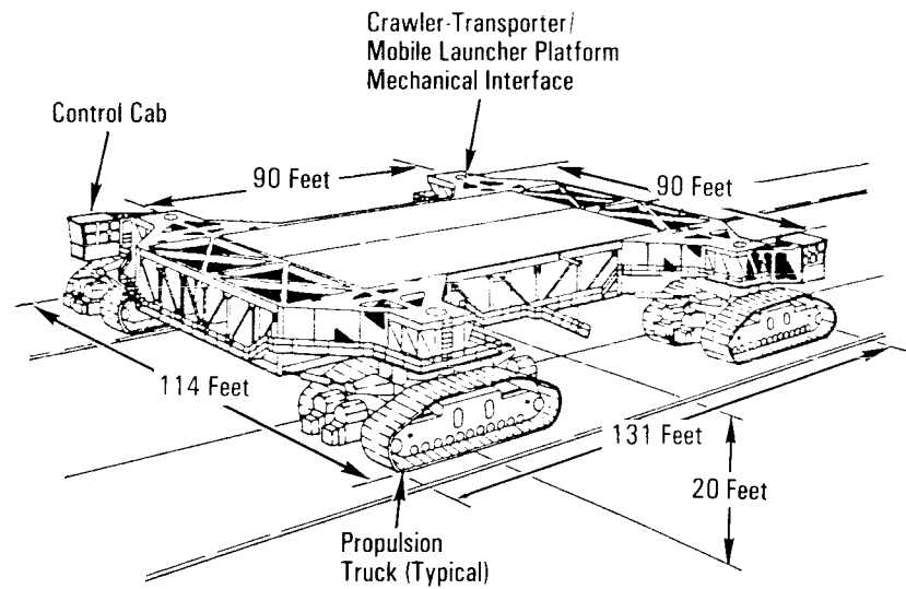
Crawler-Transporter
