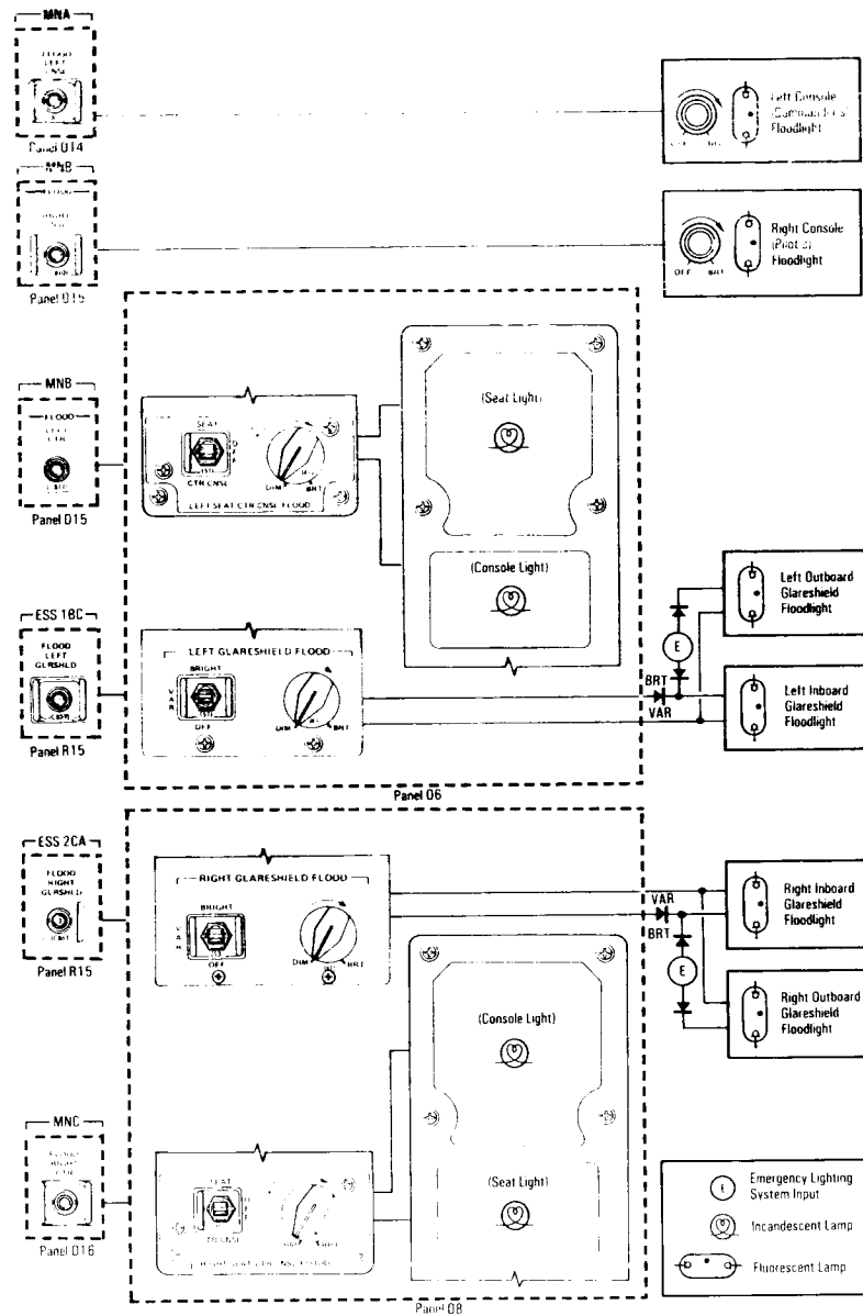
Forward Flight Deck Floodlight Control
