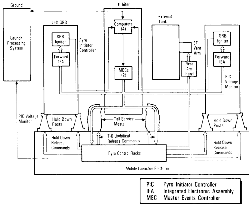
Solid Rocket Ignition, Hold-Down Release and Umbilical Retract Commands
