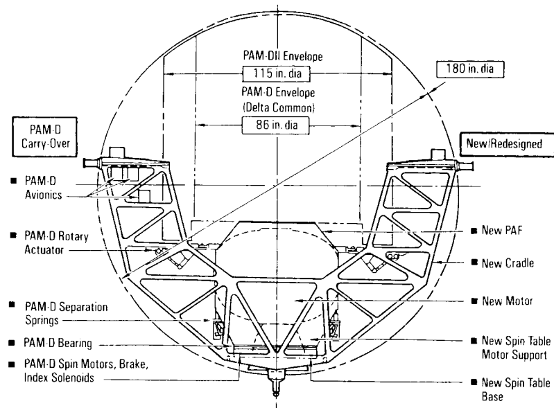
PAM-DII Flight System Hardware Derivation
