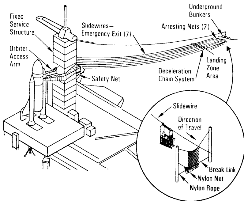
Launch Pad Emergency Exit System
