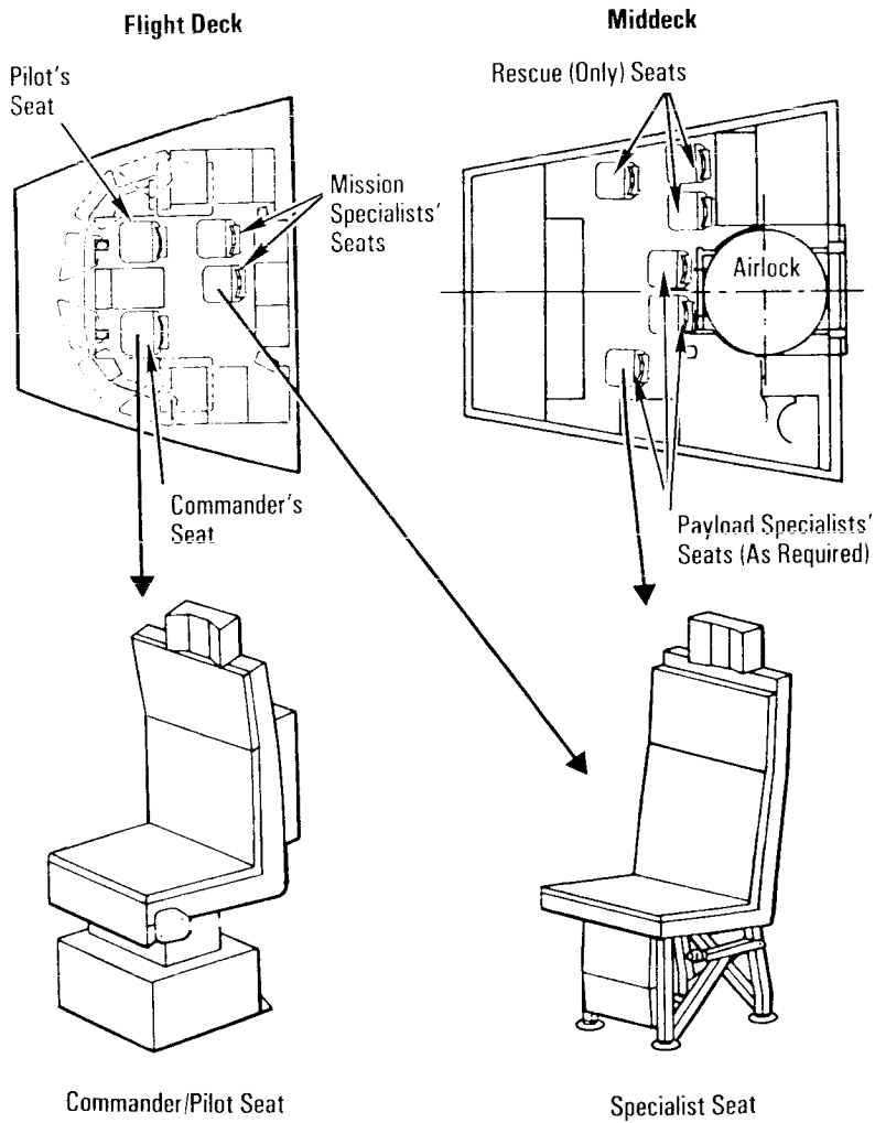
Crew Seats
