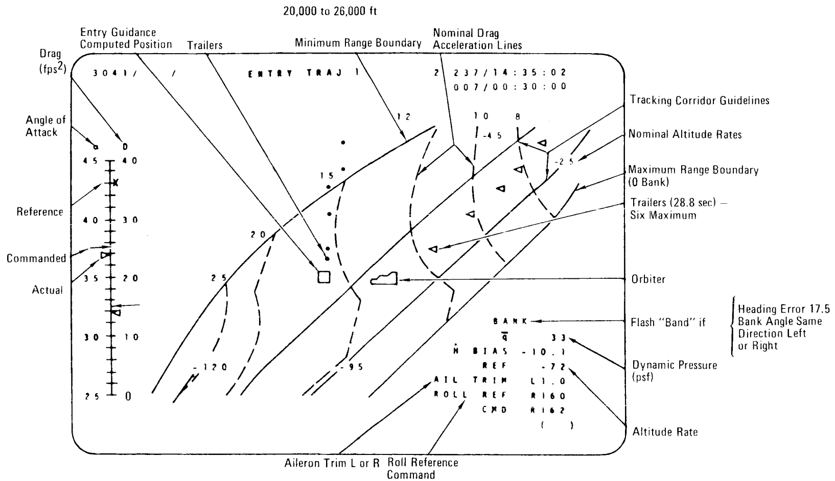
Entry Trajectory
