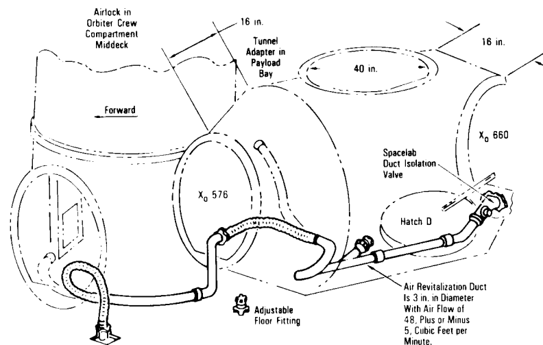
Environmental Control and Life Support System Air Circulation Duct Routing
