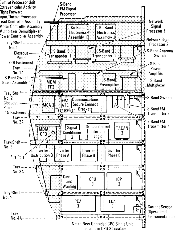
Component Locations—Bay 3A
