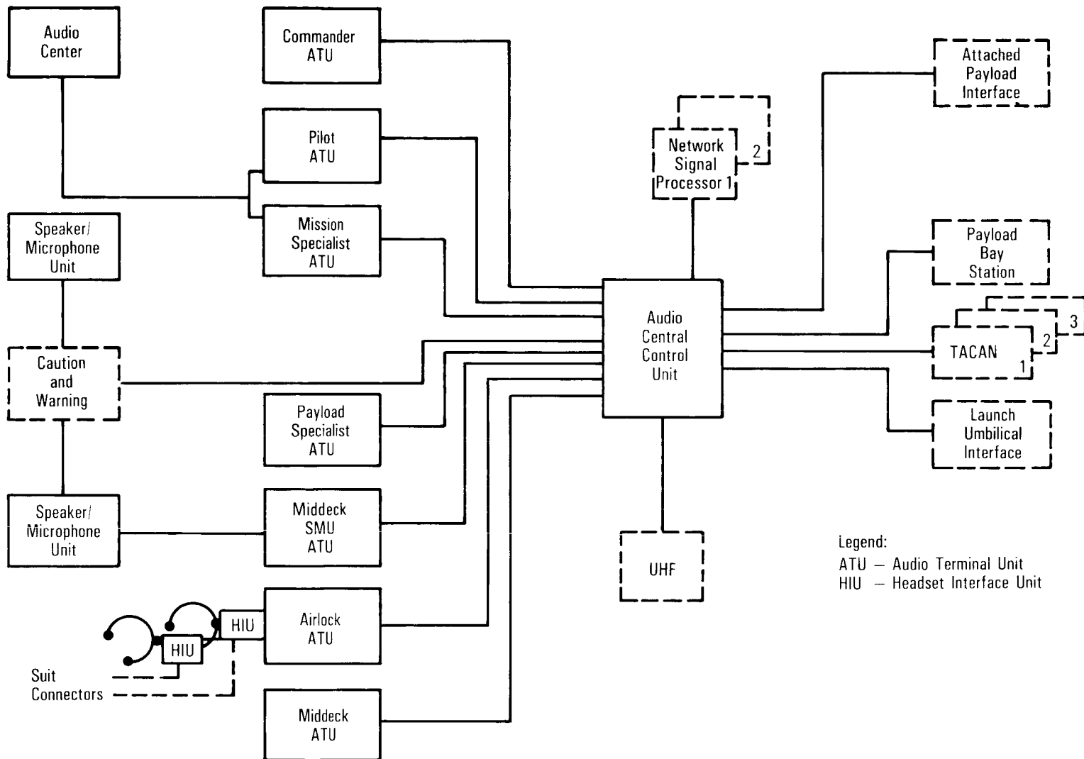
Audio Distribution System
