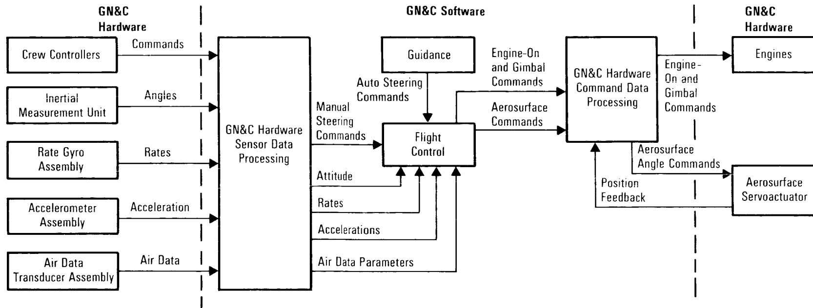
Flight Control Interfaces
