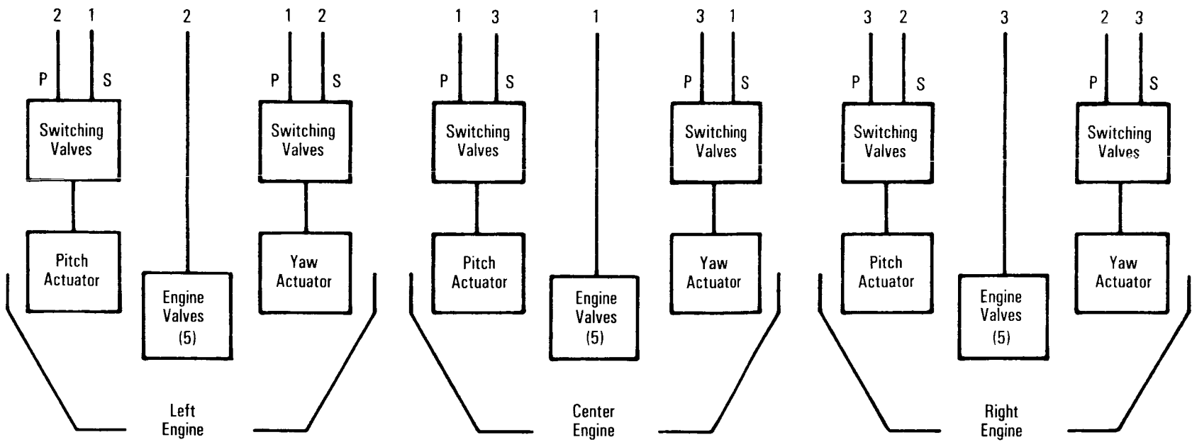
MPS Hydraulic System Distribution
