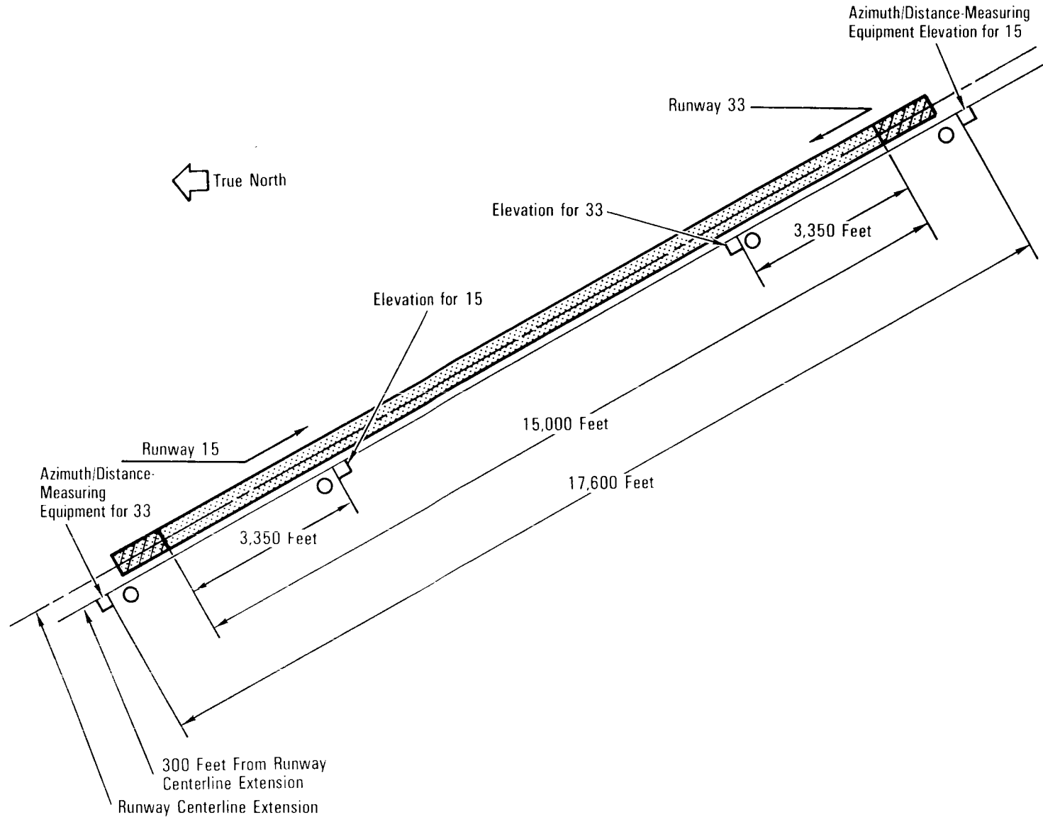
Microwave Scan Beam Landing System Locations at the Kennedy Space Center Runway
