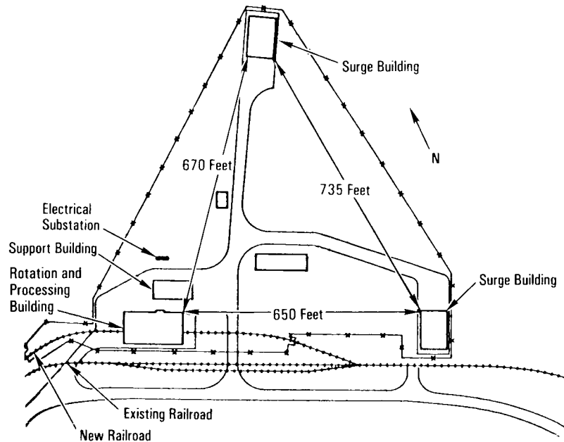
Solid Rocket Motor Rotation, Processing and Surge Facility
