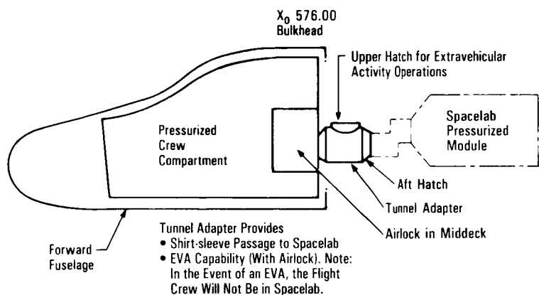
Airlock/Tunnel Adapter
