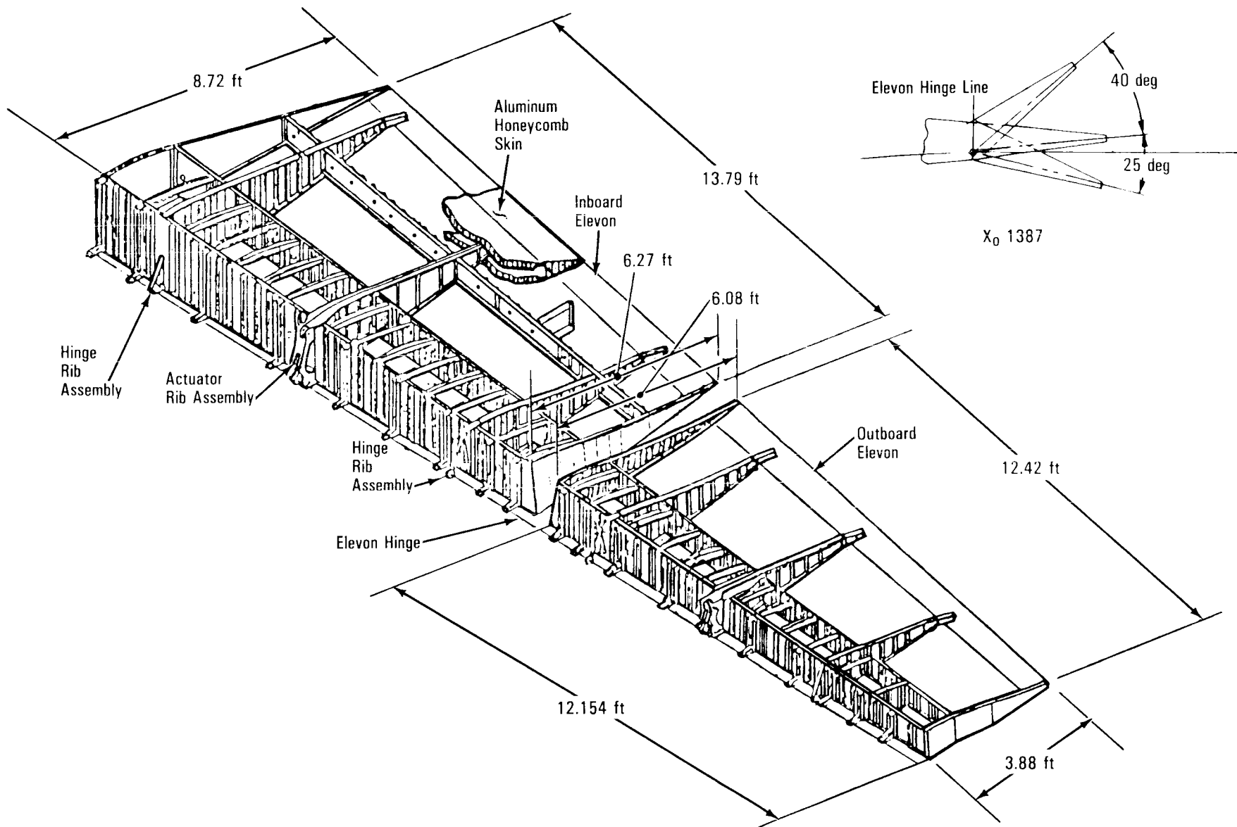
Elevon Construction
