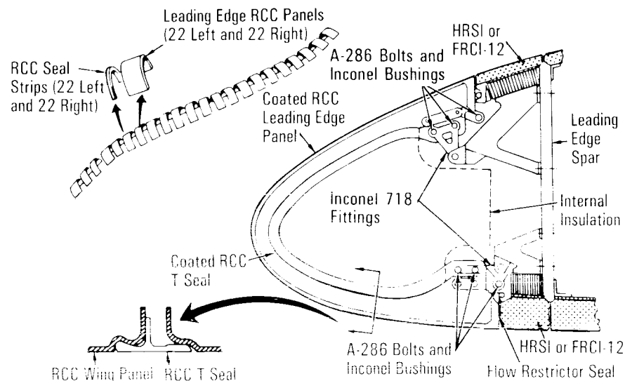
RCC Wing Leading Edge
