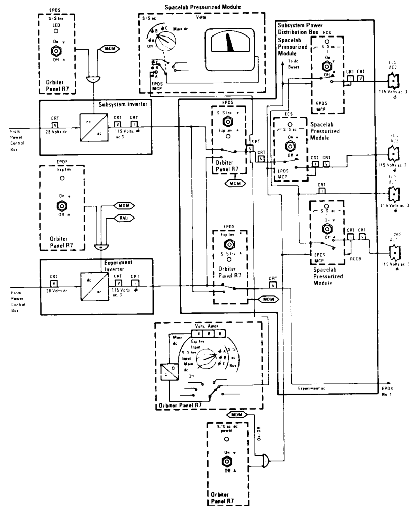
Spacelab Electric Power Distribution—Subsystem ac Power Distribution
