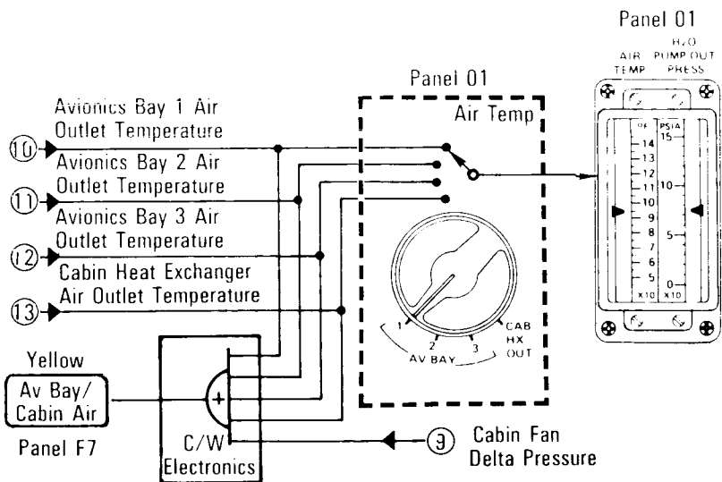
Avionics Bay and Cabin Heat Exchanger Temperature Monitoring and Caution/Warning, Crew Cabin Air
