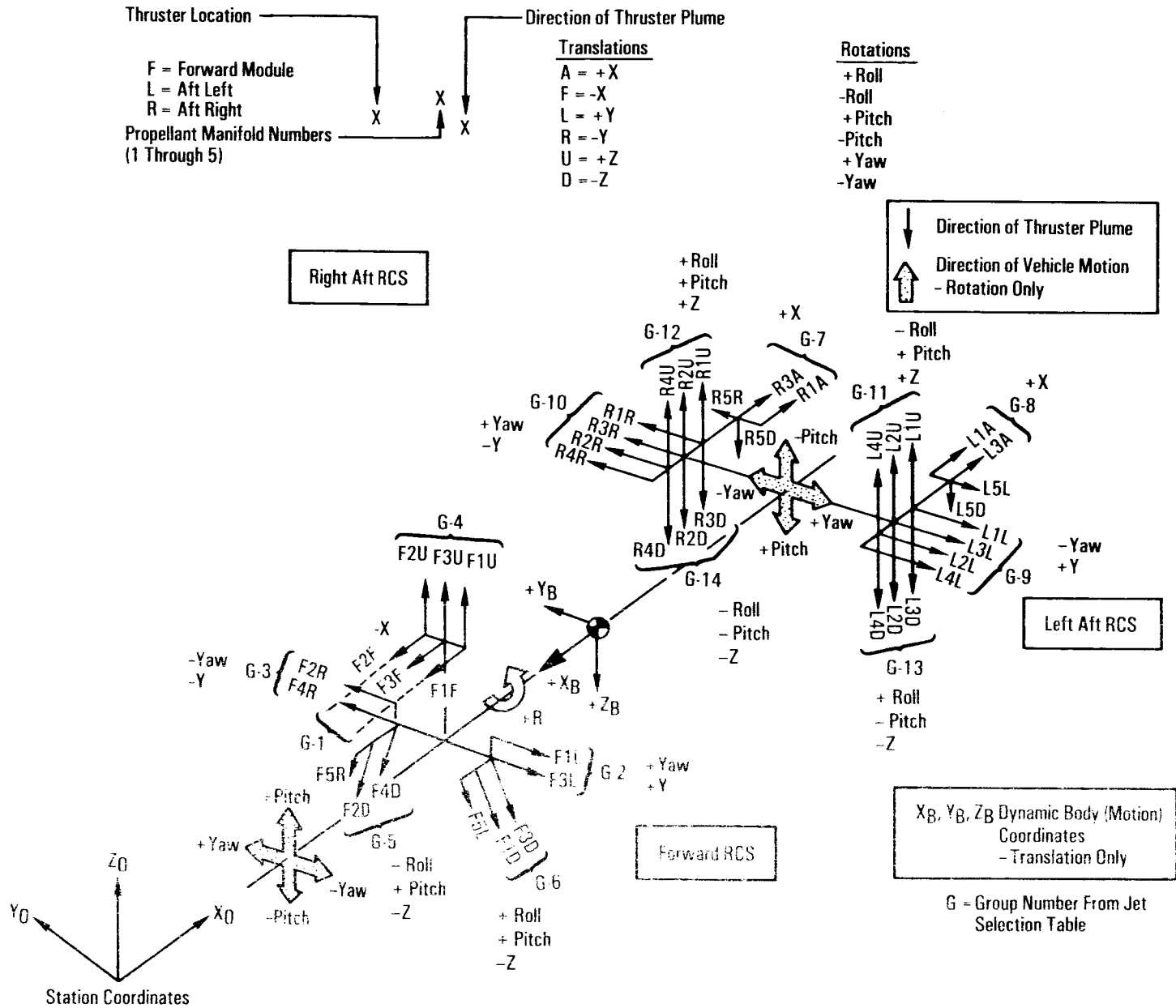
Reaction Control System Engine Identification and Direction of Vehicle Motion
