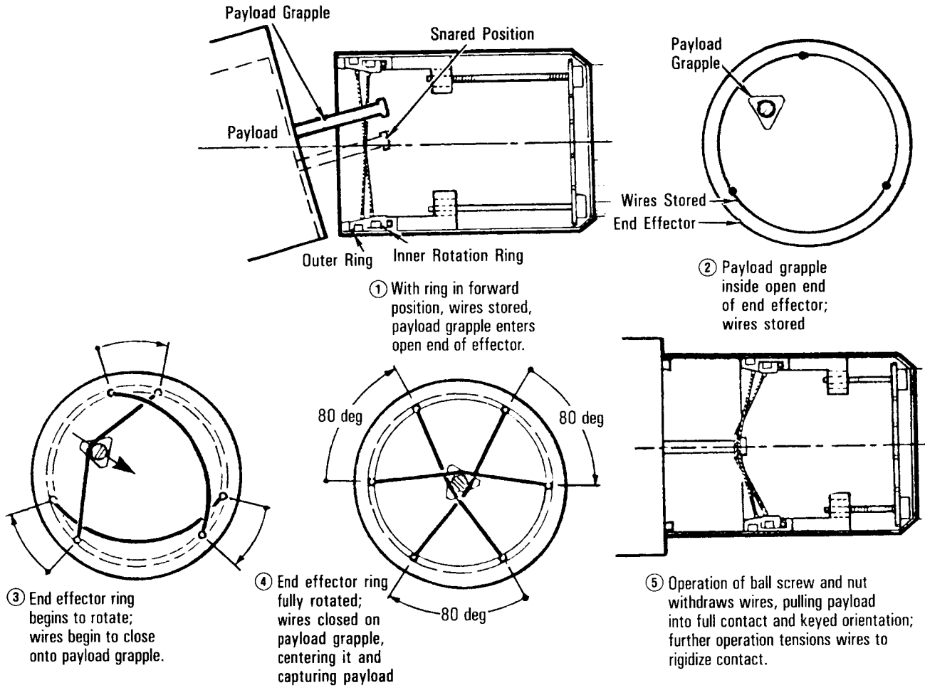
Snare Capture and Rigidization Sequence
