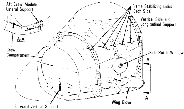
Crew Compartment—Forward Fuselage Interface
