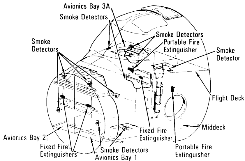
Smoke Detection and Fire Suppression System
