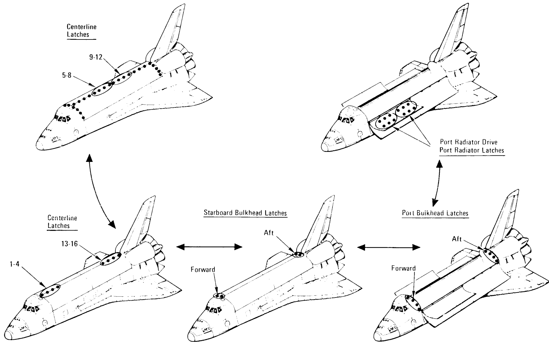
Payload Bay Door and Radiator Latches
