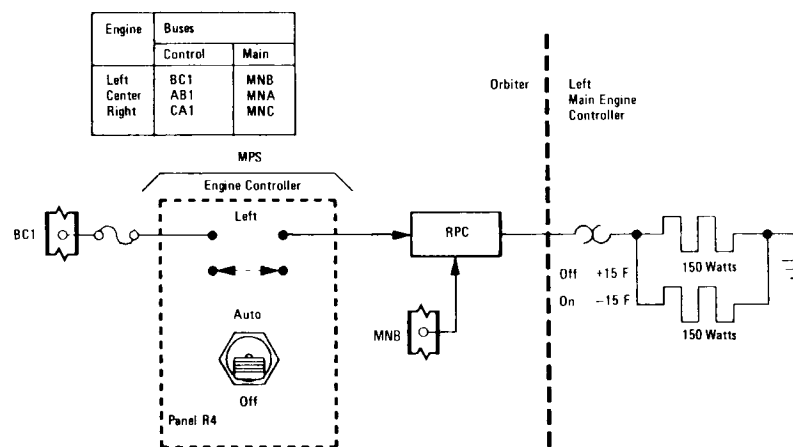
Main Engine Controller Heater Power
