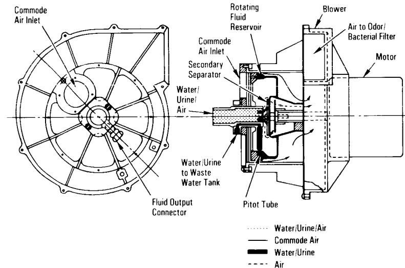
Waste Collection System Fan Separator
