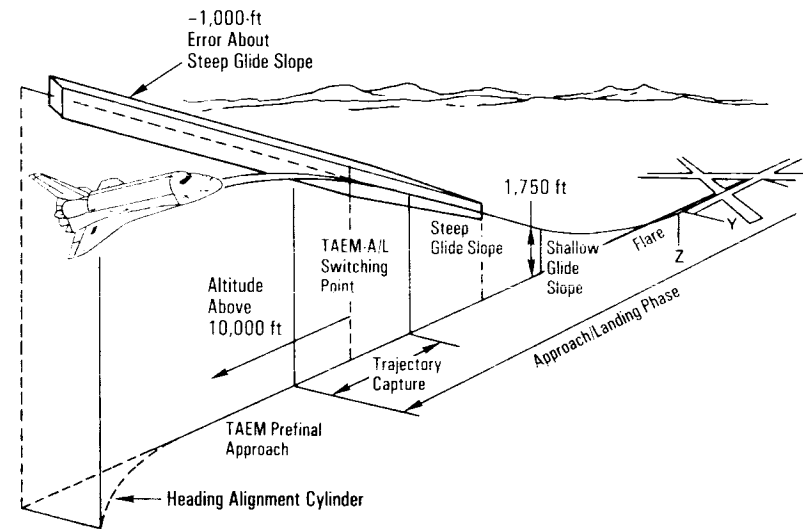
Approach and Landing Guidance Subphases
