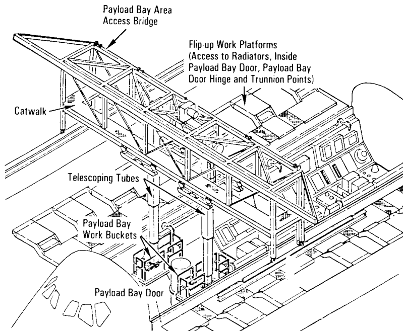
Orbiter Processing Facility Access Platforms, Overhead View
