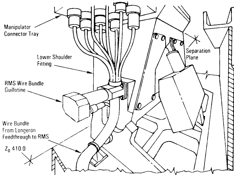
The RMS Shoulder Wire Bundles
