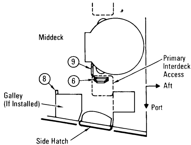
Primary Interdeck Area (Port Side Looking Inboard)
