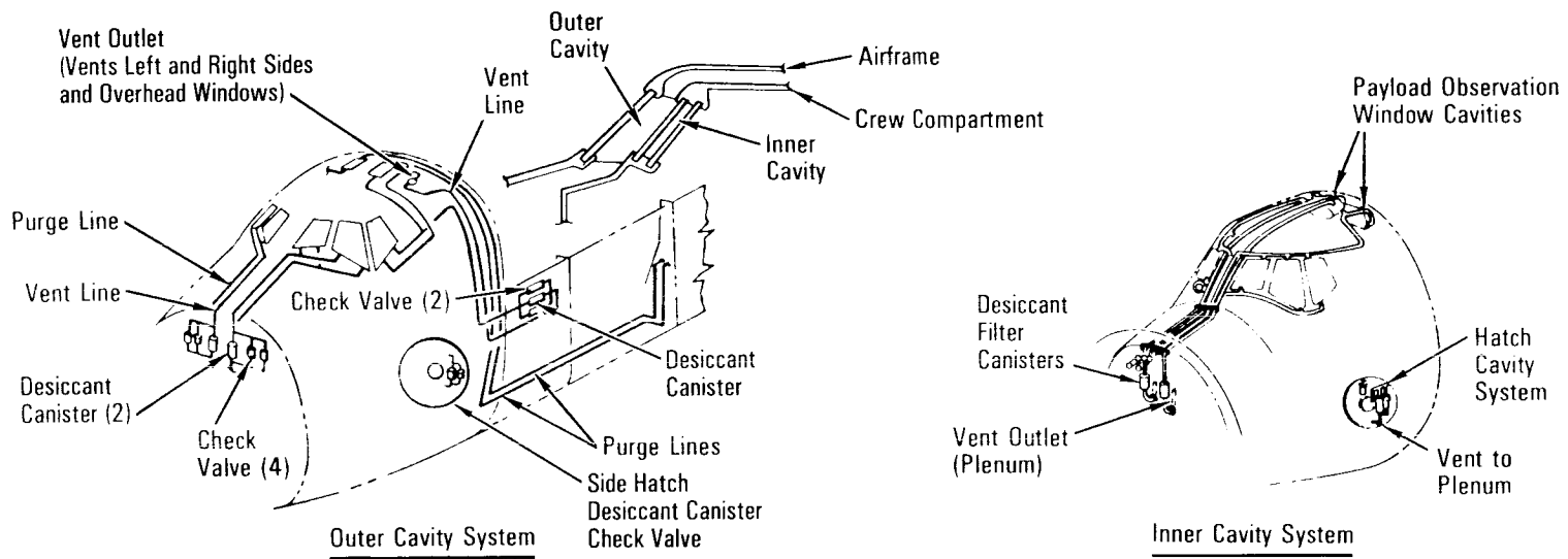
Window Cavity Conditioning System
