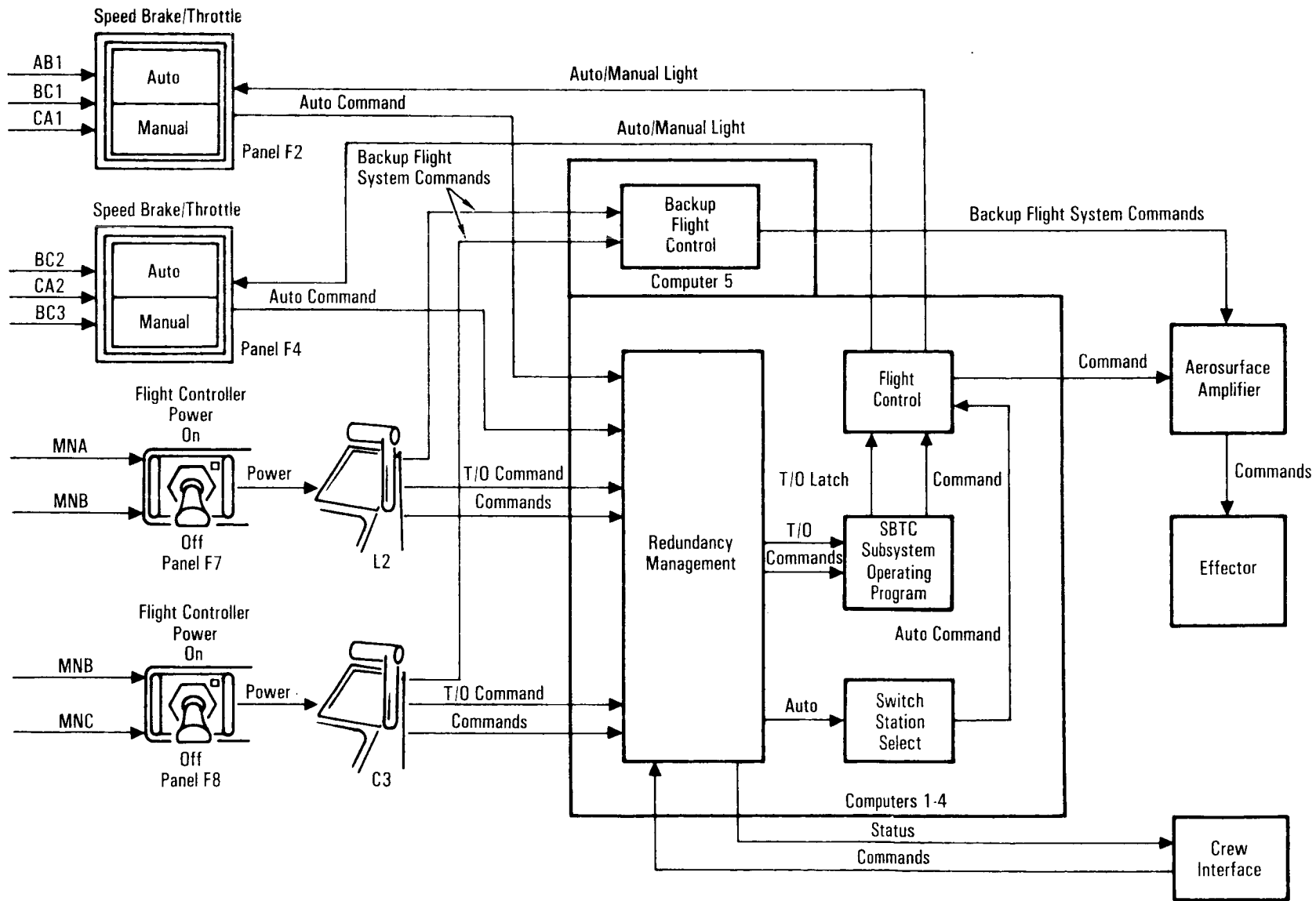
Speed Brake/Thrust Controller
