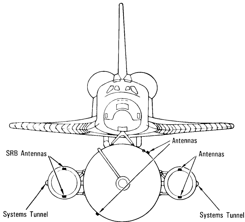
External Tank Range Safety System Antennas
