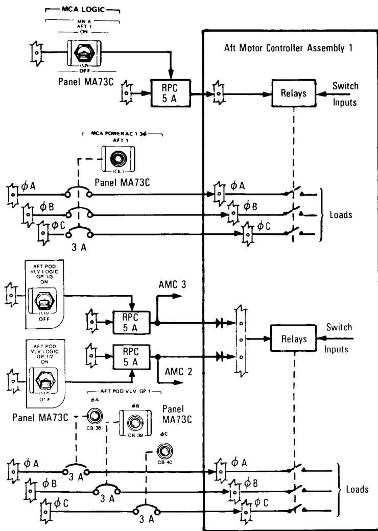
Aft Motor Controller Assembly
