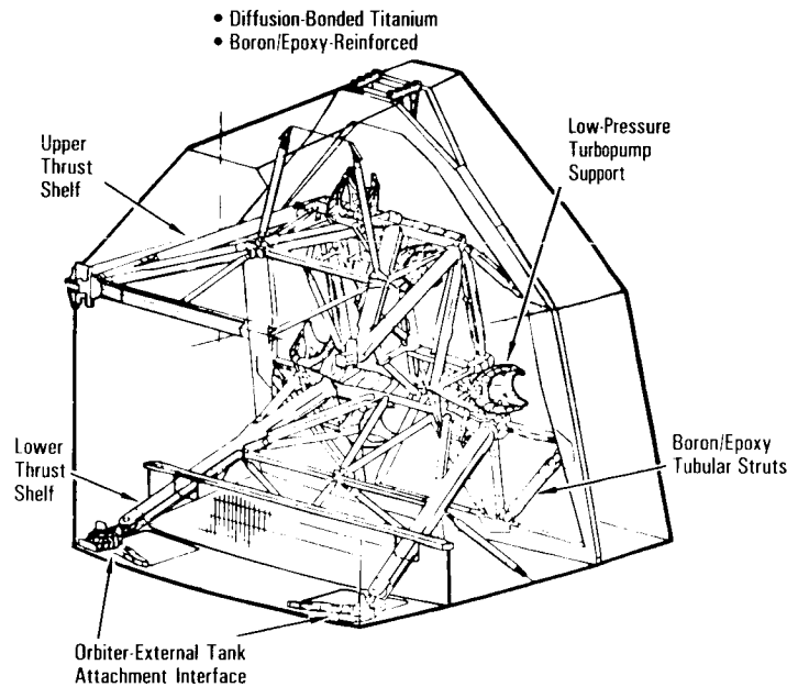
Aft Fuselage Internal Structure
