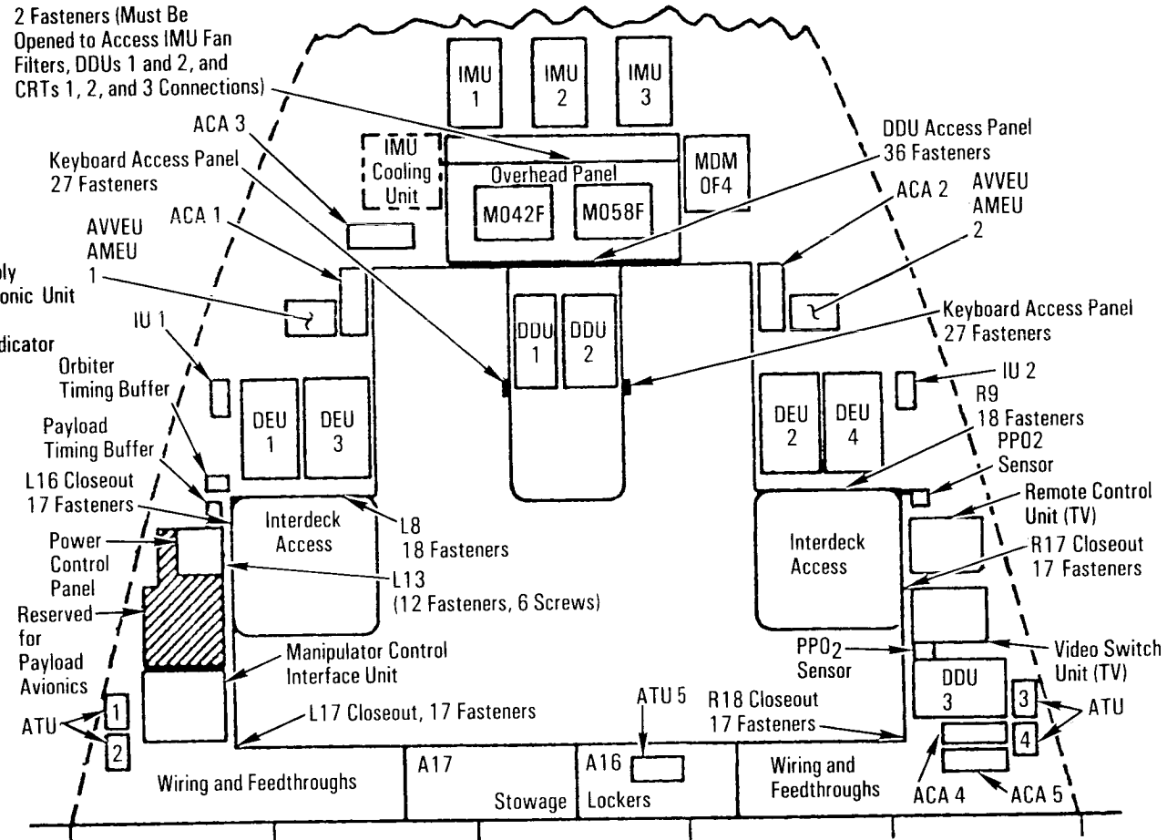
Component Locations—Flight Deck
