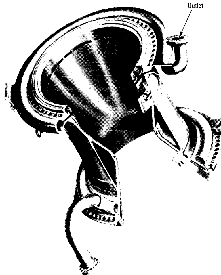
Main Combustion Chamber
