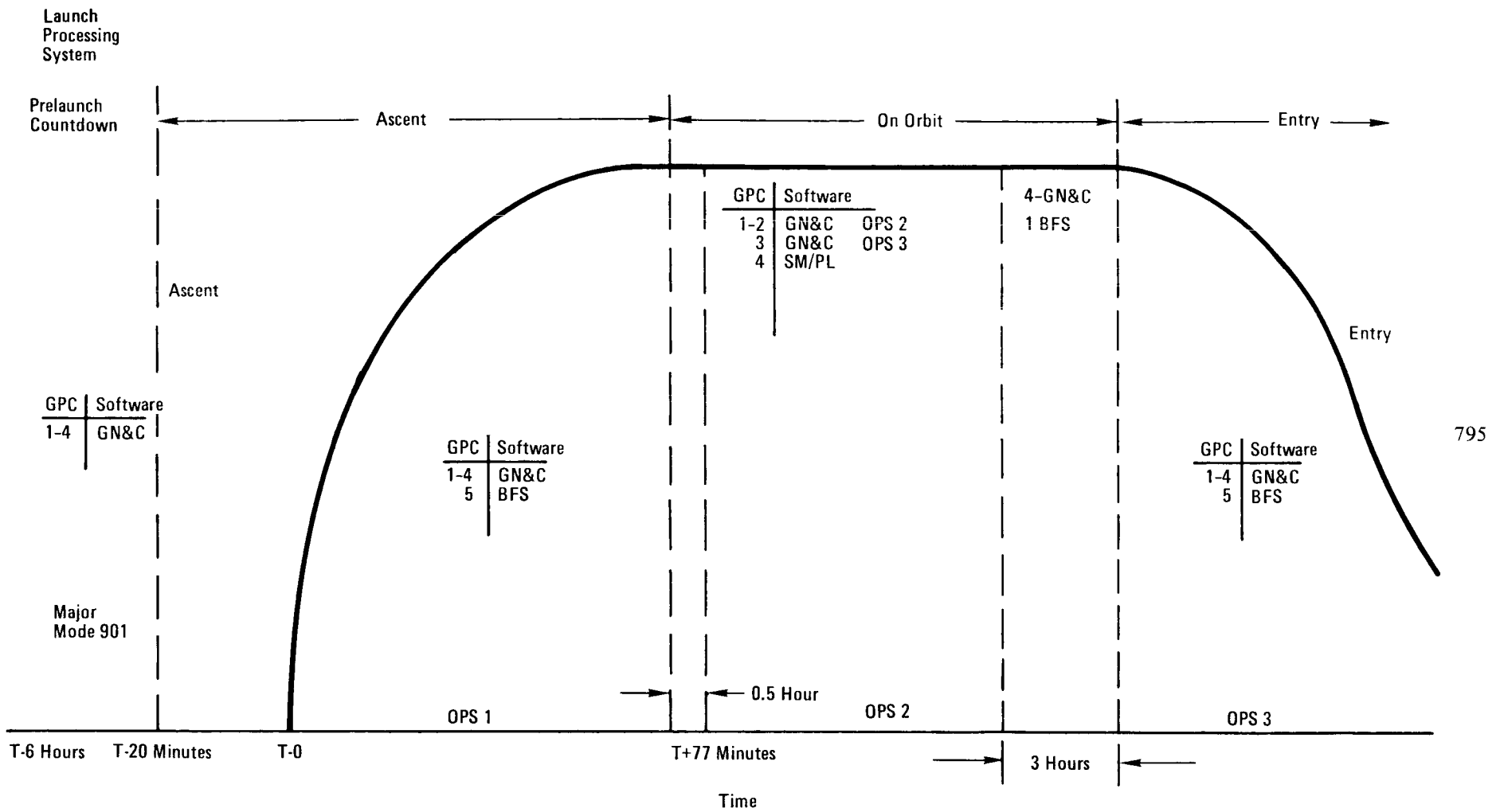
Orbiter Computer Configuration for Nominal Mission Scenario
