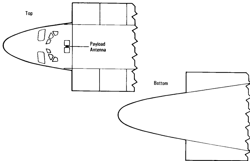
Payload Communication System Antenna Location
