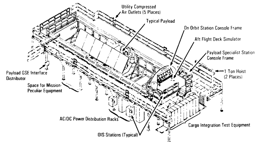
Horizontal Cargo Integration Test Equipment Stand in O&C Building
