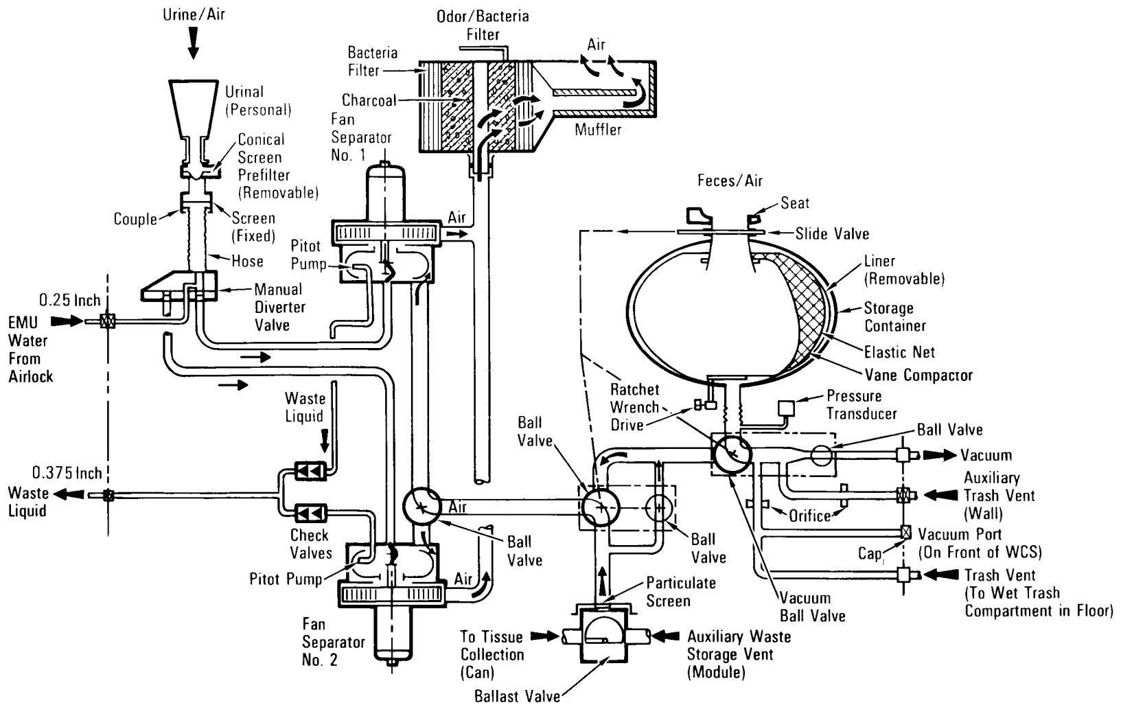
Waste Collection System
