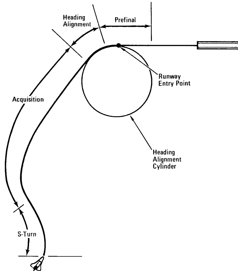
Straight-in Approach
