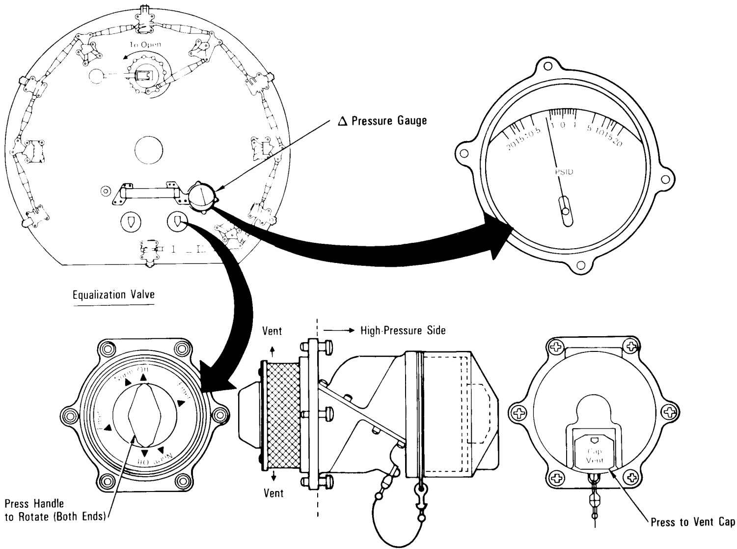
Airlock Repressurization
