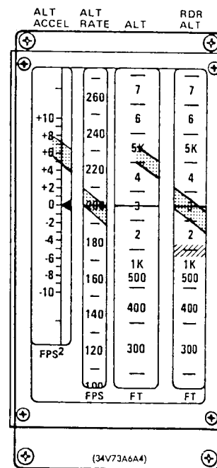
Altitude / Vertical Velocity Indicator
