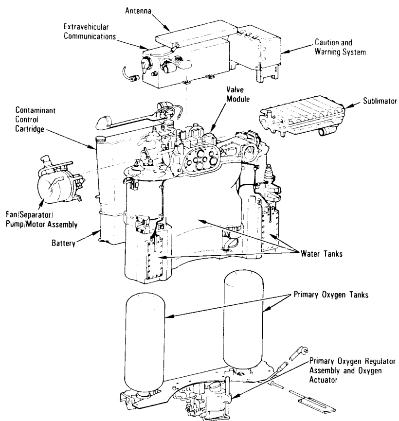
Portable Life Support System
