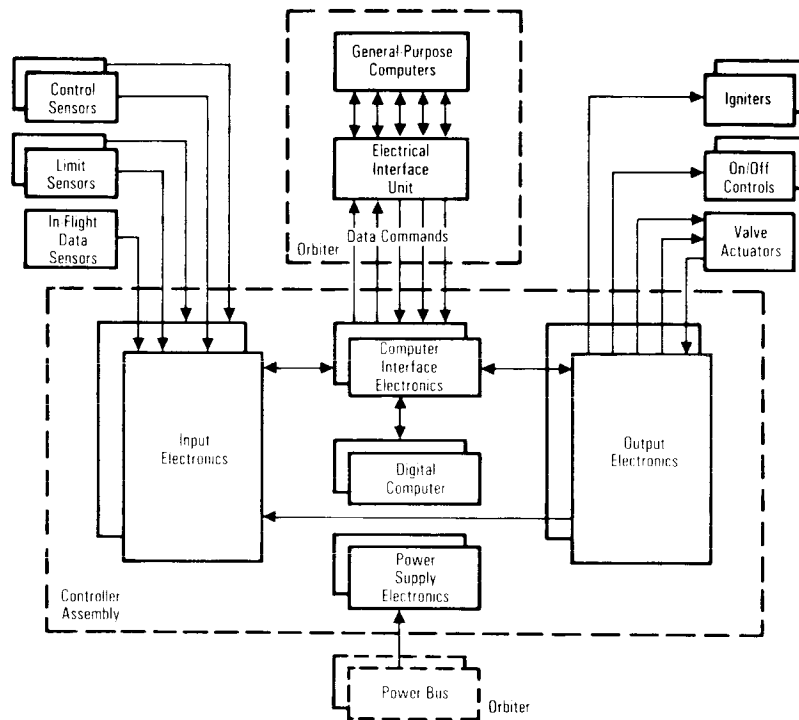
Controller Organization and Redundancy
