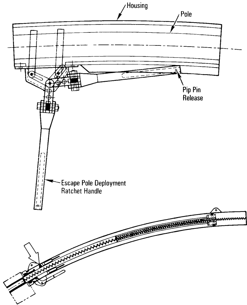
Escape Pole Stowed
