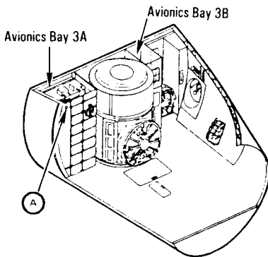
Avionics Bays 3A and 3B (Looking Aft)
