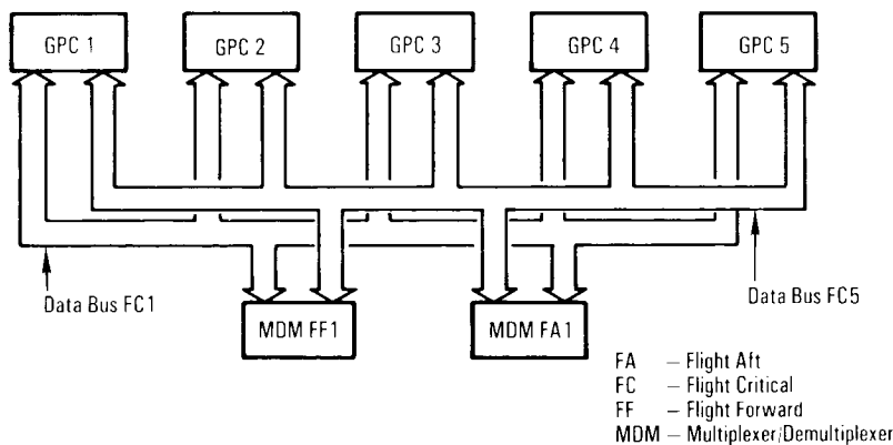
General-Purpose Computer String
