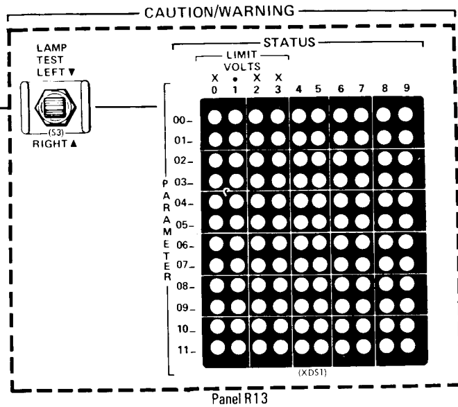
Aft Flight Deck Annunciator Light Control
