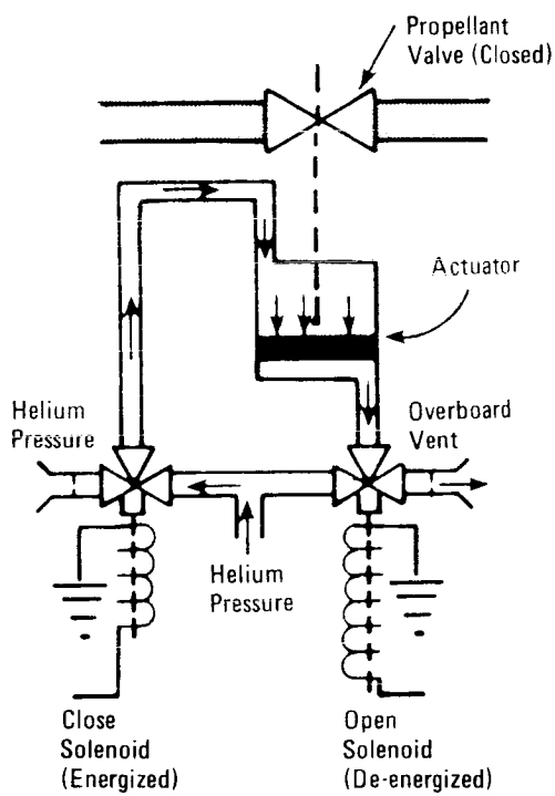
② Control Switch in Closed Position
