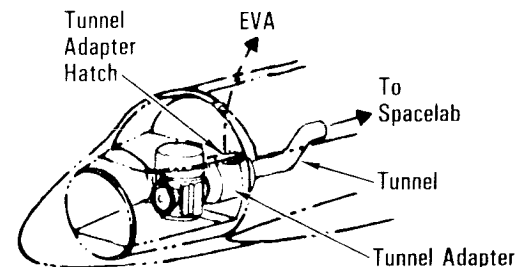
AIRLOCK IN CREW MODULE WITH TUNNEL ADAPTER
