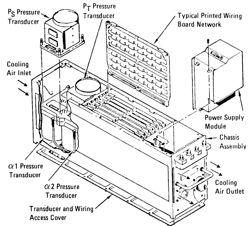
Air Data Transducer Assembly
