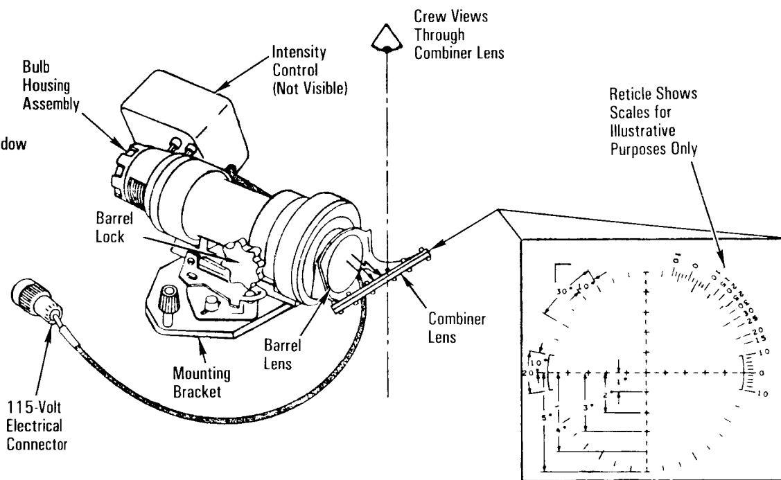
Reticle Pattern
