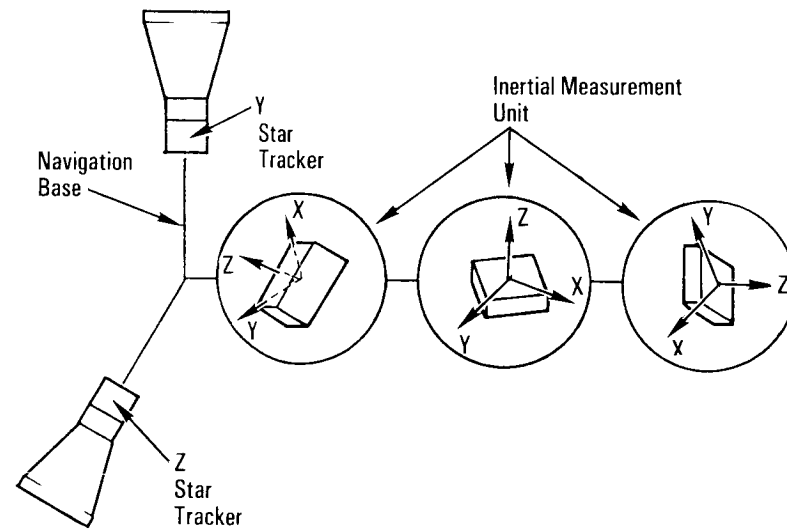
Inertial Measurement Unit Skew
