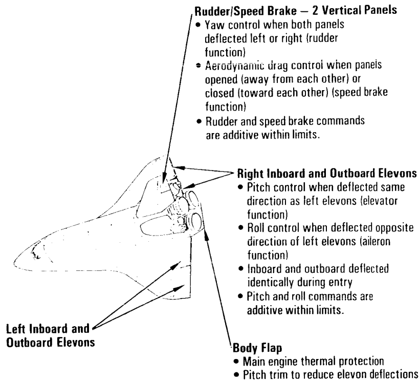
Aerodynamic Surfaces and Associated Control Axes
