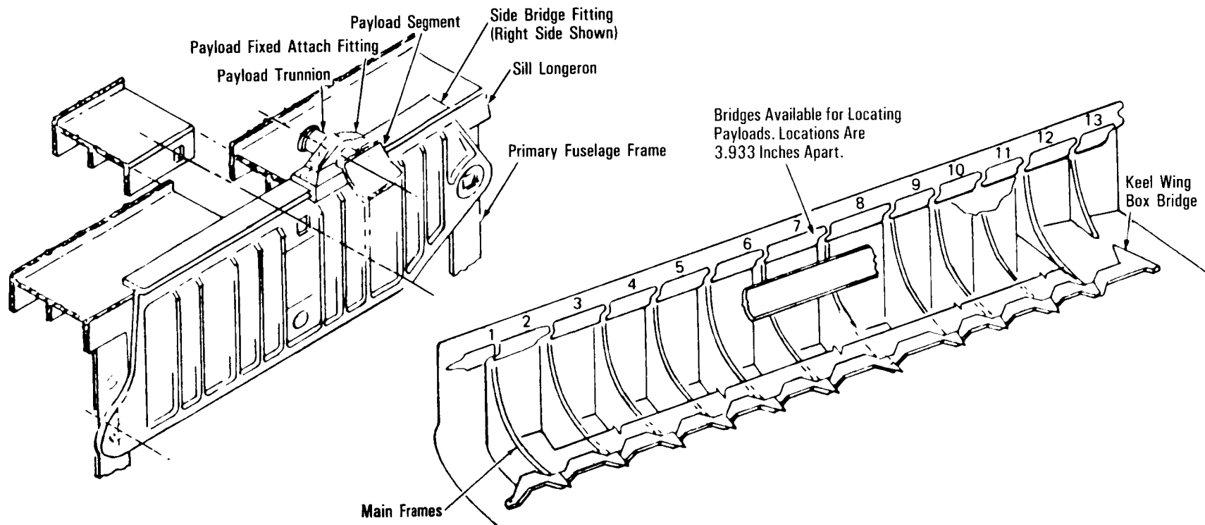
Payload Retention
