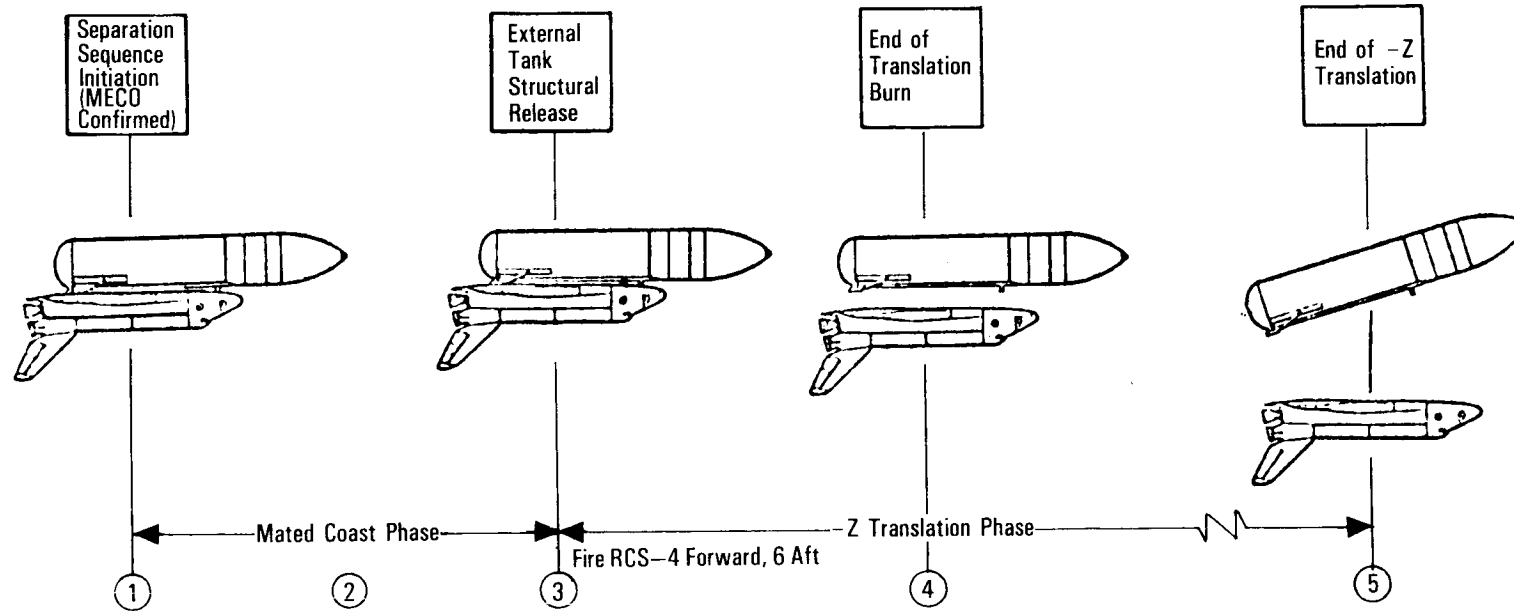
External Tank Separation
