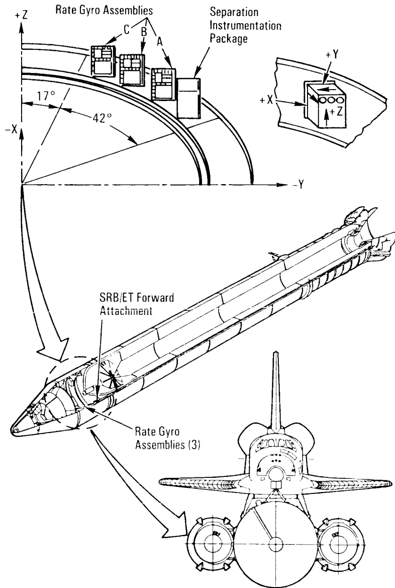
Solid Rocket Booster Rate Gyro Locations
