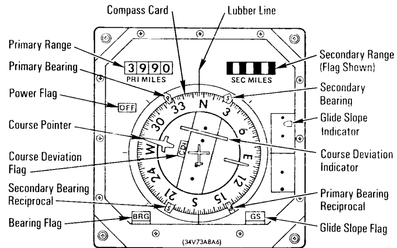
Horizontal Situation Indicator Display
