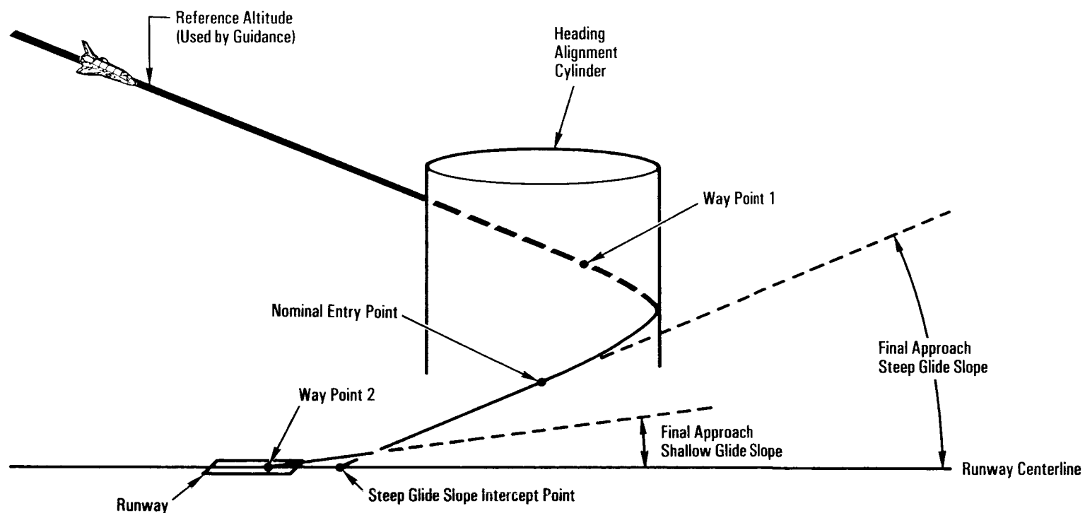
Flight Path Geometry — Side View
