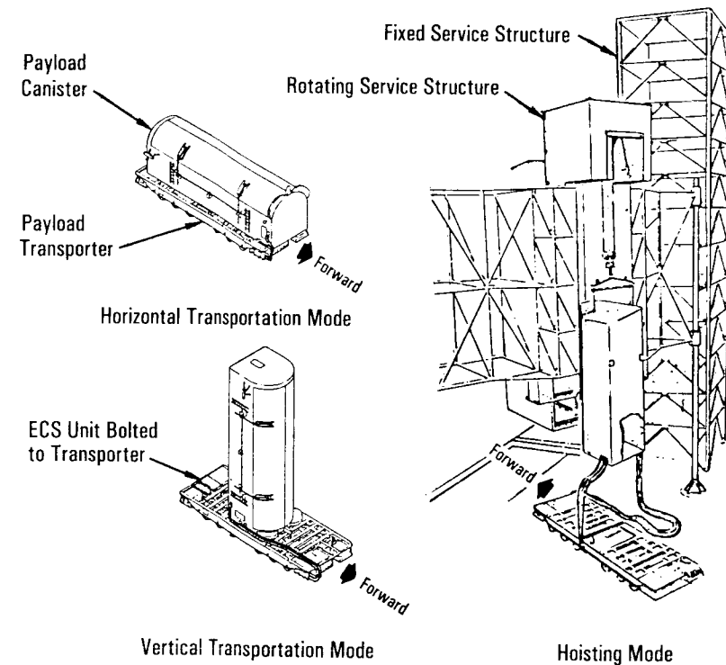
Canister Transporter Operations
