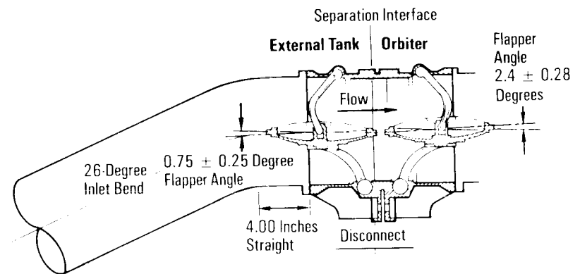
Orbiter / External Tank Liquid Hydrogen 17-Inch Disconnect Without Latch Feature
