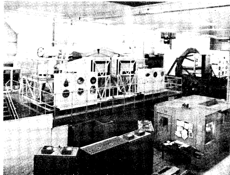
Motion Base Shuttle Mission Simulator
