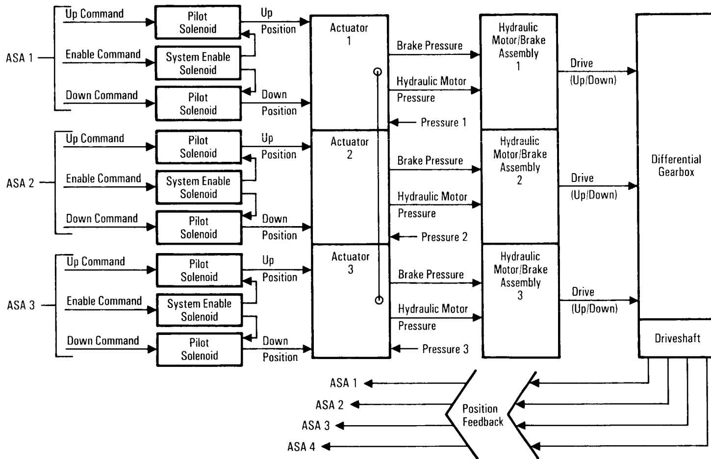
Body Flap Power Drive Unit
