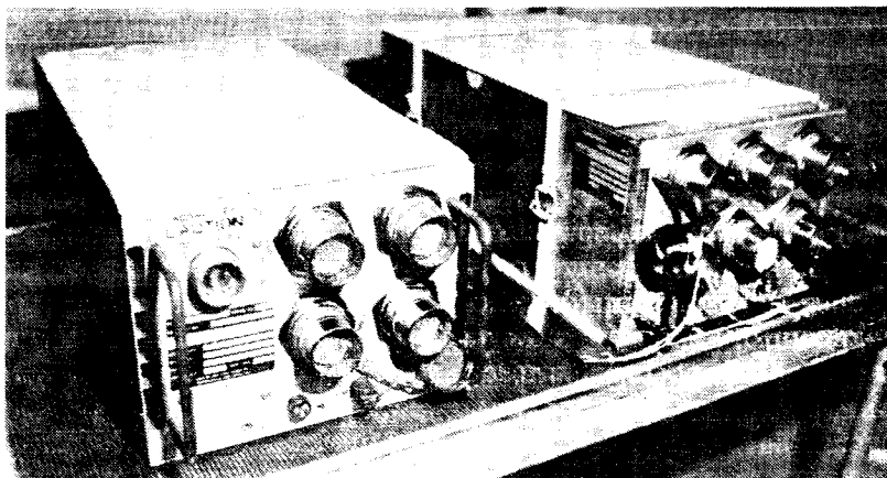
AP-101B General-Purpose Computer (IOP and CPU)
