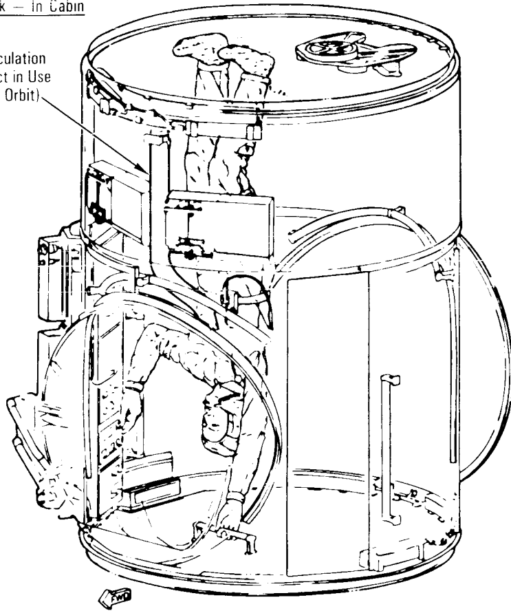
Airlock With Tunnel Adapter for Spacelab
