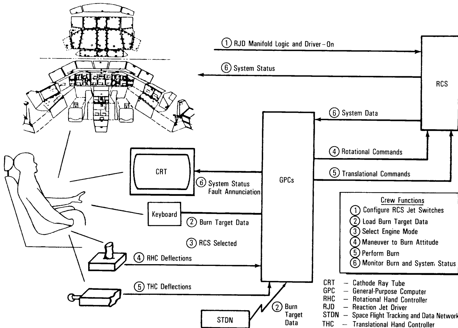
Reaction Control System
