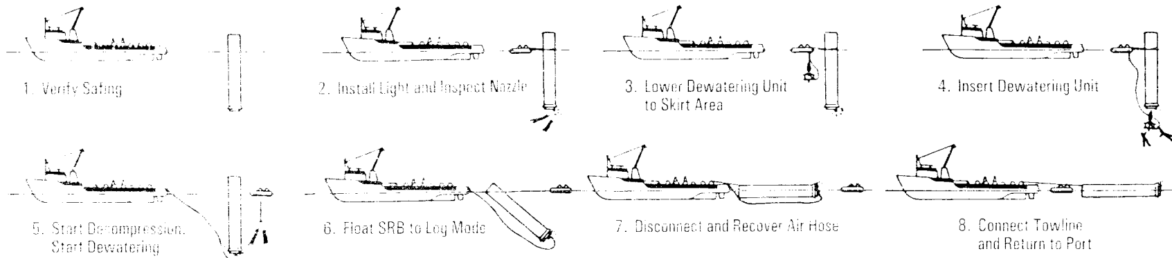
Solid Rocket Booster Recovery Procedure
