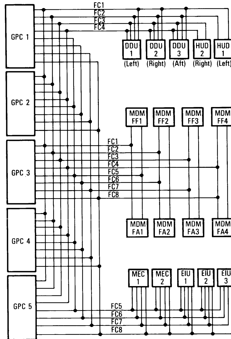
Flight-Critical Data Buses
