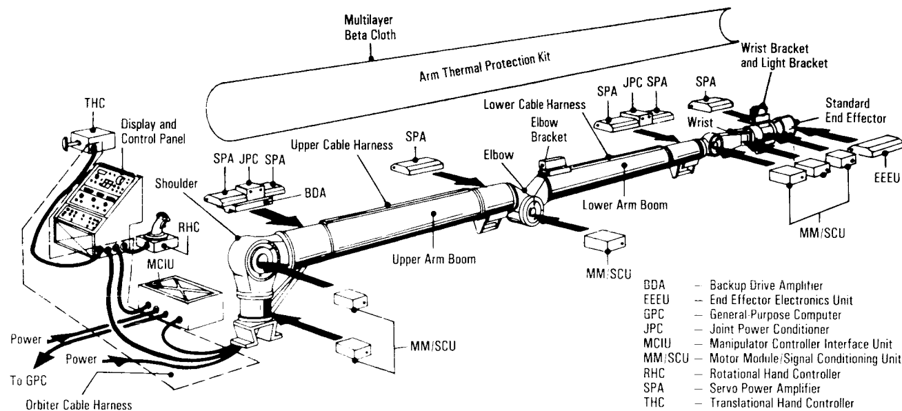
RMS Components
