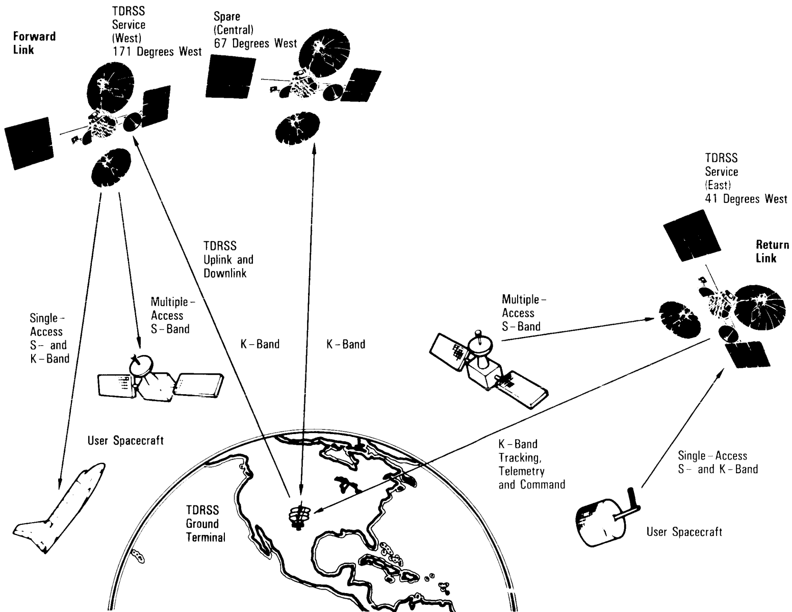
Linking Three Identical and Interchangeable Satellites With Earth Station
