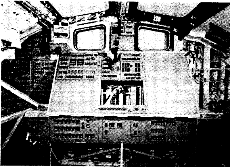
Aft Station Displays and Controls
