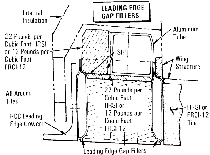
Typical TPS Gap Fillers and Thermal Barriers
