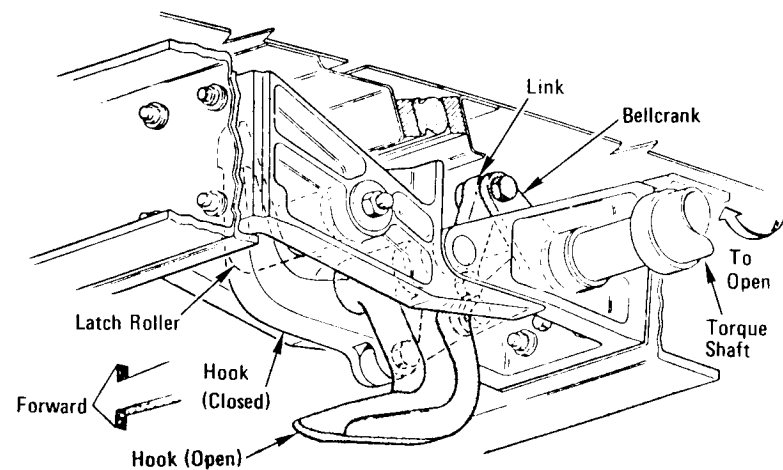
Centerline Door Latch Hook (Typical) Open Position
