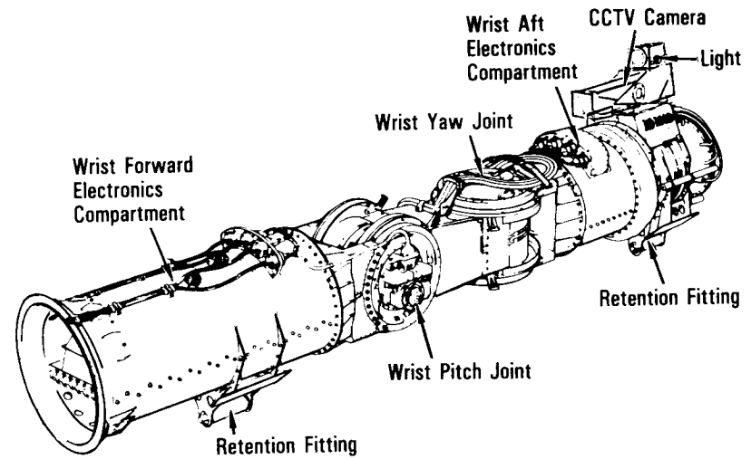
Overall Configuration of the Wrist Joint
