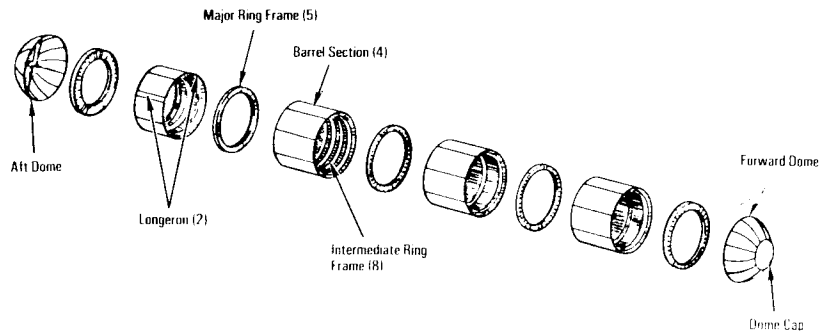
Liquid Hydrogen Tank Structure
