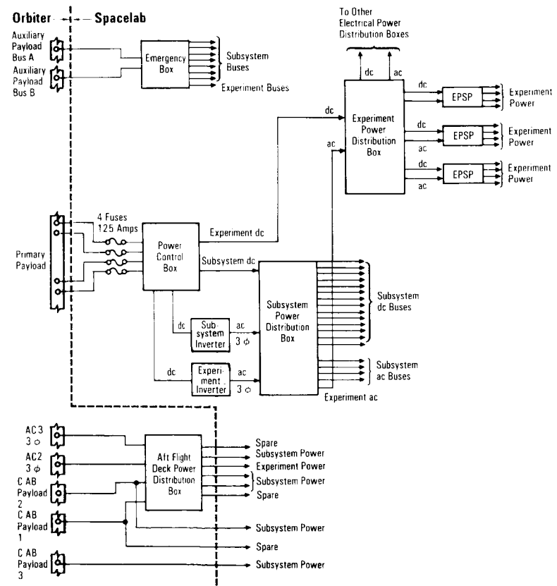
Orbiter Spacelab Electrical Power Distribution
