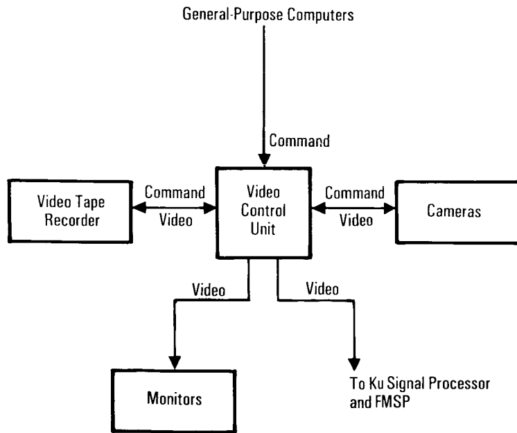
Closed-Circuit Television System
