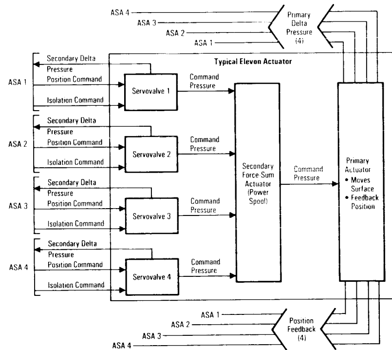
Typical Elevon Actuator
