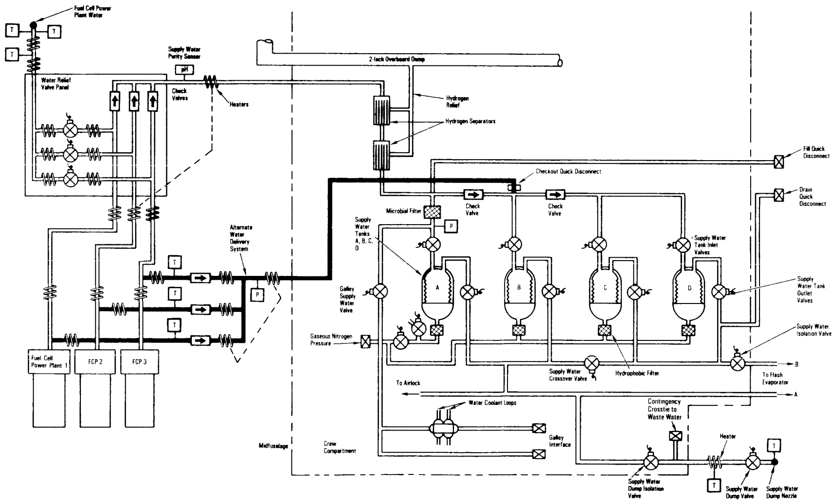
Fuel Cell Power Plant Redundant Water Relief
