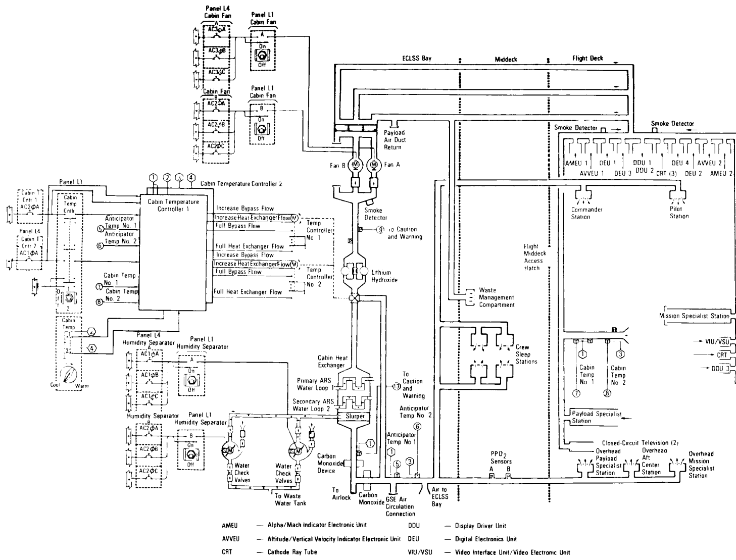
Crew Cabin Air
