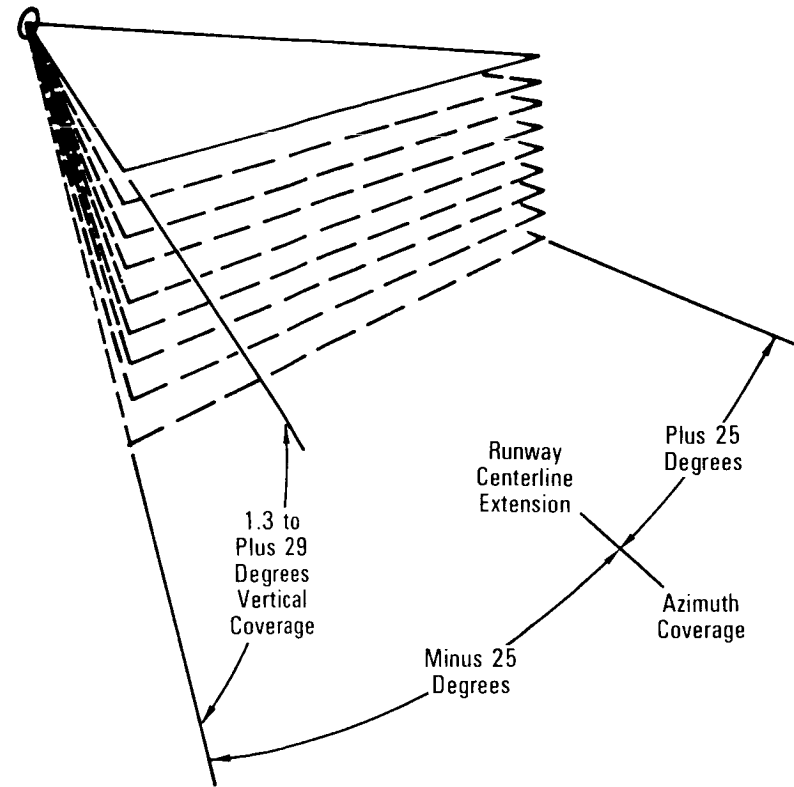
MSBLS Elevation Coverage
