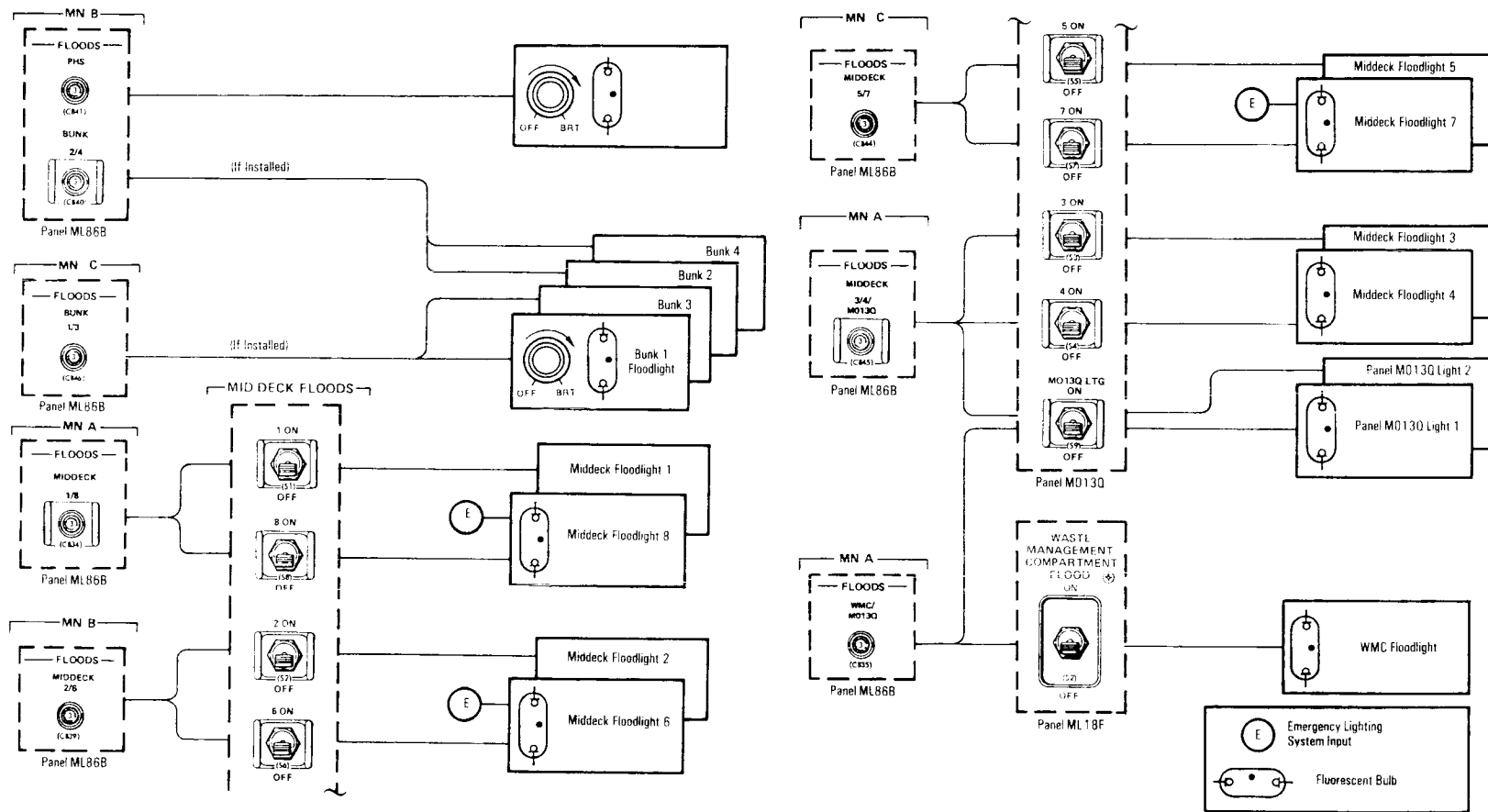
Middeck Floodlight Control
