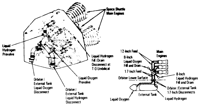
Main Propulsion System Propellant Feed System
