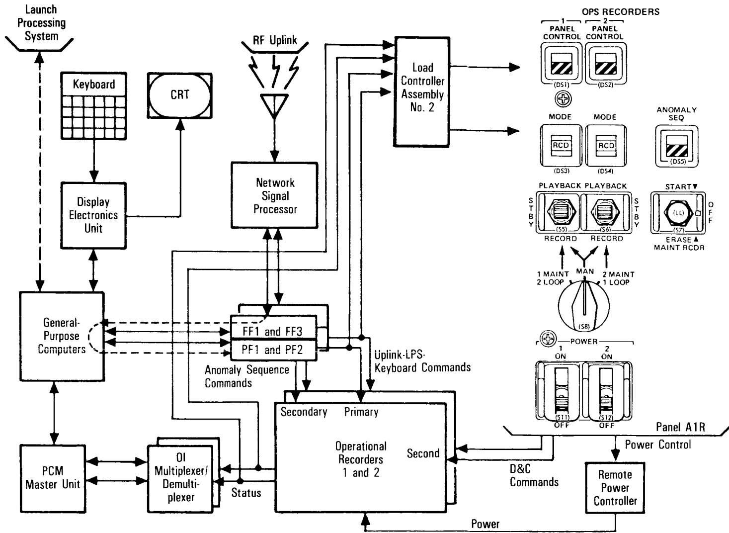
Operational Recorders
