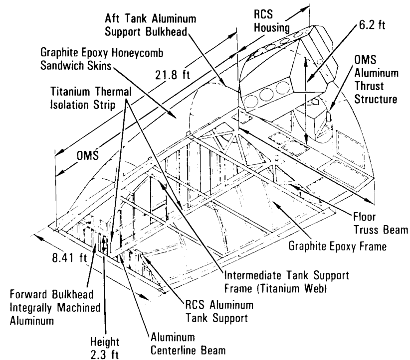
Aft Orbital Maneuvering System/Reaction Control System Pod
