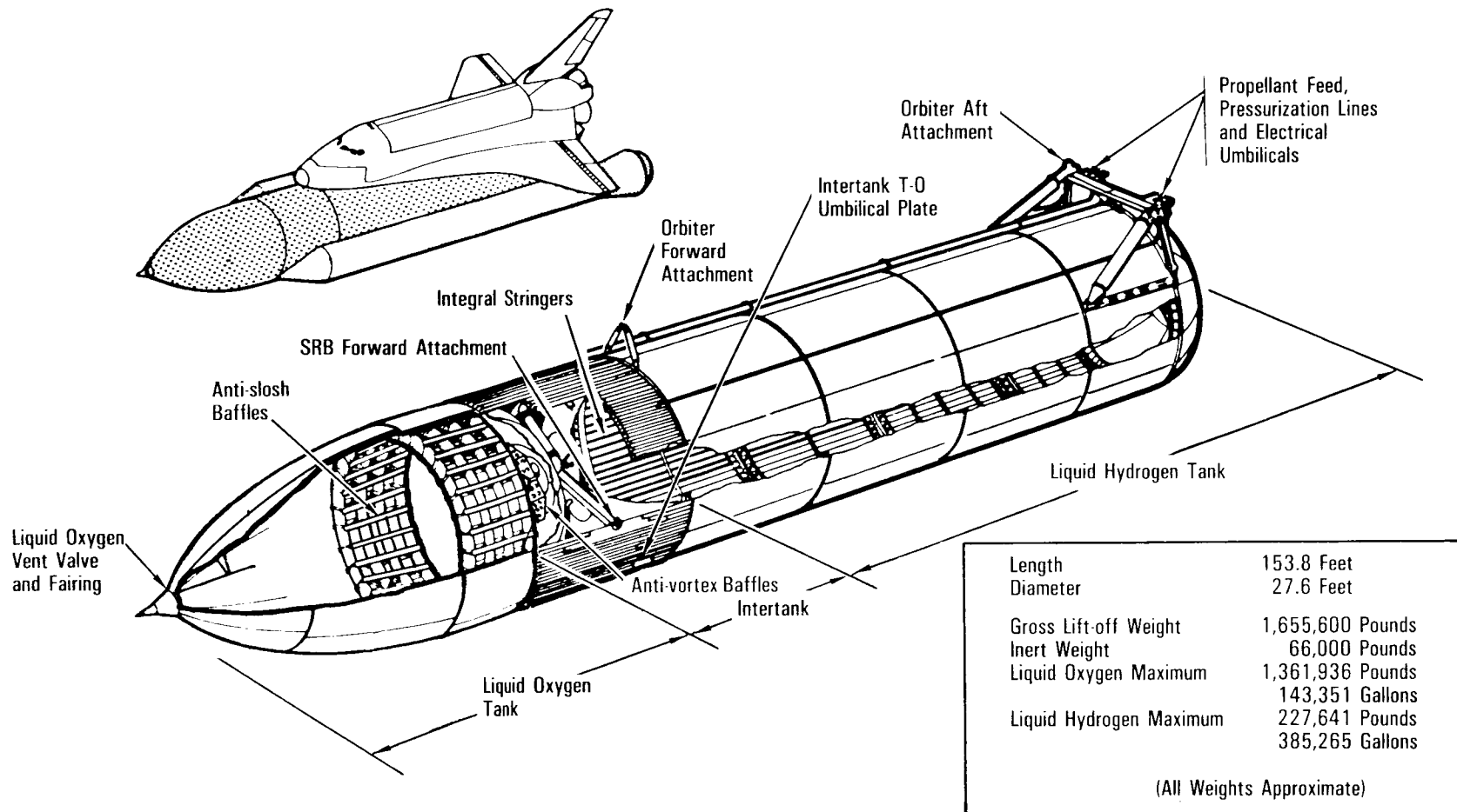
Lightweight External Tank
