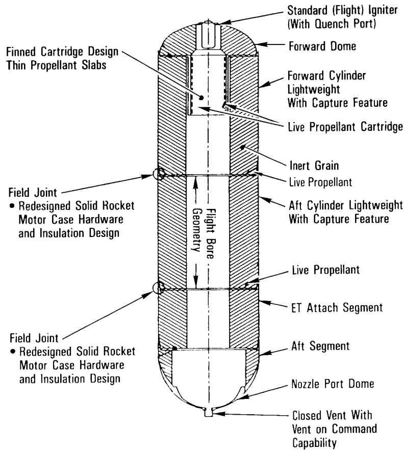
Joint Environment Simulation (JES) Configuration
