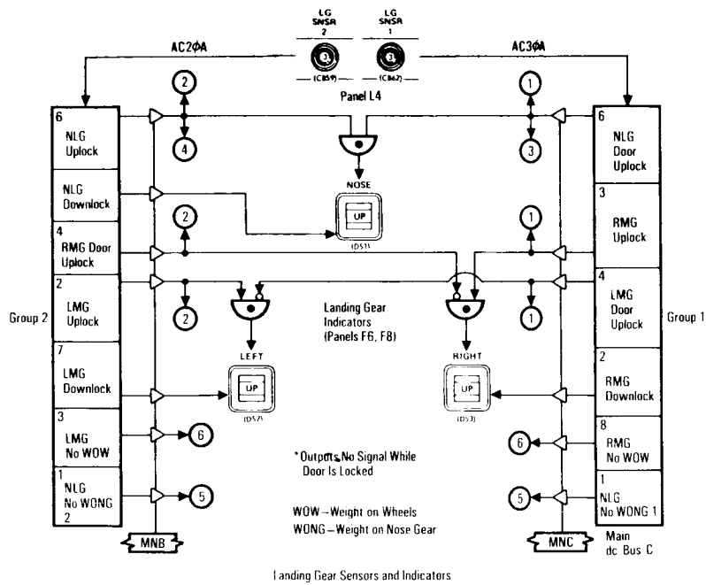
Landing Gear Sensors and Indicators
