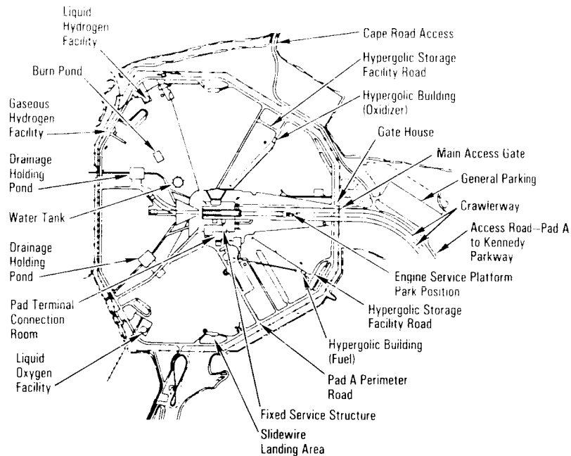
Launch Complex 39-A Surface Arrangement (Pad 39-B Similar)
