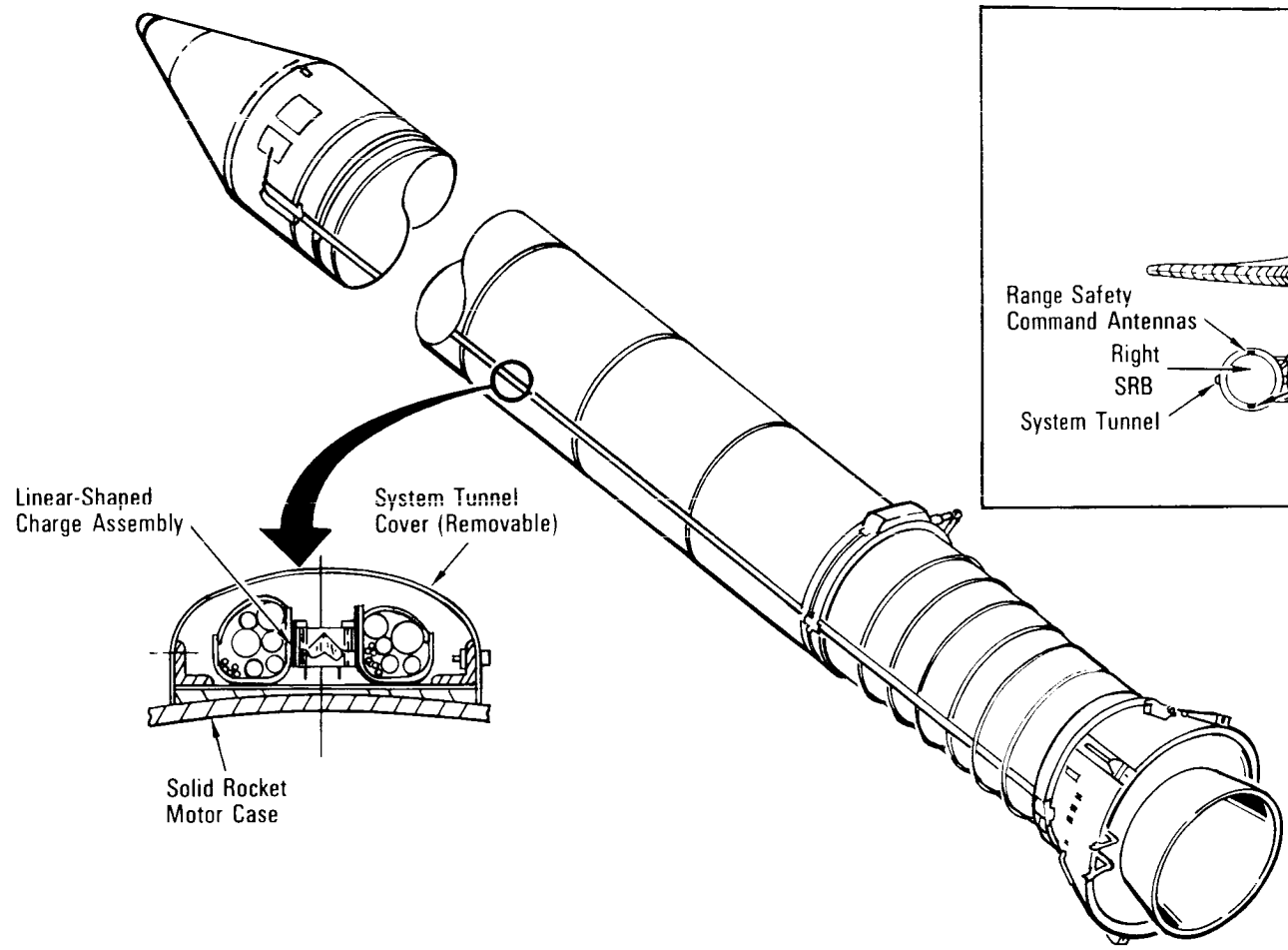
SRB Range Safety System
