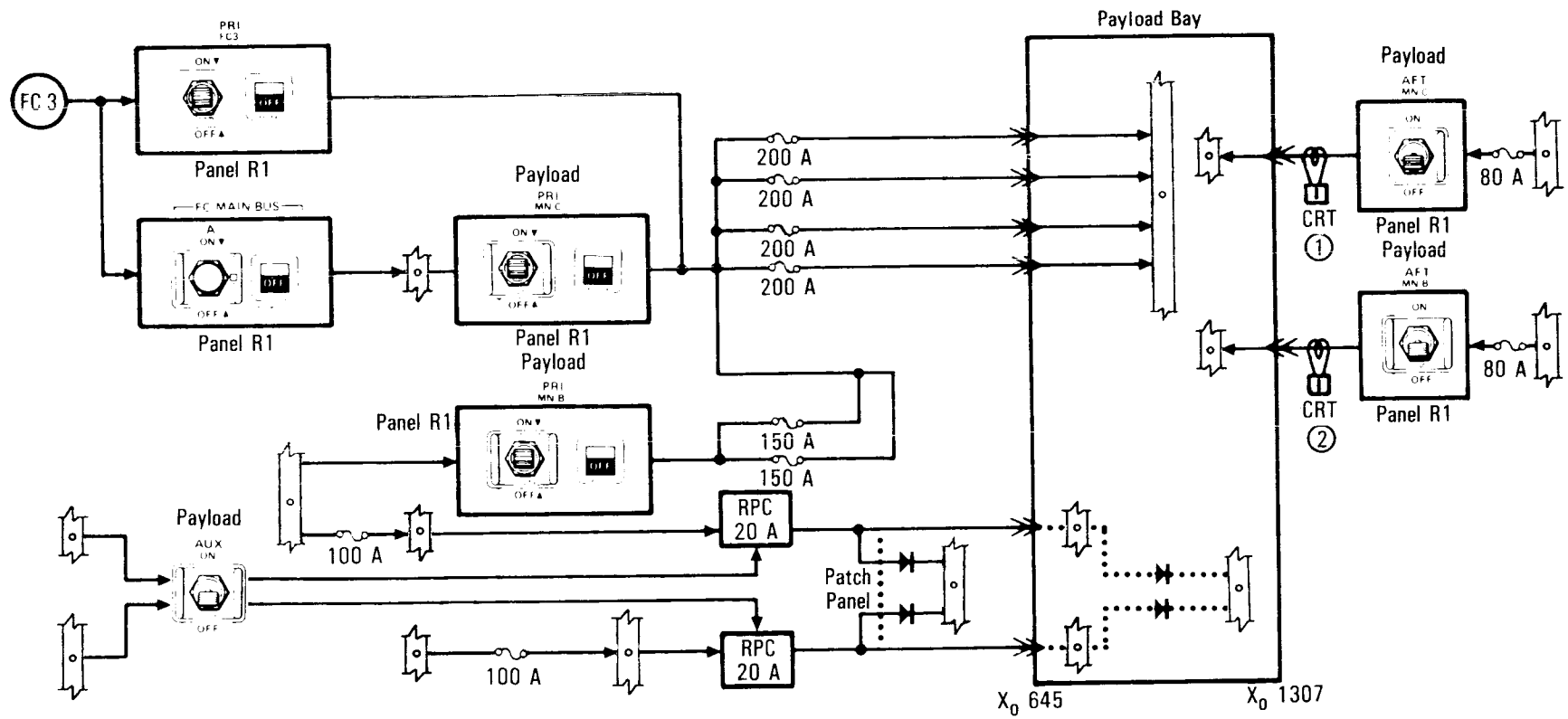
Orbiter/Payload Power Interface Schematic
