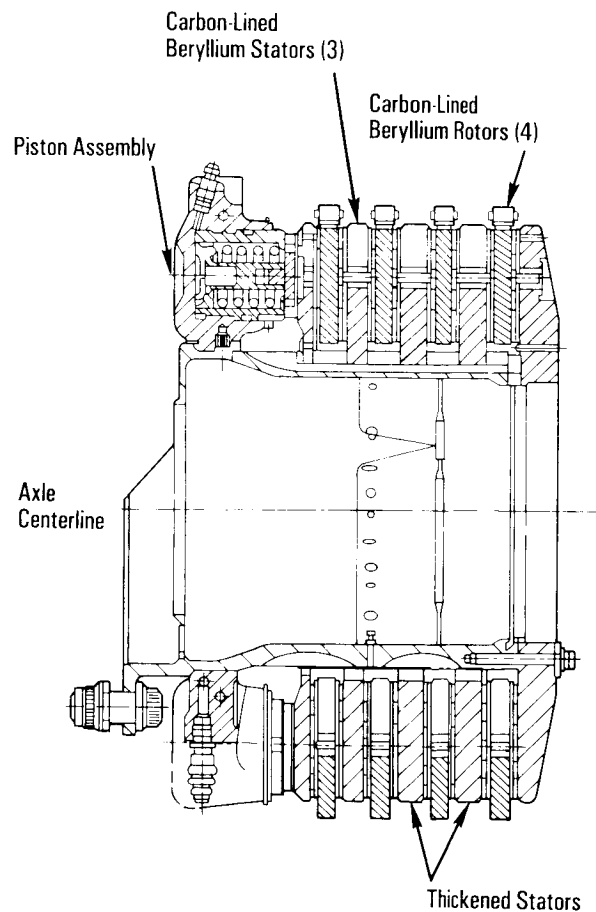
Improved Main Landing Gear Brake Assembly
