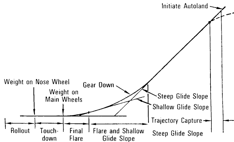
Approach and Landing Profile
