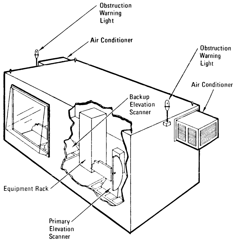
Elevation Shelter and Equipment
