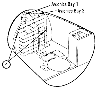
Avionics Bays 1 and 2 (Looking Forward)
