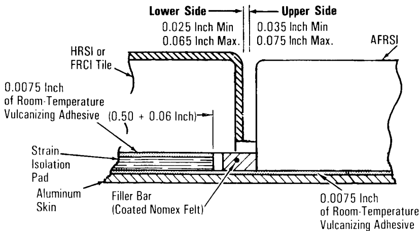
HRSI or FRCI Tile and AFRSI Interface
