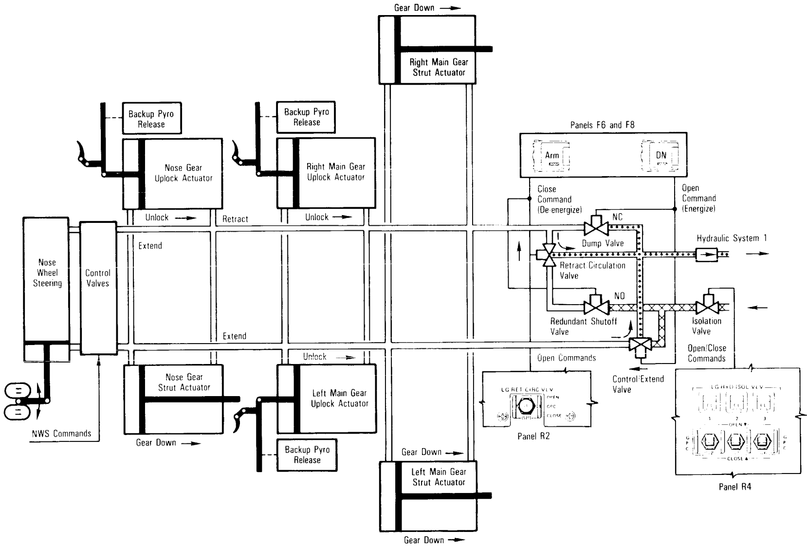
Landing Gear Hydraulics
