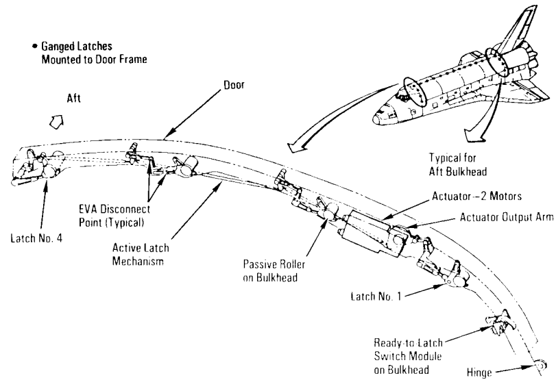
Typical Bulkhead Circular Latch System
