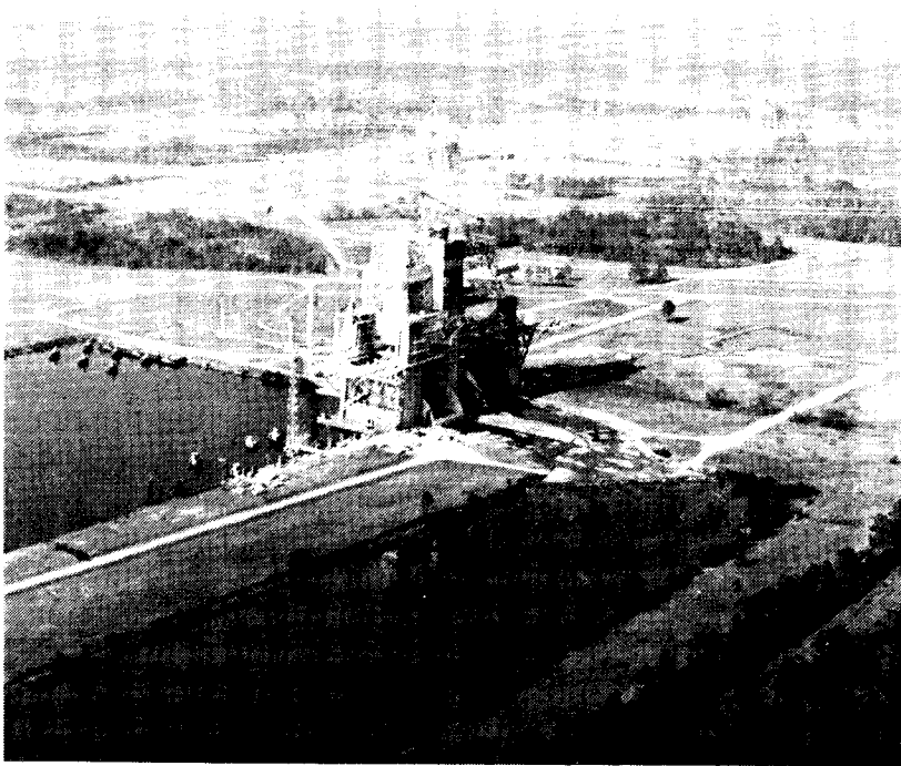
National Space Technology Laboratories test complex includes three test stands for captive-firing space shuttle main engines. The dual stand in the foreground has two test positions. The two single-engine stands are in the background.
