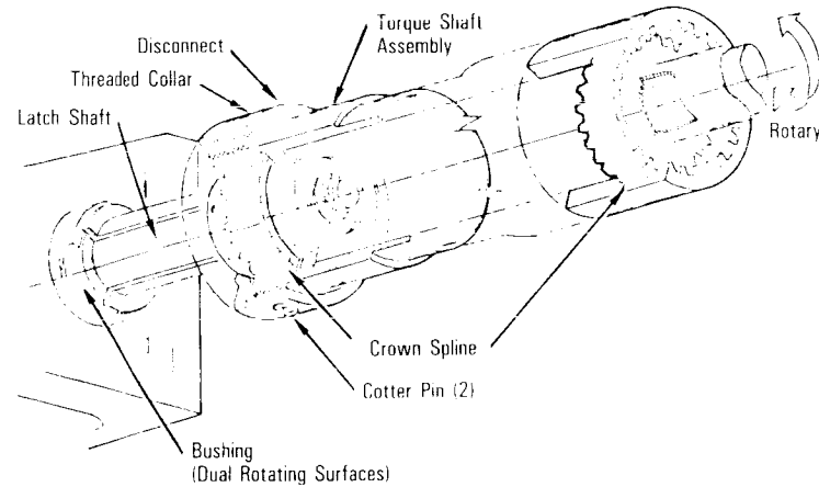
Extravehicular Activity Disconnect of Torque Shaft From Actuator and Latch Assembly of Centerline Latches
