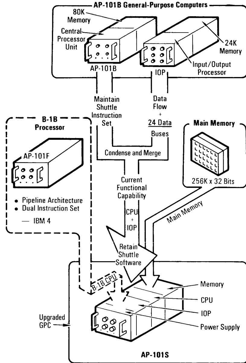
AP-101B General-Purpose Computers
