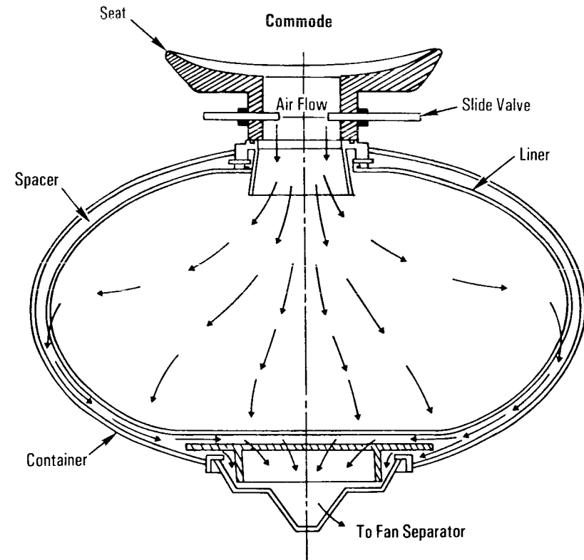
Waste Collection System Container Liner
