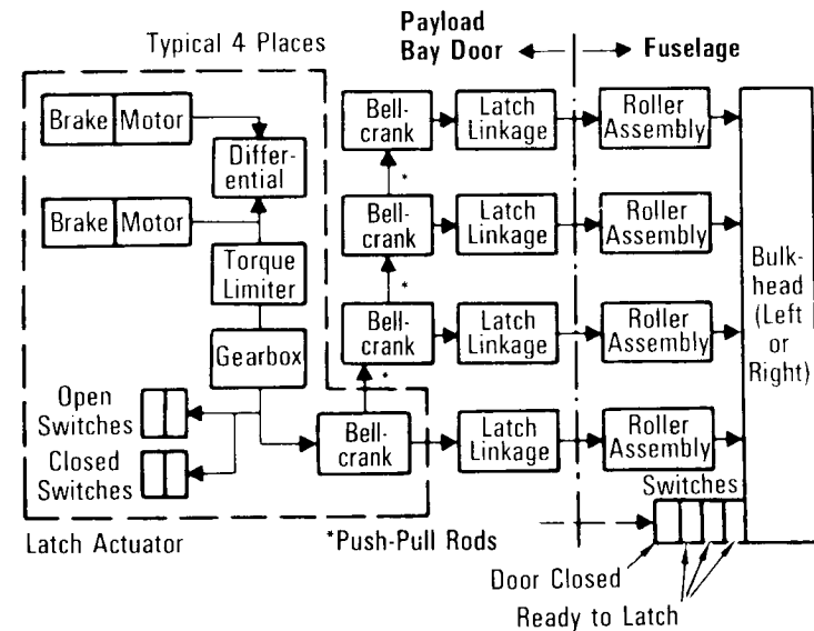
Payload Bay Door Bulkhead Latch Mechanical Block Diagram
