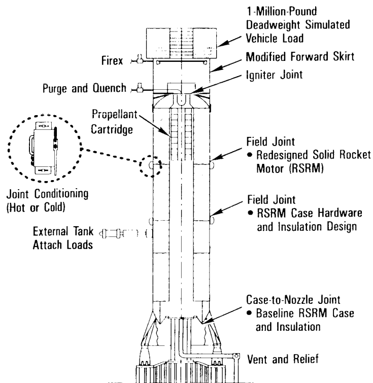
Transient Pressure Test Article (TPTA) Configuration
