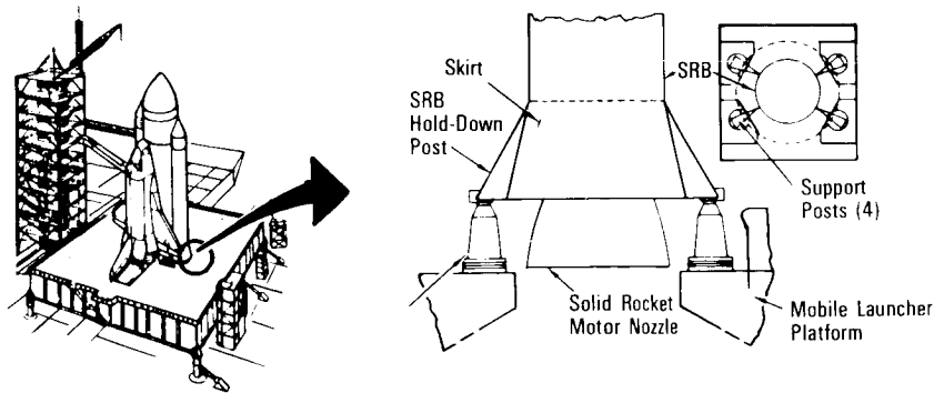
SRB Hold-Down Configuration
