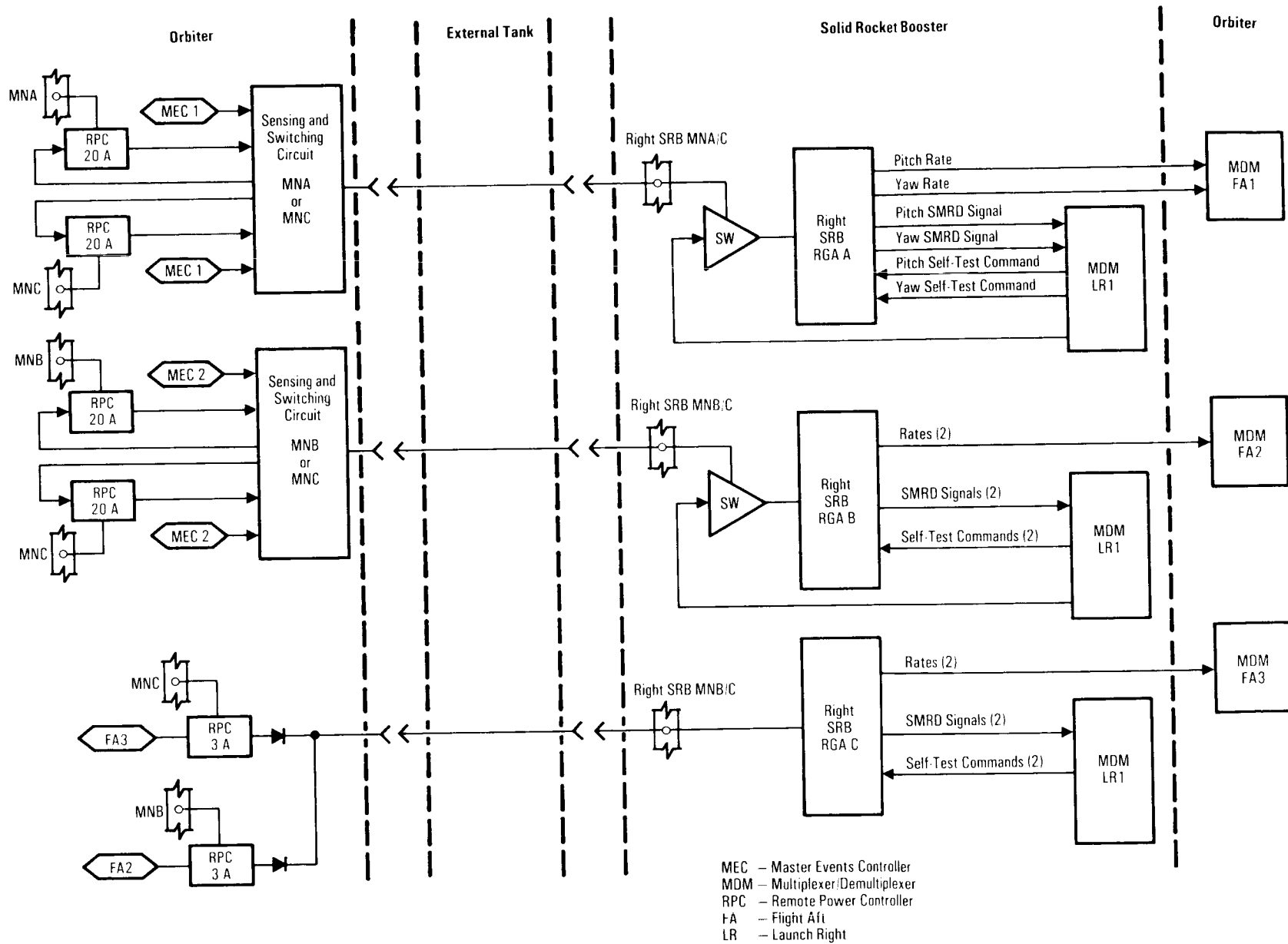
Solid Rocket Booster Rate Gyro Assembly Power and Data Interfaces
