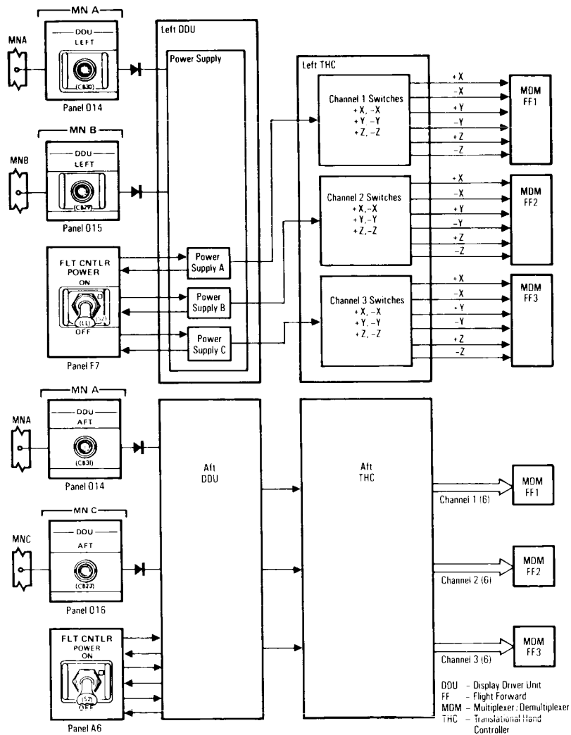
Translational Hand Controller Power and Data Interfaces
