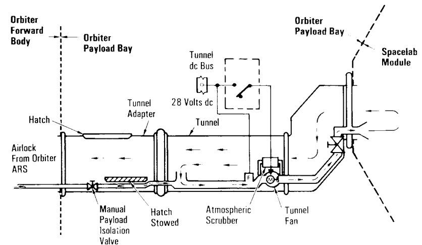
Tunnel Adapter Hatch Open—48-Cubic-Feet-Per-Minute Duct Operating
