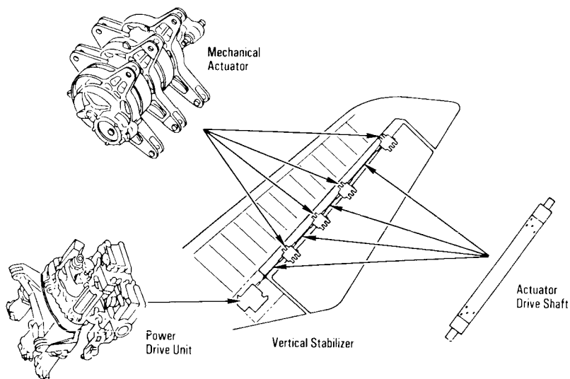
Rudder/Speed Brake Actuator Location
