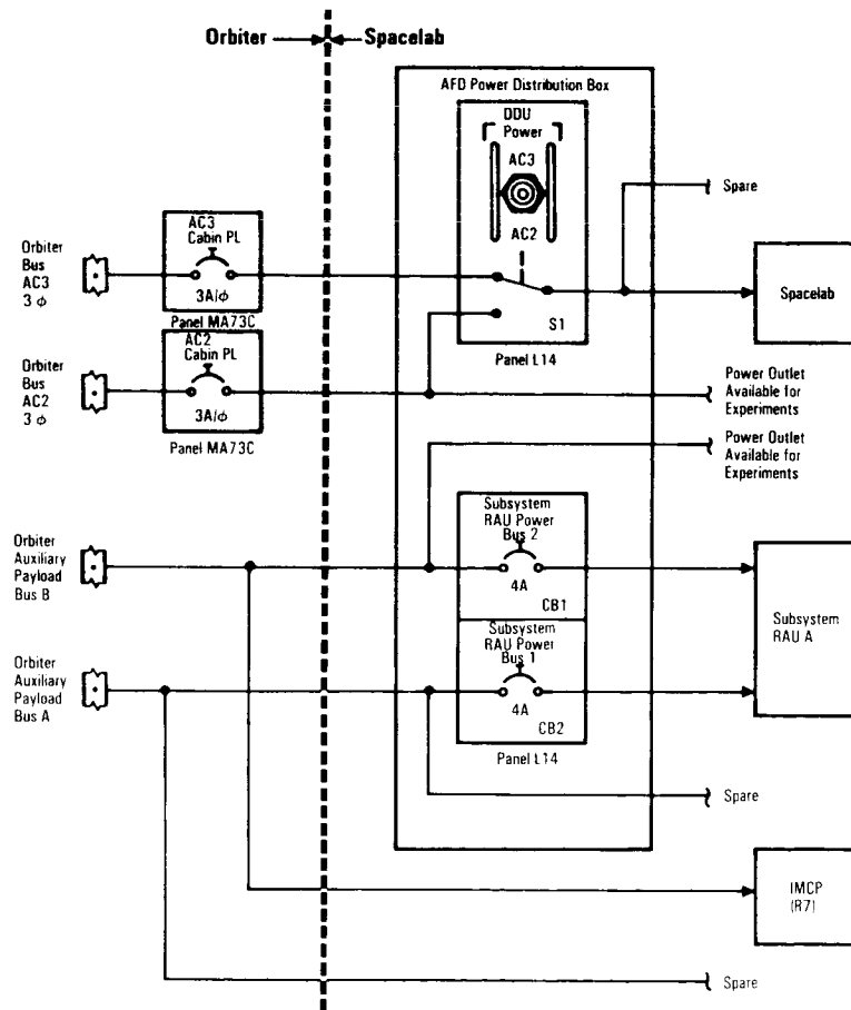
Pallet-Only Configuration—Orbiter Aft Flight Deck Power Distribution
