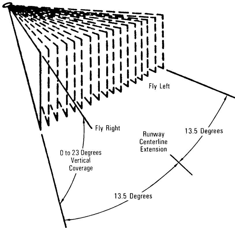
Microwave Scan Beam Landing System Azimuth Coverage and Distance-Measuring Equipment
