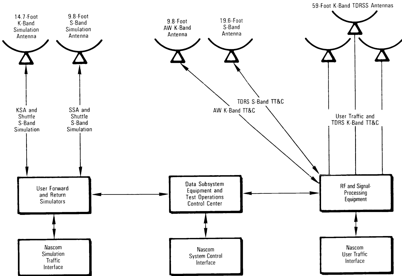
Tracking and Data Relay Satellite System Antenna
