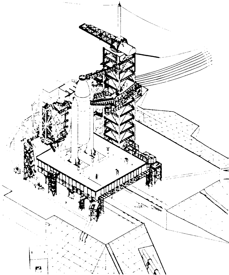
Overhead View of Shuttle in Checkout Configuration
