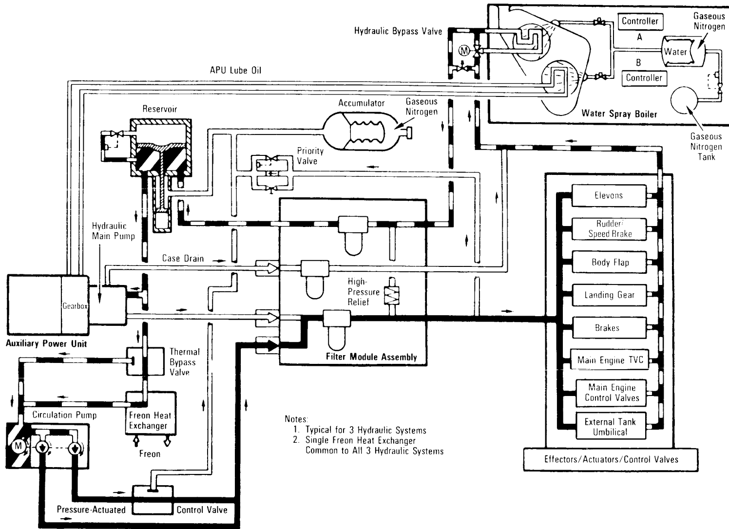
Hydraulic Power System Circulation Mode
