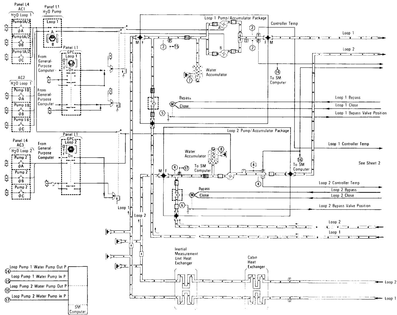
Water Coolant Loops (Sheet 1 of 3)
