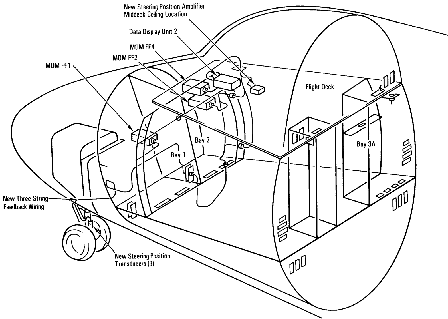
Nose Wheel Steering
