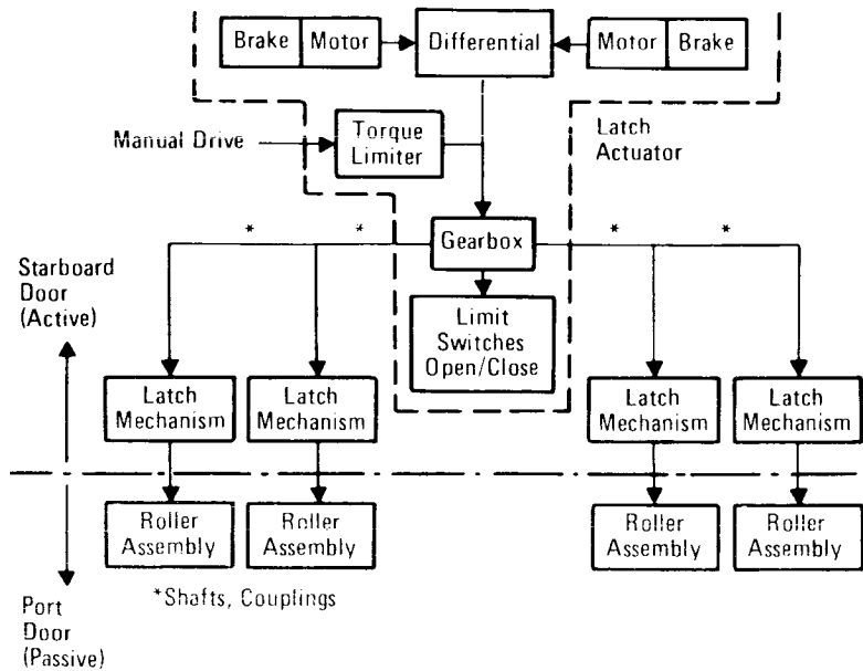
Payload Bay Doors Centerline Latch Mechanical Block Diagram
