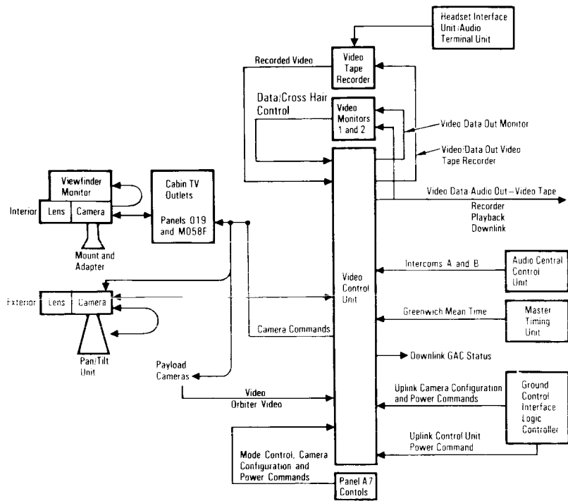
Closed-Circuit Television System
