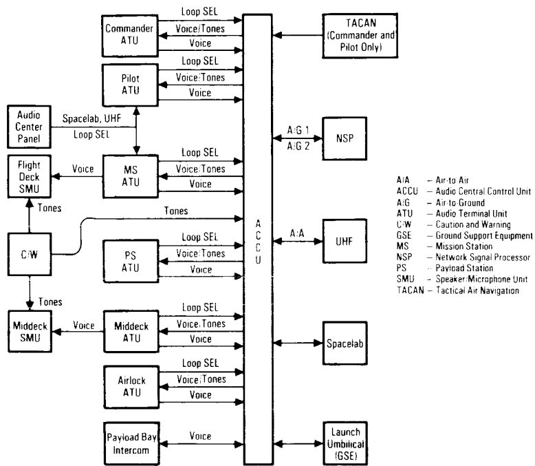
Audio System
