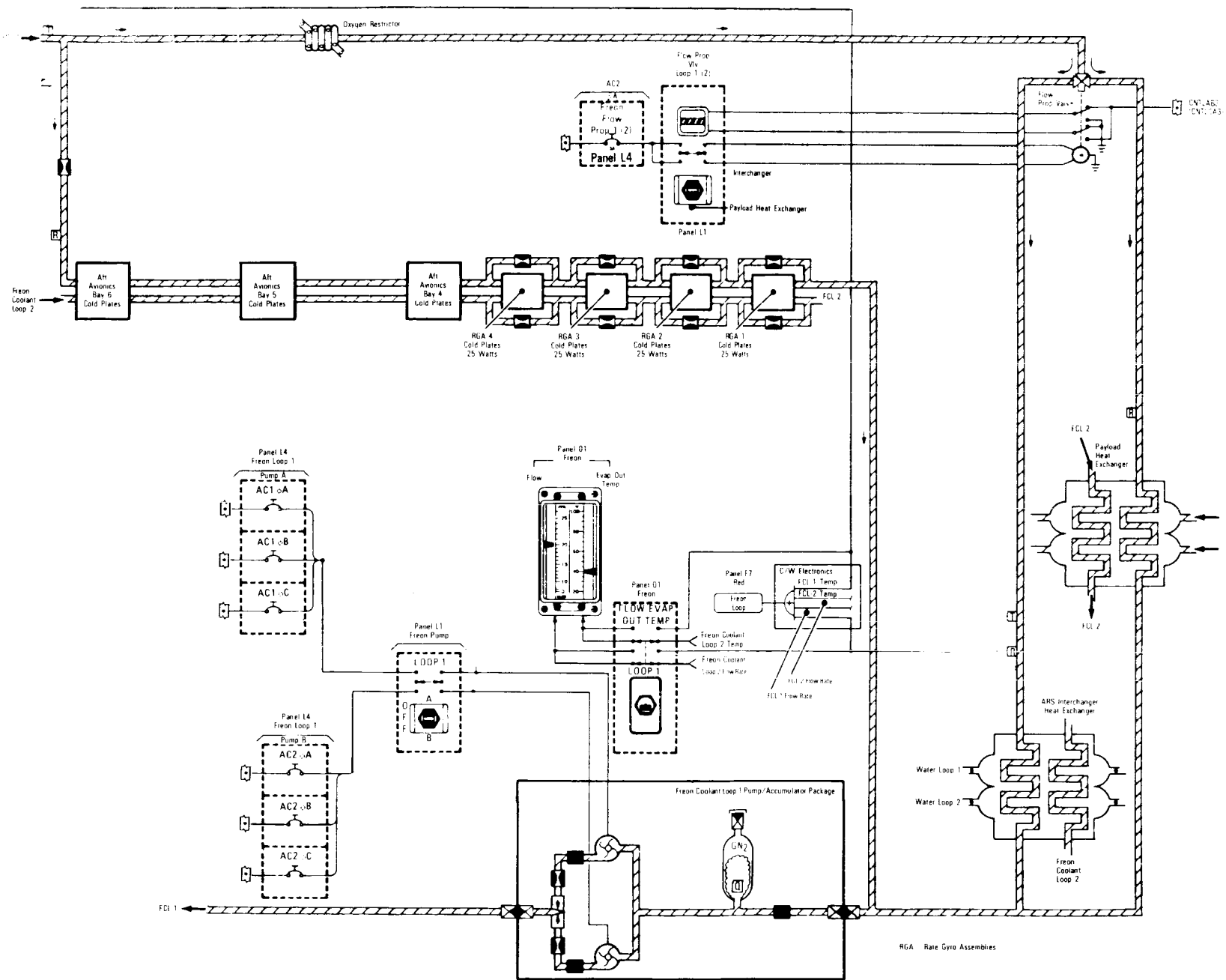
Active Thermal Control Freon-21 Coolant Loop (Sheet 3 of 3)
