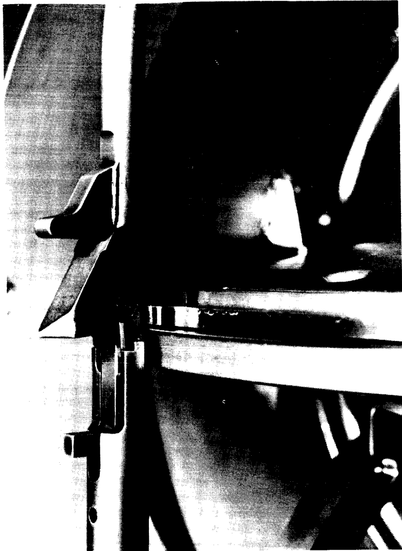
17-Inch Disconnect With Latch Engaged on Flapper Valve (Other Flapper Valve Removed to Show Latch Engaged on Flapper Valve)
