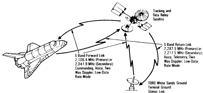
NASA S-Band Communications With TDRSS and WSGT to Mission Control Center-Houston
