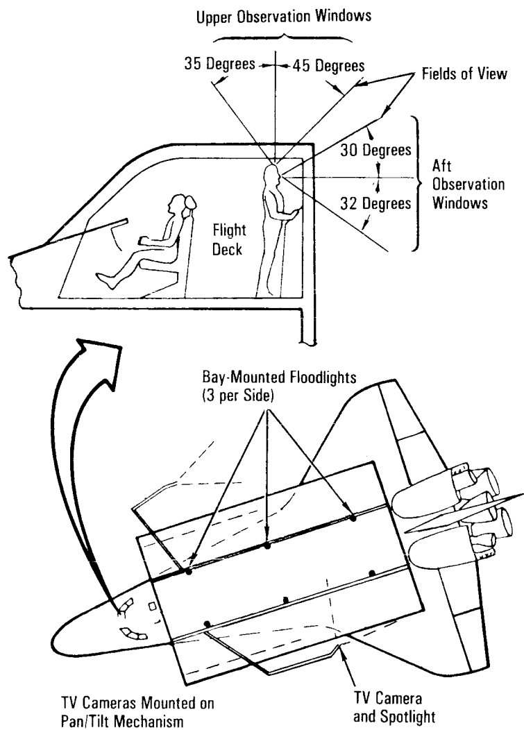
Payload Bay Television Cameras and Floodlights
