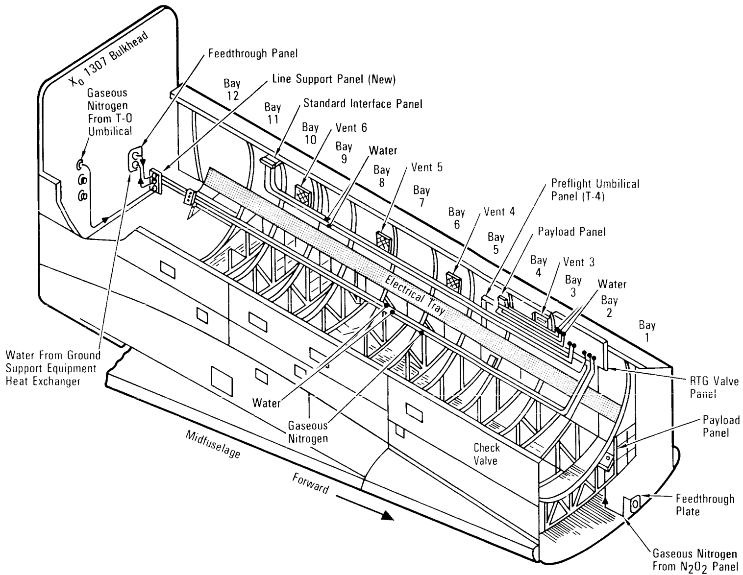
Water Coolant System for Radioisotope Thermoelectric Generator and Gaseous Nitrogen Purge System for Payload Support in Payload Bay
