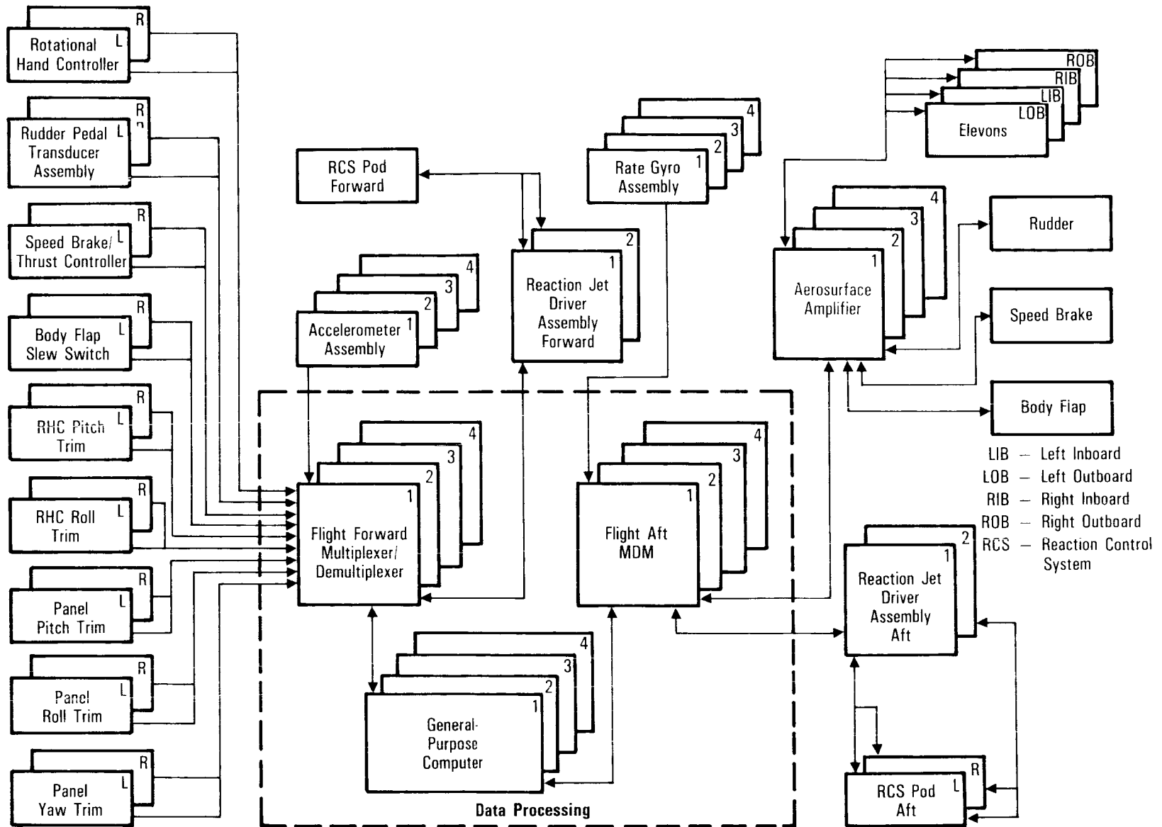
Flight Control System Hardware
