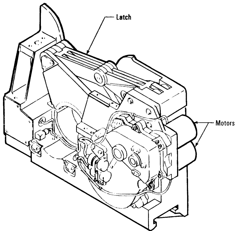
Payload Retention Latch
