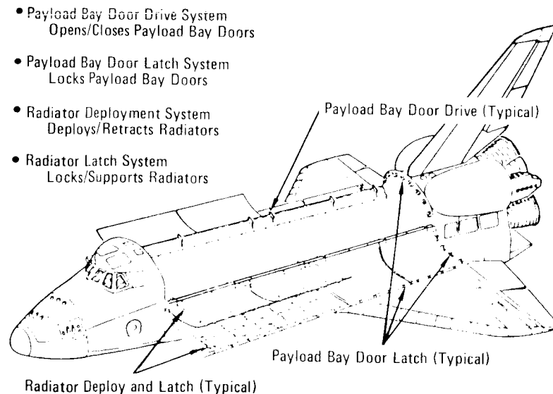
Payload Bay Door and Radiator Mechanisms
