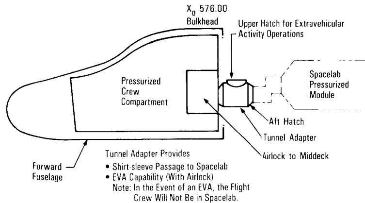
Airlock/Tunnel Adapter
