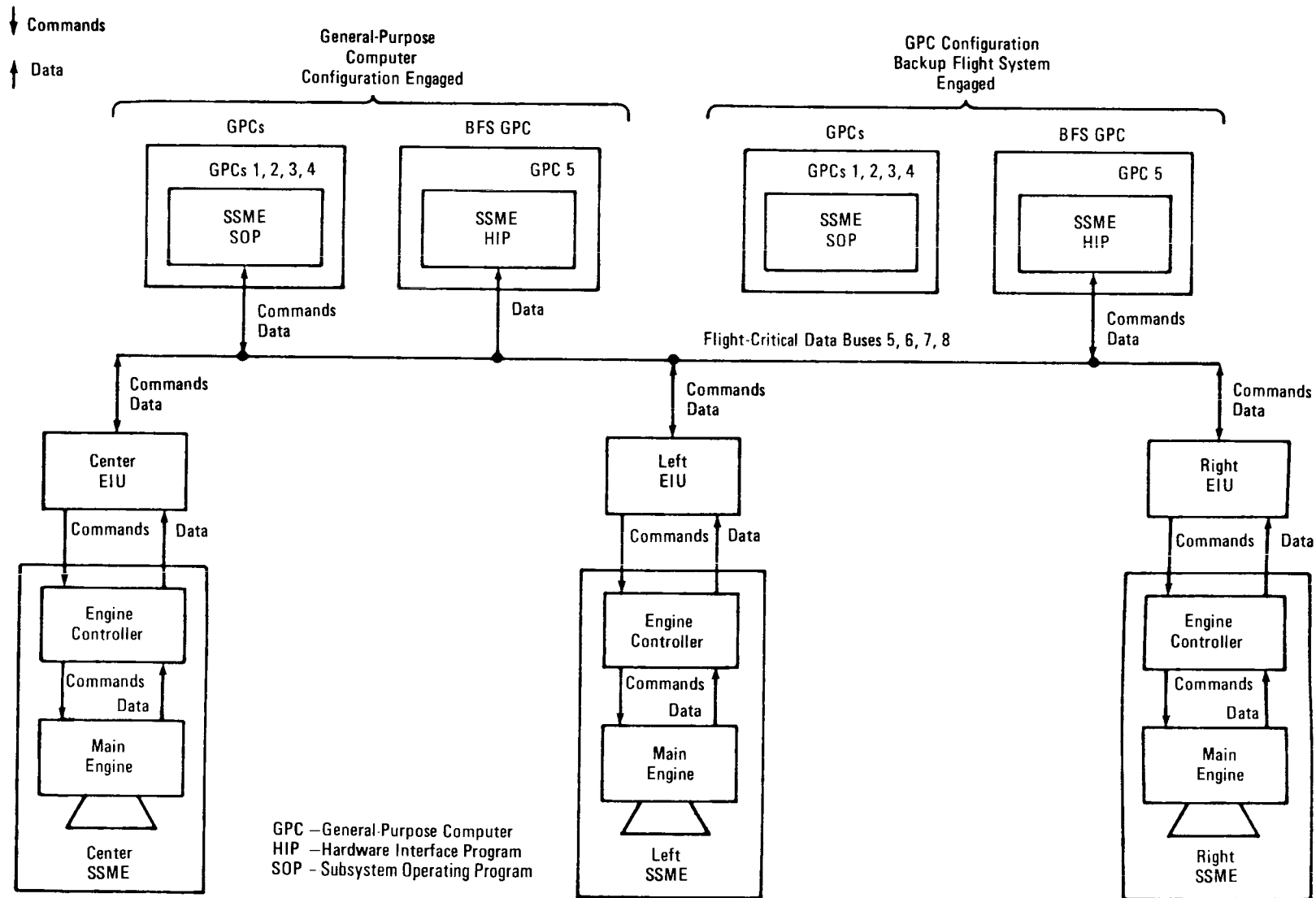
General-Purpose Computer Overview
