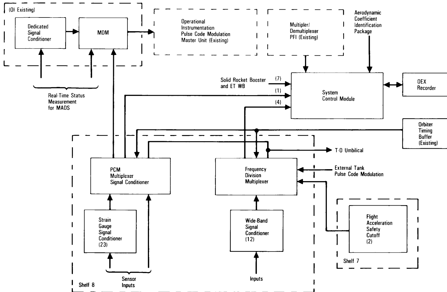
Modular Auxiliary Data System Block Diagram, OV-102 (Columbia) Only
