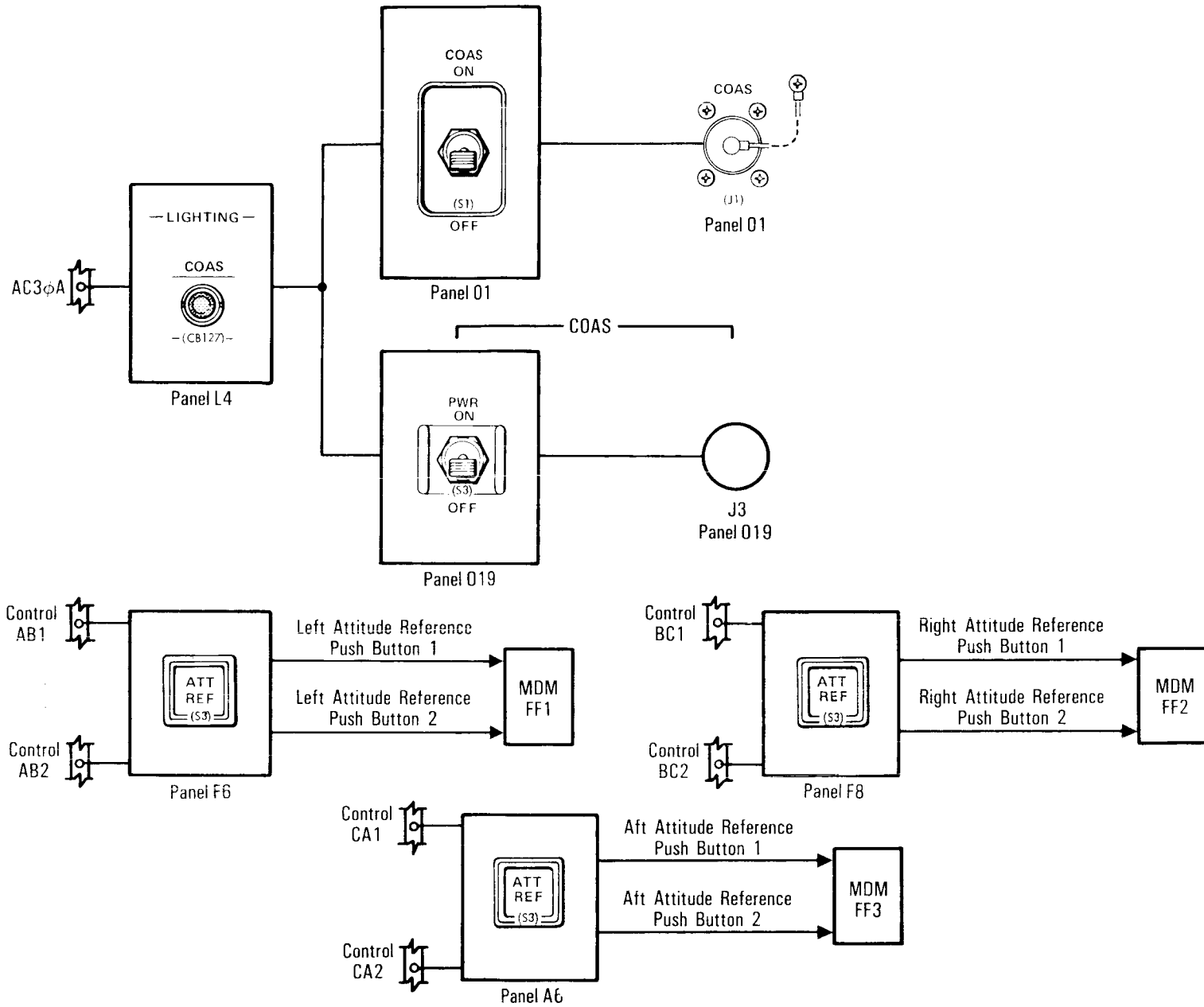
Power and Data Interfaces of Crewman Optical Alignment Sight and Attitude Reference Push Buttons
