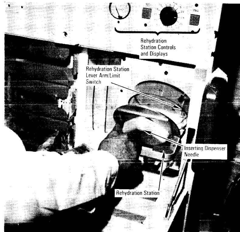
Galley Rehydration Station
