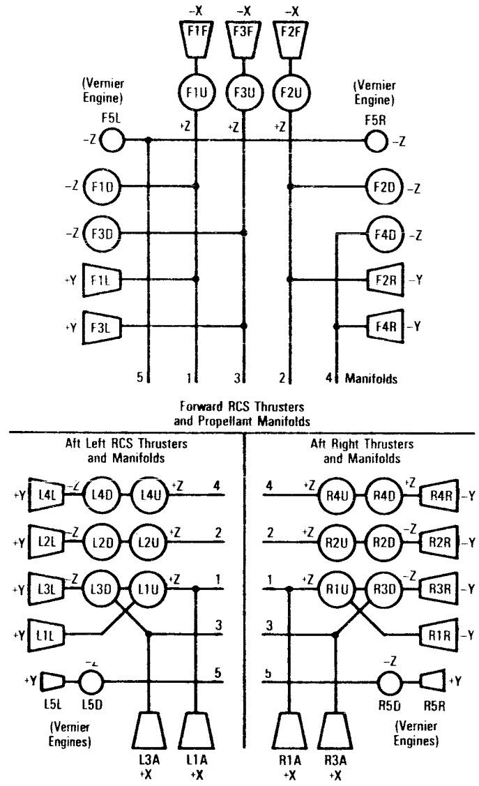
Reaction Control System Propellant Manifold Feed System to Engines
