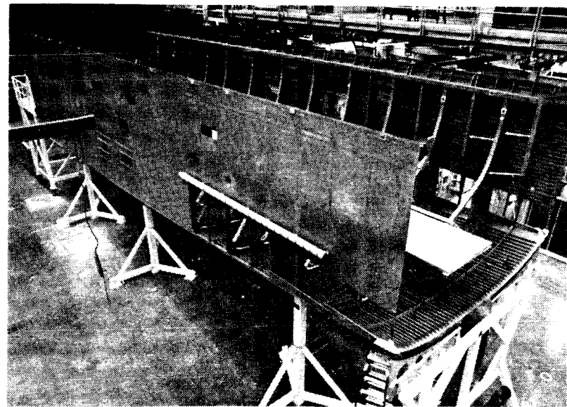
Midfuselage
