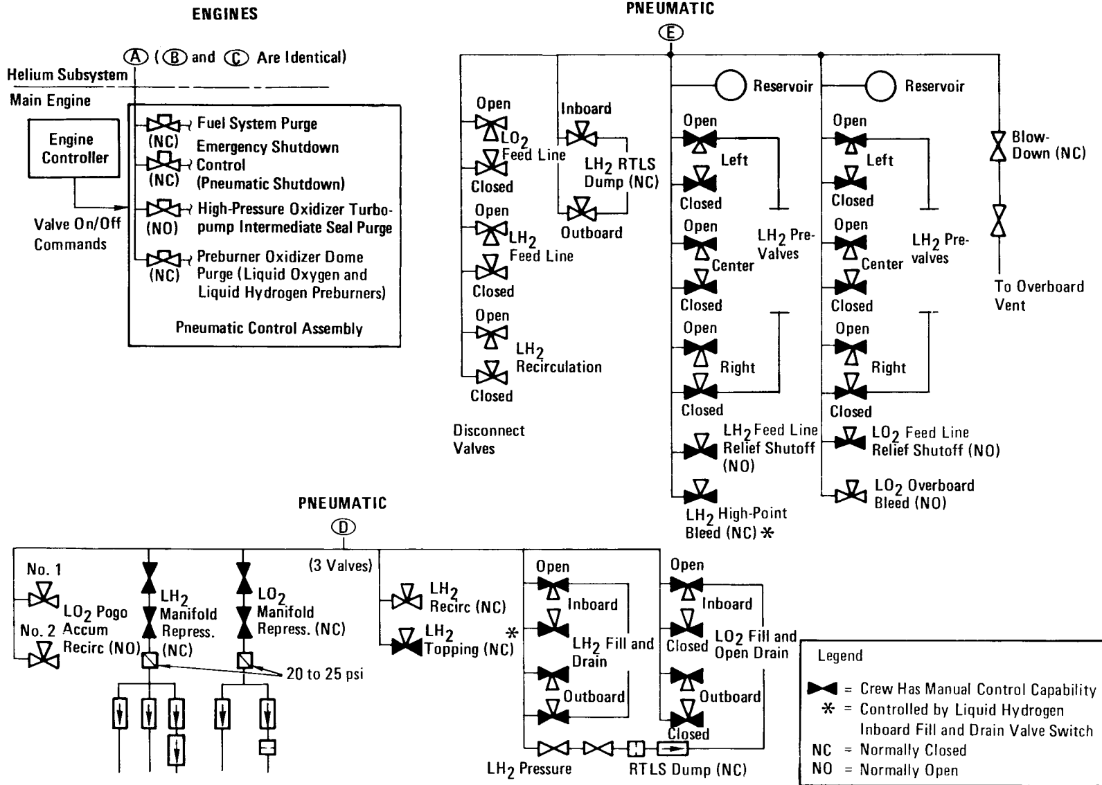
Helium System Distribution
