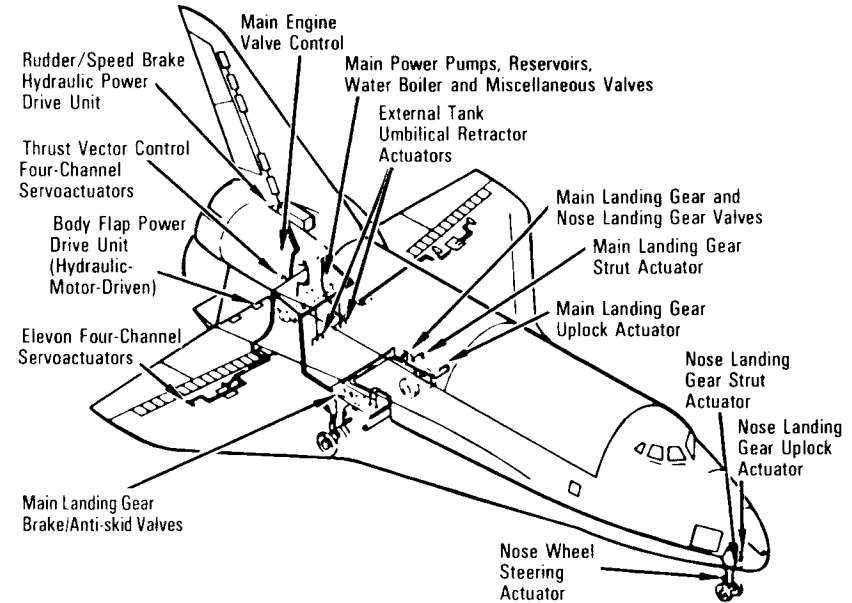
Hydraulic Systems
