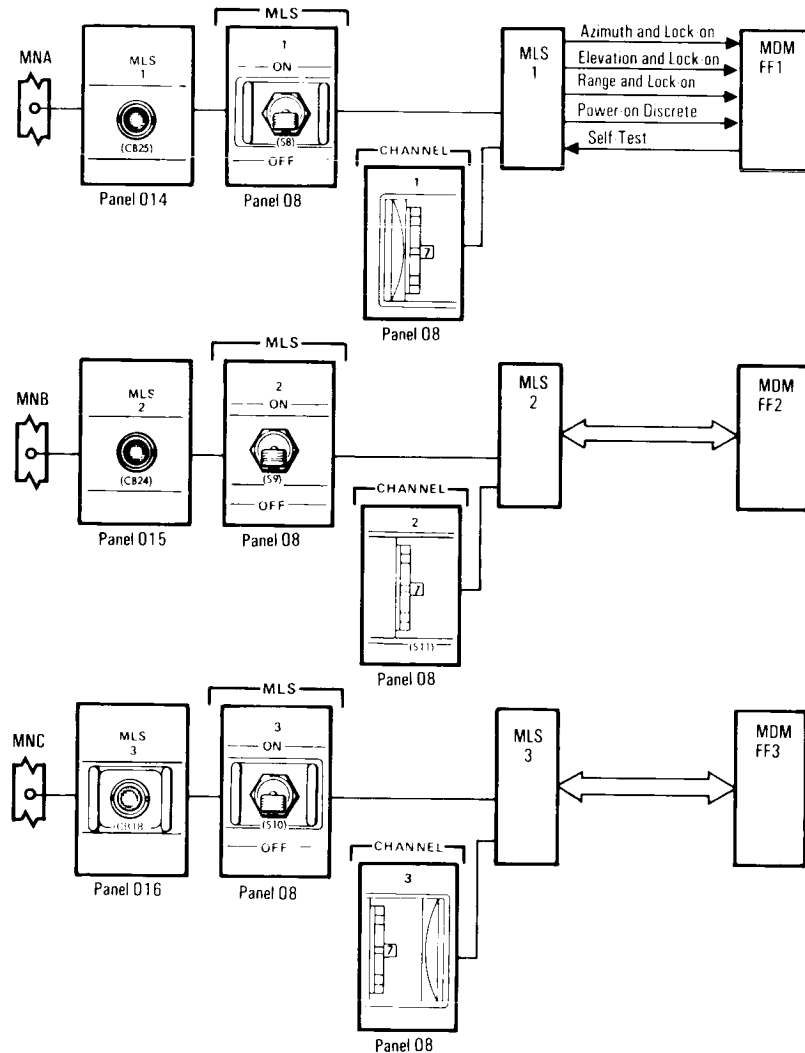
Microwave Scan Beam Landing System Power and Data Interfaces
