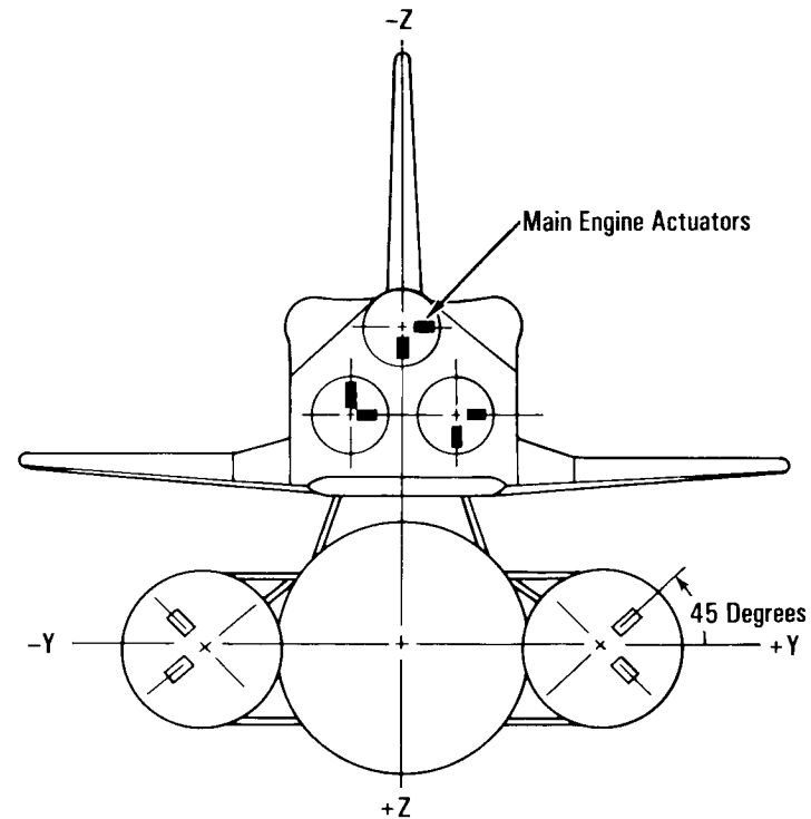
Orientation of Main Engine Actuators
