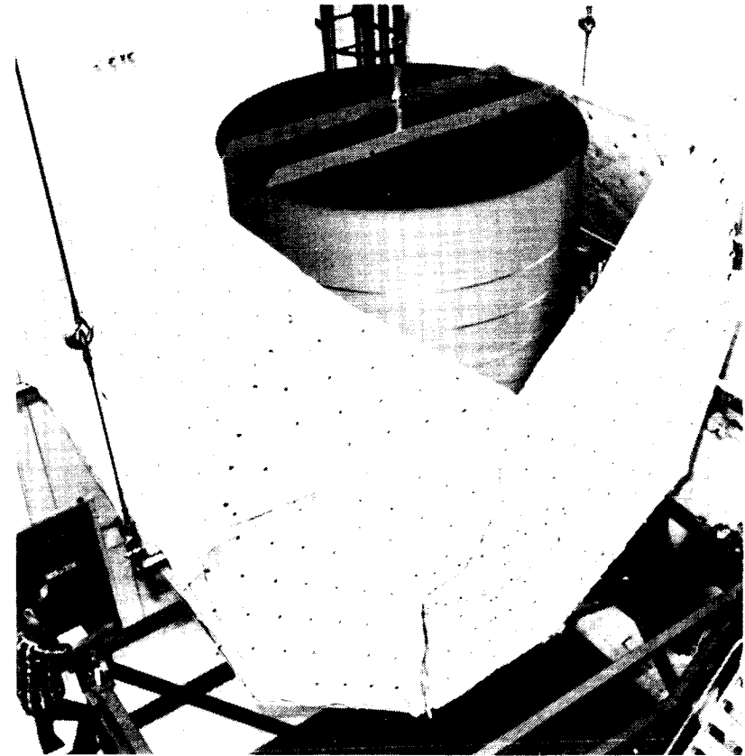
PAM Sunshield Closed
