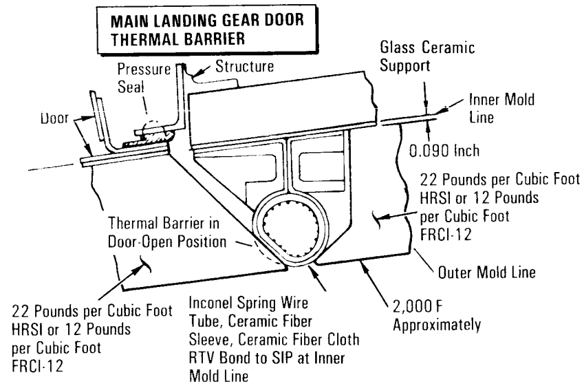
Typical TPS Gap Fillers and Thermal Barriers
