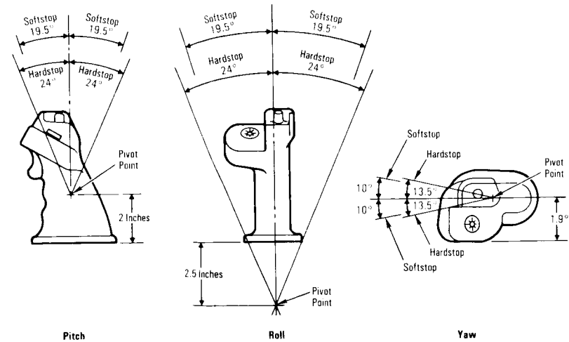
Rotational Hand Controller Mechanical Limits
