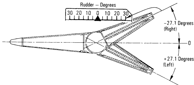
Surface Position Indicator Rudder Travel
