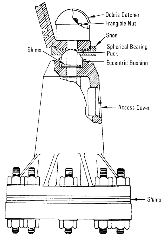
Solid Rocket Booster Support/Hold-Down
