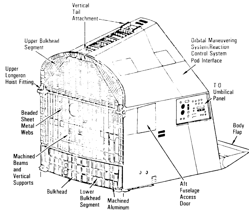
Aft Fuselage
