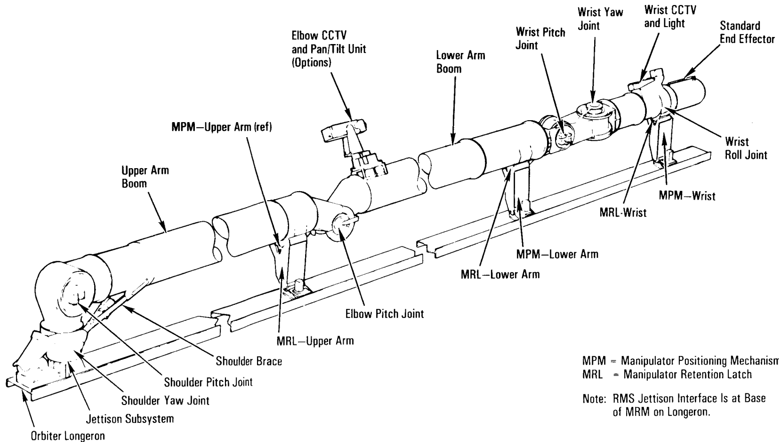
RMS—Stowed Position and General Arrangement
