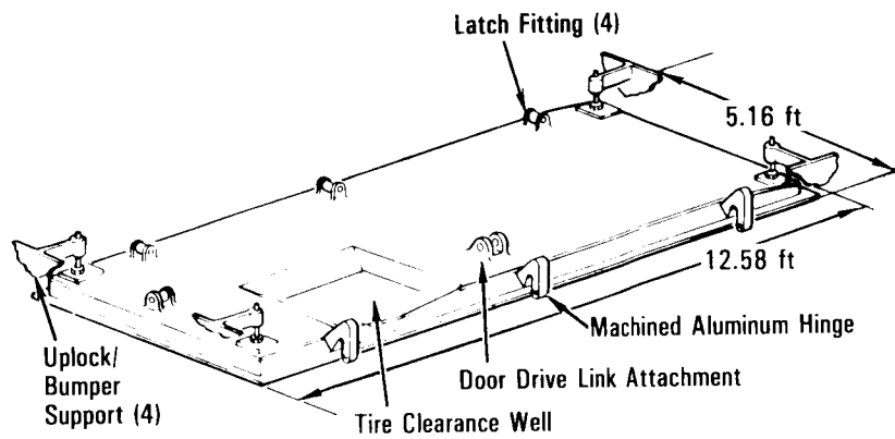
Main Landing Gear Door Construction
