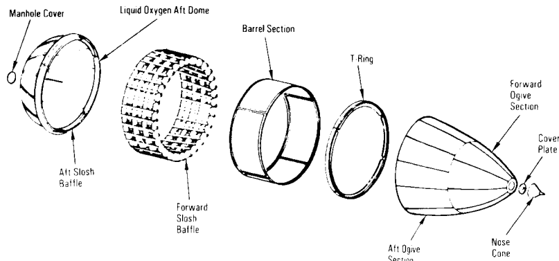
Liquid Oxygen Tank Structure
