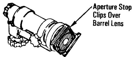
Aperture Stop Installation
