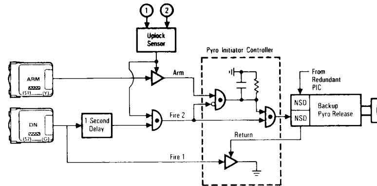
Nose Landing Gear and Main Landing Gear Uplock Release Pyro Actuator Circuit
