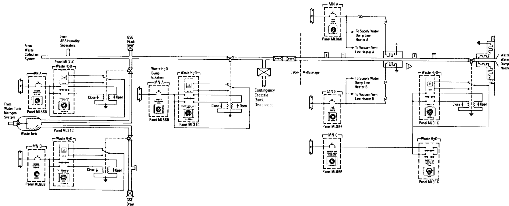
Waste Water Tank and Waste Water Dump Line
