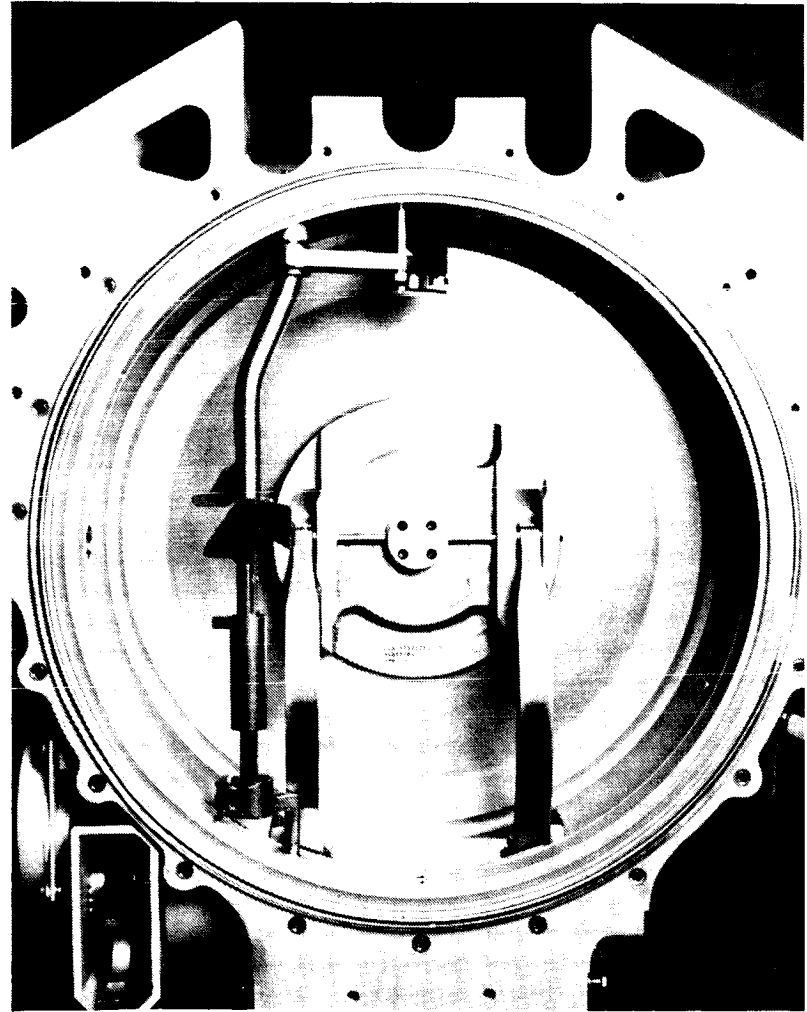
17-Inch Disconnect With Latch Feature Disengaged, Flapper Valve Closed (Other Flapper Valve Removed to Show Unlatch Disengaged, Flapper Valve Closed)
