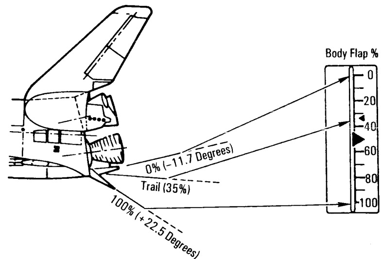
Surface Position Indicator Elevon Travel
