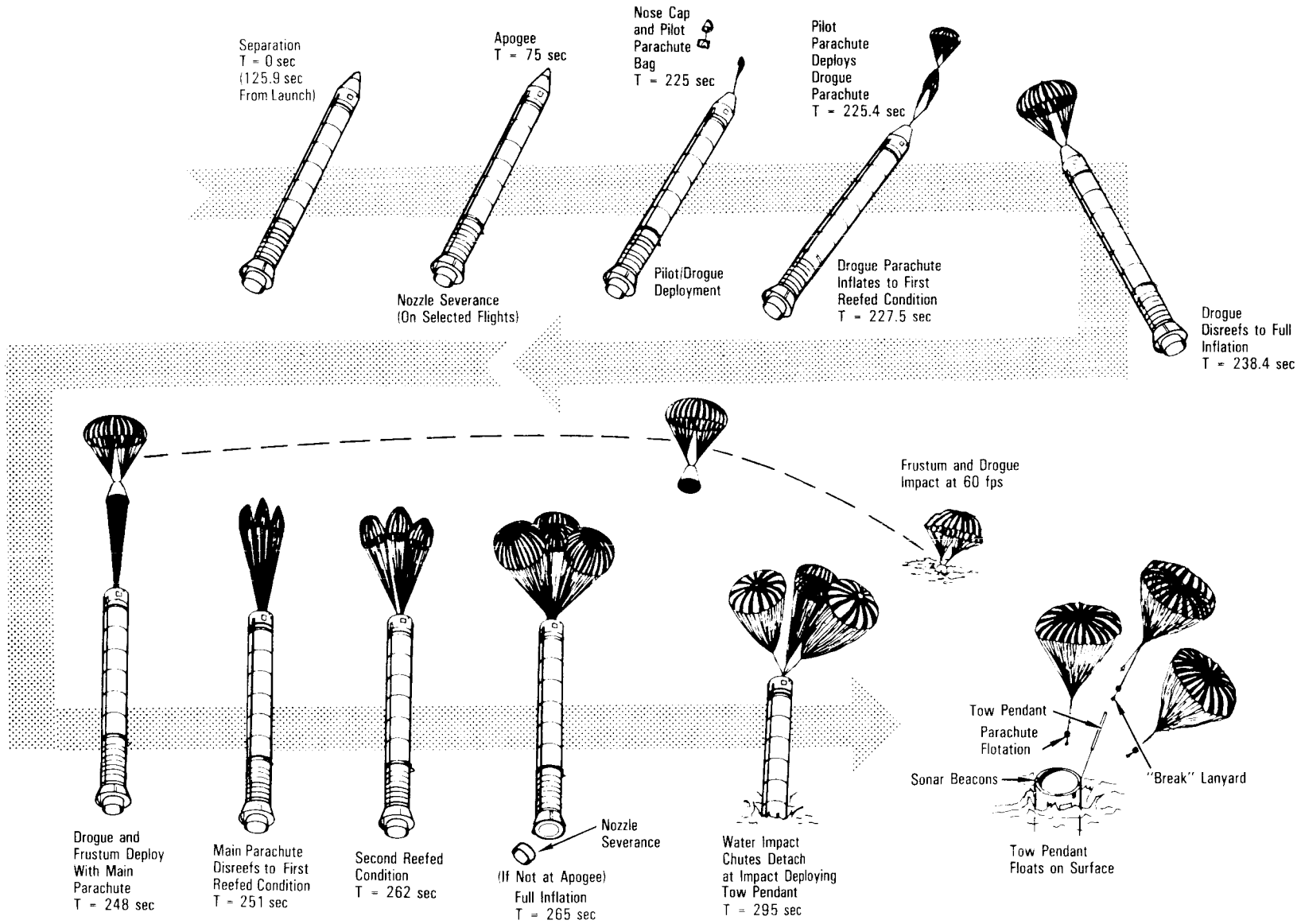
SRB Descent and Splashdown
