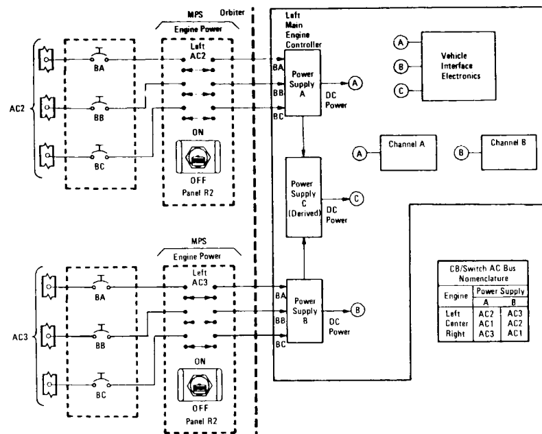
Main Engine Controller Power
