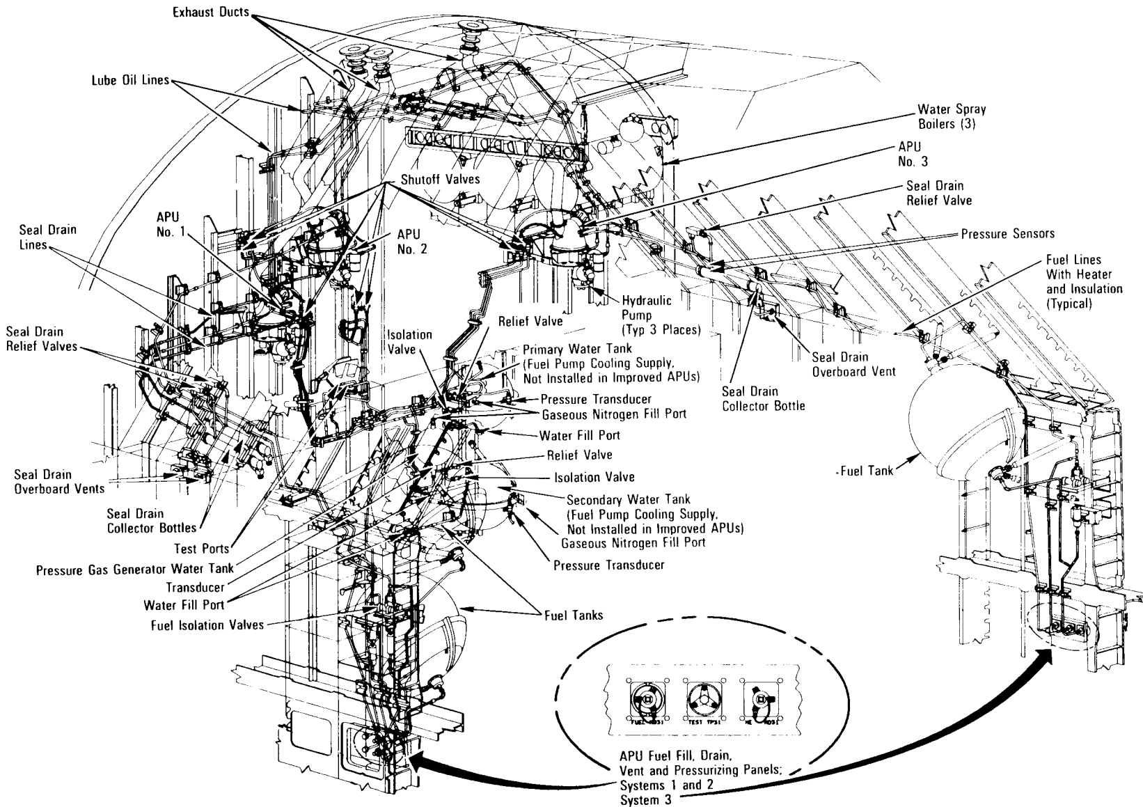
Auxiliary Power Unit/ Water Boilers
