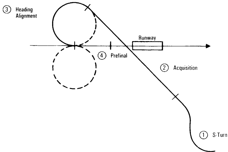
TAEM Guidance Subphases Overhead Approach
