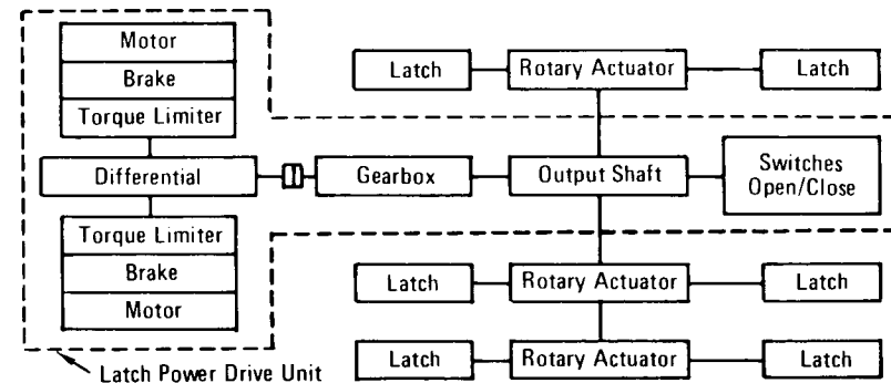
Deployable Radiator Latch System Block Diagram
