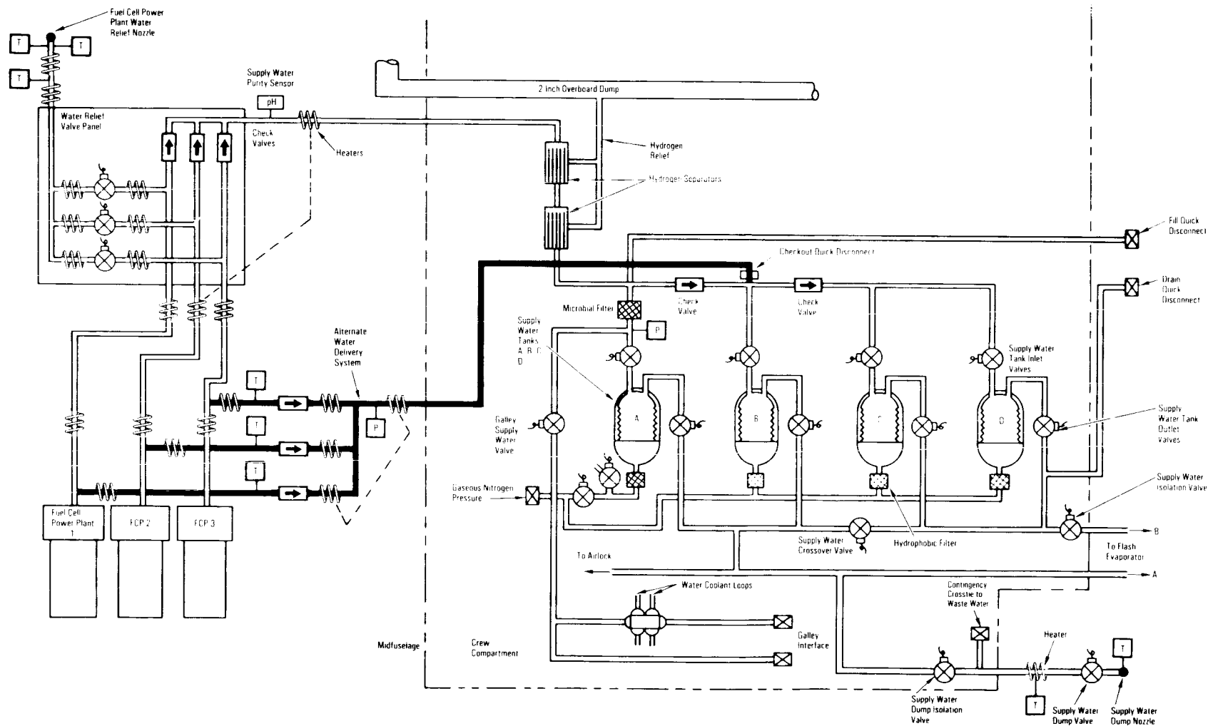
Alternate Water Delivery Systems
