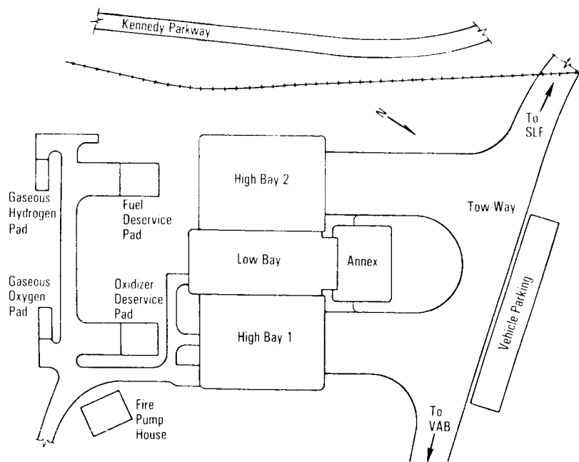
Orbiter Processing Facility
