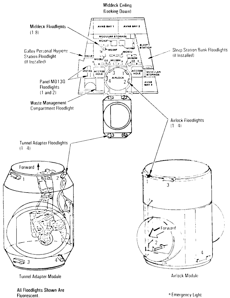
Middeck and Airlock Floodlight Locations
