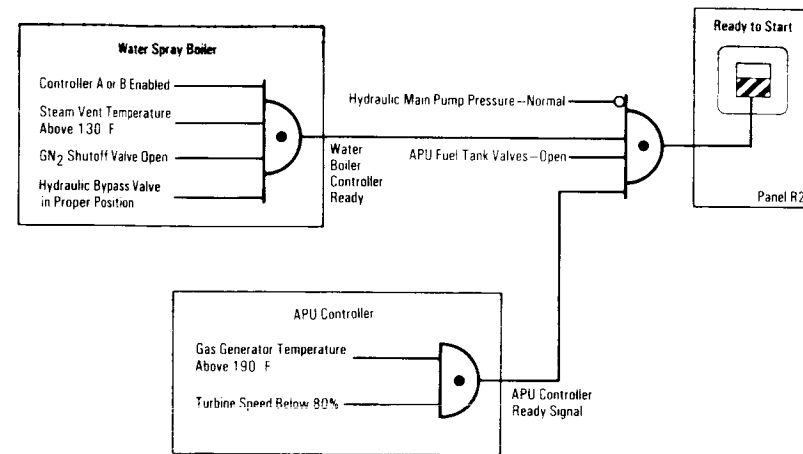
APU Ready-for-Start Talkback Indicator Logic
