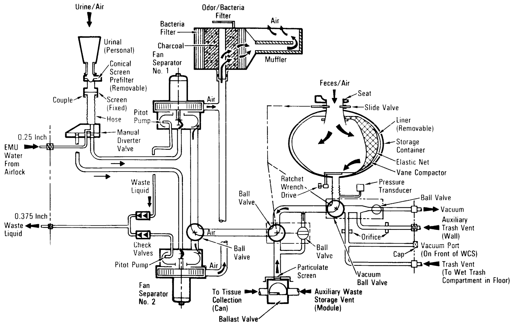
Waste Collection System, Urine/Feces Collection Mode, Handle Forward
