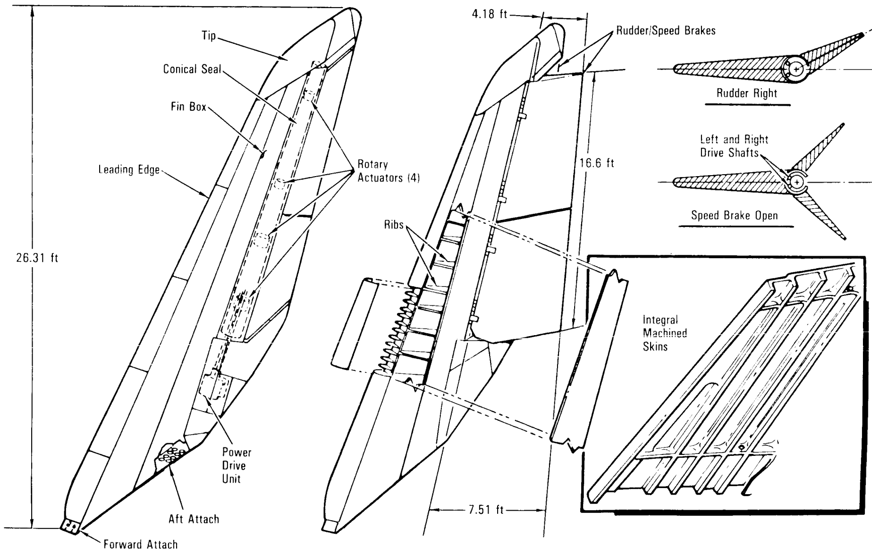
Vertical Tail
