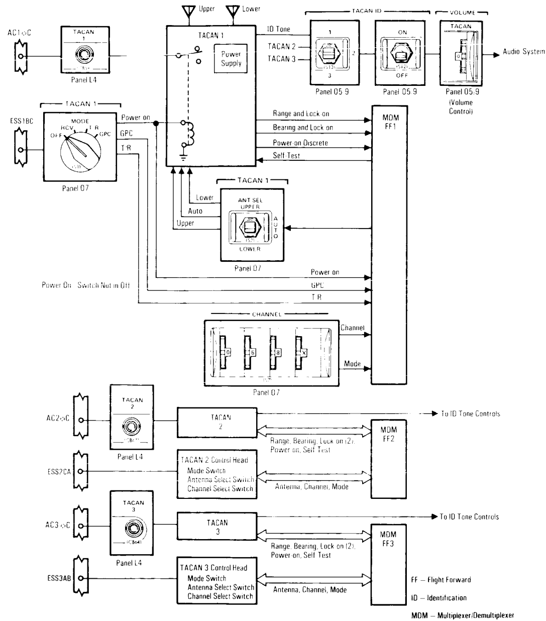
TACAN Power and Data Interfaces
