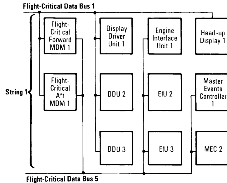
Data Processing System Components of String 1
