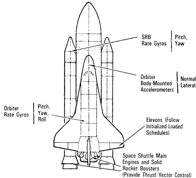
Flight Control Hardware
