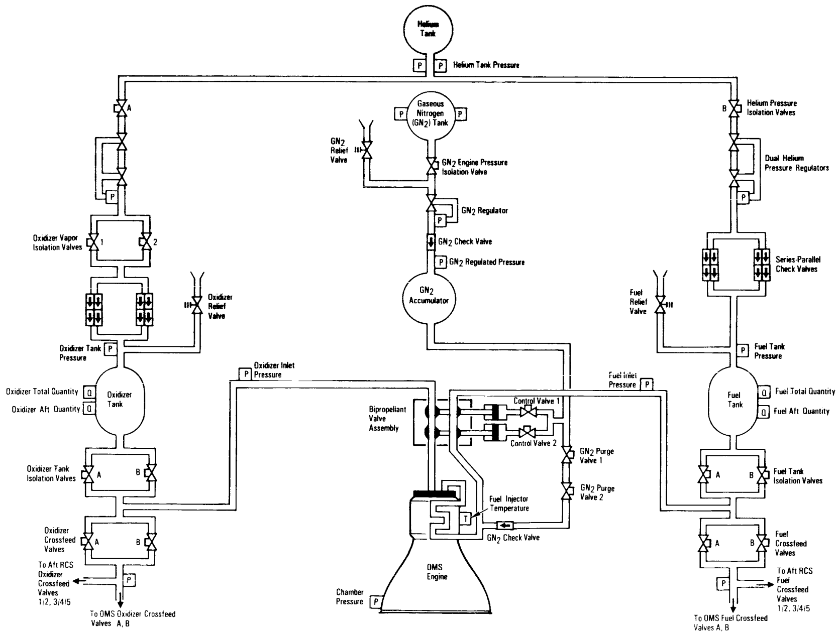
Orbital Maneuvering System Pressurization and Propellant Feed System for One Engine (Other Engine Identical)
