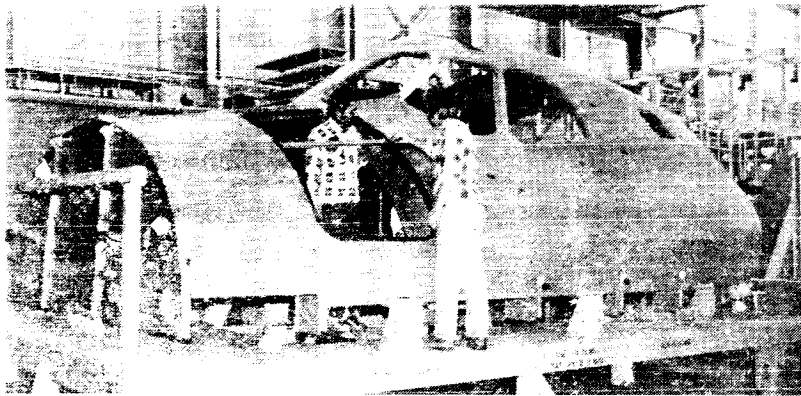
Upper Forward Fuselage
