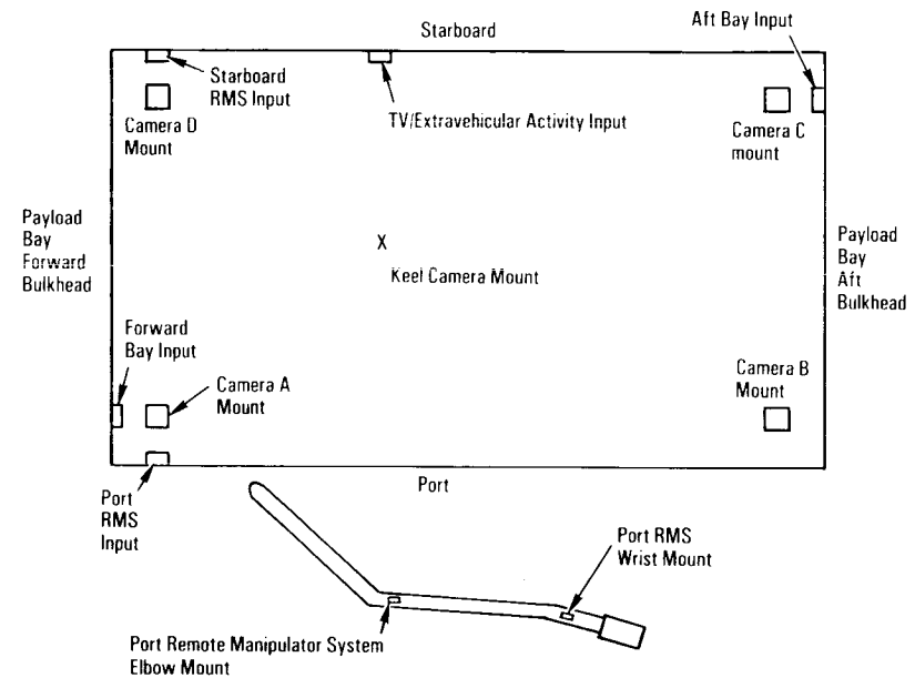
Allowable Closed-Circuit Television Camera Locations in Payload Bay and on Remote Manipulator System
