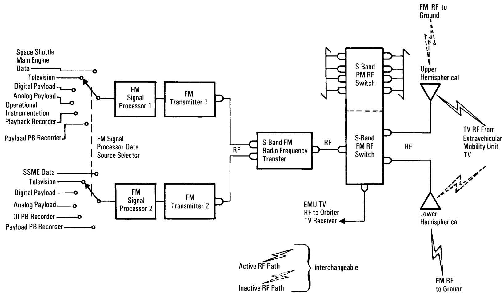
S-Band FM System Block Diagram
