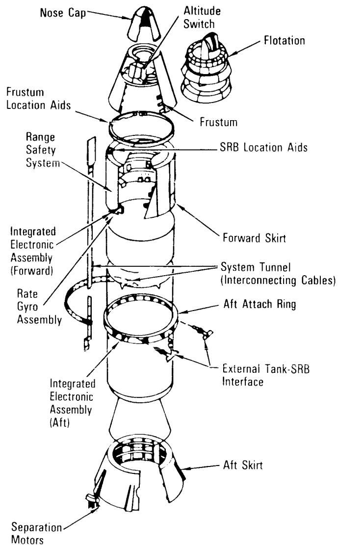
Solid Rocket Booster—Exploded View
