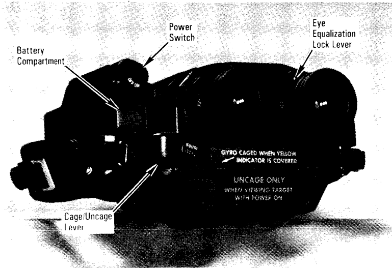
Sighting Aids—14-by-40 Gyro-stabilized Binoculars
