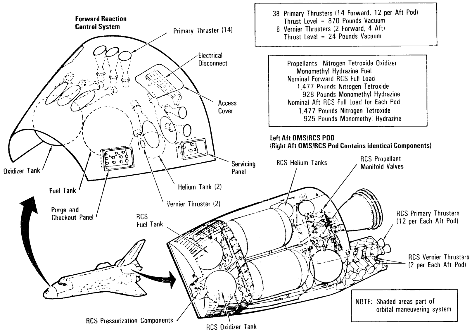
Reaction Control System
