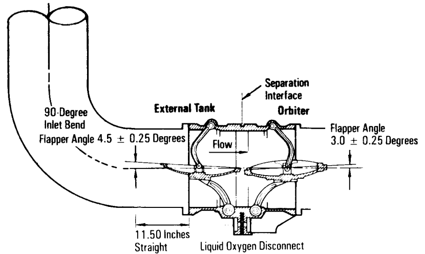
Orbiter / External Tank 17-Inch Liquid Oxygen Disconnect Without Latch Feature
