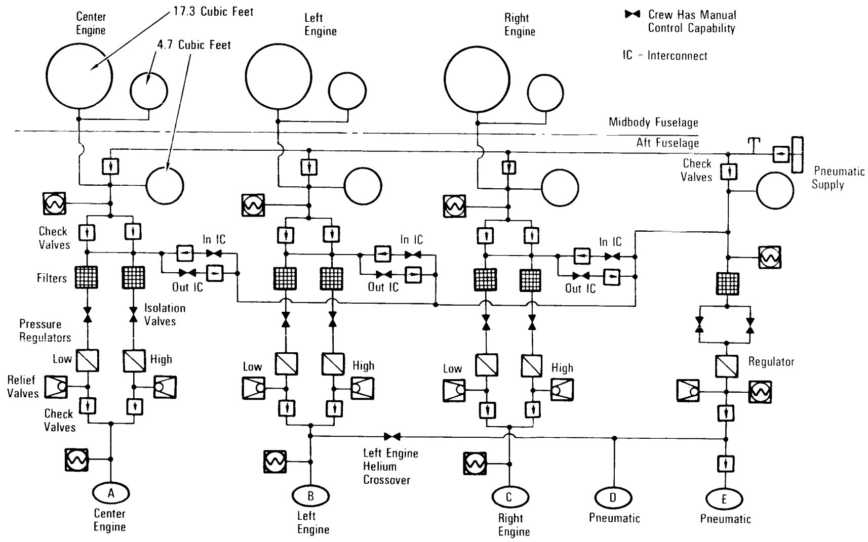
Helium System Storage and Supply
