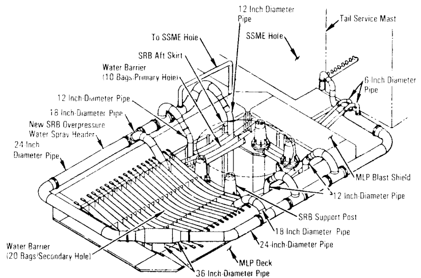
Solid Rocket Booster Overpressure Suppression System
