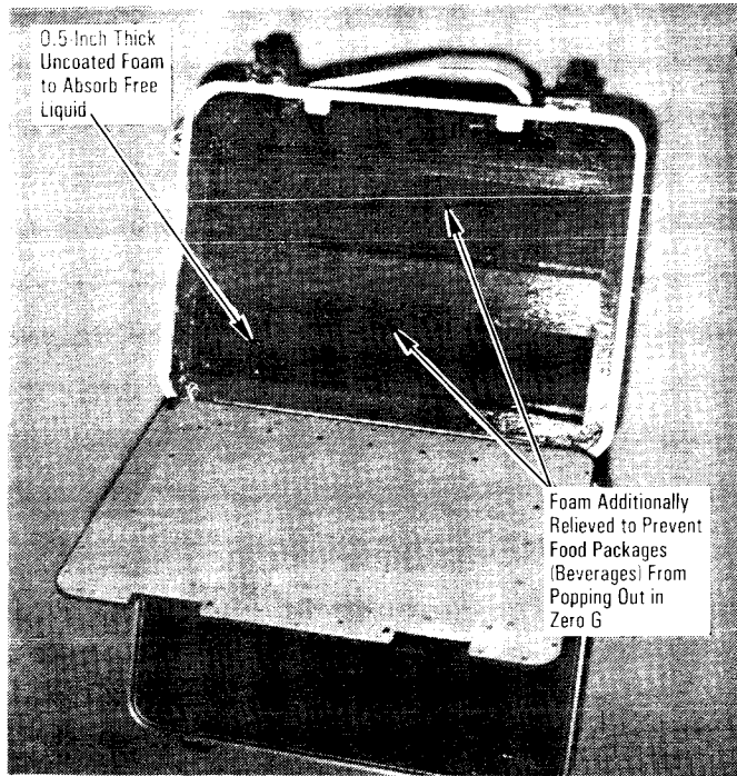
Food Warmer With Both Pouches and Packages
