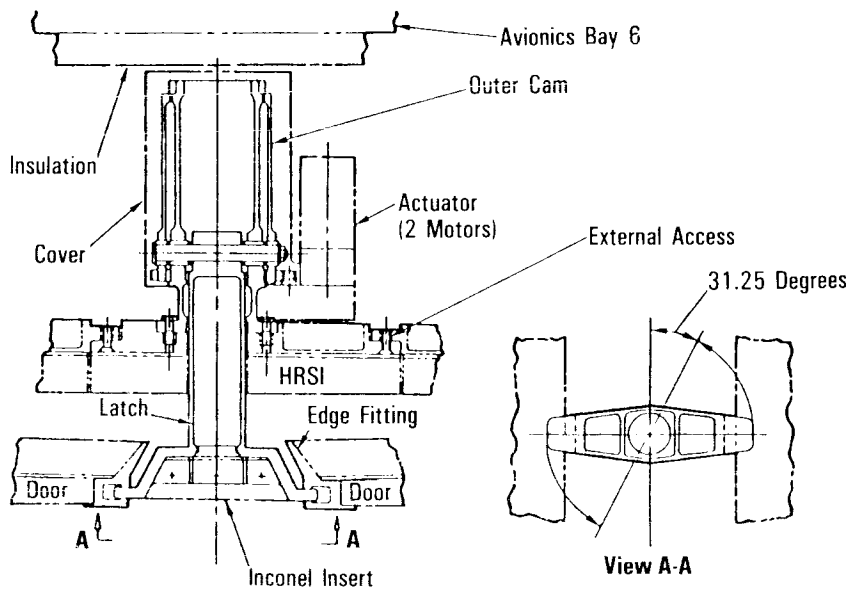
Orbiter/External Tank Umbilical Doors—Centerline Latch
