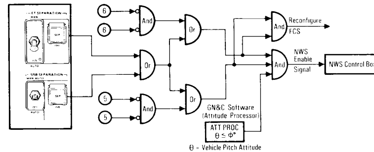
Nose Wheel Steering Enable Signal (Guidance, Navigation and Control Software)
