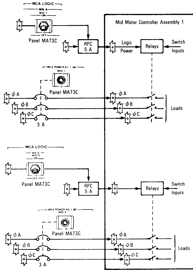
Mid Motor Controller Assembly
