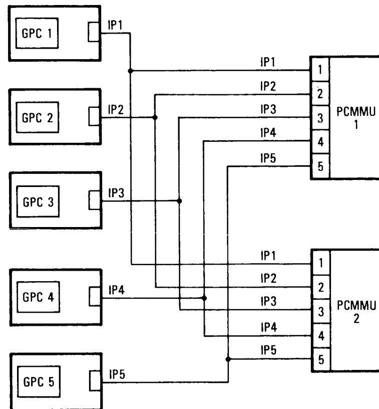
Instrumentation/Pulse Code Modulation Master Unit Computer Data Bus Interface
