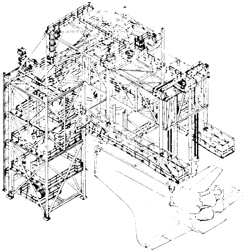
Mate/Demate Device Exterior View
