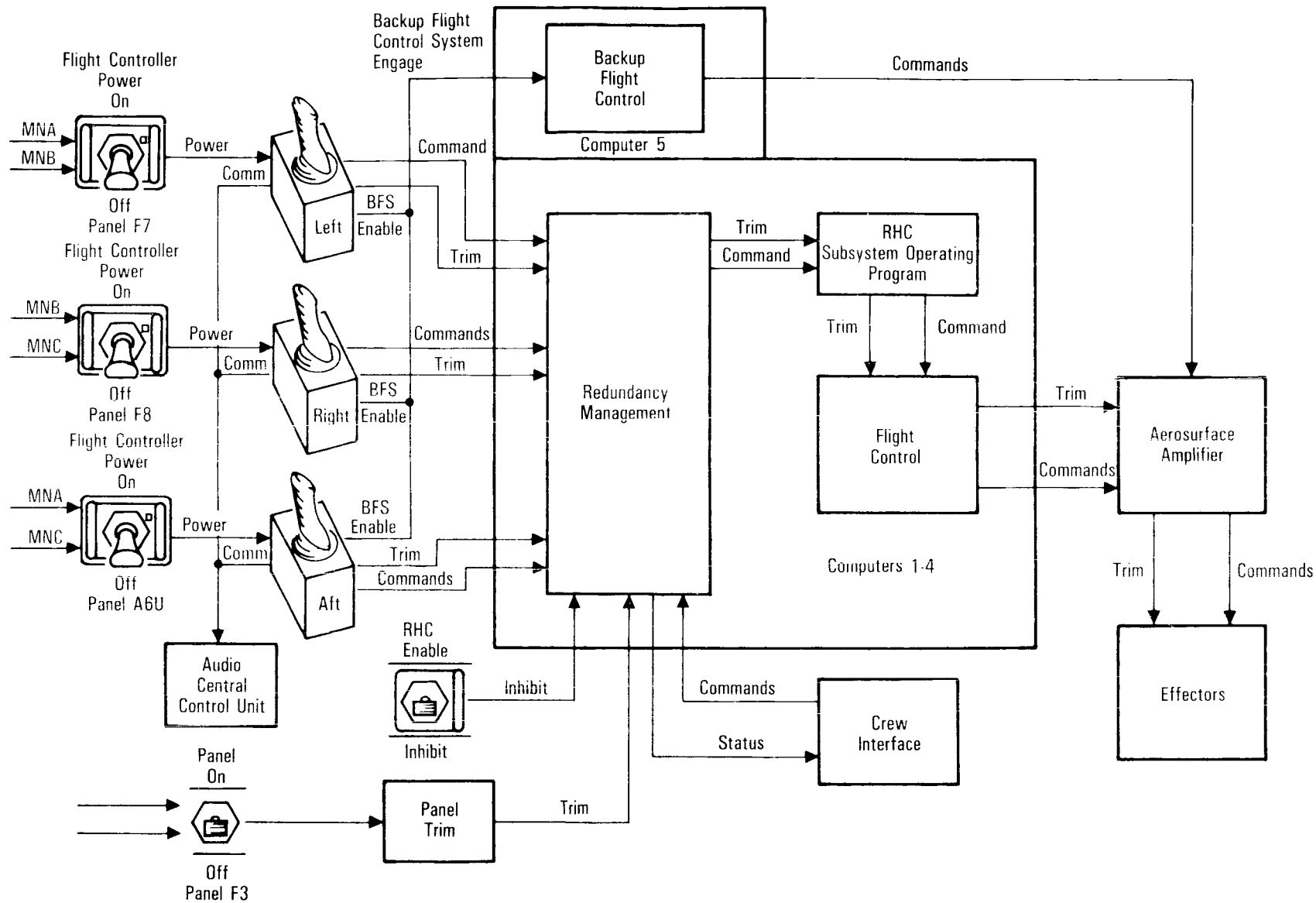
Rotational Hand Controller
