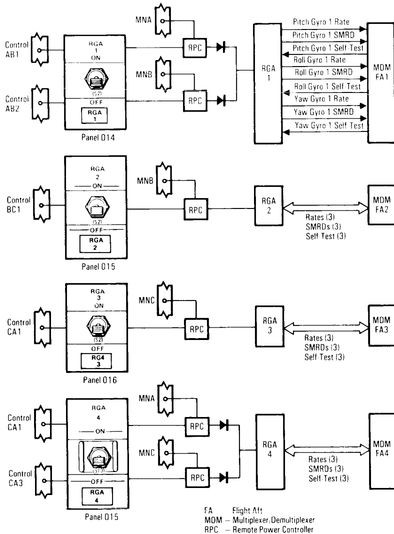
Rate Gyro Assembly Power and Data Interfaces
