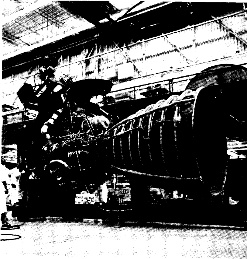
MPS Interfaces With Other Vehicle Systems
