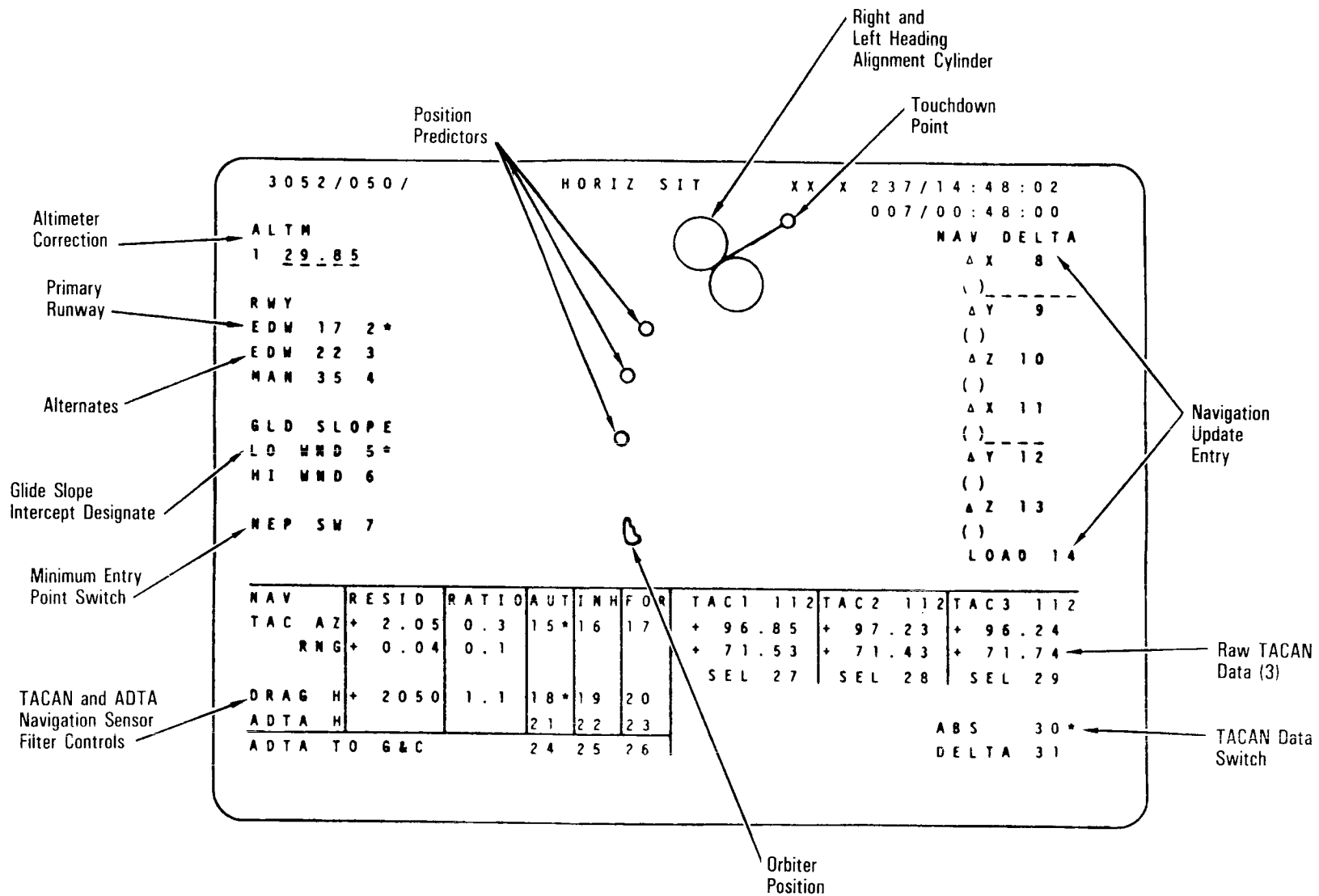
Horizontal Situation Display
