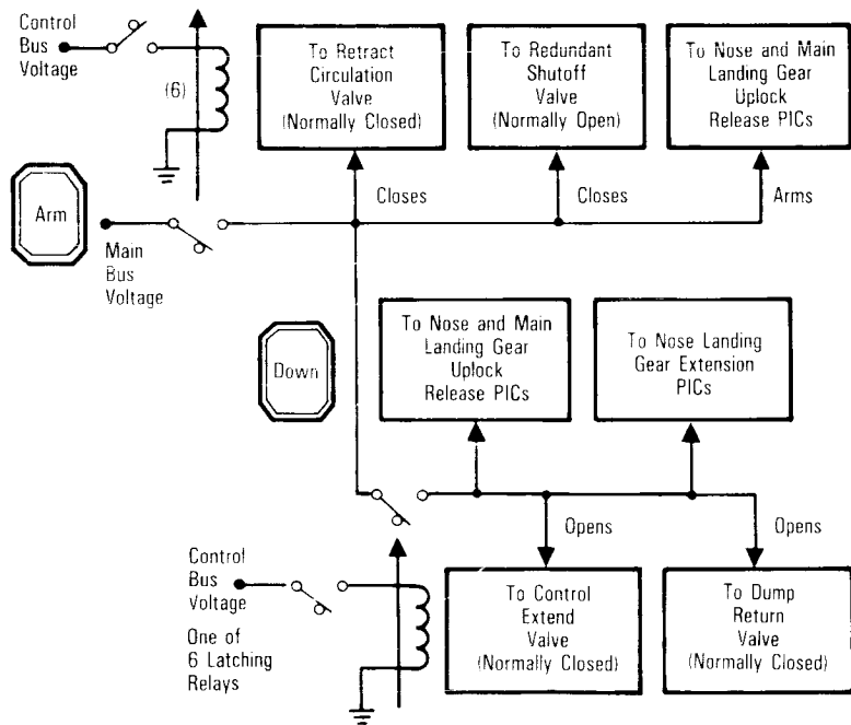
Arm/Down Circuit
