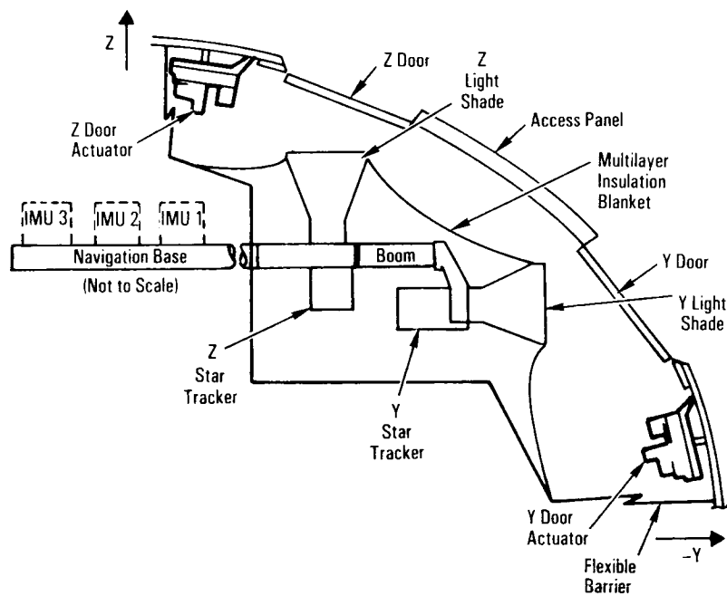
Internal View of Tracker Subsystem (Looking Aft)
