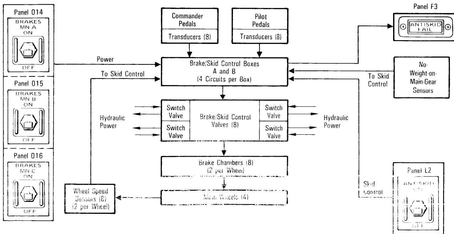
Brake/Skid Control System Overview
