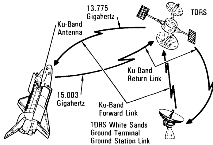
NASA Ku-Band Communication With TDRS and WSGT and Mission Control Center-Houston
