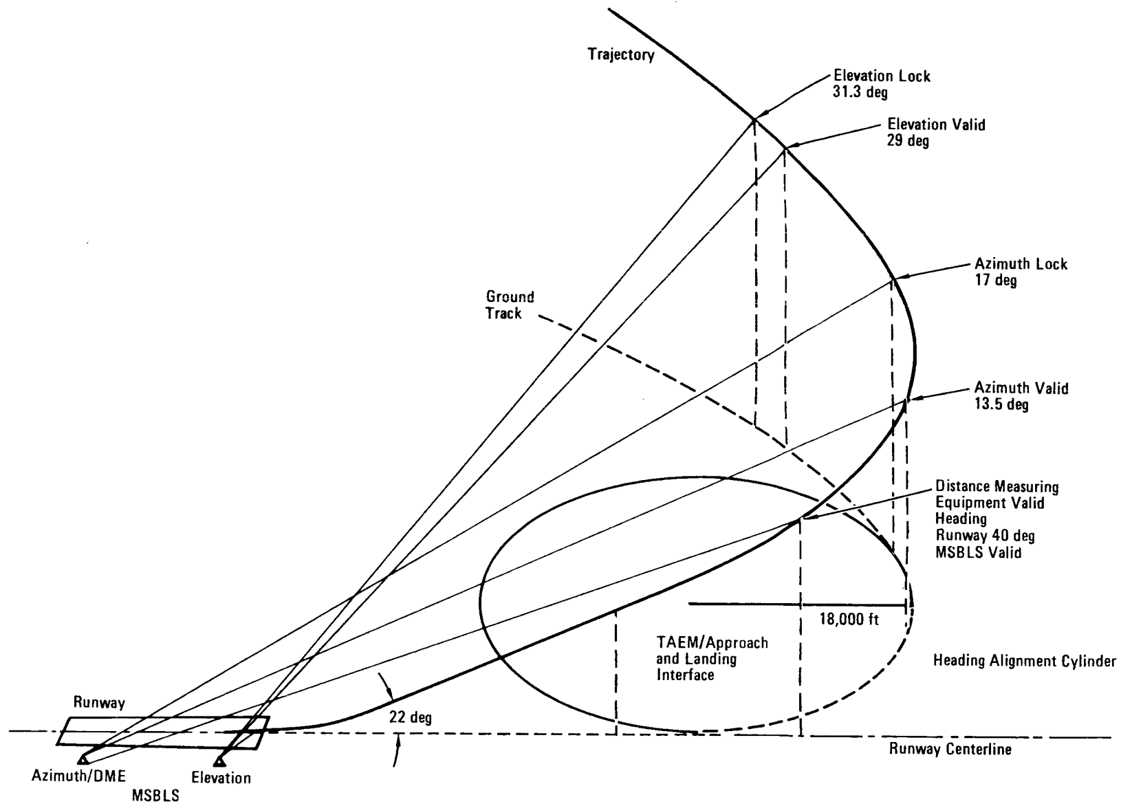
Microwave Scan Beam Landing System
