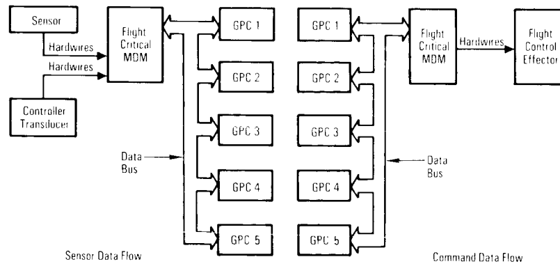
Data and Command Interfaces
