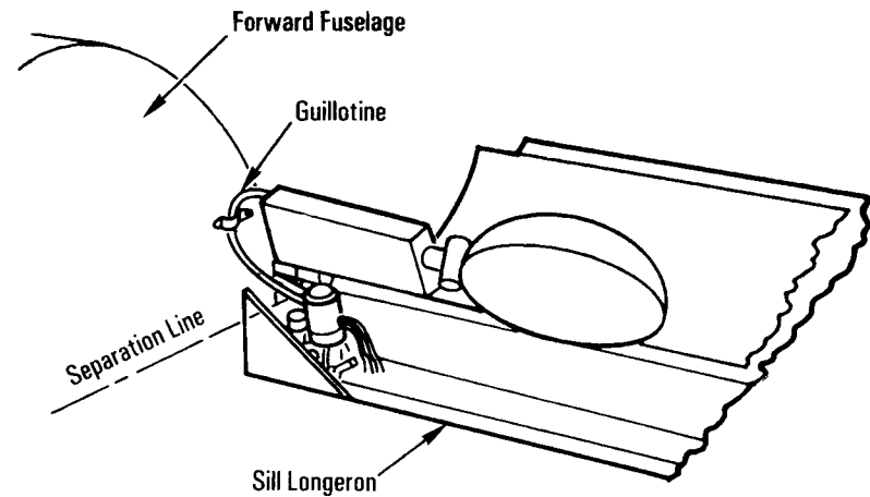
Ku-Band Antenna Jettison Separation
