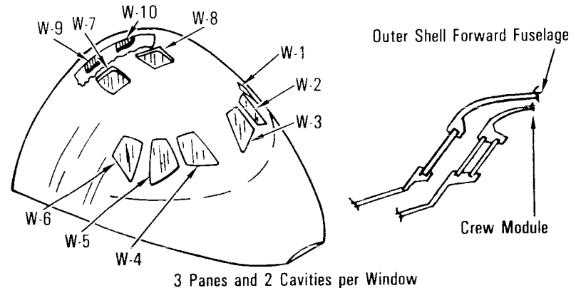
3 Panes and 2 Cavities per Window
