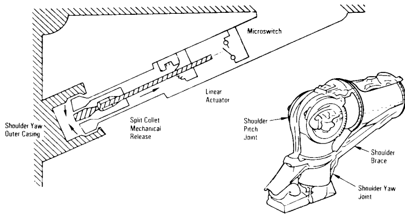
Shoulder Brace
