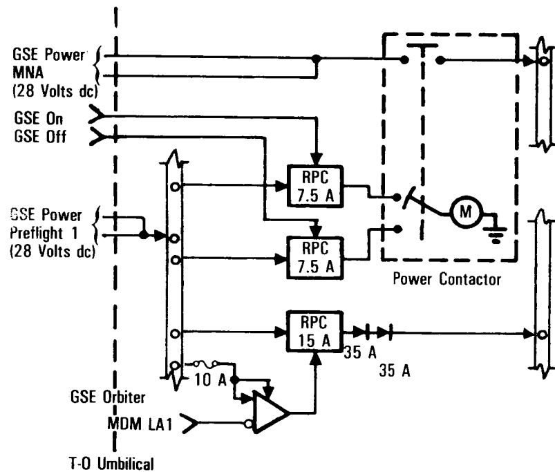
Orbiter and GSE Power Interface (MNA Only)
