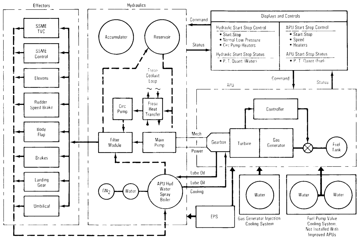
Auxiliary Power Unit, Water Spray Boiler and Hydraulic System
