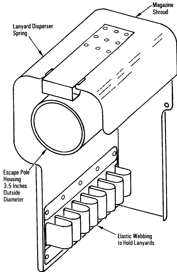
Escape Pole Magazine Assembly
