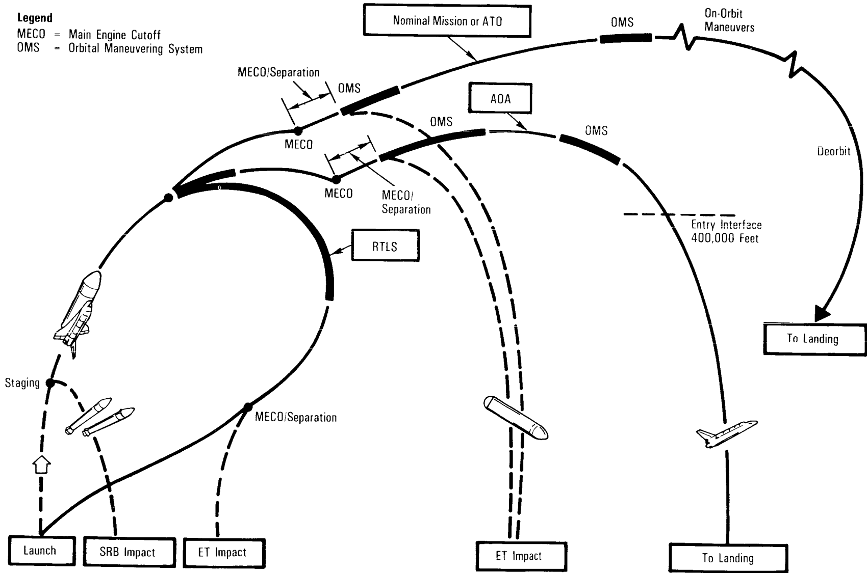
Abort and Normal Mission Profile
