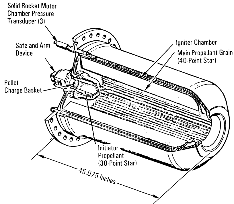
Solid Rocket Motor Igniter
