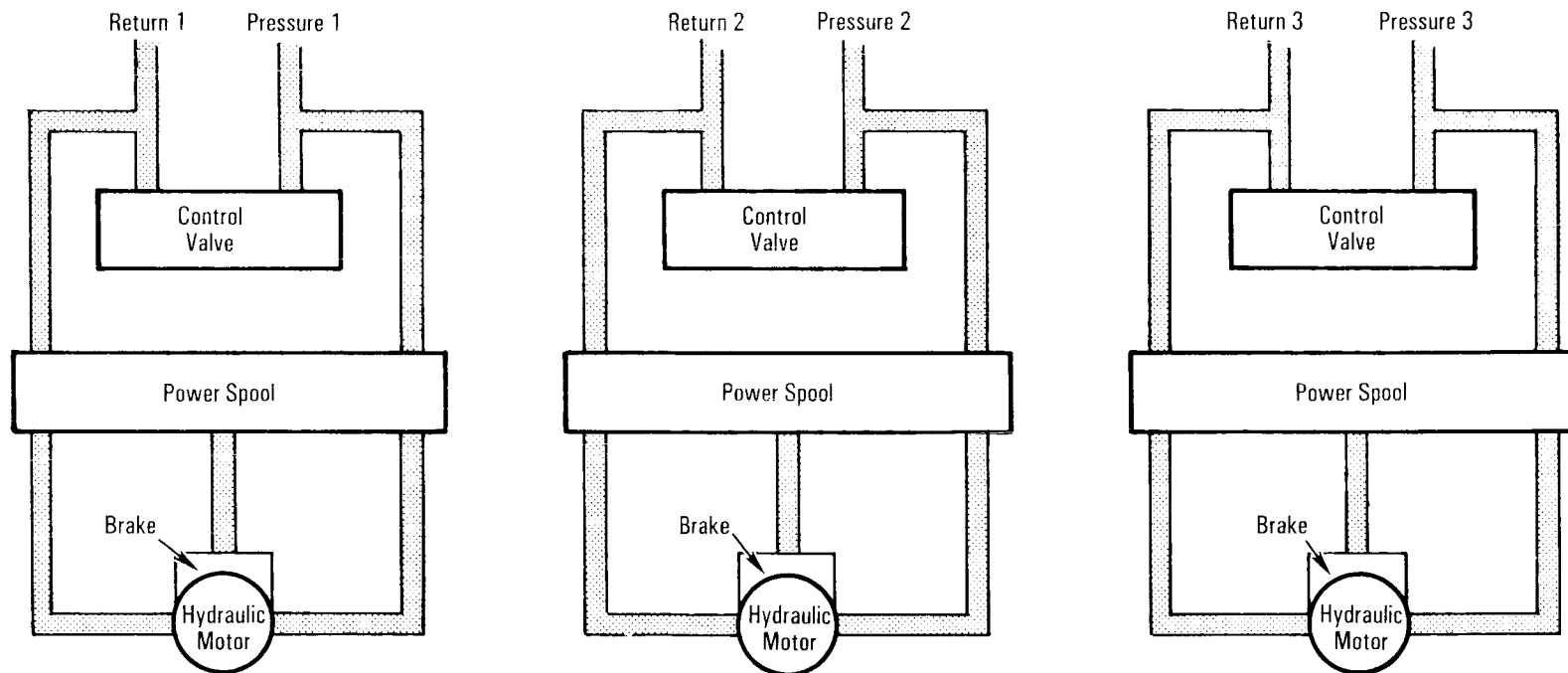
Body Flap Actuator Hydraulic Supply
