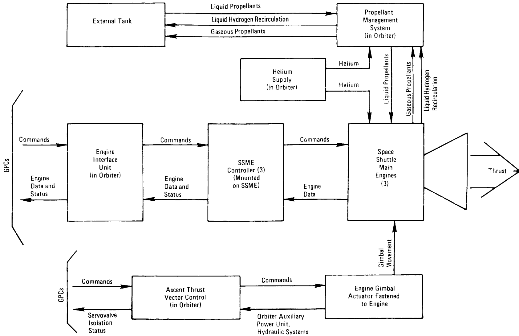
MPS Subsystem
