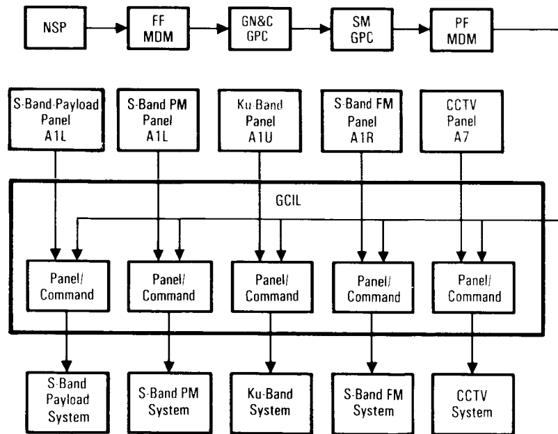
Ground Command Interface Logic (Controller)
