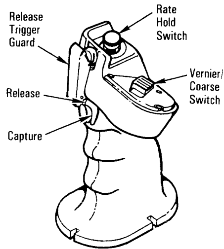
RMS Rotational Hand Controller Switches
