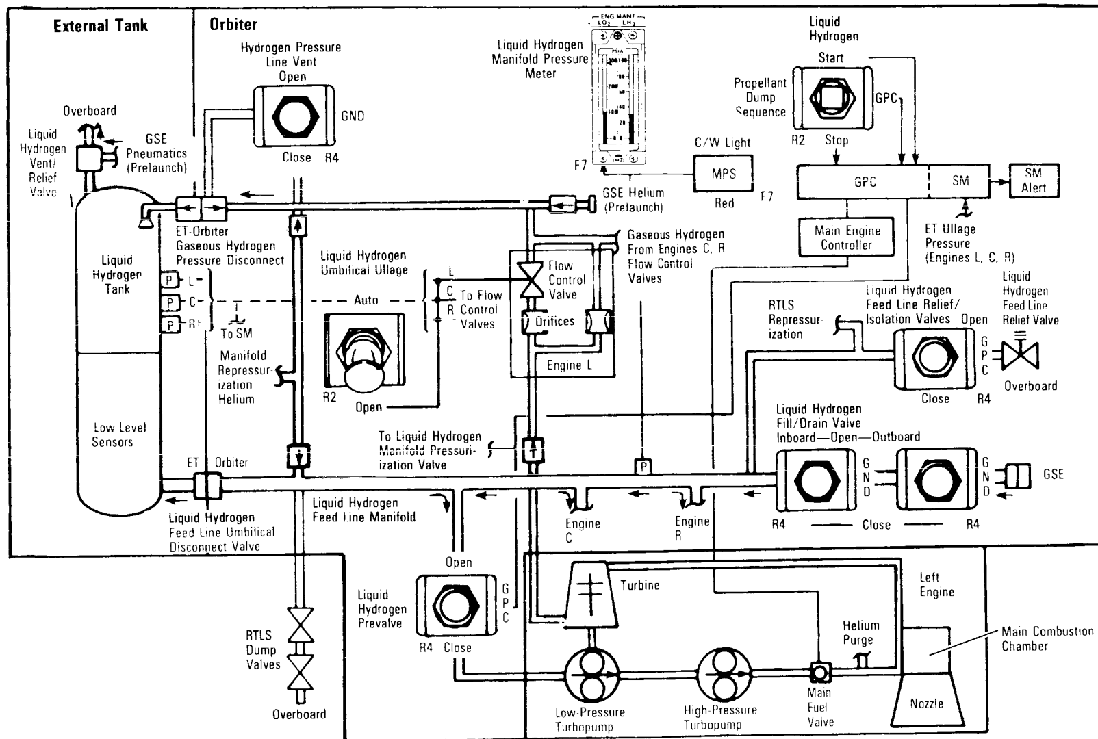
Fuel Flow
