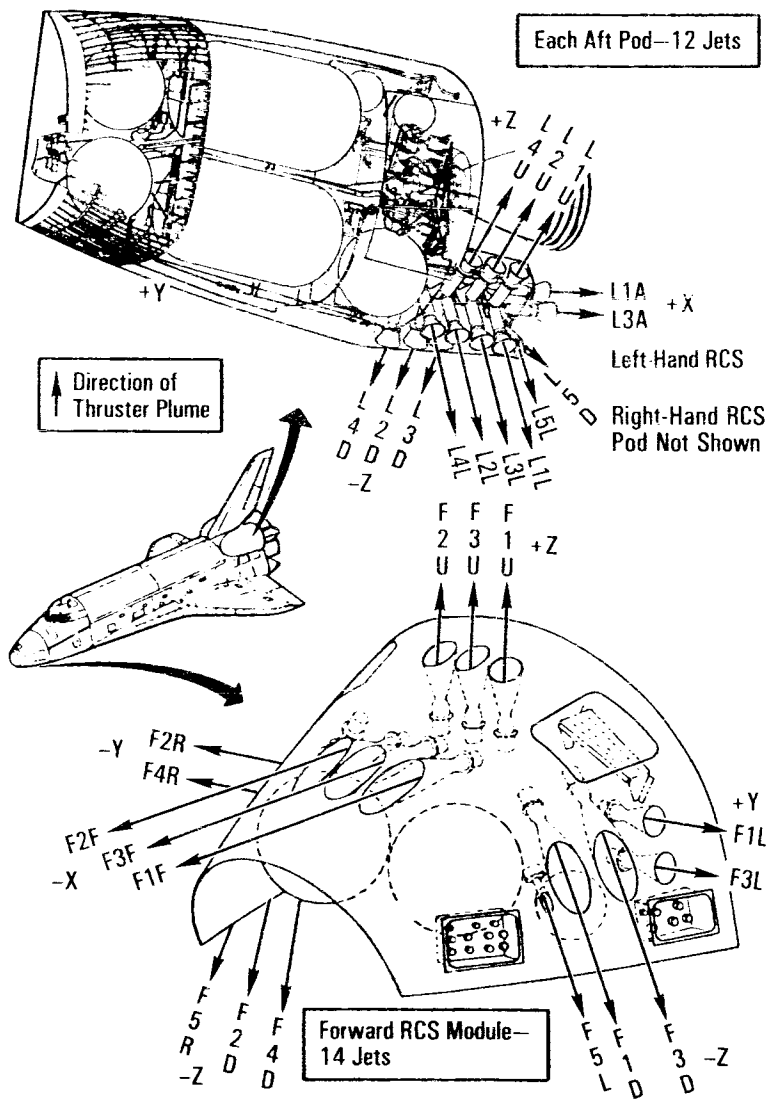
Reaction Control System Engine Location and Identification
