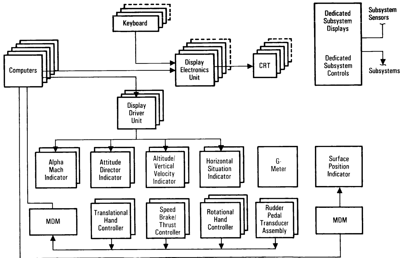
Dedicated Display and Control System
