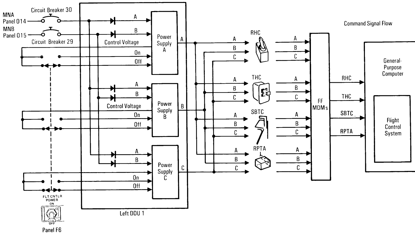
Flight Controller Power Distribution—Commander
