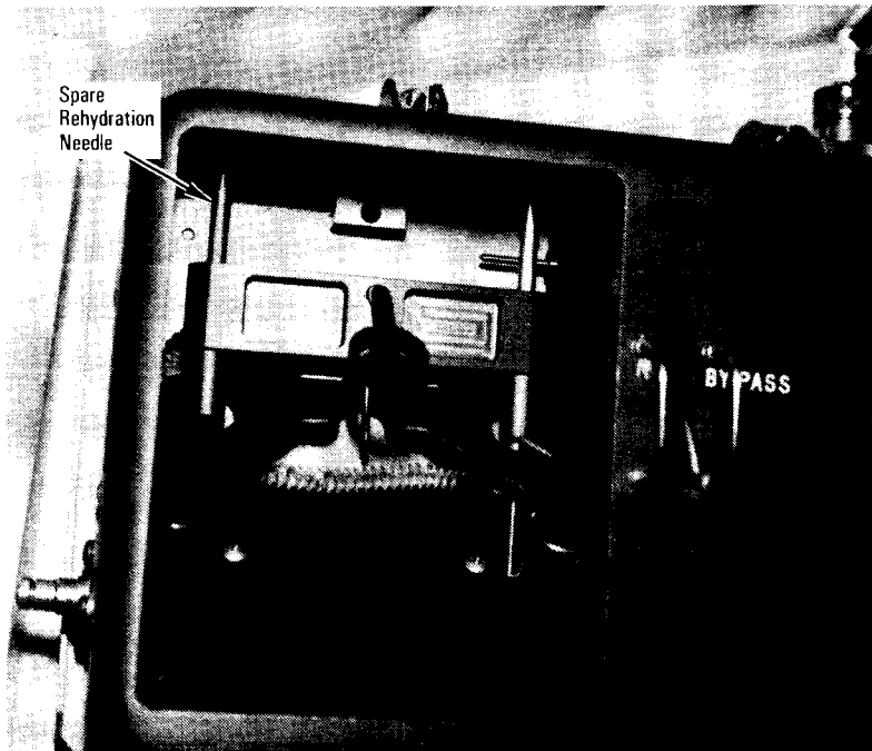
Water Dispenser
