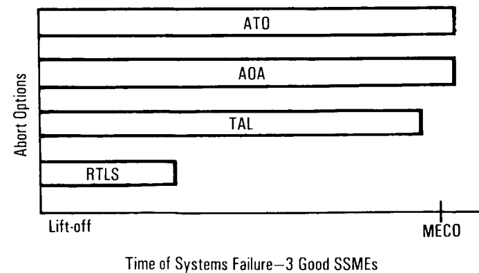
Abort Mode Options With Three Good SSMEs
