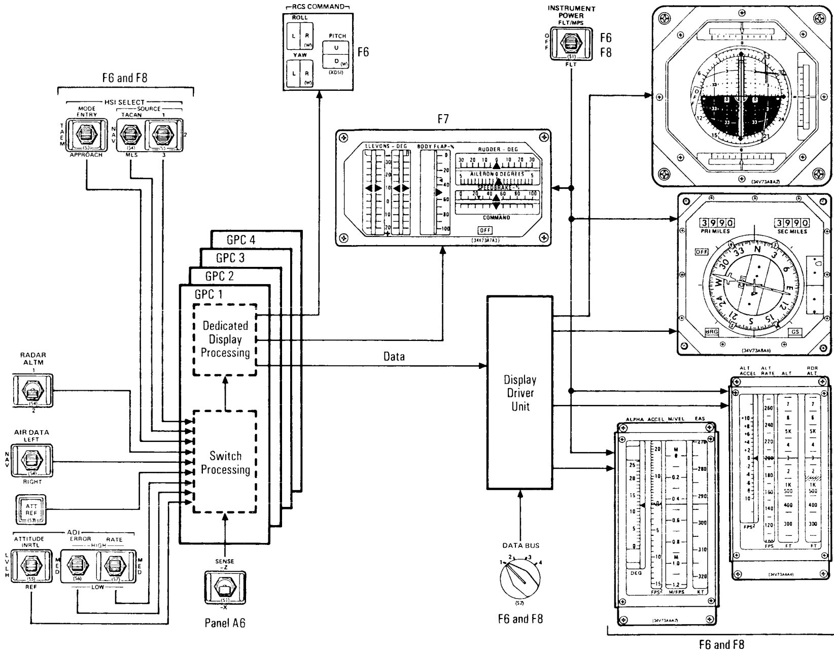
Dedicated Display System General Data Flow
