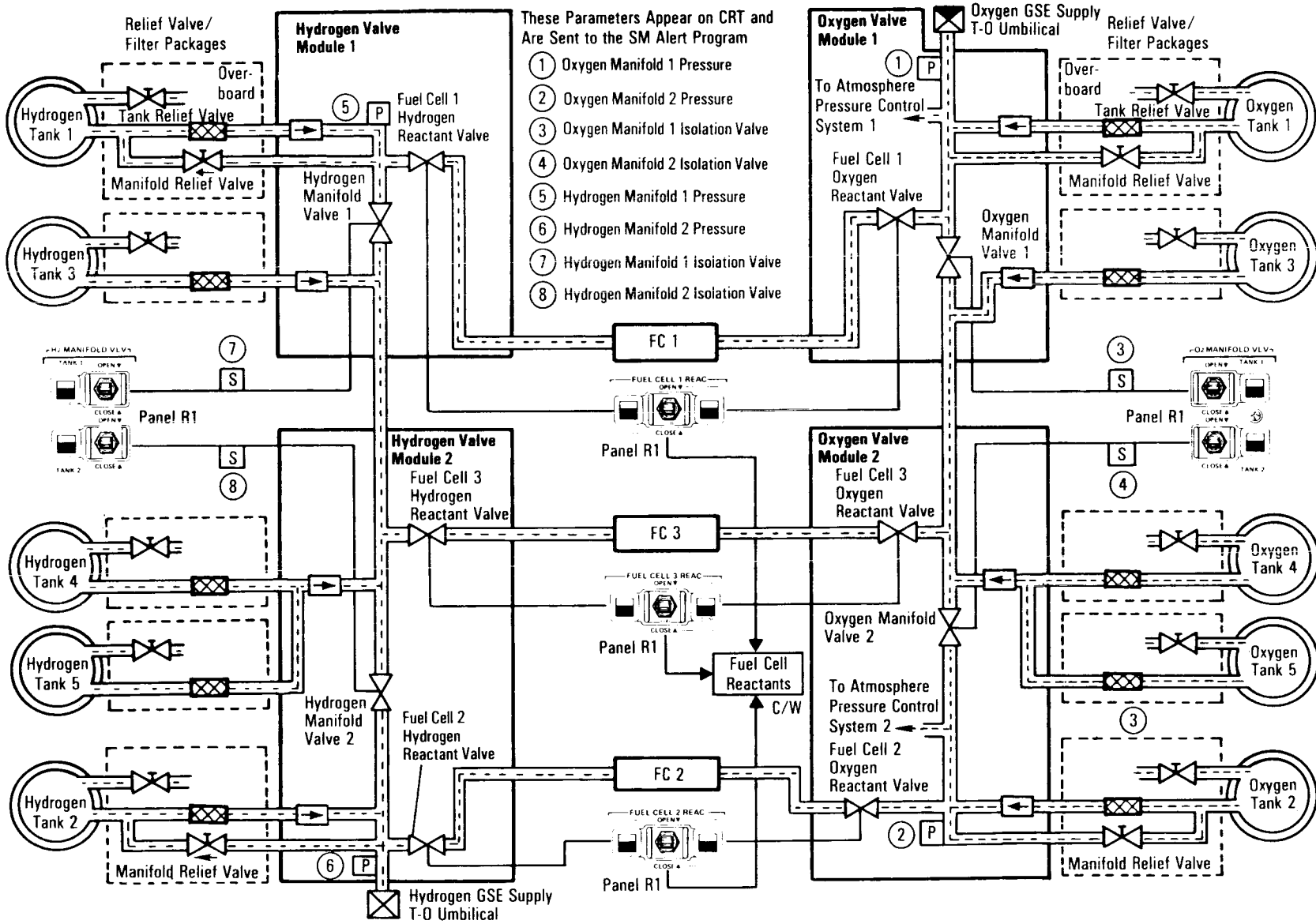
Cryogenic Oxygen / Hydrogen Power Reactant Storage and Distribution System, Fuel Cell Reactants
