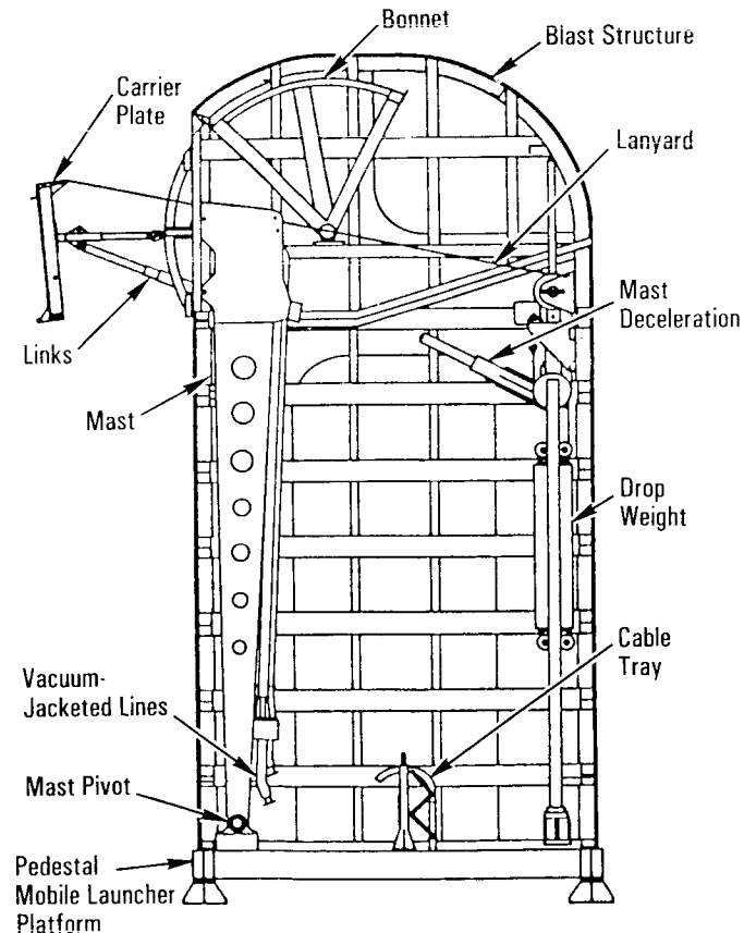
Tail Service Mast, Interior Details
