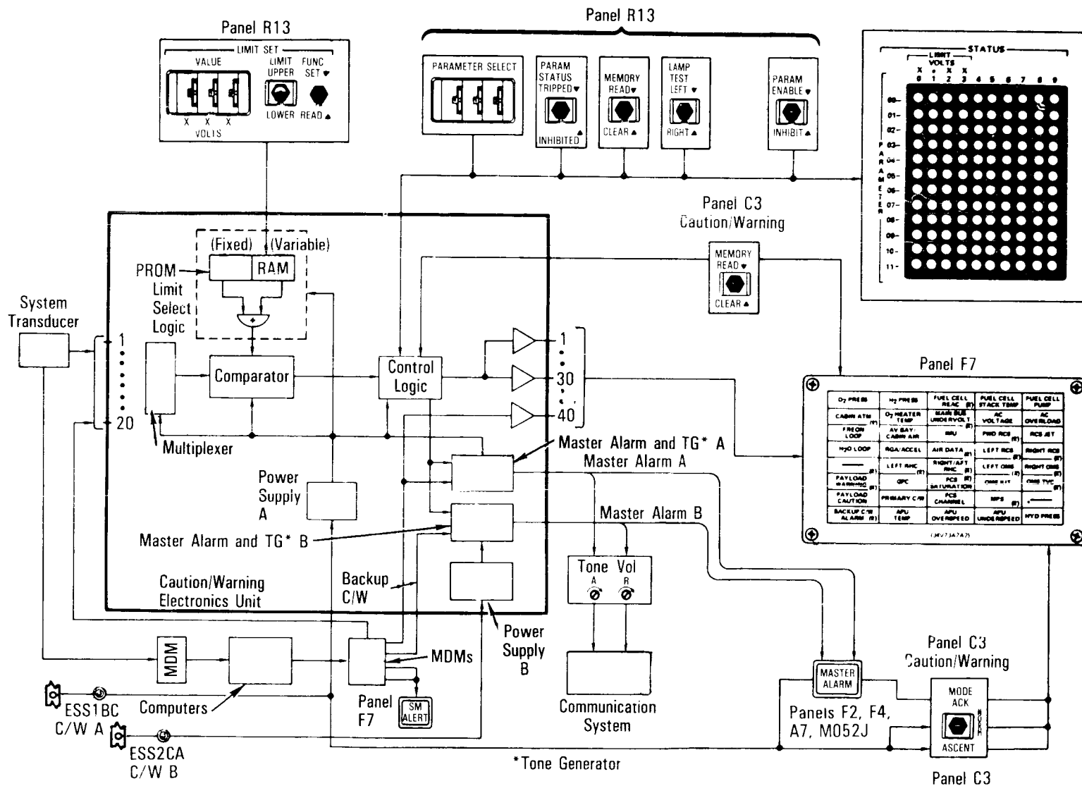
Caution and Warning System Overview
