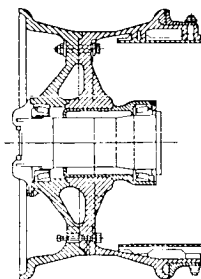
Roll-on-Rim
