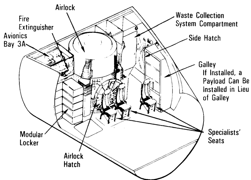
Crew Compartment Middeck
