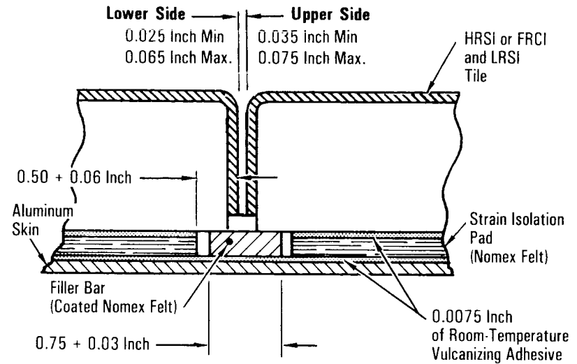
HRSI or FRCI and LRSI Tile Interface
