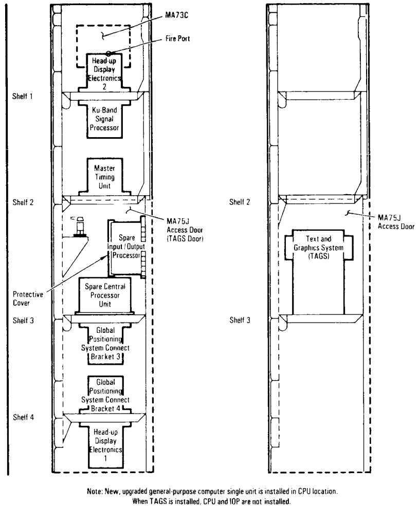
Component Locations—Bay 3B
