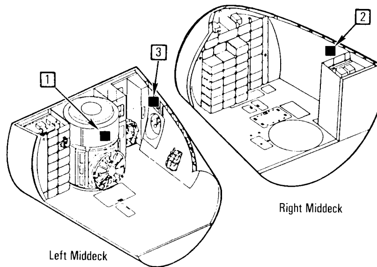
Passive Dosimeter Locations in Crew Compartment
