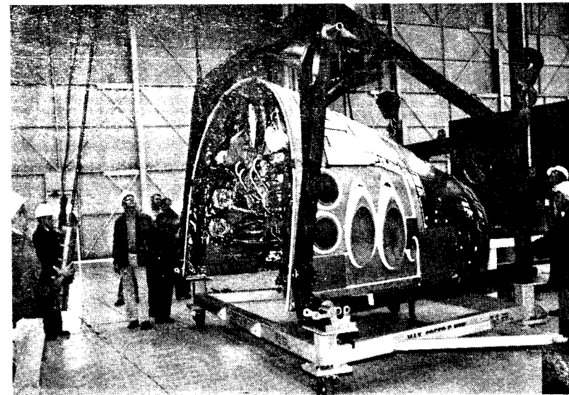
Forward RCS Module
