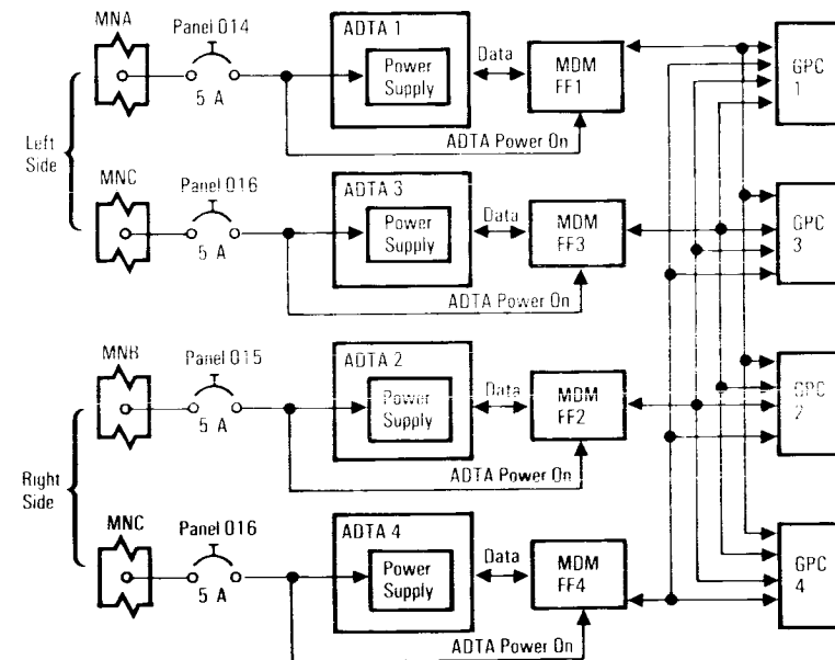
Air Data Transducer Assembly Power Interface Functional Block Diagram
