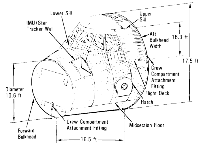
Crew Compartment
