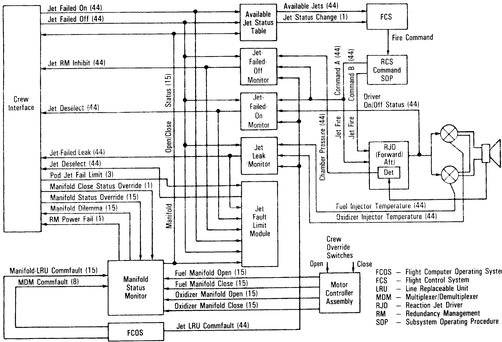
Reaction Control System Redundancy Management
