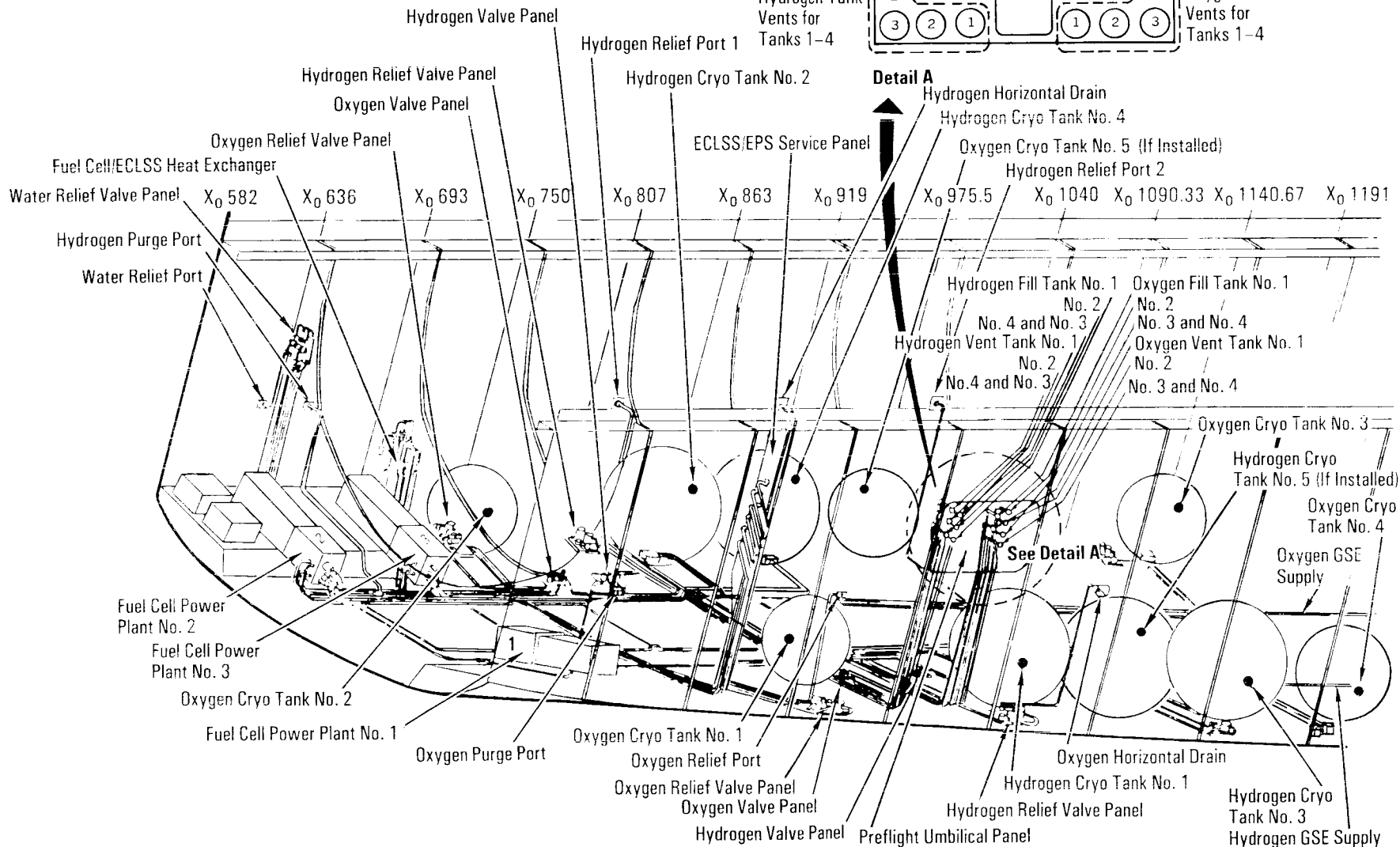
Power Reactant Storage and Distribution System
