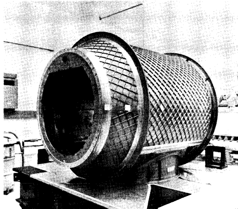
Tunnel Adapter
