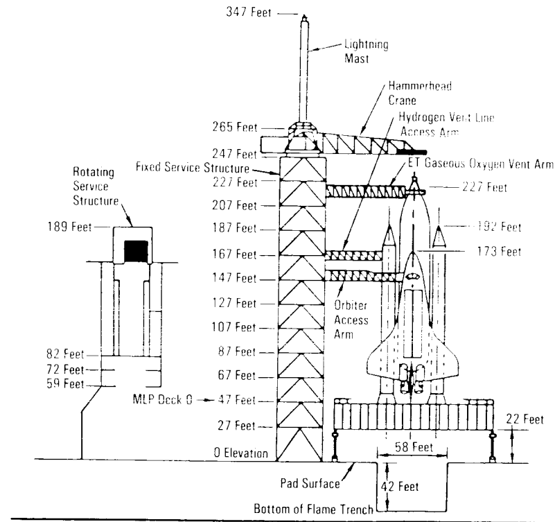
Space Shuttle/Pad Elevations
