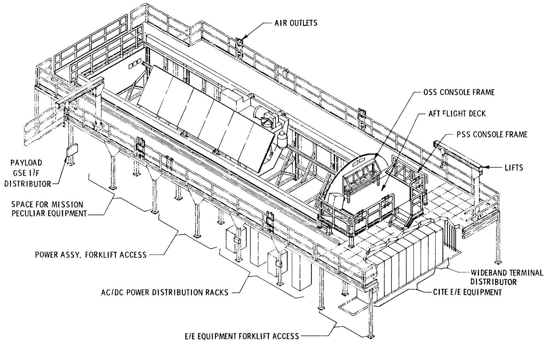
Horizontal Cargo Integration Test Equipment Stand
