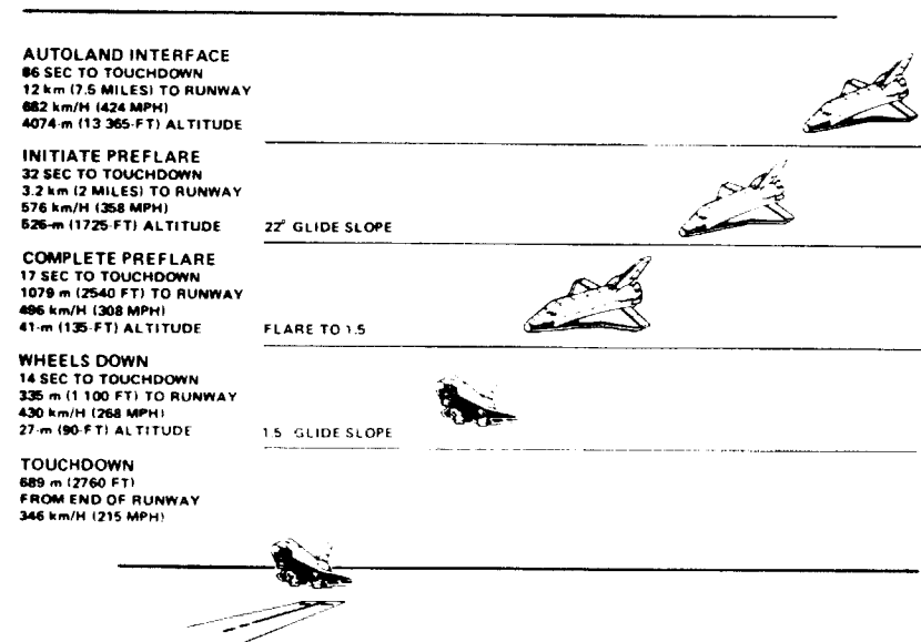
Autoland Interface to Touchdown Events
