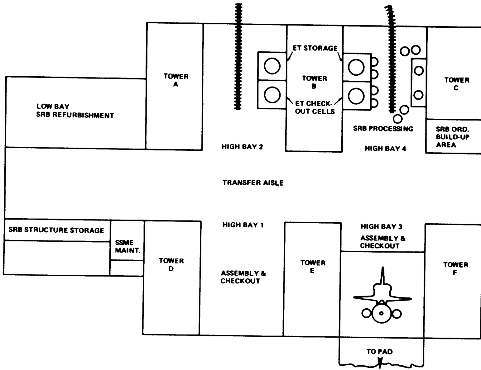
Vehicle Assembly Building Floor Plan
