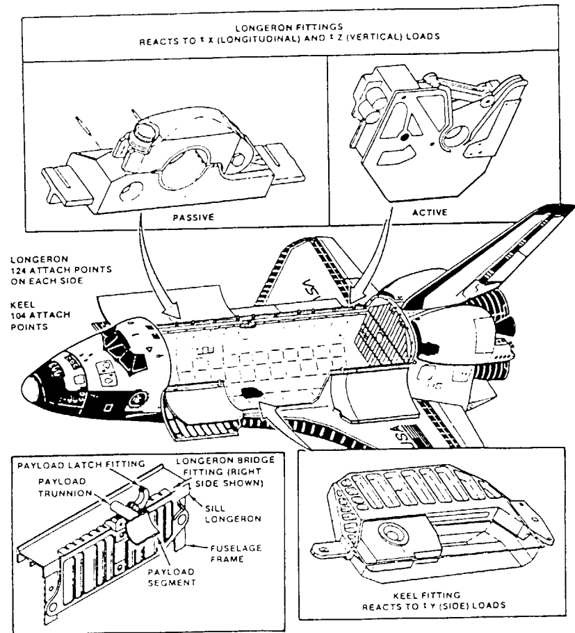
Attach fittings for payload
