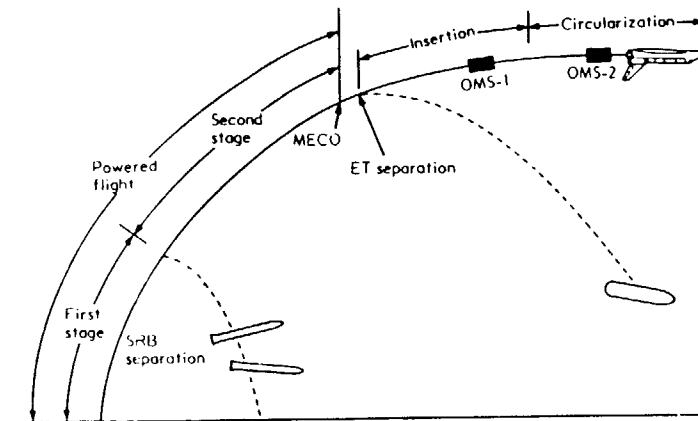
Space Shuttle Nominal Ascent Profile
