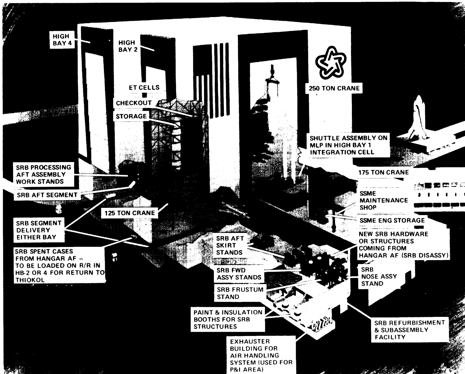
Vehicle Assembly Building cut away view
