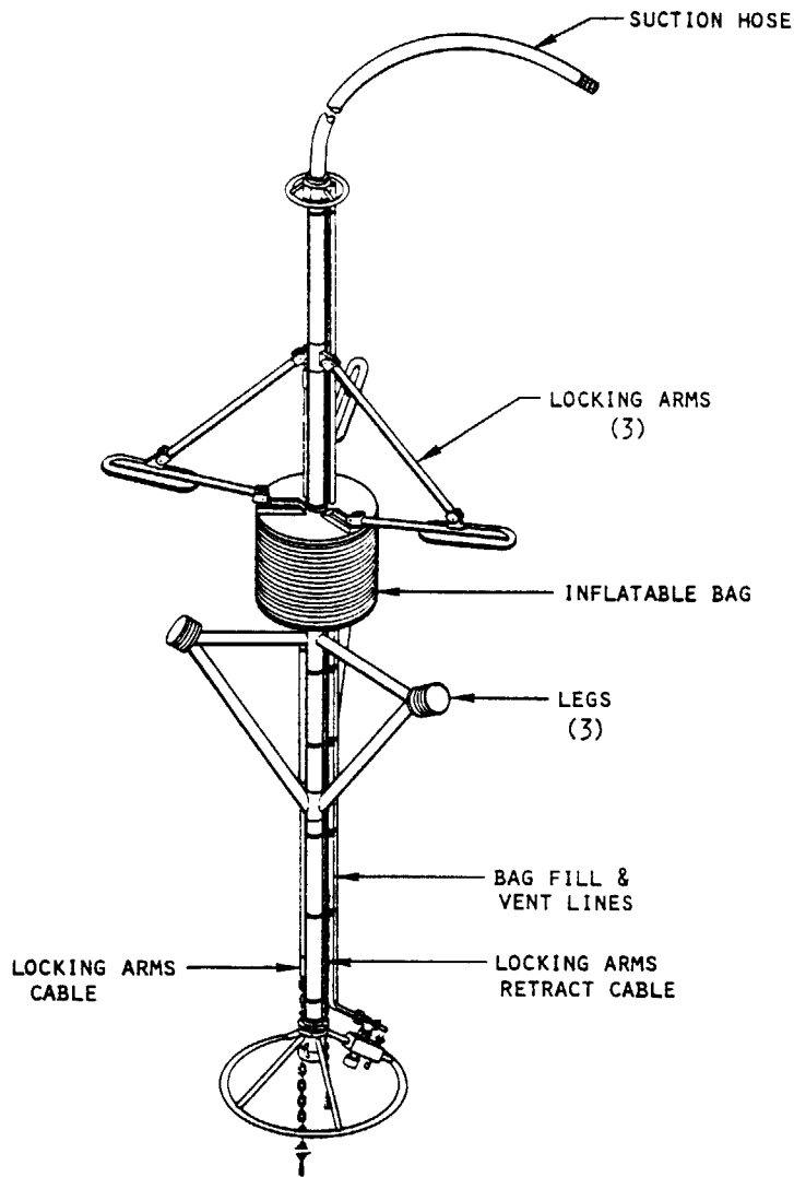
Diver Operated Plug
