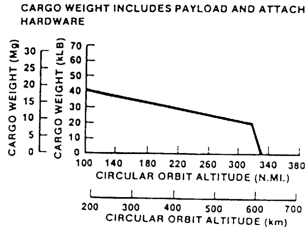
Cargo capability (57 degree inclination)
