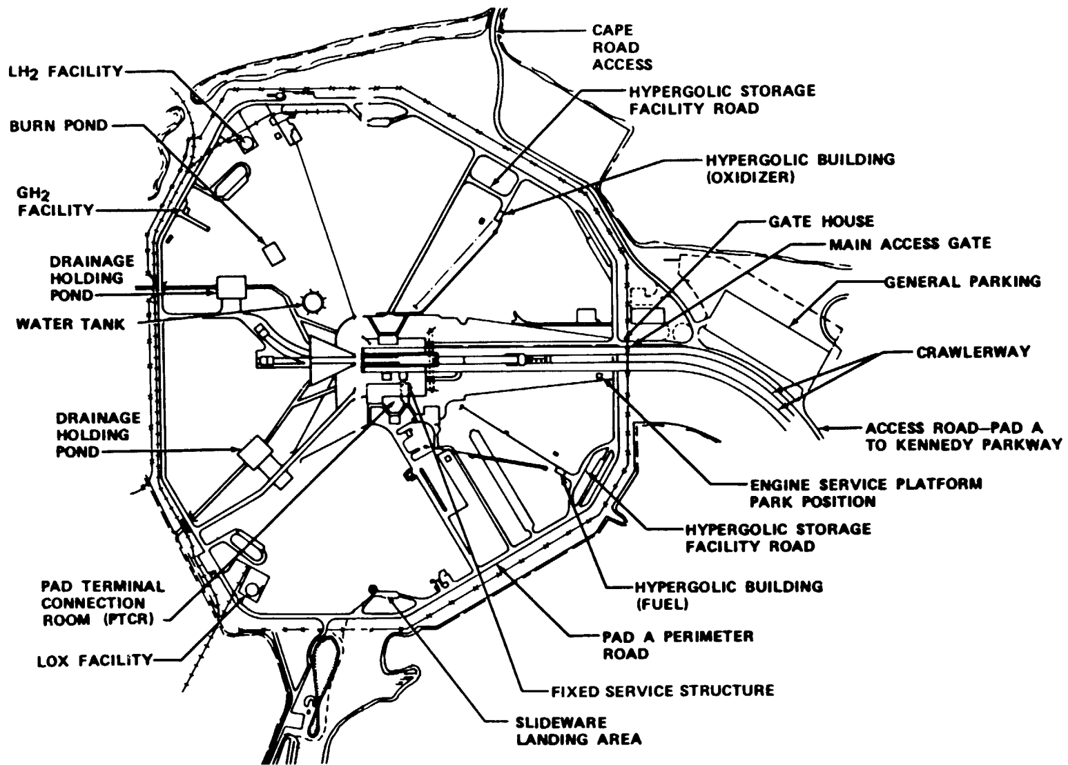
Launch Pad Facilities
