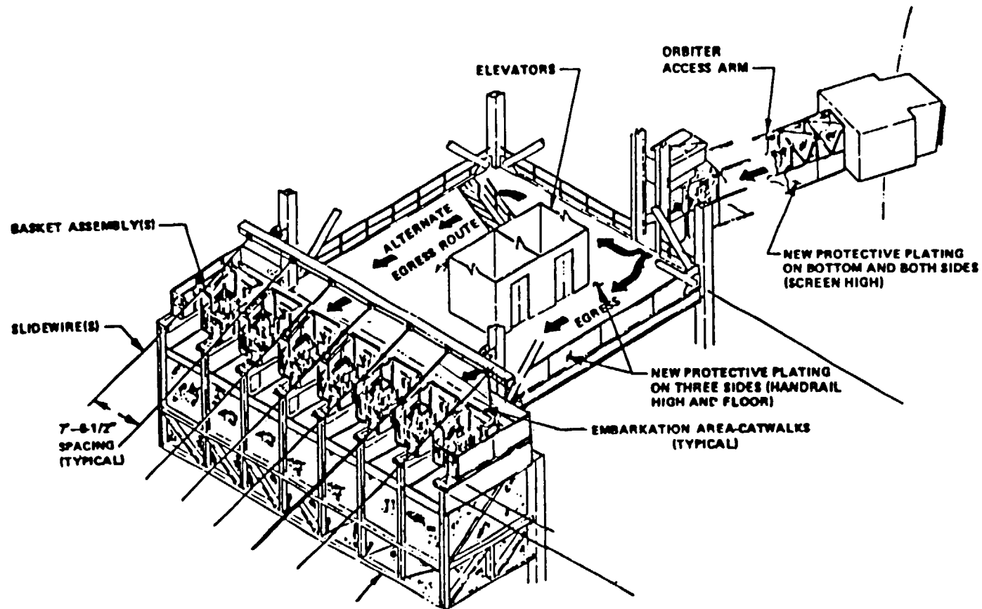
Emergency Exit System
