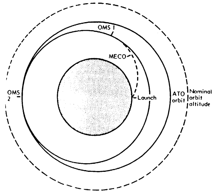
Abort Once Around (AOA) Abort Profile
