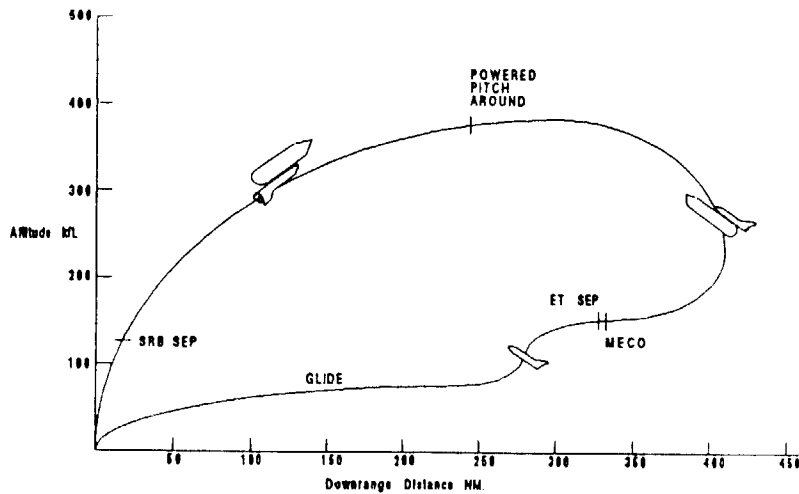
Return to Launch Site (RTL) Abort Profile
