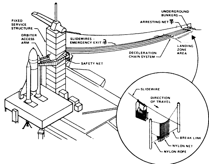
Overall View of Emergency Exit System
