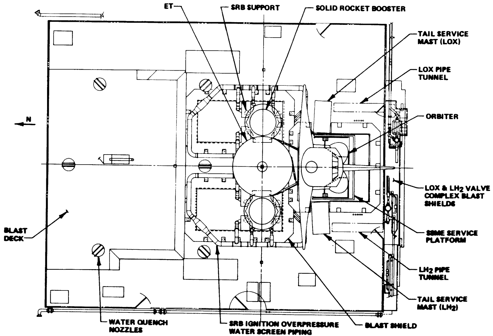
Mobile Launch Platform Floor Plan
