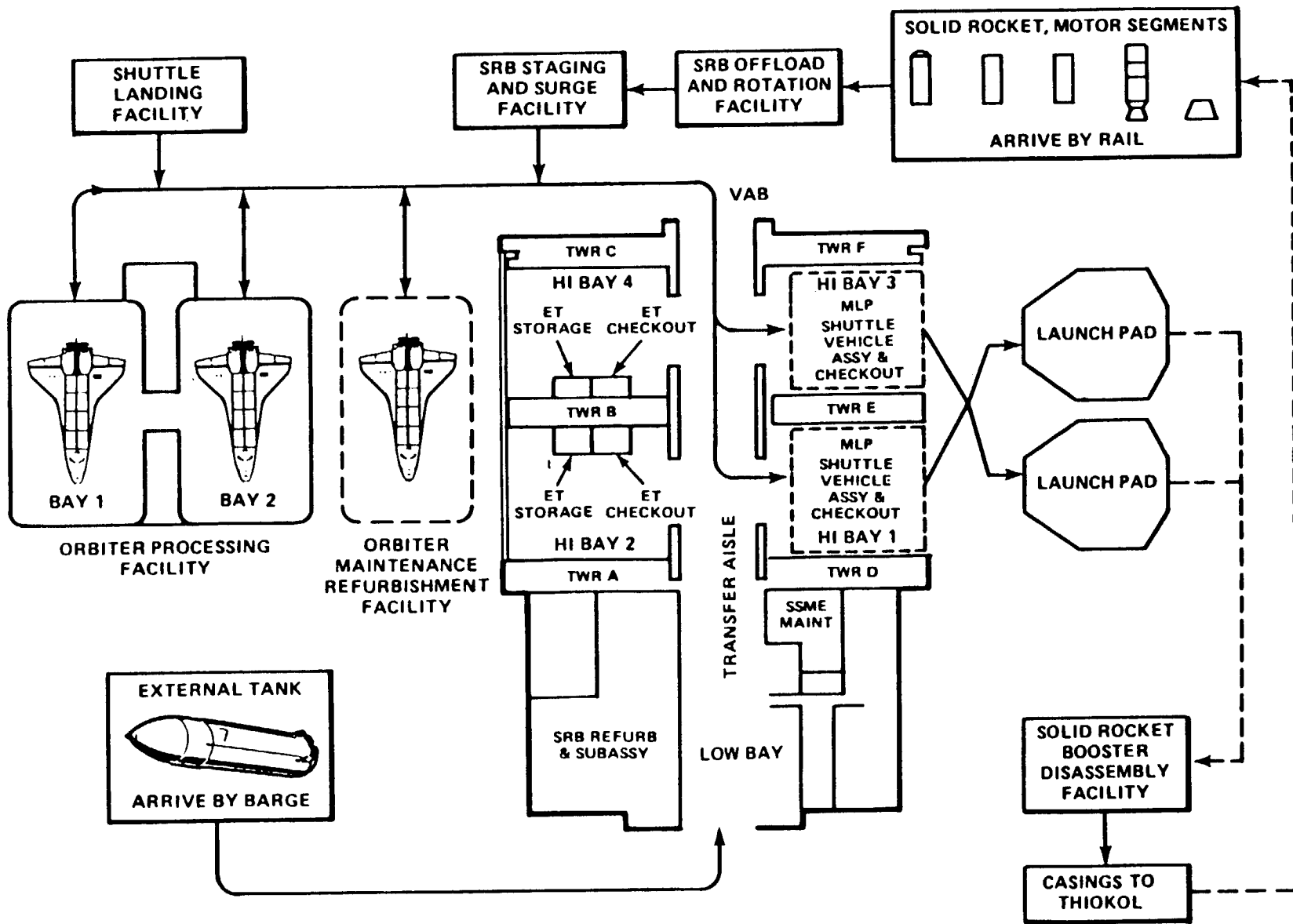
Shuttle Ground Processing Flow Diagram
