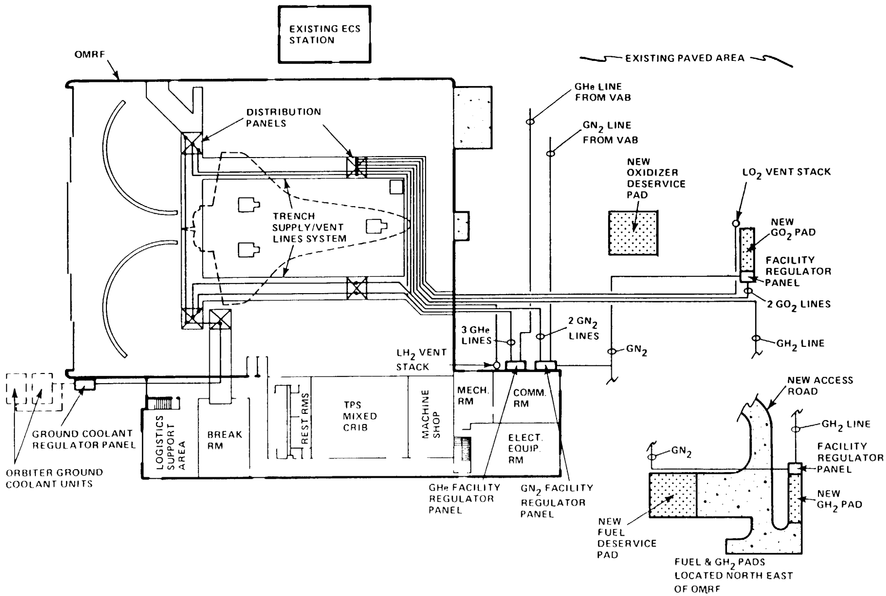
Orbiter Modification and Refurbishment Facility Floor Plan
