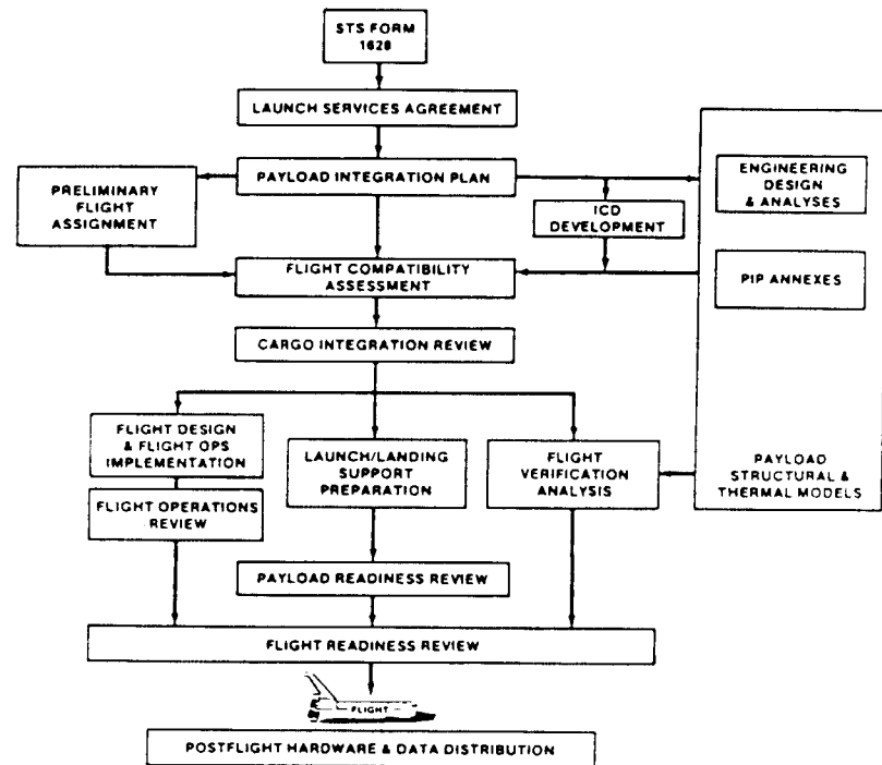
Cargo Integration Process
