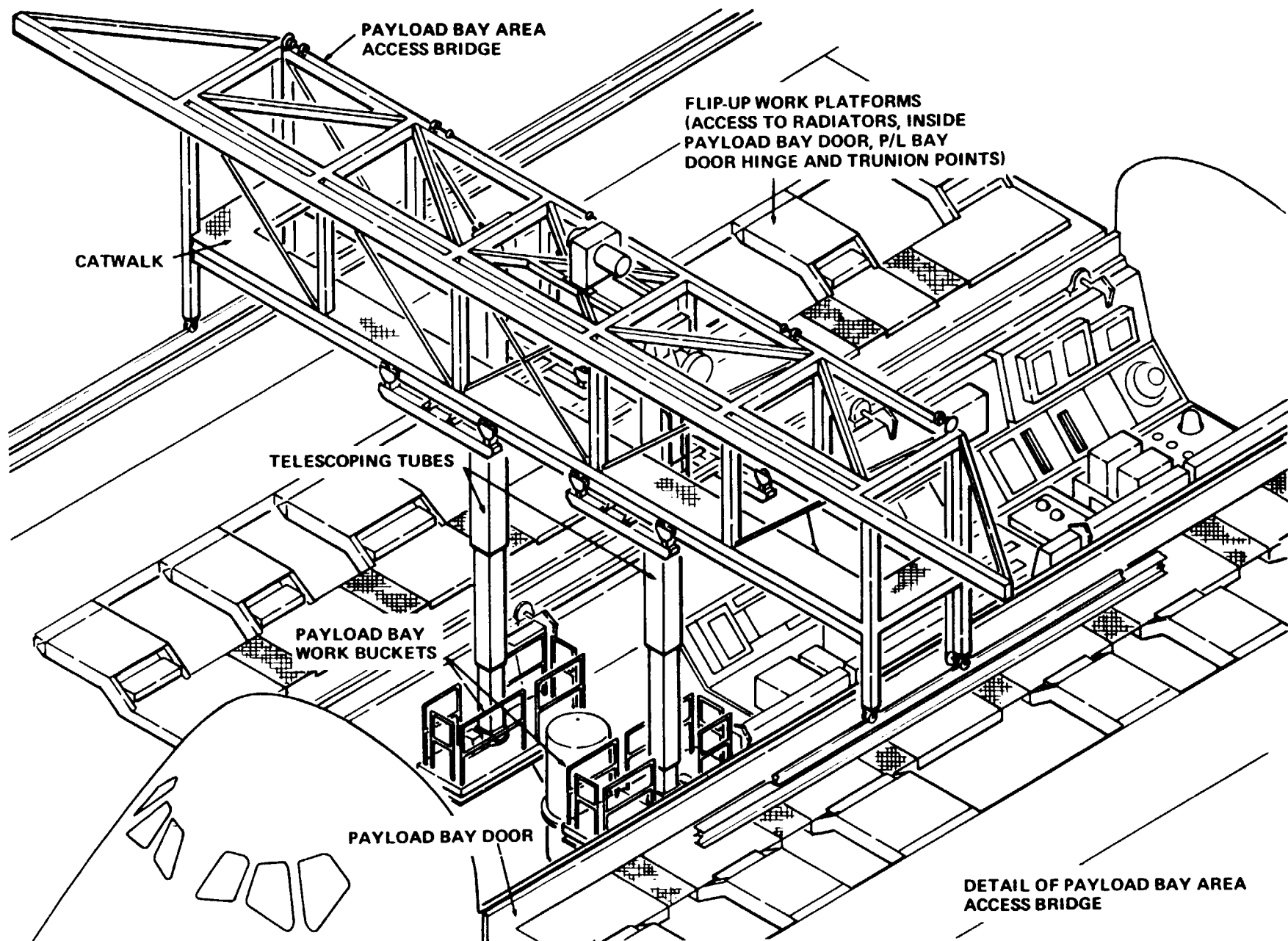
Orbiter Processing Facility Overhead Access Platforms
