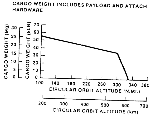
Cargo capability (28.45 degree inclination)
