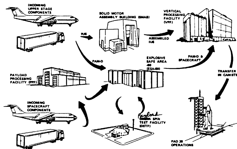
Vertical Payload Processing Flow
