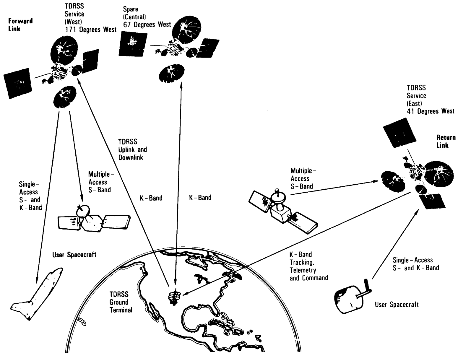
Linking Three Identical and Interchangeable Satellites with the TDRSS Earth Station at White Sands, New Mexico
