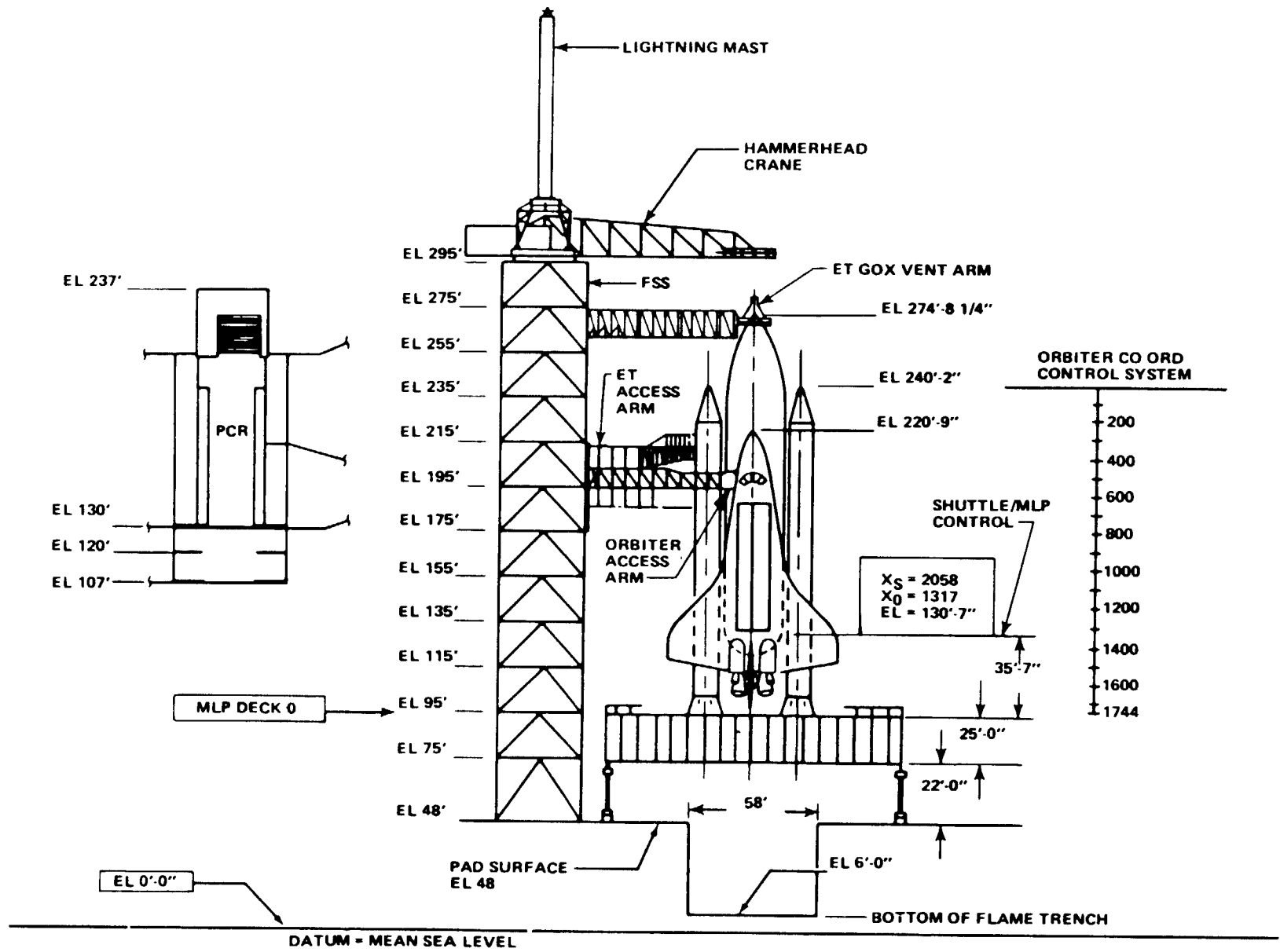
Launch Pad Elevations
