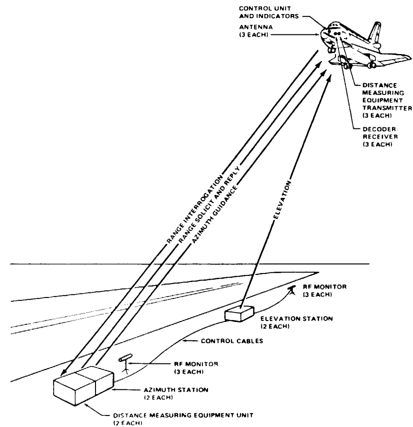
Microwave Scanning Beam Landing System
