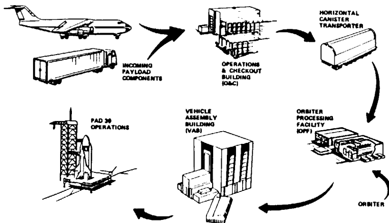
Horizontal Payload Processing Flow
