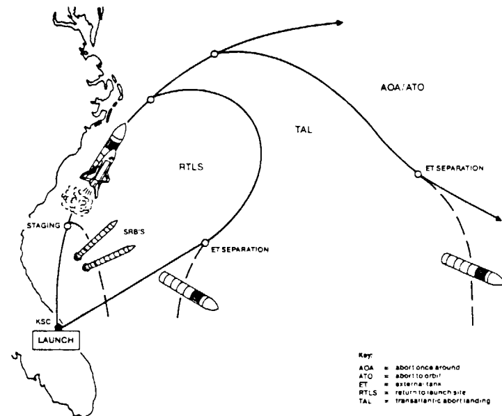
Space Shuttle Ascent Abort Modes
