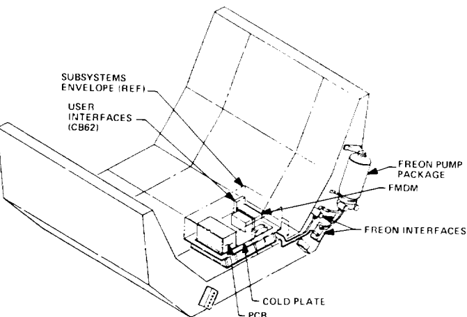
MDM Pallet Subsystem Equipment Arrangement
