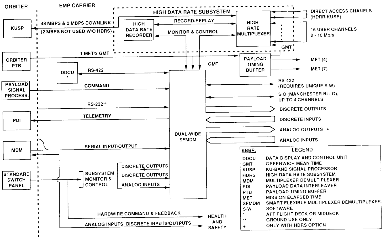
Command and Data Management System Block Diagram for the Enhanced MDM Pallet
