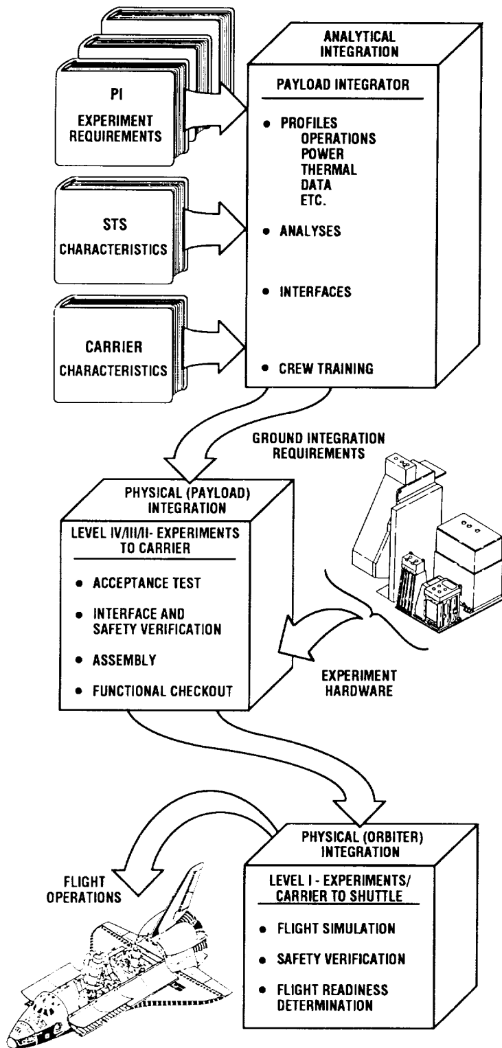
Payload Integration Flow
