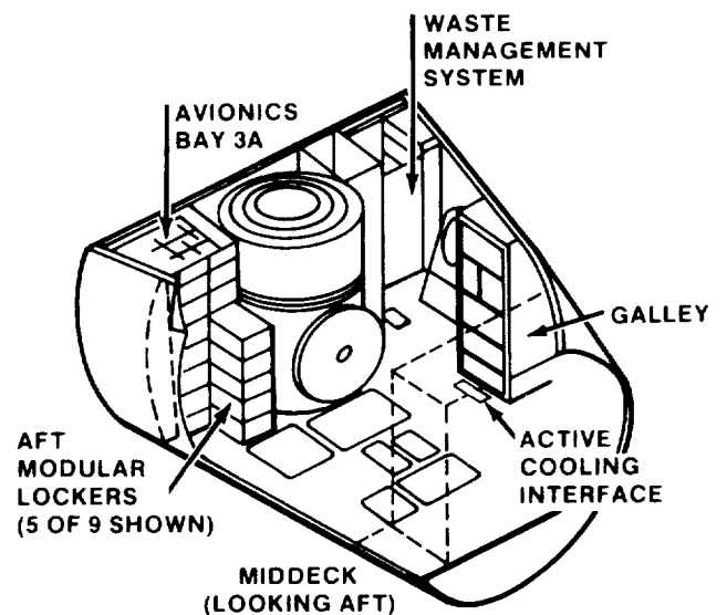
Layout of the Orbiter Middeck
