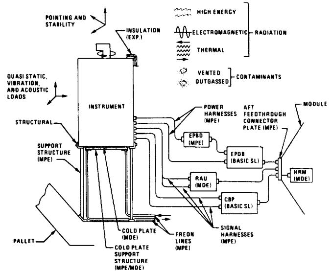
Typical Pallet-Mounted Instrument Interfaces
