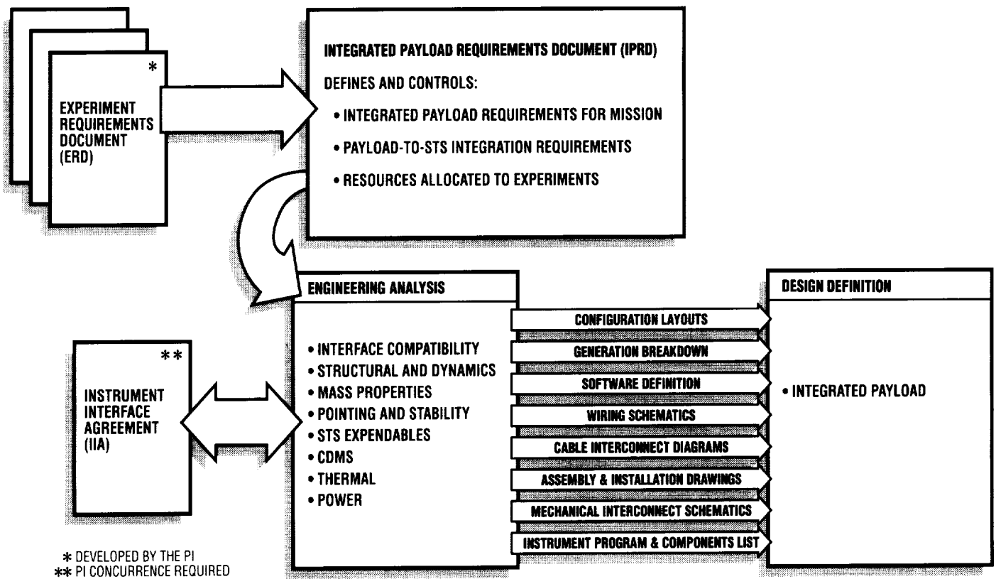
Integrated Payload Mission System Design
