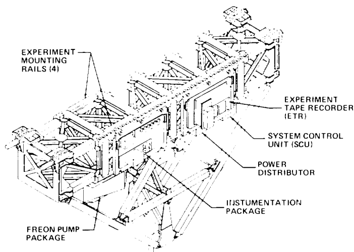
MPESS-A configuration showing component mounting (MPESS-B uses the same subsystems but includes a second MPESS.)
