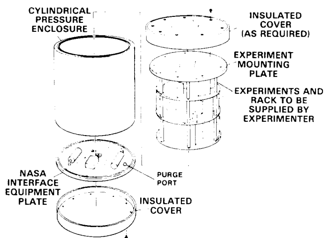
Get Away Special Container Concept
