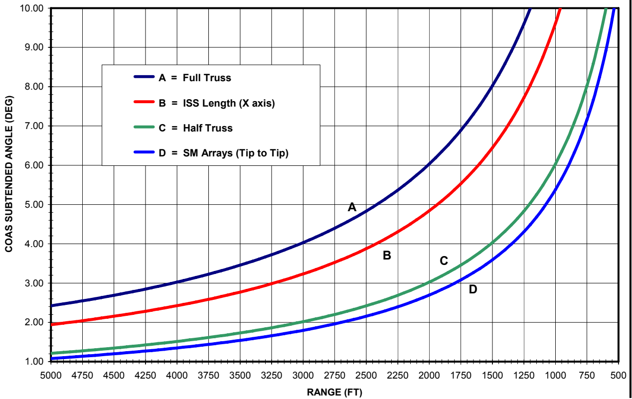
COAS SUBTENDED ANGLE VS RANGE
