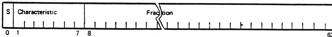
Figure 8-1. Floating Point Operands in Registers
