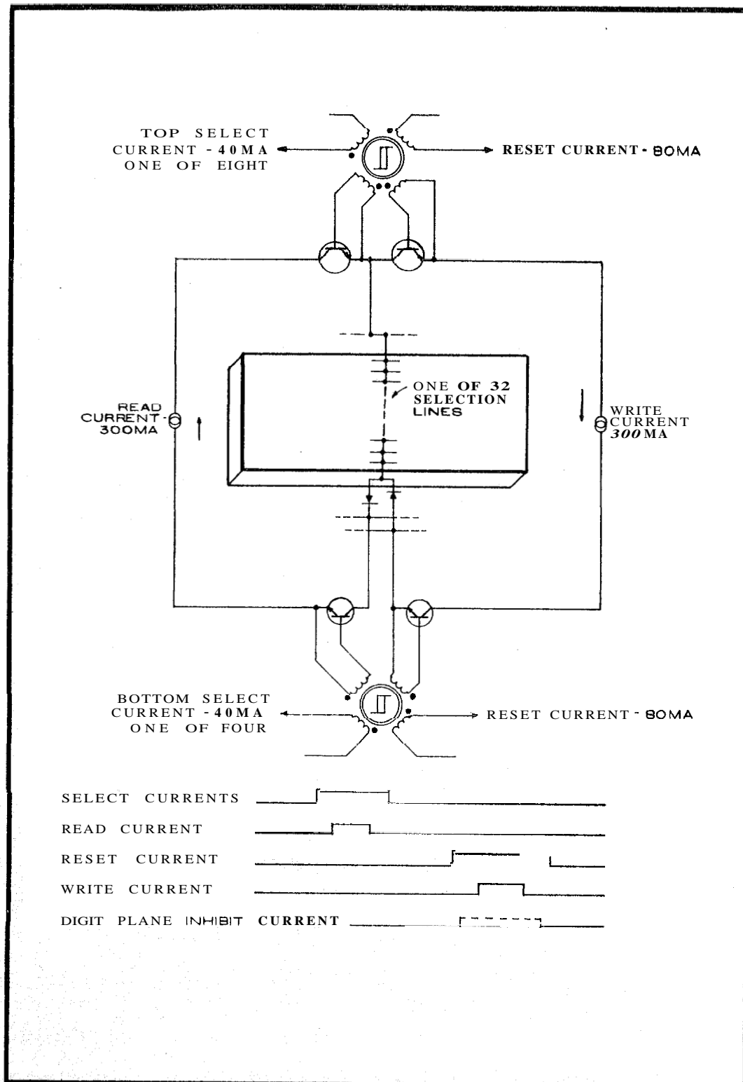
Fig. 4 Erasable memory current switching.
