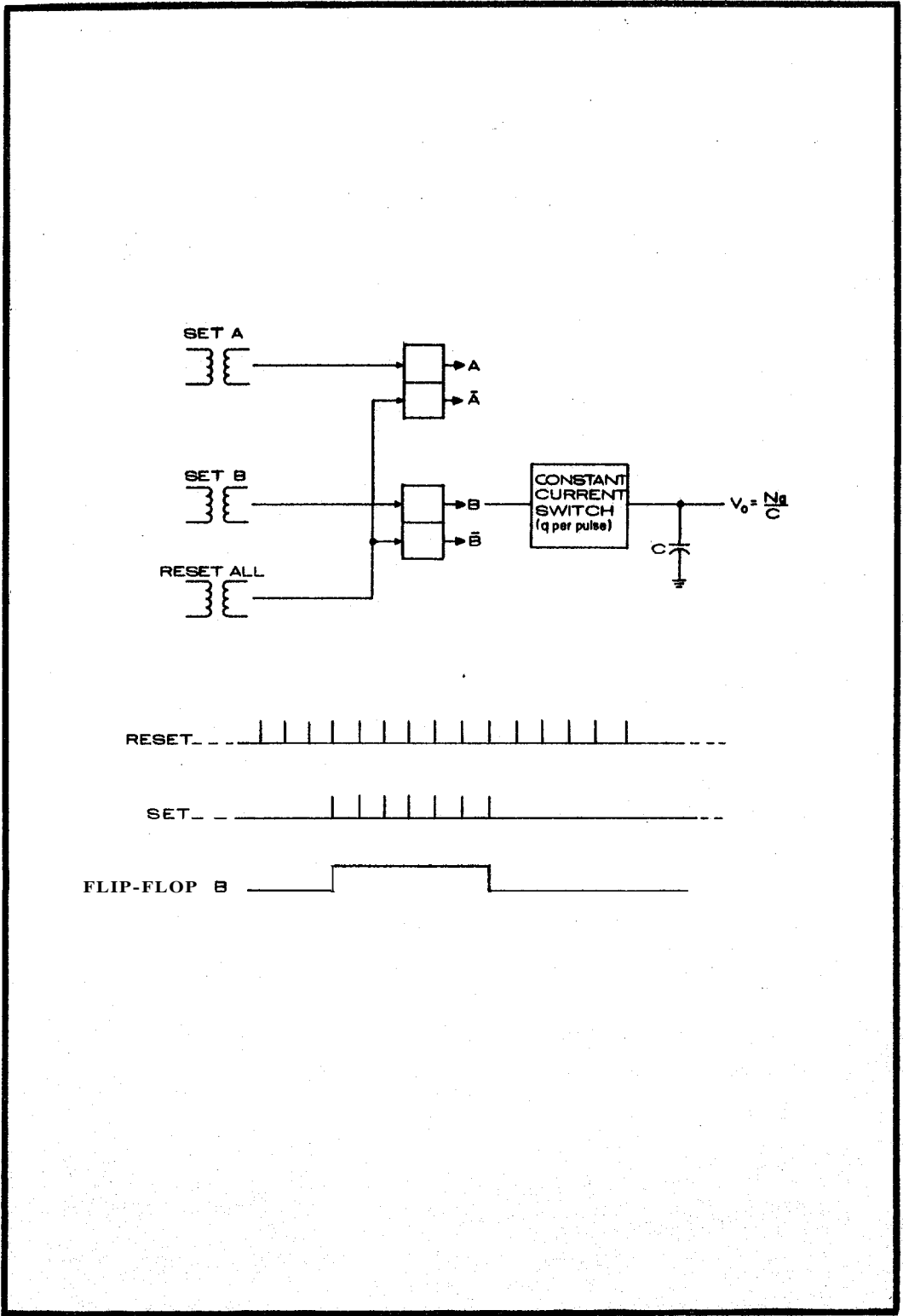
Fig. 9 Example of pulsetrain to duration to voltage conversion.
