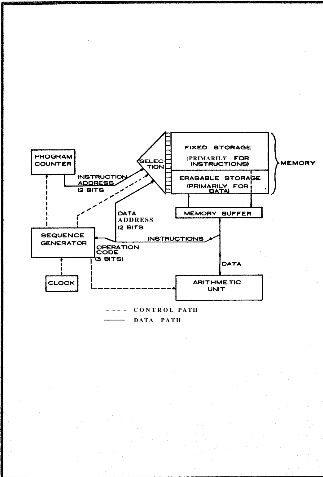
Fig. 1 Simplified block diagram of the AGC,
