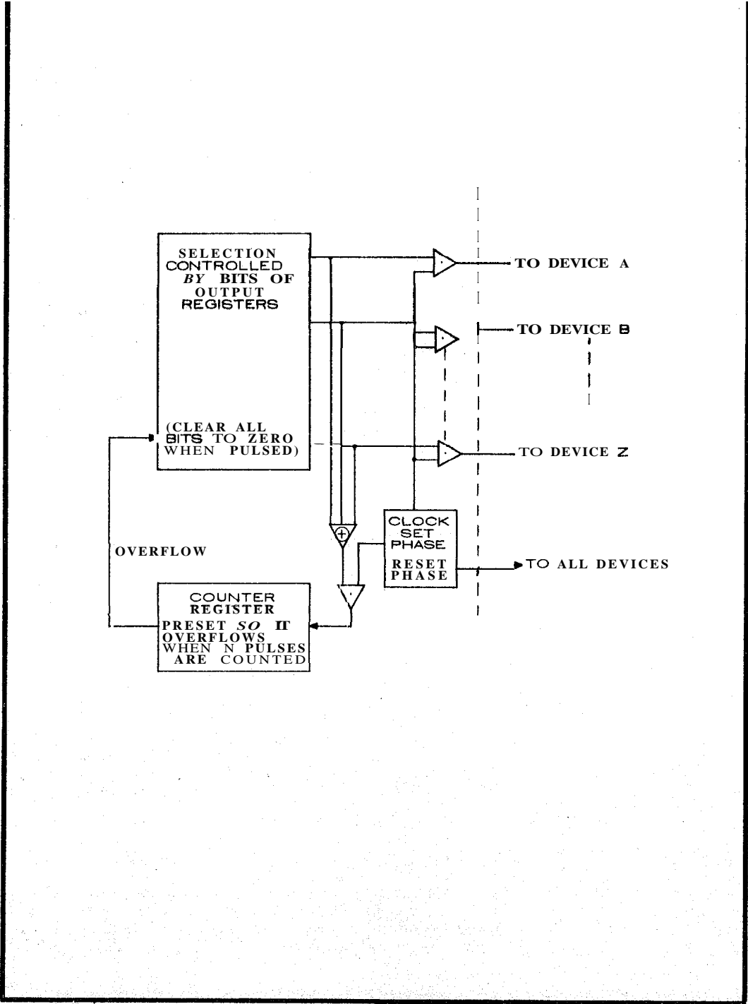
Fig. 8 Method for sending bursts of N pulses to a selected device.
