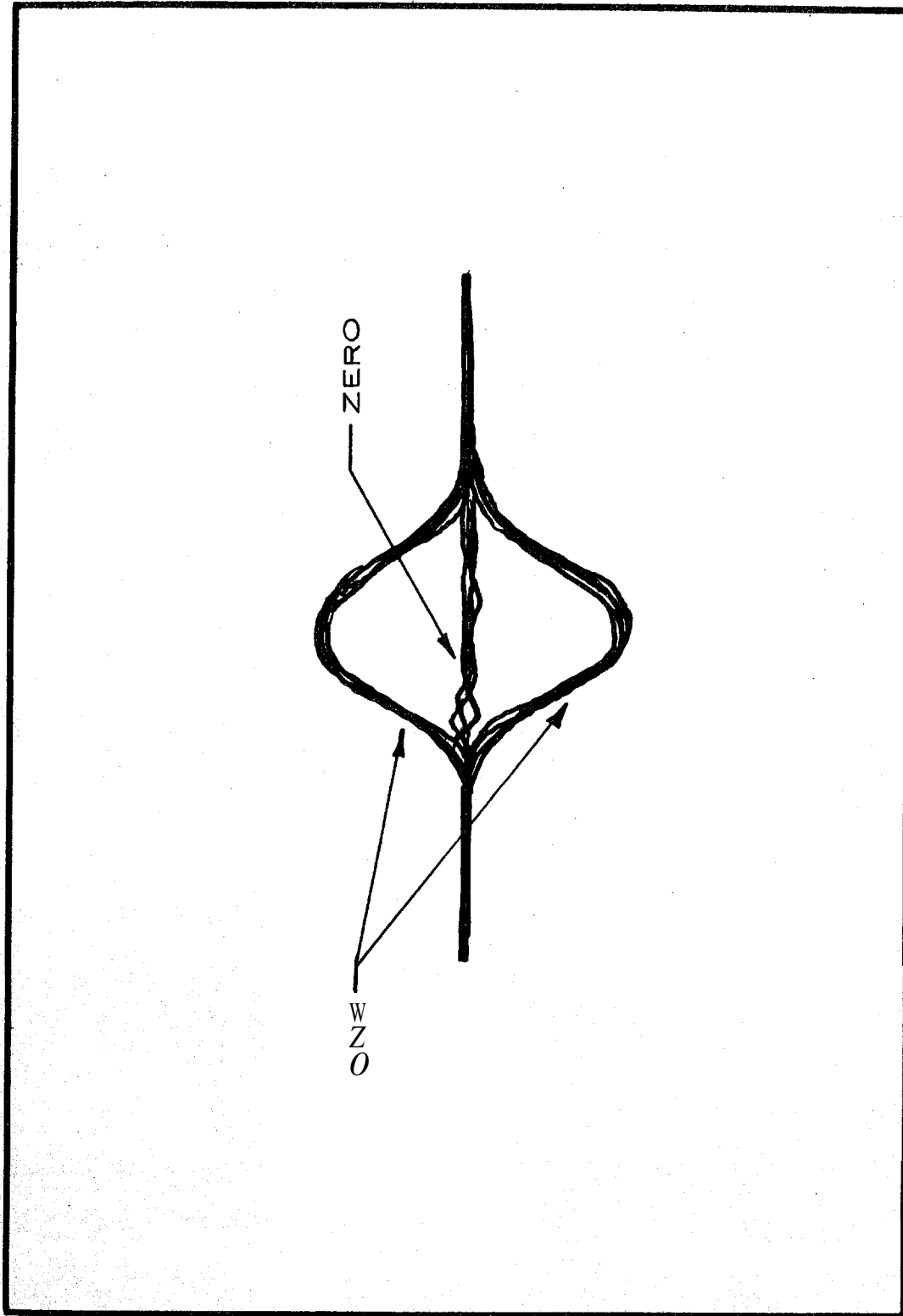
Fig. 6 Sequential output envelope of a 256 core rope memory.
