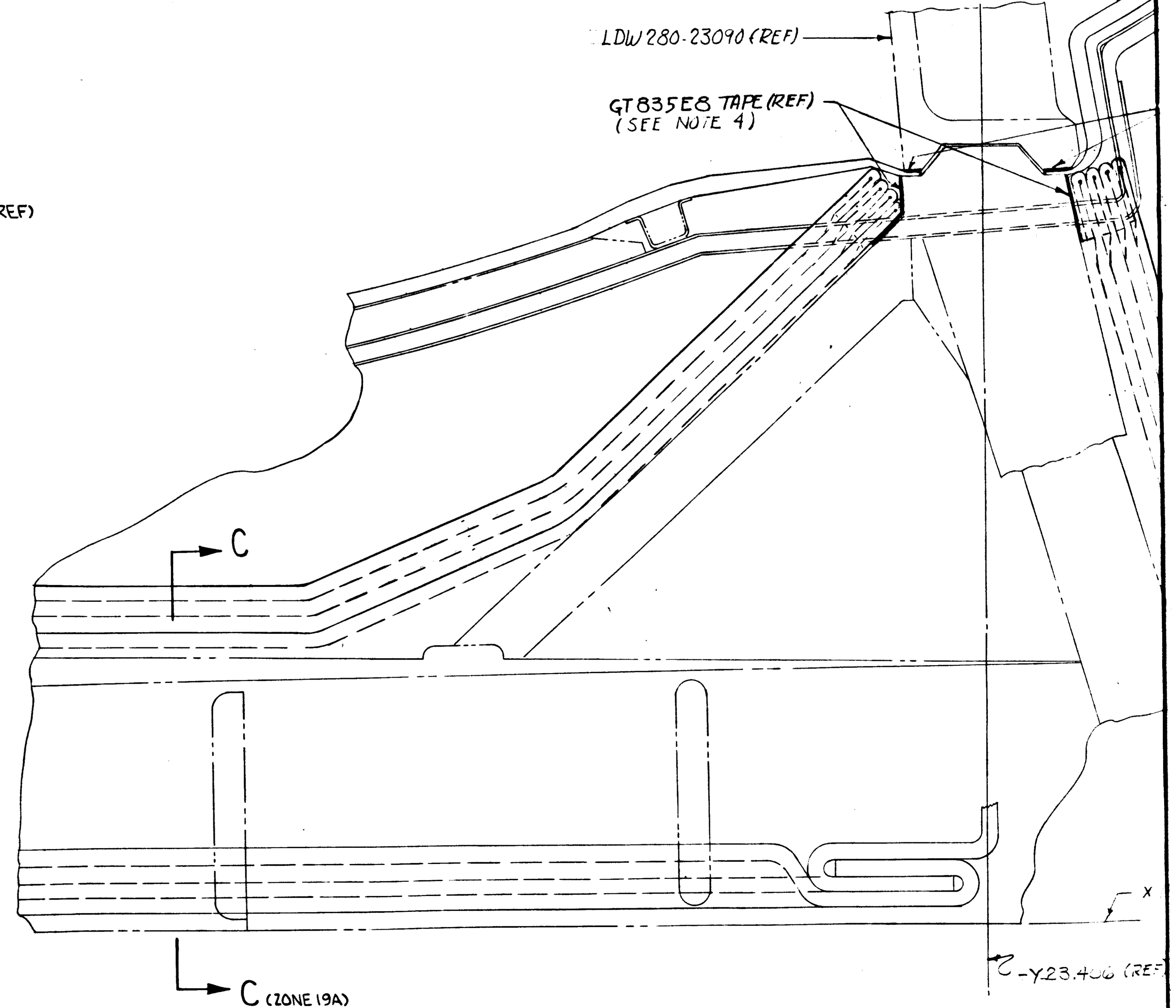
VIEW E (ZONE 7A SH4) VIEW LOOKING AFT
