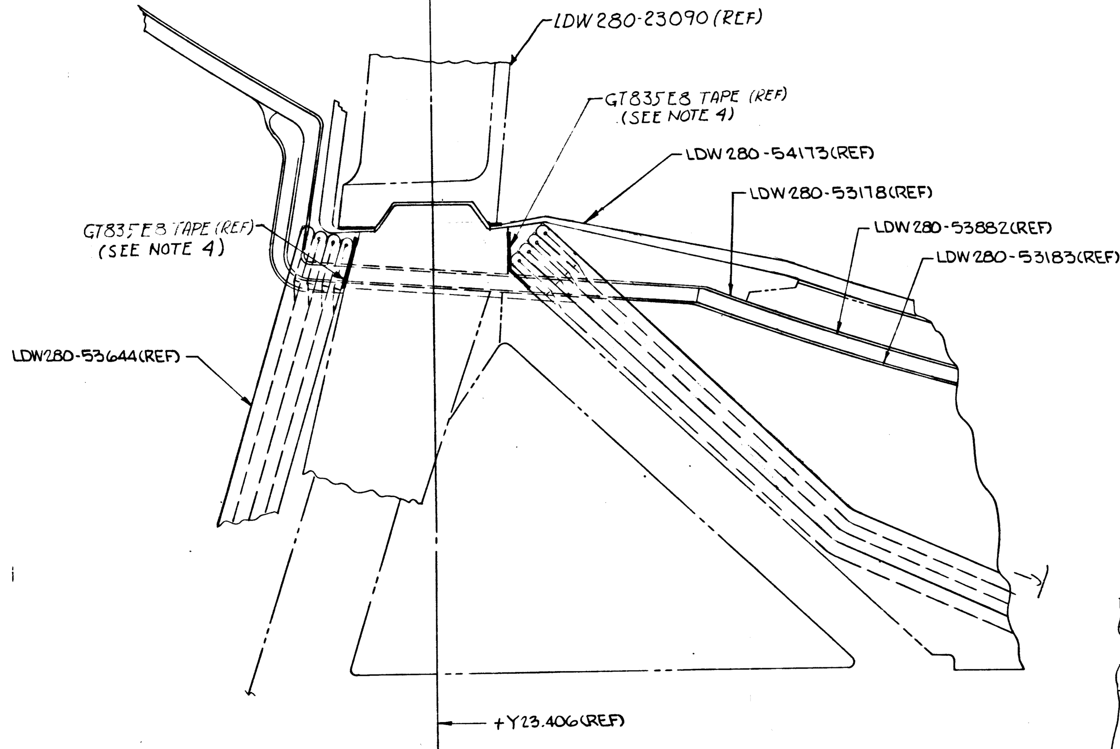
VIEW F (ZONE 8A SH4) VIEW LOOKING AFT
