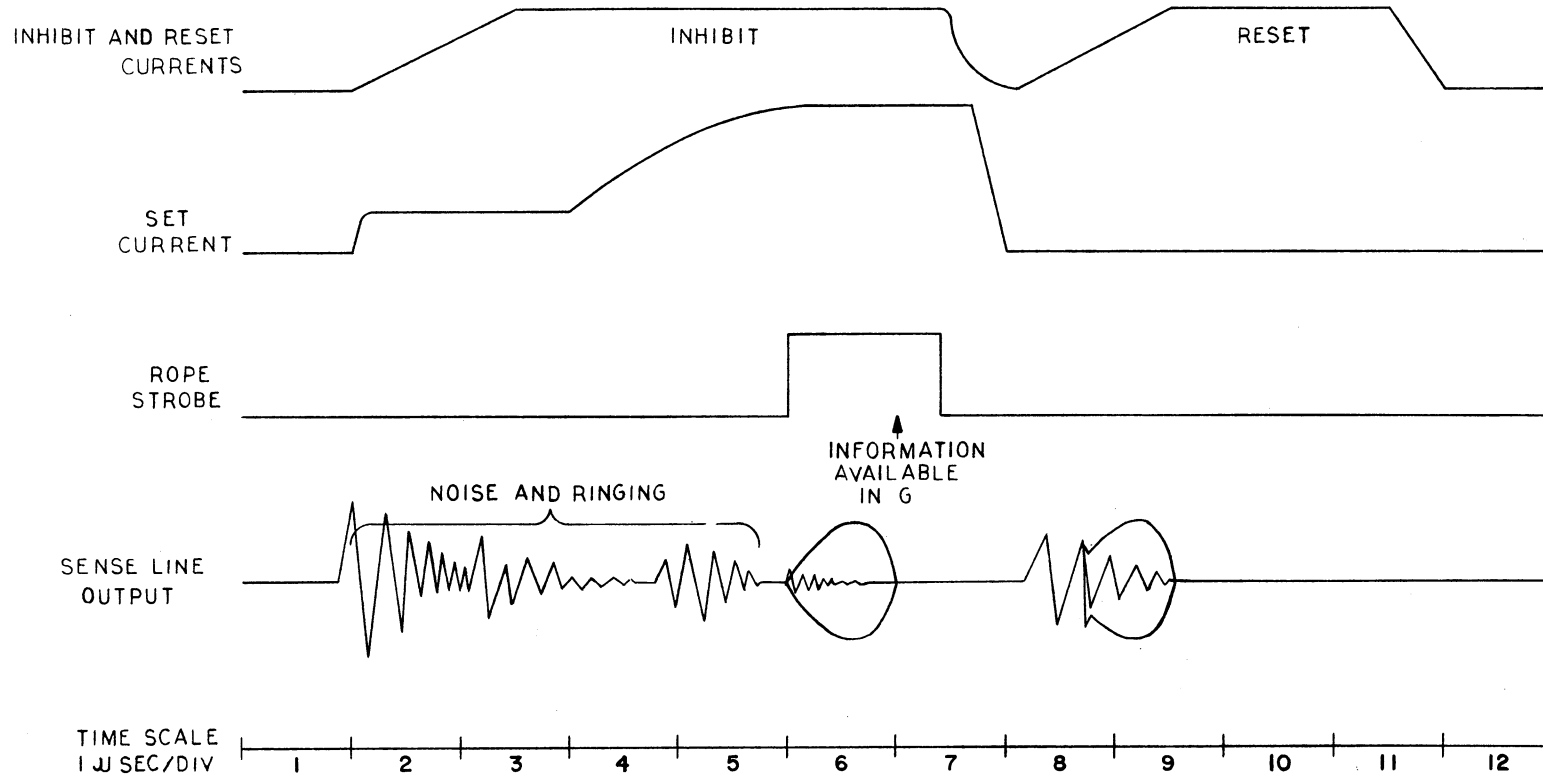
Figure 4-4. Fixed Memory Timing.
