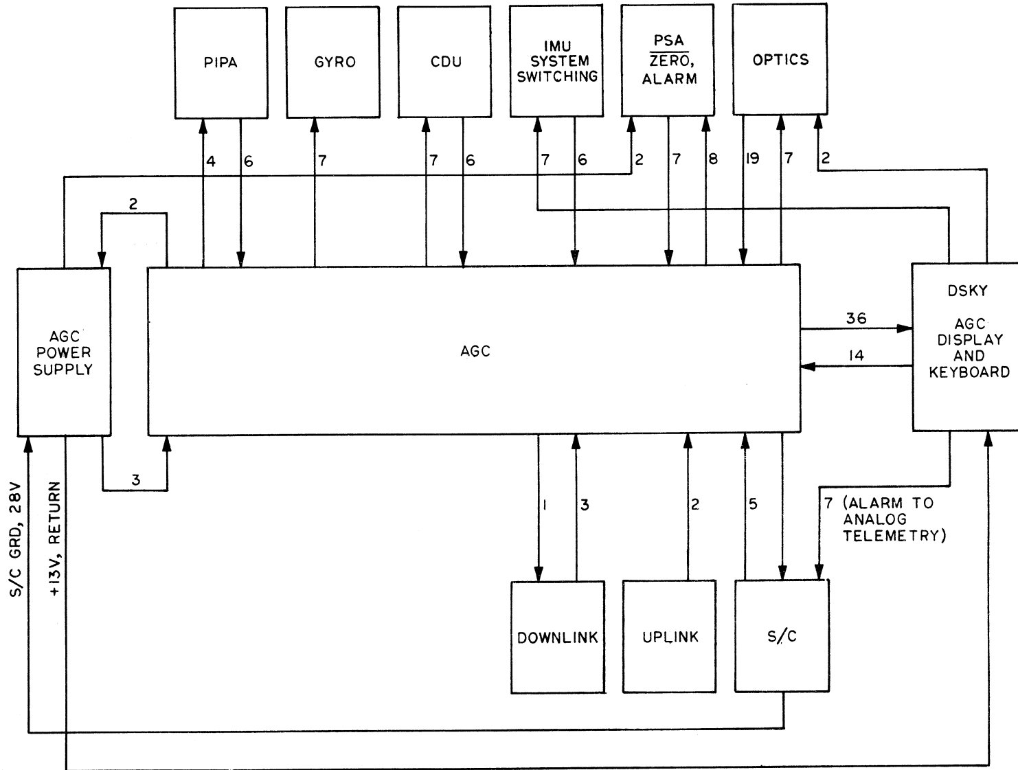
Figure 5-1. In-Out Functional Breakdown.
