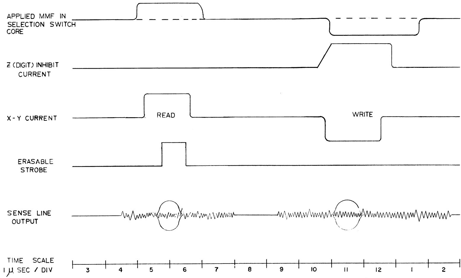
Figure 4-5. Erasable Memory Timing.
