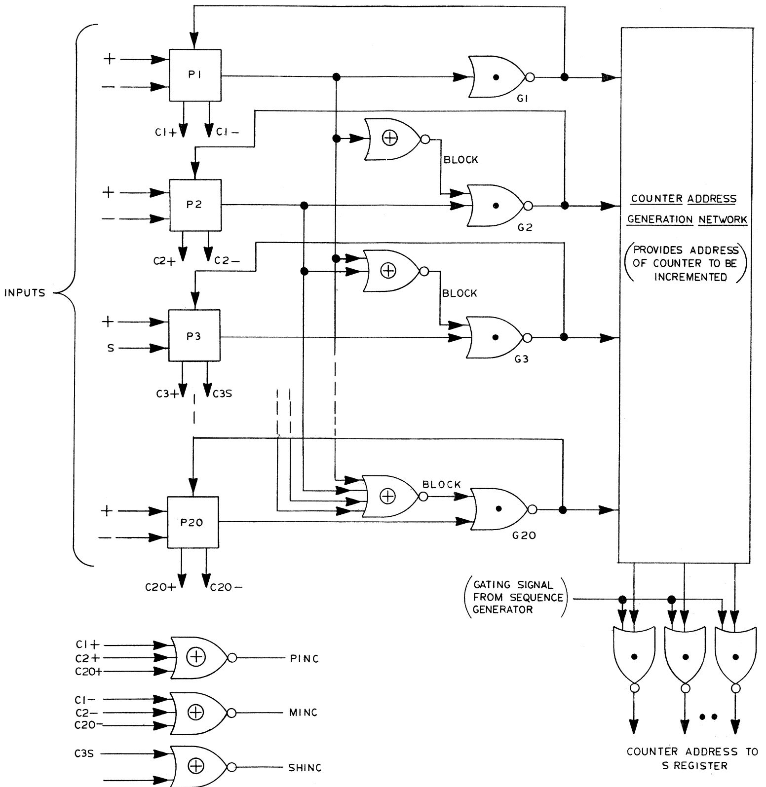
Figure 2-5. Priority System for Counters.
