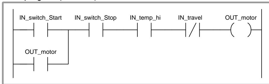
PLC program (live view)
