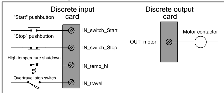
Real-world I/O wiring
