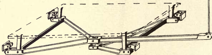
Fig. 267 Lever system of weighbridge
