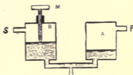
Diagrammatic Section of Manometer.
