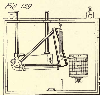
Recording Steam Meter without Pressure Compensator
