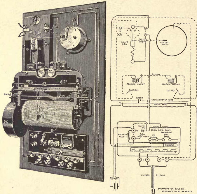
Fig 343.—Callendar Recorder
