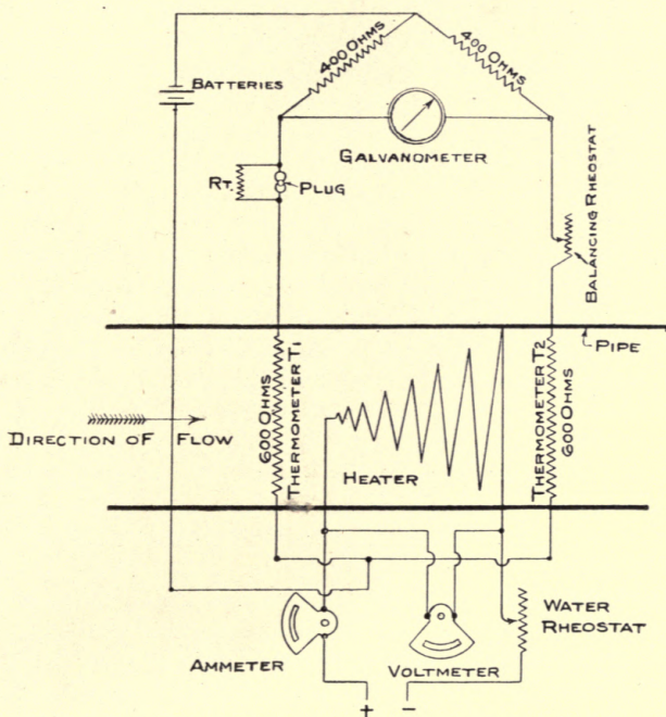
DIAGRAM OF ELECTRIC METER CONNECTIONS.
