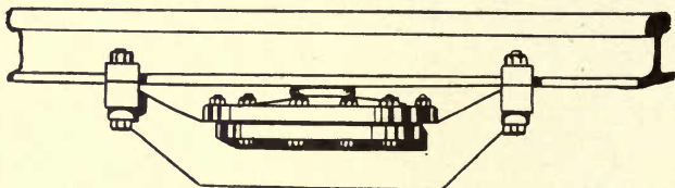
Fig 209—Contact box on rail
