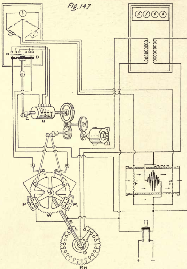
Diagrammatic sketch of automatic electric meter.
