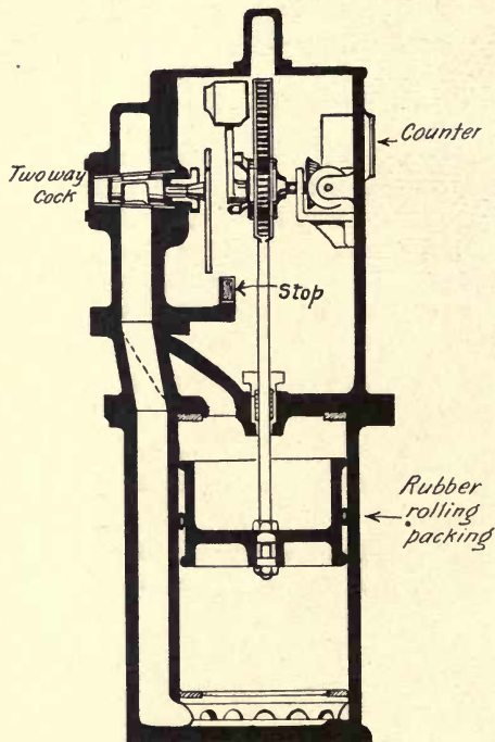
Fig. 75. Section of Cold Water Meter
