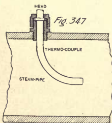
Application of Thermocouple to Steam main
