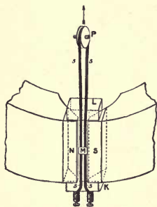
Fig. 233—Principle of oscillograph
