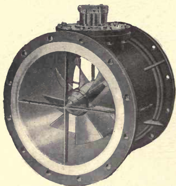
Fig. 91 Helix Meter.
