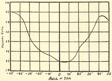
Fig. 217—Effect of yaw on Venturi
