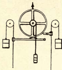
Fig 208—Recording mechanism
