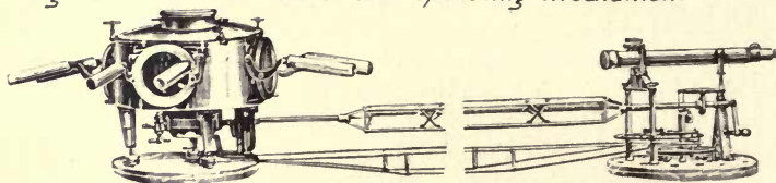
Fig. 236 Vacuum balance with operating mechanism
