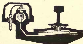
Fig 210—Section of contact box.
