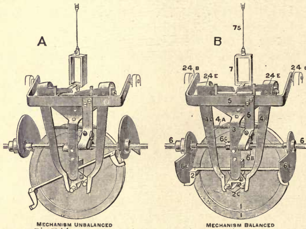
Fig. 344. — Mechanism of recording potentiometer
