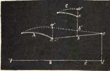
Fig. 324 - Mechanism of Richards Compensated thermograph
