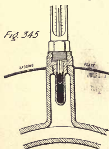
Incorrect method of mounting thermometer
