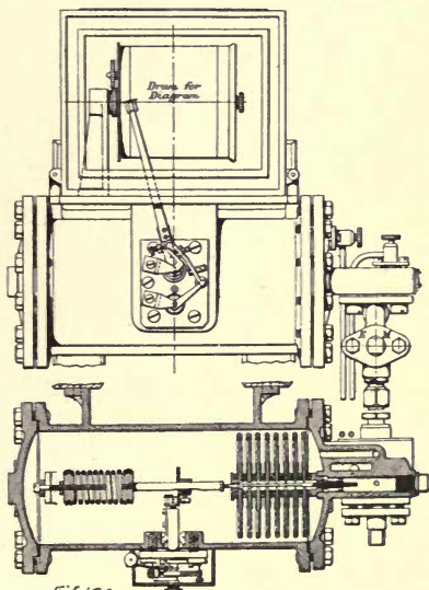
Fig. 129 Recorder non-compensated type
