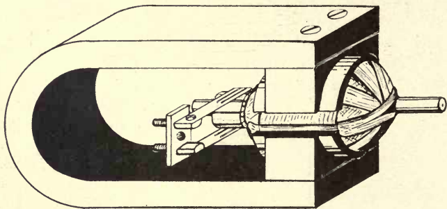
Fig. 185.—Generator of electrical tachometer
