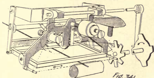
Fig. 341 Recording mechanism, with cam-actuated tapping and rocking frames. The dotted lines show path of ribbon.
