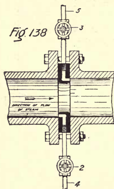
Throttle Disc in position.
