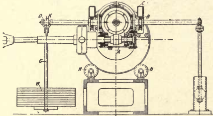
Fig. 316 Section of worm gear testing cradle.
