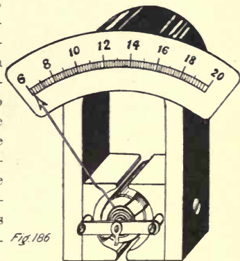
Indicator of electrical tachometer
