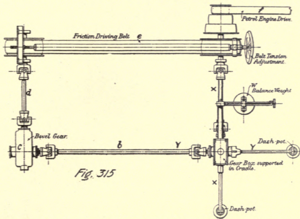
THE DAIMLER-LANCHESTER WORM GEAR TESTING MACHINE
