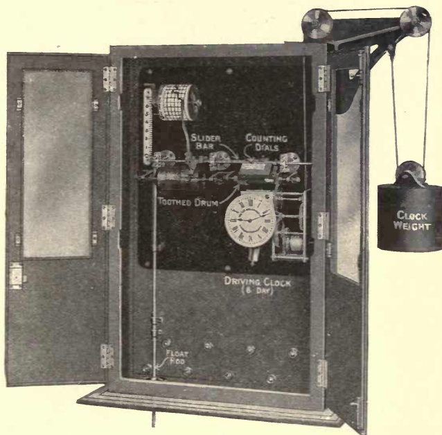
Fig. 98. COMBINED RECORDER AND INTEGRATOR
