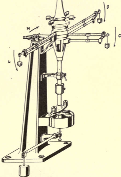
Fig. 255 Balance for measurement of forces on aircraft models
