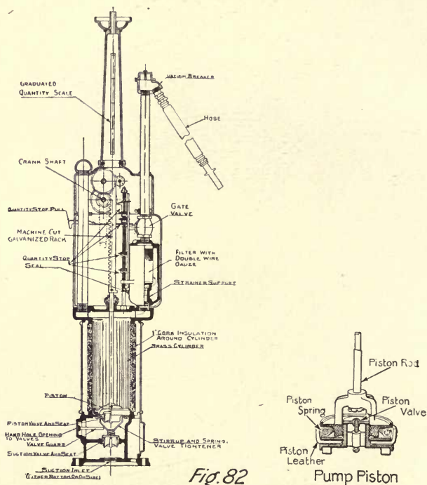
Sectional elevation of typical piston-type measuring pump
