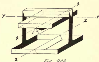
Fig. 248 Diagrammatic sketch of compensated pan suspension
