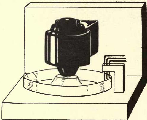
Fig. 229 - Spark chronograph
