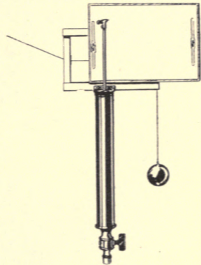
Fig. 281 Watt's Indicator
