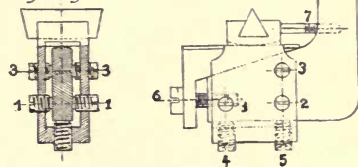
Methods of attachment of end knife edges to the beam
