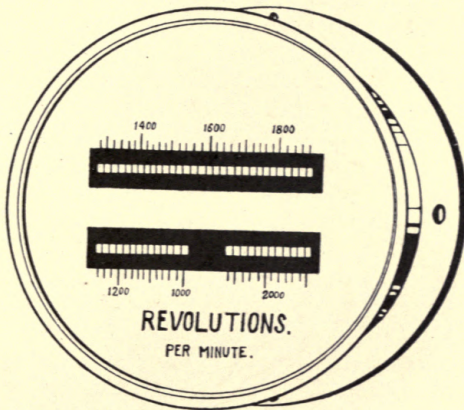
Fig. 197 - Resonance tachometer
