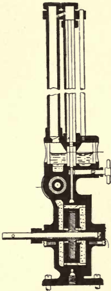
Fig. 180.—Section of Centrifugal pump tachometer
