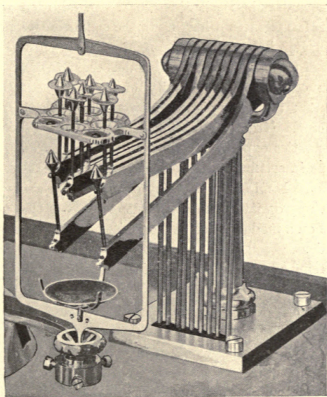
Fig. 254. —Detail of the multiple weight attachment.
