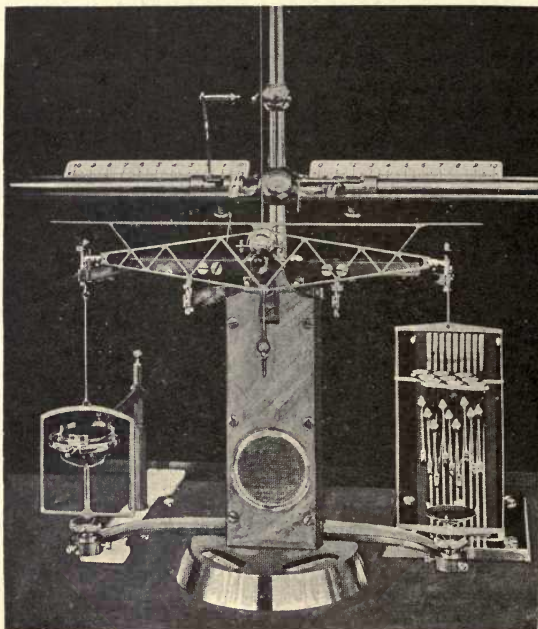
Fig. 253.—The Heusser Balance.
