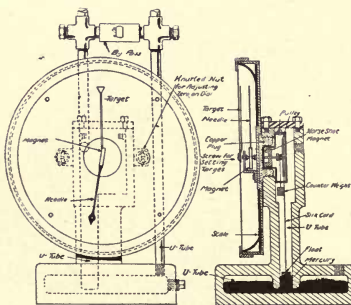
Fig. 135 Diagrammatic sketch of movement
