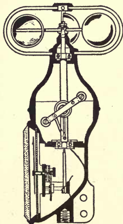
Fig. 222—Air speed indicator
