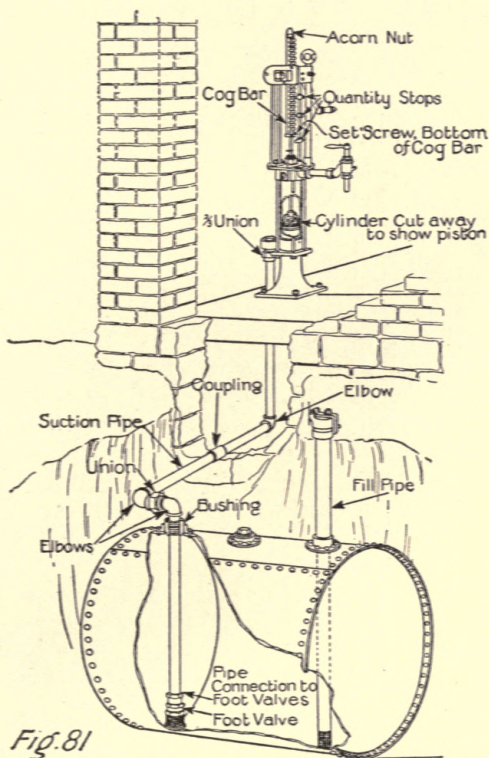
Typical piston-type measuring pump installation, showing arrangement of tank, piping, valves, etc.
