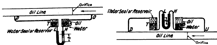
Fig. 130—DIAGRAM OF ORIFICE METER INSTALLATION FOR MEASURING HEAVY OIL
