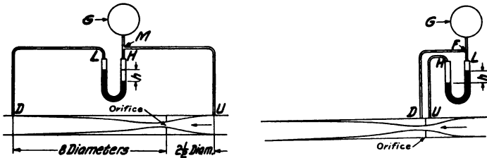
Fig. 90—FULL FLOW CONNECTIONS Fig. 91—FLANGE CONNECTIONS SKETCHES OF ORIFICE METER INSTALLATIONS. CURVED LINES ARE LINES OF STREAM FLOW
