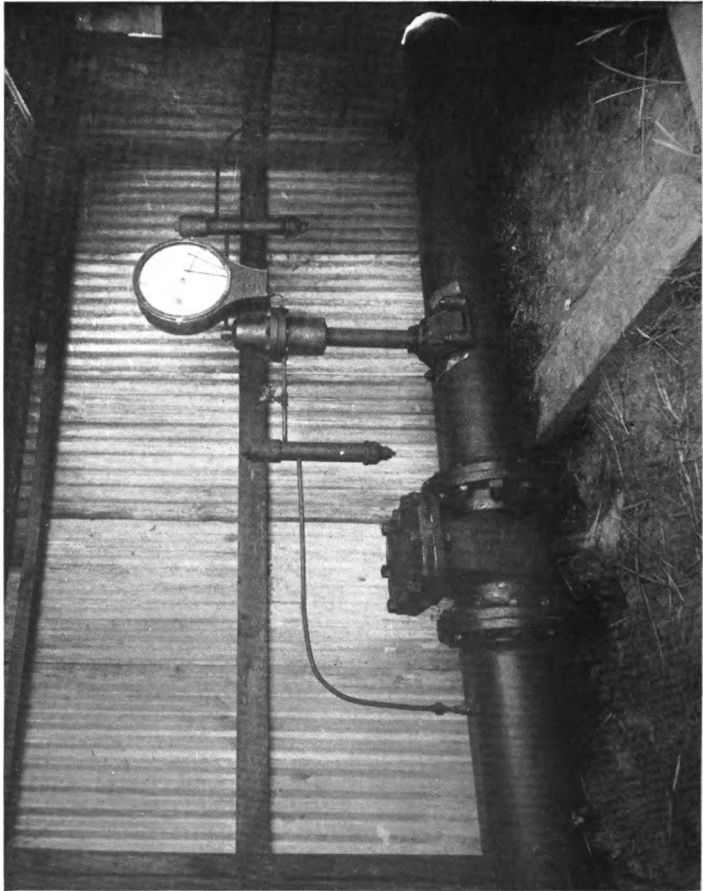
Fig. 96—ONE OF THE FIRST INSTALLATIONS OF ORIFICE METER BODY AND 50 INCH DIFFERENTIAL GAUGE \frac{3}{4} and 8 Diameter Connections
