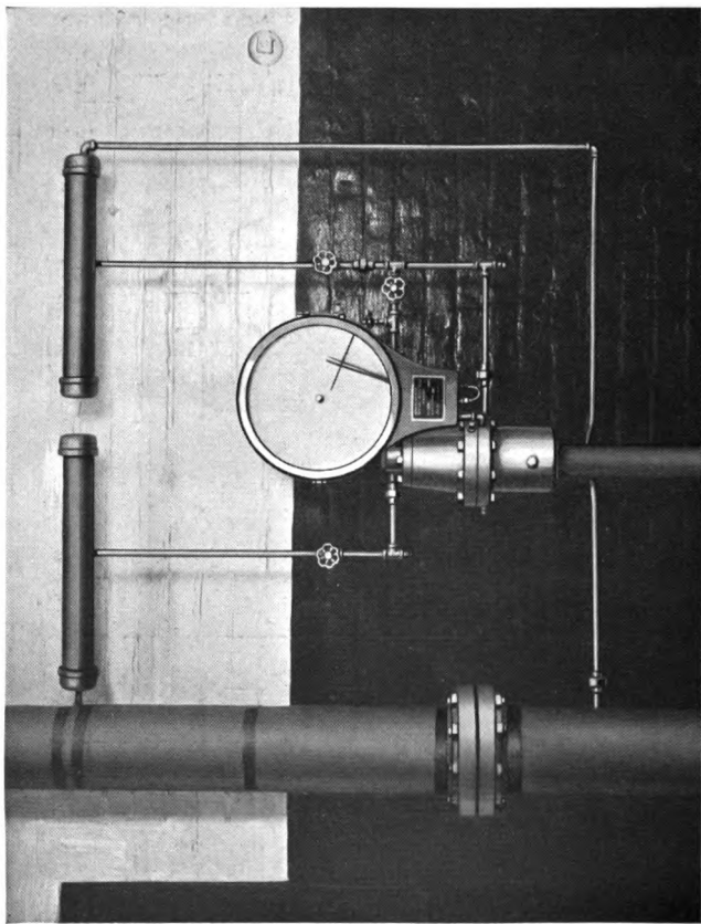
Fig. 117—MEASURING STEAM WITH A 60 INCH DIFFERENTIAL PRESSURE GAUGE
