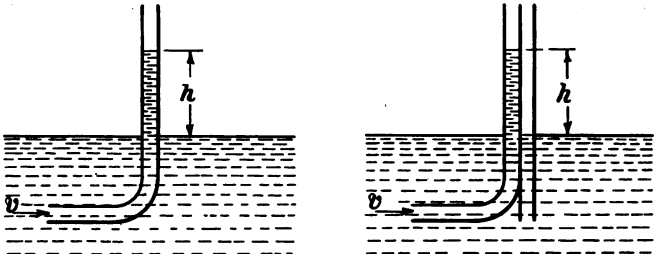
Fig. 1—PITOT TUBE USED IN MEASURING FLOWING STREAMS
