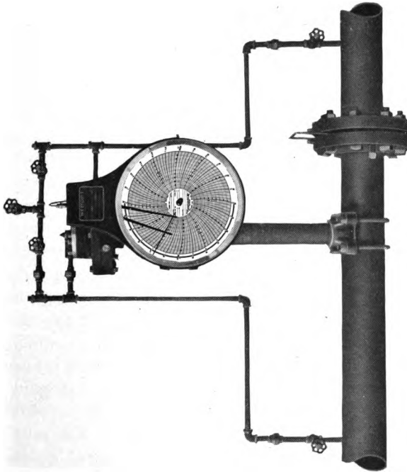
Fig. 56—80 INCH DIFFERENTIAL GAUGE INSTALLATION
