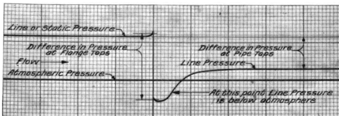
Fig. 59—SKETCH SHOWING STREAM FLOW THROUGH AN ORIFICE AND THE RELATIVE STATIC PRESSURES AT VARIOUS POINTS LONGITUDINAL SCALES ARE THE SAME
