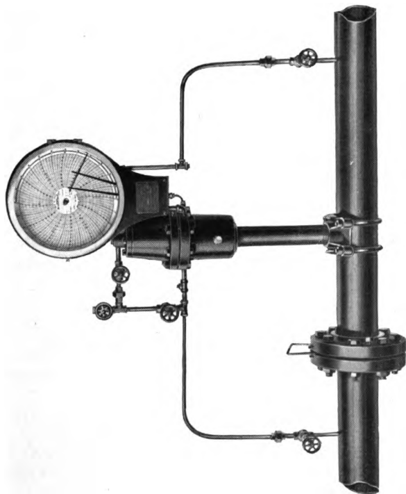
Fig. 61—ORIFICE FLANGES AND 60 INCH DIFFERENTIAL GAUGE INSTALLATION
