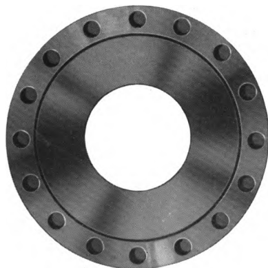
Fig. 41—ONE TYPE OF THIN PLATE ORIFICE USED IN ORIFICE BODY, Fig. 42
