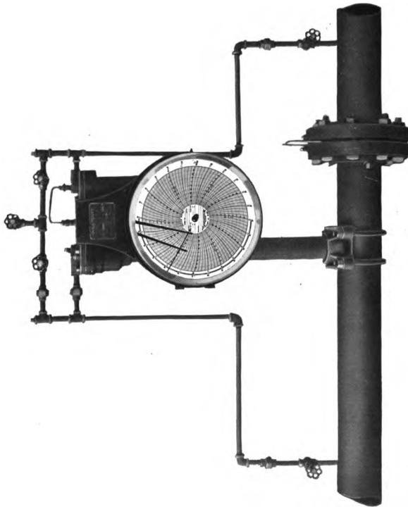
Fig. 65—50 OR 100 INCH DIFFERENTIAL GAUGE INSTALLATION
