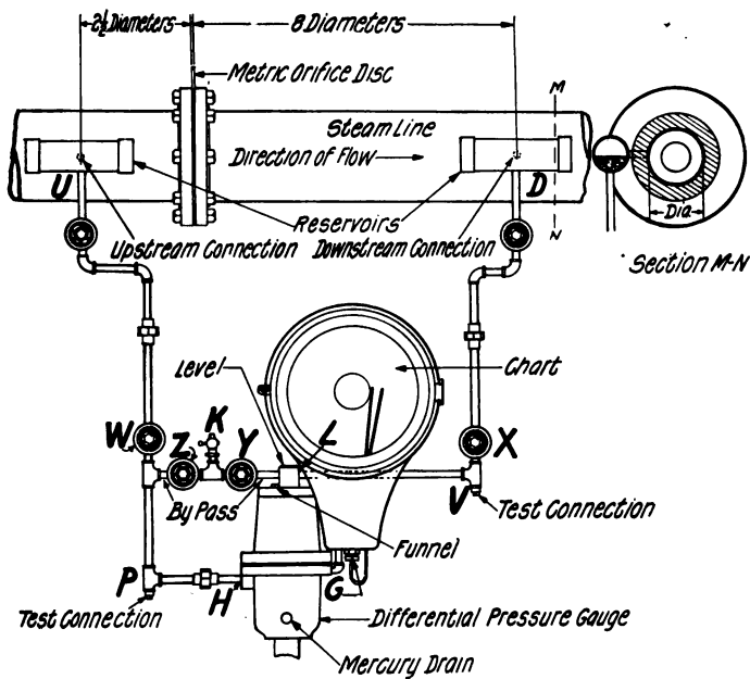
Fig. 123—50 INCH GAUGE INSTALLATION FOR MEASURING STEAM
