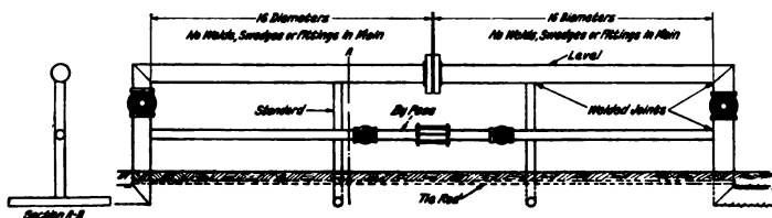
Fig. 95—AN INSTALLATION USED IN THE OSAGE INDIAN RESERVATION. SEE PAGE 164
