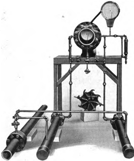
Fig. 8—"BOMBHELL" TYPE DIFFERENTIAL GAUGE. COVER REMOVED. NOTE LARGE PIPE DEADENERS IN GAUGE LINES
