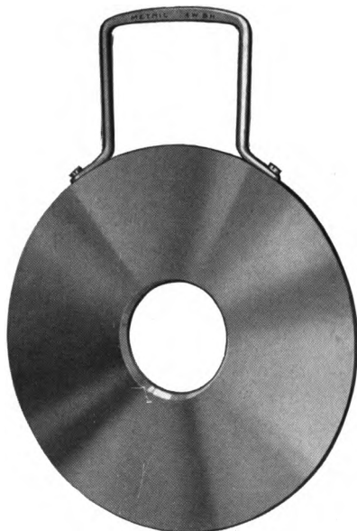
Fig. 40—THIN ORIFICE USED IN ORIFICE FLANGE
