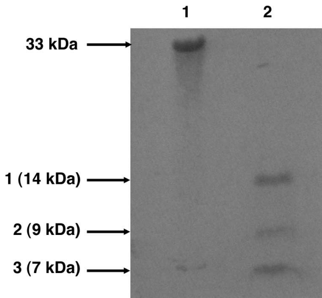
FIG. 3. SDS gel electrophoretic analysis of keratinase and its CNBr-cleaved fragments. Lane 1, intact keratinase; lane 2, CNBr-cleaved keratinase fragments. The N-terminal amino acid sequences are as follows: 1, H 2 N-AQTVPYGIPLIKADKVVQAAQGFK...; 2, H 2 N-KQAVDNAYARGVVVAAAA...; 3, H 2 N-ASP...
